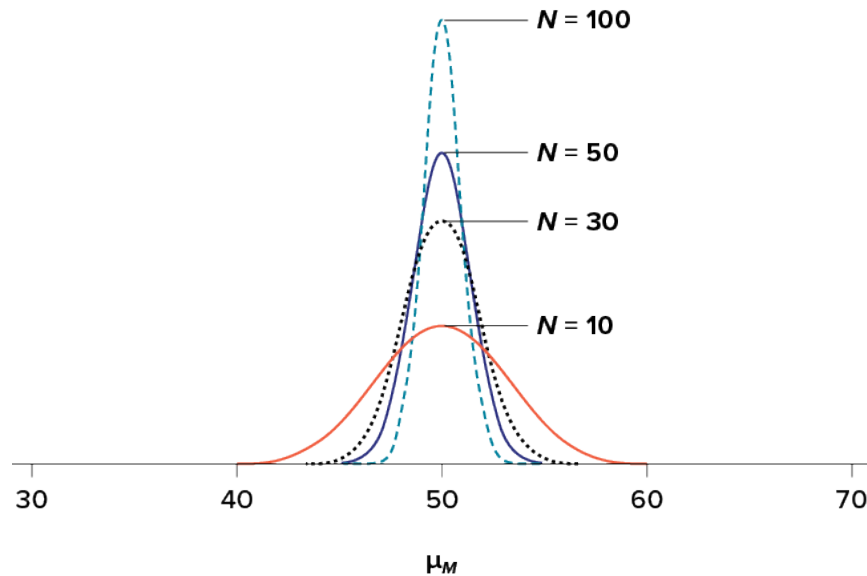
Figure 6.2. Sampling distributions from the same population with m = 50 and s = 10 but different sample sizes ( N = 10 , N = 30 , N = 50 , N = 100 ). ("Sampling Distributions with Different Sample Sizes" by Judy Schmitt is licensed under CC BY-NC-SA 4.0.)
