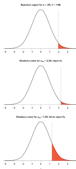
Figure 7.3. Relationship between \alpha , z_{\text{obt}} , and p . ("Relationship between alpha, z_{\text{obt}} , and p " by Judy Schmitt is licensed under CC BY-NC-SA 4.0.)
