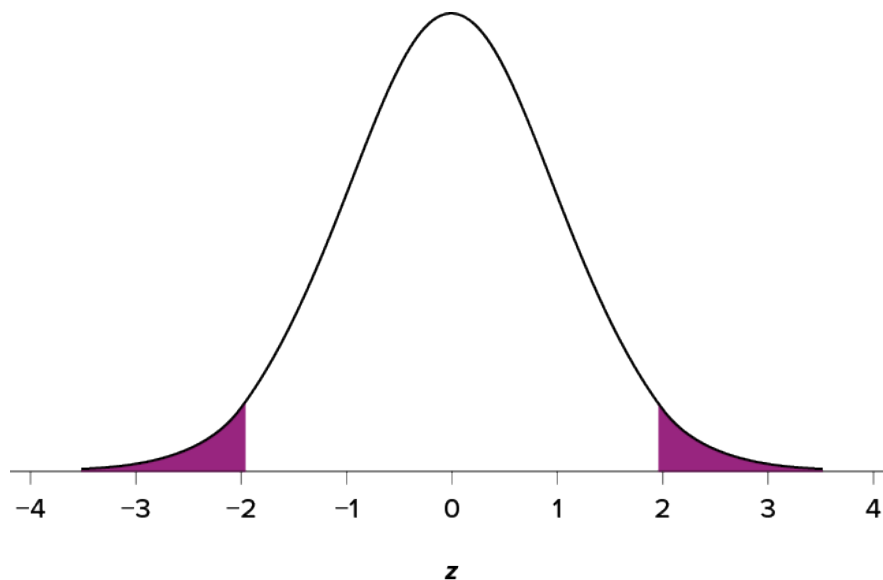
Figure 5.4. Area in the tails beyond z = -1.96 and z = 1.96 . (“Area in the Tails z \pm 1.96 ” by Judy Schmitt is licensed under CC BY-
