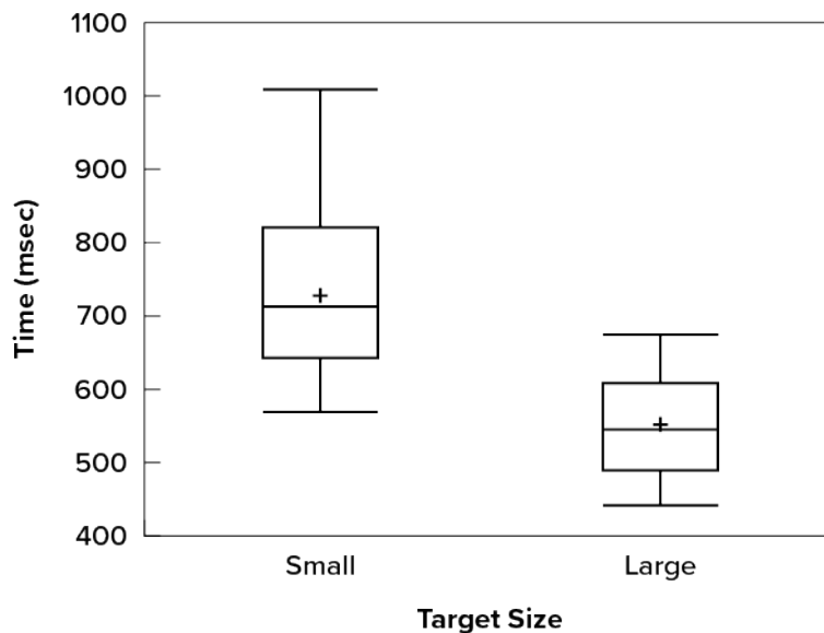
Figure 2.29. Box plots of times to move the cursor to the small and large targets. (“Cursor Task Box Plot” by Judy Schmitt is licensed under CC BY-NC-SA 4.0.)
