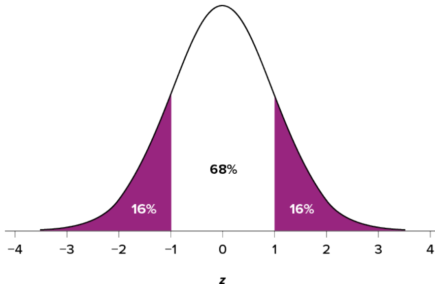
Figure 4.3. Shaded areas represent the area under the curve in the tails. (“Area under the Curve in the Tails” by Judy Schmitt is licensed under CC BY-NC-SA 4.0 .)
