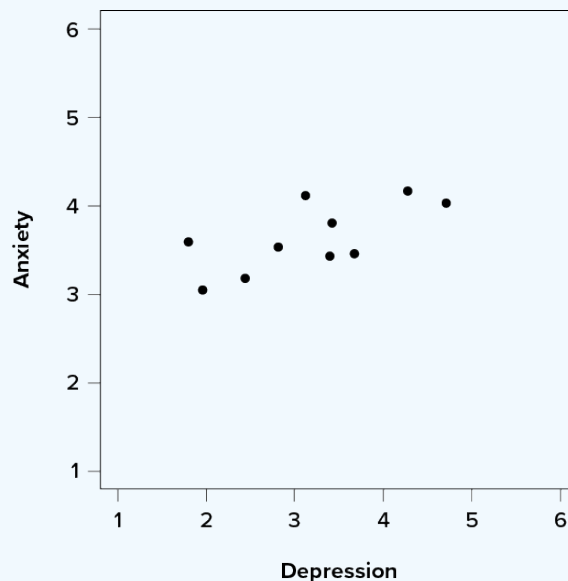
Figure 12.10. Scatter plot of depression and anxiety. ("Scatter Plot Depression and Anxiety" by Judy Schmitt is licensed under CC BY-NC-SA 4.0.)
