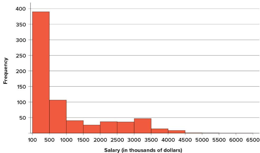
Figure 3.9. A distribution with a very large positive skew. This histogram shows the salaries of major league baseball players (in thousands of dollars). (“1994 MLB Salaries Histogram” by Judy Schmitt is licensed under CC BY-NC-SA 4.0 .)
