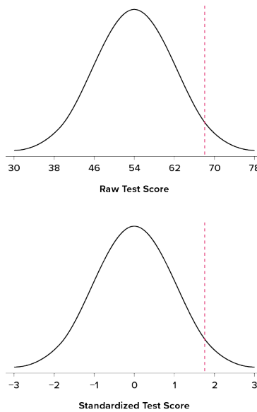
Figure 4.2. Raw and standardized versions of a single score. (“Raw and Standardized Versions of a Score” by Judy Schmitt is licensed under CC BY-NC-SA 4.0.)
