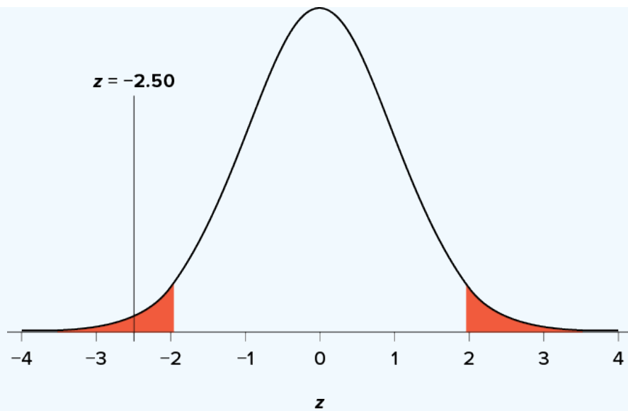
Figure 7.5. Test statistic location. (“Test Statistic Location z-2.50” by Judy Schmitt is licensed under CC BY-NC-SA 4.0.)
