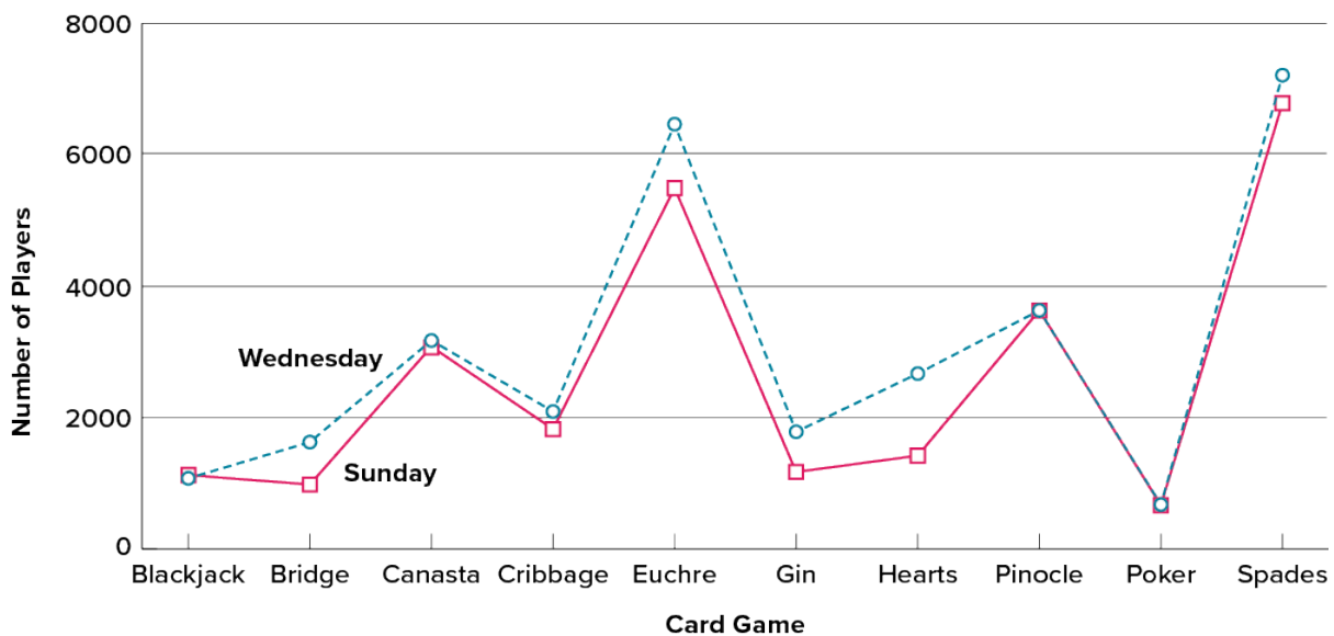
Figure 2.7. A line graph used inappropriately to depict the number of people playing different card games on Sunday and
