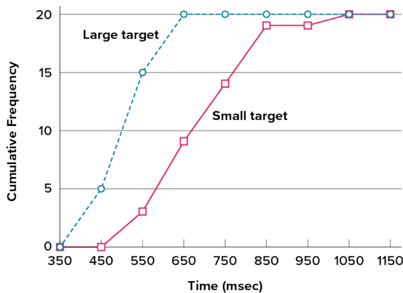
Figure 2.19. Overlaid cumulative frequency polygons for the cursor task. (“Cursor Task Cumulative Frequency Polygons” by Judy Schmitt is licensed under CC BY-NC-SA 4.0. )
