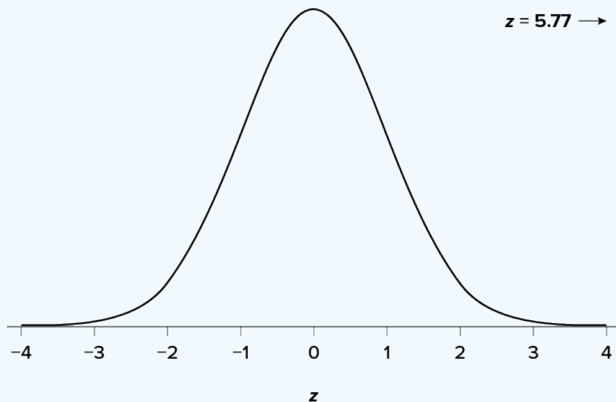
Figure 7.7. Obtained z statistic. ("Obtained z5.77" by Judy Schmitt is licensed under CC BY-NC-SA 4.0.)
