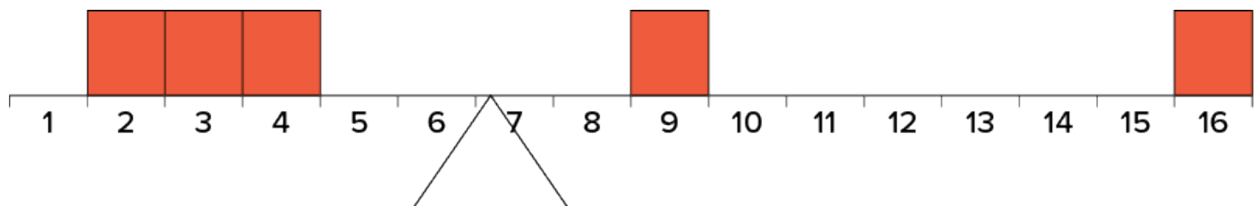
Figure 3.7. The distribution balances at the mean of 6.8 and not at the median of 4.0. (“Balance Scale Numbered” by Judy Schmitt is licensed under CC BY-NC-SA 4.0 .)
