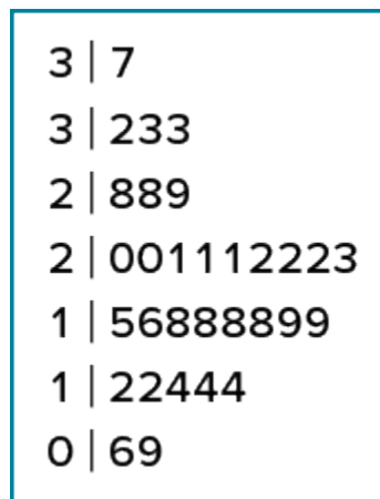
Figure 2.10. Stem-and-leaf display with the stems split in two. (“Touchdown Passes Split Stem and Leaf” by Judy Schmitt is licensed under CC BY-NC-SA 4.0. )
