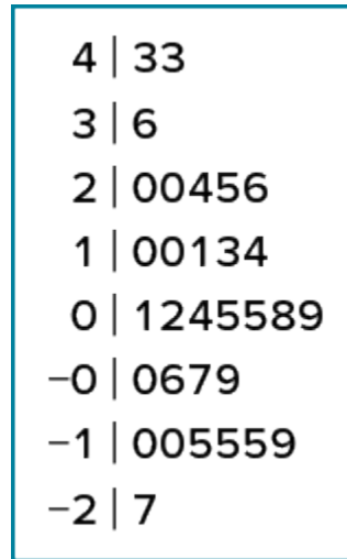
Figure 2.13. Stem-and-leaf display with negative numbers and rounding. (“ Priming Effects Stem and Leaf ” by Judy Schmitt is licensed under CC BY-NC-SA 4.0 .)
