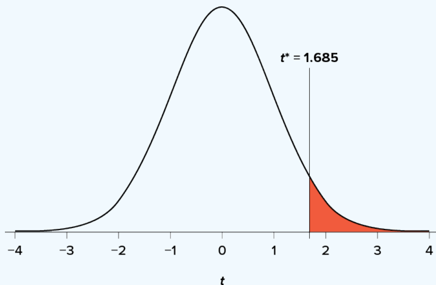
Figure 9.1. Critical region for one-tailed t test at \alpha = .05 . (“Critical Region t1.685” by Judy Schmitt is licensed under CC BY-NC-SA 4.0.)
