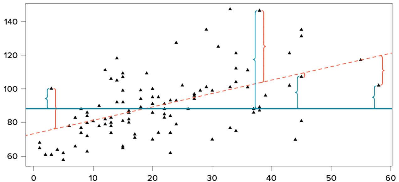
Figure 13.2. Scatter plot with residuals and deviation scores. (“Scatter Plot with Residuals and Deviation Scores” by Judy Schmitt is licensed under CC BY-NC-SA 4.0.)
