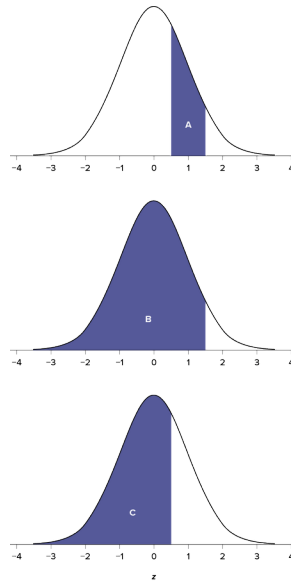
Figure 5.5. Area between z = 0.50 and 1.50 (A), along with the corresponding areas in the body (B and C). (“Area between z0.50 and z1.50 ” by Judy Schmitt is licensed under CC BY-NC-SA 4.0.)
