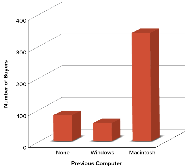
Figure 2.4. A three-dimensional version of Figure 2.2. Charts like this are less effective. (“Mac Bar Chart 3D” by Judy Schmitt is licenced under CC BY-NC-SA 4.0 .)
