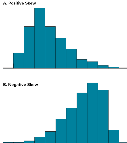
Figure 2.34. Positively skewed (A) and negatively skewed (B) distributions. (“Skewed Distributions” by Judy Schmitt is licensed under CC BY-NC-SA 4.0. )
