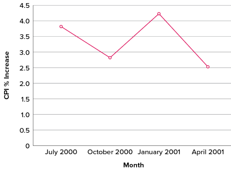
Figure 2.30. A line graph of the percent change in the CPI over time. Each point represents percent increase for the three months ending at the date indicated. (“Percent Change in CPI Line Graph” by Judy Schmitt is licensed under CC BY-NC-SA 4.0.)
