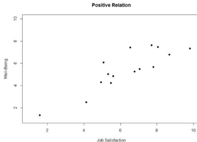
Figure 2.11.2- Scatterplot of Job Satisfaction & Well-Being (CC-BY-NC-SA Foster et al. from An Introduction to Psychological Statistics )
