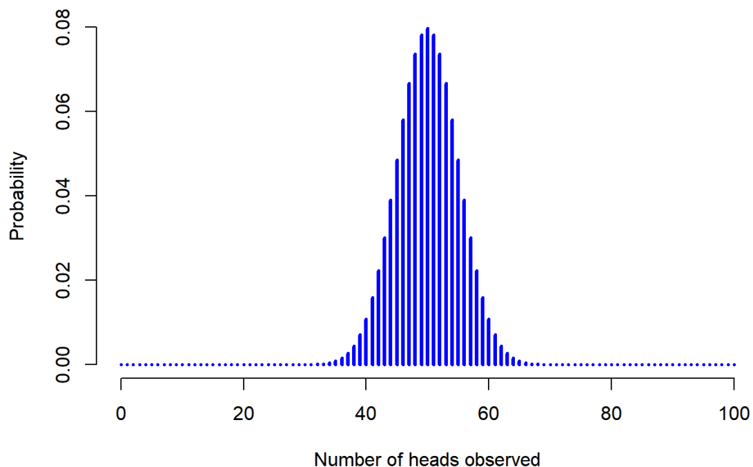
Figure 4.3.3- Probability of Heads from Flipping a Fair Coin 100 Times (CC-BY-SA Danielle Navarro from Learning Statistics with R )
