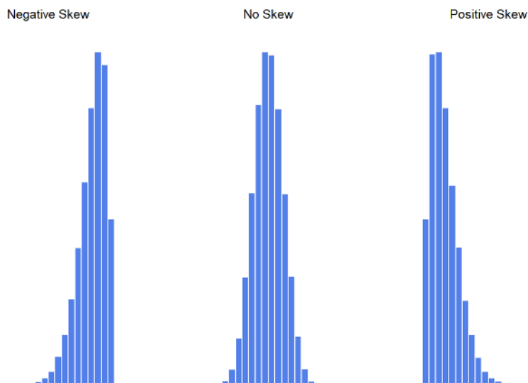
Figure 2.7.2- Diagram of Skew and No Skew (CC-BY-SA Danielle Navarro from Learning Statistics with R )
