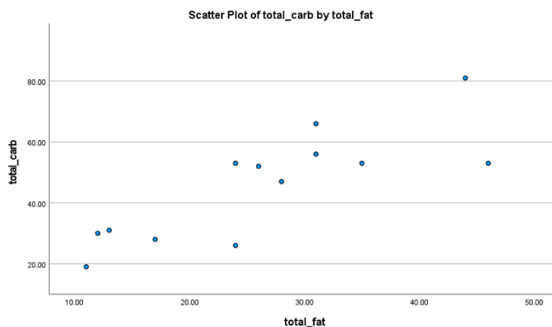
Figure 14.7.2.1: Scatterplot of Carbohydrates by Fat for 13 Chicken Meals. (CC-BY; Michelle Oja via OpenIntro.org )
