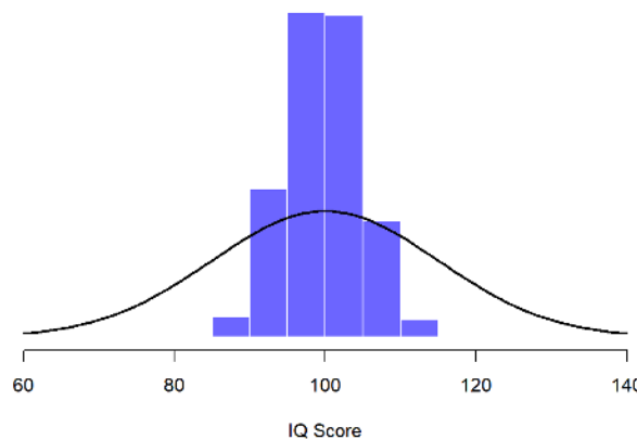
Figure 4.6.5- Distribution of Mean IQ from 10,000 Samples of 10 IQ Scores (CC-BY-SA Danielle Navarro from Learning Statistics with R )
