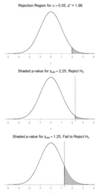
Figure 7.5.3: Relation between \alpha , z_{obs} , and p (CC-BY-NC-SA Foster et al. from An Introduction to Psychological Statistics )
