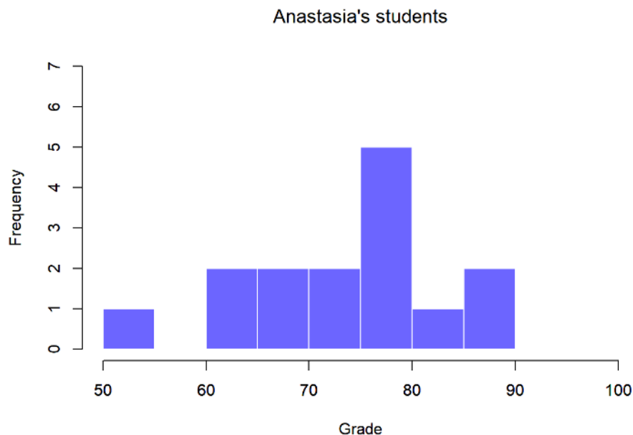
Figure 9.1.1.1- Histogram showing the overall distribution of grades for students in Anastasia's class (CC-BY-SA Danielle Navarro from Learning Statistics with R )
