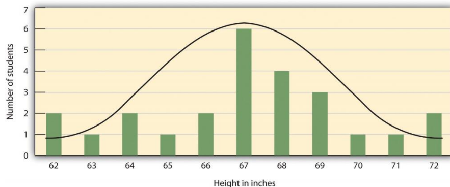
Figure 2.2.5 Height Distribution: The distribution of the heights of the students in a class will form a normal distribution. In this sample the mean ( M ) = 67.12 and the standard deviation ( s ) = 2.74.
