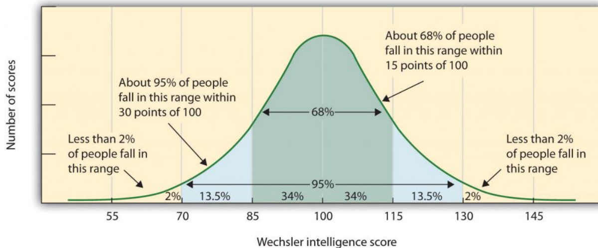
Figure 9.2.6 Distribution of IQ Scores in the General Population
