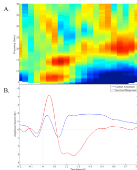
Figure 2.3.2: Example of EEG analysis output. Panel A represents changes in the relative strength of different frequencies in the EEG data over time. Panel B represents changes in the amplitude in the instantaneous EEG voltage over time. Noba Psychophysiological Methods in Neuroscience . CC BY SA-NC 4.0 International License .
