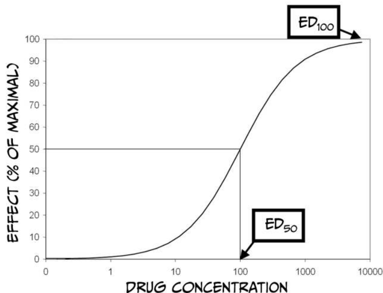
Figure 3.43 Dose-response curve
