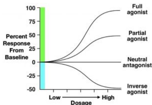
Figure 3.47. Agonist comparison
