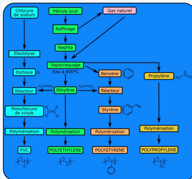
Figure #2: A Chemical Flowchart
