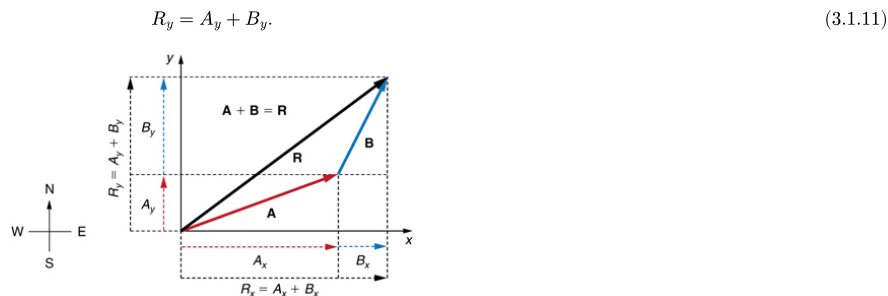
Figure 3.1.7: The magnitude of the vectors A_x and B_x add to give the magnitude R_x of the resultant vector in the horizontal direction. Similarly, the magnitudes of the vectors A_y and B_y add to give the magnitude R_y of the resultant vector in the vertical direction.
