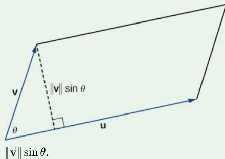
Figure 5.1.6: The parallelogram with adjacent sides \vec{u} and \vec{v} has base \|\vec{u}\| and height
