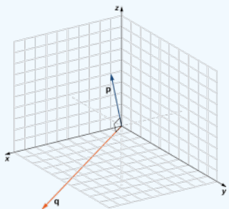
Figure 4.1.4: Vectors \vec{p} and \vec{q} form a right angle when their initial points are aligned.
