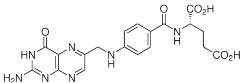
Skeletal formula
