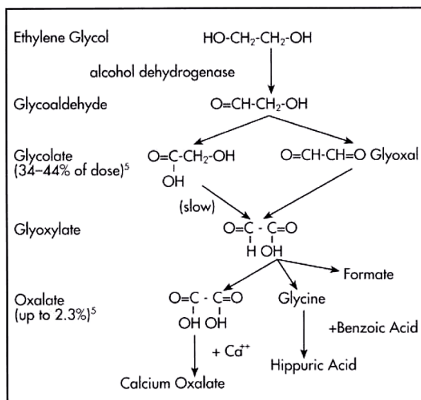
Figure 8.6.2: Metabolism of Ethylene Glycol
