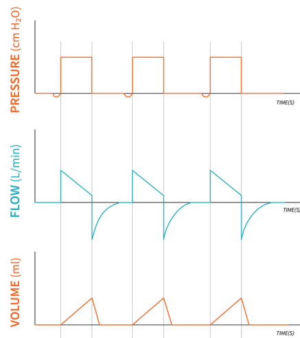
Figure 6.4.1: “Pressure Support Ventilation Diagram” by Freddy Vale, CC BY-NC-SA 4.0
