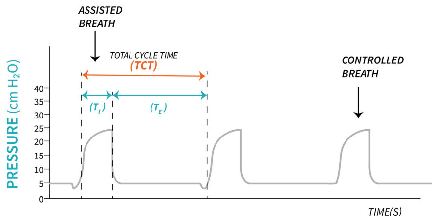
Figure 2.3.2: "Trigger Diagram" by Freddy Vale, CC BY-NC-SA 4.0
