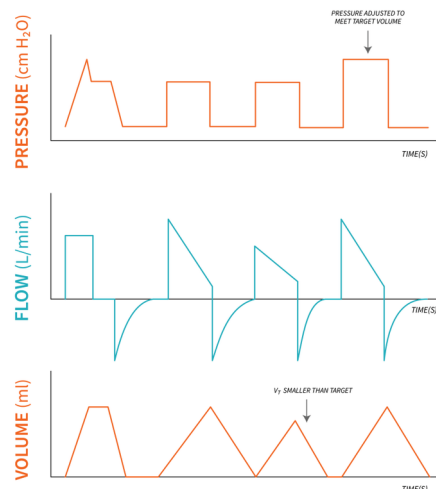
Figure 5.7.1: "PRVC Diagram" by Freddy Vale CC BY-NC-SA 4.0
