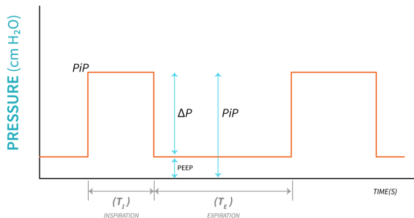
Figure 5.6.2: “Pressure – Time in PCV Waveform” by Freddy Vale, CC BY-NC-SA 4.0
