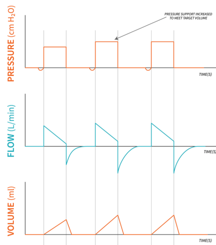
Figure 6.7.1: "Pressure Support with Target Volume" by Freddy Vale, CC-BY-NC-SA
