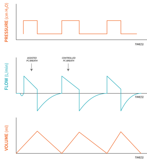
Figure 5.6.1: "PCV Waveforms" by Freddy Vale, CC BY-NC-SA 4.0
