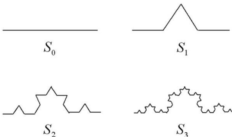
Figure 12.8: Construction of the Koch curve.
