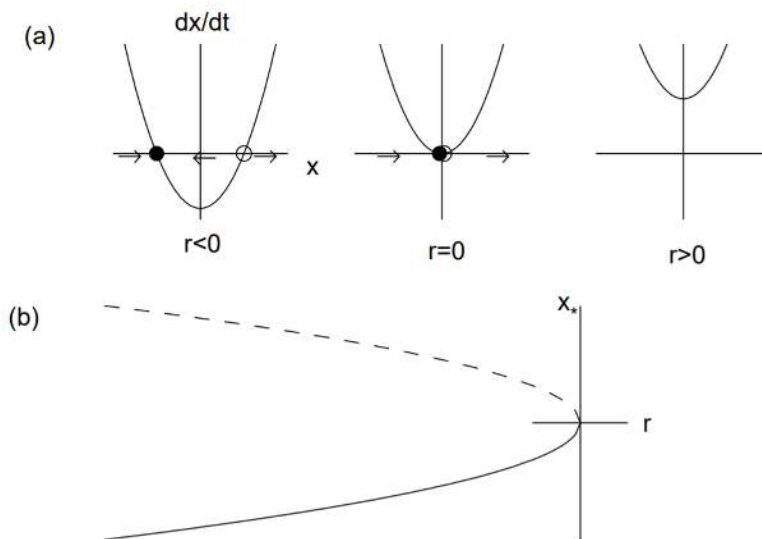
Figure 12.1: Saddlenode bifurcation. (a) \dot{x} versus x ; (b) bifurcation diagram.
