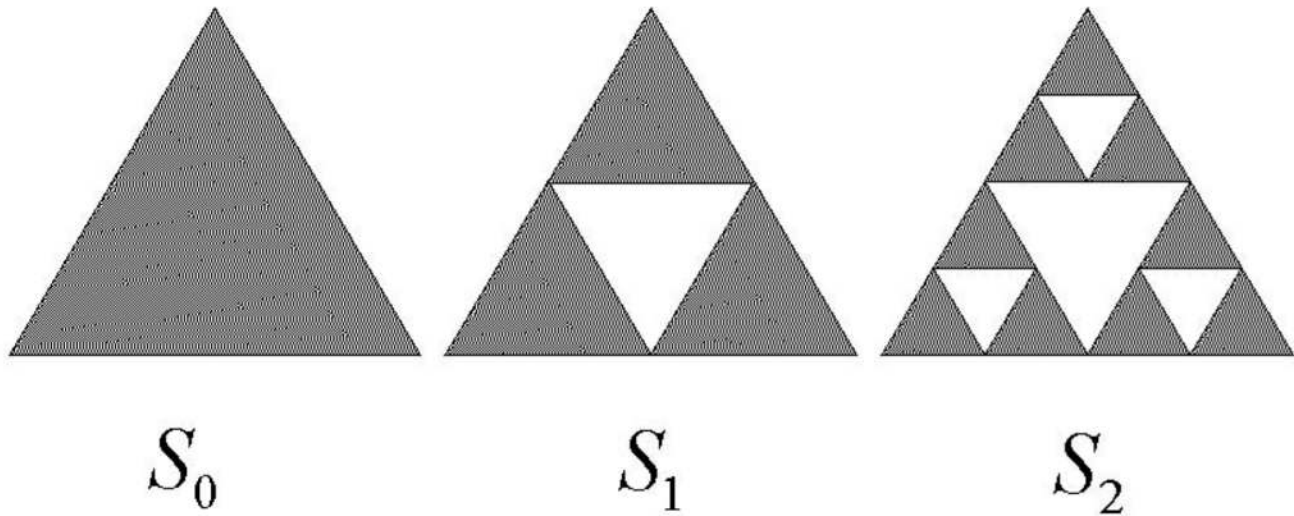
Figure 12.6: Construction of the Sierpinski triangle.
