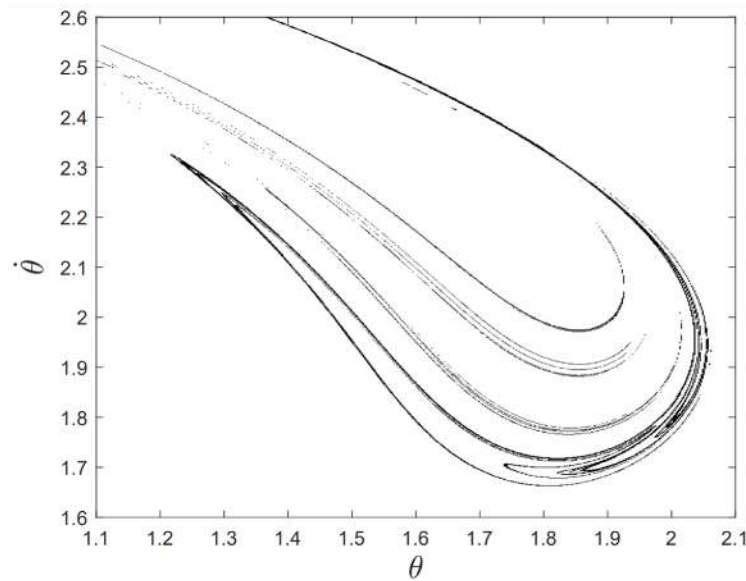
Figure 13.11: A Poincaré section of the chaotic pendulum. The values of the parameters are q = 4 , f = 1.5 , and \omega = 2/3 . The top figure shows the entire attractor and the bottom figure is a blow-up of the region inside the drawn rectangle.
