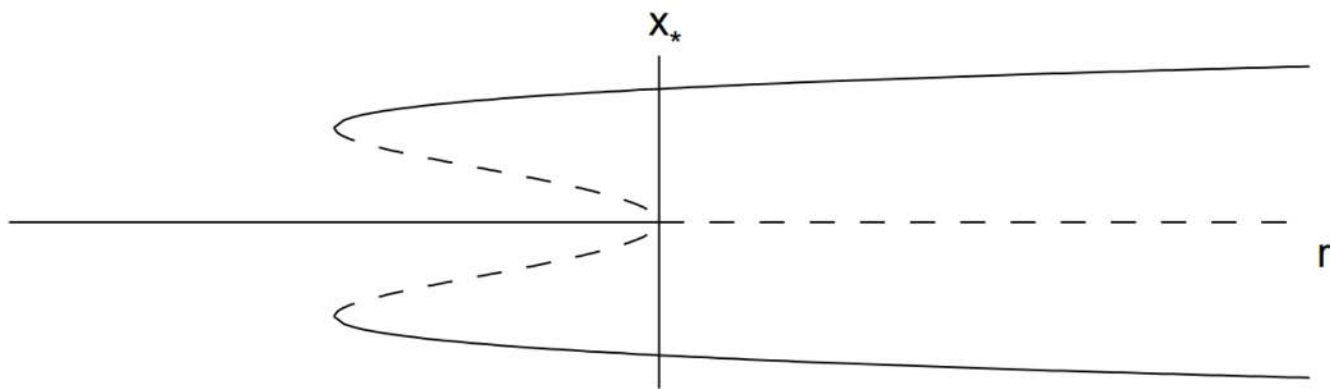
Figure 12.4: Subcritical pitchfork bifurcation diagram.
