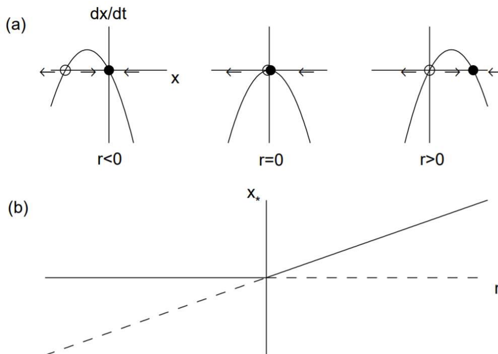
Figure 12.2: Transcritical bifurcation. (a) \dot{x} versus x ; (b) bifurcation diagram.
