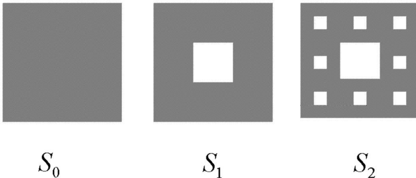
Figure 12.7: Construction of the Sierpinski Carpet
