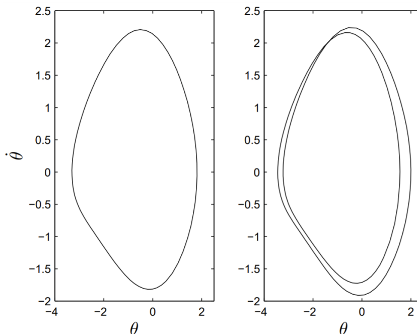
Figure 13.6: Phase-space projection of the pendulum solution before and after the first period-doubling bifurcation. In both plots, f = 1.5, \omega = 2/3 . (a) q = 1.34 and the oscillation has period one; (b) q = 1.36 and the oscillation has period two.
