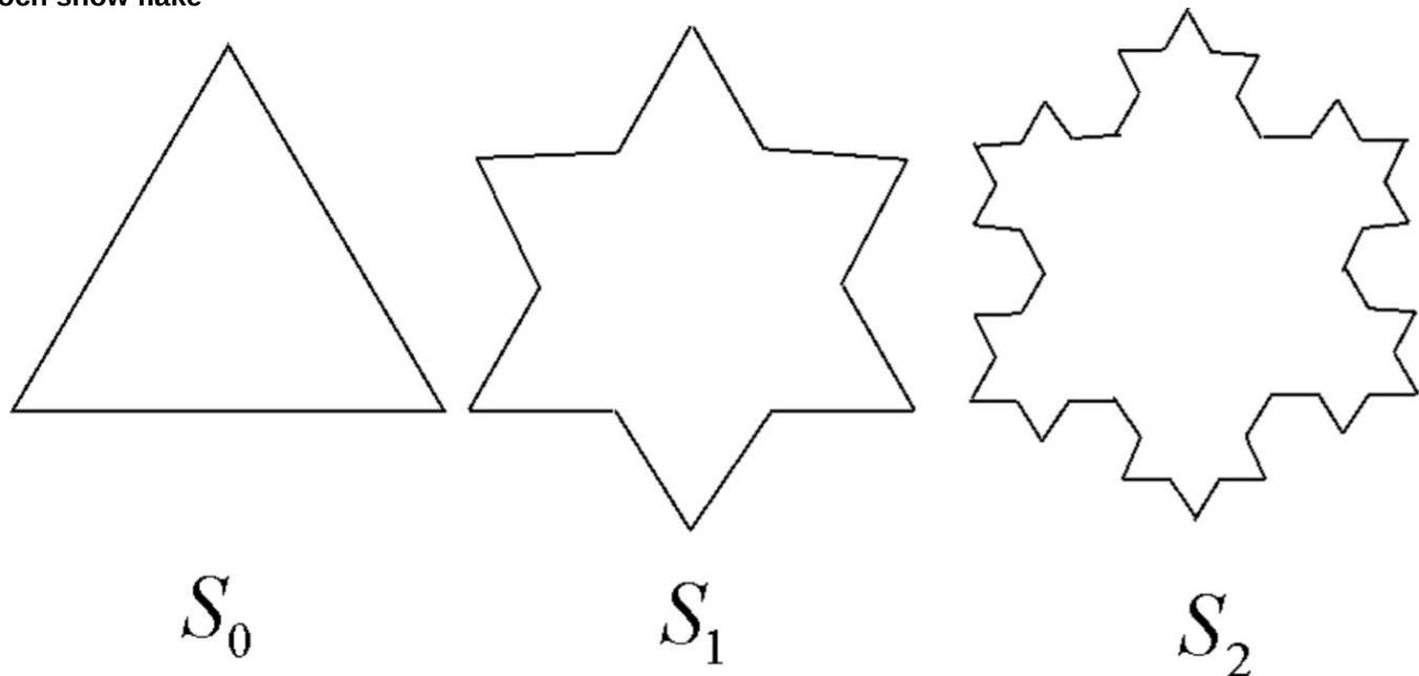
Figure 12.9: Construction of the Koch snow flake.
