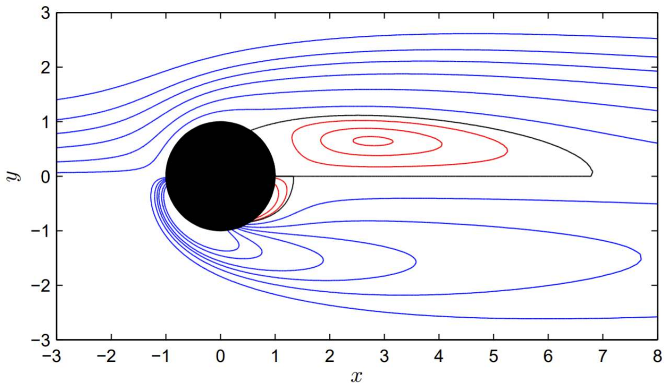
Figure 17.1: Contour plots of the stream function ( y > 0 ) and vorticity ( y < 0 ) for Re = 50 . Negative contours are in red, the zero contour in black, and positive contours in blue. The contour levels for the stream function are -0.05, -0.04, -0.02, 0, 0.05, 0.2, 0.4, 0.6, 0.8, 1.1 and those for the vorticity are -0.2, -0.05, 0, 0.25, 0.5, 0.75, 1, 1.5, 2
