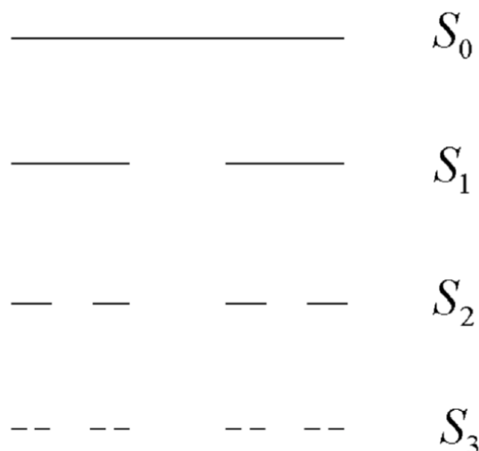
Figure 12.5: Construction of the Cantor set.
