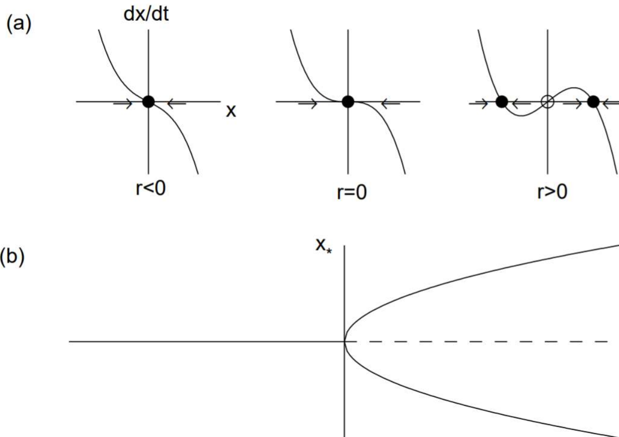
Figure 12.3: Supercritical pitchfork bifurcation. (a) \dot{x} versus x ; (b) bifurcation diagram.
