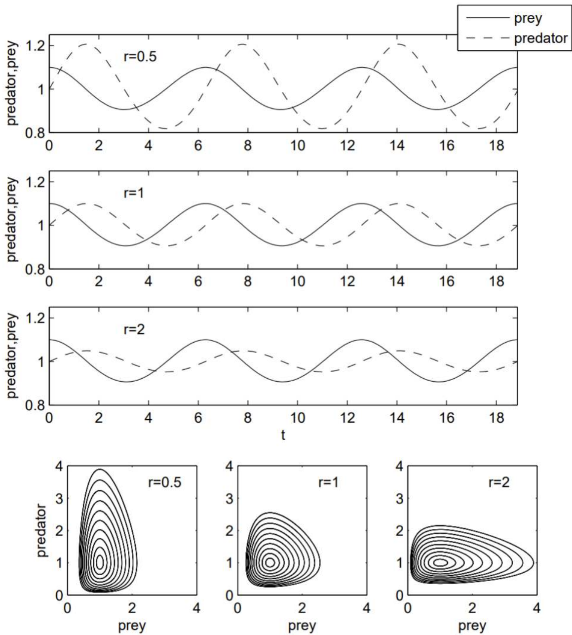
Figure 1.5: Solutions of the dimensionless Lotka-Volterra equations. Upper plots: timeseries solutions; lower plots: phase portraits.
