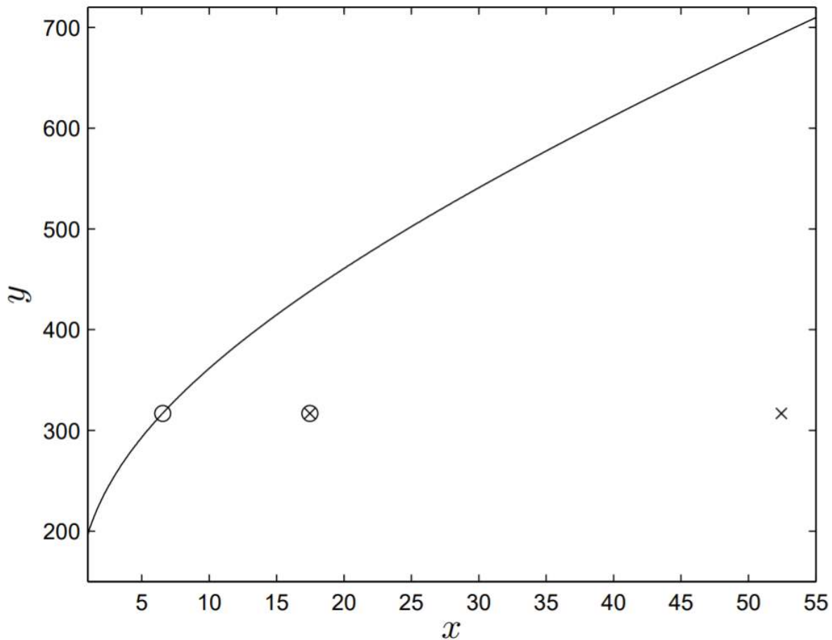
Figure 2.7: Solution curve of y versus x with brood size B = 286 , obtained by solving (2.7.14). Values for B, m, p and g are taken from Table 2.3. The cross, crossed open circle and open circle correspond to y = mg and x = mfB/p with f = 1, 1/3 and 1/8 , respectively.
