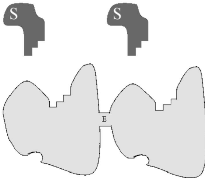
Figure 6.4: Cooperativity.
