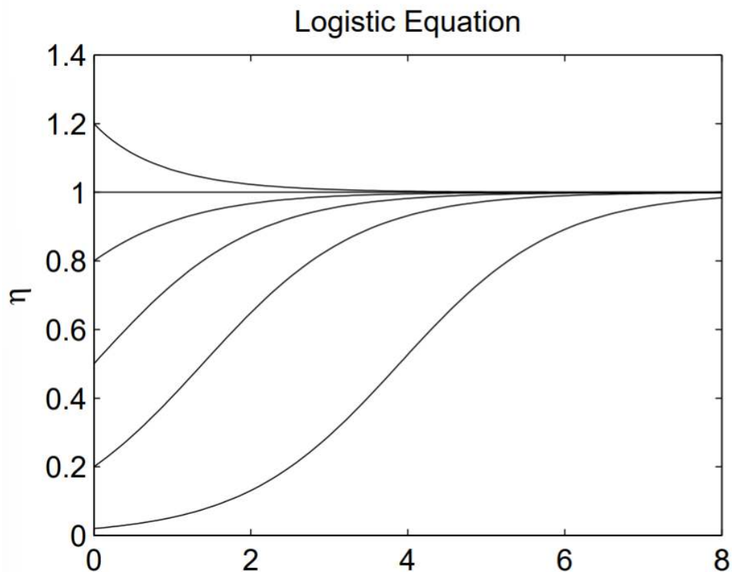
Figure 1.3: Solutions of the dimensionless logistic equation
