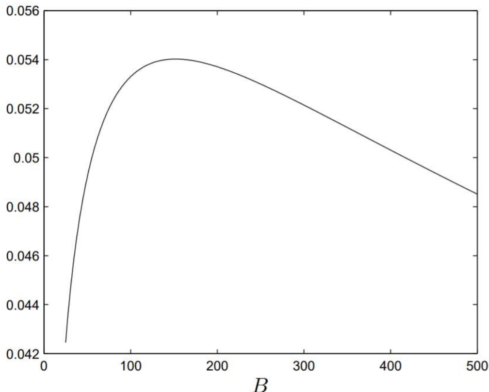
Figure 2.6: A plot of r = r(B) , which demonstrates that the Malthusian growth rate r is maximum near a brood size of B = 152
