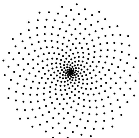
Figure 2.2: Simulation of a sunflower head for (a) \alpha = 1/7 ; (b) \alpha = \pi - 3 .
