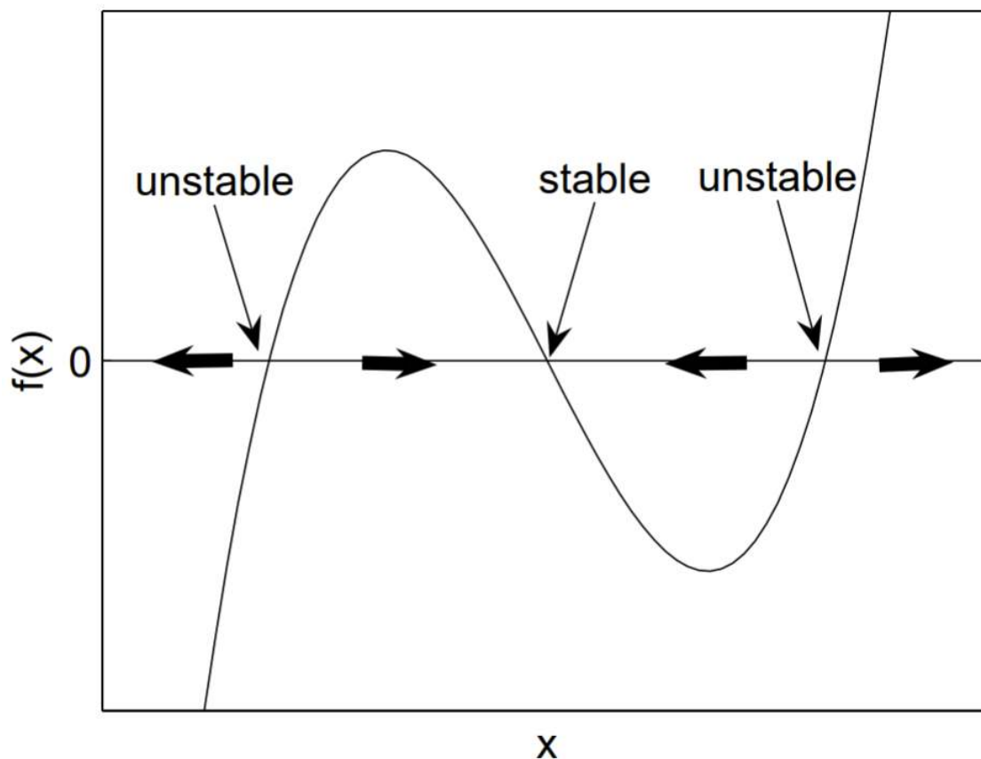
Figure 1.1: Determining one-dimensional stability using a graphical approach.
