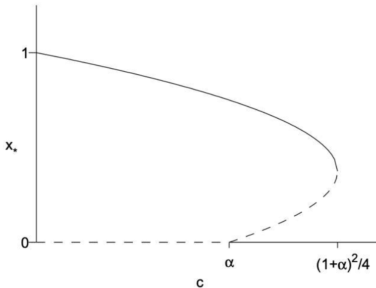
Figure 11.6: Fishery bifurcation diagram.
