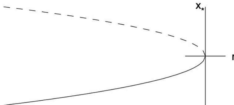
Figure 11.2: Saddle-node bifurcation. (a) \dot{x} versus x ; (b) bifurcation diagram.
