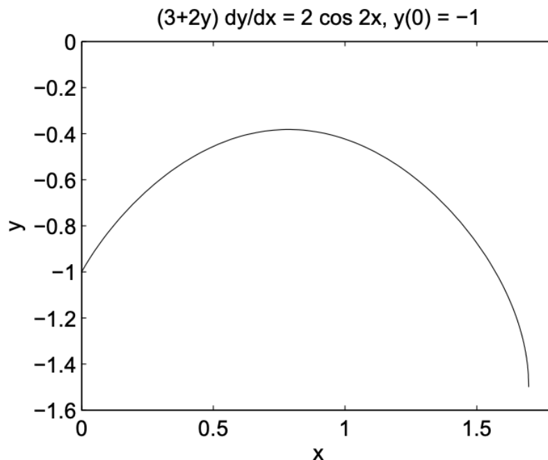
Figure 7.3: Solution of the following ode: (3 + 2y)y' = 2 \cos 2x , y(0) = -1 .
