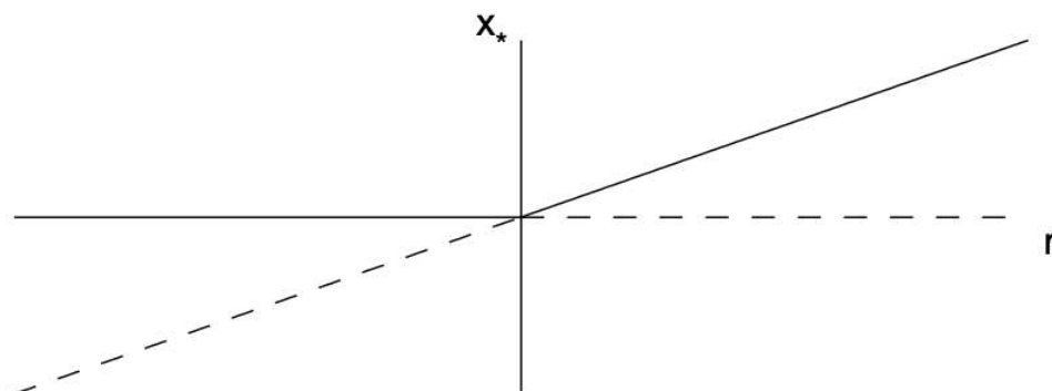
Figure 11.3: Transcritical bifurcation. (a) \dot{x} versus x ; (b) bifurcation diagram.
