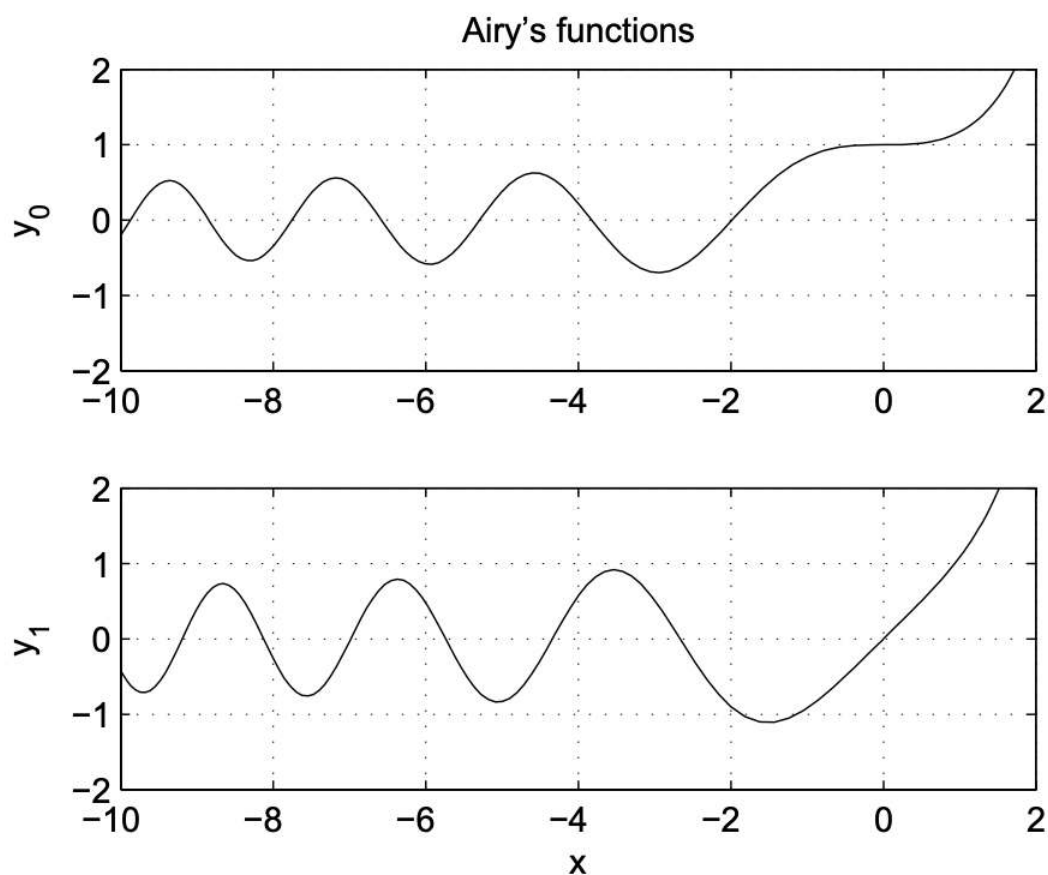
Figure 9.1: Numerical solution of Airy's equation.
