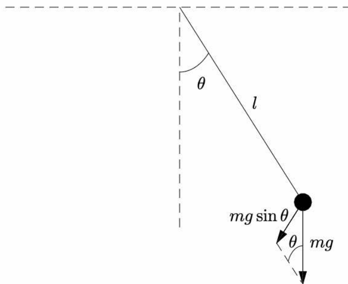
Figure 8.3: The pendulum.
