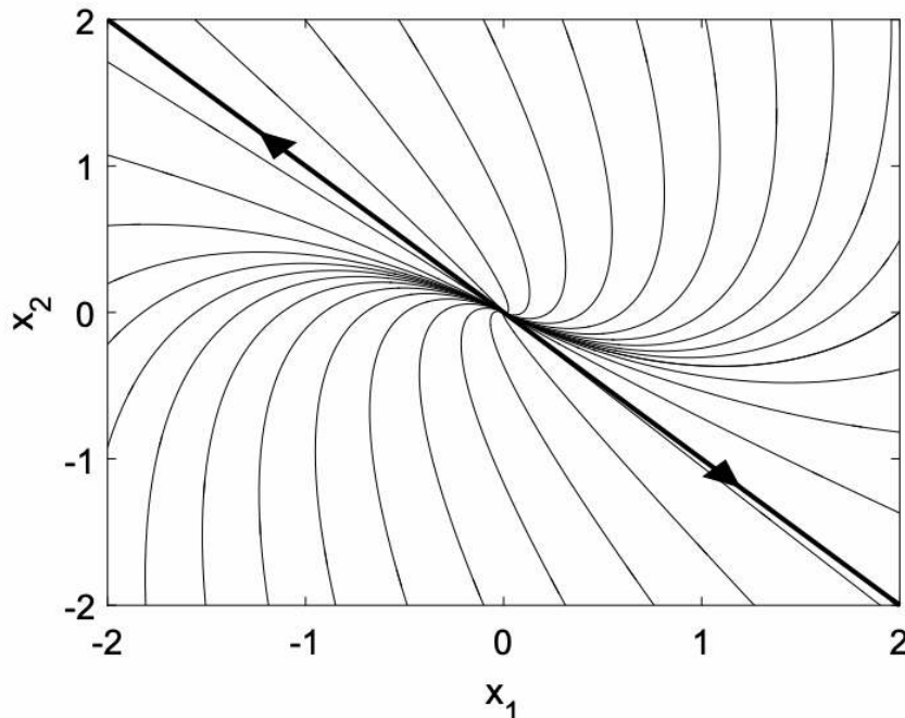
Figure 10.3: Phase portrait for example with only one eigenvector.
