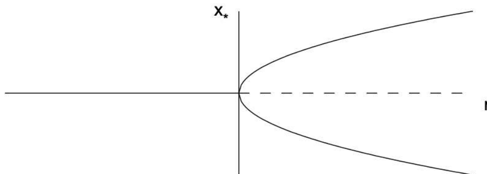
Figure 11.4: Supercritical pitchfork bifurcation. (a) \dot{x} versus x ; (b) bifurcation diagram.
