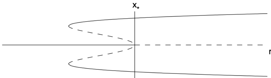
Figure 11.5: Subcritical pitchfork bifurcation.
