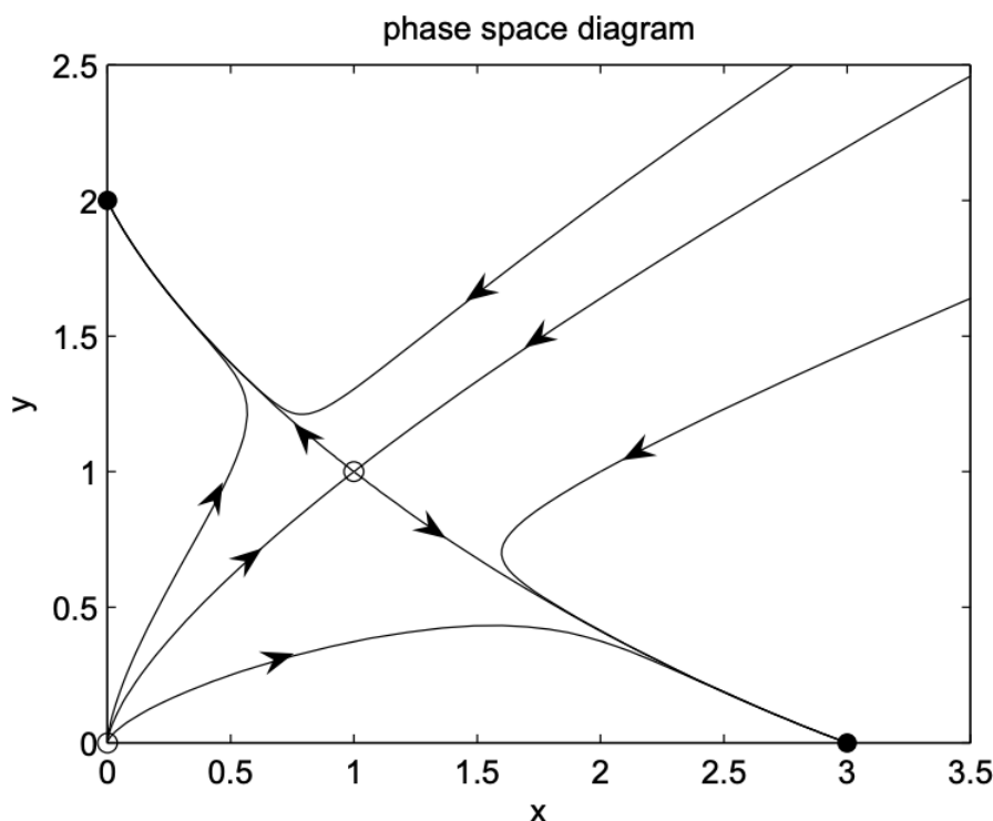
Figure 11.1: Phase space plot for two-dimensional nonlinear system.
