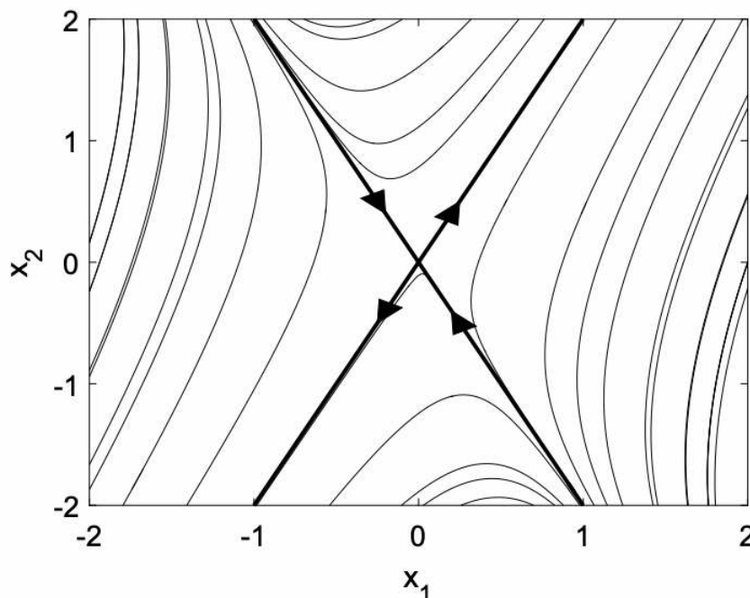
Figure 10.1: Phase portrait for example with two real eigenvalues of opposite sign.
