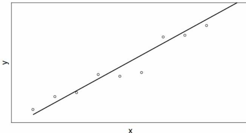
Figure 3.9.1: Linear Regression
