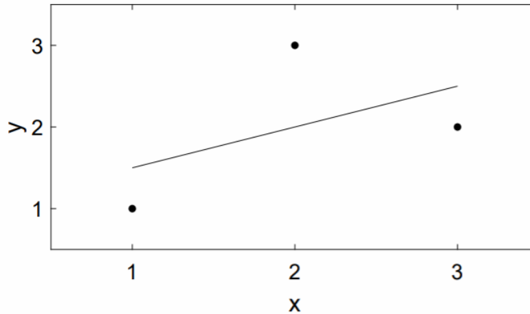
Figure 3.10.1: Solution of the toy least-squares problem.
