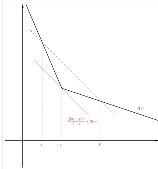
Figure 4.12: Subdifferential mean value theorem.
