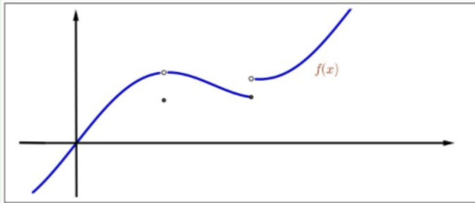
Figure 3.6: Lower semicontinuity.
