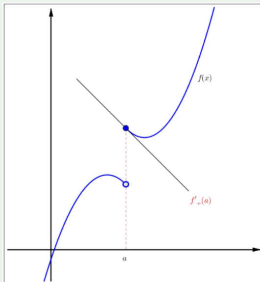
Figure 4.4: Right derivative.
