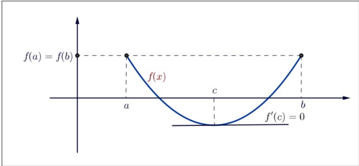
Figure 4.2: Illustration of Rolle's Theorem.
