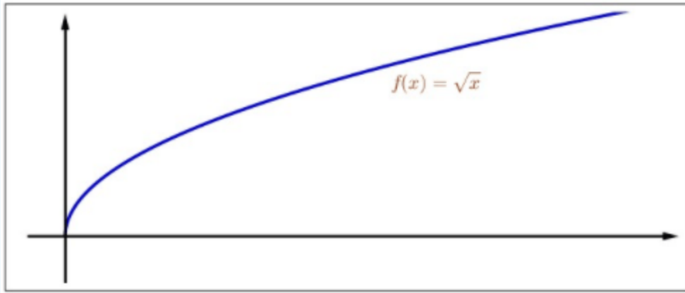
Figure 3.4: The square root function.
