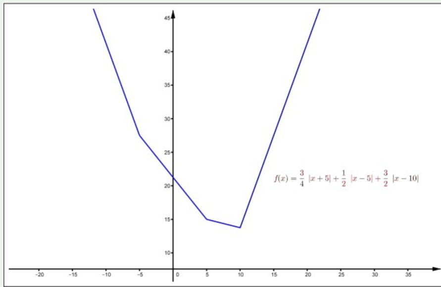
Figure 4.7: A nondifferentiable convex function.
