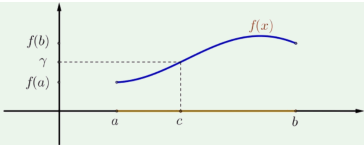
Figure 3.3: Illustration of the Intermediate Value Theorem.
