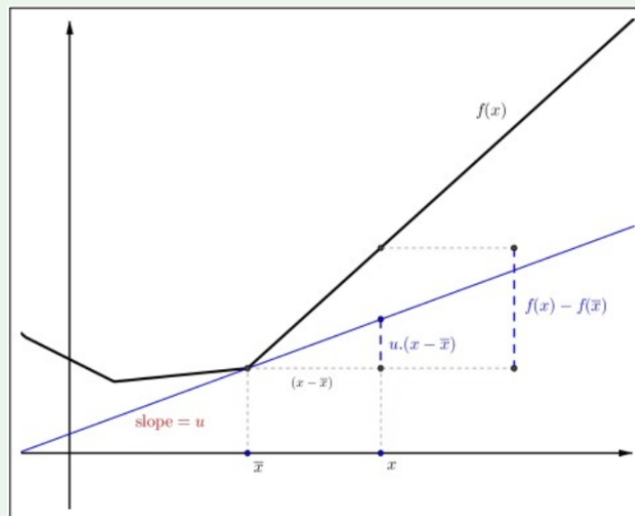
Figure 4.8: Definition of subderivative.
