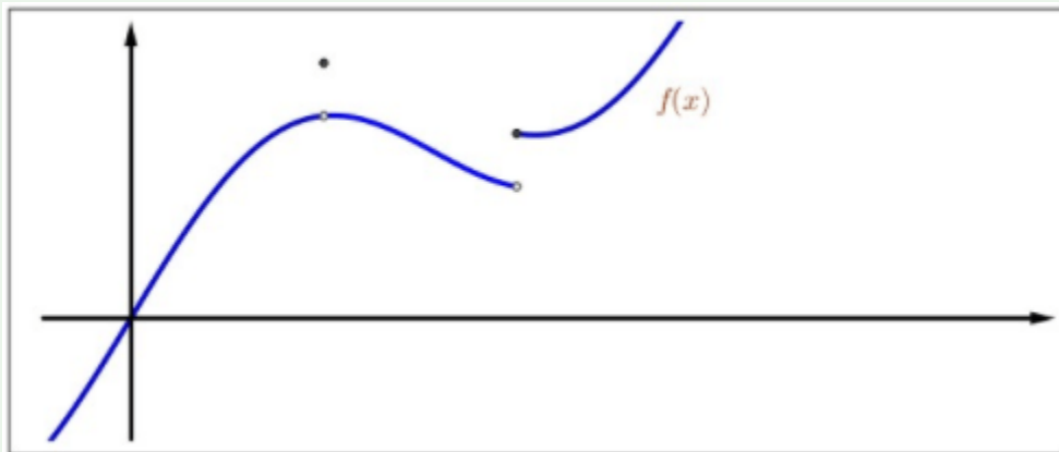
Figure 3.7: Upper semicontinuity.
