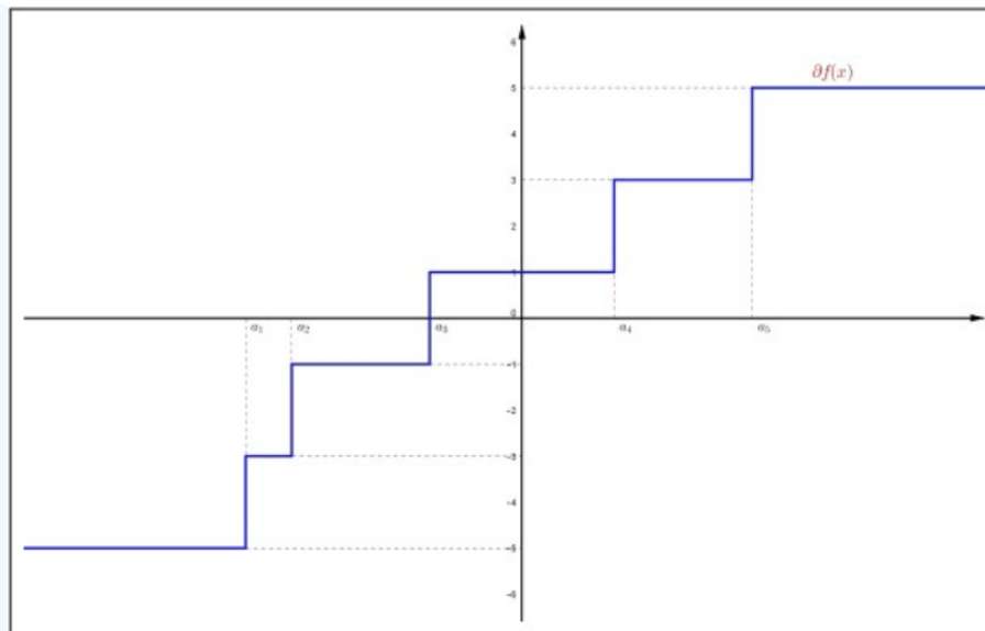
Figure 4.10: Subdifferential of f(x) = \sum_{i=1}^{2k-1} |x - a_i| .
