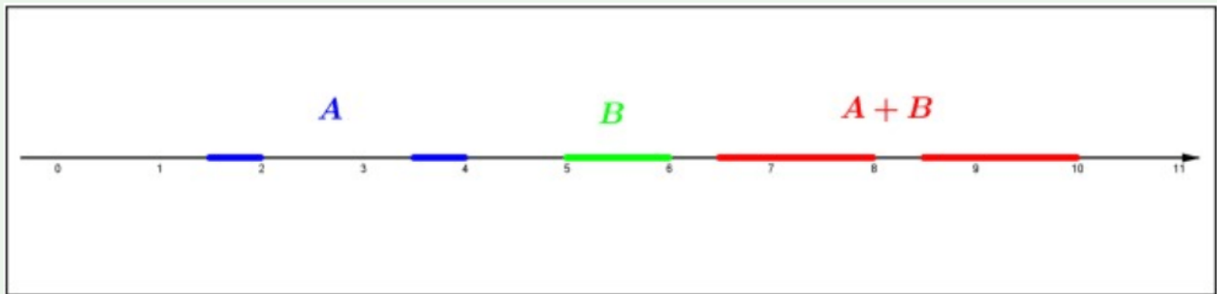
Figure 4.9: Set addition.
