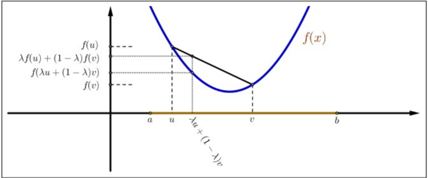
Figure 4.6: A Convex Function.
