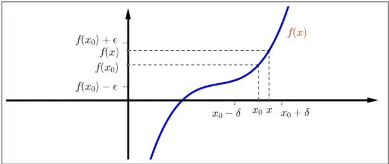
Figure 3.1: Definition of Continuity.
