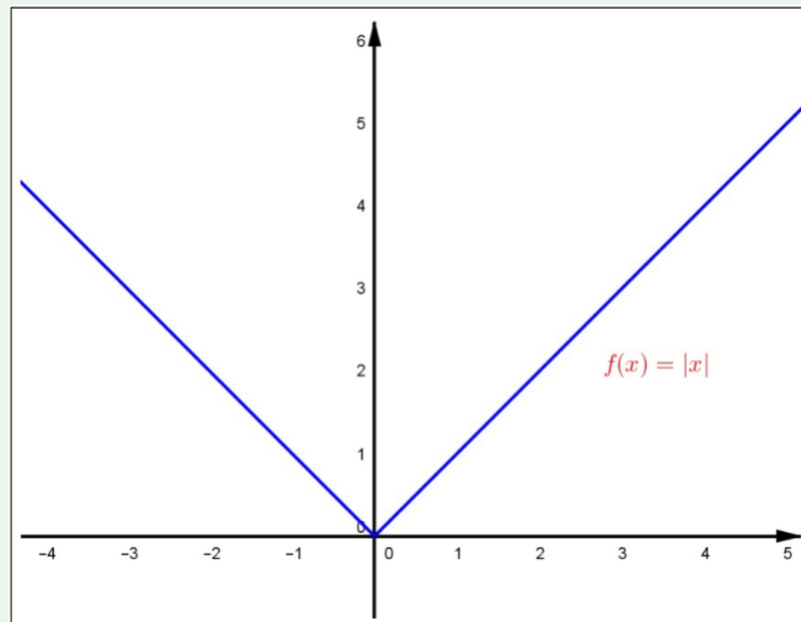
Figure 1.1: The absolute value function.
