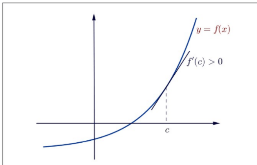
Figure 4.5: Strictly Increasing Function.
