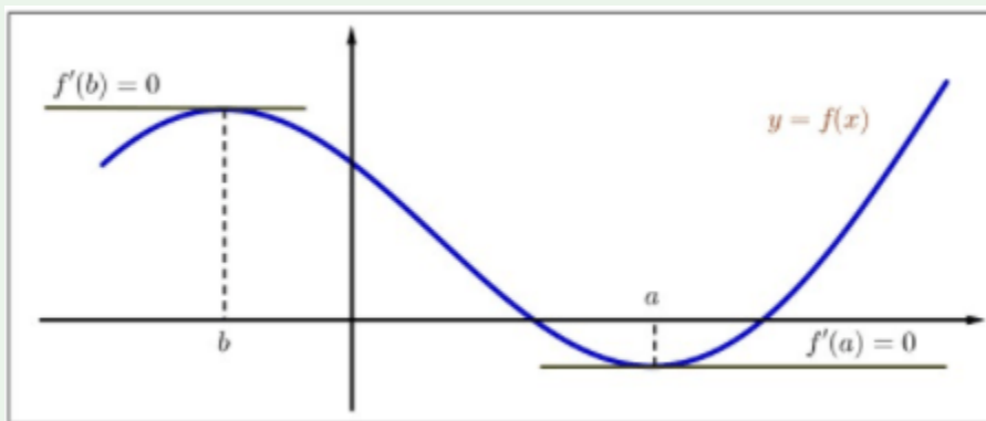
Figure 4.1: Illustration of Fermat's Rule.
