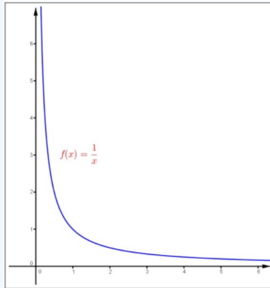
Figure 3.5: Continuous but not uniformly continuous on (0, \infty) .
