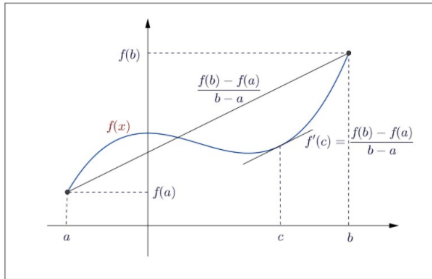
Figure 4.3: Illustration of the Mean Value Theorem.
