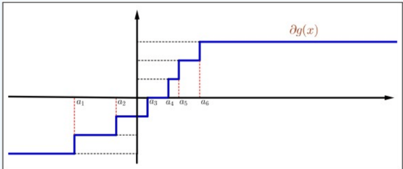
Figure 4.11: Subdifferential of g(x) = \sum_{i=1}^{2k} |x - a_i| .
