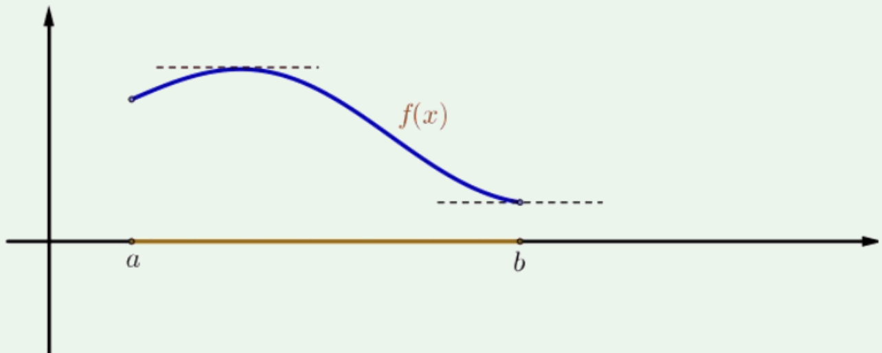
Figure 3.2: Absolute maximum and absolute minimum of f on [a, b] .
