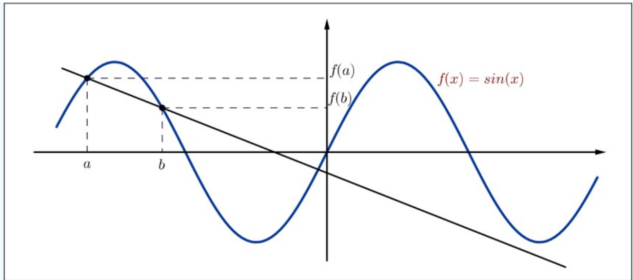
Figure 5.1: The function f(x) = \sin(x) .
