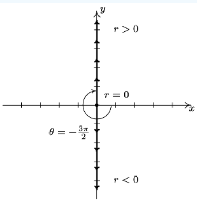
In \theta = -\frac{3\pi}{2} , r is free
