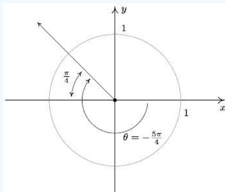
Finding \cos\left(-\frac{5\pi}{4}\right) and \sin\left(-\frac{5\pi}{4}\right)
