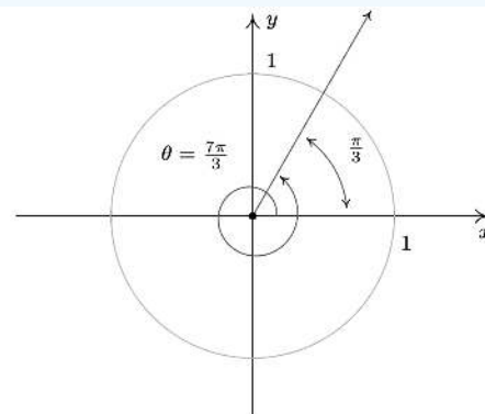
Finding \cos\left(\frac{7\pi}{3}\right) and \sin\left(\frac{7\pi}{3}\right)
