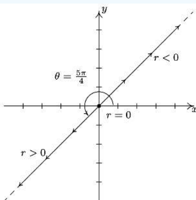
In \theta = \frac{5\pi}{4} , r is free
