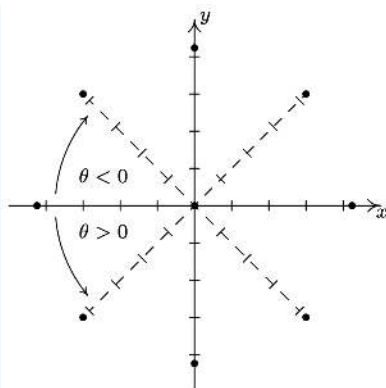
In r = -3\sqrt{2} , \theta is free
