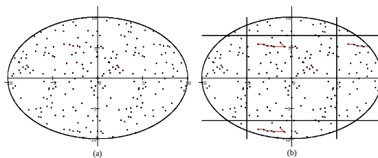
Figure 8.2.5: The positions of N objects in a catalog. (Copyright; author via source)
