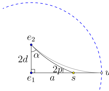
Figure 7.3.3: A detected parallax in a hyperbolic universe puts a bound on its curvature. (Copyright; author via source)
