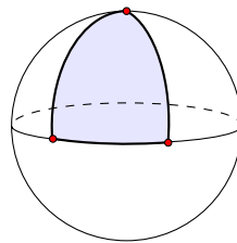
Figure 1.1.4: A triangle on a sphere. (Copyright; author via source)
