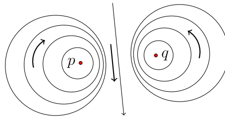
Figure 3.5.4: An elliptic Möbius transformation fixing p and q swirls points around type II clines of p and q . (Copyright; author via source)
