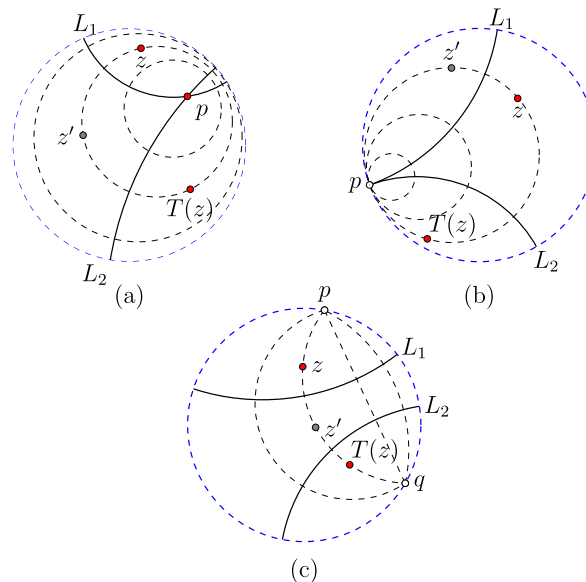
Figure 5.1.3: The three types of transformations in \mathcal{H} : (a) hyperbolic rotation (b) parallel displacement (c) hyperbolic translation. (Copyright; author via source)
