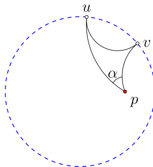
Figure 5.4.1: A \frac{2}{3} -ideal triangle having interior angle \alpha has area equal to \pi - \alpha . (Copyright; author via source)
