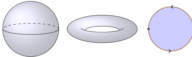
Figure 7.5.4: The sphere S^2 , the torus T^2 , and the projective plane P^2 . (Copyright; author via source)
