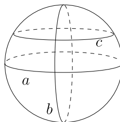
Figure 1.3.2: Geodesics on the sphere are great circles. (Copyright; author via source)
