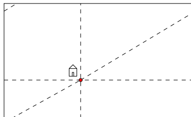
Figure 7.6.2: A flat torus has many closed geodesic paths. The length of the shortest closed geodesic path equals the length of the short side of the rectangle on which the torus is modeled. (Copyright; author via source)
