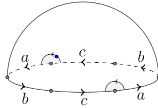
Figure 1.3.6: A surface with homogeneous elliptic geometry. (Copyright; author via source)
