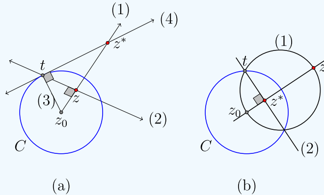
Figure 3.2.6: Constructing the symmetric point (a) if z is inside the circle of inversion; (b) if z is outside the circle of inversion. (Copyright; author via source)
