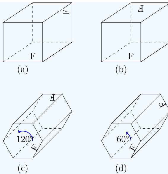
Figure 8.1.3: Four Euclidean 3-manifolds: (a) the quarter turn manifold; (b) the half turn manifold; (c) the one-third turn manifold; and (d) the one-sixth turn manifold. (Copyright; author via source)
