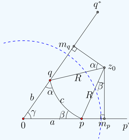
Figure 5.4.10: Deriving the hyperbolic law of sines. (Copyright; author via source)
