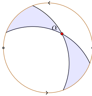
Figure 6.3.3: A lune in P^2 with angle \alpha . (Copyright; author via source)
