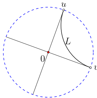
Figure 5.2.3: Through a point not on a given hyperbolic line L there exist two hyperbolic lines parallel to L . (Copyright; author via source)
