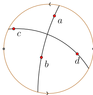
Figure 6.2.2: Elliptic lines go through antipodal points. (Copyright; author via source)
