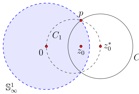
Figure 5.1.2: Constructing a circle C orthogonal to S^1_\infty about which z_0 is inverted to 0. (Copyright; author via source)
