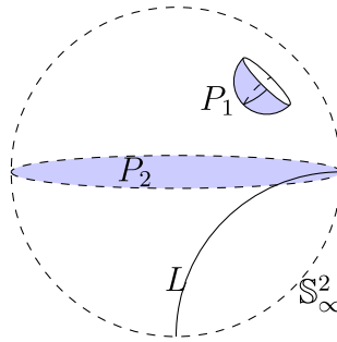
Figure 8.1.1: One model of hyperbolic space \mathbf{H}^3 , the open unit 2-ball. (Copyright; author via source)
