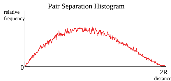
Figure 8.2.4: A pair separation histogram in a simply connected universe. (Copyright; author via source)
