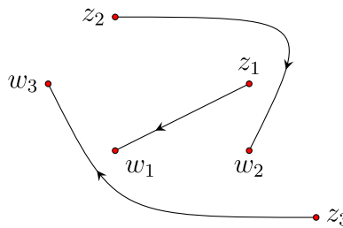
Figure 3.4.1: We can build a Möbius transformation that sends z_1 \mapsto w_1 , z_2 \mapsto w_2 , and z_3 \mapsto w_3 . (Copyright; author via source)
