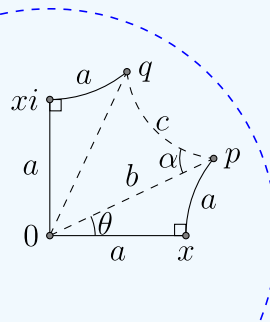
Figure 5.4.11: A journey that would trace a square in the Euclidean plane does not get you home in (\mathbb{D}, \mathcal{H}) . But how close will the finish point q be to the starting point p ? (Copyright; author via source)
