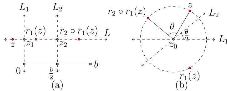
Figure 3.1.1: (a) Translations and (b) rotations are compositions of reflections. (Copyright; author via source)
