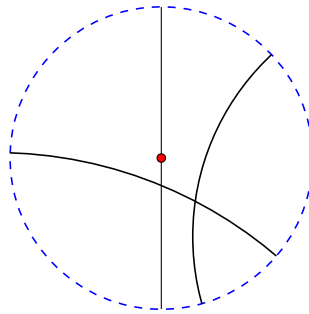
Figure 5.2.1: A few hyperbolic lines in the Poincaré disk model. (Copyright; author via source)
