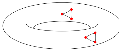
Figure 1.3.1: This torus surface is not homogeneous. (Copyright; author via source)
