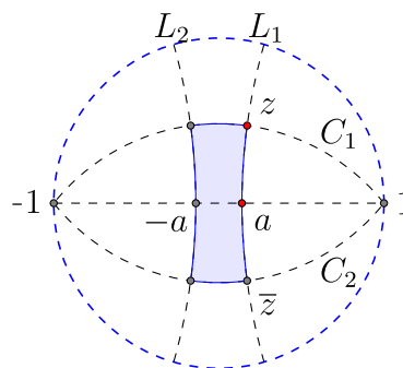
Figure 5.4.6: Blocks in \mathbb{D} : Four-sided, right-angled figures whose opposite sides have equal length. (Copyright; author via source)
