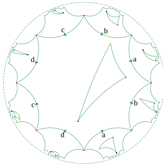
Figure 7.7.3: A triangle in H_2 , with various images of it. (Copyright; author via source)
