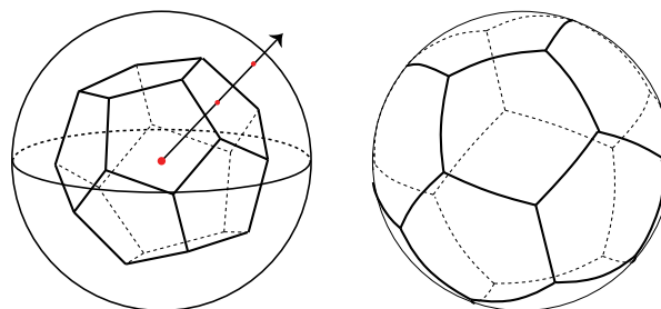
Figure 7.5.10: A dodecahedron and sphere are homeomorphic. (Copyright; author via source)
