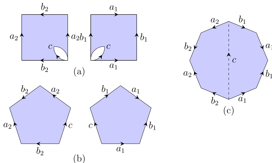
Figure 7.5.8: H_2 constructed from an octagon. (Copyright; author via source)
