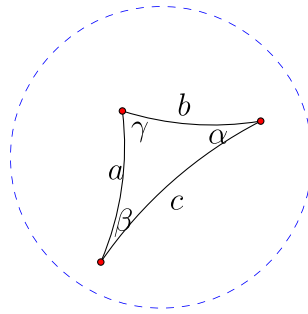
Figure 5.4.4: Relating angles and lengths in a hyperbolic triangle. (Copyright; author via source)
