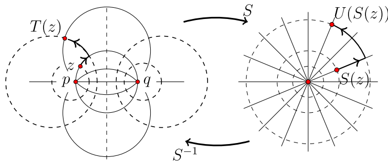
Figure 3.5.3: Tracking the image of z if T fixes p and q . (Copyright; author via source)
