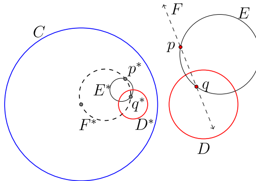
Figure 3.2.3: Inversion preserves symmetry points: If p and q are symmetric with respect to D and we invert about cline C then the image points are symmetric with respect to the image of D . (Copyright; author via source)
