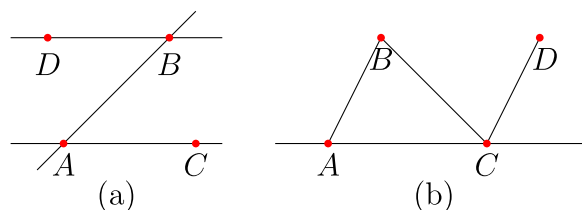
Figure 1.2.2: Two consequences of the parallel postulate. (Copyright; author via source)
