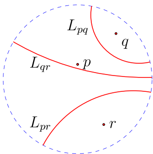
Figure 5.3.3: Three noncollinear points need not determine a circle in hyperbolic geometry. (Copyright; author via source)
