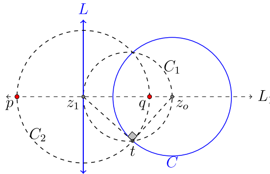
Figure 3.2.4: Finding two points symmetric with respect to a line and circle. (Copyright; author via source)
