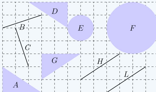
Figure 4.1.1: Figures in the plane. (Copyright; author via source)
