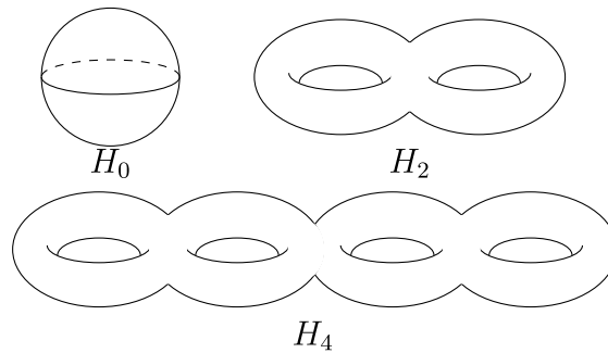
Figure 7.5.6: Some handlebody surfaces. (Copyright; author via source)
