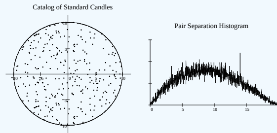
Figure 8.2.8: A catalog of images for a two-dimensional Euclidean universe, with corresponding PSH. (Copyright; author via source)
