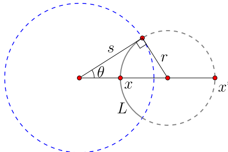
Figure 7.3.2: Deriving Lobatchevsky's formula. (Copyright; author via source)
