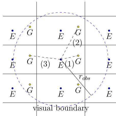
Figure 8.2.2: Detecting multiple images with a tiling of the universal covering. (Copyright; author via source)
