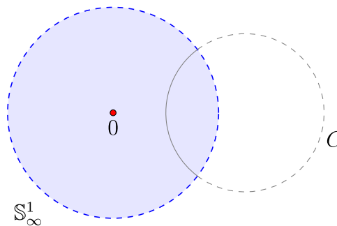
Figure 5.1.1: Inversion about a cline orthogonal to the unit circle takes \mathbf{D} to \mathbf{D} . (Copyright; author via source)
