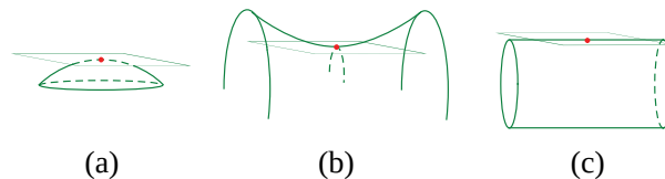
Figure 7.1.2: The curvature of a surface at a point can be (a) positive; (b) negative; or (c) zero. (Copyright; author via source)
