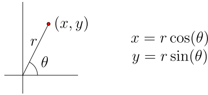
Figure 2.2.1: Polar coordinates of a point in the plane. (Copyright; author via source)
