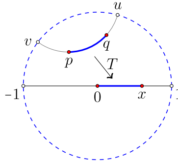
Figure 5.3.2: To find the distance between p and q , we may first transform p to 0 and q to the positive real axis. (Copyright; author via source)
