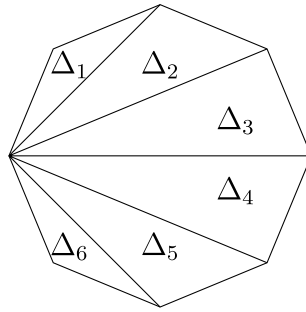
Figure 7.4.1: Splitting an n -gon into n - 2 triangles in the case n = 8 . (Copyright; author via source)
