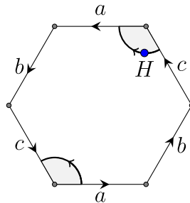
Figure 1.3.5: A hexagonal video screen. (Copyright; author via source)
