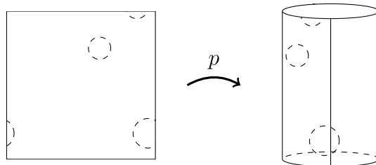
Figure 7.7.1: Bending a sheet of paper into a cylinder. (Copyright; author via source)
