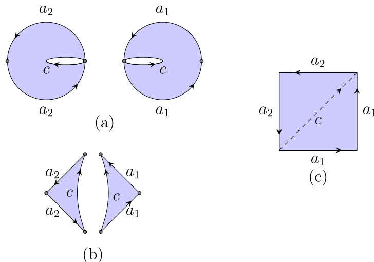
Figure 7.5.7: Constructing C_2 . (Copyright; author via source)
