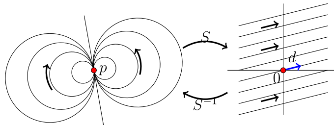
Figure 3.5.6: A parabolic map fixing p pushes points along clines that are mutually tangent at p . (Copyright; author via source)
