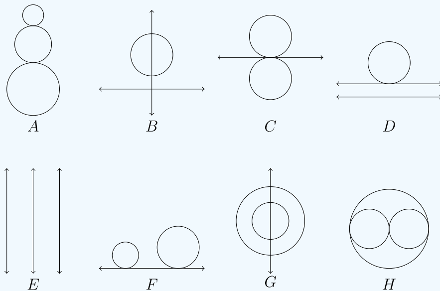
Figure 4.2.1: Which of these figures are congruent in (\mathbb{C}^+, \mathcal{M}) ? (Copyright; author via source)
