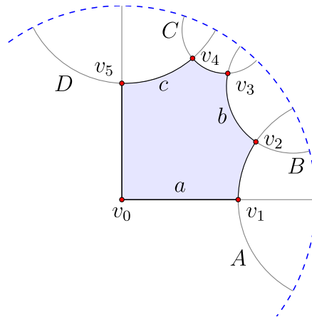
Figure 5.4.7: Building a right hexagon in the hyperbolic plane that has alternate side lengths (a, b, c) . (Copyright; author via source)
