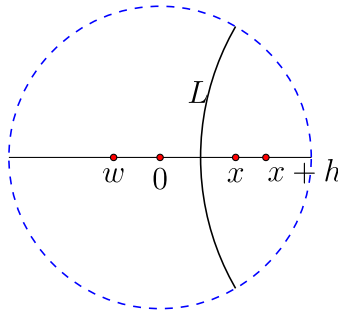
Figure 5.3.1: Reflection of the hyperbolic plane sending x to 0 and x + h to w . (Copyright; author via source)
