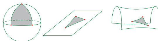
Figure 1.3.3: Depending on the shape of the surface, geodesic triangles can have angle sum greater than, less than, or equal to 180^\circ . (Copyright; author via source)
