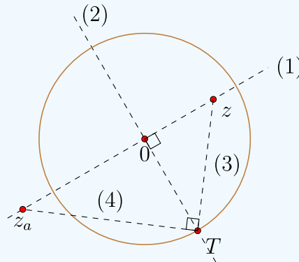
Figure 6.1.3: Constructing the antipodal point to z . (Copyright; author via source)
