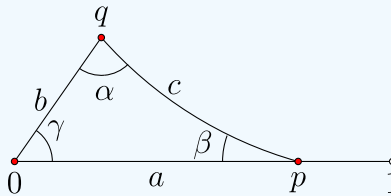
Figure 5.4.9: A hyperbolic triangle with one corner at the origin and one leg on the positive real axis. (Copyright; author via source)
