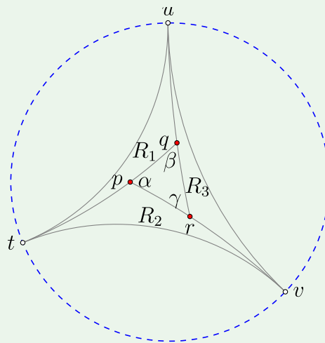
Figure 5.4.3: Determining the area of a hyperbolic triangle. (Copyright; author via source)
