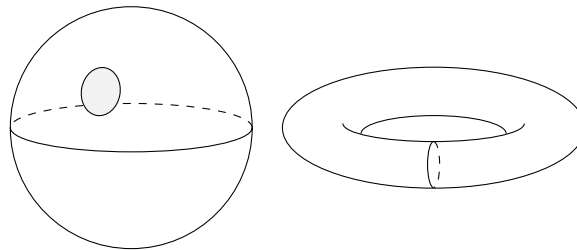
Figure 7.5.1: The sphere and torus are topologically distinct. (Copyright; author via source)
