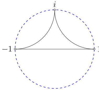
Figure 5.4.2: All ideal triangles are congruent to this one. (Copyright; author via source)
