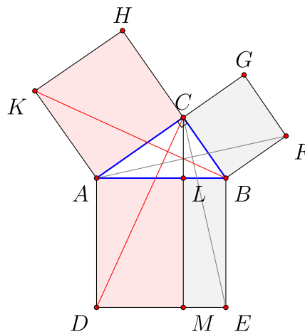
Figure 1.2.1: Proving the Pythagorean theorem. (Copyright; author via source)
