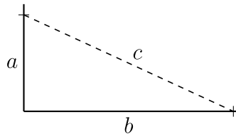
Figure 1.1.1: Measure a , b , and c and check whether a^2 + b^2 = c^2 . If equality holds, the corner is square! (Copyright; author via source)
