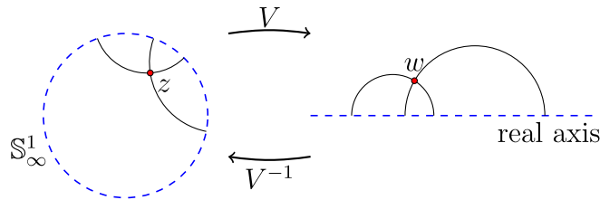
Figure 5.5.2: Mapping the disk to the upper half-plane. (Copyright; author via source)
