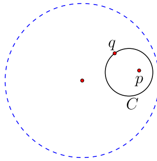
Figure 5.2.4: A hyperbolic circle centered at p through q . (Copyright; author via source)
