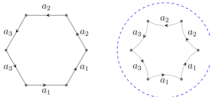
Figure 7.6.1: C_3 admits hyperbolic geometry. (Copyright; author via source)
