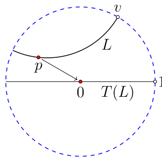
Figure 5.2.2: Any hyperbolic line is congruent to the hyperbolic line on the real axis. (Copyright; author via source)
