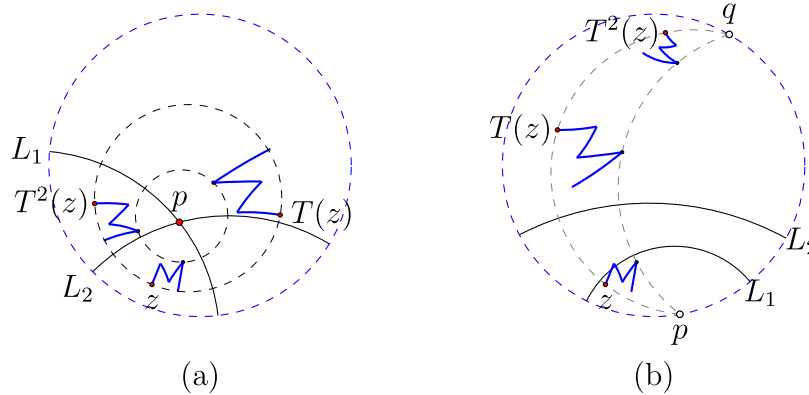
Figure 5.1.4: Moving an 'M' about the hyperbolic plane, by (a) rotation about p ; and (b) translation fixing ideal points p and q . (Copyright; author via source)
