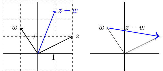
Figure 2.1.1: Complex numbers as vectors in the plane. (Copyright; author via source)
