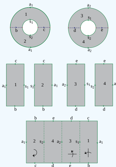
Figure 7.5.13: C_2 is homeomorphic to the Klein bottle K^2 . (Copyright; author via source)
