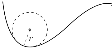
Figure 7.1.1: The curvature of a curve. (Copyright; author via source)
