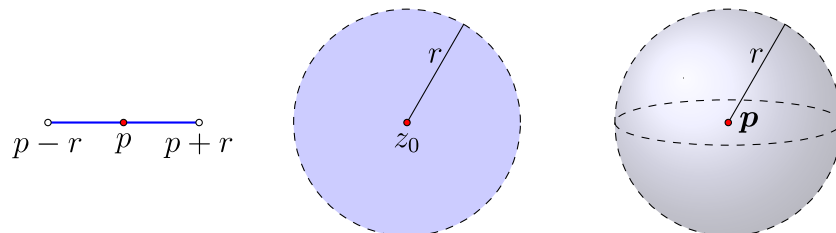
Figure 7.5.2: Open n -balls for n = 1, 2, 3 . (Copyright; author via source)
