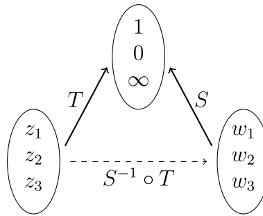
Figure 3.4.2: A schematic for building a Möbius transformation that sends z_i \mapsto w_i for i = 1, 2, 3 . Go through the points 1, 0, \infty . (Copyright; author via source)
