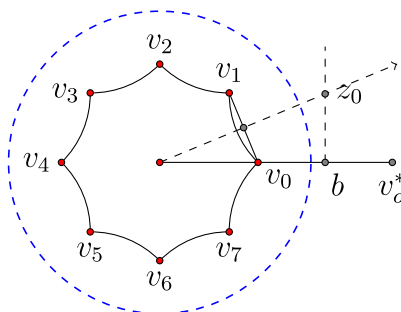
Figure 5.4.8: Building an octagon with interior angles equal to 45^\circ . (Copyright; author via source)
