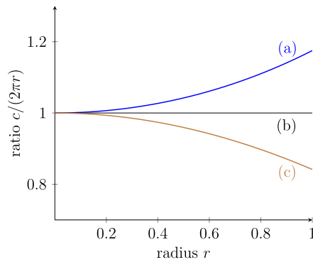
Figure 7.1.3: Plotting the ratio \frac{c}{2\pi r} against r in (a) hyperbolic geometry, (b) Euclidean geometry, and (c) elliptic geometry. (Copyright; author via source)
