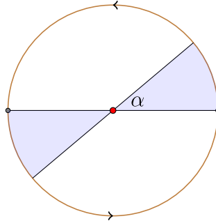
Figure 6.3.4: A lune whose elliptic lines intersect at the origin. (Copyright; author via source)
