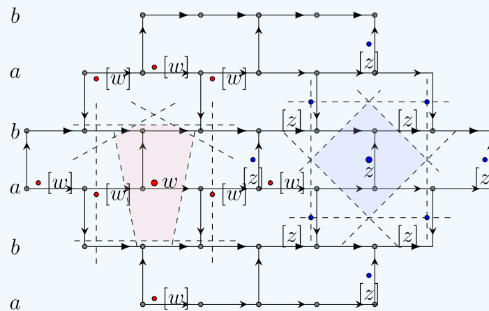
Figure 7.7.5: The Dirichlet domain at a point is obtained by considering perpendicular bisectors with its nearest images, and its shape can vary from point to point, as at points z and w . In the figure all vertically oriented edges are c edges. All horizontally oriented edges in a given row have the same label, either a or b as indicated. (Copyright; author via source)
