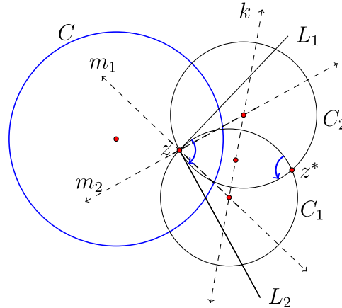
Figure 3.2.2: Inversion in a circle preserves angle magnitudes. (Copyright; author via source)
