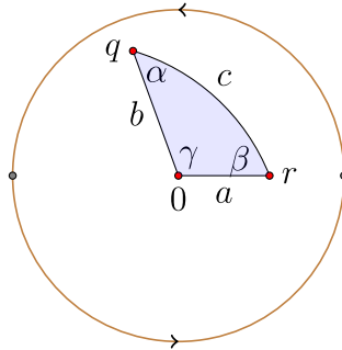
Figure 6.3.5: An elliptic triangle with side lengths and angles marked. (Copyright; author via source)
