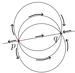
Figure 3.5.5: A hyperbolic Möbius transformation fixing p and q pushes points away from one fixed point and toward the other along type I clines of p and q . (Copyright; author via source)
