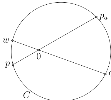
Figure 6.1.2: A cline C containing a pair of antipodal points p and p_a must be a great circle. In the figure, w = q_a . (Copyright; author via source)
