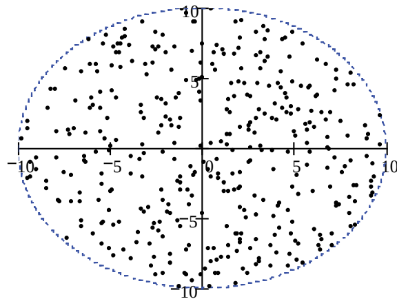
Figure 8.2.3: The positions of N objects in a catalog. (Copyright; author via source)
