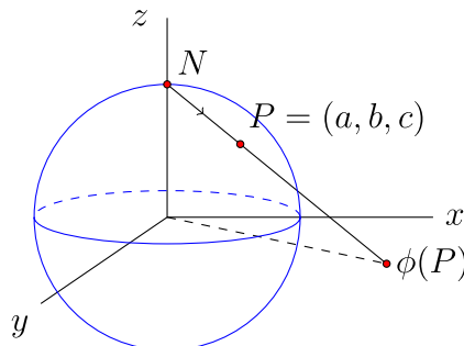
Figure 3.3.1: Stereographic projection. (Copyright; author via source)
