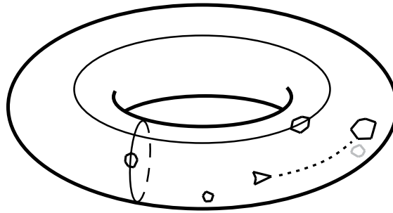
Figure 1.1.3: The video screen in Figure 1.1.2 is equivalent to a torus. (Copyright; author via source)
