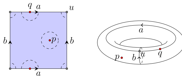
Figure 7.5.3: The flat torus is a 2-manifold as well as a surface (Copyright; author via source)
