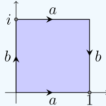
Figure 8.2.7: Building the Klein bottle as a quotient of \mathbb{C} . (Copyright; author via source)
