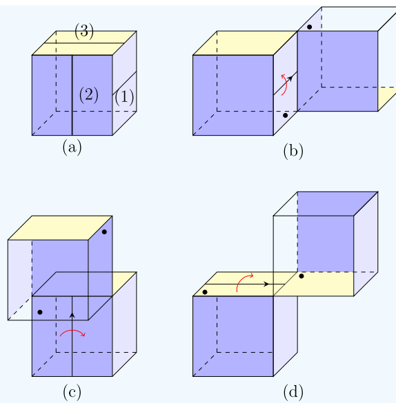
Figure 8.1.2: Describing the Hantzsche-Wendt Manifold via a group of transformations. (Copyright; author via source)
