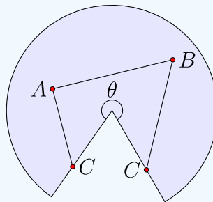
Figure 1.3.4: A triangle on a cone. (Copyright; author via source)
