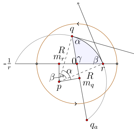
Figure 6.3.6: Deriving the elliptic law of sines. (Copyright; author via source)
