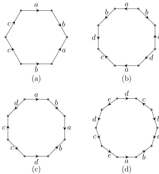
Figure 7.5.12: Four polygonal surfaces. (Copyright; author via source)
