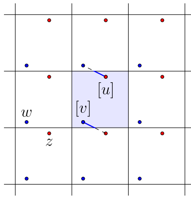
Figure 7.7.2: The distance between two points in the torus viewed as a quotient of \mathbb{C} . (Copyright; author via source)
