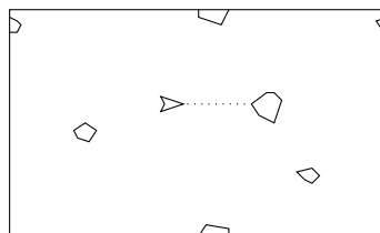
Figure 1.1.2: A finite two-dimensional world with no boundary. (Copyright; author via source)
