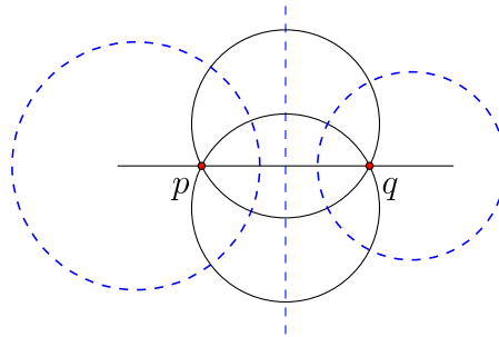
Figure 3.5.1: Type I clines (solid) and Type II clines (dashed) of p and q . (Copyright; author via source)
