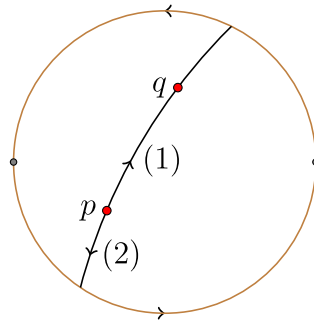
Figure 6.3.1: There is a single elliptic line joining points p and q , but two elliptic line segments. The distance from p to q is the shorter of these two segments. (Copyright; author via source)
