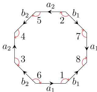
Figure 7.5.11: This cell division of H_2 has a single vertex. (Copyright; author via source)
