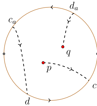
Figure 6.2.1: A leisurely stroll from p to q in the projective plane P^2 . (Copyright; author via source)
