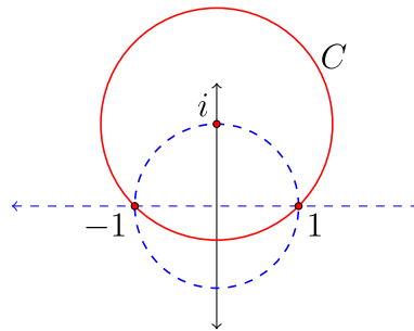
Figure 5.5.1: Inversion in C maps the unit disk to the upper-half plane. (Copyright; author via source)
