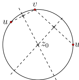
Figure 3.2.1: Constructing the unique circle through three points not on a single line. (Copyright; author via source)
