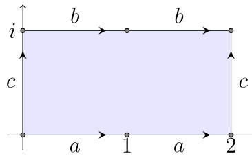
Figure 7.7.4: Building a Klein bottle from a hexagon. (Copyright; author via source)
