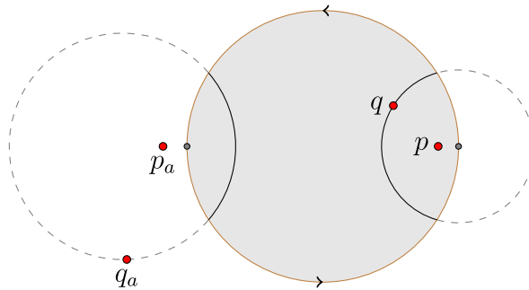
Figure 6.3.2: The elliptic circle centered at p through q in \mathbb{P}^2 may consist of portions of two distinct clines. (Copyright; author via source)
