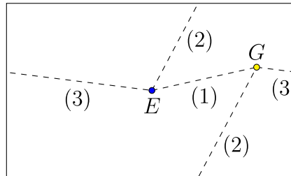
Figure 8.2.1: Seeing multiple images of the same object in the torus. (Copyright; author via source)
