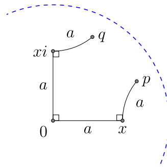
Figure 5.4.5: A journey that would trace a square in the Euclidean plane does not get you home in (\mathbb{D}, \mathcal{H}) . (Copyright; author via source)
