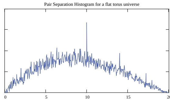
Figure 8.2.6: A pair separation histogram in a torus universe. (Copyright; author via source)
