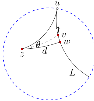
Figure 7.3.1: The angle of parallelism \theta of a point z to a line L . (Copyright; author via source)
