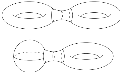
Figure 7.5.5: Some connected sums. (Copyright; author via source)
