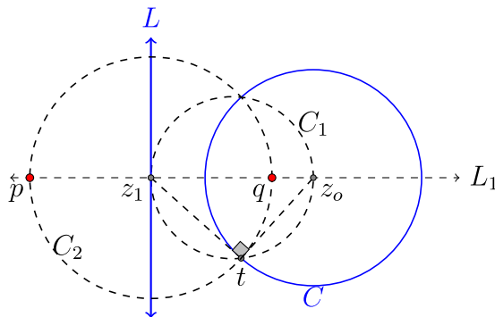
Figure 3.2.5: By inversion we may transform two circles to a circle and a line. (Copyright; author via source)
