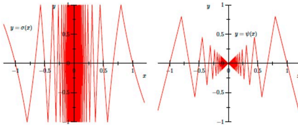
Figure 5.1.2: Graphs of y = \sigma(x) and y = \psi(x)
