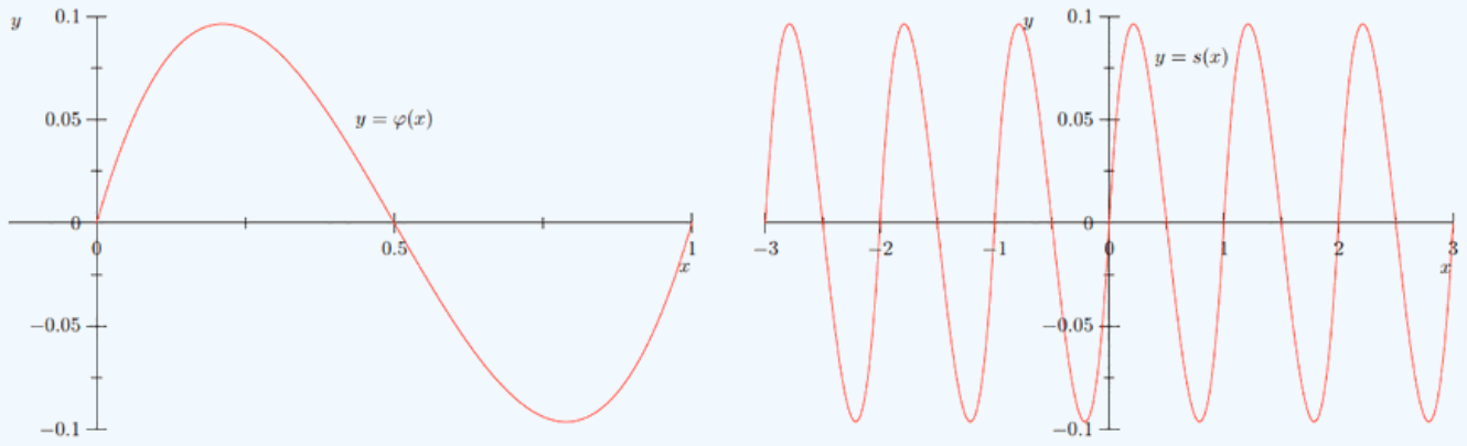
Figure 6.4.1: Graphs of y = \varphi(x) and y = s(x)
