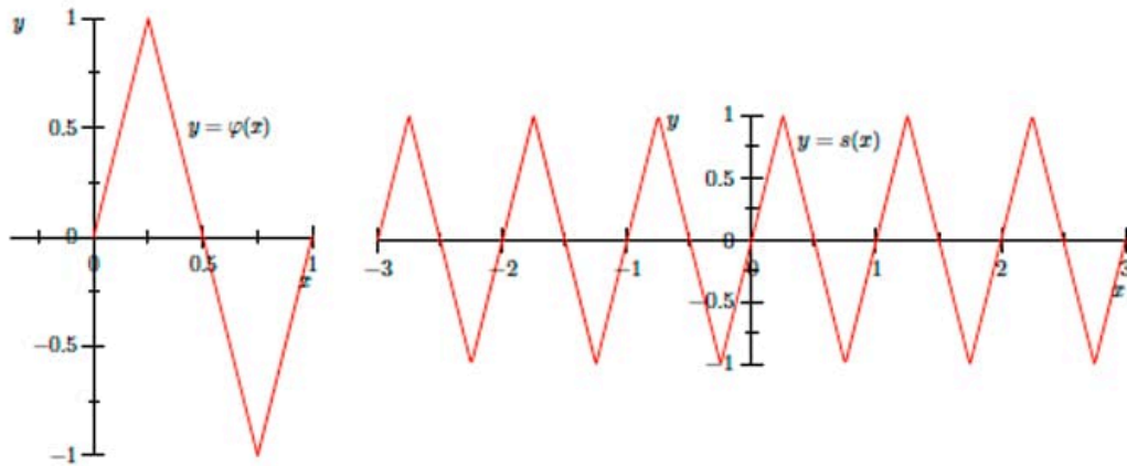
Figure 5.1.1: Graphs of y = \varphi(x) and y = s(x)
