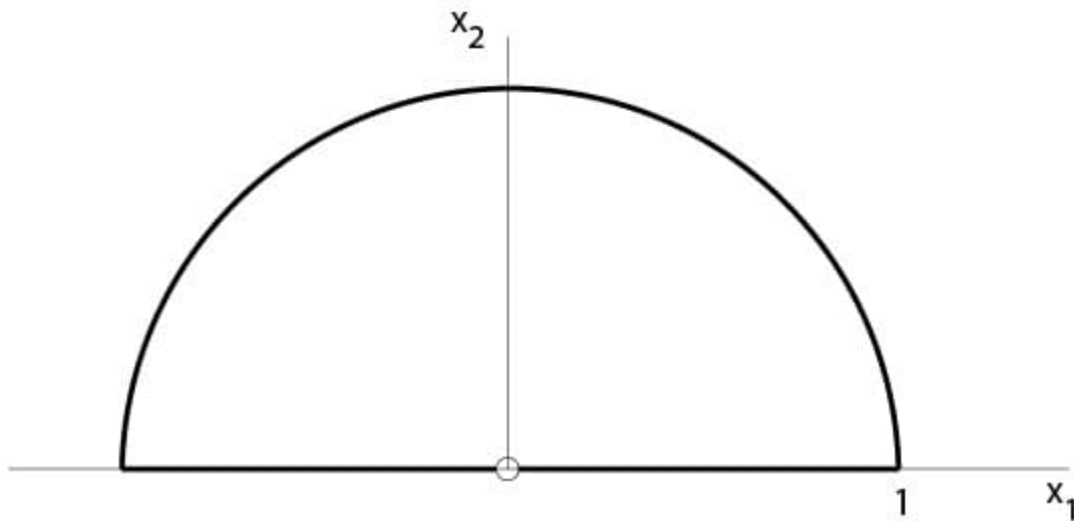
Figure 7.3.1.1: Counterexample
