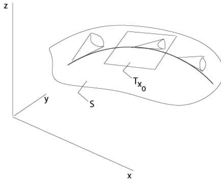
Figure 2.3.4: Monge cones along a curve on the surface
