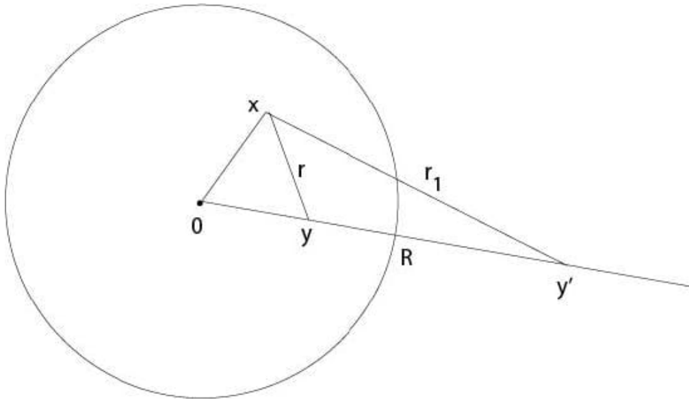
Figure 7.4.1.1: Reflection on \partial B_R(0)
