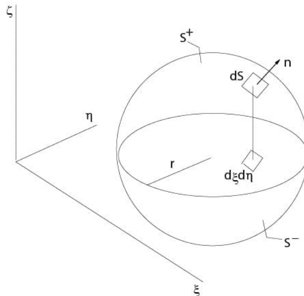
Figure 4.2.2.1: Domains of integration
