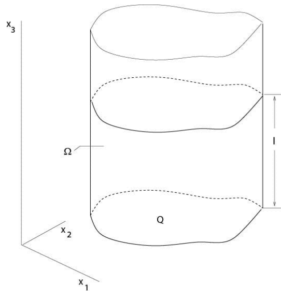
Figure 6.4.1.1: Diffusion in a tube
