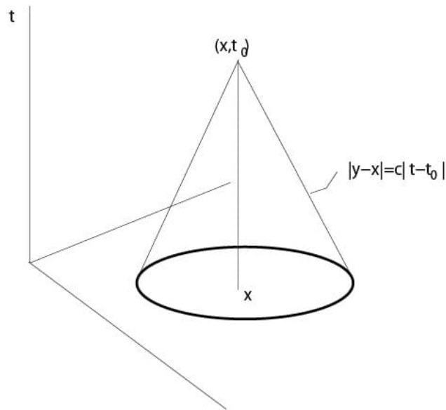
Figure 4.2.1.2: Domain of dependence, case n = 3 .
