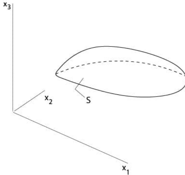
Figure 3.1.2: Transformed flat manifold \mathcal{S}
