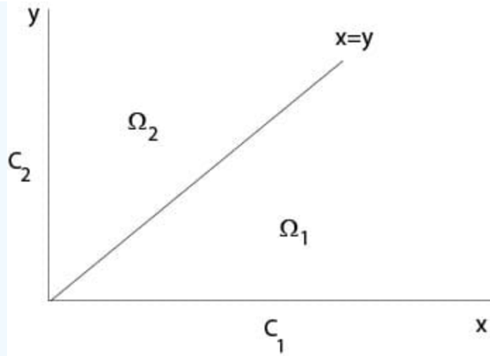
Figure 2.2.2.4: Domains to the chemical kinetics example
