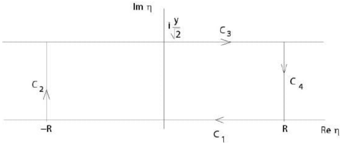
Figure 5.1.1: Proof of (5.1.12)
