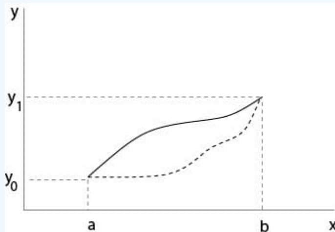
Figure 1.2.1.1: Admissible Variations
