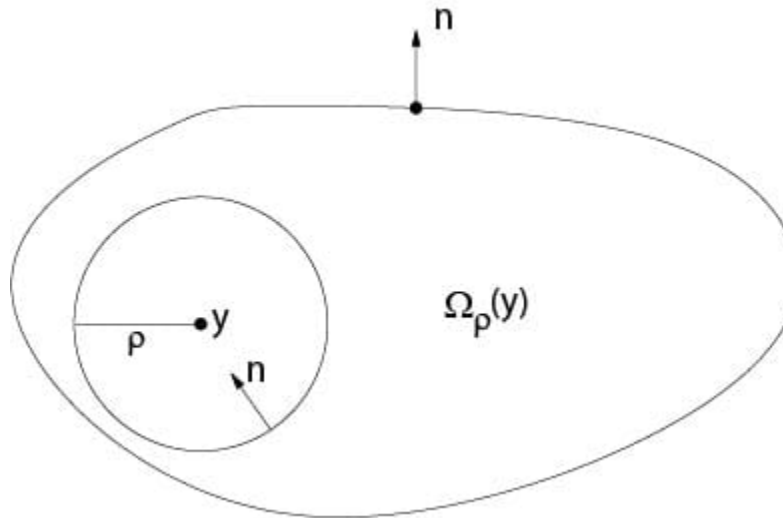
Figure 7.2.2: Notations to Theorem 7.1
