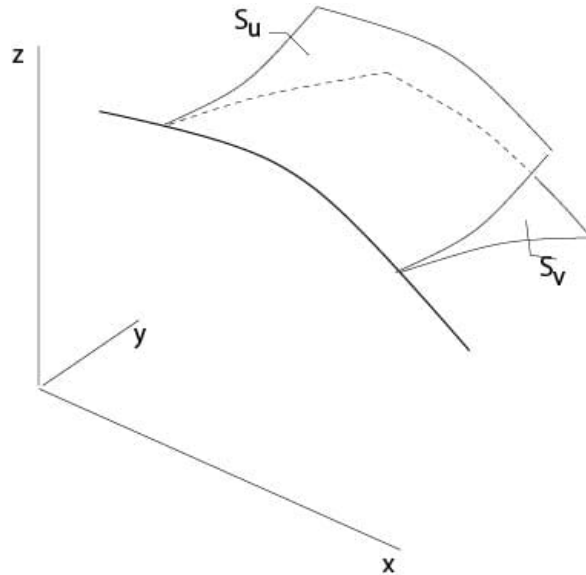
Figure 2.2.2.3: Multiple solutions
