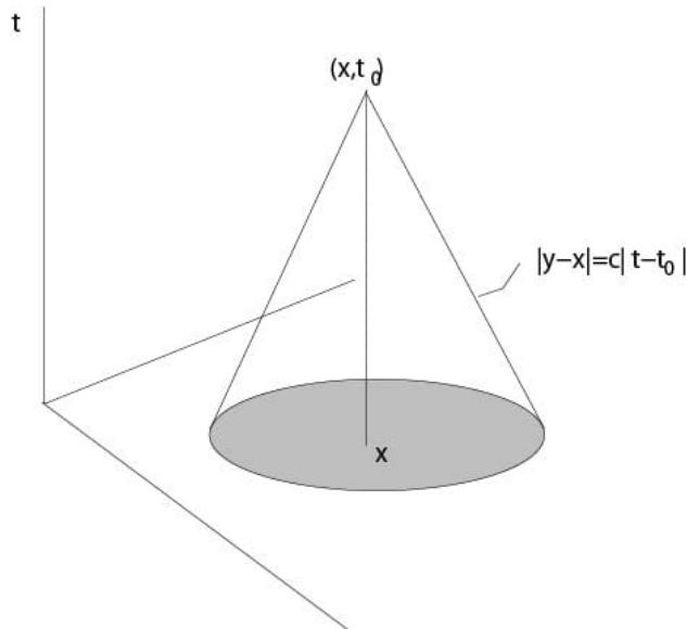
Figure 4.2.2.2: Interval of dependence, case n = 2
