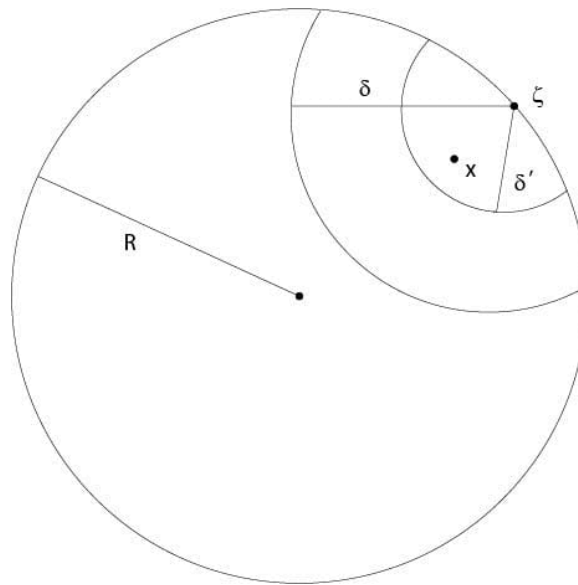
Figure 7.4.1.2: Proof of Theorem 7.2
