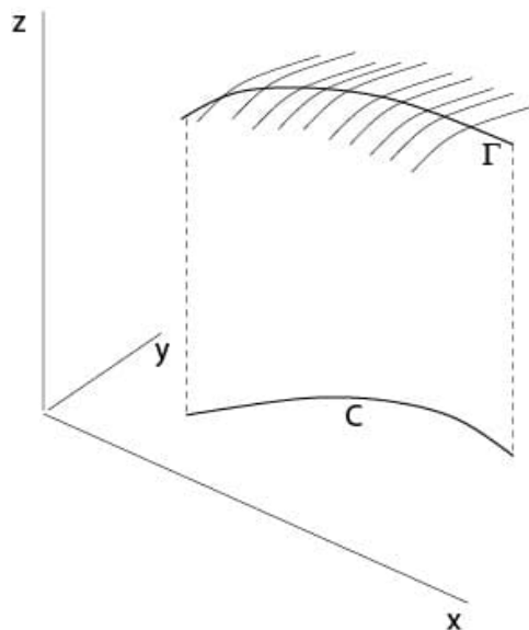
Figure 2.2.2.1: Cauchy initial value problem
