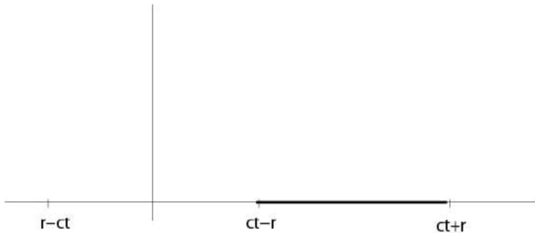
Figure 4.2.1.1: Changed domain of integration
