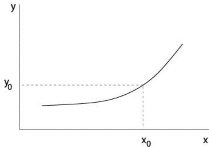
Figure 1.0.1: Initial value problem
