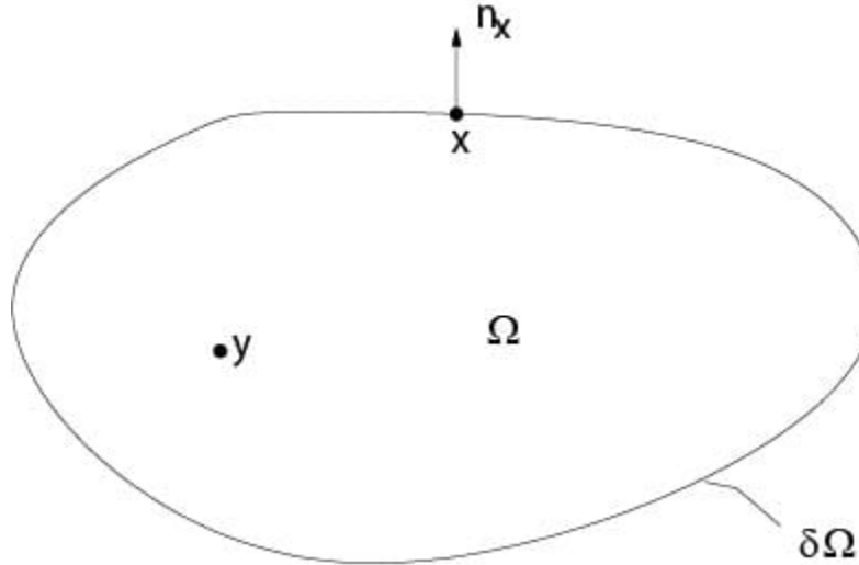
Figure 7.2.1: Notations to Green's identity
