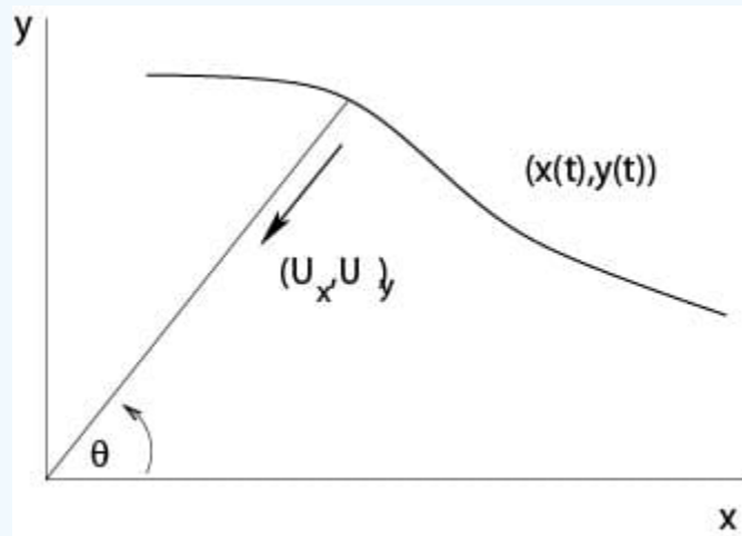
Figure 2.5.1: Motion in a central field
