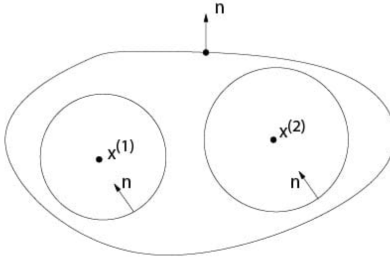
Figure 7.4.1: Proof of Proposition 7.7
