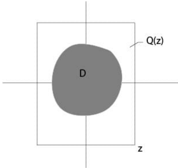
Figure 3.5.1.1: Definition of D^{\text{int}} Q(z)
