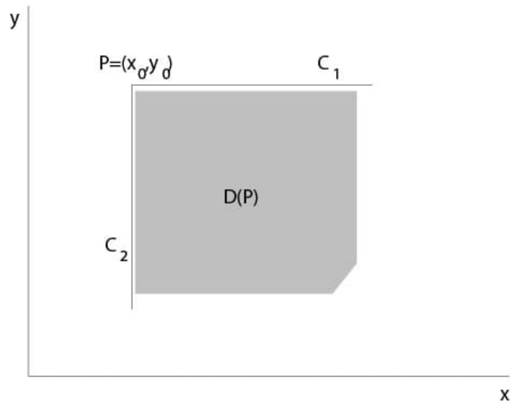
Figure 4.4.2: Definition of Riemann's function
