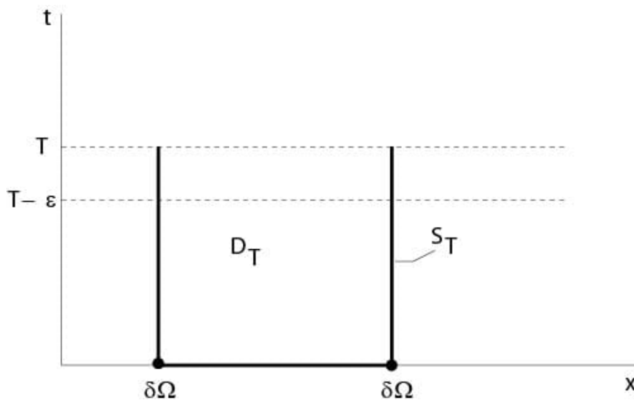
Figure 6.3.1: Notations to the maximum principle
