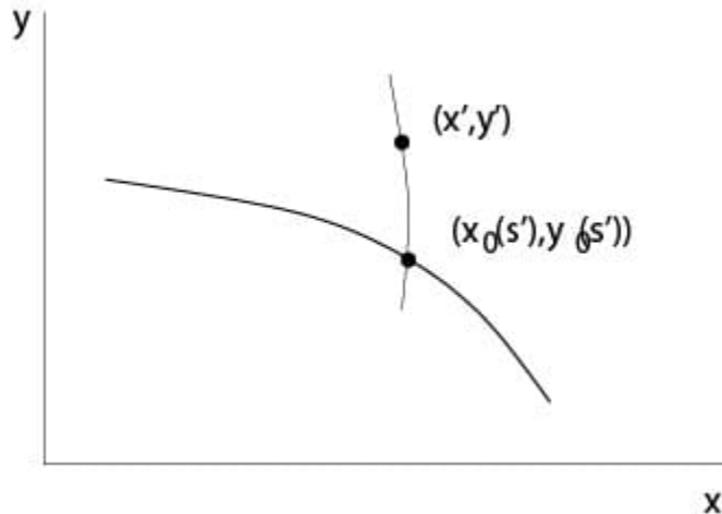
Figure 2.2.2.2: Uniqueness proof
