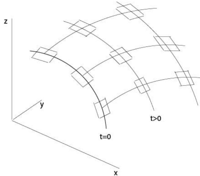
Figure 2.3.1.1: Construction of the solution
