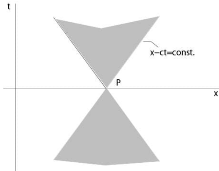
Figure 4.2.1: Domain of influence
