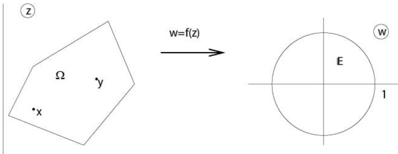
Figure 7.4.2.1: Conformal mapping
