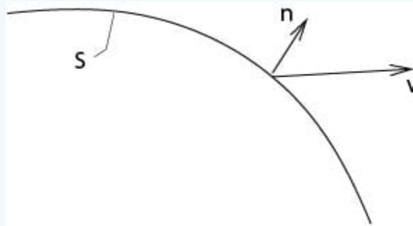
Figure 3.3.1.3: Definition of relative speed
