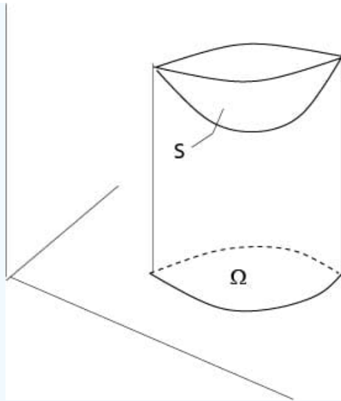
Figure 1.2.2.1: Comparison surface
