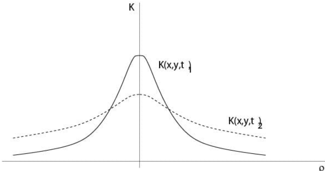
Figure 6.1.1: Kernel K(x, y, t) , \rho = |x - y| , t_1 < t_2
