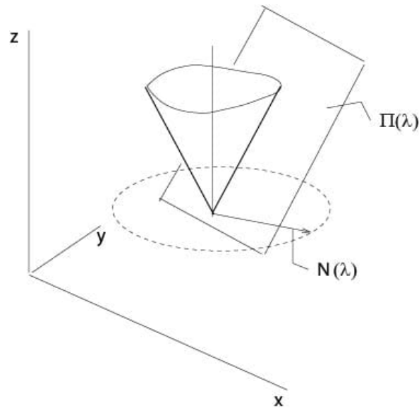
Figure 2.3.2: Monge cone in an example
