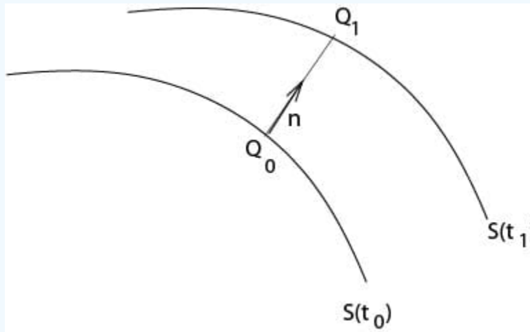
3.3.1.2: Definition of the speed of a surface
