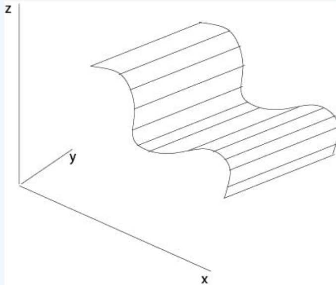
Figure 2.1.2: Cylinder surfaces
