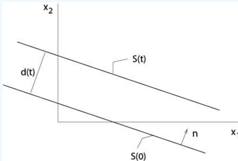
Figure 3.3.1.1: d'(t) is the speed of plane waves
