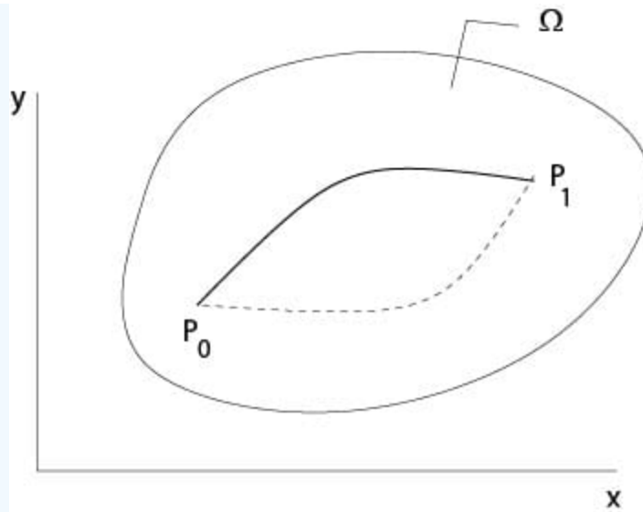
Figure 1.1.1: Independence of the path
