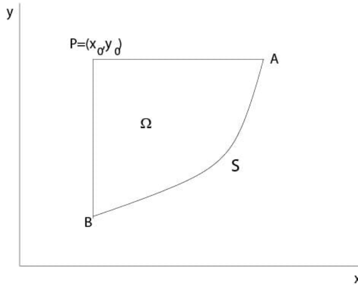
Figure 4.4.1: Riemann's method, domain of integration
