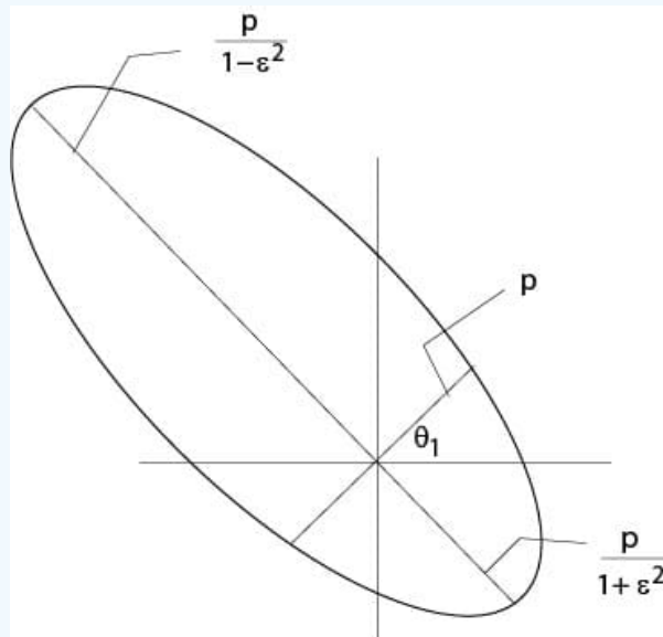
Figure 2.5.2: The case of an ellipse
