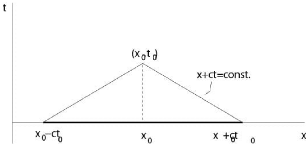
Figure 4.1.1: Interval of dependence
