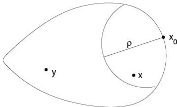
Figure 7.5.1: Proof of Theorem 7.3
