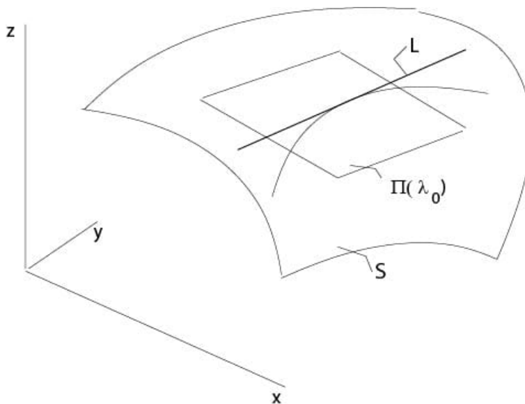
Figure 2.1.1: Curve on a surface
