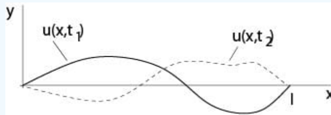
Figure 1.1.2: Oscillating string
