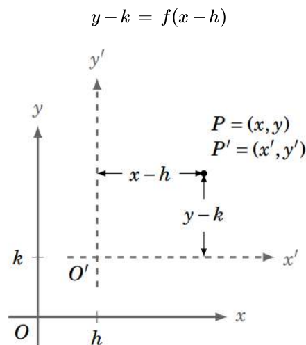
Figure 7.4.1: Translation
