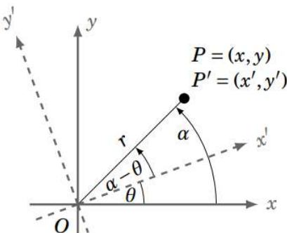
Figure 7.4.3: Rotation
