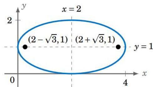
Figure 7.4.2: Ellipse \frac{(x-2)^2}{4} + (y-1)^2 = 1
