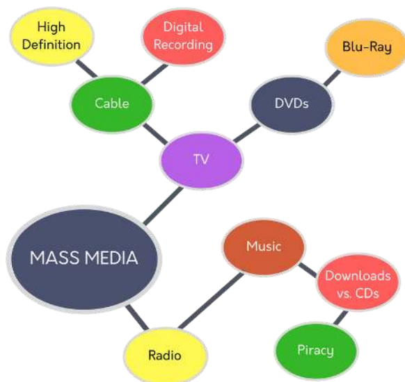
Figure 4.2 Clustering
