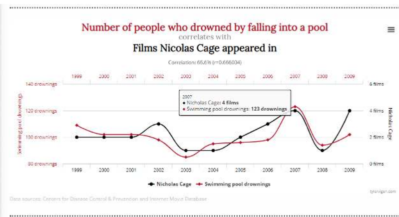
Fig 4.5 Drownings correlate to Nicolas Cage Films. Source: Spurious correlations: http://www.tylerlervigen.com/spurious-correlations
