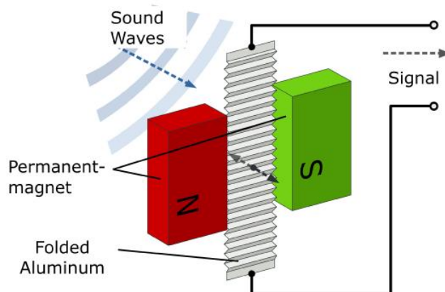
Figure 10.2.7: A folded piece of thin metal (the ribbon) is suspended between two magnets. When sound waves move the ribbon, an audio signal is created. (CC BY-SA 3.0; Arne Nordmann (norro) via Wikimedia Commons )
