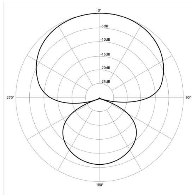
Figure 10.2.2.4: Hypercardioid polar pattern. (CC BY-SA 3.0; Galak76 via Wikimedia Commons)
