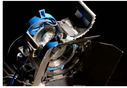
Figure 9.4.2: Fresnel light open.
