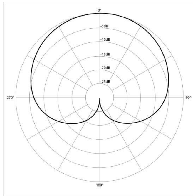
Figure 10.2.2.2: Cardioid polar pattern. (CC BY-SA 3.0; Galak76 via Wikimedia Commons)
