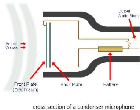
Figure 10.2.4: Two plates are charged with electricity (from a battery or phantom power). When sound moves the diaphragm, the space between the plates creates an audio signal. (CC BY-SA 3.0; Jim Dearden via Stack Exchange)
