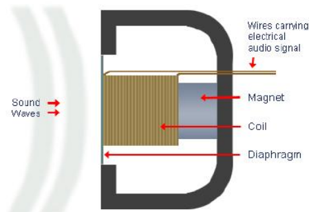
Cross-Section of Dynamic Microphone
