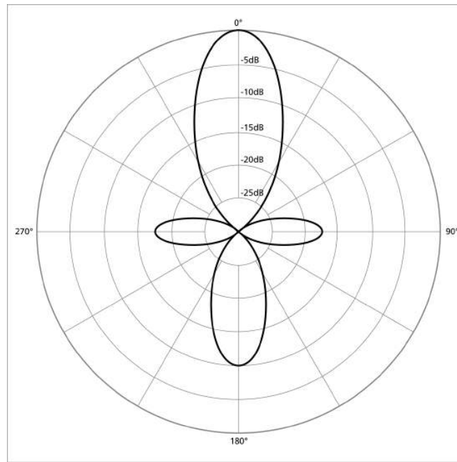
Figure 10.2.2.6: Shotgun microphone polar pattern. (CC BY-SA 3.0; Galak76 via Wikimedia Commons)
