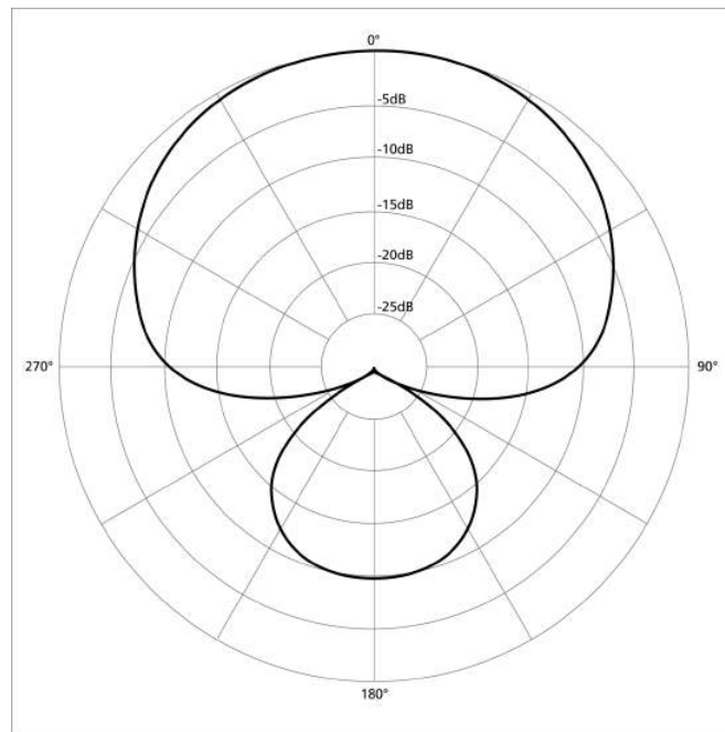
Figure 10.2.2.3: Supercardioid polar pattern. (CC BY-SA 3.0; Galak76 via Wikimedia Commons)
