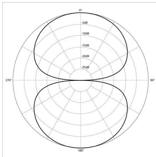
Figure 10.2.2.5: Bidirectional (or Figure 8) polar pattern. (CC BY-SA 3.0; Galak76 via Wikimedia Commons)
