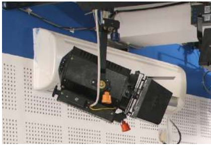
Figure 9.4.1: Fresnel Light.
