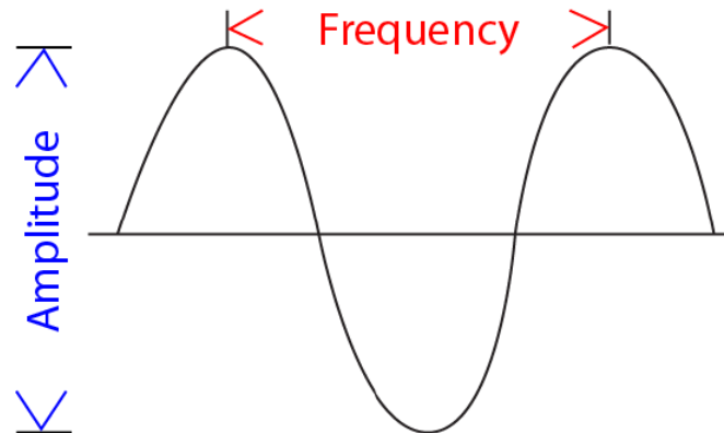
Figure 10.1.1: Amplitude and Frequency. ( CC0 1.0 Universal Public Domain Dedication ; Justin Evans via Wikimedia Commons )
