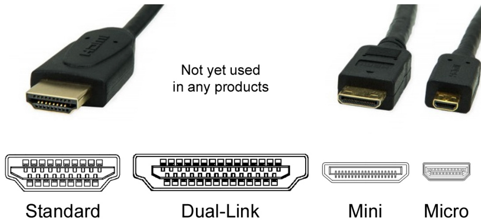
Figure 10.3.5: HDMI connectors in Standard, Mini, and Micro sizes.
