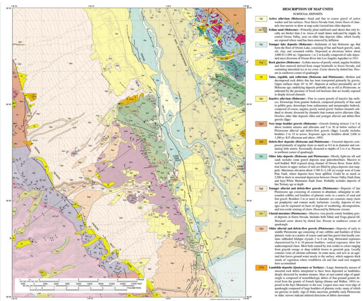
Figure 12.15: Geologic Map for Mount Whitney, California (USGS). Image is in the public domain.
