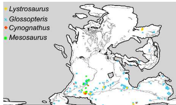
Figure 4.2: Distribution of Four Fossil Groups During the Super Continent Gondwanaland. Image by Wikimedia is licensed under the CC-BY-SA 4.0 license .
