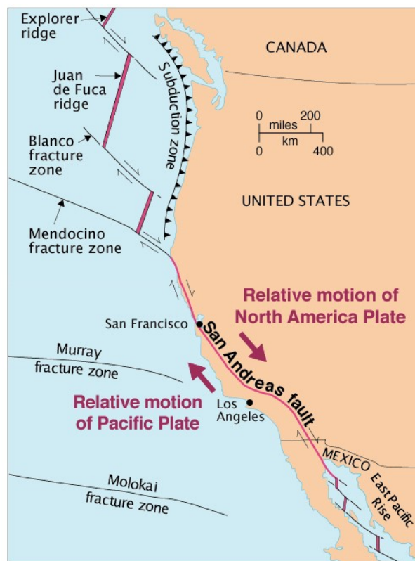
Figure 2.10: The San Andreas Fault. Image by the USGS is in the public domain.
