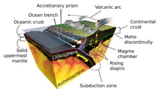
Figure 10.5: Diagram of the Geologic Process of Subduction. Subduction-en.svg from Wikimedia Commons by K. D. Schroeder is licensed under CC BY SA 4.0
