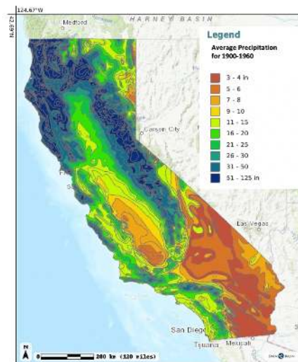
Figure 3.3: California's Annual Precipitation for 1900-1960. Image by Jeremy Patrich is used under a CC-BY 4.0 license .
