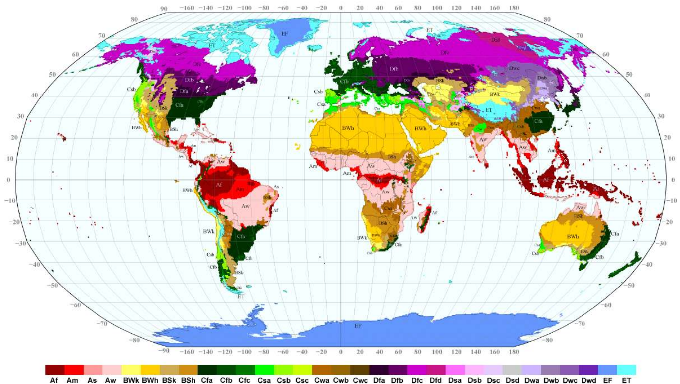
Figure 3.6: Köppen-Geiger Climate Subdivisions. Köppen-Geiger Climate Subdivisions Köppen and Geiger further divided each major division (A, B, C, D, E, F, H) into smaller groups based upon precipitation and temperature patterns. Image by NOAA is in the public domain.
