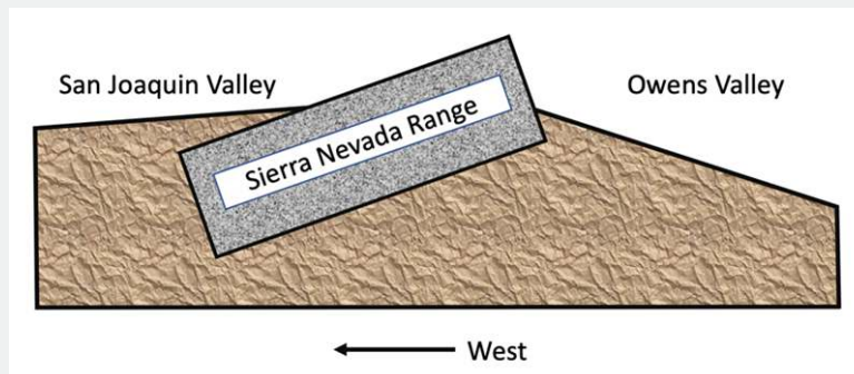
Figure 12.14: Schematic of the Sierra Nevada Fault Block. Image by Jeremy Patrich is licensed under CC-BY 4.0 .
