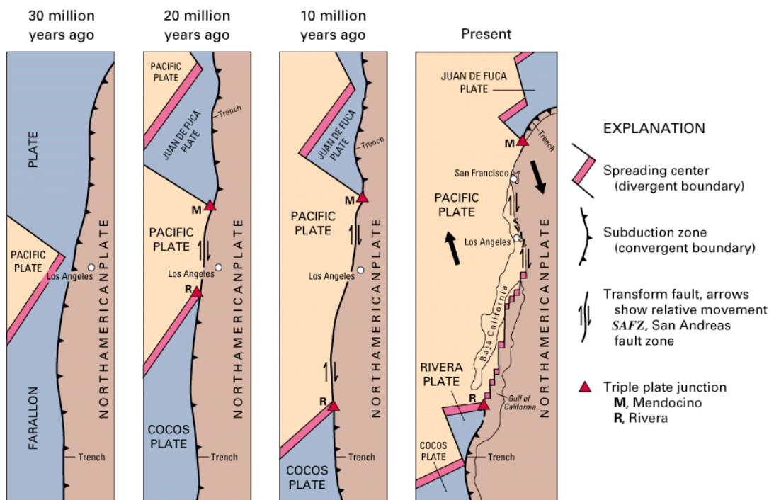
Figure 2.5: Illustrating the Shrinking of the Farallon Plate Beneath the North American & Caribbean Plates. Image is used under a CC-BY 4.0 license.
