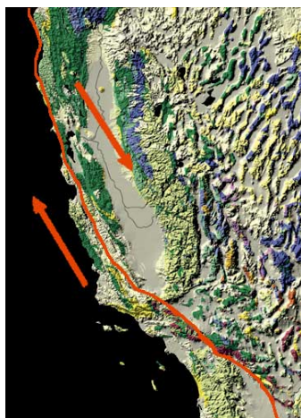
Figure 13.11: The San Andreas Fault & General Direction of Plate Movement. Image by Wikipedia is in the public domain.
