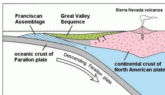
Figure 11.13: Image of Deposition in the Great Valley Sequence. Image is in the public domain.
