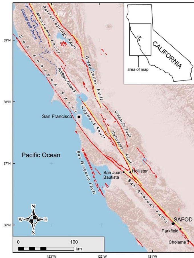
Figure 2.7: Map of Central & Northern California's Faults. Image is in the public domain.
