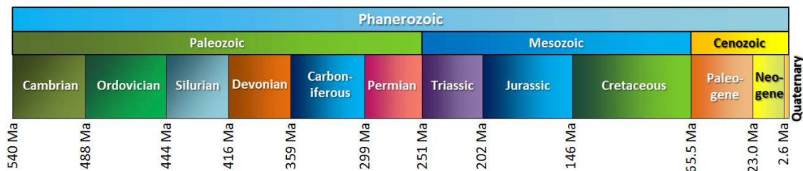
Figure 2.3: The Eras and Periods of the Phanerozoic. Image is used under a CC-BY 4.0 license.
