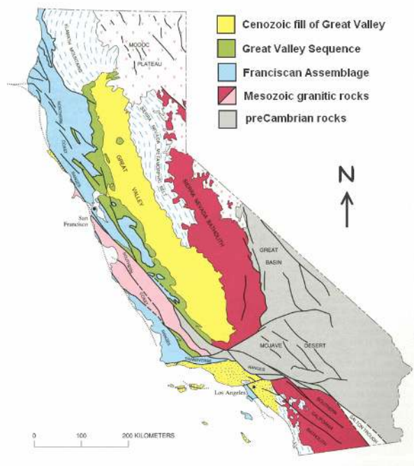
Figure 11.12: Geologic Map of the Great Valley Sequence. Image is in the public domain.
