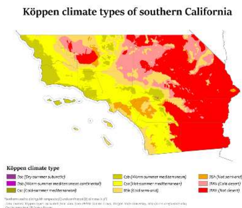
Figure 13.2 Köppen Climate Types of Southern California. Image by Wikipedia is licensed under CC BY-SA 4.0 .
