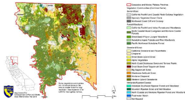
Figure 8.8: Map of the Cascade & Modoc Plateau. Image by USGS and CDFW is licensed under public domain.
