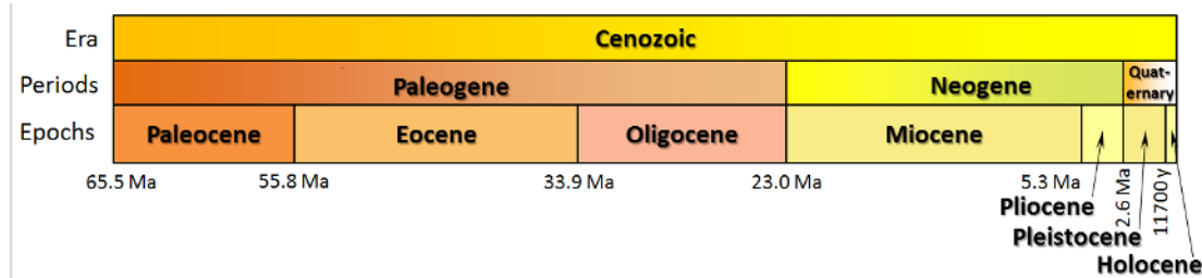
Figure 2.4: The Periods and Epochs of the Cenozoic. Image is used under a CC-BY 4.0 license.
