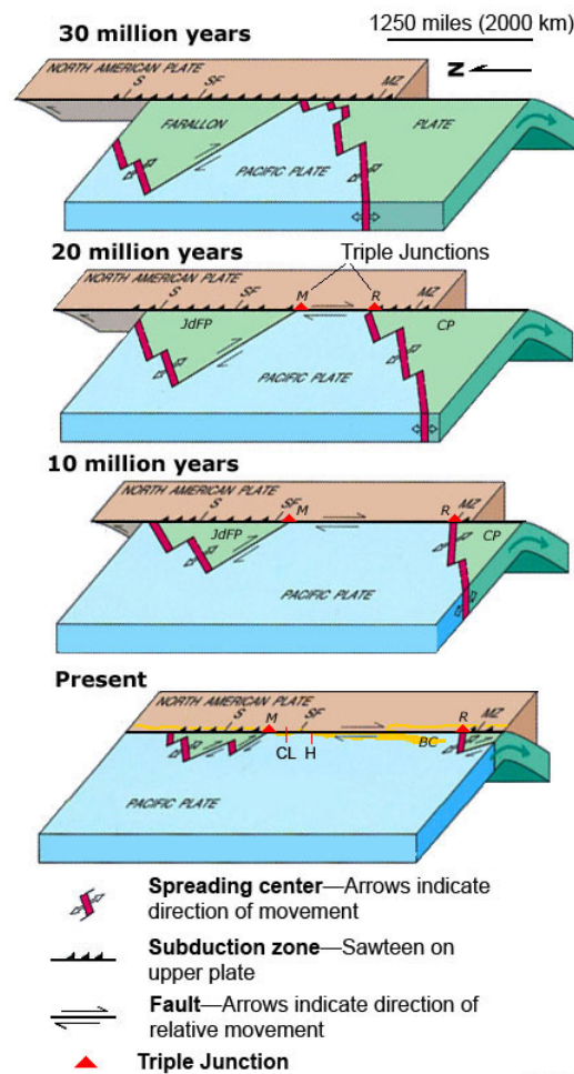
Figure 2.11: Assembling California Over the Past 30 Million Years. Image by the USGS is in the public domain.
