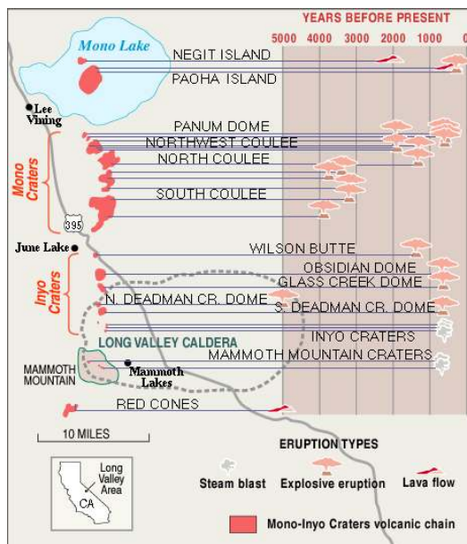
Figure 12.9: Map of Volcanoes Between Mono Lake & the Long Valley Caldera. Image is in the public domain.
