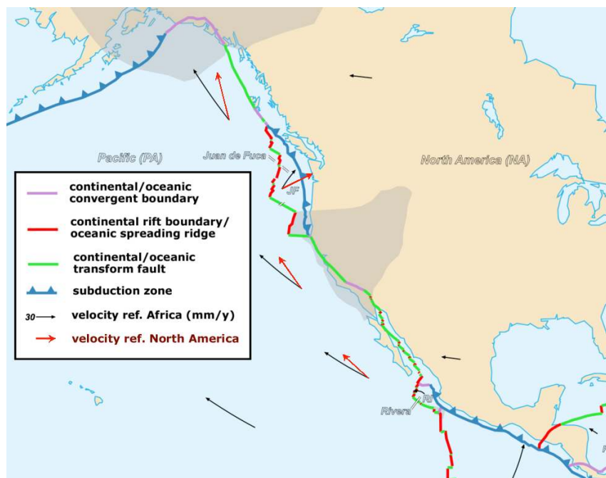
Figure 2.6: Relative Plate Motions of Western Portion of North America. Image is used under a CC BY-SA 3.0 license.
