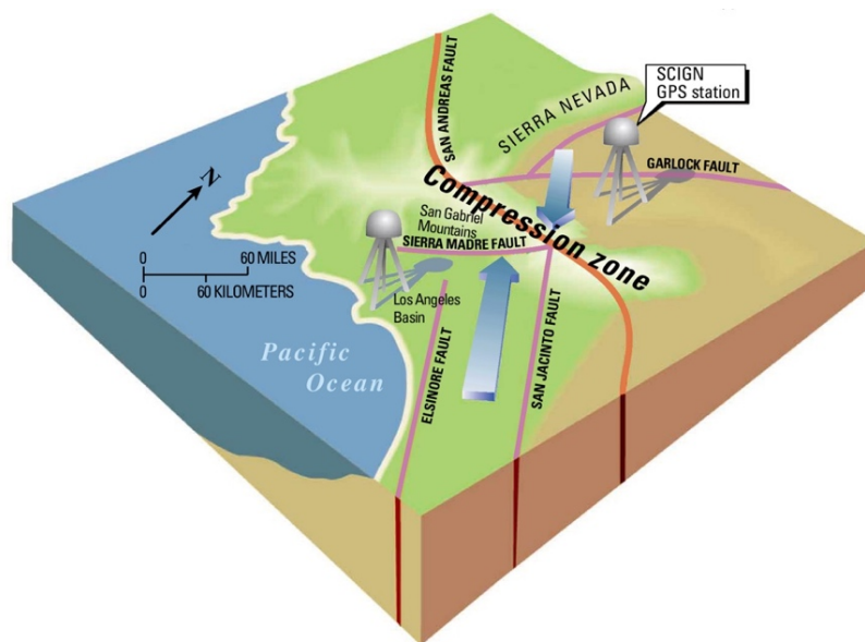
Figure 2.8: Model of Southern California Showing the Motion of the Pacific & North American Plates. Graphic by the USGS is in the public domain.
