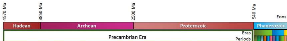
Figure 2.2: The Eons of Earth's History. Image is used under a CC-BY 4.0 license.
