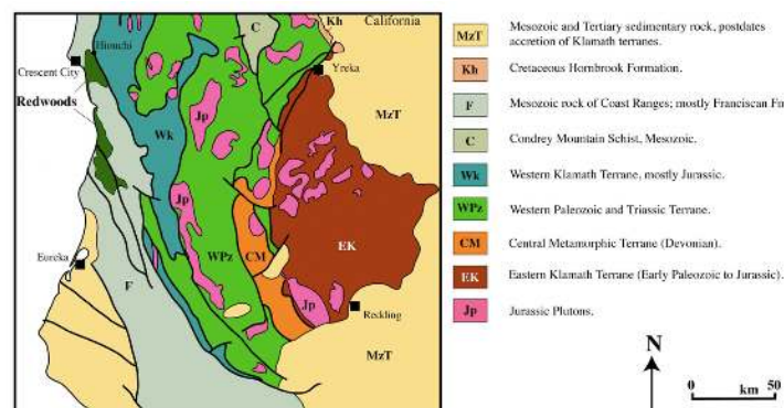
Figure 8.4: Geologic Map of the Klamath Mountains Region- California. Image by M.B. Miller is used by USDA and is in the public domain.
