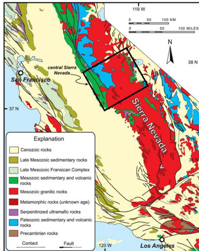
Figure 10.4: Geologic Map of The Sierra Nevada & Surrounding Areas. Image by California Geological Survey is licensed under USGS.
