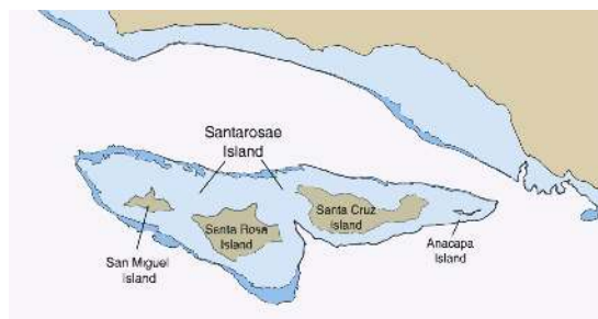
Figure 4.5: A Map of Santarosae Island, around 15,000 years ago, which today makes up the Channel Islands, California. Image by University of Nebraska, Lincoln Digital Commons is in the public domain.
