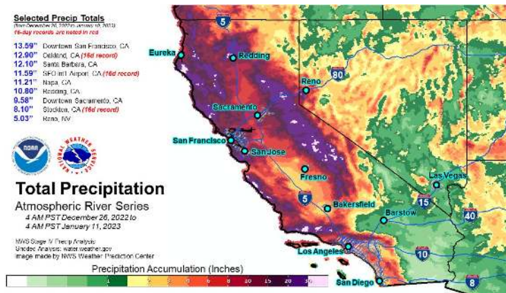
Figure 3.9: Precipitation Totals from December 26 th - January 10 th , 2023. Image by NOAA is in the public domain.
