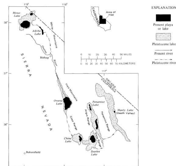
Figure 12.23: Map Showing the System of the Pleistocene Lakes in Eastern California. Image is in the public domain.
