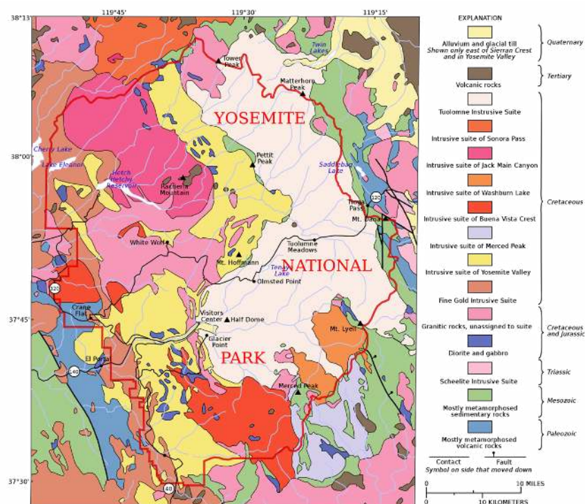
Figure 10.6: Geologic Map of Yosemite National Park- California. Image by United States Geological Survey, remixed by Grandiose, licensed under CC BY-SA 3.0
