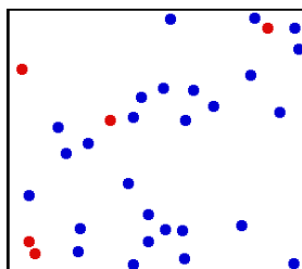
Figure 1.4.4: Animation of molecular motions in an ideal gas. From en.wikipedia.org .
