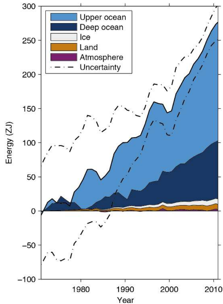
Figure 1.6.13: Changes in Earth's Heat Content.
