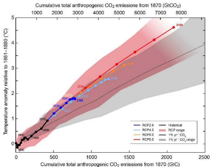
Figure 1.8.9). Colored lines show multi-model means from the RCP scenarios and colored plume indicates uncertainties. Results from exponential CO 2 increase experiments at a rate of 1% per year are shown as the black line and grey shading. RCP scenarios lead to somewhat larger warming because they include additional non-CO 2 forcings. From ipcc.ch .
