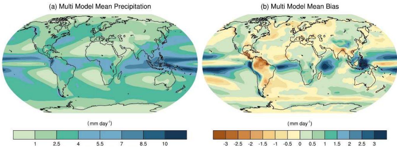
Figure 1.7.4: As Figure 1.7.3 but for annual mean precipitation.
