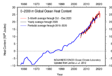
Figure 1.2.8: Observational estimates of global ocean heat content (0-2 km) from NOAA. From 1960 to 2005 ocean temperatures were measured mainly using research ships (blue line). Since 2005 autonomous ARGO floats have increased the data density both in space and time (red and black lines).
