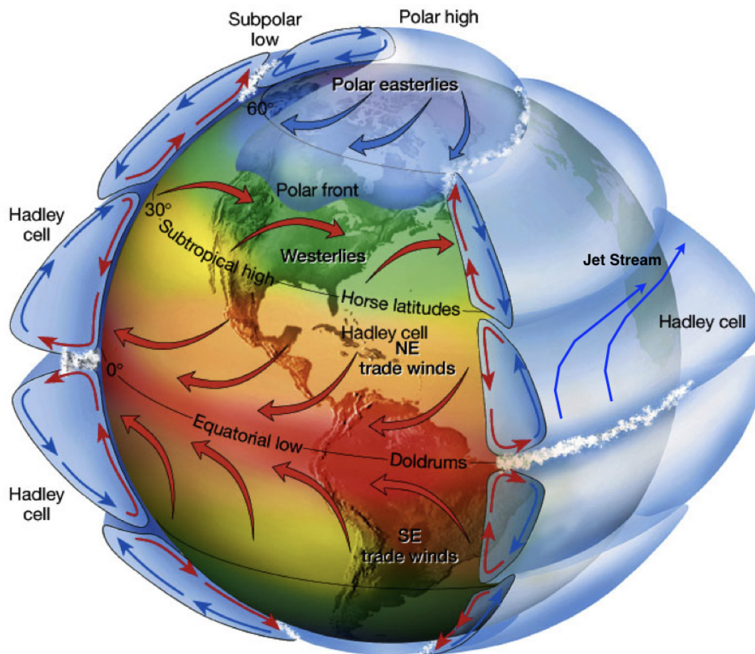
Figure 1.6.7: Atmospheric Circulation on a Rotating Earth. Modified from ux1.eiu.edu .
