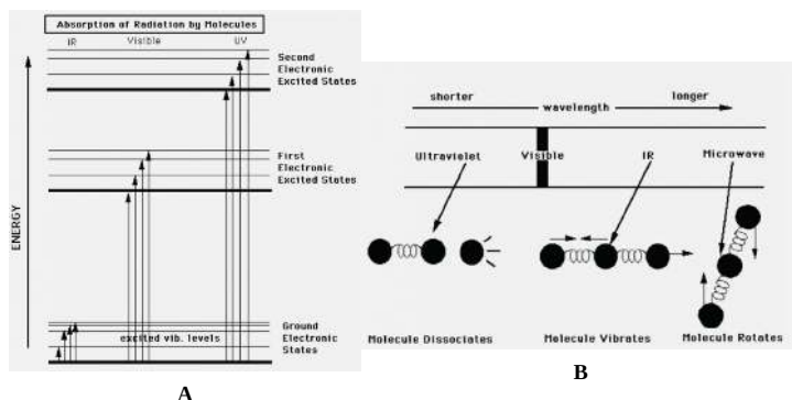
Figure 1.4.2: Interactions of electromagnetic radiation with molecules. A: Absorption of a high-energy photon with an ultraviolet or visible wavelength can lead to excited electronic states. Each excited electronic energy state has sub-states with different vibrational levels. Absorption of a lower energy, infrared photon can excite a vibrational level without changing the electronic state. B: Absorption of low-energy photons at microwave or infrared wavelengths can lead to rotation or vibration of molecules, whereas high-energy photons at ultraviolet wavelengths can break apart molecules. From wag.caltech.edu.
