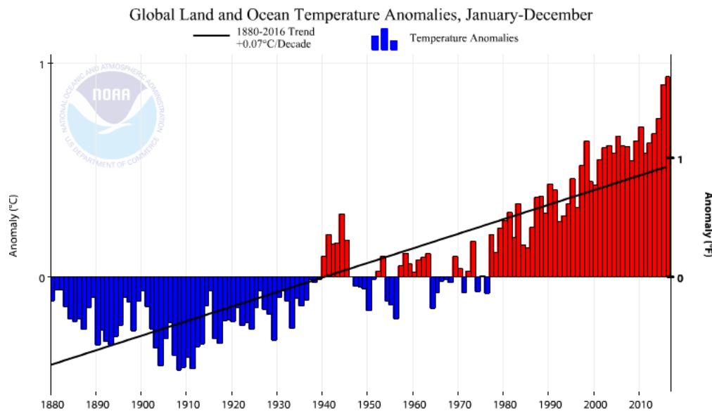
Figure 1.1.2: Averaged over land and ocean the increase in Earth's temperature over the past 100 years has been approximately 0.7°C (0.07°C/decade). This result is very robust. Several groups around the world have analyzed the available data in different ways and came to the same conclusion. This is a key figure.
