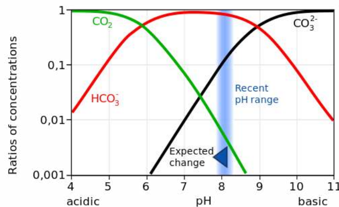
Figure 1.5.10: Ratios of carbonate species concentrations as a function of the pH. Currently average seawater has a pH of about 8.1. Therefore most carbon in the ocean is in the form of bicarbonate. Addition of anthropogenic \text{CO}_2 decreases the pH. From Wikipedia.org .
