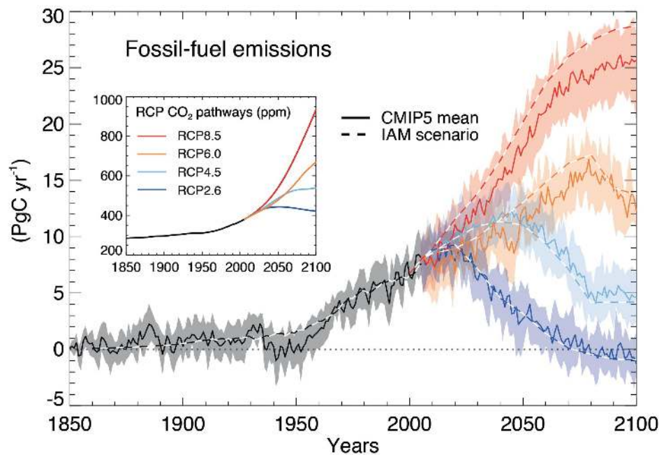
Figure 1.8.2: Evolution of CO 2 emissions and concentrations (inset) for RCP scenarios. Emissions are calculated from simple carbon cycle box models given the CO 2 concentrations. Uncertainties in these calculations are indicated by the shading and the two different lines labeled CMIP5 mean and IAM scenario. From ipcc.ch .
