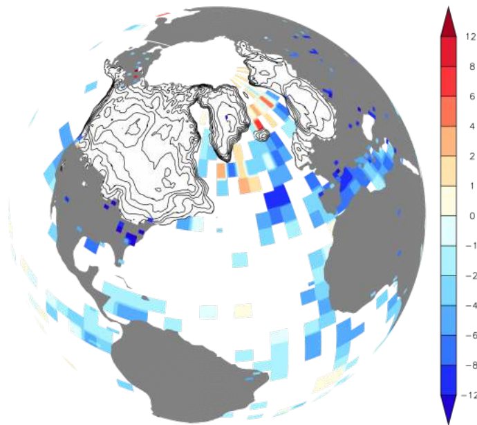
Figure 1.3.10: Reconstructions of ice sheets (contour lines show 500 m elevation differences) and surface temperature differences from modern (color scale in K) for the Last Glacial Maximum. From PAGES news.
