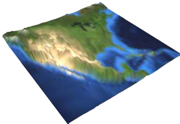
Figure 1.7.2: Illustrations of land surfaces (green and brown colors) and sea floor (blue) at fine (top; ~10 km) and coarse (bottom; ~100 km) resolution. Note that the elevations and depths are strongly exaggerated with respect to horizontal distances. From ucar.edu .
