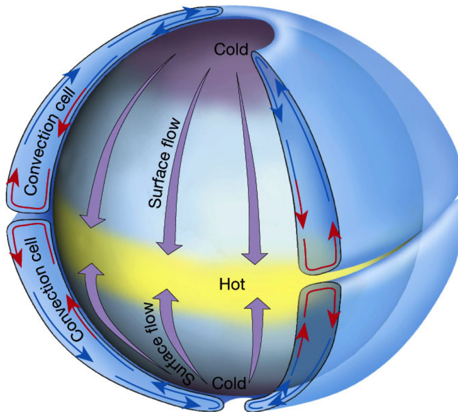
Figure 1.6.6: Atmospheric Circulation on a Non-Rotating Earth. Figure 7.5 in The Atmosphere , 8th edition, Lutgens and Tarbuck, 8th edition, 2001. From ux1.eiu.edu .
