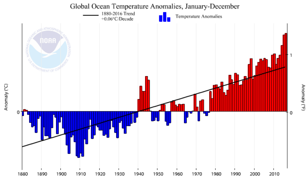
Figure 1.1.11: Averaged over the global ocean the year-to-year variations are still smaller ( \sim 0.5^{\circ}\text{C} ) than over land and the trend is also smaller ( 0.06^{\circ}\text{C}/\text{decade} ).
