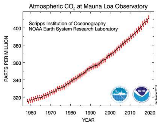
Figure 1.2.10: Atmospheric CO 2 measured at Hawaii's Mauna Loa Observatory. The measurements were pioneered by Charles Keeling from Scripps Institution of Oceanography in 1958. From noaa.gov .
