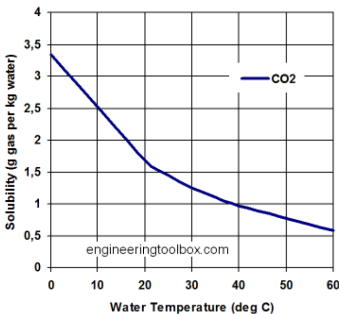
Figure 1.5.9: Solubility of \text{CO}_2 in water. From engineeringtoolbox.com .
