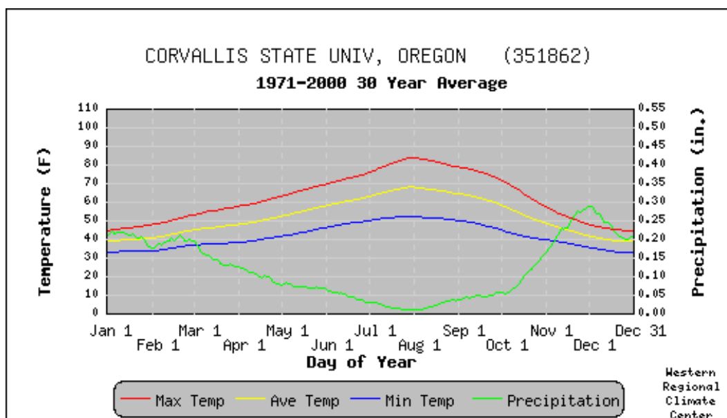
Figure 1.1.5: Climatology of temperature and precipitation in Corvallis, Oregon. The difference between the red and blue curve denotes the average diurnal cycle.
