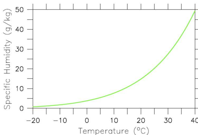
Figure 1.4.16: The Clausius-Clapeyron relation describes the amount of water vapor (in g water per kg of moist air) that air at saturation can hold as a function of temperature. All points along the green line represent 100% relative humidity. The lower a point is below the green line the lower its relative humidity will be. E.g. a point half way between the green line and the zero line would have 50% relative humidity.
