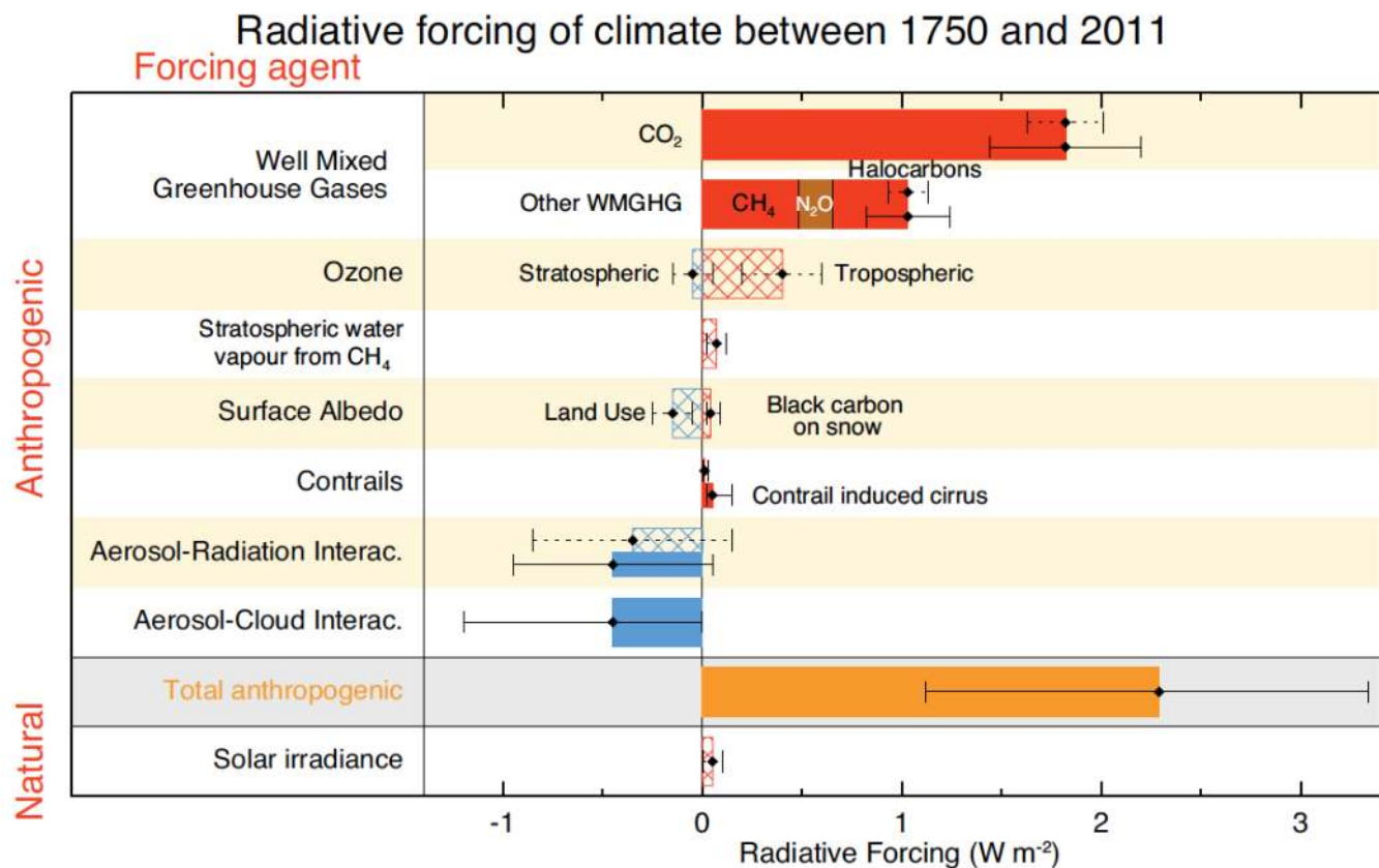
Figure 1.4.13: Summary of radiative forcings. From IPCC (2013). Hatched bars denote low confidence and scientific understanding.
