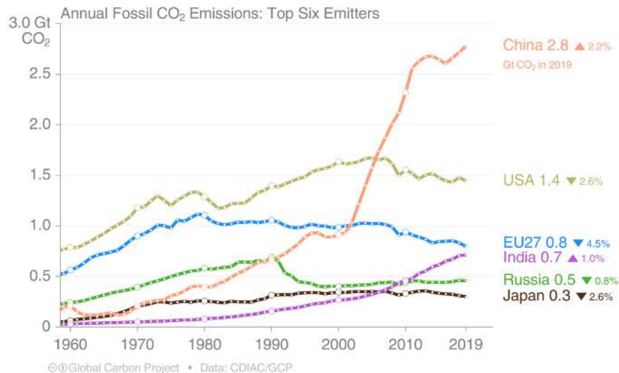
Figure 1.5.4: Carbon emissions from the top four fossil fuel emitters. From globalcarbonproject.org .
