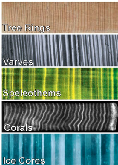
Figure 1.3.2: Layered paleoclimate archives. Varves are layered sea or lake sediments.
