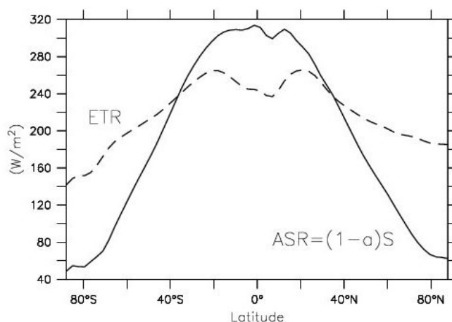
Figure 1.6.3: Absorbed solar radiation (ASR, solid) and emitted terrestrial radiation (ETR, dashed) zonally averaged as a function of latitude from satellite data of Earth's Radiation Budget Experiment.
