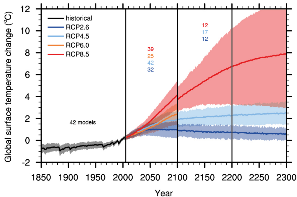
Figure 1.8.3. Global average surface temperature projections relative to 1986-2005. Shading indicates the 5 and 95% range and the line is the multi model mean. The black line with the grey shading represents historical simulations including variations in volcanic forcing. Since volcanic forcing is impossible to predict for the future, changes in natural radiative forcings are not considered in the projections. The number of climate models used is indicated. Not all models have simulated the full period until year 2300, which leads to a jump in the red line at year 2100. From ipcc.ch .
