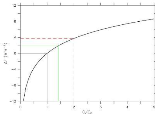
Figure 1.4.9: Radiative forcing ( \Delta F ) in watts per square meter as a function of the atmospheric CO 2 concentration ( C ) relative to a reference value ( C_0 ) according to eq. (2; black thick line). The black straight lines indicate the reference state C = C_0 ( \Delta F = 0 ). The green and red dashed lines indicate the current (2016) state relative to the pre-industrial C/C_0 = 400 \text{ ppm} / 280 \text{ ppm} = 1.4 ( \Delta F = 1.9 \text{ Wm}^{-2} ) and that for a doubling of CO 2 ( \Delta F_{2x} = 3.7 \text{ Wm}^{-2} ) respectively.
