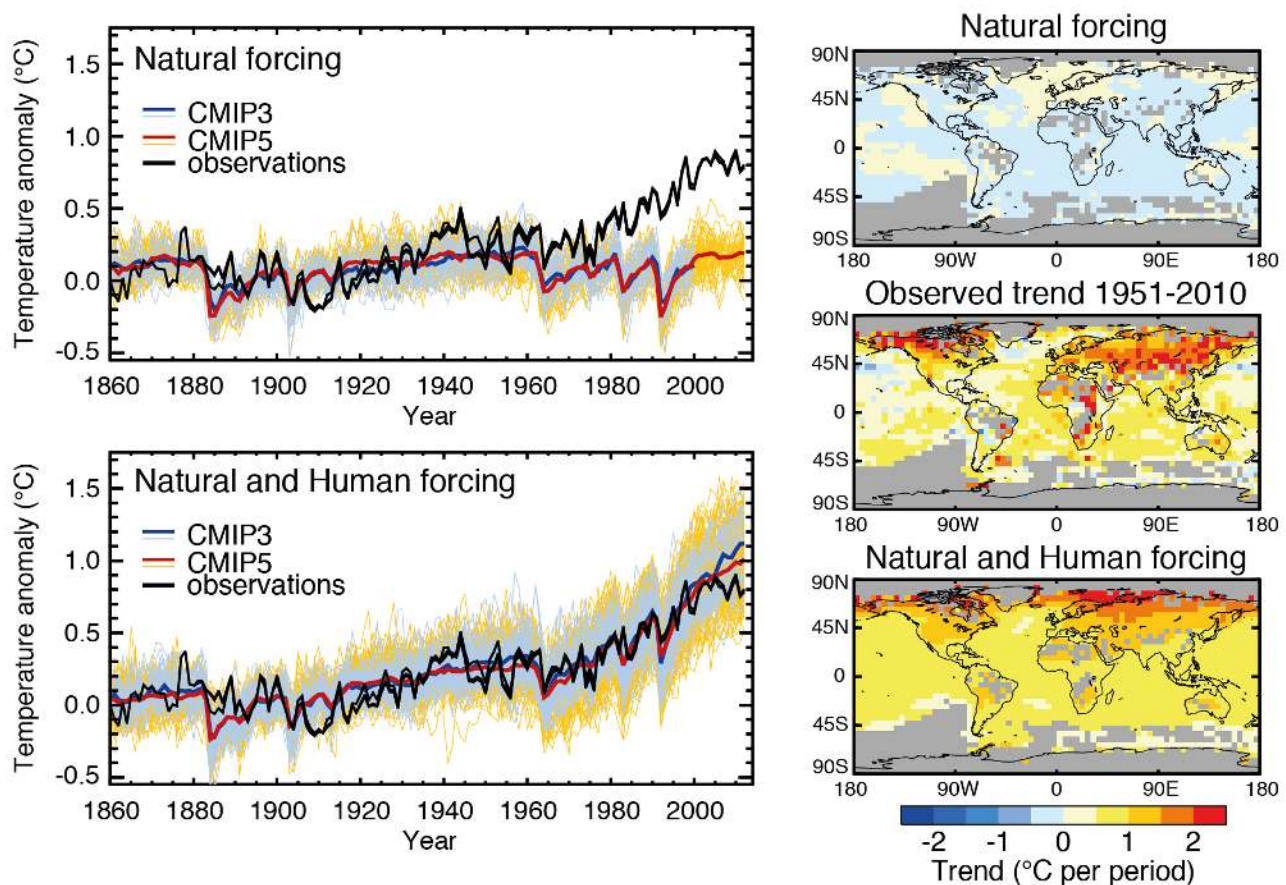
Figure 1.7.8: Comparison of climate model simulations with observed surface temperature changes. Left panels show timeseries of globally averaged surface temperatures from the current generation of climate models (CMIP5; yellow thin lines show individual models, red thick line shows the multi model mean) and the previous generation (CMIP3; blue lines, mostly obscured by the overlain yellow lines). Two sets of simulations are shown. Top panels show models forced with natural forcings only, bottom panels show models forced with both natural and human forcings. From ipcc.ch . This is a key figure.
