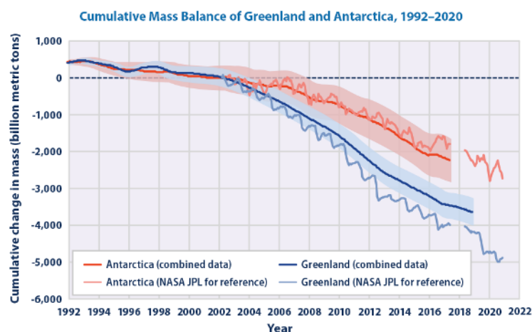
Figure 1.2.7: Changes in the Antarctic (top) and Greenland (bottom) ice sheet mass. Pale lines are from satellite gravity measurements. From the US Environmental Protection Agency (EPA; epa.gov ). Satellite data are from NASA .
