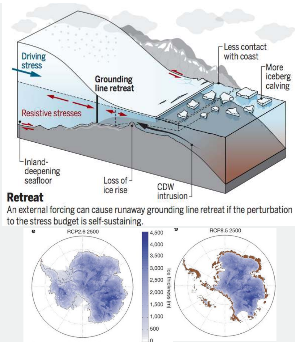
Figure B1.8.4: Antarctic ice sheet vulnerabilities. Top: Schematic illustration of the West Antarctic ice sheet from carbonbrief.org . Bottom: Projection of the Antarctic ice sheet at year 2500 for emission scenarios RCP2.6 (left) and RCP8.5 (right) from DeConto and Pollard, (2016).
