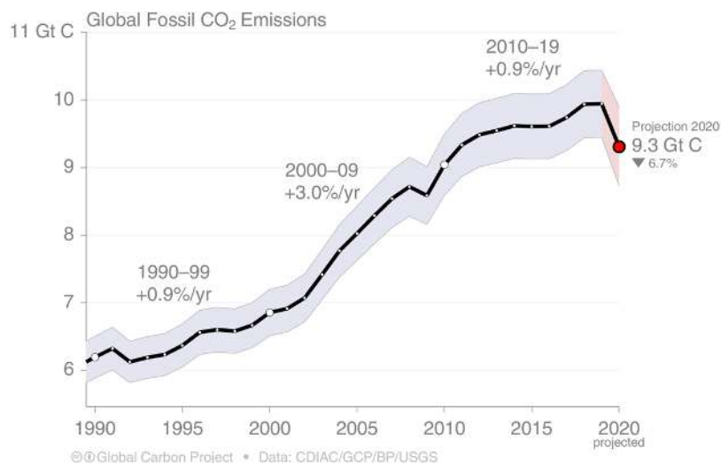
Figure 1.5.3: Estimates of carbon emissions from fossil fuel burning and cement production since 1990. From globalcarbonproject.org .
