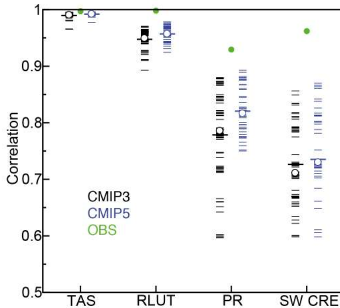
Figure 1.7.5: Correlation coefficient for the annual mean surface air temperature (TAS), outgoing longwave radiation (RLUT; in chapter 6 we called this variable emitted terrestrial radiation from the atmosphere: ETR_a ), precipitation (PR), and the shortwave cloud radiative effect (SW CRE). The correlation coefficient -1 \leq r \leq 1 is a measure of pattern agreement. See this Wikipedia.org page for a detailed definition of r . If two variables are unrelated r = 0 , whereas if they are perfectly in linear agreement r = 1 . Each short horizontal line is one model. The longer line is the multi model mean and the circles are the median. Results are shown for the current generation of climate models from the Climate Modeling Intercomparison Project 5 (CMIP5) and the previous generation (CMIP3). Green dots show correlation coefficients for alternative observational datasets indicating uncertainties in the observations. They represent the best the models could do given uncertainties in the observations. From ipcc.ch .
