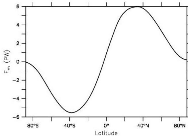
Figure 1.6.4: Meridional (northward is positive) heat transport in the climate system as a function of latitude implied from integration of the differences in the fluxes shown in Figure 1.6.3. Units are peta watts (1 PW = 10^{15} W).
