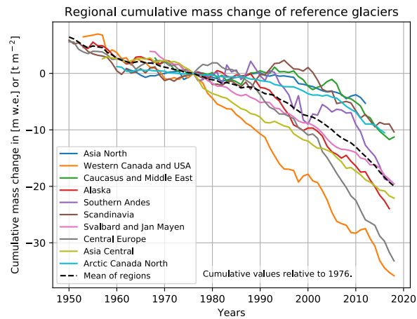
Figure 1.2.6: Cumulative mass balance in meters water equivalent (w.e.) of mountain glaciers. From the World Glacier Monitoring Service .
