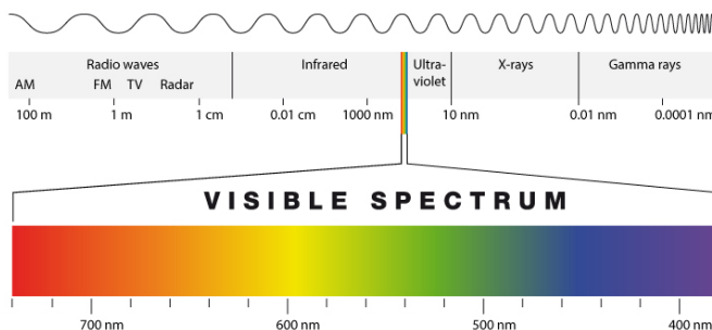
Figure 1.4.1: The Spectrum of Electromagnetic Radiation. Electromagnetic radiation ranges from radio-waves with wavelengths of hundreds of meters and more, to gamma rays, with wavelengths of 10^{-12} m, which is as small as the size of an atomic nucleus. From chromacademy.com.
