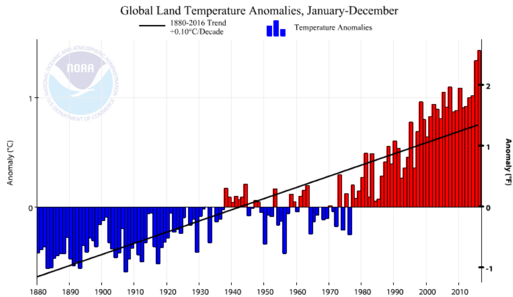
Figure 1.1.10: This figure shows anomalies (differences) with respect to the 1901-2000 average of global averaged land temperatures. Averaged over all of Earth's land areas the year-to-year variations are further reduced ( \sim 1^{\circ}\text{C} ) and the trend is with 0.1^{\circ}\text{C}/\text{decade} slightly larger than that in the U.S.
