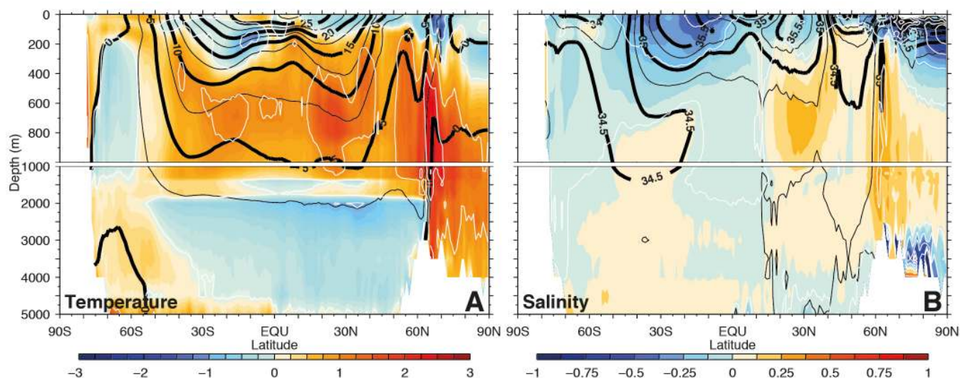
Figure 1.7.6: Zonally averaged differences in temperature (A) and salinity (B) between the multi model mean and observations (color contours and white lines). Black lines indicate observed temperature and salinity from the World Ocean Atlas 2009. From ipcc.ch .
