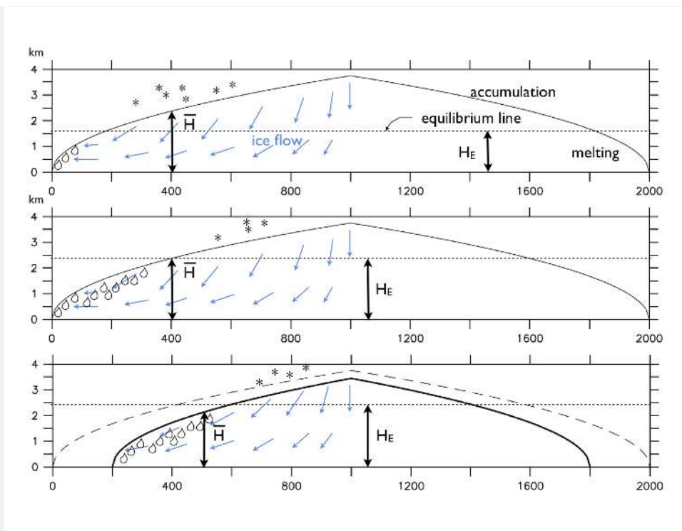
Figure B1.8.1): Schematic section across an idealized ice sheet. The horizontal axis represents the distance in km from its left margin. The vertical axis represents elevation above the flat base.
