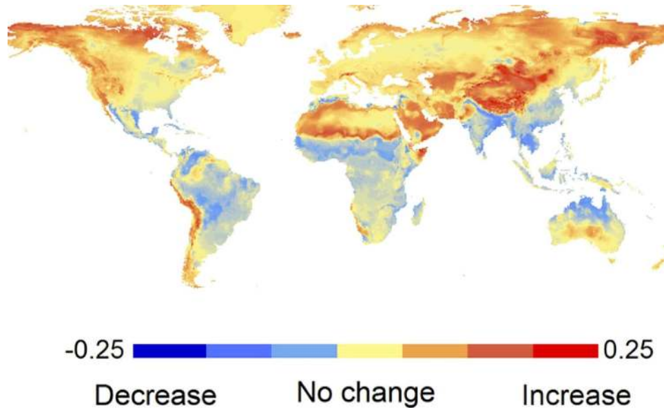
Figure 1.8.11: Projected change in fire probability from 1971-2000 to 2070-2099 for the high SRES-A2 emissions scenario using a statistical method and climate models. From Moritz et al. (2012).
