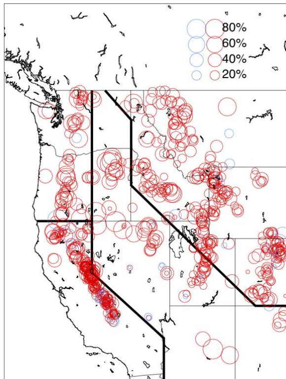
Figure 1.8.15: Linear trends in April 1 st Snow Water Equivalent (SWE) observed for the period 1955-2016. Red circles indicate decreased snowpack, blue increased. From Mote et al. (2018) .
