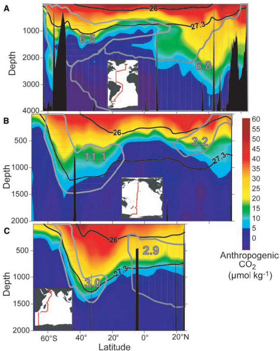
Figure 1.5.13: Latitude-depth sections of anthropogenic carbon in the Atlantic (A), Pacific (B), and Indian (C) oceans. Note that the depth scale is different in panel (A) from the other panels. Black lines denote two surfaces of constant potential density (expressed in \sigma_\theta = density – 1000 kg m -3 ). Movements in the ocean are preferentially along lines of constant potential density because it requires no change in energy (adiabatic). Grey outlines and numbers denote different intermediate and deep water masses and their anthropogenic carbon content in PgC. From pmel.noaa.gov .
