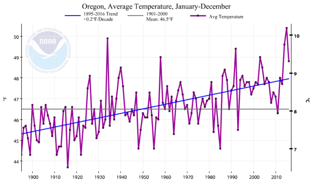
Figure 1.1.8: Averaged over the state of Oregon temperature fluctuations from year-to-year are reduced (1-2°C) compared with the figure from Salem and there is a strong (0.1°C/decade) warming trend.
