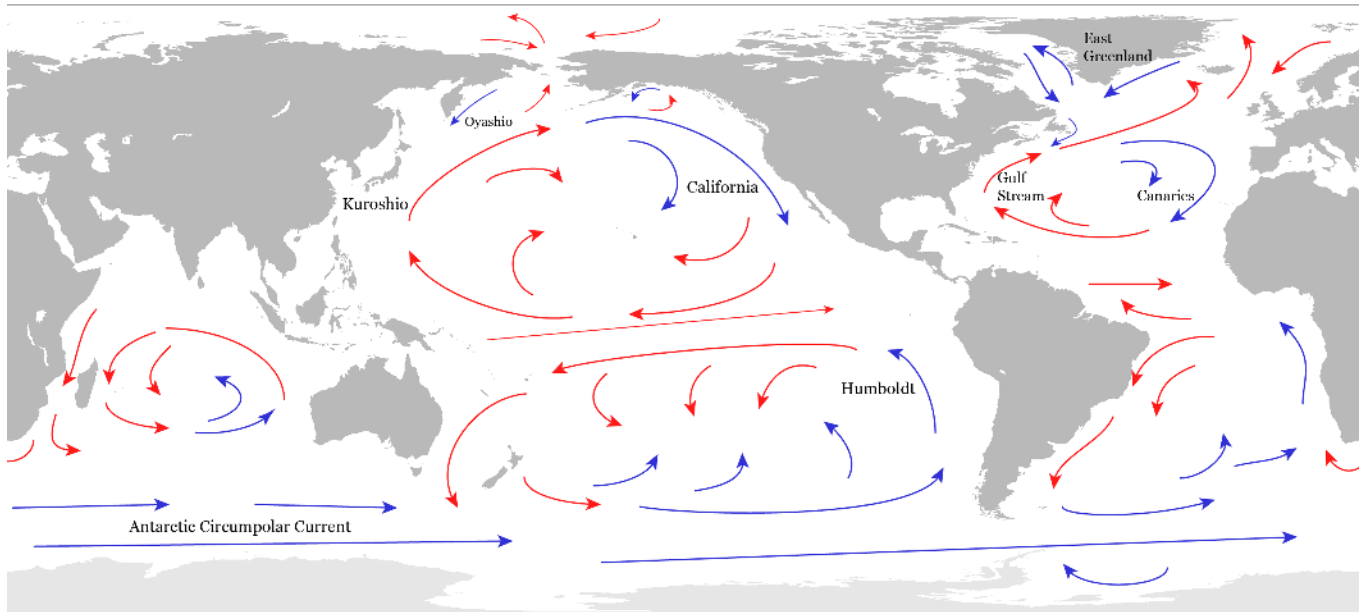
Figure 1.6.16: Sketch of the Surface Circulation of the Ocean. After Peixoto and Oort (1992).
