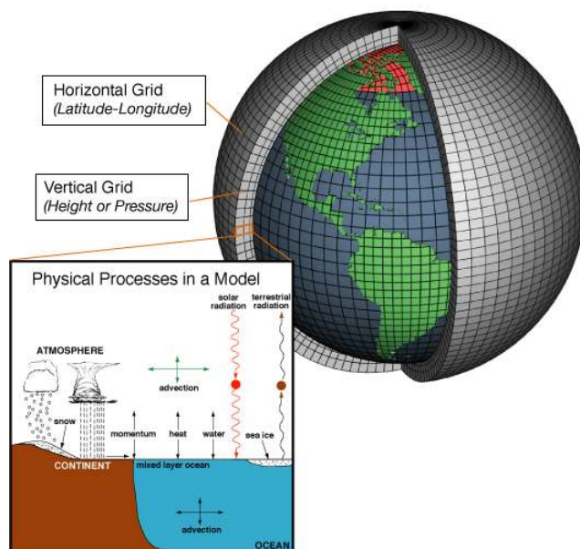
Figure 1.7.1: Schematic of a three-dimensional coupled climate model. From Wikipedia.org .
