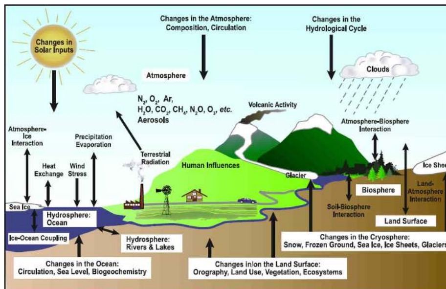
Figure 1.1.2: Schematic view of components of the climate system and processes involved in their interactions. From Le Treut et al. (2007).
