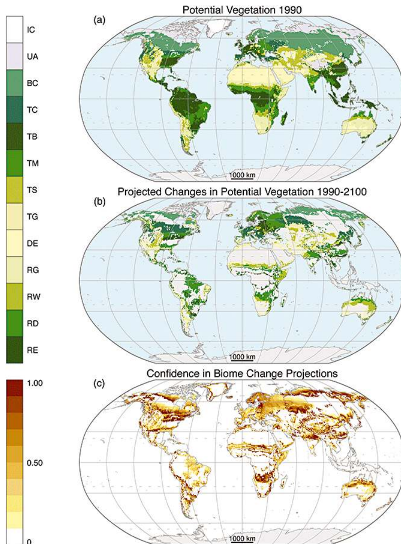
Figure 1.8.10: Modeled potential vegetation in 1990 (a), projected changes by the end of the century (b) and the confidence in the projections (c). Biomes from poles to equator are ice (IC), tundra and alpine (UA), boreal conifer forest (taiga, BC), temperate conifer forest (TC), temperate broadleaf forest (TB), temperate mixed forest (TM), temperate shrubland (TS), temperate grassland (TG), desert (DE), tropical grassland (RG), tropical woodland (RW), tropical deciduous broadleaf forest (RD), tropical evergreen broadleaf forest (RE). From Gonzalez et al. (2010).
