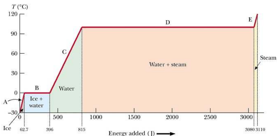
Figure 1.6.10: Effects of heat added ( \Delta H ) on the temperature of one gram of water. Starting from ice at -30^{\circ}\text{C} we need to add about 63 J to warm it up to the melting point (line A). About 333 J are required to melt the ice (line B). During this process the temperature stays constant. Once all ice is melted into water adding more heat causes the water temperature to increase until the boiling point (line C). The slope of line C is the heat capacity of water (at constant pressure) c_{p,\text{water}} = \Delta H/\Delta T = 4.2 \text{ J}/(\text{g}^{\circ}\text{C}) . Once the water boils any added heat is used to vaporize water and the temperature stays at the boiling point until all water is vaporized. The latent heat of vaporization is \sim 2270 \text{ J/g} . Thus, the energy required to vaporize water is more than five times as much as to warm it from 0^{\circ}\text{C} to 100^{\circ}\text{C} .
