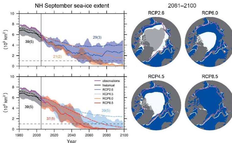
Figure 1.8.7): Projections of Arctic sea ice in September. Results from all models are shown as dashed lines in the time series panels on the left and as white shading in the maps on the right. Results from a subset of models that agree best with observed sea ice (numbers in brackets) are shown as solid lines and grey shading. From ipcc.ch .
