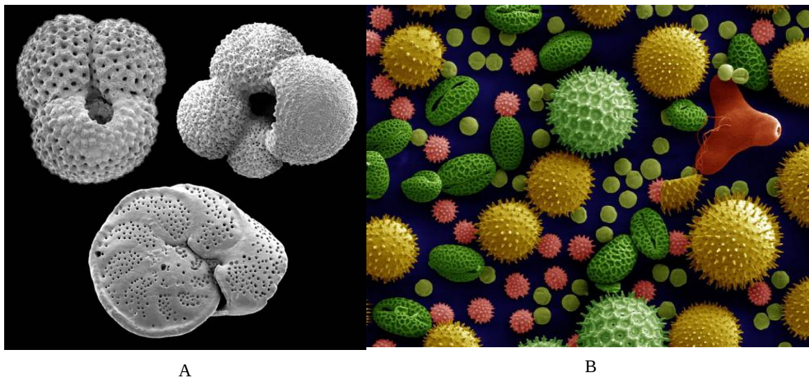
Figure 1.3.1: Electron microscope pictures of fossil foraminifera (A, two planktic foraminifera on top and one benthic foraminifera on the bottom) and pollen (B).
