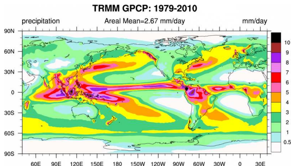
Figure 1.6.8: Annual mean precipitation estimated from observations. From ucar.edu .
