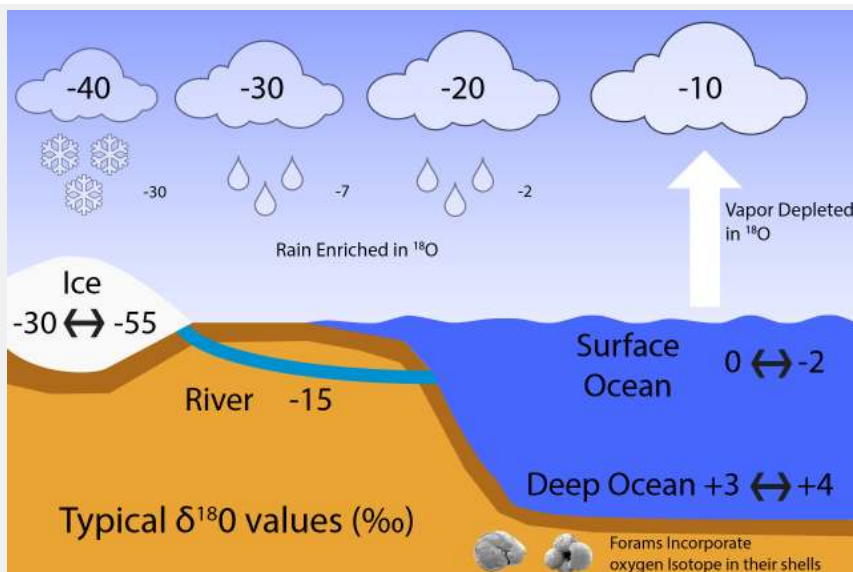
Figure B1.3.2: Typical \delta^{18}\text{O} values (in permil). Surface ocean water has \delta^{18}\text{O} values of around zero. Due to fractionation during evaporation less heavy isotopes make it into the air, which leads to negative delta values of around -10 ‰. Condensation prefers the heavy isotopes for reasons analogous to evaporation. In this example the first precipitation thus has a \delta^{18}\text{O} value of about -2 ‰, the remaining water vapor will be further depleted in ^{18}\text{O} relative to ^{16}\text{O} thus that its \delta^{18}\text{O} value is approximately -20 ‰. Any subsequent precipitation event further depletes ^{18}\text{O} . This process is known as Rayleigh distillation and leads to very low \delta^{18}\text{O} values of less than -30 ‰ for snow falling onto ice sheets. Thus, ice has very negative \delta^{18}\text{O} of between -30 and -55 ‰. Deep ocean values today are about +3 to +4 ‰. During the LGM, as more water was locked up in ice sheets, the remaining ocean water became heavier in \delta^{18}\text{O} by about 2 ‰. We know this because foraminifera build their calcium carbonate ( \text{CaCO}_3 ) shells using the surrounding sea water. Thus they incorporate the oxygen isotopic composition of the water into their shells which are preserved in the sediments and can be measured in the lab.
