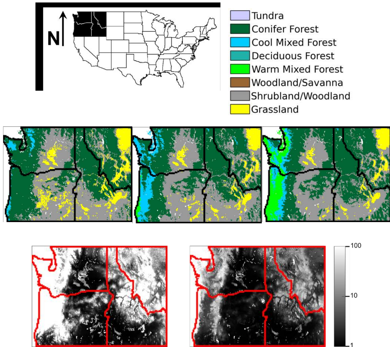
Figure 1.8.16: Projected changes in vegetation (center row with legend in top right) and fire frequency (bottom) in the Pacific Northwest (filled area in the top left map of the USA). Vegetation is shown for years 1971-2000 (left), 2036-2065 (center) and 2071-2100 (right). Fire frequency in years is shown for the 20th century (left) and the 21st century (right). Modified from Sheehan et al. (2015). Simulations without fire suppression are shown. Figure courtesy of Tim Sheehan.
