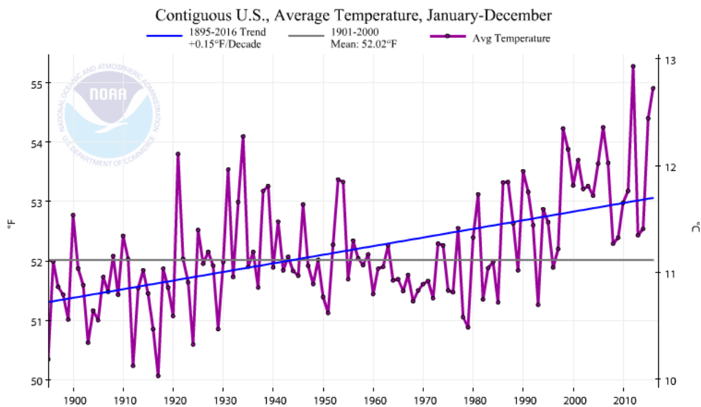
Figure 1.1.9: Averaged over the contiguous U.S. the year-to-year variability has slightly decreased compared to Oregon. The warming trend is similar but slightly lower.
