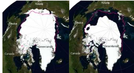
Figure 1.2.3: Arctic sea ice extent in September 1979 (left) and 2020 (right) from satellite observations. The purple line denotes the median ice extent from 1981-2010. In 1979 the ice extent was 7.1 million sq km, in 2020 it was 3.9 million sq km. Images from the National Snow and Ice Data Center ( NSIDC ).
