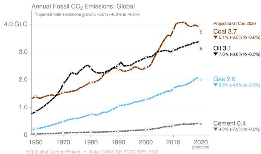
Figure 1.5.5: Contributions to fossil fuel emissions from coal, oil, and gas burning and cement production. From globalcarbonproject.org .
