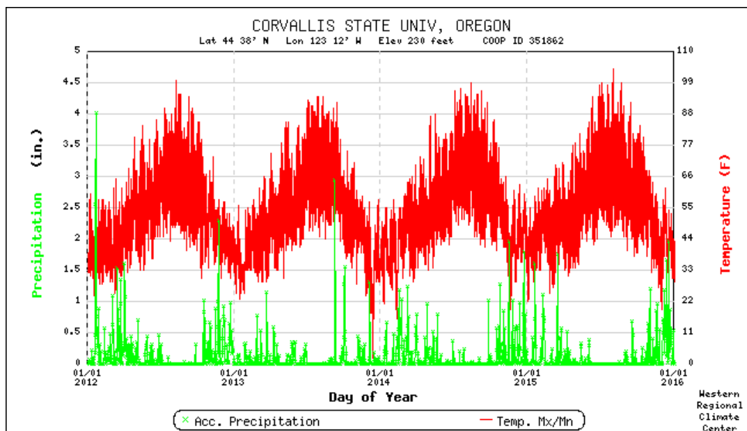
Figure 1.1.4: Local weather data (daily minimum and maximum temperature and daily precipitation) from Corvallis, Oregon, from 2012 to 2016. Large variations in temperatures from ~40°F in winter to ~65°F in summer indicate the seasonal (or annual) cycle. Precipitation, which is very episodic, also shows a large annual cycle with lots of rain in winter and less rain in summer. The mean seasonal cycle is shown in Figure 1.1.5. From wrcc.dri.edu
