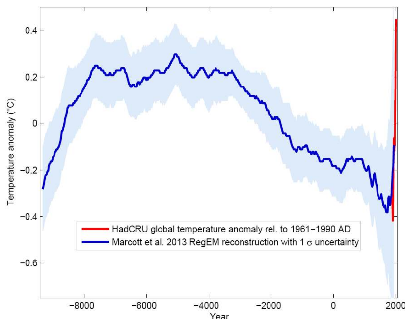
Figure 1.3.6: Holocene global surface temperature reconstruction from Marcott et al. (2013, blue) with shaded error ranges together with the instrumental record (red) as a function of time in years CE. From RealClimate .
