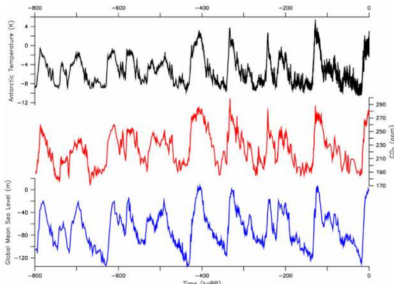
Figure 1.3.11: Glacial-interglacial Cycles. Top: Antarctic temperature anomaly estimated from deuterium ratios measured in the ice (Jouzel et al., 2007). Deuterium (D) is the heavy hydrogen isotope ^2\text{H} . In \text{H}_2\text{O} it works similar to the heavy oxygen isotope as a local temperature proxy. Center: Atmospheric \text{CO}_2 concentrations from ice cores (Lüthi et al., 2008). Bottom: Global sea level changes ( \text{ASL} = [\delta^{18}\text{O} - 3.2 \text{‰}] \times [-120 \text{ m} / 1.69 \text{‰}] ) estimated from oxygen isotopes ( \delta^{18}\text{O} ) measured in benthic foraminifera from deep-sea sediments (Lisiecki and Raymo, 2004). This is a key figure.
