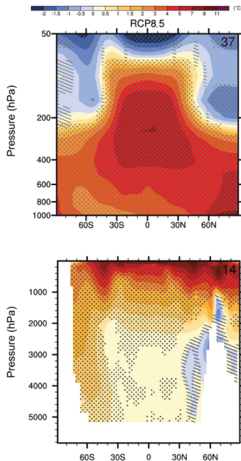
Figure 1.8.5). Hatching indicates where changes are not significant with respect to 2 sigma variations of internal variability. Click on the ocean panel to see results for other scenarios. From ipcc.ch .
