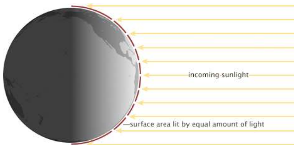
Figure 1.6.2: The amount of incoming sunlight on Earth is spread over a larger area at the poles than at the equator. This leads to less heating of the poles compared to the equator. From earthobservatory.nasa.gov .
