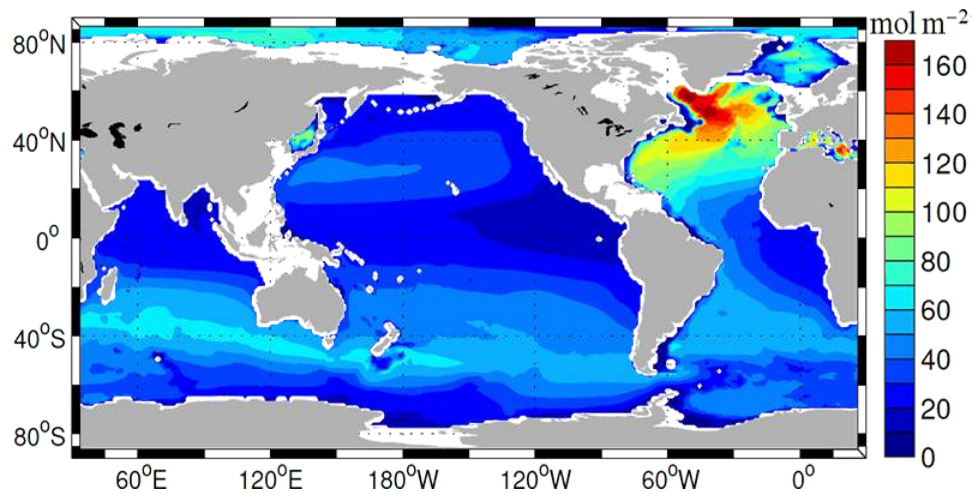
Figure 1.5.12: Anthropogenic carbon in the ocean estimated from observations (Khatriwala et al., 2013). From rapid.ac.uk .
