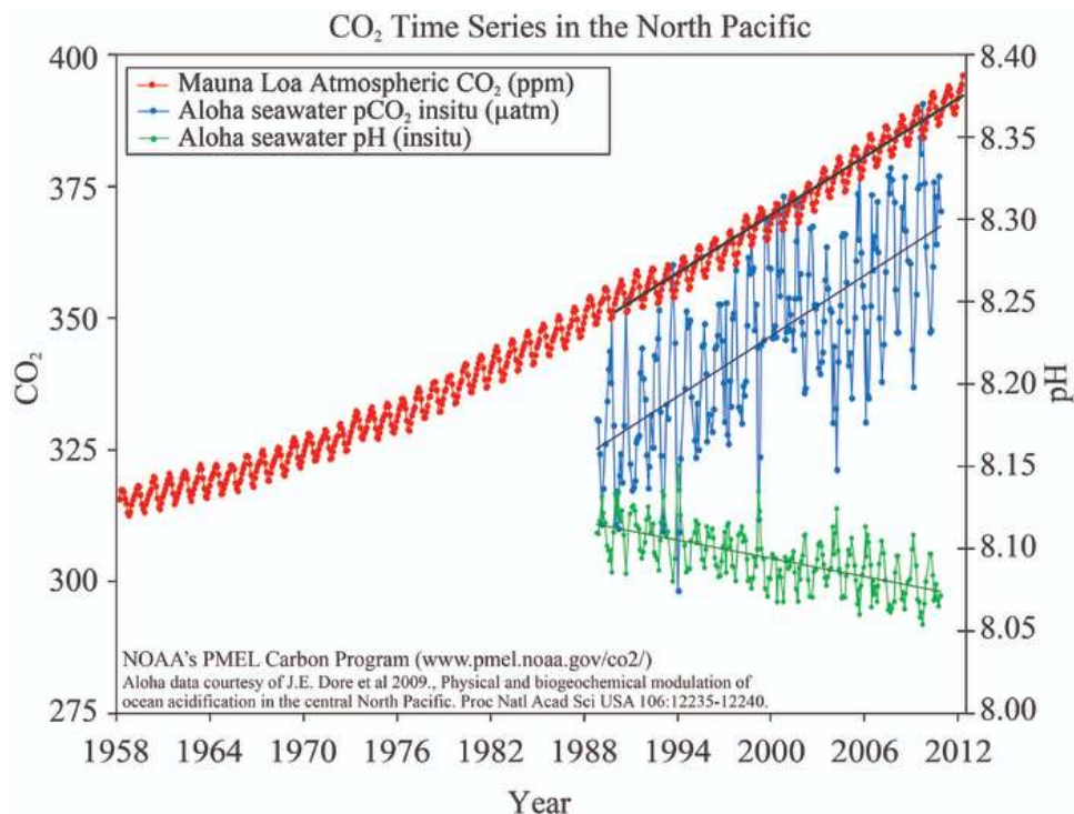
Figure 1.5.11: Measurements of seawater \text{pCO}_2 (blue) and pH (green) at ocean station Aloha near Hawaii together with the Mauna Loa record of atmospheric \text{CO}_2 (red). From pmel.noaa.gov .
