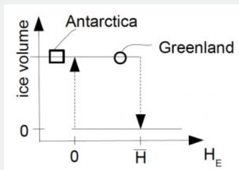
Figure B1.8.2): Schematic hysteresis curve for an ice sheet. The vertical and horizontal axes represent ice volume and height of the equilibrium line, respectively.
