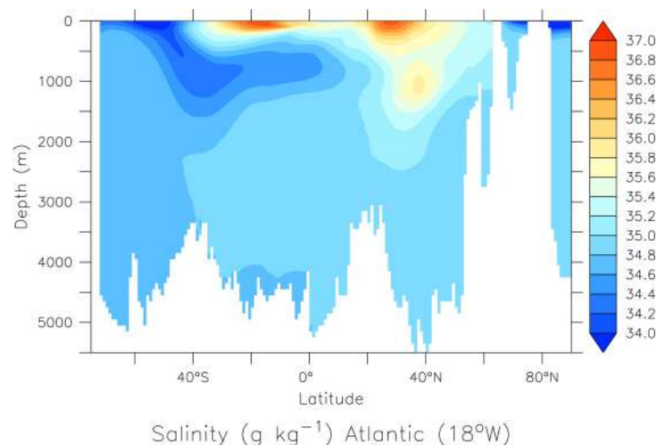
Figure 1.6.19: Salinity (in grams salt per kg of sea water) section through the Atlantic ocean at 18°W as a function of latitude and depth.
