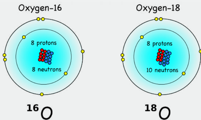
Figure B1.3.1: Oxygen's most common (99.8%) isotope oxygen-16 ( ^{16}\text{O} ) has 8 protons (red) and 8 neutrons (blue) such that its mass is 16 atomic units. Oxygen-18 ( ^{18}\text{O} ) has two additional neutrons, which makes it (18 - 16)/16 = 12.5\% heavier than ^{16}\text{O} . It is also much rarer (0.2%) than ^{16}\text{O} . From Montessori Muddle .
