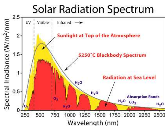
Figure 1.4.5: Solar radiation spectra for the incident sunlight at the top-of-the-atmosphere (yellow), at sea level (red), and a blackbody curve (grey). From en.wikipedia.org .
