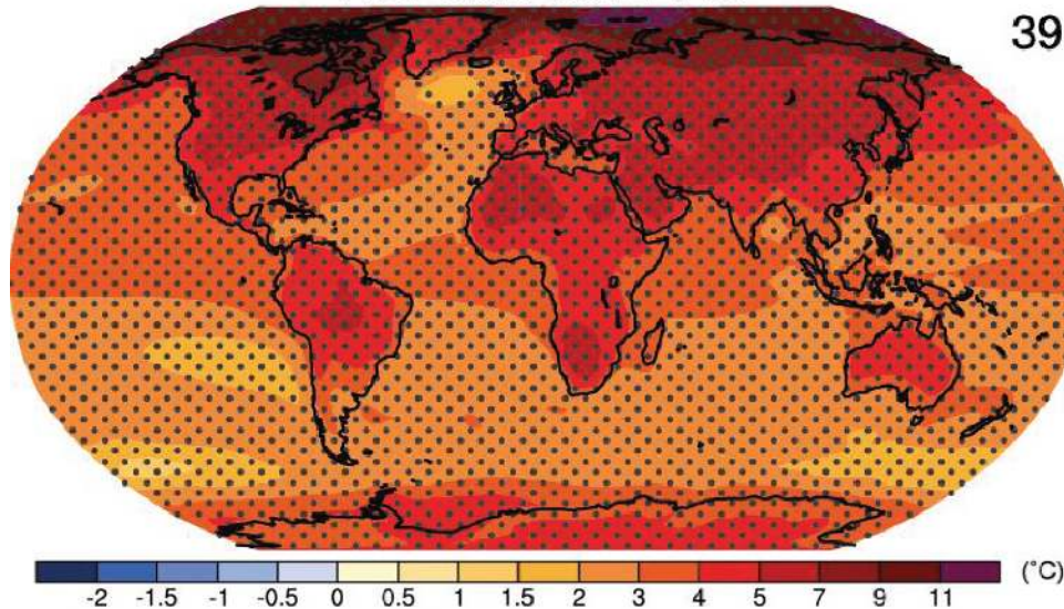
Figure 1.8.4: Surface temperature changes projected for the business-as-usual scenario RCP8.5 at the end of the 21 st century. Stippling indicates regions of highly significant changes, where the multi model mean is larger than two standard deviations of modeled internal variability and where at least 90% of models agree on the sign of the change. Click on the map to see projections for other scenarios and times. From ipcc.ch .
