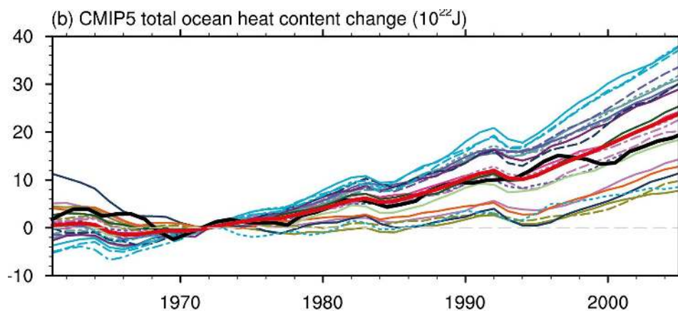
Figure 1.7.7: Changes in ocean heat content simulated by the CMIP5 models (thin lines), and their multi model mean (red thick line), compared to observations (black thick line). From ipcc.ch .
