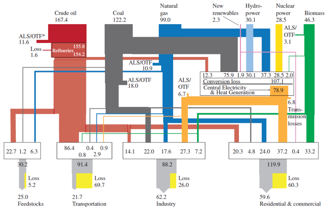
Figure 1.11.2: Energy flows in the world economy in 2005 in exajoules (1EJ = 10 18 J) per year from primary sources top to end-use sector (bottom). ALS = Autoconsumption, losses, stock changes. OTF = other transformation to secondary fuels. From GEA (2012).
