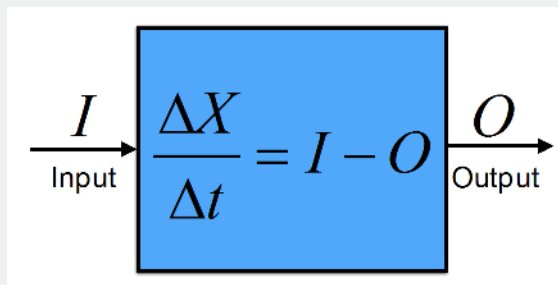
Figure B1.4.1.1: Illustration of the budget equation. A box containing a conserved quantity X that does not include internal sources or sinks will change in time according to the external inputs minus the outputs.
