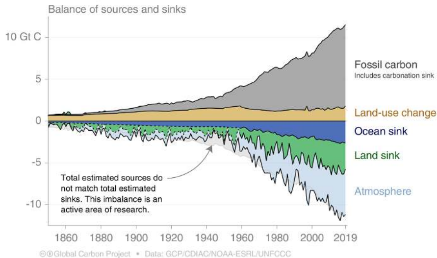
Figure 1.5.2: Anthropogenic Carbon Sources and Sinks in Billion Metric Tons of Carbon Per Year (Gt C/yr) as a function of the year. Positive numbers show sources from fossil fuel burning and cement production (gray) and deforestation (yellow). Negative numbers show uptake by land (green), atmosphere (light blue), and ocean (dark blue). From Le Quéré et al. (2018). Image from globalcarbonproject.org .
