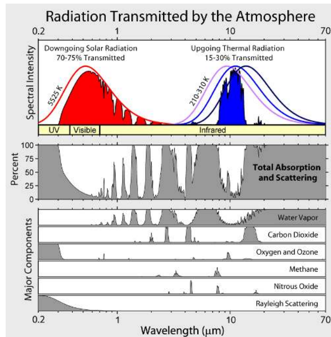
Figure 1.4.6: Radiation transmitted and absorbed by the cloud-free atmosphere. The left part of the figure shows the solar radiation and the right part shows Earth's radiation. The blackbody curve at 5525 K (red curve in the top panel) represents the incident (downgoing) solar radiation at the top-of-the-atmosphere. The red filled area is the radiation transmitted through the atmosphere. The difference between the two (the white area between the red curve and the red area) is the amount absorbed by the atmosphere. For Earth's radiation blackbody curves are shown for three temperatures (210, 260, and 310 K) and represent upgoing radiation from the surface. This is a key figure. From commons.wikimedia.org
