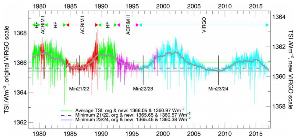
Figure 1.4.14: Total solar irradiance variations. Top: measurements based on various satellites as a function of time.
