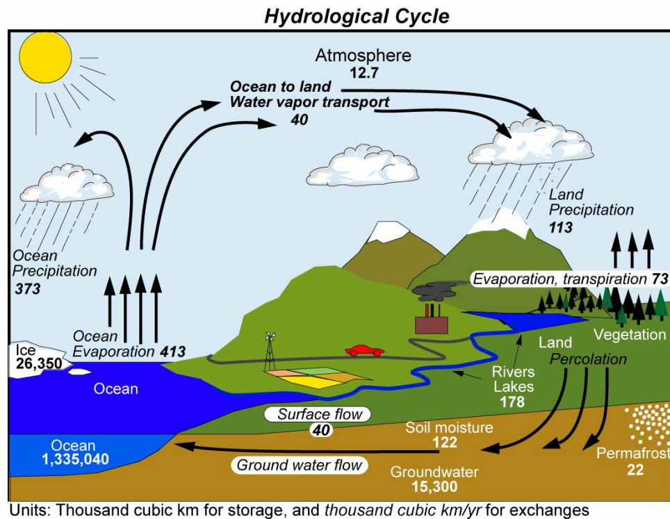
Figure 1.6.14: The Global Water Cycle. Fluxes are indicated in slanted font . From Trenberth et al. (2007). Image from ucar.edu .
