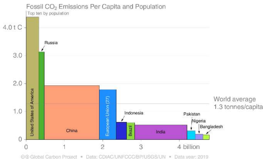
Figure 1.5.6: Carbon emissions per person in tC/yr. The width of the boxes represents the population. From globalcarbonproject.org .
