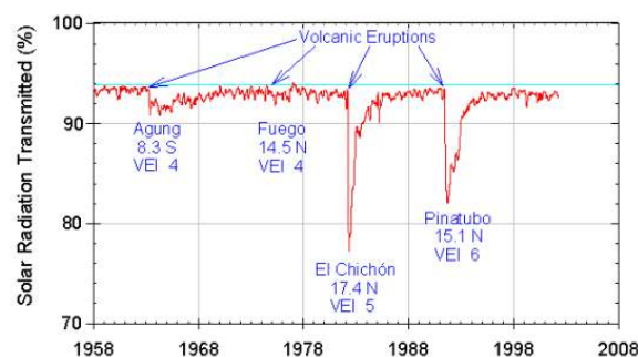
Figure 1.4.11: Effects of volcanic eruptions.
