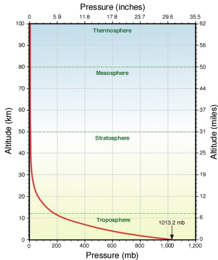
Figure 1.6.5: Air Pressure as a Function of Altitude. From physicalgeography.net .
