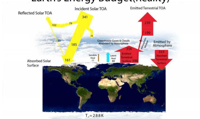
Figure 1.4.8: Earth's energy budget estimated from modern observations and models. Adapted from Trenberth et al. (2009).
