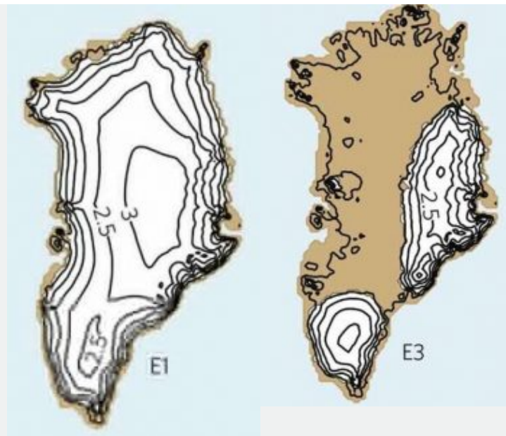
Figure B1.8.3): Greenland fully glaciated (left) and mostly deglaciated (right). Contour lines denote ice sheet thickness in km. From Robinson et al. (2012) at nature.com .
