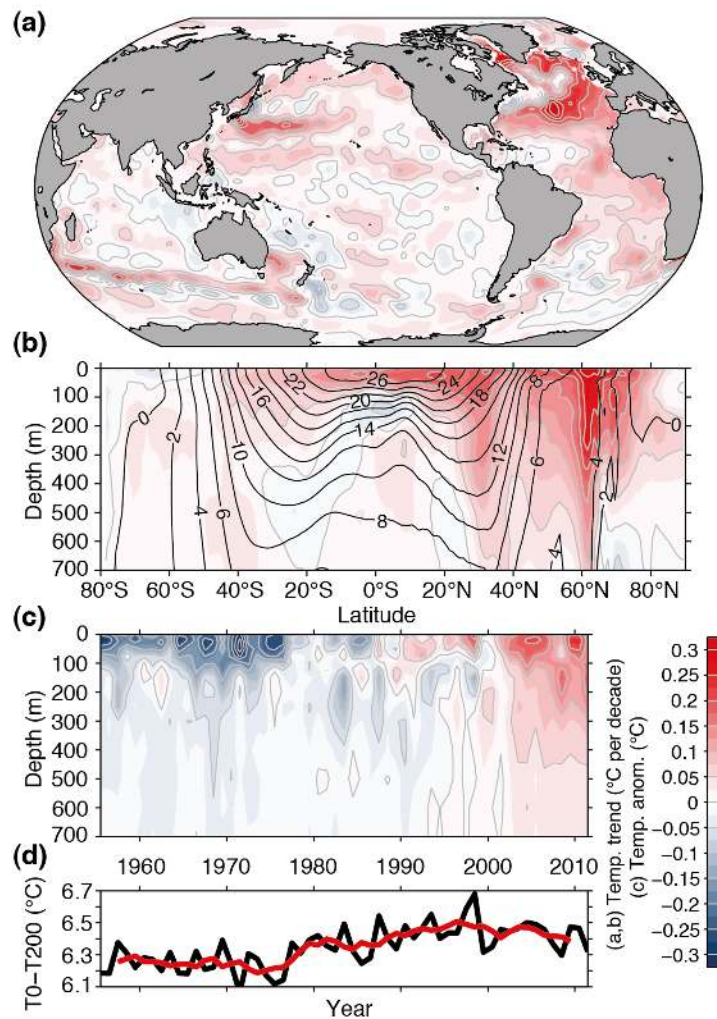
Figure 1.6.20: (a) Temperature trend over the top 700 m from 1971-2010. (b) Zonally averaged temperature trend. Black contour lines represent the mean temperature distribution. (c) Horizontally averaged temperature changes. (d) Changes in temperature difference between 200 m and the surface. From Rhein et al. (2013). Image from ipcc.ch.
