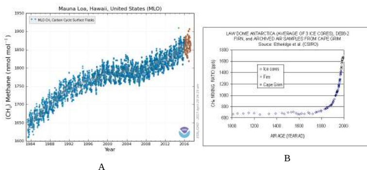
Figure 1.4.10: Atmospheric methane concentrations as a function of time A : recent air measurements at Mauna Loa. B : Ice core, firn, and air measurements from Antarctica. Note that most methane sources are in the northern hemisphere, which leads to higher concentrations there compared with the Southern Hemisphere.
