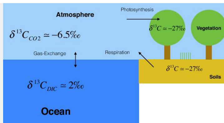
Figure B2.1.5.2: Schematic Distribution of Carbon Isotopes in the Carbon Cycle Components.
