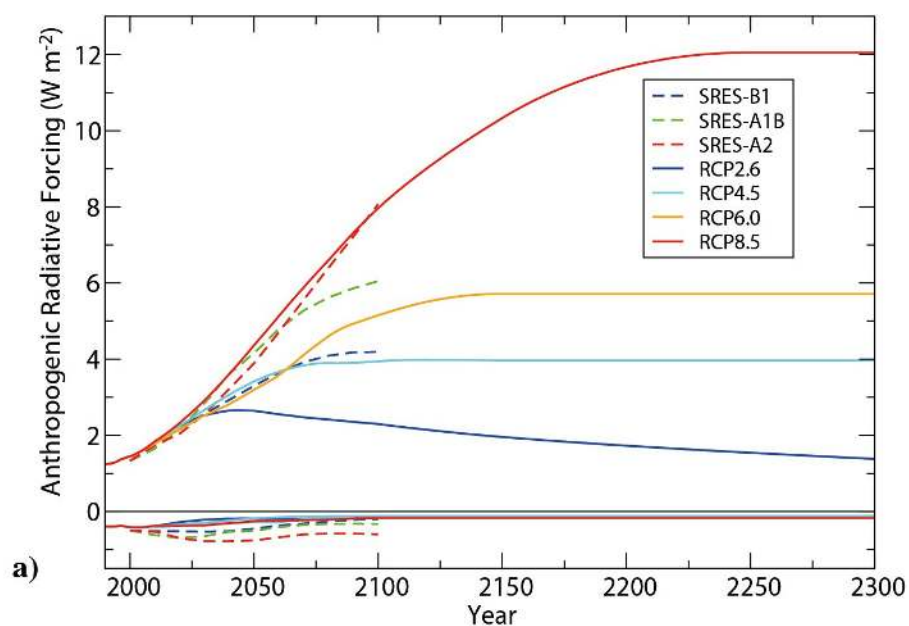
Figure 1.8.1: Anthropogenic radiative forcing as a function of time for the current (RCP) and previous (SRES) IPCC scenarios. From ipcc.ch.
