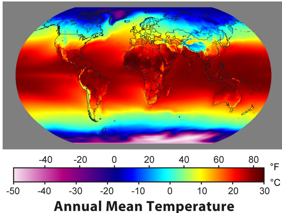
Figure 1.6.1: Annual mean surface temperature distribution. From wikimedia.org .
