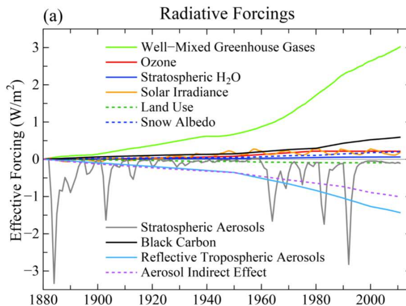
Figure 1.4.12: Radiative forcings as a function of time. From data.giss.nasa.gov .
