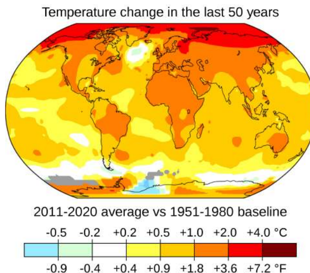
Figure 1.2.2: Global Map of Recent Surface Temperature Change. From Wikipedia's Climate Change based on data from NASA's Goddard Institute for Space Studies (GISS).
