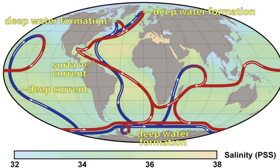
Figure 1.6.18: Cartoon of the Deep Ocean Circulation. Red and blue ribbons represent surface and deep currents, respectively. From Wikipedia.org.
