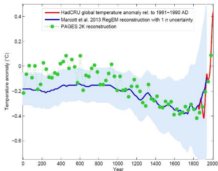
Figure 1.3.5: Global multi-proxy temperature reconstructions from the PAGES 2k project based on 7 continental scale regional reconstructions (green) compared with an independent reconstruction that includes the whole Holocene (Marcott et al., 2013; blue with shaded error range; see also Figure 1.3.7 ) and the instrumental record (red). The PAGES 2k reconstruction represents 30-year averages. It includes many more data than the lower resolution Marcott et al. (2013) reconstruction, particularly for the last 1,000 years. Thus the error range of the PAGES 2k reconstruction is presumably much smaller than that indicated by the blue shading. From RealClimate .
