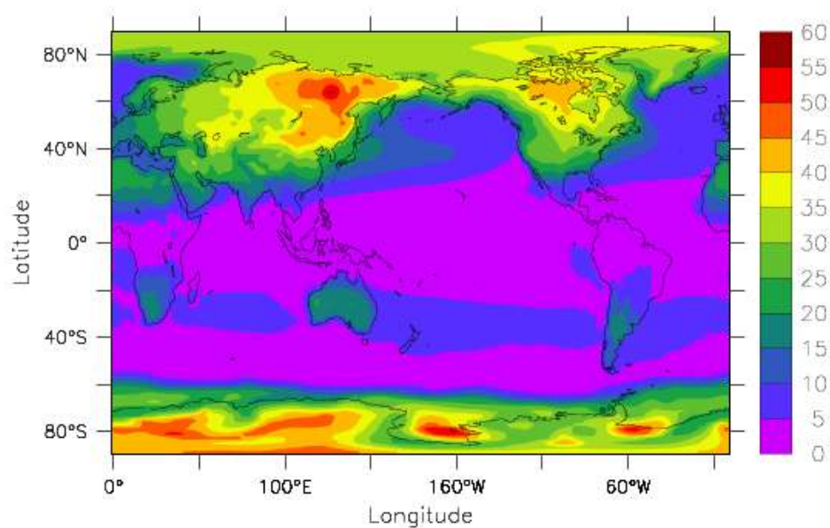
Figure 1.6.12: Amplitude of the Seasonal Cycle of Surface Temperatures. Plotted is the maximum minus the minimum of the average seasonal cycle from 1958 to 1996 from the National Center for Environmental Prediction (NCEP) Reanalysis. Units are in degrees Celsius.
