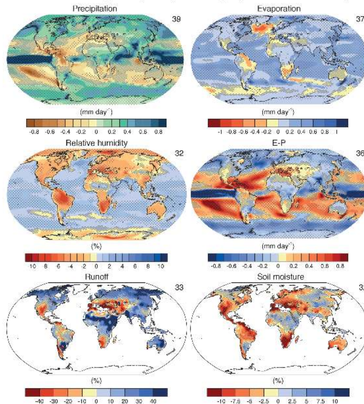
Figure 1.8.6): As Figure 1.8.4), but for changes in the hydrological cycle. From ipcc.ch .
