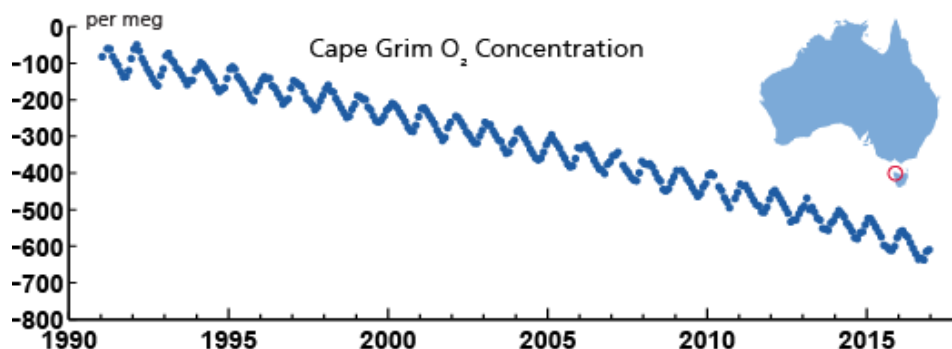
Figure 1.5.8: Measurements of atmospheric oxygen to nitrogen ratios from Cape Grim, Tasmania. Similar measurements exist from other locations. Image from scrippsco2.ucsd.edu.
