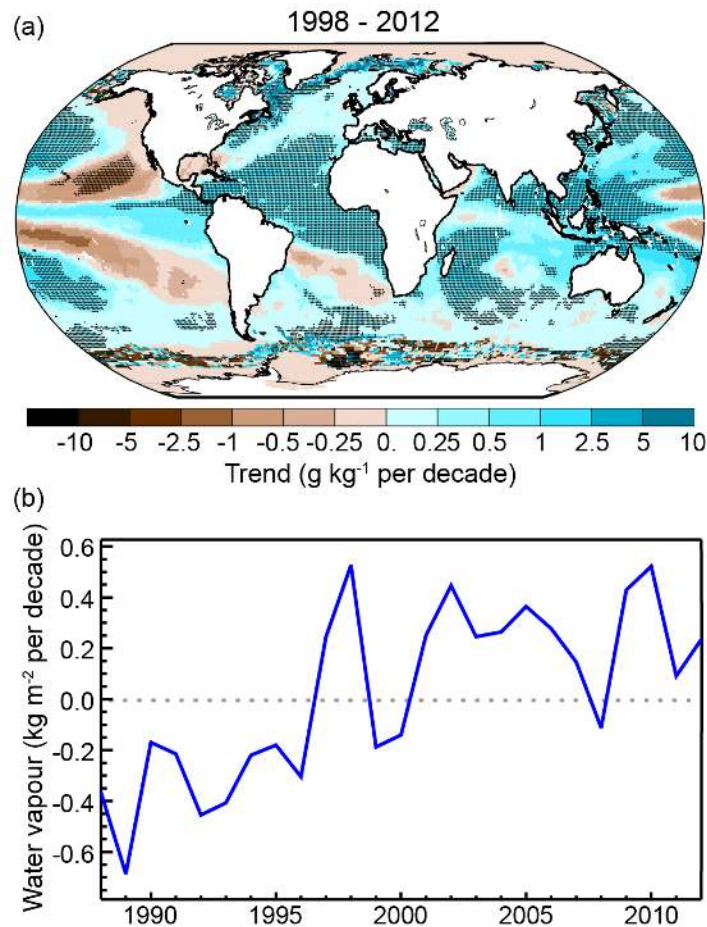
Figure 1.6.15: (a) Observed changes in surface specific humidity estimated from satellites. Dark shading indicates significant changes. (b) Changes in globally averaged water vapor content. From Harmann et al. (2013). Image from ipcc.ch.
