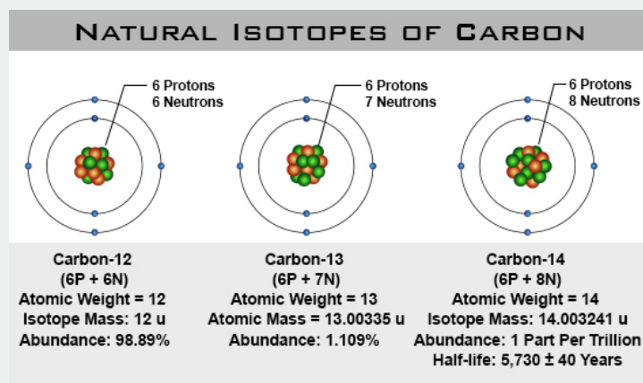
Figure B2.1.5.1: Illustration of the Atomic Structure of Carbon Isotopes. The nucleus consists of protons (red) and neutrons (green). It is surrounded by electrons (blue).
