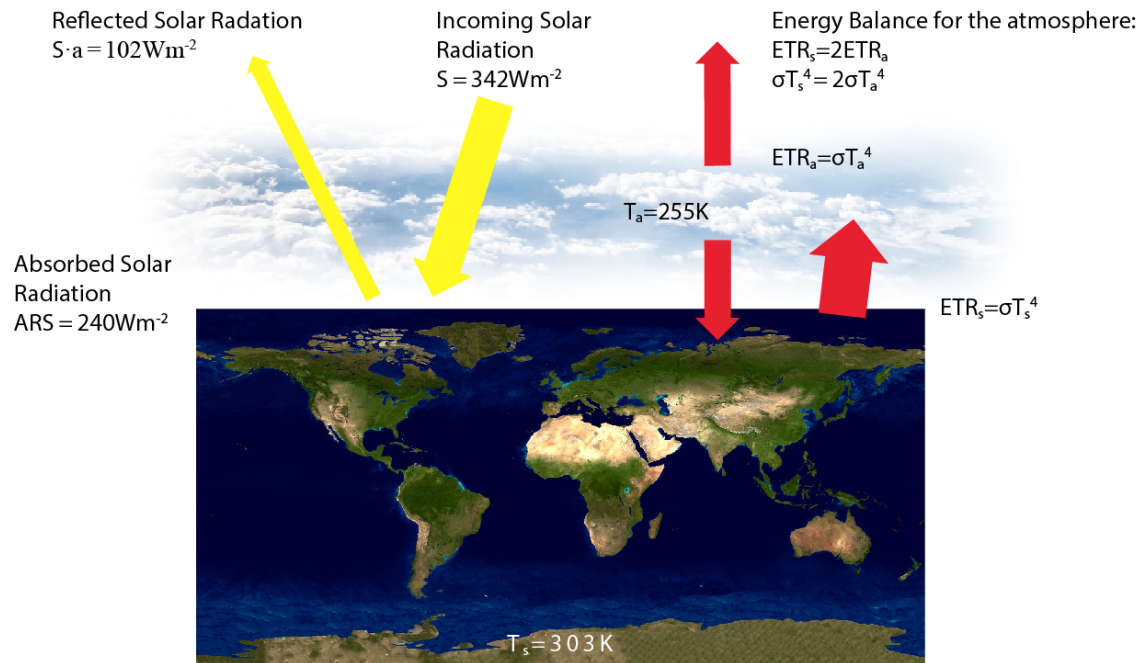
Figure B1.4.3.1: As Figure 1.4.5 but for the 'Perfect Greenhouse' model.
