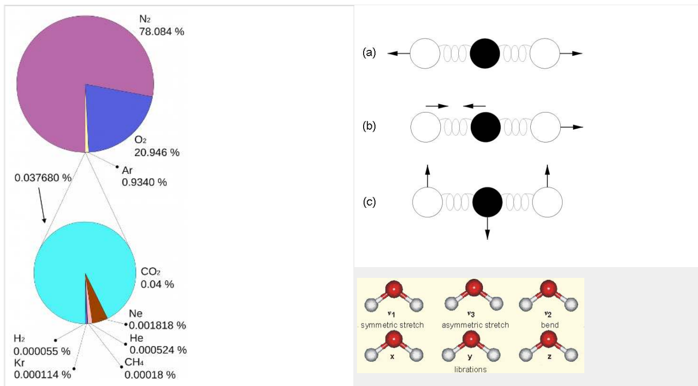
Figure 1.4.7: Left: Composition of the dry atmosphere. Water vapor, which is not included in the image, varies widely but on average makes up about 1 % of the troposphere. Top right: Vibrational modes of CO 2 . The black circles in the center represent the carbon atom, which carries a positive charge, whereas the oxygen atoms (white) carry negative charges. The asymmetric stretch mode (b) and the bend mode (c) lead to an electrical dipole moment, whereas the symmetrical stretch (a) does not. Modes (b) and (c) correspond to the absorption peaks around 4 and 15 \mu\text{m} , respectively (Figure 1.4.7). Bottom right: Vibrational modes of H 2 O. The red balls in the center represent the negatively charged oxygen atom, whereas the white balls represent the positively charged hydrogen atoms. Due to its angle, it has a permanent dipole moment and various modes of vibration and rotation.
