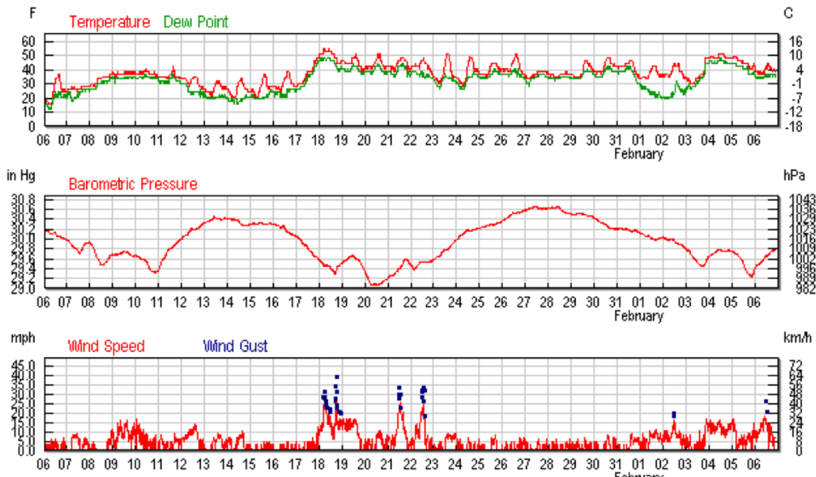
Figure 1.1.3: Weather data from Corvallis, Oregon from January 2017. In the upper panel we can see diurnal cycles in temperature. Pressure varies on longer timescales. Low pressure is associated with storms (high winds and wind gusts).
