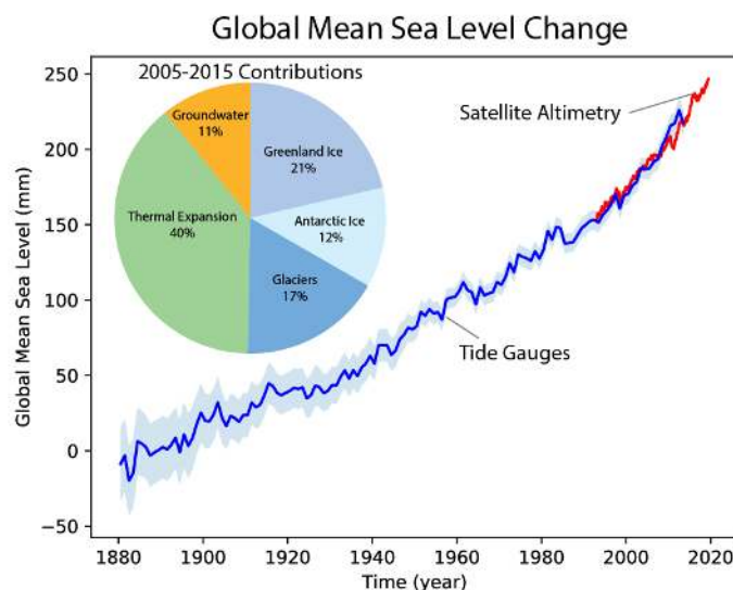
Figure 1.2.9: Observed global mean sea level estimated from satellites (red) and tide gauges (blue). Data from nasa.gov and csiro.au . The pie chart shows the relative contributions from melting of land ice ( 1.8 \pm 0.1 mm/yr), thermal expansion of sea water ( 1.4 \pm 0.3 mm/yr) and groundwater pumping (0.4 mm/yr; estimated as the residual) during 2005-2015 (IPCC, 2019). The total rate of sea level rise during this period ( 3.6 \pm 0.5 mm/yr) is larger than during earlier periods. This acceleration of sea level rise is caused by recently increased melting of the Greenland and Antarctic ice sheets.
