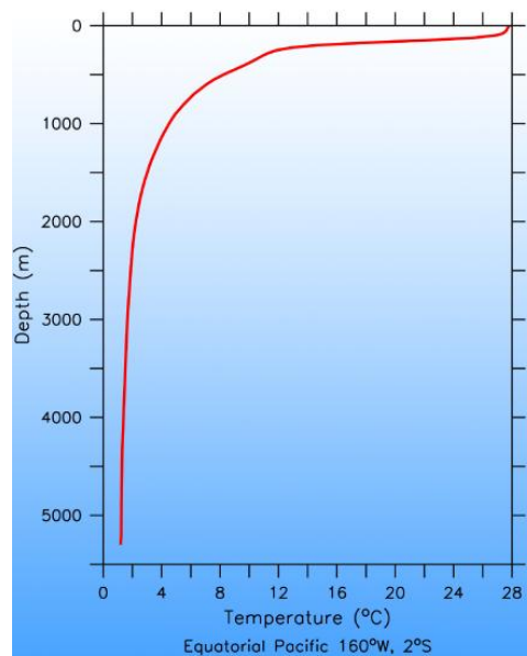
Figure 1.6.17: Typical Temperature Profile with Depth in the Ocean.
