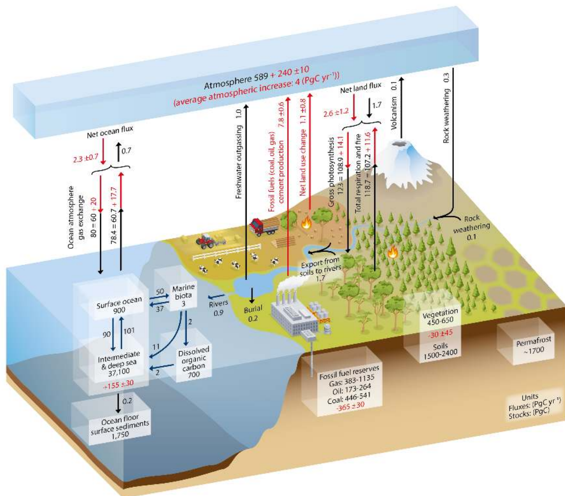
Figure 1.5.1: The Carbon Cycle. Numbers in boxes represent reservoir mass, also called carbon stocks, inventories, or storage in PgC (1 Pg = 10^{15} g = 1 Gt). 2.1 PgC = 1 ppm atmospheric \text{CO}_2 . Numbers next to arrows indicate fluxes in PgC/yr. Black numbers and arrows represent estimates of the natural (pre-industrial) carbon cycle. Red numbers and arrows indicate estimates of anthropogenic effects for 2000-2009. From Ciais et al. (2013). Image from ipcc.ch . See additional material at the end of this chapter for a figure showing the sizes of the reservoirs and fluxes in proportion to the size of the boxes and arrows.
