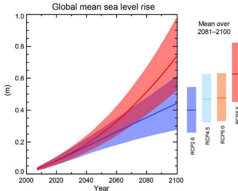
Figure 1.8.8): Global sea level rise projected for the 21 st century. The blue and red curves show projections for scenarios RCP2.6 and RCP8.5, respectively. The shading indicates the likely (66-100%) uncertainty range. Bars on the right show the 2081-2100 averages for four scenarios. From ipcc.ch .
