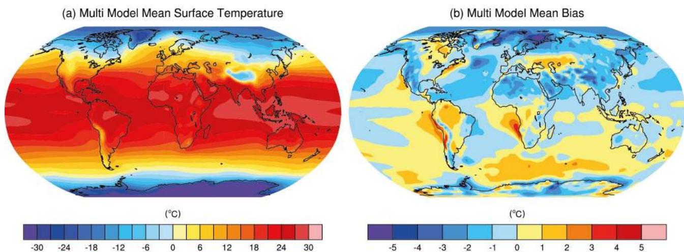
Figure 1.7.3: Annual mean surface air temperature distribution from 1980-2005 as simulated by climate models (a) and their bias (b). The bias b = T_m - T_o is the difference between the model simulated temperature T_m and that estimated from observations T_o . From ipcc.ch.
