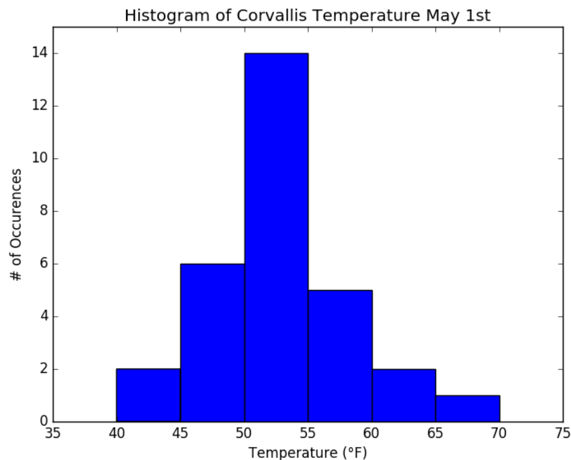
Figure 1.1.6: Histogram of 30 year (1985-2016) temperatures in Corvallis on May 1st. Most years (14 out of the 30) the temperature is between 50 and 55°F. The mean of the distribution is 52.8°F, its standard deviation of \sigma = 5.4^\circ\text{F} represents its width (about 2/3 of all years have temperatures within \pm 1 \sigma of the mean). The histogram, although it approximates well a Gaussian (normal) distribution, is slightly asymmetric such that very warm years (65-70) occur slightly more often than very cold extremes (35-40). The tails of the distribution are the upper and lower bins. They represent rare or extreme events. Only one year was warmer than 65°F. This year (2014) can be regarded as an extreme event. It was a record warm year in Oregon.
