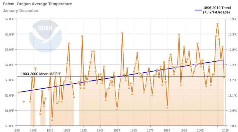
Figure 1.1.7: Annual average temperature changes in Salem, Oregon. Note the large year-to-year variations of 2-3°C and the small overall trend (blue line).
