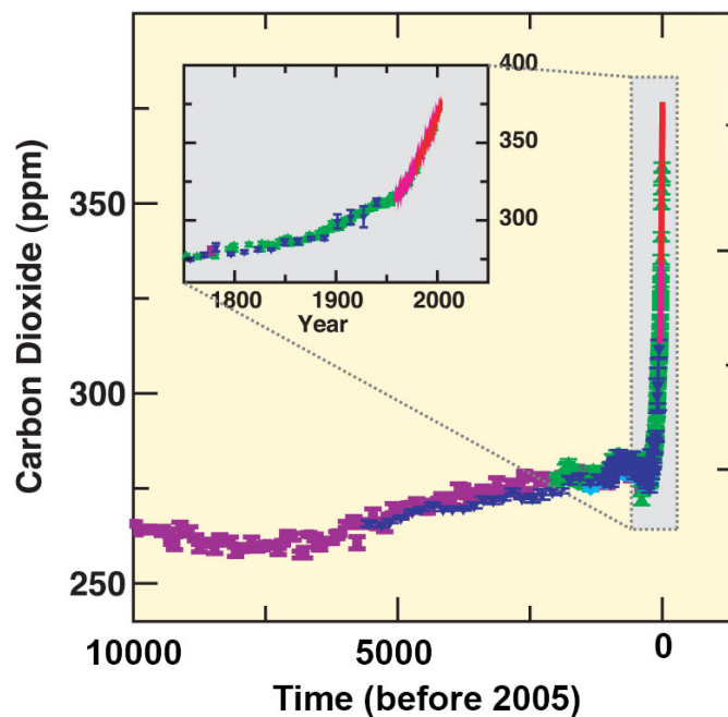
Figure 1.3.8: Ice core CO 2 measurements of ancient air. The different colors indicate different ice cores. The inset zooms into the last 200 years and includes in red the modern air measurements from Mauna Loa (see Figure 8 in Chapter 2). Note that the ice core measurements agree well with the modern data where they overlap. From IPCC (2007) .
