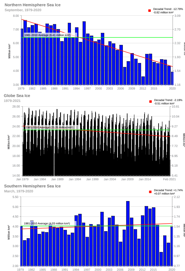
Figure 1.2.4: Changes in late summer sea ice extent in the Arctic (top) and Antarctic (bottom), and global monthly sea ice extent (center). From NOAA .
