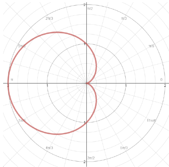
Cardioide r = 1 - \cos(\theta) .
