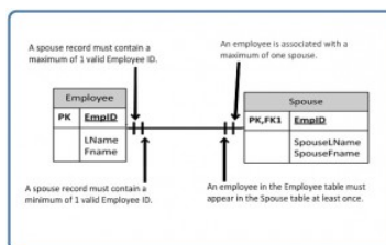
Figure 4.3.7: Example of a one and only one mandatory relationship symbol, by A. Watt.
