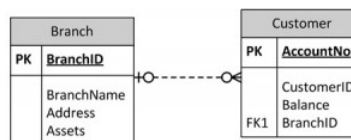
Figure 5.1.5: Examples of bank account tables that contain one entity each, by A. Watt.
