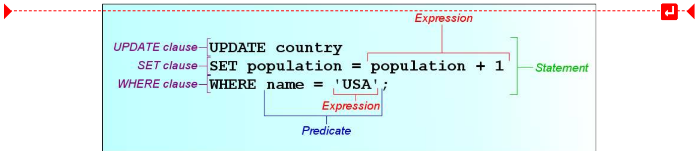
Figure 9.1.1: Example of an SQL Statement. ("Sql statement anatomy" by SqlPac is licensed under CC BY-SA 3.0)
