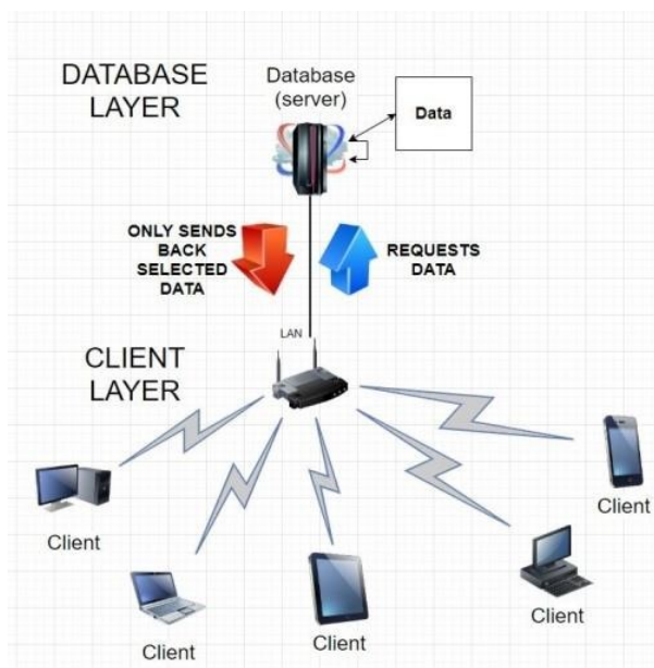
Figure 11.3.1: Visual of two-tier architecture (two layers) (Made via Draw.io, Martin Nguyen, 2020)
