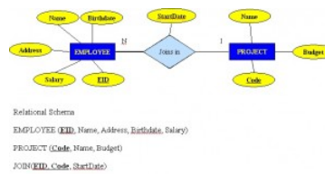
Figure 3.6.2: Example where employee has different start dates for different projects.
