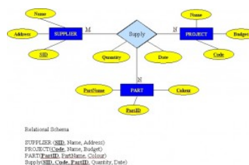
Figure 3.6.4: Example of a ternary relationship.
