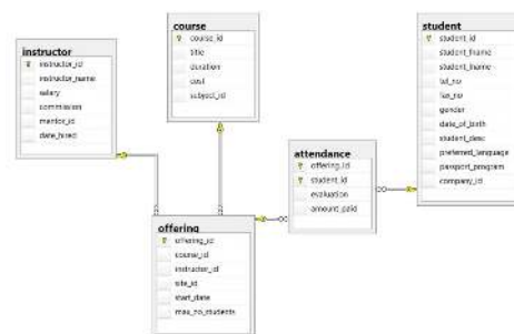
Figure 3.6.9: ERD of school database for questions 7-10, by A. Watt.
