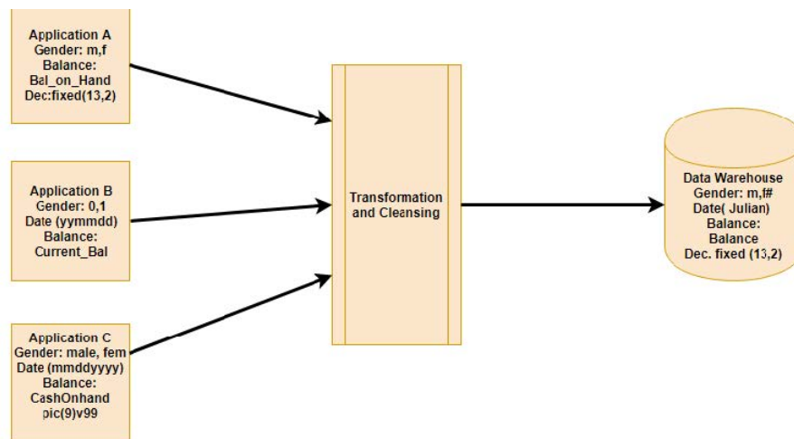
Figure 13.1.1: Sample Data Warehouse (North, 2021)
