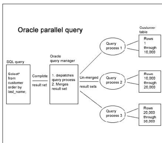
Figure 12.6.1.1: Oracle Parallel Query. (Burleson Consulting, 2014 )
