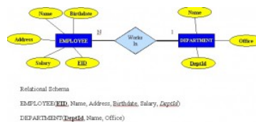
Figure 3.6.1: Example of a one to many relationship.
