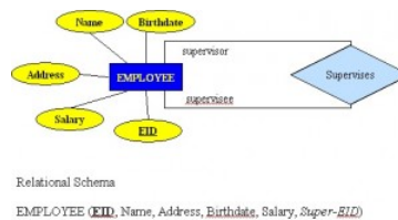
Figure 3.6.3: Example of a unary relationship.
