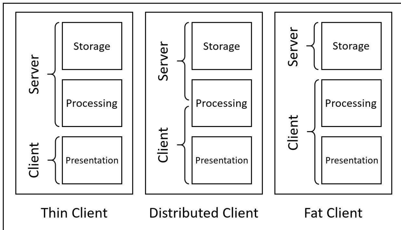
Figure 11.2.1: Client distribution models (made via Microsoft PowerPoint, Michael Nolan 2020)
