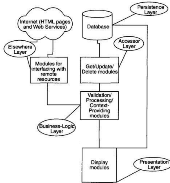
Figure 11.1.1: A graphic demonstrating the architecture of multi tier architecture.
