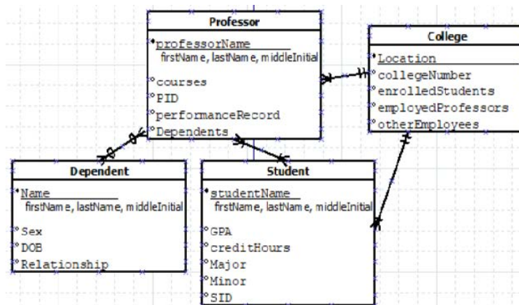
Figure 6.3.8: ER Diagram with Corrected Keys. ("Module_2 - Relationship Diagram for Data Analysis & SQL" by Dr Sarah North, Affordable Learning Georgia)
