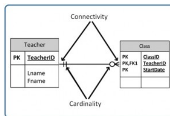
Figure 4.2.1: Position of connectivity and cardinality on a relationship symbol, by A. Watt.
