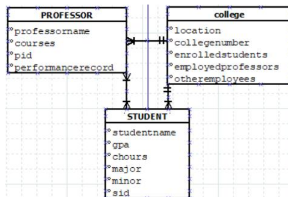
Figure 6.3.6: ER Diagram With Corrected Relation Formatting. ("Module_2 - Relationship Diagram for Data Analysis & SQL" by Dr Sarah North, Affordable Learning Georgia)
