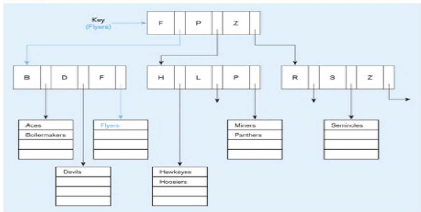
Figure 12.5.1: Three Types of File Organizations (Venkataraman, R., Topi, H. (2011))
