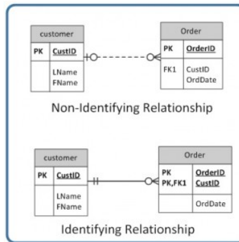
Figure 4.3.1: Identifying and non-identifying relationship, by A. Watt.
