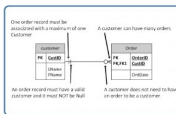
Figure 4.3.3: Example usage of a zero to many optional relationship symbol, by A. Watt.
