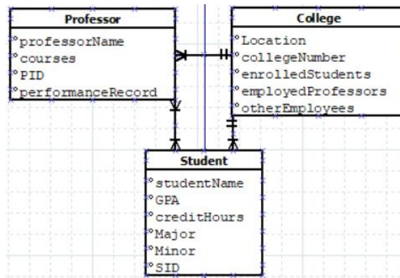
Figure 6.3.7: ER Diagram With Corrected Attribute Format. ("Module_2 - Relationship Diagram for Data Analysis & SQL" by Dr Sarah North, Affordable Learning Georgia)
