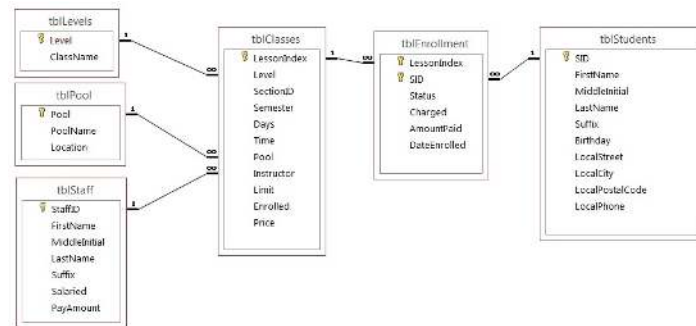
Figure 4.3.16: ERD for questions 1-5. (Diagram by A. Watt.)
