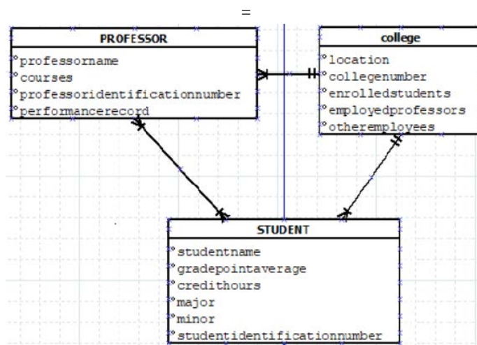
Figure 6.3.5: ER Diagram With Corrected Relation Types. ("Module_2 - Relationship Diagram for Data Analysis & SQL" by Dr Sarah North, Affordable Learning Georgia)
