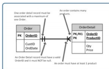
Figure 4.3.9: Example of a one to many mandatory relationship symbol, by A. Watt.
