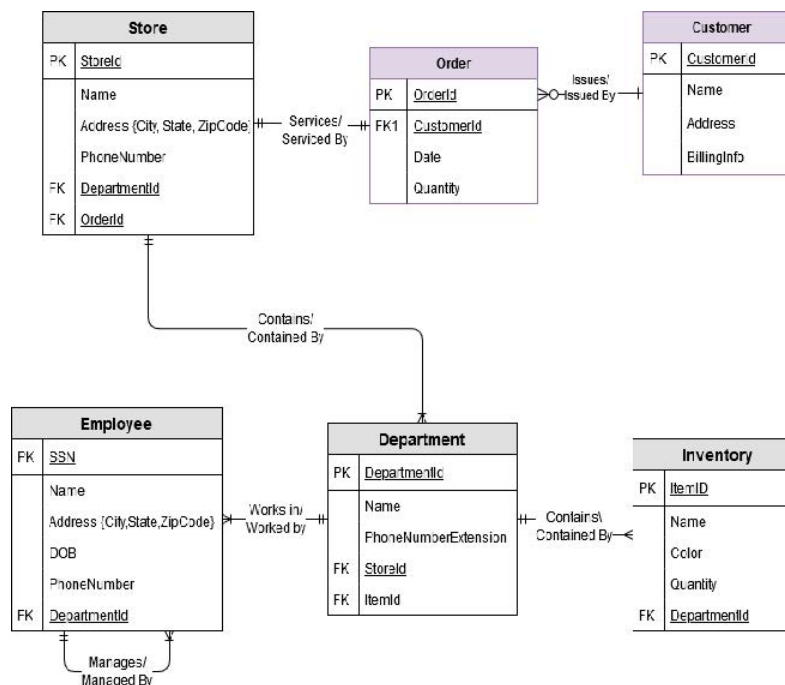
Figure 6.4.1: Store ER Diagram. ("Module_2 - Relationship Diagram for Data Analysis & SQL" by Dr Sarah North, Affordable Learning Georgia)
