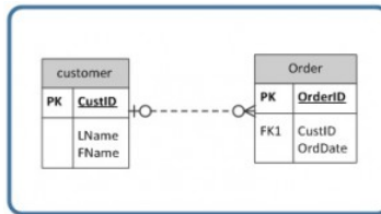
Figure 4.3.12: The relationship between a Customer table and an Order table, by A. Watt.
