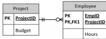
Figure 5.1.7: Solution: separate tables for Project and Employee, by A. Watt.
