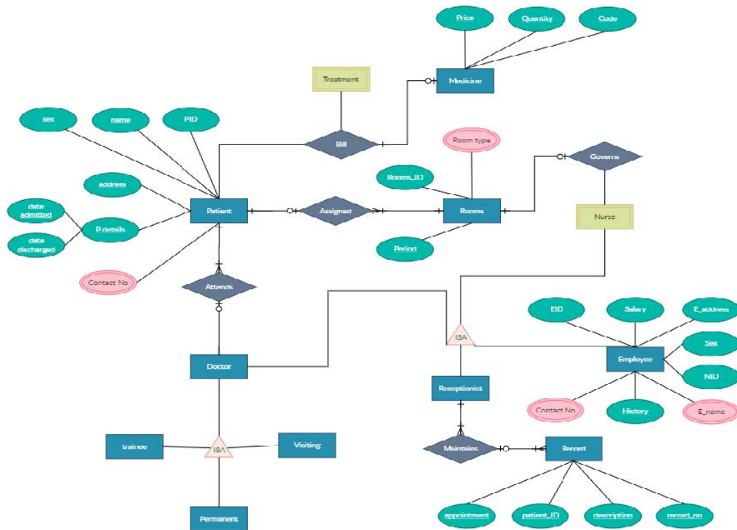
Figure 6.3.1: Basic Hospital ERD. ("Module_2 - Relationship Diagram for Data Analysis & SQL" by Dr Sarah North, Affordable Learning Georgia)
