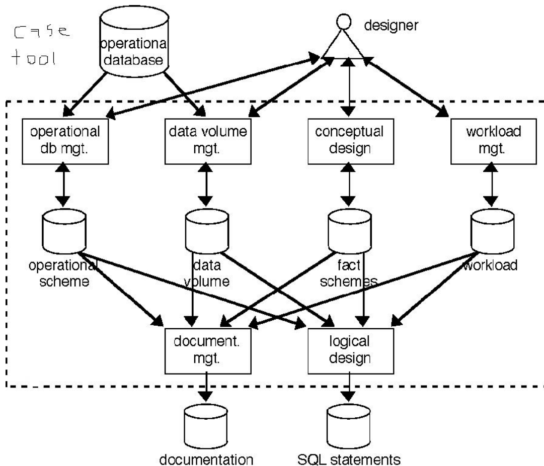
Figure 13.1.2: Database Diagram (North, 2021)
