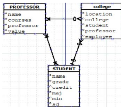
Figure 6.3.3: College, Professor, Student ER Diagram. ("Module_2 - Relationship Diagram for Data Analysis & SQL" by Dr Sarah North, Affordable Learning Georgia)
