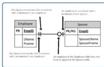
Figure 4.3.5: Example usage of a zero to one optional relationship symbol, by A. Watt.
