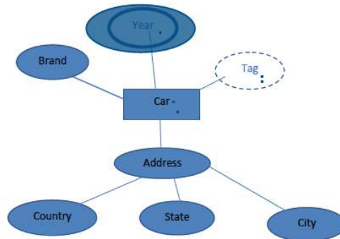
Figure 7.1.1: Multiple Different Types of Attributes. ("Module_3: Mapping ER to Schema, Normalization" by Dr Sarah North, Affordable Learning Georgia is licensed under CC BY 4.0)
