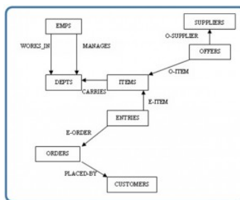
Figure 2.1.1: Network model diagram.
