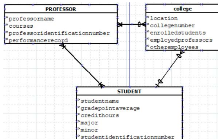
Figure 6.3.4: ER Diagram with Corrected Attribute Names. ("Module_2 - Relationship Diagram for Data Analysis & SQL" by Dr Sarah North, Affordable Learning Georgia)
