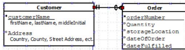
Figure 6.4.1: Entity-to-Entity Relation. ("Module_2 - Relationship Diagram for Data Analysis & SQL" by Dr Sarah North, Affordable Learning Georgia)
