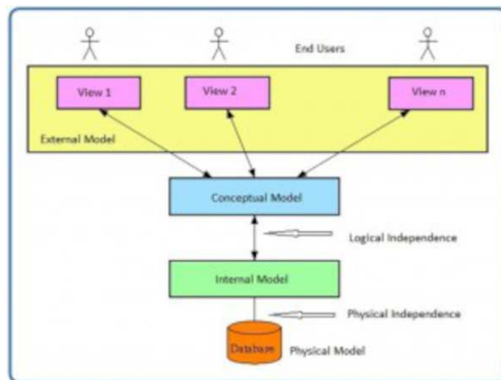
Figure 2.3.1: Data abstraction layers. (CC-BY-SA; Adrienne Watt via Website )
