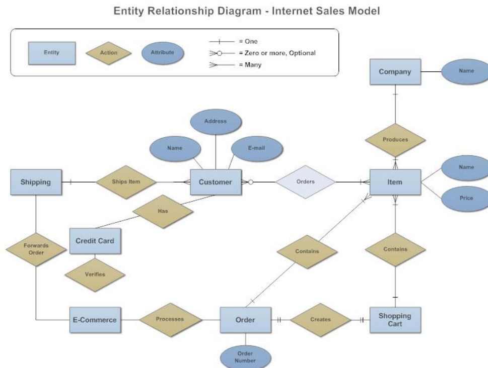
Figure 6.1.1: Original Style ERD ("Module_2 - Relationship Diagram for Data Analysis & SQL" by Dr Sarah North, Affordable Learning Georgia)
