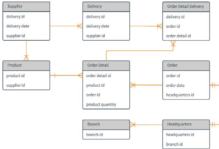
Figure 6.1.2: New Style ERD. ("Module_2 - Relationship Diagram for Data Analysis & SQL" by Dr Sarah North, Affordable Learning Georgia)
