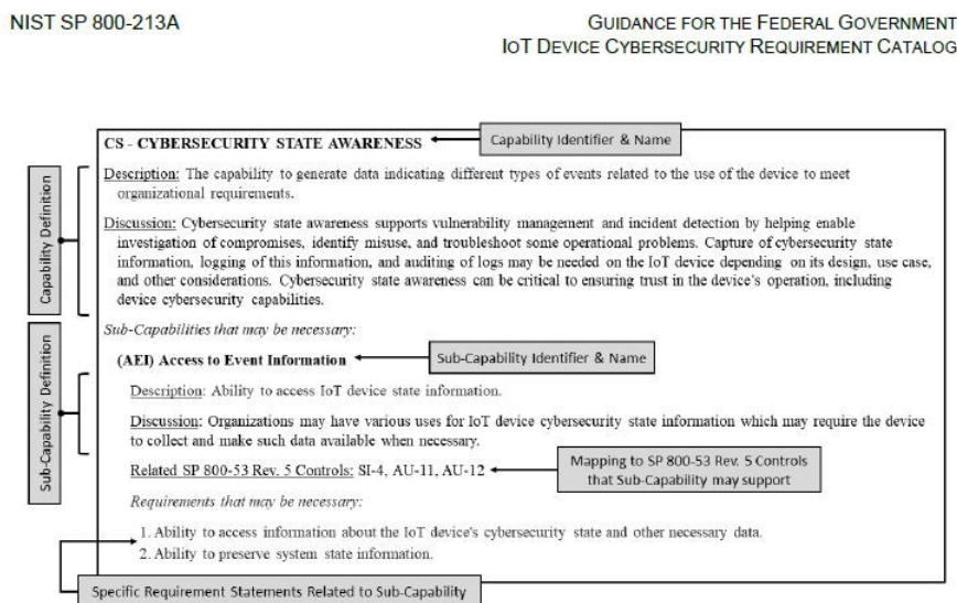
Figure 1: Capability and Sub-Capability Structure
