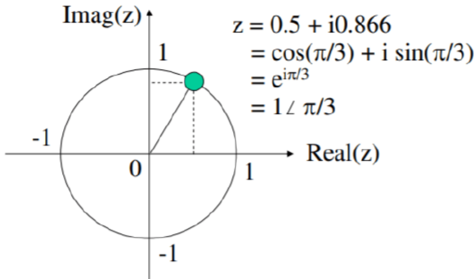
Figure 2.7.1: Imaginary number z represented as a graph on the Cartesian plane, with the x-axis representing the real part of z and the y-axis representing the imaginary part of z .
