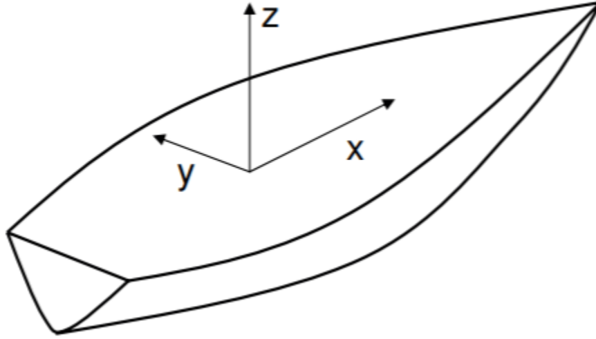
Figure 10.1.1: Convention for the body-referenced coordinate system on a vehicle: x is forward, y is sway to the left, and z is heave upwards. Looking forward from the vehicle "helm," roll about the x axis is positive counterclockwise, pitch about the y -axis is positive bow-down, and yaw about the z -axis is positive turning left.
