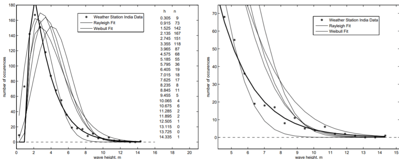
Figure 6.8.1: compare and contrast the long-term distribution of actual wave heights against the data set's Rayleigh fit and several trial Weibull fits.
