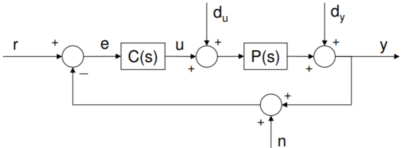
Figure 11.5.1, accounting for the additional factors of process disturbance d , reference command r , and sensor noise n .
