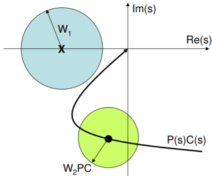
Figure 12.5.1: graph of a system that meets the criteria for good performance as outlined above. The disk at the critical point X , with radius |W_1| , does not intersect with the disk of radius |W_2PC| centered on the nominal locus PC .
