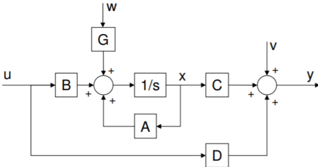
Figure 11.4.1: block diagram illustrates the relationship between the different variables introduced in Equations 11.4.1 - 11.4.2.
