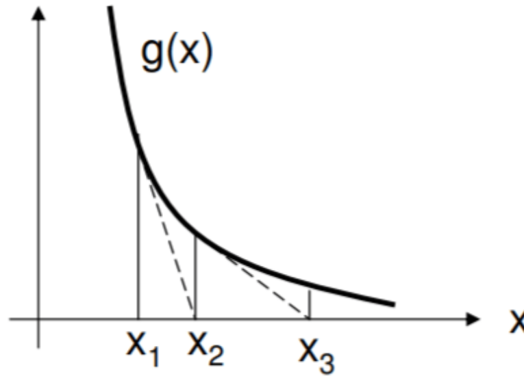
Figure 7.2.2: a error that must be considered when Newton's method is used to approximate the zero of a function; the lines tangent to the points x_1 through x_3 have progressively flatter slopes, and thus become increasingly likely to overshoot the zero of g(x) that is desired.
