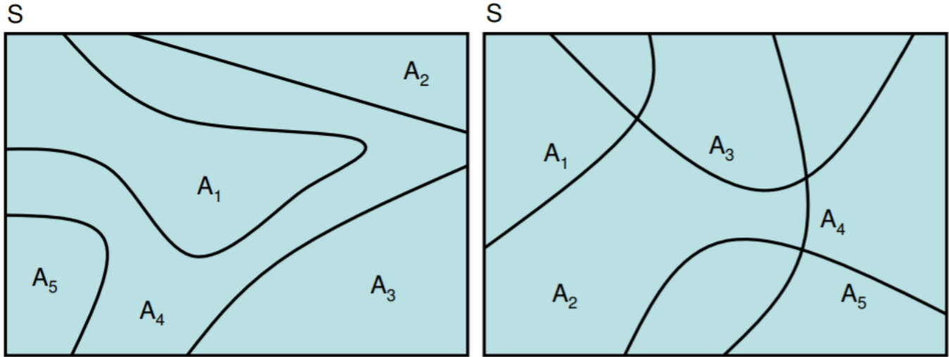
Figure 3.1.1: A visual representation of simple events (left), where A_1 through A_5 do not overlap each other, compared to composite events (right), where events A_1 through A_5 overlap so that a sample may invoke multiple events.
