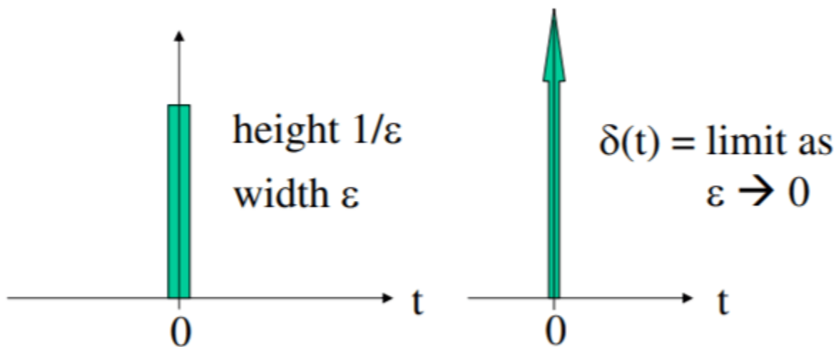
Figure 2.4.1: graph of rectangle with area = 1 centered at t = 0 , showing how the limit changes as the rectangle width \epsilon approaches 0.
