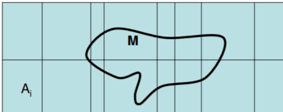
3.1.2: A visual representation of an event space completely occupied by simple events A_i , and an event M that incorporates elements of multiple possible A_i .
