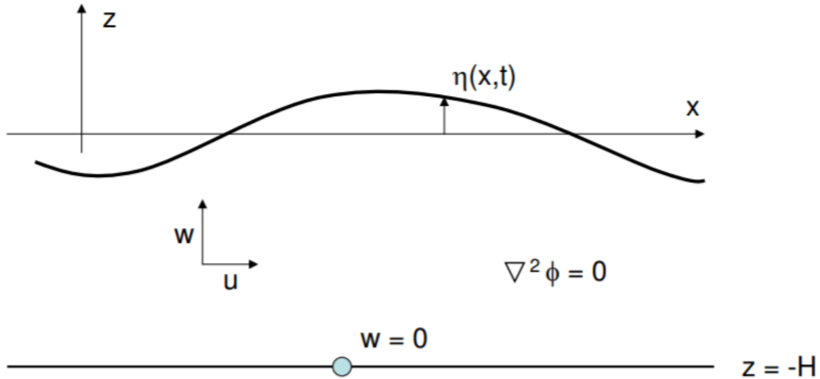
Figure 6.4.1: the degrees of freedom available to moving water at the ocean surface vs. at the sea floor.
