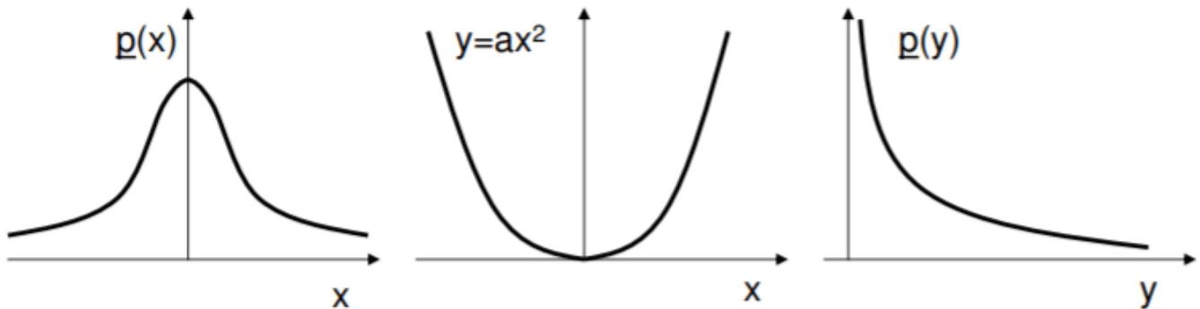
Figure 3.7.1: Graph of the function y = ax^2 from the example problem above (center). Graphs of the probability density functions of the x values and of the y values of y = ax^2 (left and right, respectively).
