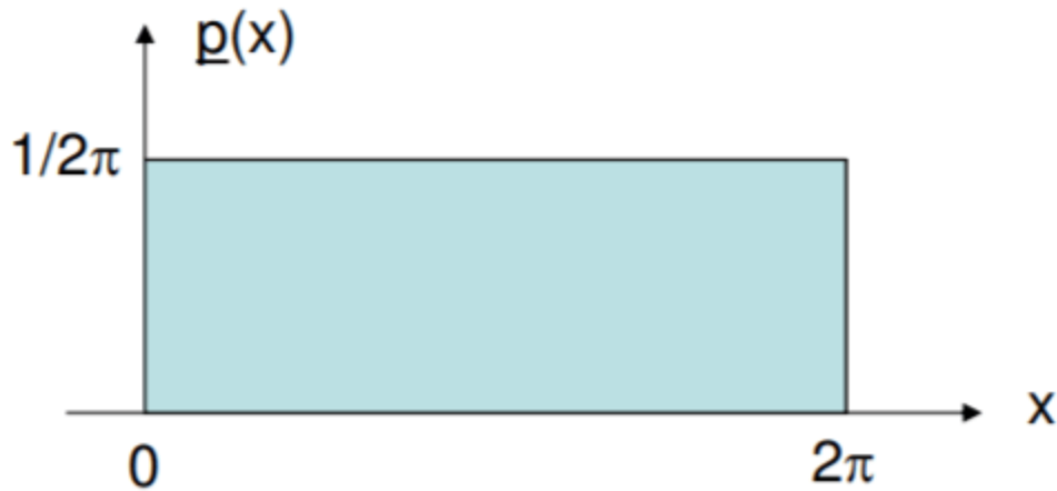
Figure 3.5.1: Graph of the example probability distribution function given above, with a random variable x that is equally likely to occur at any value between 0 and 2\pi .
