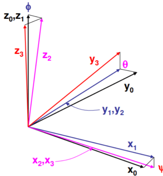
Figure 9.2.1: successive application of three Euler angles transforms the original coordinate frame into an arbitrary orientation.
