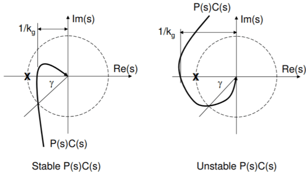
Figure 12.3.1: comparison of graphs demonstrates how differences in the value of the gain margin ( k_g ) determine the stability or instability of the OL transfer function, as explained in the previous section.
