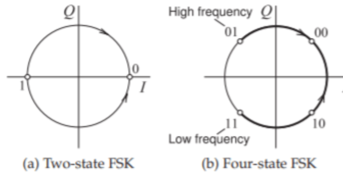
Figure 2.6.2: Constellation diagrams of FSK modulation. In two-state FSK a symbol indicates whether a bit is a '0' or a '1'. In four-state FSK there are four symbols and each symbol has a different frequency and indicates the values of two bits.
