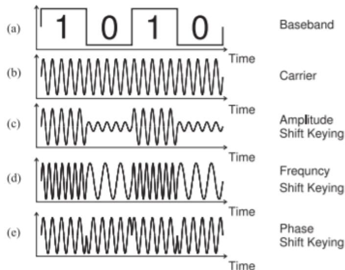
Figure 2.5.2: Modes of digital modulation: (a) modulating bitstream; (b) carrier ; (c) carrier modulated using amplitude shift keying (ASK); (d) carrier modulated using frequency shift keying (FSK); and (e) carrier modulated using binary phase shift keying (BPSK).
