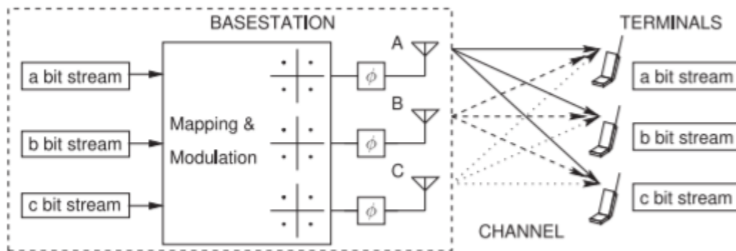
Figure 5.8.1: A massive MIMO system with beams from the basestation antennas to each terminal unit.
