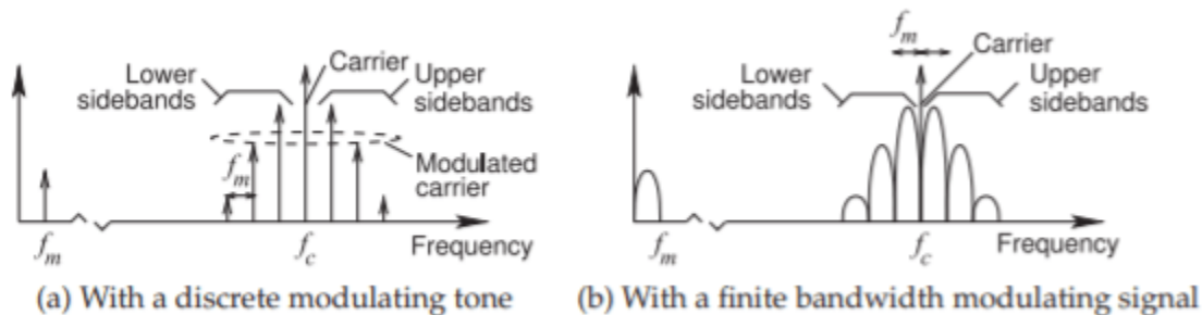
Figure 2.4.4: Spectrum of a phase-modulated carrier which includes the carrier at f_c and upper and lower sidebands with the spectrum of the discrete modulating signal at f_m .
