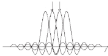
Figure 5.7.1: OFDM spectrum with four subcarriers showing orthogonality.
