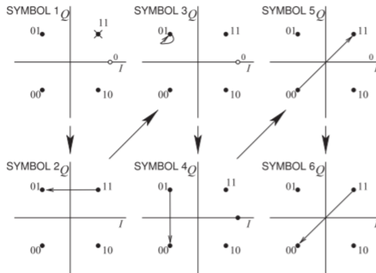
Figure 2.13.10: Constellation diagram and transitions for the bit sequence 110101001100 sent as the set of symbols 110101001100 using QPSK. Note that symbols 2 and 3 are identical, so there is no transition. The SYMBOL numbers indicated reference the symbol at the end of the transition (end of the arrow). The assignment of bits to symbols (e.g., assigning the bits '11' to the symbol in the first quadrant) is arbitrary in general but the assignment of symbols is defined in a particular standard.
