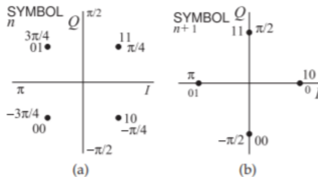
Figure 2.13.11: Constellation diagram of \pi/4 -QPSK modulation: (a) initial constellation diagram at one symbol; and (b) the constellation diagram at the time of the next symbol.
