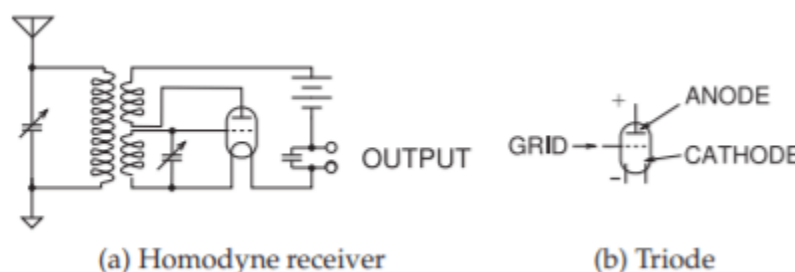
Figure 3.3.1: Colebrook's original homodyne receiver: (a) circuit with an antenna, tunable bandpass filter, and triode amplifier; and (b) triode vacuum tube.
