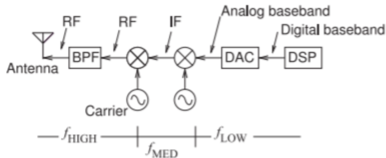
Figure 1.3.6: A simple transmitter with low, f_{\text{LOW}} , medium, f_{\text{MED}} , and high frequency, f_{\text{HIGH}} , sections. The mixers can be idealized as multipliers, shown as circles with crosses, that boost the frequency of the input baseband or IF signal by the frequency of the carrier.
