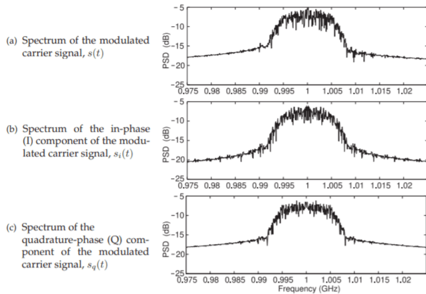
Figure 3.7.12: Spectra of the digitally modulated RF signals for 1024 symbols (4096 bits), a time duration of 102.4 \mu s, and using a 524,288 point FFT.
