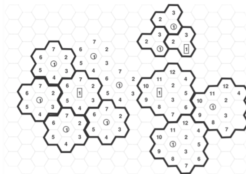
Figure 4.11.1: Cells arranged in clusters. Shown are 3 – cell clusters (top right), 7 – cell clusters (bottom left), and 12 – cell clusters (bottom right).
