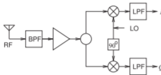
Figure 3.14.7: Direct conversion quadrature demodulator.
