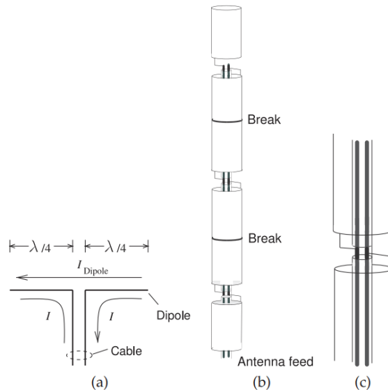
Figure 4.3.4: Dipole antenna: (a) current distribution; (b) stacked dipole antenna; and (c) detail of the connection in a stacked dipole antenna.
