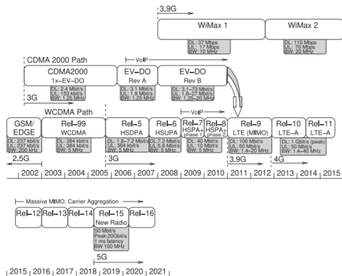
Figure 5.16.4: Timeline for implementation of 3G, 4G and 5G. DL indicates the downlink data rate; UL indicates the uplink data rate; BW indicates the channel bandwidth. Development supports Internet protocol (IP) and voice over IP (VoIP). The two 3G paths become a single long term evolution (LTE) path. LTE is the concept of smoothly evolving through 4G and into 5G utilizing existing infrastructure and adding capability [25]. Beginning with Release 99 (Rel-99) the timeline is controlled by 3GPP. The dates refer to the first significant commercial availability of the standard and the official release dates can be found at http://www.3gpp.org .
