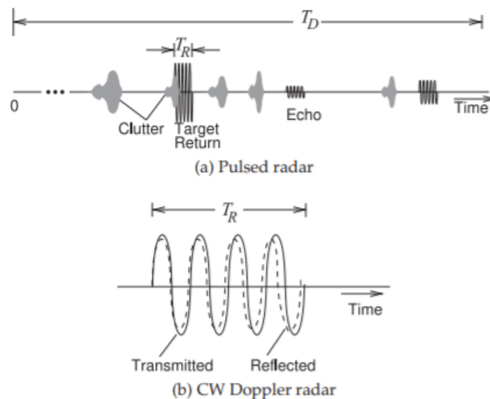
Figure PageIndex4: Radar returns. The strength of the reflected signal depends on the radar cross section (RCS), \sigma , of the target. \sigma = 0.01 \text{ m}^2 for a bird, < 0.1 \text{ m}^2 for a stealth aircraft, 1 \text{ m}^2 for a human, 2\text{--}6 \text{ m}^2 for a conventional fighter plane, 100 \text{ m}^2 for a large commercial aircraft, 200 \text{ m}^2 for a truck, 10,000\text{--}100,000 \text{ m}^2 for a container ship.
