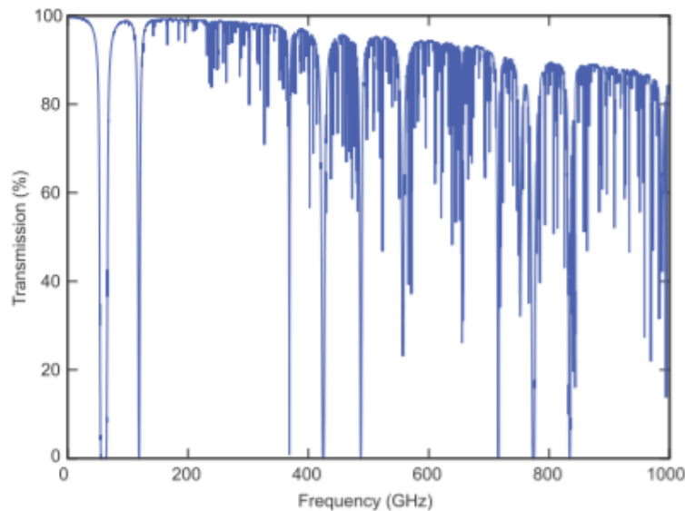
Figure 1.2.1: Atmospheric transmission at Mauna Kea, with a height of 4.2 km, on the Island of Hawaii where the atmospheric pressure is 60% of that at sea level and the air is dry with a precipitable water vapor level of 0.001 mm. After [5].
