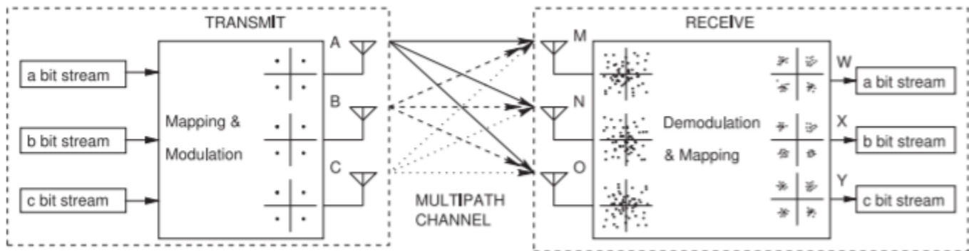
Figure 5.7.4: A MIMO system showing multiple paths between each transmit antenna and each receive antenna.
