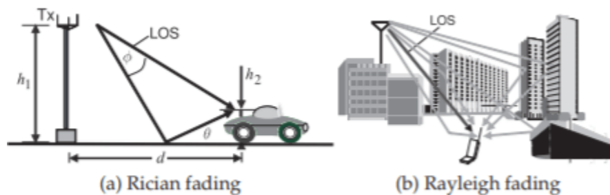
Figure 4.6.1: Multipath propagation: (a) line of sight (LOS) and ground reflection paths only; and (b) in an urban environment.
