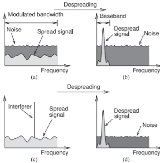
Figure 5.6.2: Increase in SNR obtained by despreading a spread-spectrum signal: (a) the spectrum of noise and a spread-spectrum signal that has a power below the level of the noise; (b) the despread signal, where the power distribution of the noise is not changed but the despread signal is confined to a narrower bandwidth called the baseband bandwidth; (c) a signal with a single-tone interferer; and (d) after despreading where the power of the interferer spread across the the original bandwidth.
