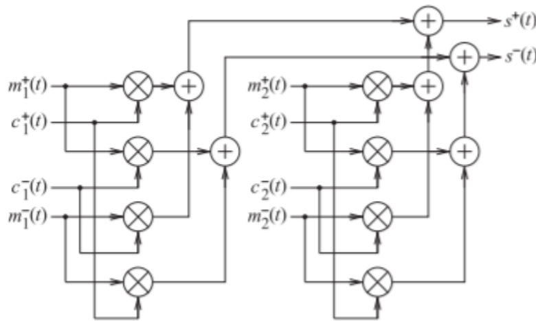
Figure 3.4.5: Differential implementation of a Hartley SSB-SC modulator: s^+(t) , s^-(t) are the positive and negative components of the differential modulated signal s(t) ; (c_1^+(t), c_1^-(t)) is the differential carrier; (m_1^+(t), m_1^-(t)) is the differential quadrature-modulated IF carrier; (c_2^+(t), c_2^-(t)) is the differential carrier shifted 90^\circ ; and m_2^+(t) and m_2^-(t) are the 90^\circ phase-shifted versions of m_1^+(t) and m_1^-(t) , respectively.
