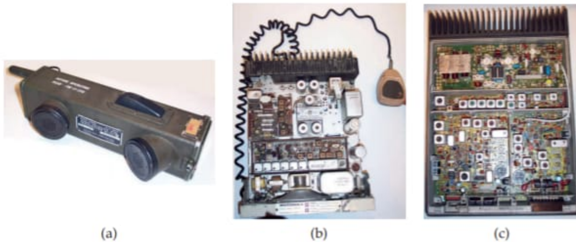
Figure 5.2.1: Early radios: (a) walkie-talkie with a push-to-talk (PTT) switch on top and using simplex communication; (b) Motorola business dispatcher two-way radio operating at 33.220 MHz designed in the 1960s as a dash mount unit; and (c) the Mitrek two-way radio designed by Motorola in 1977. The radio has two PC boards and was crystal controlled with a channel scanning control head. The radio was trunk mounted, with the control head, microphone, and speaker mounted under the dash board. The units in (b) and (c) are approximately 20 cm long.
