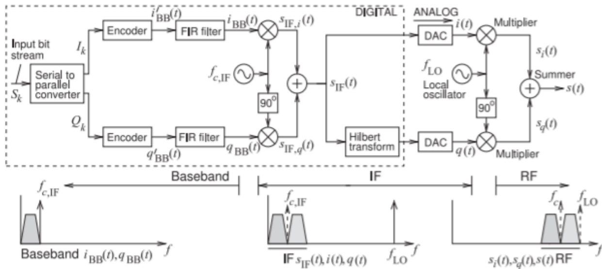
Figure 3.7.15: Complete SDR transmitter with bistream S_k input to an IF quadrature modulator producing a DSB-SC signal, s_{IF} , with IF carrier of frequency f_{c,IF} . Each finite-impulse response (FIR) filter implements raised cosine filtering. Then an analog SSB-SC quadrature modulator upconverts the IF as a DSB-SC RF signal centered at the RF carrier frequency f_c = f_{LO} - f_{c,IF} . The Hilbert transform implements a 90° phase shift.
