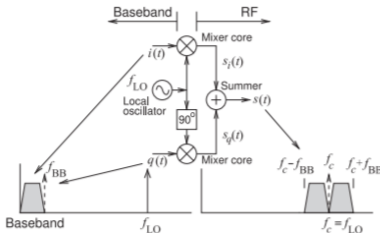
Figure 3.15.1: Double-sideband suppressed-carrier (DSB-SC) modulation. Quadrature modulator with independent modulating baseband signals i(t) , the in-phase component input to the in-phase mixer core, and q(t) , the quadrature component driving the quadrature-phase mixer core. This results in a modulated signal with two sidebands around the local oscillator or carrier frequency. Each RF sideband has a mix of the information in i(t) and q(t) .
