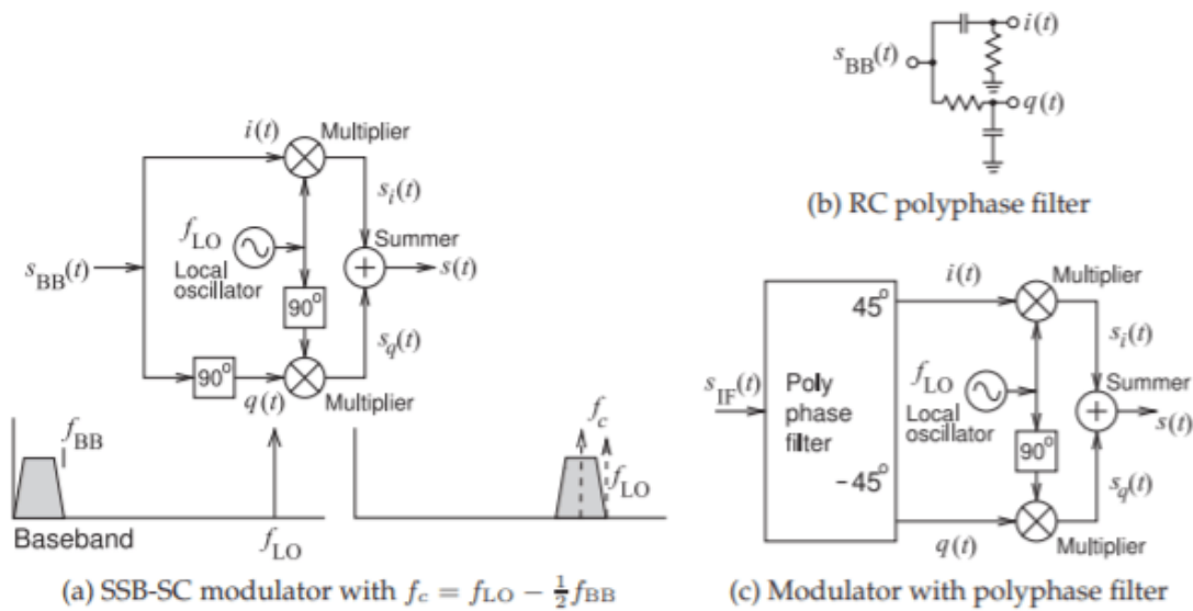
Figure 3.7.4: Quadrature modulator as a single-sideband, suppressed-carrier (SSB-SC) modulator. At the design frequency the polyphase filter in (b) the phase of i(t) is advanced by 45^\circ and the phase of q(t) is retarded by 45^\circ .
