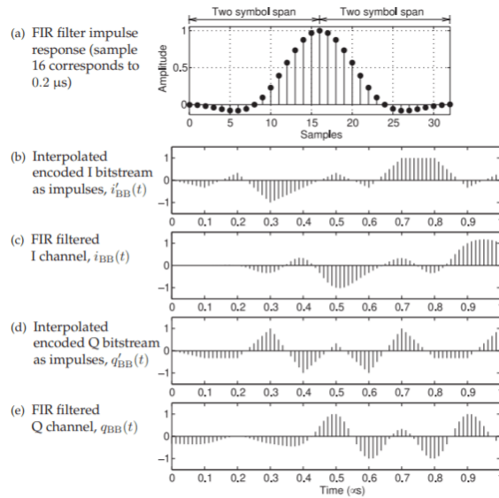
Figure 3.7.18: Sampled baseband signals for 16-QAM modulation corresponding to the analog baseband signals in Figure 3.7.17.
