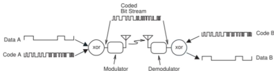
Figure 5.16.1: Depiction of direct sequence CDMA transmission. If code B is code A, then data B is the same as data A with some corruption by noise.
