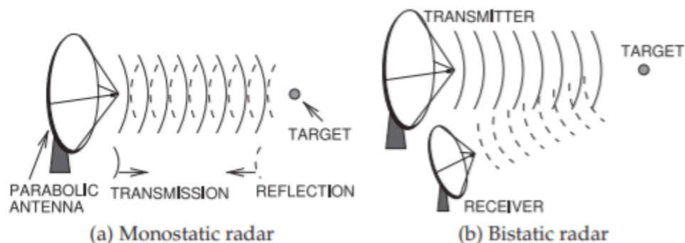
Figure 5.10.1: Radar system: (a) monostatic radar with the same site used for transmission of the radar signal and receipt of the reflection from the target; and (b) bistatic radar with different transmit and receive sites.
