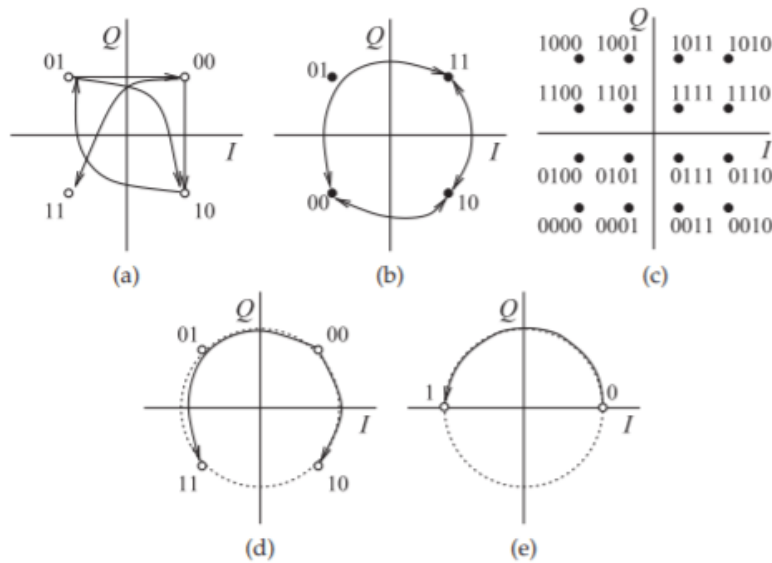
Figure 2.13.18: Constellation diagrams for various modulation formats: (a) OQPSK; (b) GMSK; (c) 16-QAM; (d) SOQPSK (also FOQPSK); and (e) SBPSK.
