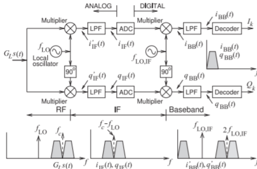
Figure 3.9.1: SDR receiver with RF input signal G_L s(t) with the first LO frequency, f_{LO} , less than the carrier signal f_c . Note that 2f_{LO,IF} = f_c - f_{LO} .
