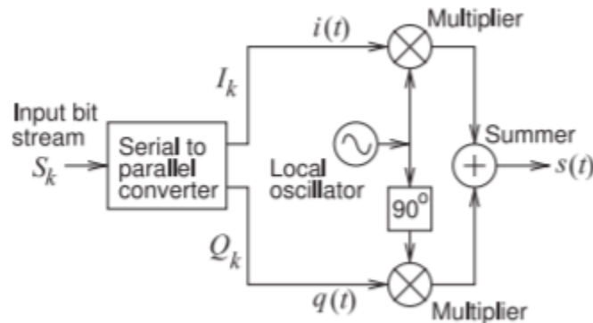
Figure 3.4.6: Quadrature modulator block diagram. An input bitstream, S_k , is divided into two bitstreams, I_k and Q_k , which are applied to the multipliers as (possibly filtered) waveforms i(t) and q(t) . The output of the multipliers (appropriately filtered) are summed to yield a modulated carrier signal, s(t) . The 90^\circ block shifts the carrier by 90^\circ .
