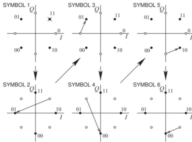
Figure 2.13.12: Constellation diagram states and transitions for the bit sequence 110101001000 sent as the set of symbols 110101001000 using \pi/4 -QPSK modulation.
