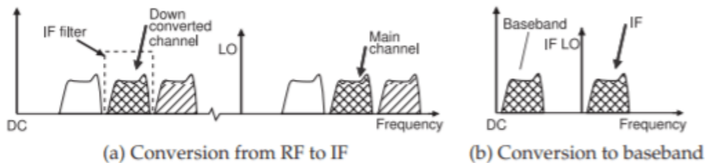
Figure 3.14.4: Frequency conversion using superheterodyne mixing.
