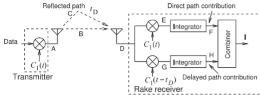
Figure 5.16.3: Rake receiver used to decode two paths, a direct path and a path with excess delay t_D . The integrators eliminate incorrectly recovered data.
