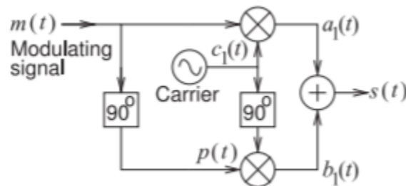
Figure 3.1.1: Hartley modulator implementing singlesideband suppressed-carrier (SSB-SC) modulation. The “90°” blocks shift the phase of the signal by +90°. The mixer indicated by the circle with a cross is an ideal multiplier, e.g. a_1(t) = m(t) \cdot c_1(t) .
