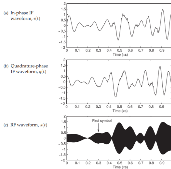
Figure 3.7.19: Waveforms in the RF quadrature modulator where the in-phase IF signal i(t) is just the output, s_{IF}(t) of the IF quadrature multiplier. The first 0.2 \mu s can be ignored as the FIR filter output is settling. (The IF sampling interval is 3.125 \text{ ns} . The Hilbert transform operates on 2^{16} = 65,537 IF samples or 204.8 \mu s of data corresponding to 2048 symbols or 8192 bits. The RF time step is 31.25 \text{ ps} . The RF signal spectrum was calculated using a 2^{22} point FFT.
