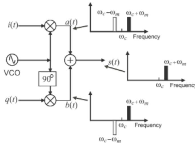
Figure 3.6.2: Quadrature modulator showing intermediate spectra.
