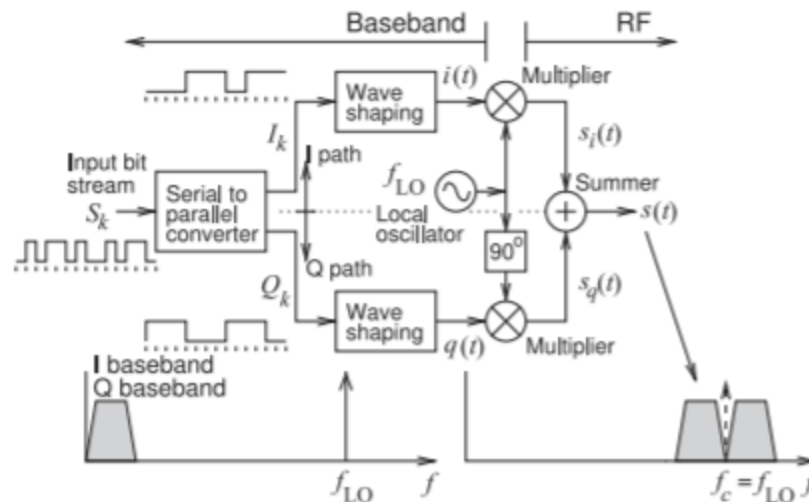
Figure 3.7.7: Digital quadrature modulators with independent binary I and Q channels yielding double sideband, suppressed carrier (DSB-SC) modulation.
