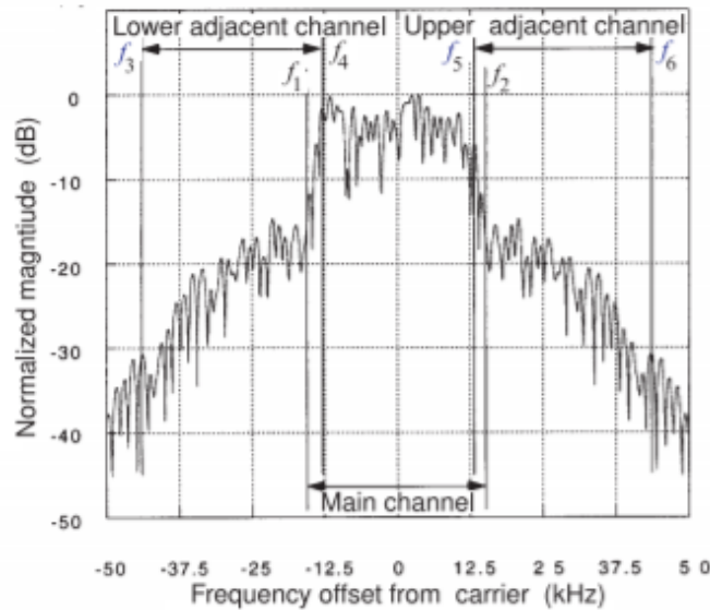
Figure 2.8.2: Spectrum defining adjacent channel and main channel integration limits using a \pi/4 -DQPSK modulation scheme.
