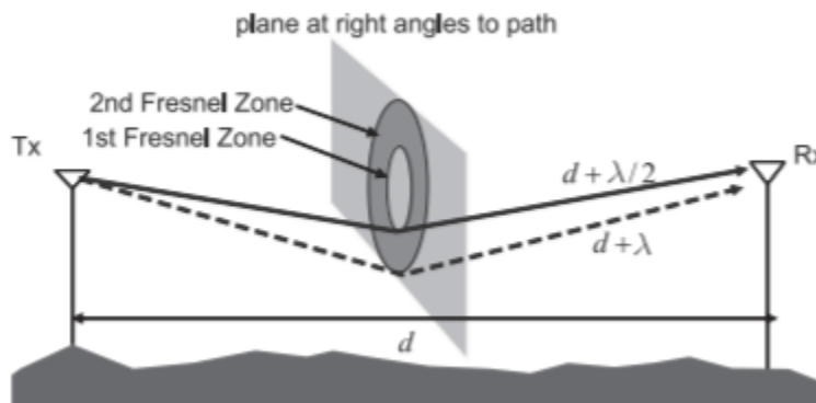
Figure 4.6.11: Fresnel zones in a plane perpendicular to the LOS path, which has length d .
