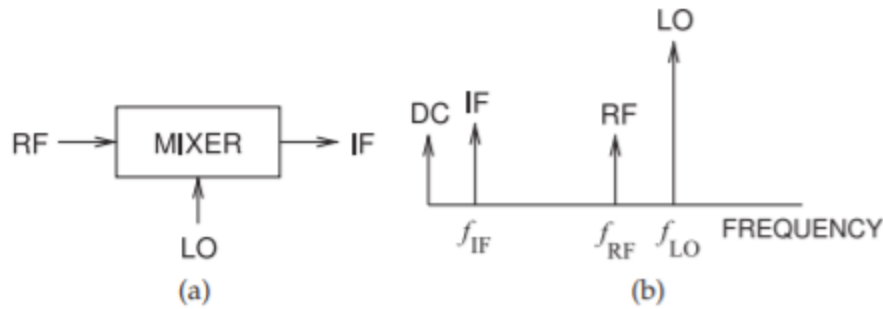
Figure 3.4.3: Simple mixer circuit: (a) block diagram; and (b) spectrum.
