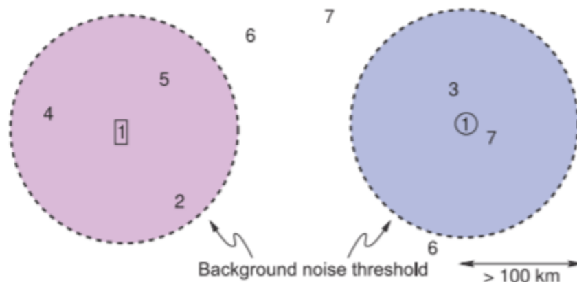
Figure 5.3.2: Interference in a conventional radio system. The two transmitters, 1, are at the centers of the coverage circles defined by the background noise threshold.
