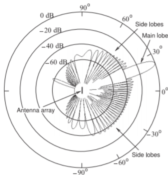
Figure 4.12.2: Electric field pattern from a 30 element array of antennas spaced 0.65\lambda apart. The sidelobe levels are about 40 dB below the power level of the main lobe. The same signal is presented to the antenna elements except that phases of the signal at each antennas is adjusted to produce a main beam directed at 20 degrees. The signals to each antenna are thus correlated. After [29].
