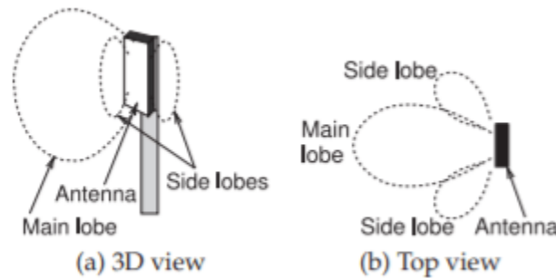
Figure 4.5.1: Field pattern produced by a microstrip antenna.
