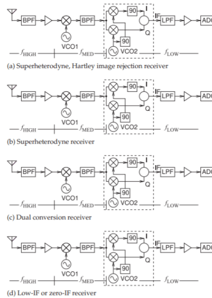
Figure 3.14.2: Architectures of modern receivers: (a) superheterodyne receiver using the Hartley architecture for image rejection; (b) superheterodyne receiver; (c) dual-conversion receiver; and (d) low-IF or zero-IF receiver. BPF, bandpass filter; LPF, lowpass filter; ADC, analog-to-digital converter; VCO, voltage-controlled oscillator; 90°, 90° phase shifter; f_{\text{HIGH}} , f_{\text{MED}} , and f_{\text{LOW}} indicate relatively high-, medium-, and low-frequency sections.
