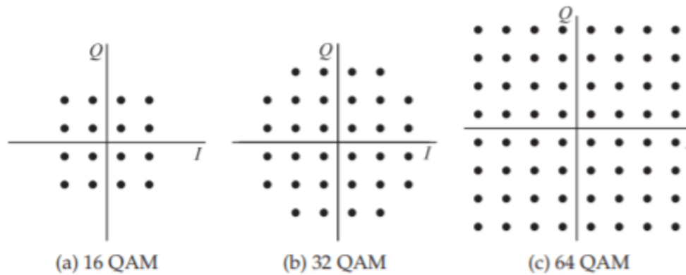
Figure 2.13.20: QAM constellation diagrams.
