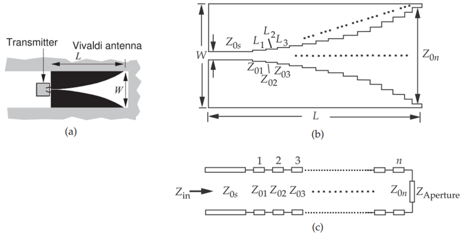
Figure 4.3.5: Vivaldi antenna showing design procedure: (a) the antenna; (b) a stepped approximation; and (c) transmission line approximation. In (a) the black region is a metal sheet.
