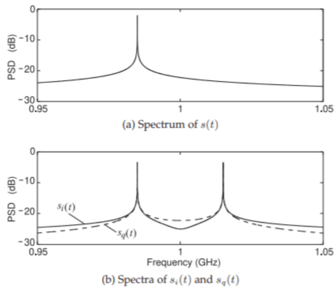
Figure 3.7.5: Spectra of the modulated signal with f_{LO} = 1 GHz. (Simulated time = 65.536 \mu s , 223 point FFT.)
