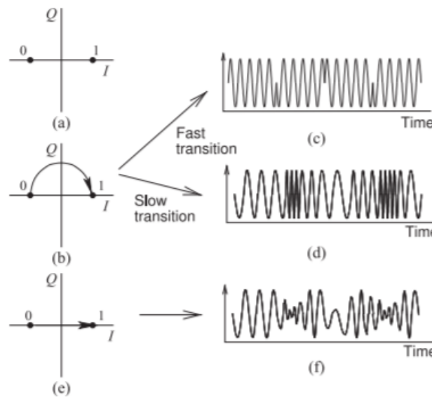
Figure 2.13.6: BPSK modulation: (a) constellation diagram; (b) constellation diagram with a constant amplitude transition; (c) time-domain waveform if the transition is fast; (d) time-domain waveform if the transition is slow; (e) constellation diagram with transition through the origin; and (f) time-domain waveform if the transition goes through the origin and is slow.
