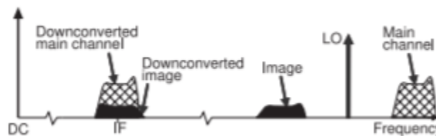
Figure 3.14.5: Frequency conversion using heterodyne mixing showing the effect of image distortion with the down-converted image overlapping the down-converted main channel.
