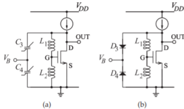
Figure 3.3.2: A common source Hartley voltage-controlled oscillator (VCO): (a) with nonlinear capacitors; and (b) with diodes which have a variable capacitance when reverse biased.
