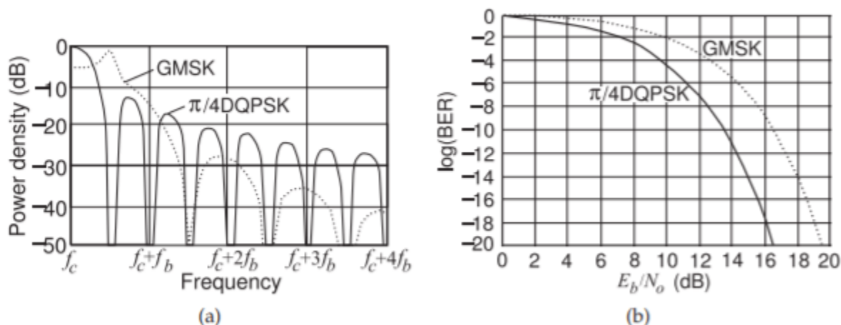
Figure 2.8.4: Comparison of GMSK and \pi/4 DQPSK: (a) power spectral density as a function of frequency deviation from the carrier; and (b) BER versus signal-to-noise ratio (SNR) as E_b/N_o (or energy per bit divided by noise per bit).
