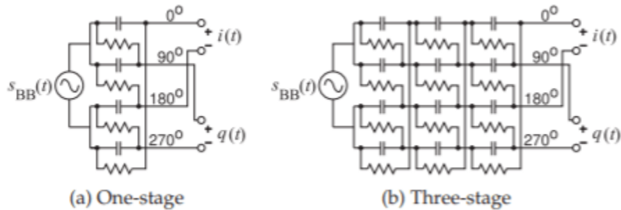
Figure 3.16.2: Differential polyphase filters.
