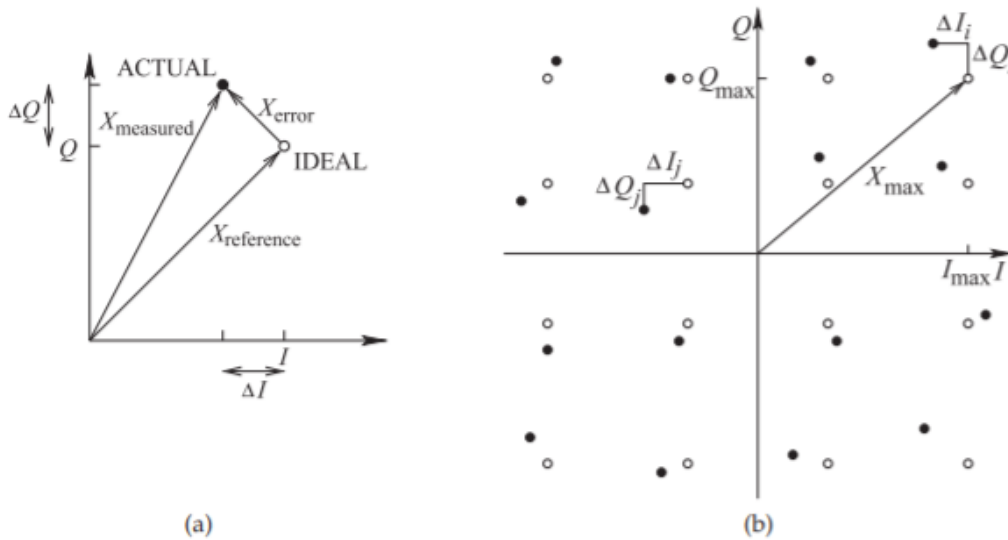
Figure 2.8.5: Partial constellation diagram showing quantities used in calculating EVM: (a) definition of error and reference signals; and (b) error quantities used when constellation points have different powers.
