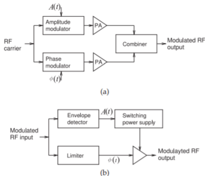
Figure 3.14.1: Polar modulator architectures: (a) amplitude- and phasemodulated components amplified separately and combined; and (b) the amplitude used to modulate a power supply driving a saturating amplifier with phase modulated input.
