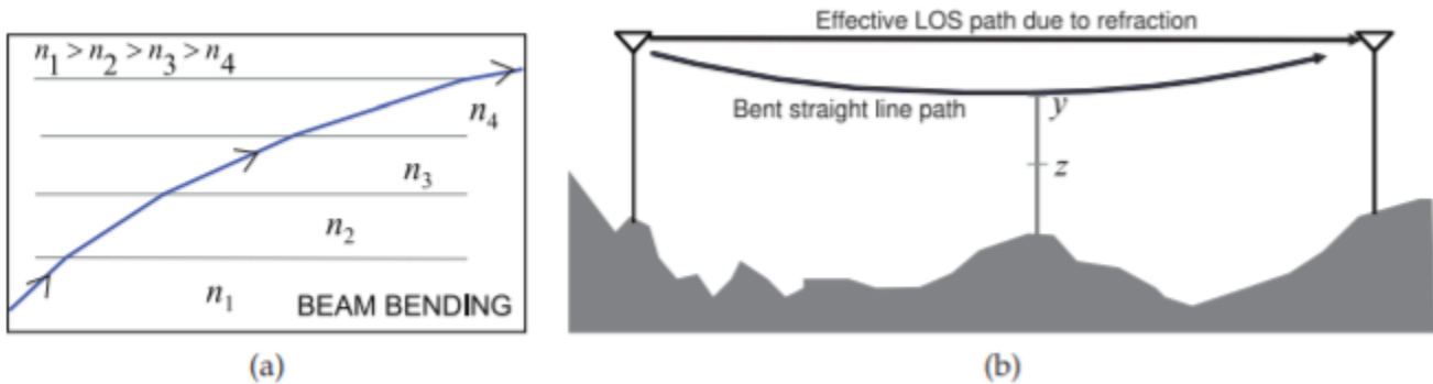
Figure 4.6.10: Beam bending by density variation in air: (a) refraction index profile with the air density reducing with height; and (b) incorporating beam bending in a curved-earth model.
