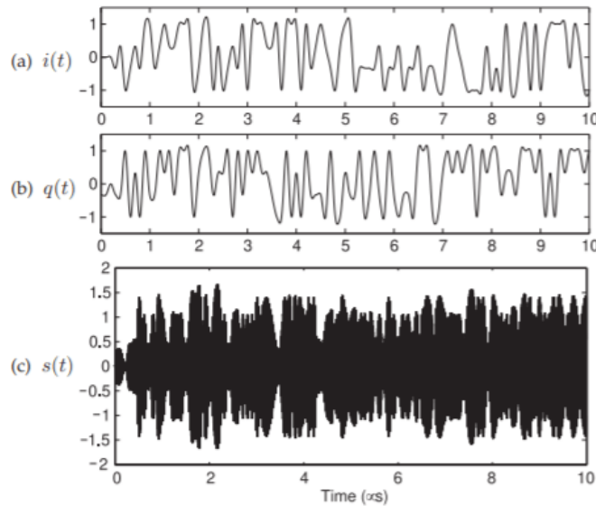
Figure 3.7.20: In-phase and quadrature-phase waveforms and RF waveforms in the RF quadrature modulator.
