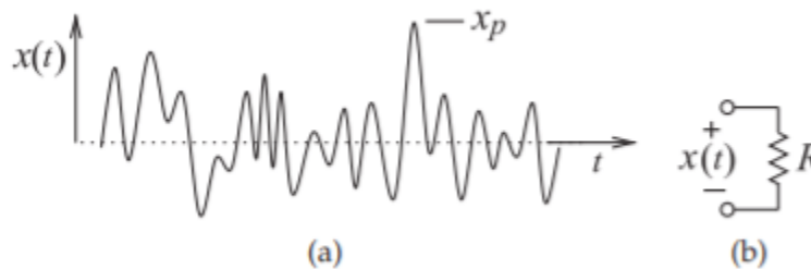
Figure 2.2.1: Definition of crest factor: (a) arbitrary waveform; and (b) voltage across a resistor.
