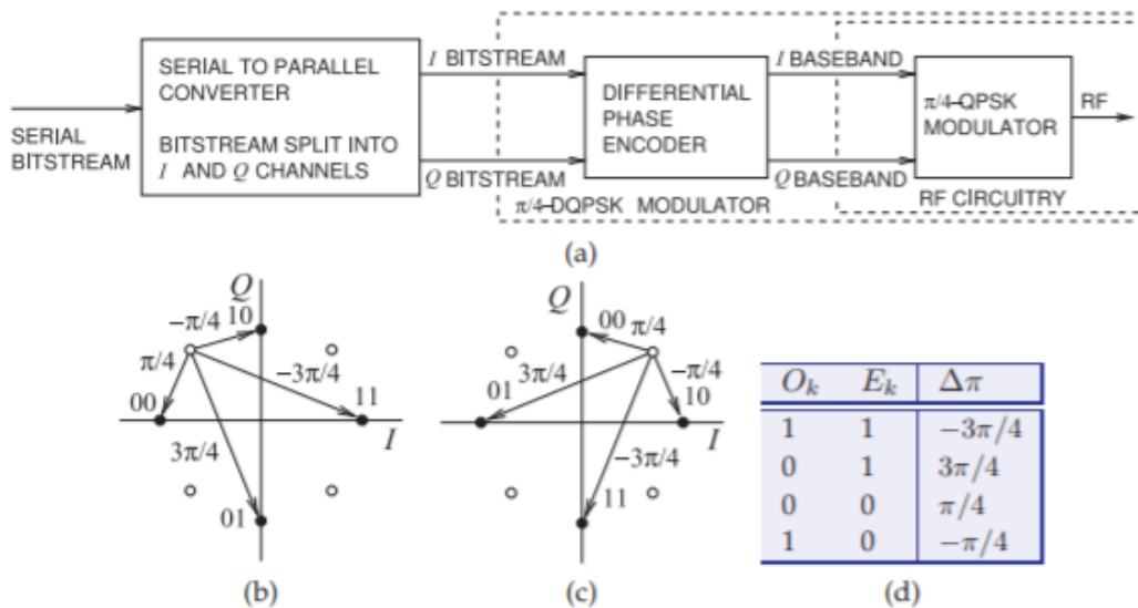
Figure 2.13.13: A \pi/4 -DQPSK modulator: (a) differential phase encoder with a \pi/4 -QPSK modulator; (b) constellation diagram of \pi/4 -DQPSK; (c) a second constellation diagram; and (d) phase changes in a \pi/4 -DQPSK modulation scheme. Note that the information is in the phase change rather than the phase state.
