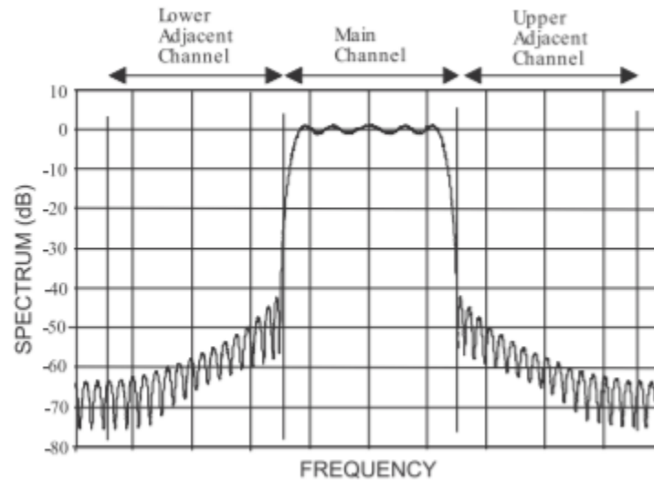
Figure 2.13.16: Detailed spectrum of a \pi/4 -DQPSK signal showing the main channel and lower and upper adjacent channels.
