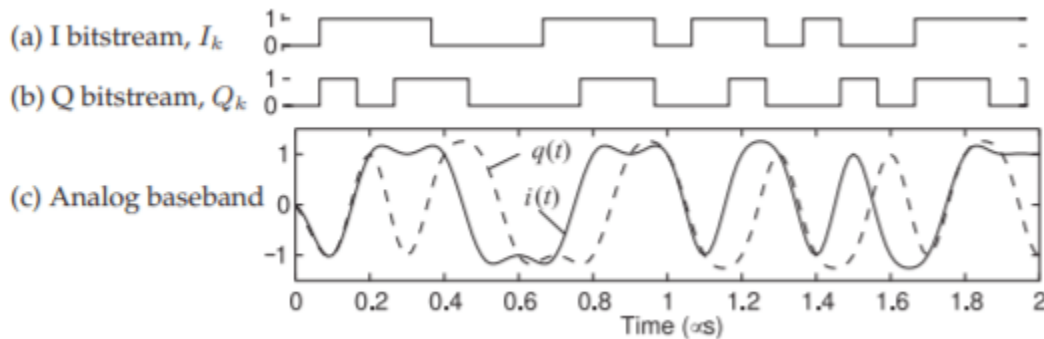
Figure 3.7.8: Baseband signals for a four state binary quadrature modulator. The I_k and Q_k bitstreams are derived from the random bitstream S_k = 00111011010010111100101100100100111110 and taken as (I_k, Q_k) pairs. The initial setting is i(0) = 0 = q(0) .
