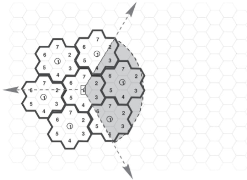
Figure 4.11.2: Cells in a cellular radio system with a trisector antenna, such as in Figure 4.11.3, showing the area of possible interference as a shaded region.
