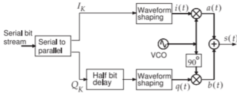
Figure 2.13.17: Block diagram of an OQPSK modulator.
