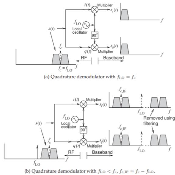
Figure 3.7.24: Quadrature demodulators used to down-convert an I/Q modulated RF signal.
