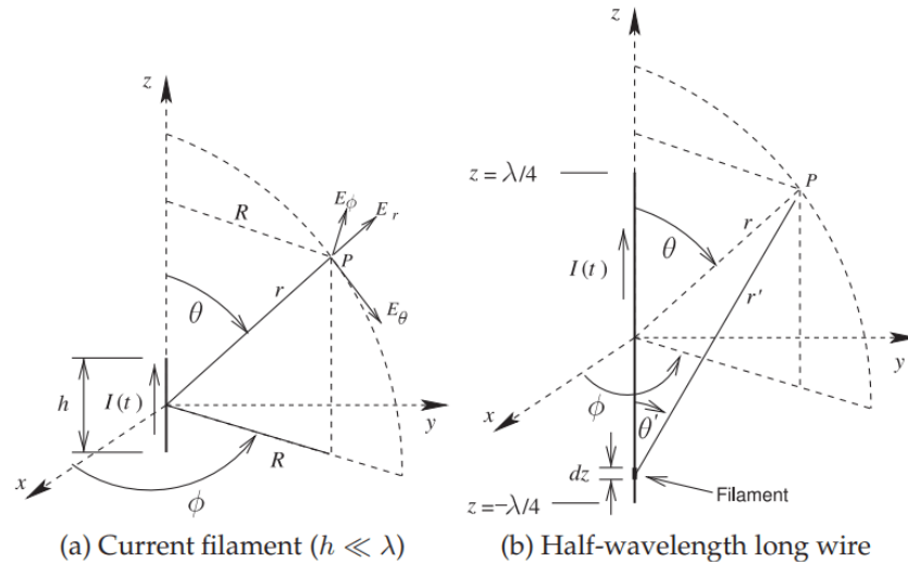
Figure 4.2.1: Wire antennas. The distance from the center of an antenna to the field point P is r . R = r \sin \theta .
