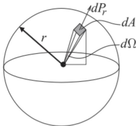
Figure 4.4.1: Free-space spreading loss. The incremental power, dP_r , intercepted by the shaded region of incremental area dA is proportional to 1/r^2 . The solid angle subtended by the shaded area is the incremental solid angle d\Omega . The integral of dA over the surface of the sphere, i.e. the area of the sphere is 4\pi r^2 . The total solid angle subtended by the sphere is the integral of d\Omega over the sphere and is 4\pi steradians (or 4\pi sr).
