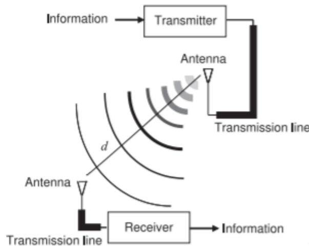
Figure 4.1.1: RF link.
