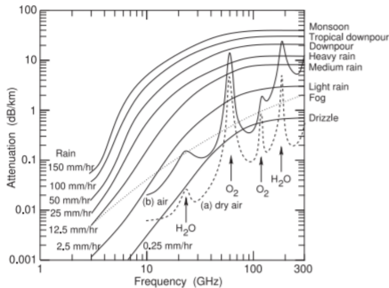
Figure 4.6.7: Excess attenuation due to atmospheric conditions showing the effect of rain on RF transmission at sea level. Curve (a) is atmospheric attenuation, due to excitation of molecular resonances, of very dry air at 0°C, curve (b) is for typical air (i.e. less dry) at 20°C. The attenuation shown for fog and rain is additional (in dB) to the atmospheric absorption shown as curve (b).
