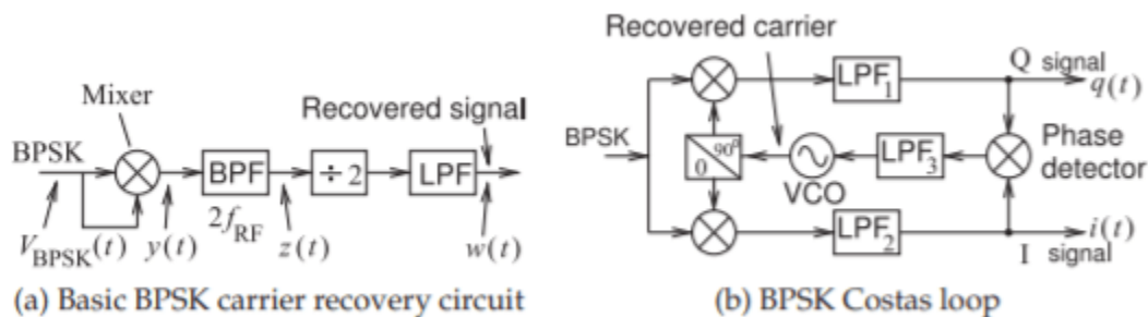
Figure 2.13.7: Block diagram of carrier recovery circuits for BPSK signals.
