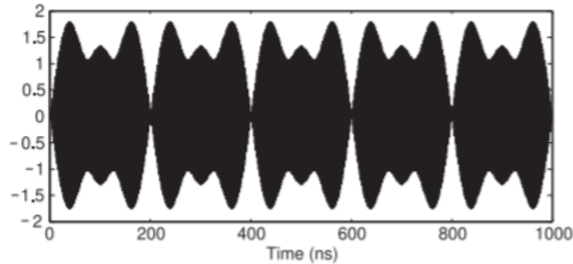
Figure 3.7.2: A 1 GHz carrier modulated by a 10 MHz sinusoidal i(t) and a 15 MHz sinusoidal q(t) .
