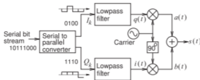
Figure 2.13.9: QPSK modulator block diagram. I_k and Q_k are similar to a stream of one-bit binary signals but are analog with a either a positive value or a negative voltage so that after lowpass filtering i(t) and q(t) each have either a positive or a negative voltage at each clock tick.
