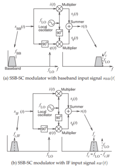
Figure 3.7.1: Quadrature modulator with the i(t) component derived directly from the input signal and q(t) derived from a 90^\circ negatively phase-shifted input signal. The IF signal in (b) is typically a DSB-SC signal with intermediate carrier frequency f_{c, IF} set in DSP.
