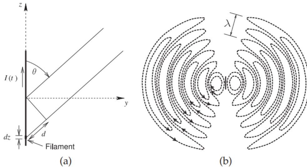
Figure 4.3.1: Wire antenna: (a) geometry for calculating contributions from current filaments of length dz with coordinate z ( d = -z \sin \theta ); and (b) instantaneous electric field in the y-z plane due to a \lambda/2 long current element. There is also a magnetic field.
