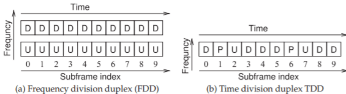
Figure 5.7.3: Duplex schemes used in 4G with ten subframes in a 10 ms frame.
