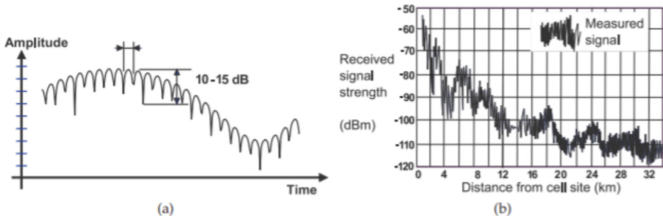
Figure 4.6.5: Fast and slow fading: (a) in time as a radio and obstructions move; and (b) in distance.
