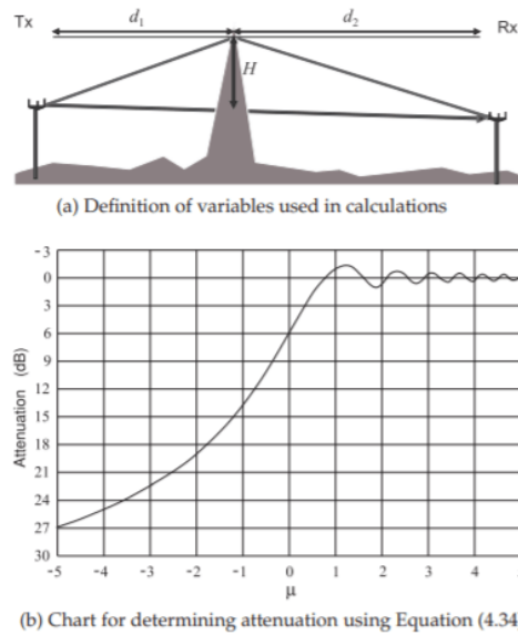
Figure 4.6.3: Knife-edge diffraction.
