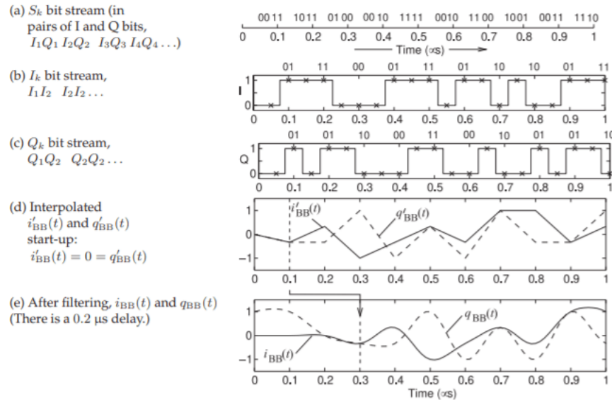
Figure 3.7.17: Baseband signals for 16-QAM modulation with markers showing the baseband bit impulse times. The bit pairs shown above each bit waveform 0.1 \mu s intervals.
