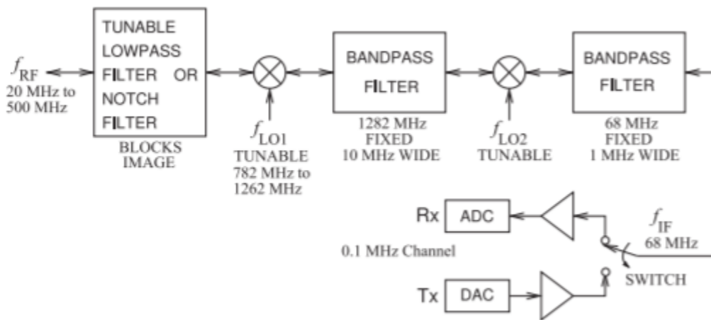
Figure 3.14.8: Bilateral double-conversion transceiver for wideband operation of an emergency or military radio.
