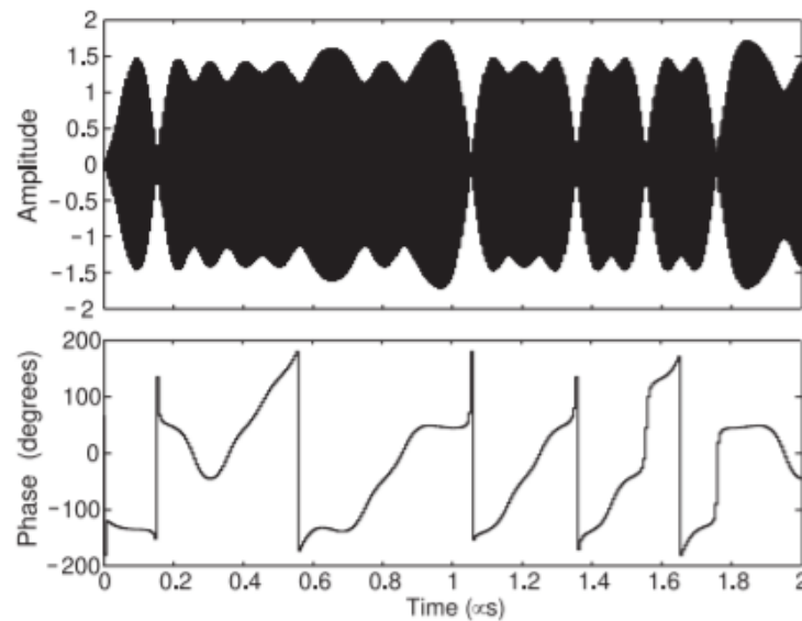
Figure 3.7.10: Amplitude and phase of the modulated carrier signal s(t) as the output of a binary modulator with a 20 Mbit/s digital baseband signal. Note that the rapid phase transitions occur when the amplitude of the modulated carrier goes to zero. (The rapid switch between 180^\circ and -180^\circ when the amplitude is not zero is a continuous smooth phase change.)
