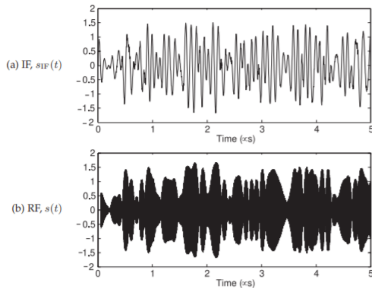
Figure 3.7.23: Comparison of the IF and RF modulated signals.
