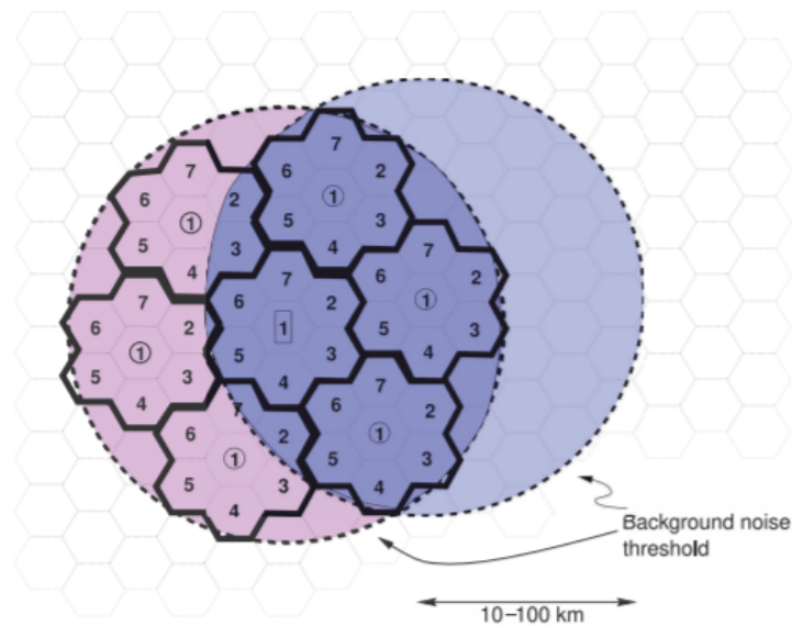
Figure 5.3.3: Interference in a cellular radio system.
