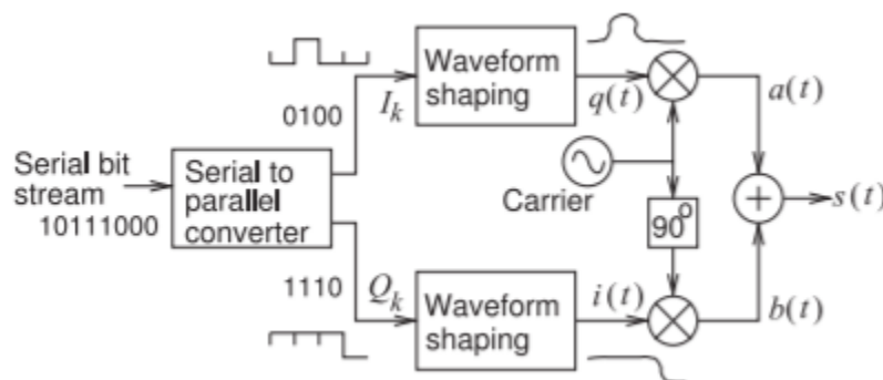
Figure 2.14.1: QAM modulator block diagram. In QAM modulation i(t) and q(t) address the real and imaginary components of a phasor. The wave-shaping block ensures that the symbol has the correct amplitude and phase at each clock tick.
