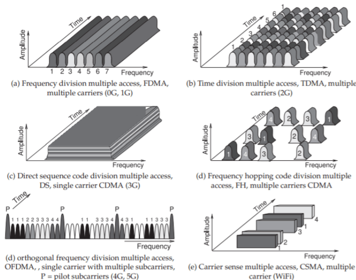
Figure 5.4.1: Multiple access schemes for supporting multiple users with each user indicated by a numeral except for (b), TDMA, where the numerals indicate time slots.
