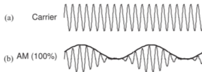
Figure 2.1.1: AM showing the relationship between the carrier and modulation envelope: (a) carrier; and (b) 100% amplitude modulated carrier.
