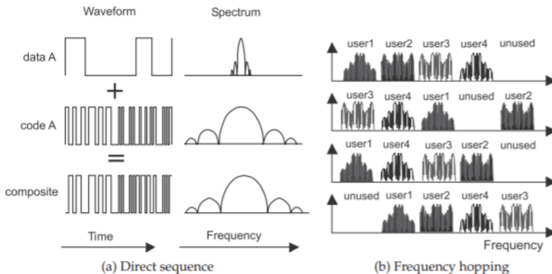
Figure 5.4.3: Basis of multiuser spread-spectrum communication.
