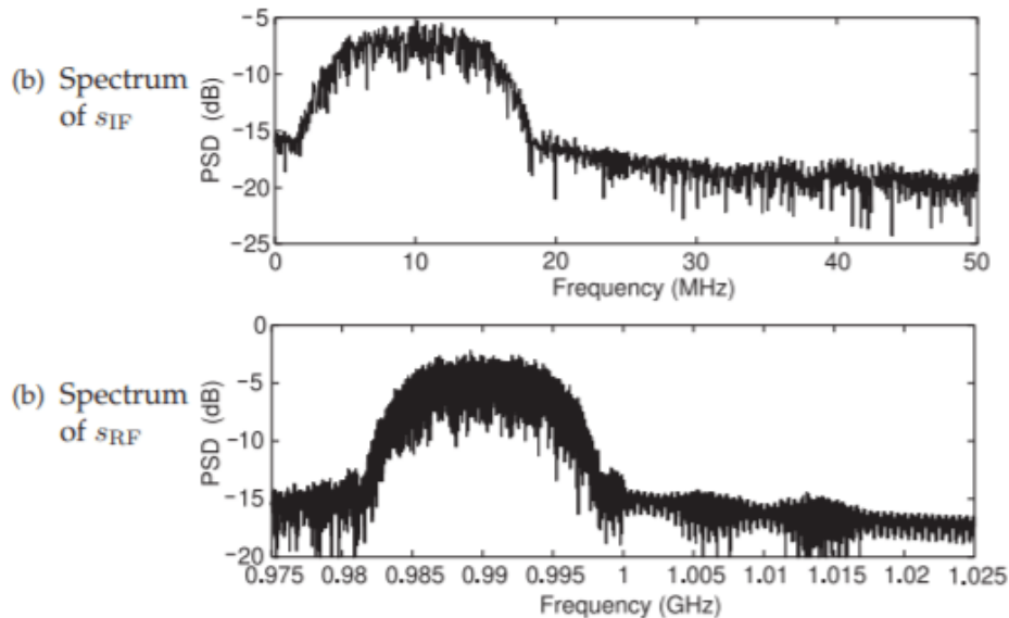
Figure 3.7.21: Spectrum of the IF and RF modulated carriers.
