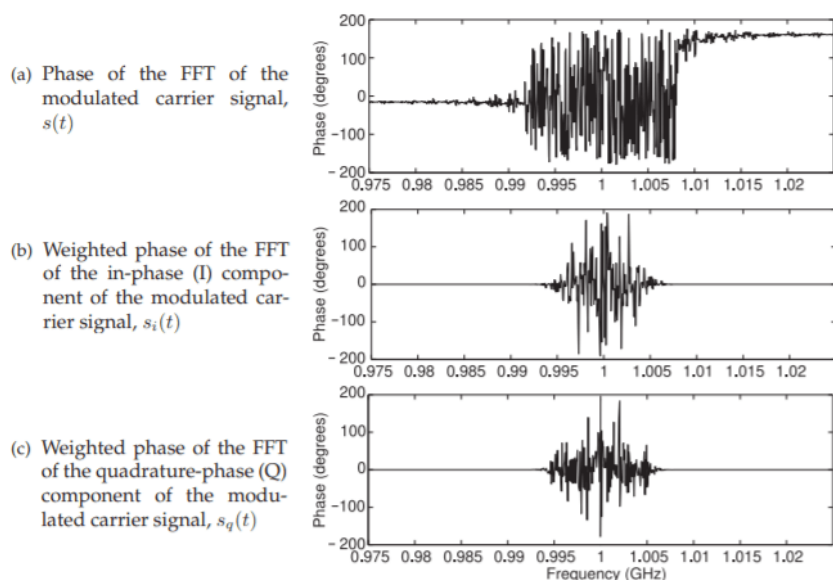
Figure 3.7.13: Phase of the FFT of the digitally modulated RF signal and its components. The phase of the s_i(t) and s_q(t) has
