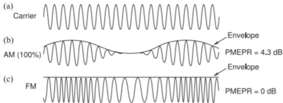
Figure 2.5.1: Comparison of 100% AM and FM highlighting the envelopes of both: (a) carrier; (b) AM signal; and (c) FM signal with constant envelope.
