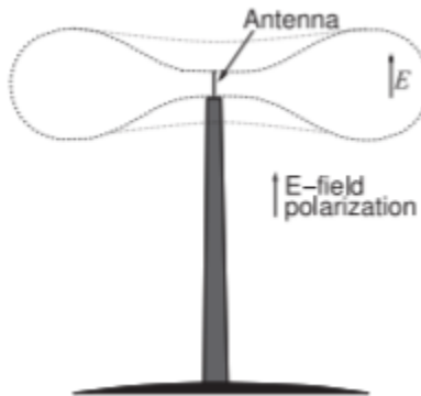
Figure 4.5.2: A base station transmitter pattern.
