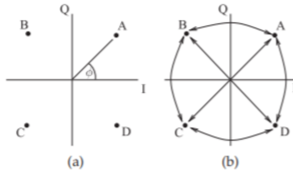
Figure 2.13.8: QPSK modulation: (a) constellation diagram; and (b) constellation diagram with possible transitions. Each constellation point indicates the phase, \phi , of the modulated carrier, i.e. \cos(\omega_c t + \phi) where \omega_c is the radian frequency of the carrier.
