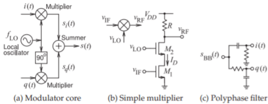
Figure 3.16.1: Quadrature modulator. The simple modulator in (b) is based on a FET cascode amplifier and the polyphase filter in (c) has a 90^\circ phase difference between i(t) and q(t) .
