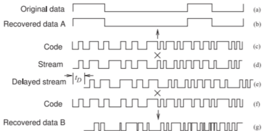
Figure 5.16.2: Decoding of a direct sequence coded stream showing a code aligned with the data stream and a data stream delayed by t_D .
