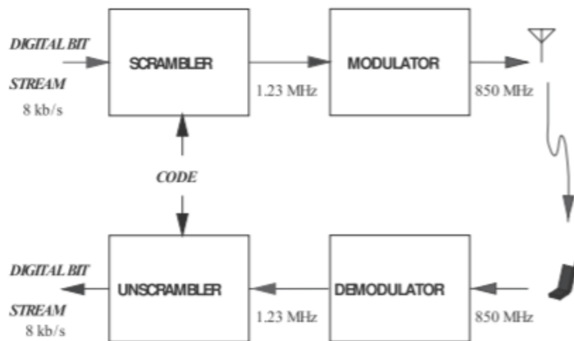
Figure 5.4.2: Block schematic of the operation of a CDMAOne spread spectrum radio.
