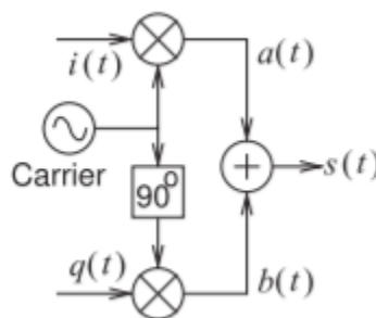
Figure 2.13.4: Quadrature modulator block diagram. In PSK modulation i(t) and q(t) have the same amplitude and indicate a phase \phi of the modulated carrier so that i(t) = \cos[\phi(t)] and q(t) = \sin[\phi(t)] . The particular example shows two possible values of I_k and Q_k and this indicates QPSK modulation.
