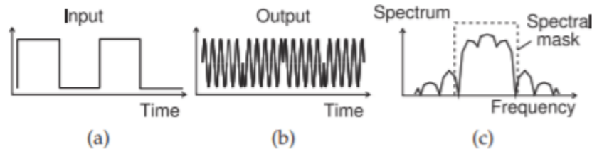
Figure 2.13.1: Binary PSK modulation: (a) modulating bitstream; (b) the modulated waveform; and (c) its spectrum after smoothing the transitions from one phase state to another.
