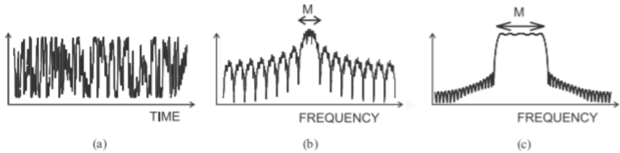
Figure 2.13.15: Details of digital modulation obtained using differential phase shift keying ( \pi/4 - DQPSK): (a) modulating waveform; (b) spectrum of the modulated carrier, with M denoting the main channel; and (c) details of the spectrum of the modulated carrier focusing on the main channel.
