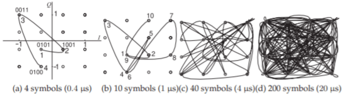
Figure 3.7.22: Constellation diagram with trajectories of the phasor of f_c for various symbol lengths with the first symbol at 0.3 \mu\text{s} . Each symbol has 4 bits. In (a) and (b) the first symbol is labeled '1', etc.
