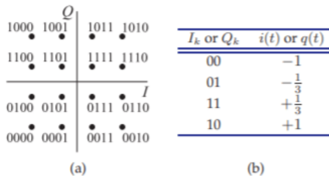
Figure 3.7.16: 16-QAM modulation: (a) constellation diagram; and (b) table translating binary value of I (or Q ) to an absolute value i(t) (or q(t) ).
