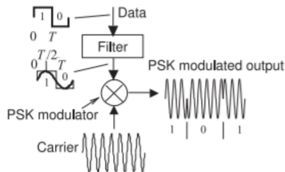
Figure 2.13.2: A binary phase shift keying (PSK) modulation system.
