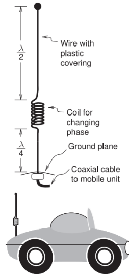
Figure 4.3.3: Mobile antenna with phasing coil extending the effective length of the antenna.
