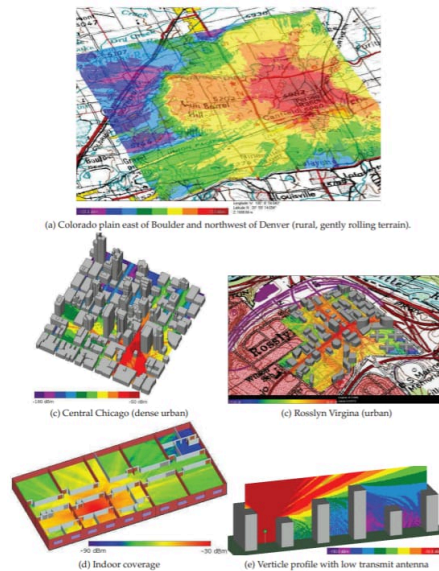
Figure 4.12.1: Radio coverage profiles with 900 MHz transmitter except for (d) which is for 2.45 GHz. Calculated using Wireless Insite®. Copyright Remcom, Inc. Used with permission.
