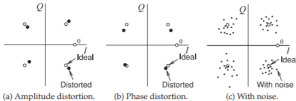
Figure 2.8.3: Impact of signal impairments on the constellation diagram of QPSK.
