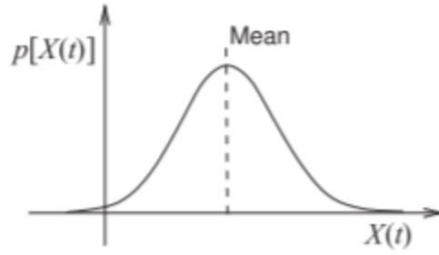
Figure 5.A.1: Gaussian distribution.
