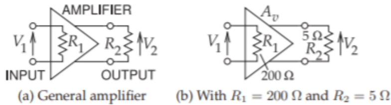
Figure 1.6.3: Amplifiers each with an input resistance R_1 and output resistance R_2 .
