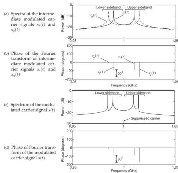
Figure 3.7.3: Spectrum of signals in the quadrature modulator of Figure 3.7.1(a) with 10 MHz in phase, i(t) , and 15 MHz quadrature-phase, q(t) , modulating signals. (Simulated time = 65.536 \mu s, using a 223 point FFT.)
