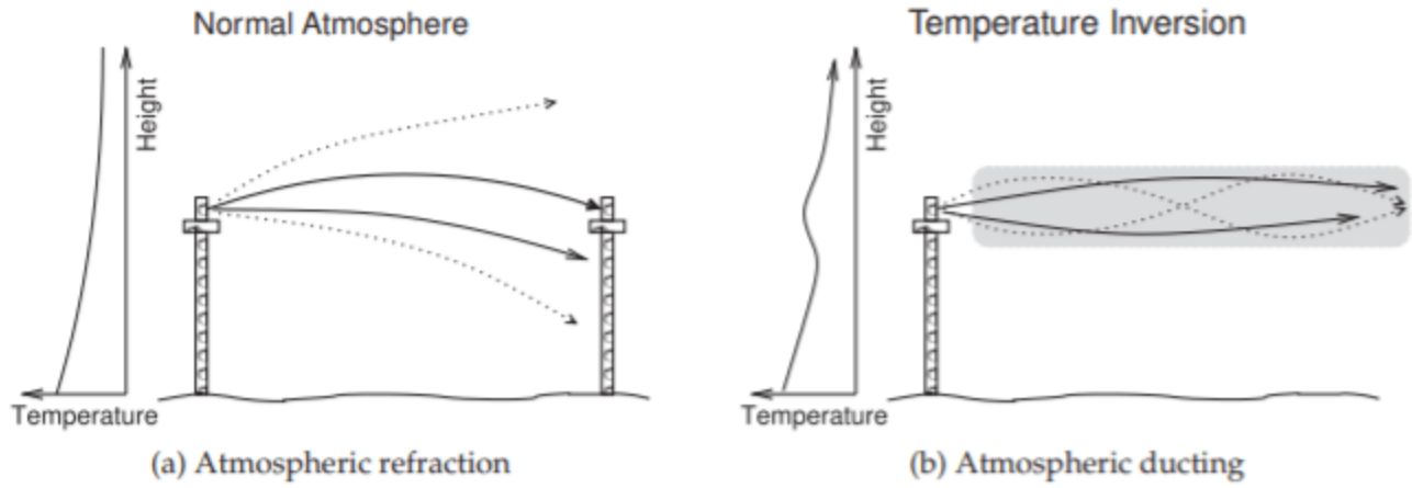
Figure 4.6.8: Fading resulting from ducting: (a) normal atmospheric refraction (normally the temperature of air drops with increasing height and the lower refractive index at high heights results in a concave refraction); and (b) atmospheric ducting (resulting from temperature inversion inducing an air layer with higher dielectric constant than the surrounding air).
