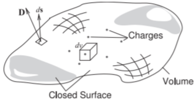
Figure 1.3.4: Diagram illustrating Gauss's law. Charges are distributed in the volume enclosed by the closed surface. An incremental area is described by the vector dS , which is normal to the surface and whose magnitude is the area of the incremental area.
