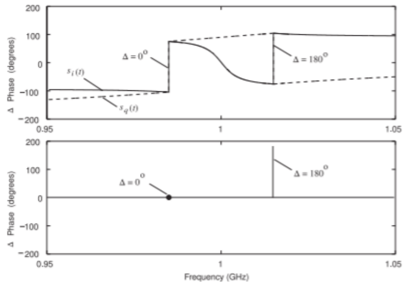
Figure 3.7.6: Phase of the modulated signal. (Simulated time = 65.536 \mu s, 223 point FFT.)
