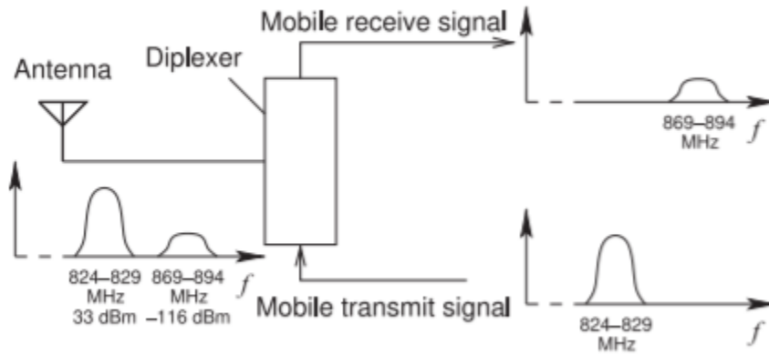
Figure 5.2.3: A diplexer which separates receive and transmit signals. A diplexer is a type of duplexer. However not all duplexers are diplexers.
