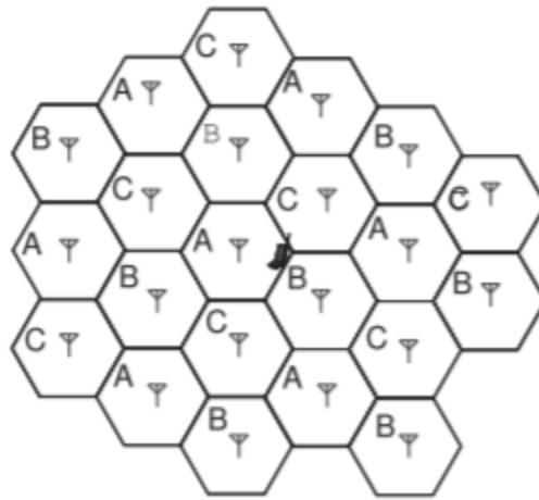
Figure 4.11.4: Three-cell cluster with mobile unit at the edge of cells A, B, and C.
