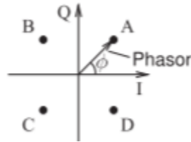
Figure 2.13.3: Phasor diagram of QPSK modulation. Here there are four discrete phase states of the phasor indicated by the points A, B, C, and D. The PSK modulator moves the phasor from one phase state to another. The task at the receiver is determining the phase of the phasor.
