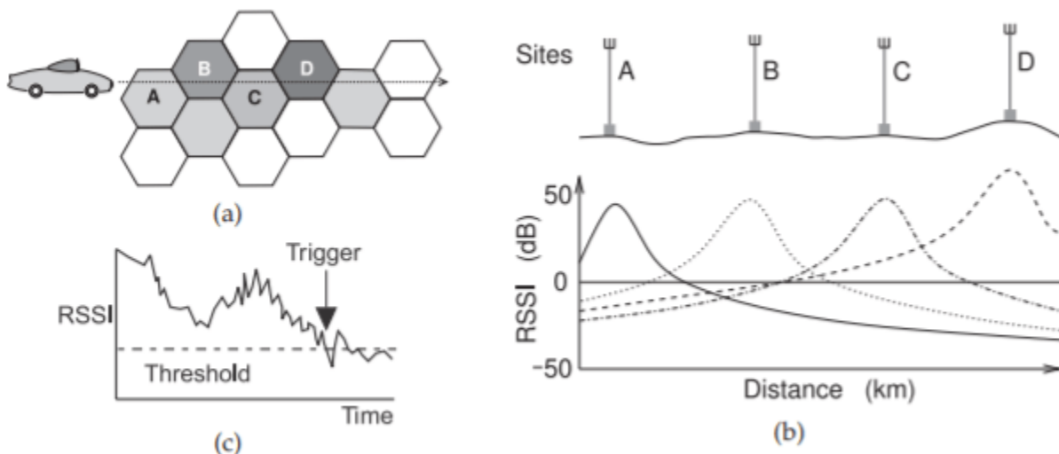
Figure 5.3.4: Process of handoff: (a) movement of a mobile unit through cells; (b) received signal strength indicator (RSSI) during movement of a mobile unit through cells; and (c) RSSI of a mobile unit showing the handoff triggering event.
