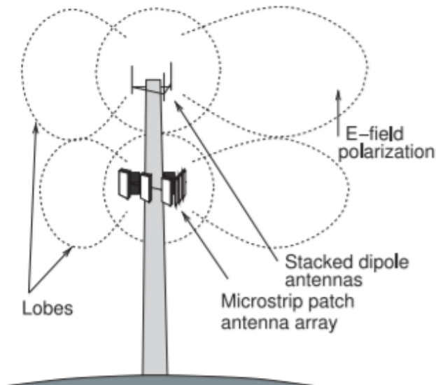
Figure 4.11.3: Base station with trisector stacked-dipole transmit and microstrip patch receive antennas.
