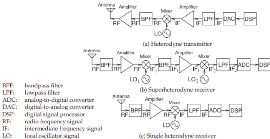
Figure 3.4.1: RF front ends: (a) a one-stage transmitter; (b) a receiver with two mixing (or heterodyning) stages; and (c) a receiver with one heterodyne stage.
