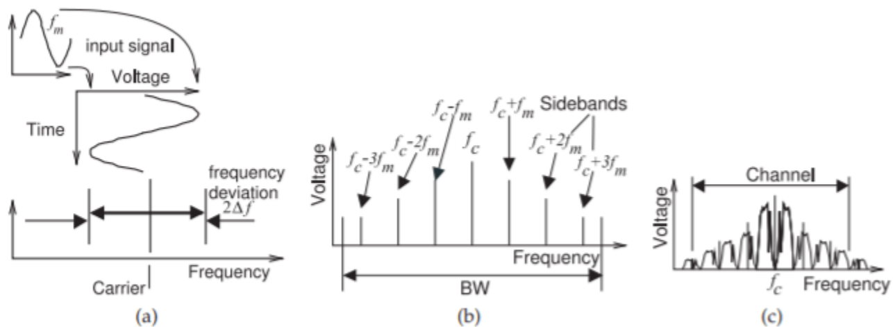
Figure 2.4.5: Frequency modulation: (a) sinusoidal baseband signal shown varying the frequency of the carrier and so FM modulating the carrier; (b) the spectrum of the resulting FM-modulated waveform; and (c) spectrum of the modulated carrier when it is modulated by a broadband baseband signal such as voice.
