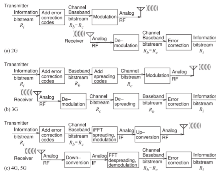
Figure 5.6.1: Flow of information in digital cellular radio with R_i , R_b , and R_c being the information, baseband, and channel bit rates, respectively.
