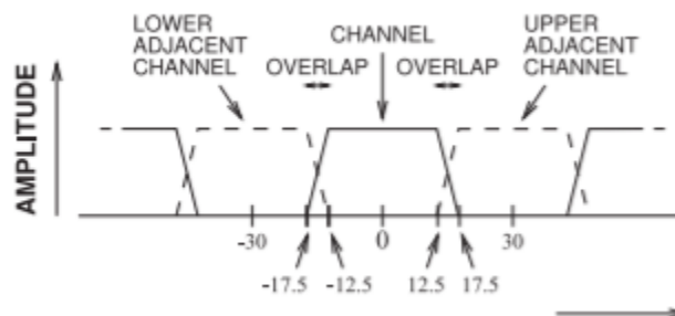
Figure 2.8.1: Adjacent channels showing overlap in the AMPS and DAMPS cellular systems.
