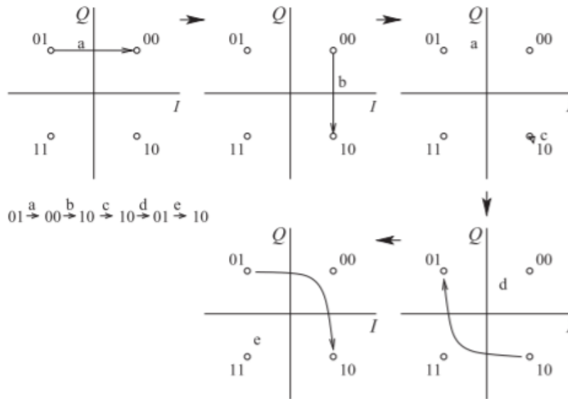
Figure 2.13.19: Constellation diagram of OQPSK modulation for the bit sequence 010010100110.
