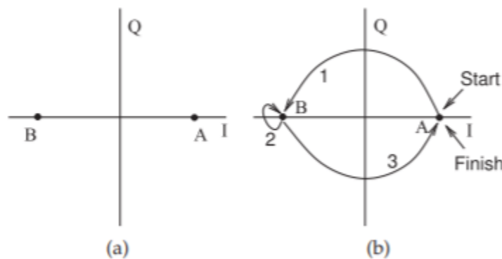
Figure 2.13.5: BPSK modulation with constellation points A and B: (a) constellation diagram; and (b) constellation diagram with possible transitions from one phase state to the other, or possibly no change in the phase state. In practical systems the transition should not go through the origin, as then the RF signal would drop below the noise level.
