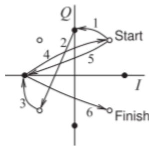
Figure 2.13.14: Constellation diagram of \pi/4 -DQPSK modulation showing six symbol intervals coding the bit sequence 000110110101.
