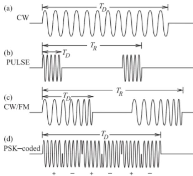
Figure 5.10.2: Radar waveforms: (a) continuous wave; (b) pulsed wave; (c) frequency modulated continuous wave; and (d) phase-encoded (PSK-coded) waveform.
