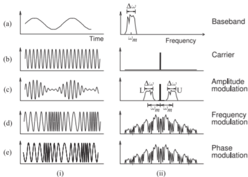
Figure 2.4.1: Basic analog modulation showing the (i) waveform and (ii) spectrum for (a) baseband signal; (b) carrier; (c) carrier modulated using amplitude modulation; (d) carrier modulated using frequency modulation; and (e) carrier modulated using phase modulation.
