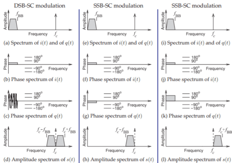
Figure 3.16.3: Spectra of the baseband i(t) and q(t) signals and the modulated s(t) signal, see Figure 3.16.1(a), for double sideband (DSB) and single sideband (SSB) suppressed-carrier (SC) modulation. Here the carrier frequency f_c = f_{LO} , the LO frequency in Figure 3.16.1(a).
