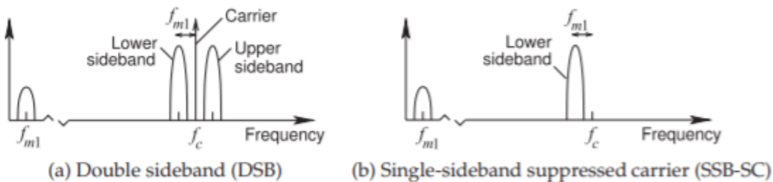
Figure 3.2.1: Spectrum of a modulated carrier with a modulating signal of finite bandwidth f_m with f_{m1} being the center frequency of the baseband signal.
