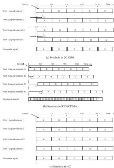
Figure 4.10.1: The effect of excess delay on symbol interference when there are four paths. The excess delay of each path, \tau_{d,x} , increases by 100 ns. Five symbols are shown: A, B, C, D, and E. The 2G GSM standard has a symbol duration of 3.6928 \mu s, the 3G WCDMA standard has a symbol duration of 260 ns, and the 4G OFDM standard has a symbol duration of 71.35 \mu s. The situation with 5G is similar to that for 4G.
