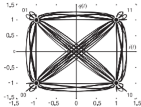
Figure 3.7.9: Constellation diagram for the binary quadrature modulator. This is also the phasor diagram (with appropriate scaling) of the modulated carrier signal with constellation points sampled at 0.1 \mu\text{s} intervals shown as large dots. There are four constellation points corresponding to four symbols and each symbol represents two bits of information.
