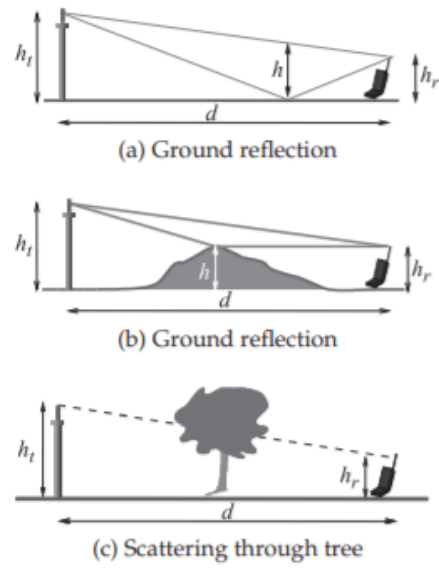
Figure 4.6.2: Common paths contributing to multipath propagation.
