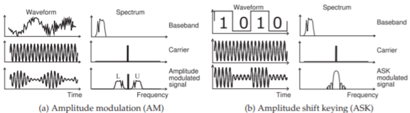
Figure 1.3.5: Waveform and spectra of simple modulation schemes. The modulating signal, at the top in (a) and (b), is also called the baseband signal.
