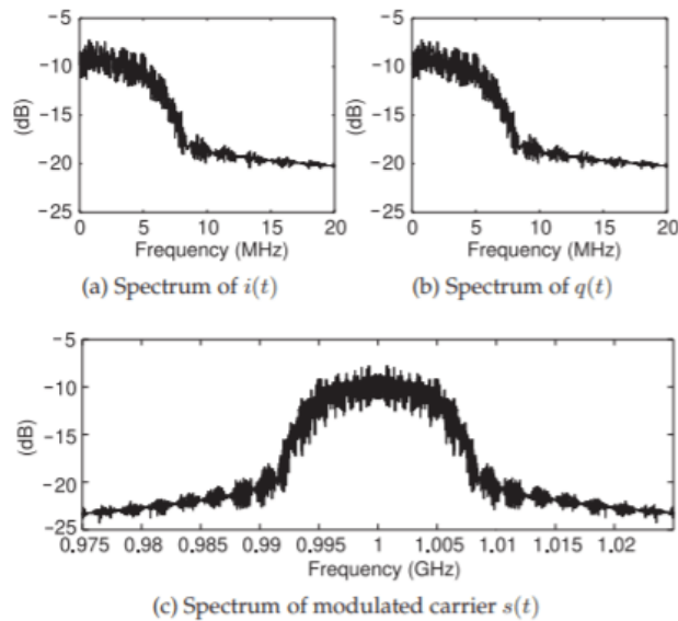
Figure 3.7.11: Spectra of signals in the digital modulator with a 20 Mbit/s input stream, S_k , and a 1 GHz LO. (1024 symbols, a time duration of 102.4 \mu s, and using a 524,288 point FFT)
