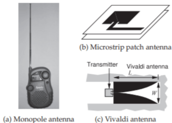
Figure 4.1.2: Representative resonant, (a) and (b), and traveling-wave, (c), antennas.
