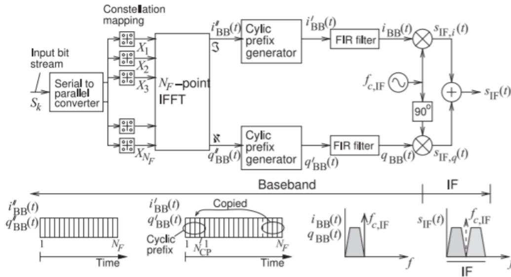
Figure 5.7.5: Block diagram of an OFDM modulator.
