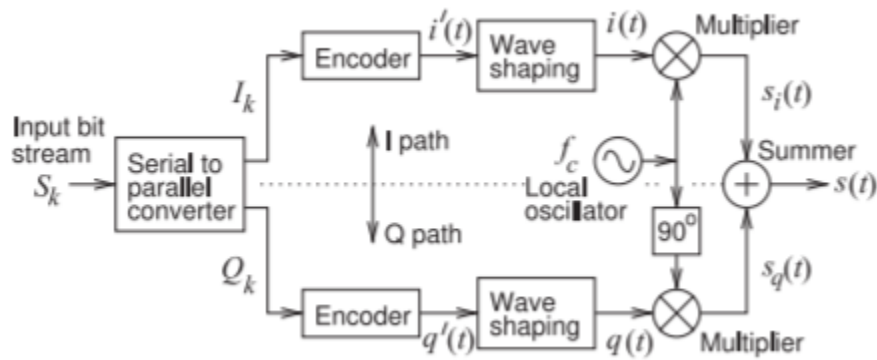
Figure 3.7.14: High-order digital quadrature modulator with independent I and Q paths yielding double sideband, suppressed carrier (DSB-SC) modulation.
