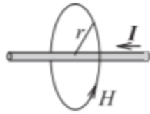
Figure 1.3.3: Diagram illustrating Ampere's law. Ampere's law relates the current, I , on a wire to the magnetic field around it, H .
