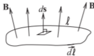
Figure 1.3.2: Diagram illustrating Faraday's law. The contour \ell encloses the surface.
