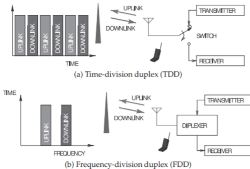
Figure 5.2.2: Duplex schemes.
