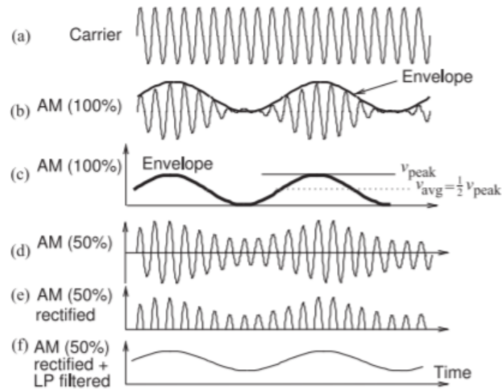
Figure 2.4.2: AM showing the relationship between the carrier and modulation envelope: (a) carrier; (b) 100% amplitude modulated carrier; (c) modulating or baseband signal; (d) 50% amplitude-modulated carrier; (e) rectified 50% AM modulated signal; and (f) rectified and lowpass (LP) filtered 50% modulated signal. The envelope contains only amplitude information and for AM the envelope is the same as the baseband signal.
