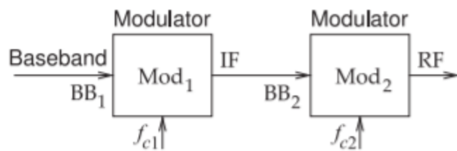
Figure 3.2.2: Two-stage modulator with the baseband signal, BB_1 , input to the first modulator, Mod_1 , producing the intermediate frequency signal IF_1 . This becomes the baseband signal, BB_2 , for the second modulator, Mod_2 , producing the radio frequency signal, RF .
