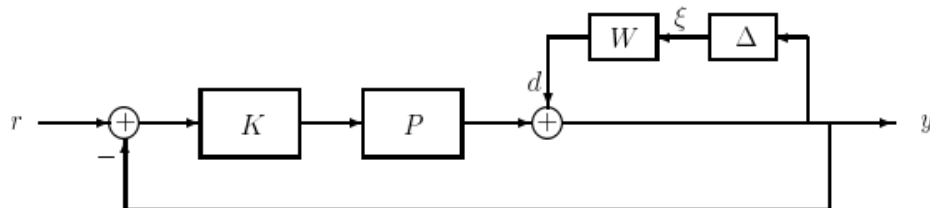
Figure 20.6: Plant with disturbance.
