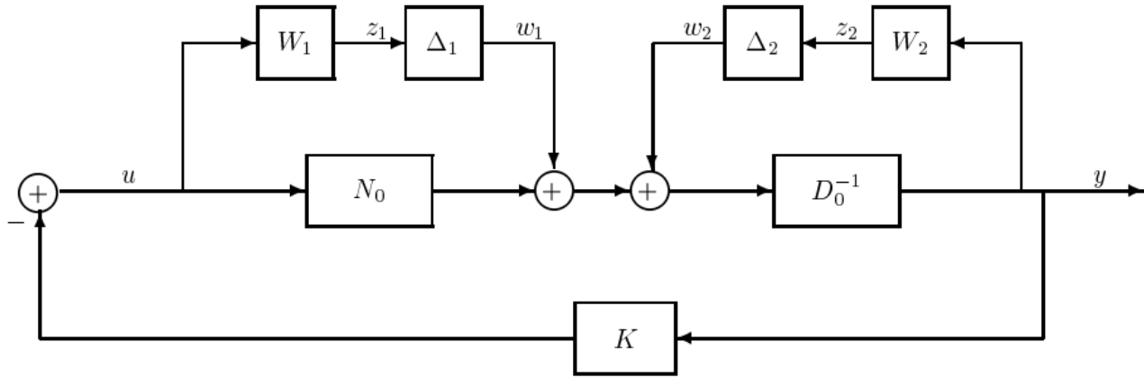
Figure 21.7: Coprime Factor Perturbation Model
