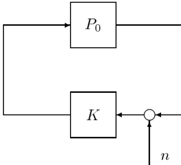
Figure 20.9: Quantization Modeled as Bounded Noise
