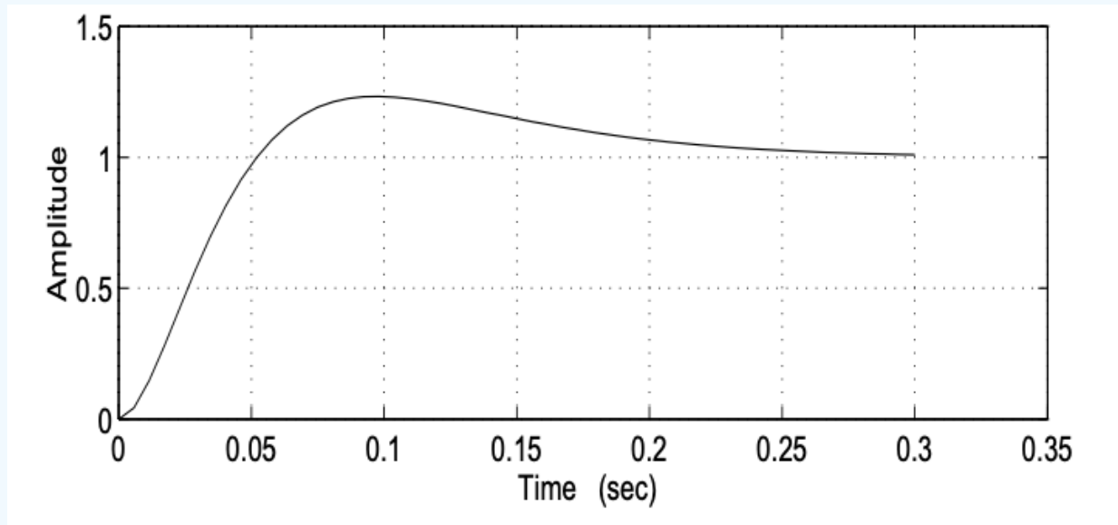
Figure 19.11: Step Response
