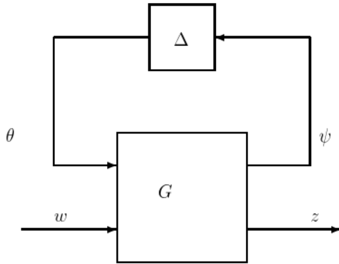
Figure 20.3: Standard model for uncertainty.
