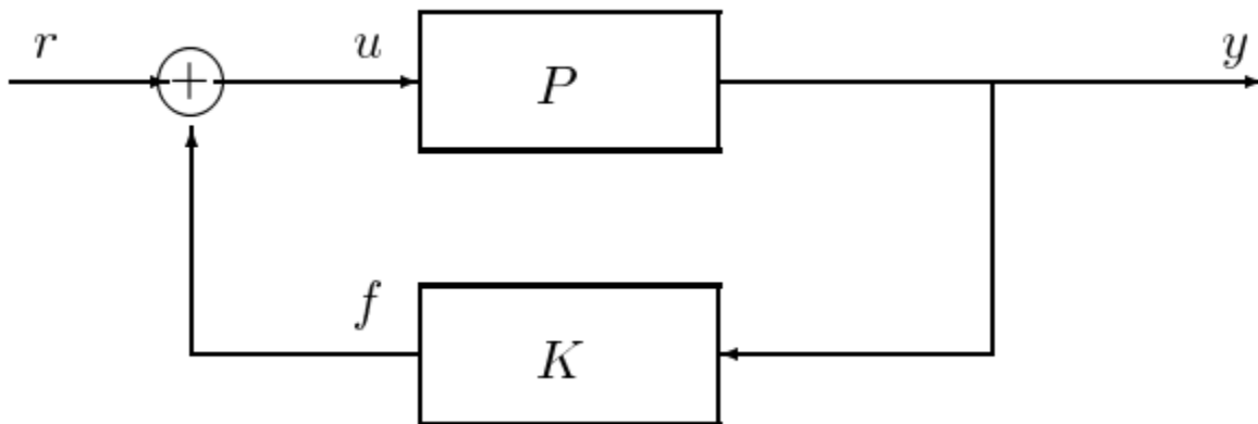
Figure PageIndex1: Block diagram of the prototype feedback control configuration.
