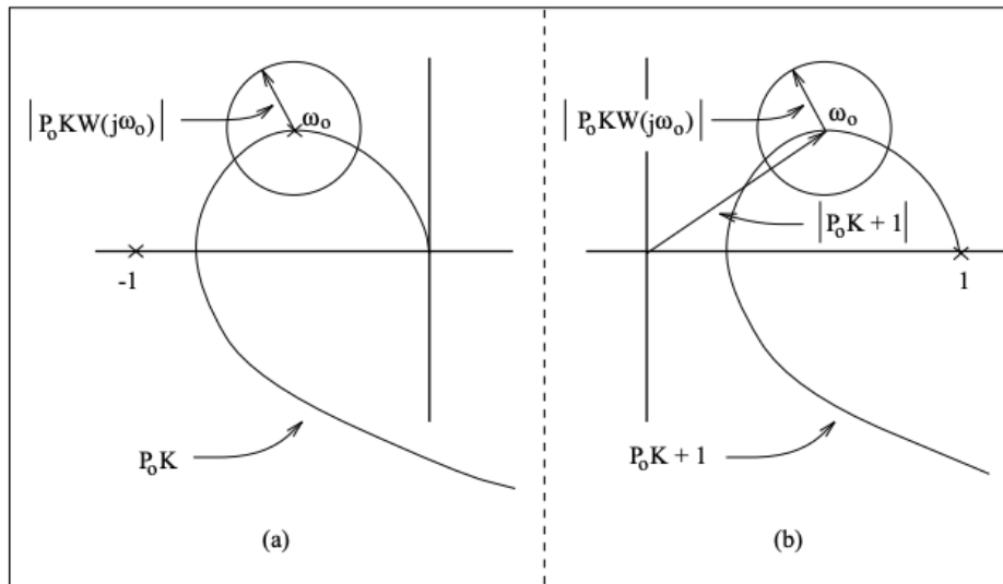
Figure 20.5: Relation of Nyquist criterion and robust stability.
