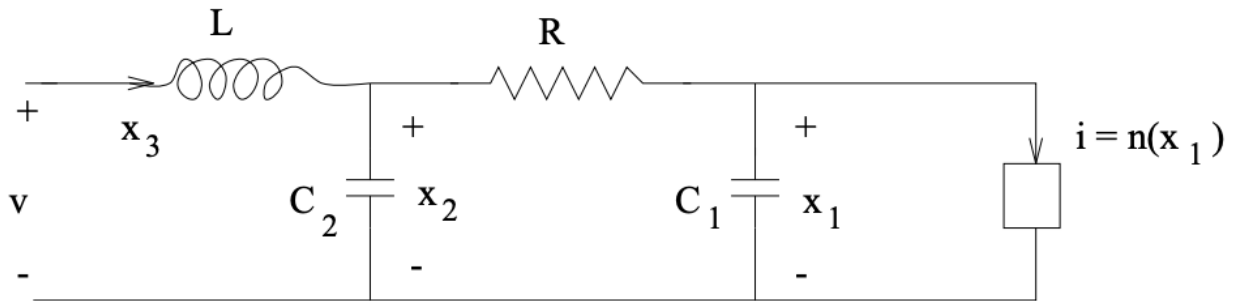
Figure 7.2.1: Nonlinear Circuit
