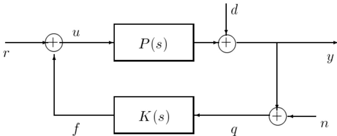
Figure PageIndex4: Including plant disturbances d and measurement noise n .
