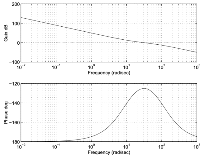
Figure 19.9: Open-loop Bode Plot
