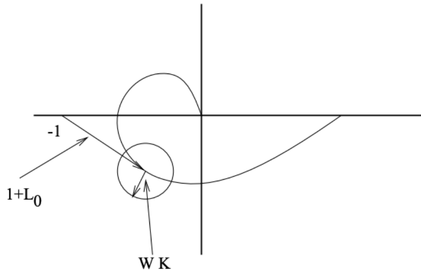
Figure 19.6: Nyquist Plot Illustration Robust Stability
