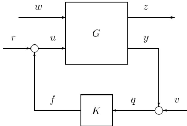
Figure 17.4.4: A more general feedback configuration
