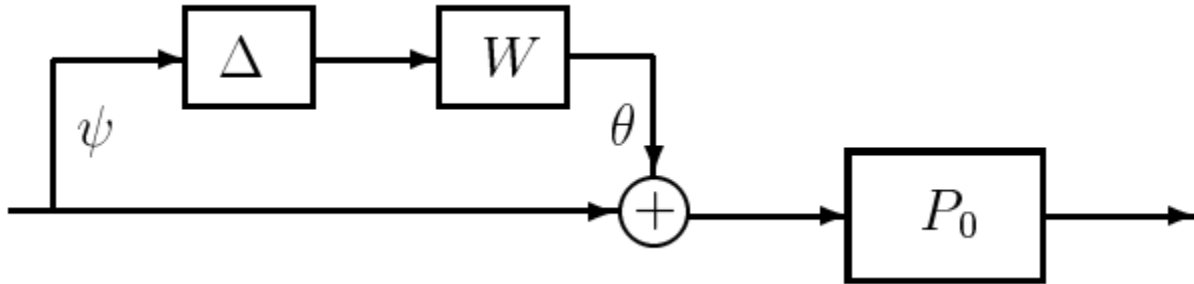
Figure 20.2: Representation of uncertainty as multiplicative perturbation at the plant input.
