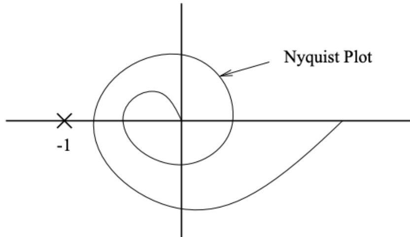
Figure 19.5: Nyquist Plot
