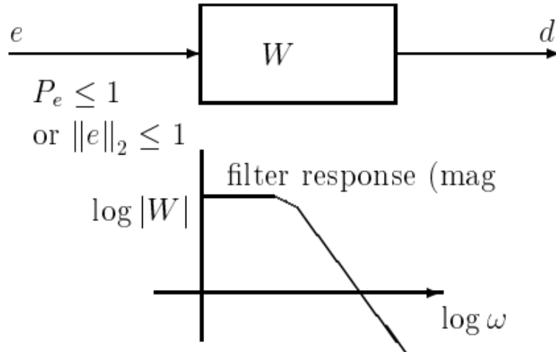
Figure 18.1.2: Representing the plant disturbance d as the output of a shaping filter W whose input e is an arbitrary bounded energy or bounded power signal, or possibly white noise.
