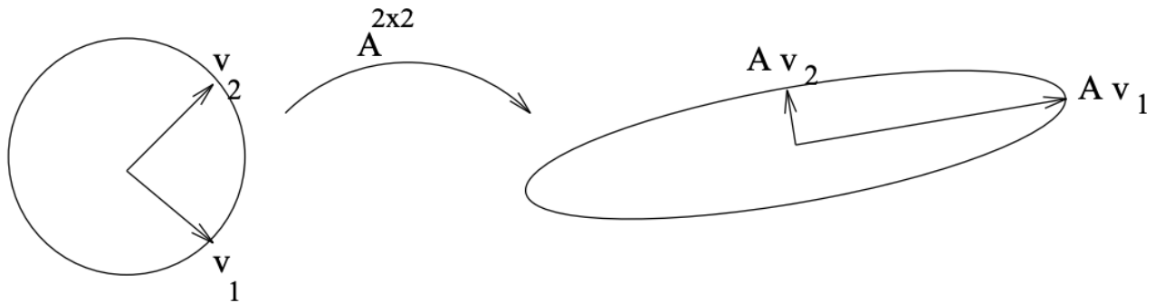
Figure 4.4.1: Graphical depiction of the mapping involving A^{2 \times 2} . Note that Av_1 = \sigma_1 u_1 and that Av_2 = \sigma_2 u_2 .
