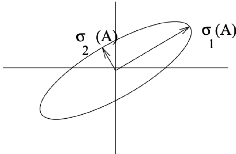
Figure 5.5.1: Depiction of how A (a real 2 \times 2 matrix) maps the unit circle. The major axis of the ellipse corresponds to the largest singular value, the minor axis to the smallest.
