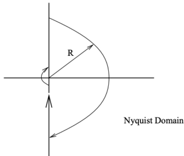
Figure 19.4 : Nyquist Domain.
