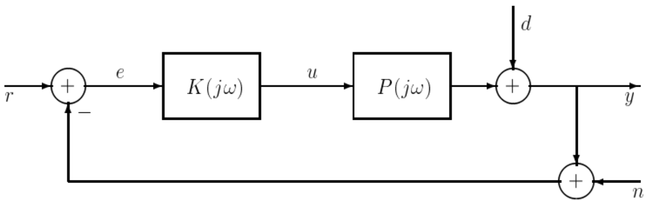
Figure 18.1.1: Standard feedback configuration with noise, disturbance, and reference inputs.
