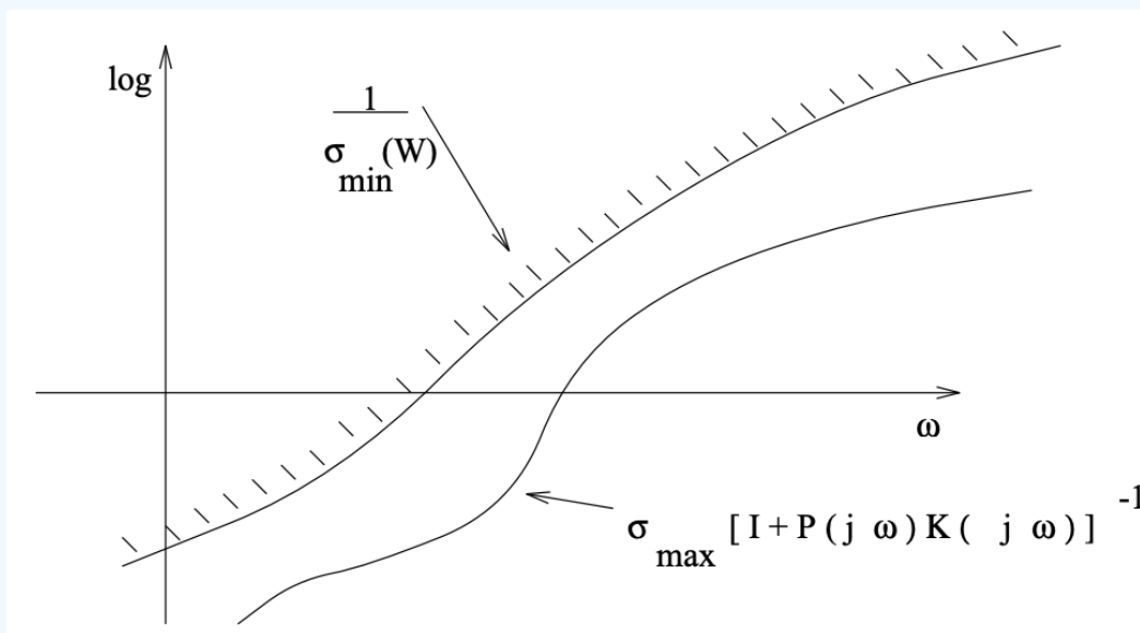
Figure 18.2.1: Singular value plot for a MIMO system
