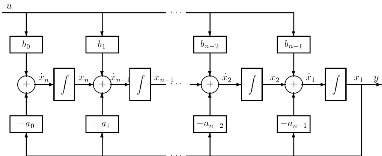
Figure 8.3.1: Observability Canonical Form
