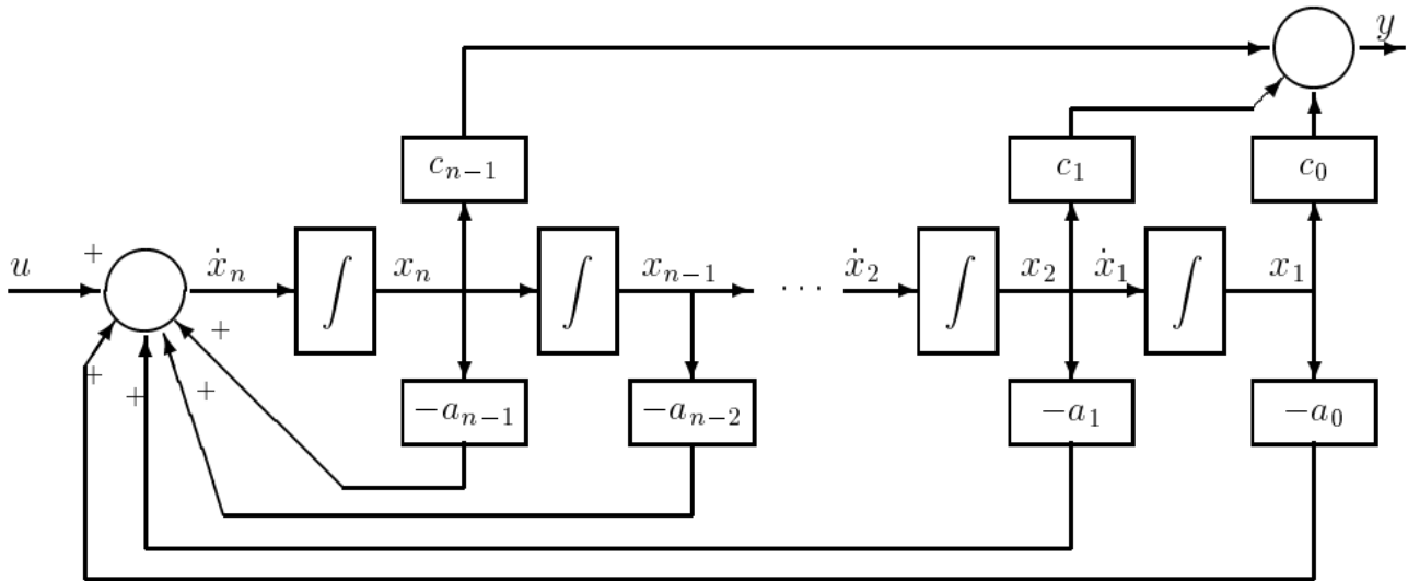
Figure 8.3.2: Reachability Canonical Form
