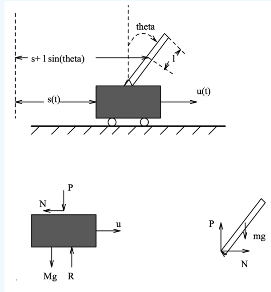
Figure 6.1.2: Inverted Pendulum
