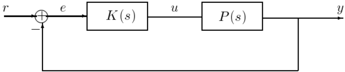
Figure PageIndex2: A ("servo") feedback configuration where the tracking error between the command r and output y is directly applied to the controller.
