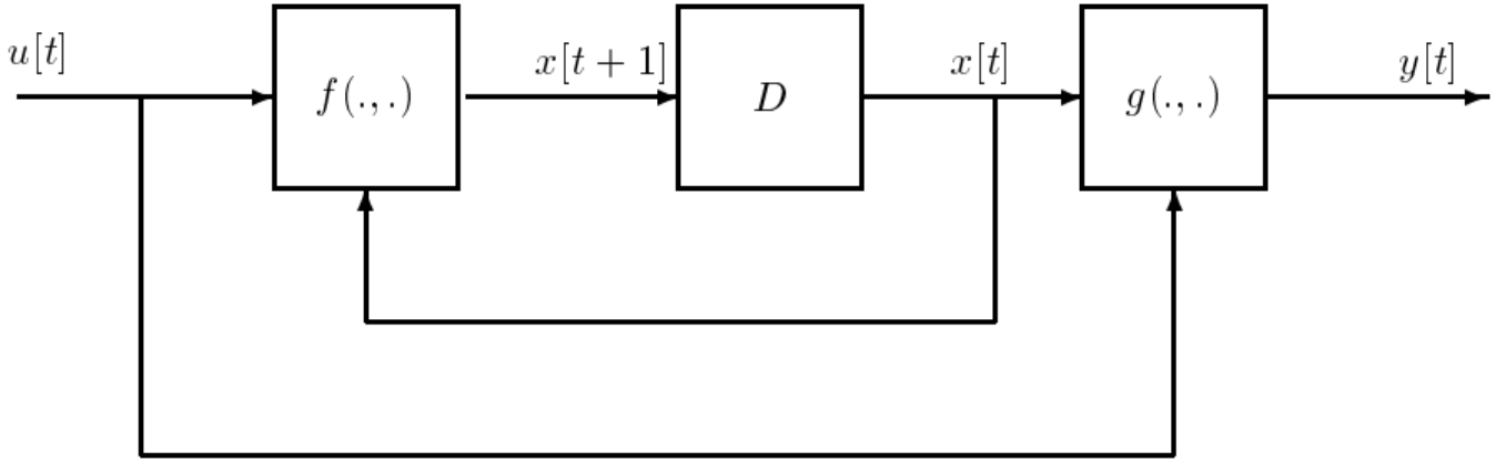
Figure 8.2.1: Simulation Diagram
