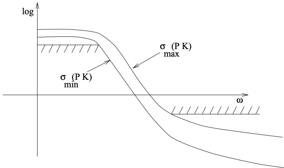
Figure 18.2.2: Singular value bounds for the open loop gain, P(j\omega)K(j\omega) .
