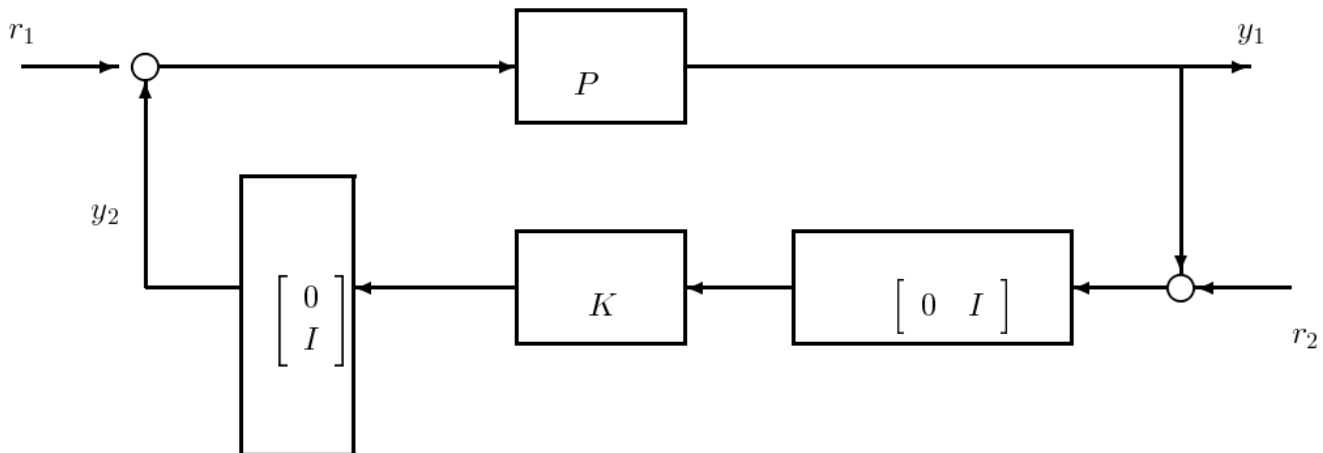
Figure 17.5.1: A more general feedback configuration.
