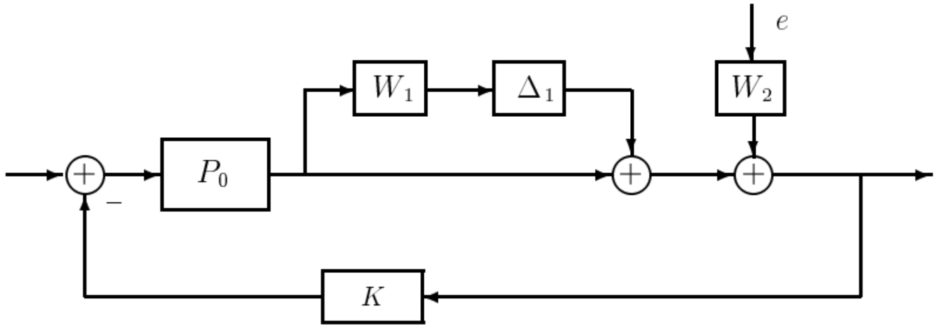
Figure 21.1: Uncertain Plant with Disturbance
