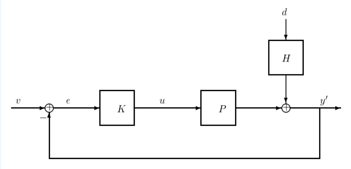
Figure 17.4.2: Example of a unity feedback system.
