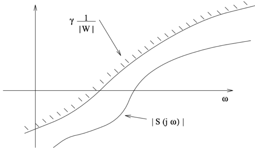
Figure 18.1.3: Graphical interpretation of the sensitivity function being bounded by a scaled reciprocal of the weighting filter frequency response.
