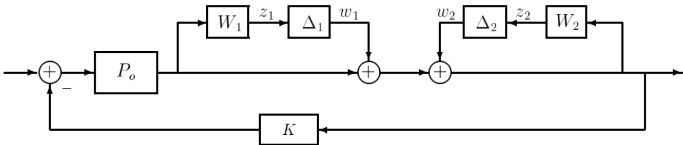
Figure 21.2: Robust Performance Model
