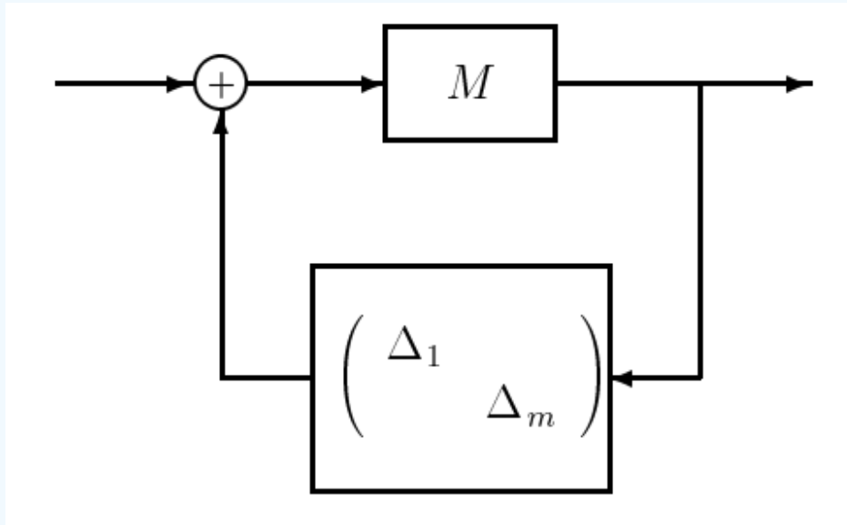
Figure 21.3: M- \Delta Feedback Form
