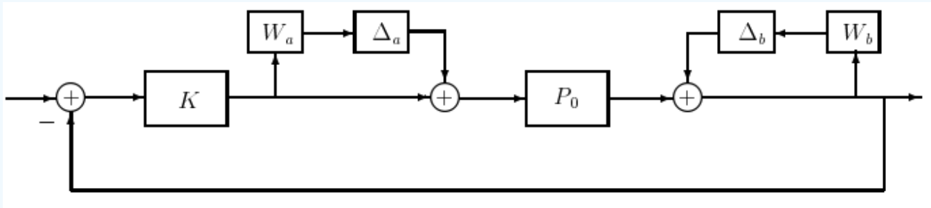
Figure 20.4: Plant with multiple uncertainties.
