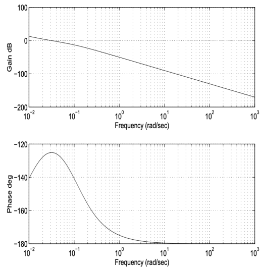
Figure 19.13: Loop Gain P_0K_1
