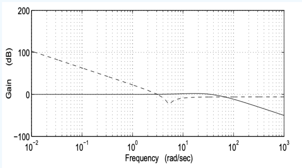
Figure 19.12: |T_0(j\omega)| and [l(\omega)]^{-1}
