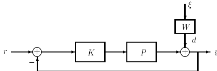
Figure 20.6: Plant with disturbance.
