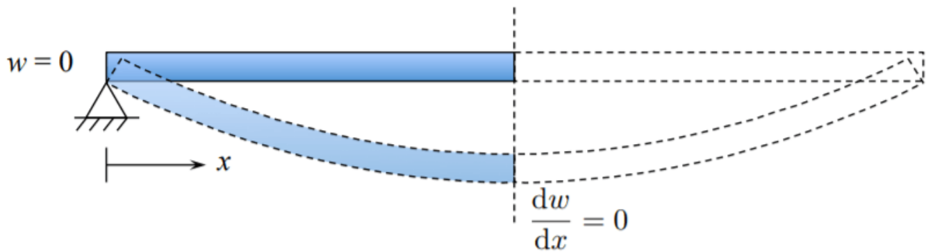
Figure 4.3.2: Symmetry boundary condition.
