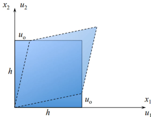
Figure 1.2.3: Imposing constant deformative gradients.
