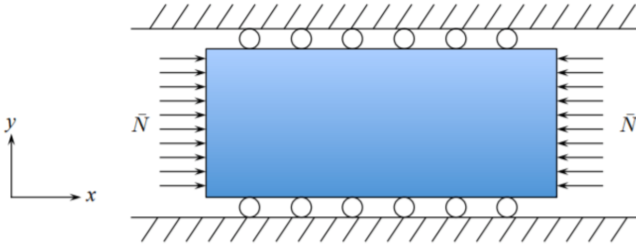
Figure 10.2.2: Constrained compression of the plate.
