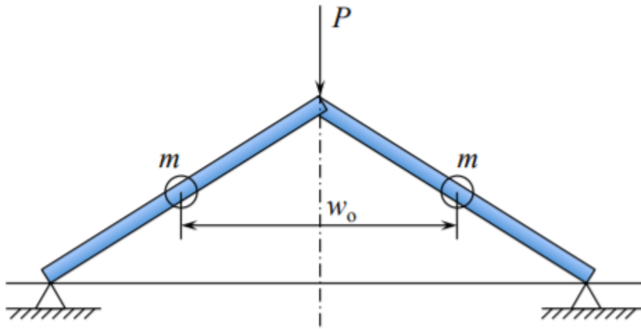
Figure 9.4.1: The equivalent two massless bars and two lumped masses.
