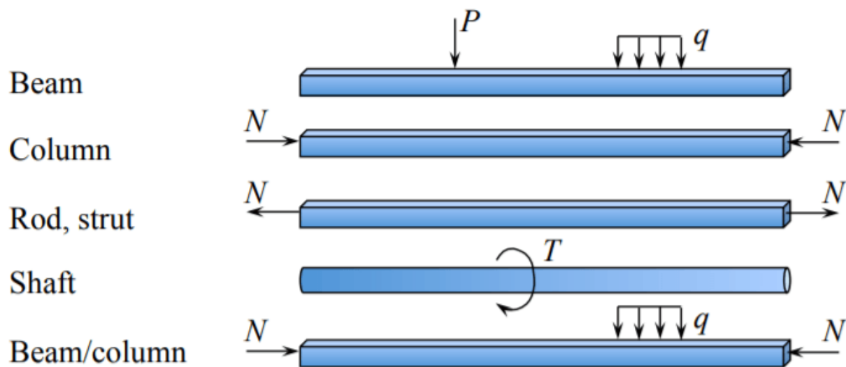
Figure 1.4.1: The type of loading distinguishes between five different types of structures.
