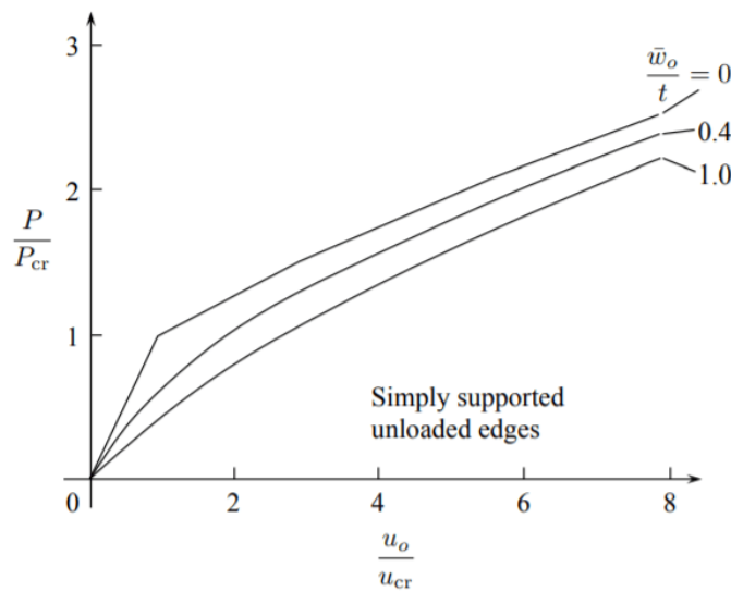
Figure 10.7.1: Load-displacement curves for imperfect simply supported plates.
