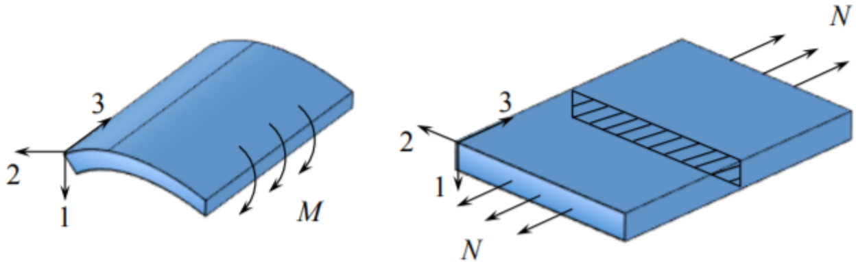
Figure 3.3.2: Tension of bending of a wide sheet/plate gives rise to plane strain.
