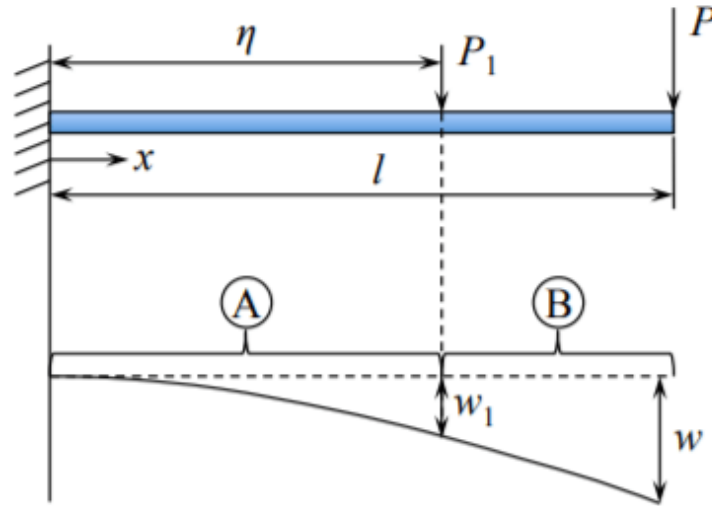
Figure 7.6.5: Cantilever beam loaded by two point forces.
