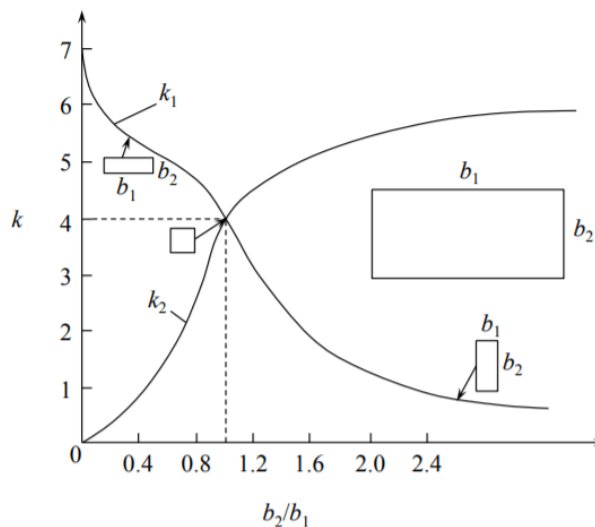
Figure 10.4.7: Buckling coefficients of a rectangular plate as a function of b_2/b_1 .
