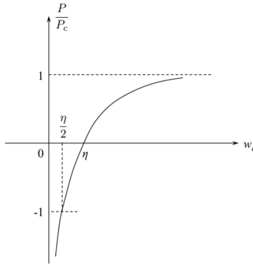
Figure 9.3.1: Relationship between the axial load and lateral deflections.
