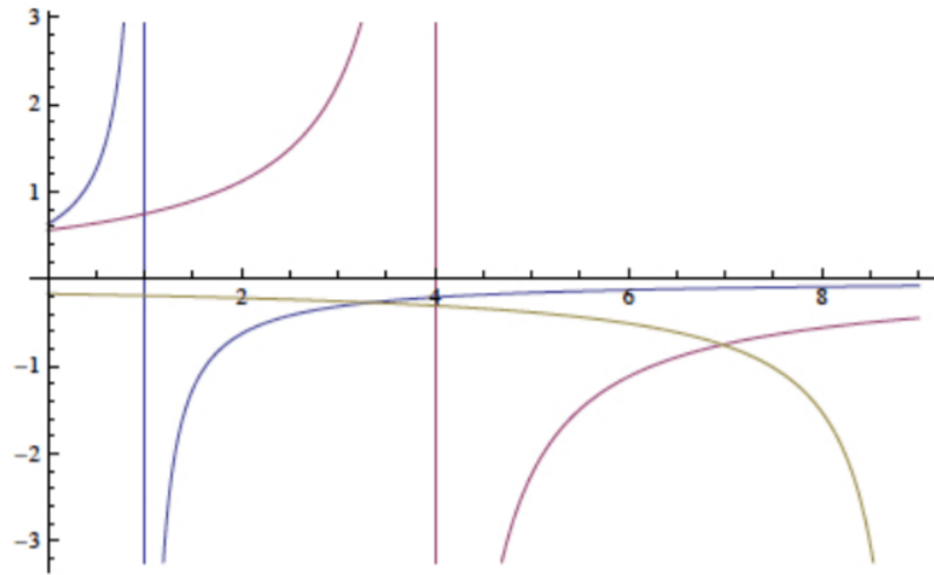
Figure 8.7.4: The deformation amplitudes of the first three modes vs. load \bar{P} curves, for the imperfection shape described by Eqn. 8.7.6.
