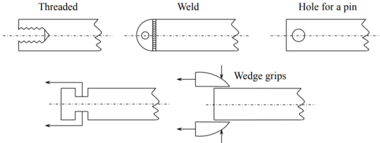
Figure 2.1.2: How to apply tension to the end of a bar.
