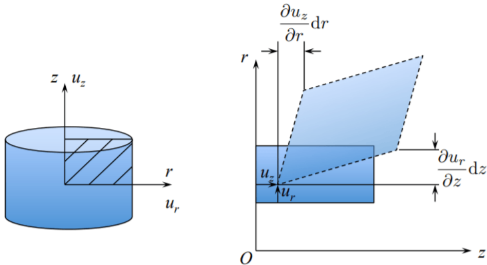
Figure 1.3.5: Change of angles are \{r, z\} plane.
