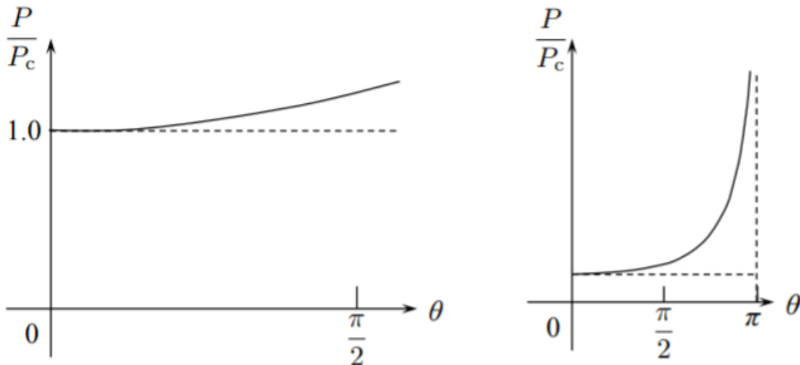
Figure 8.2.4: Plot of the secondary equilibrium path.
