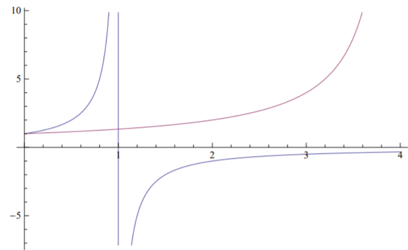
Figure 8.7.2: The deformation amplitudes B_1 , B_2 vs. load \bar{P} curves, for the case A_1 = 1 .
