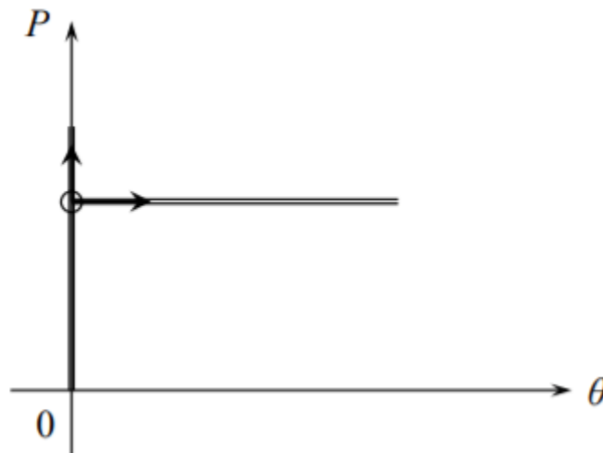
Figure 8.2.3: Two equilibrium paths intersect at the bifurcation point.
