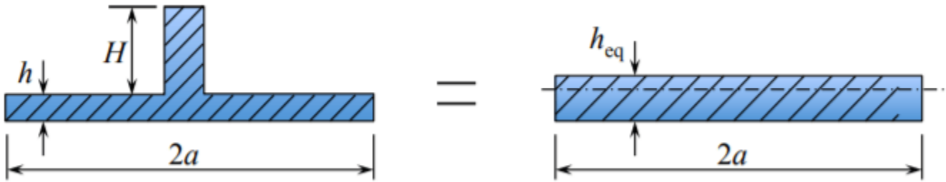
Figure 6.8.1: Geometry of plate/beam combination and the equivalent thickness plate.
