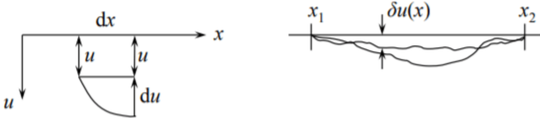
Figure 2.2.1: The local increment \delta u over the infinitesimal length dx and the global small (virtual) displacement from the equilibrium configuration satisfying kinematic boundary conditions.
