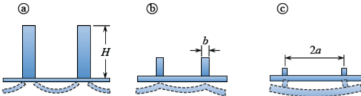
Figure 6.6.7: Heavy, intermediate and light stiffeners.
