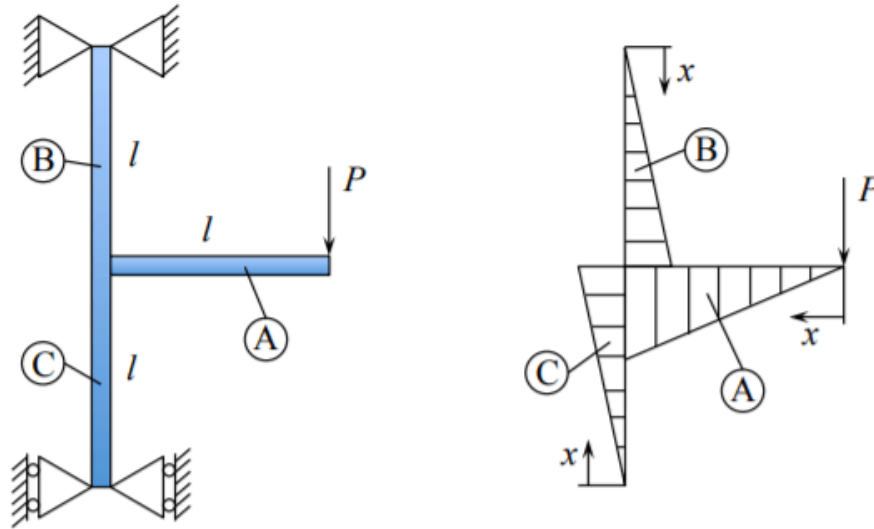
Figure 7.6.2: Statically determined system and bending moment distribution.
