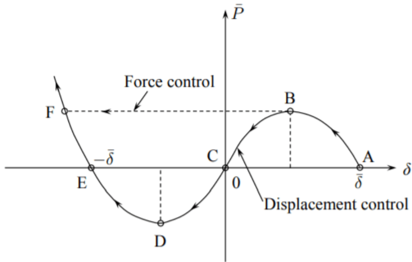
Figure 9.3.4: Equilibrium path in the snap-through problem.
