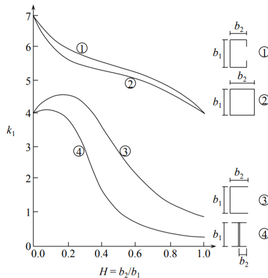
Figure 10.4.8: Buckling coefficients for four types of sections.
