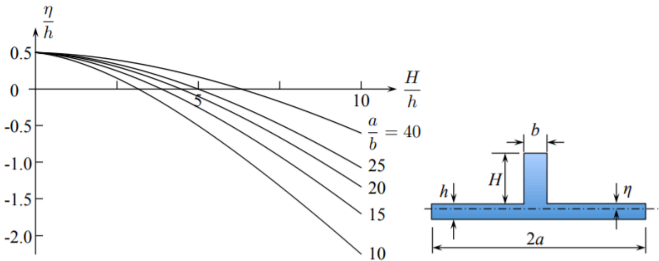
Figure 6.8.2: Neutral axis of the plate/beam combination moves from the plate center towards the original axis of the beam.
