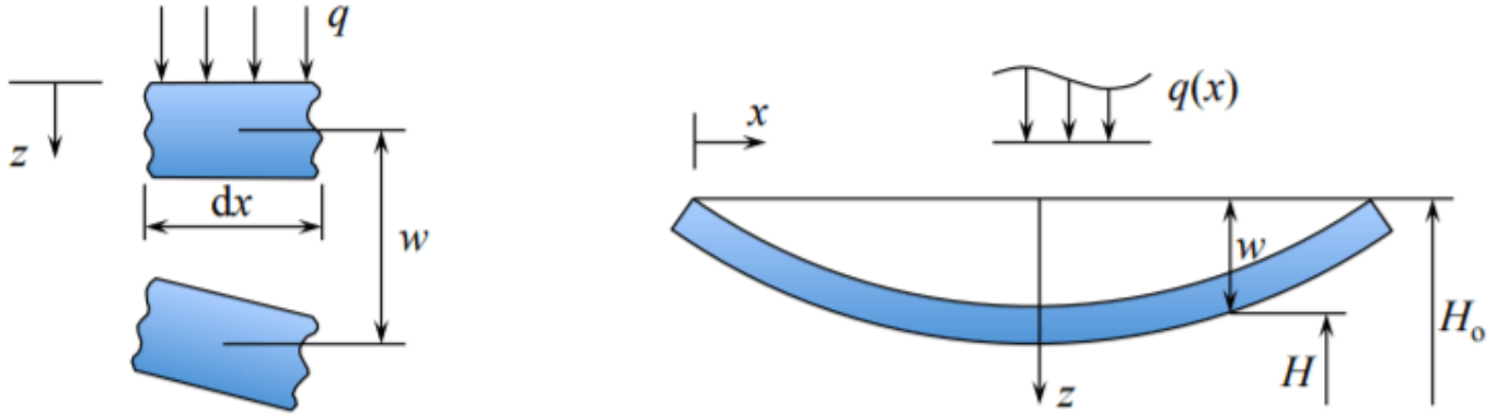
Figure 7.1.2: Potential energy of a beam element and the entire beam.
