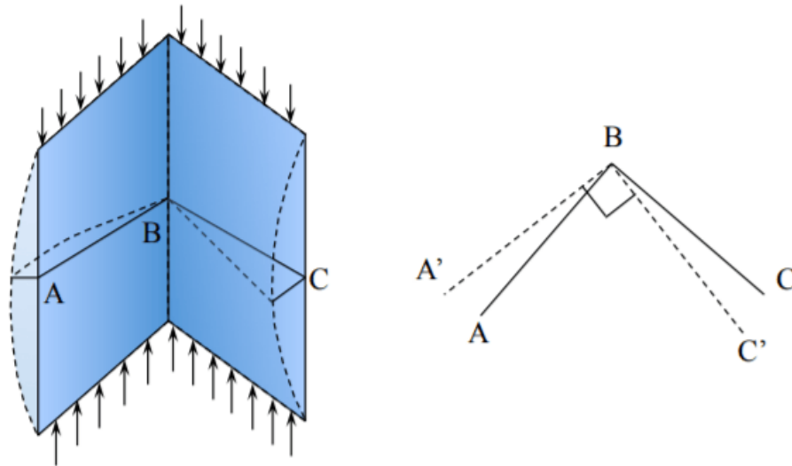
Figure 10.4.2: Buckling mode of an angle element.
