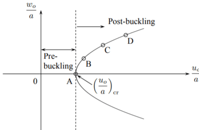
Figure 10.5.2: The out-of-plane displacement amplitude.
