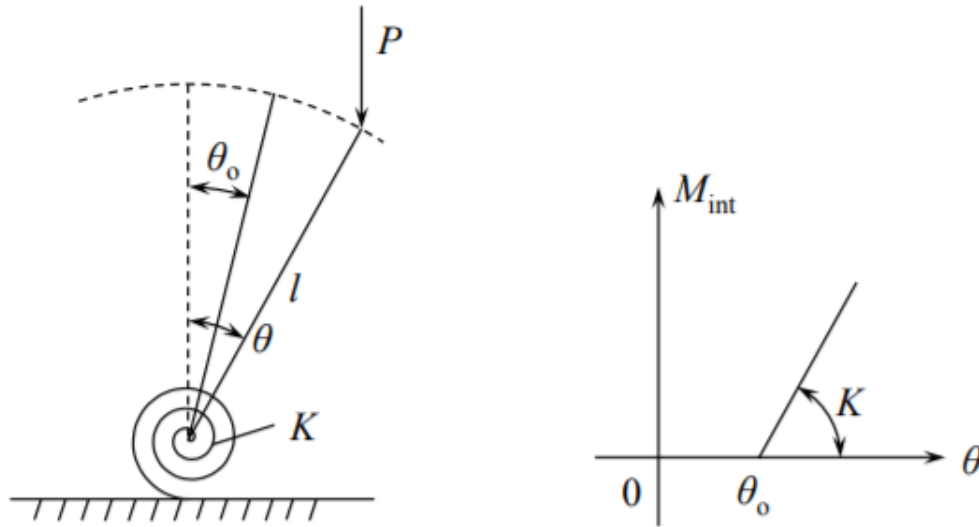
Figure 8.4.1: The initial inclination angle \theta_o is a measure of structural imperfection.
