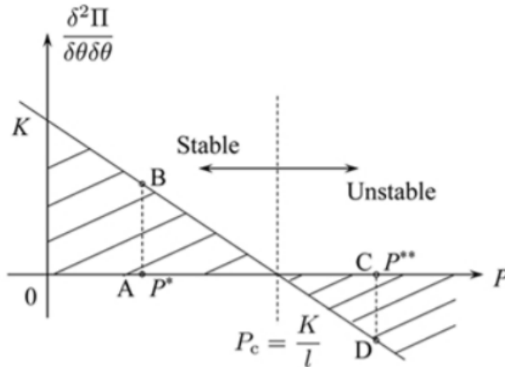
Figure 8.2.1: Stable and unstable range in column buckling.
