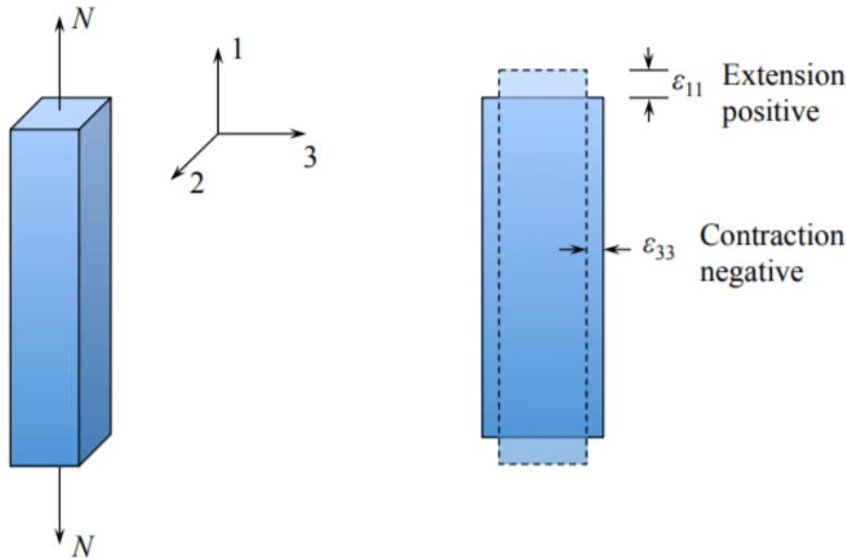
Figure 3.2.1: Uniaxial tension of a bar.
