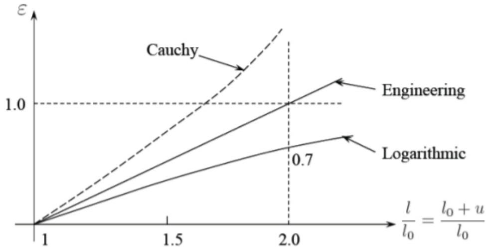
Figure 1.1.1: Comparison of three definitions of the uniaxial strain.
