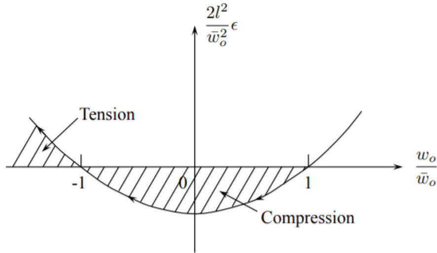
Figure 9.3.3: Transition from compressive into tensile strain.
