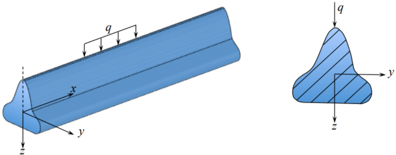
Figure 1.4.2: A prismatic slender beam with a symmetric cross-section.
