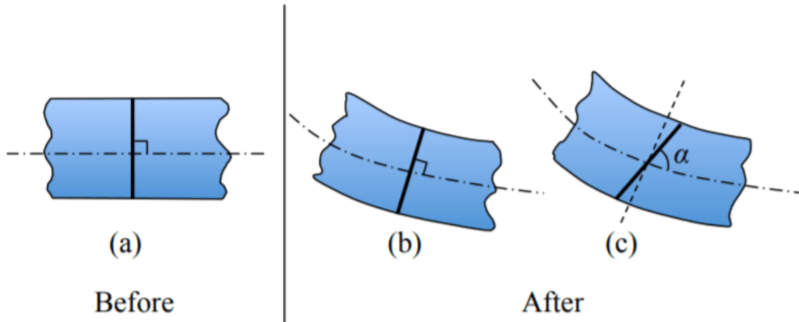
Figure 1.5.2: Testing the normal-remains-normal hypothesis.
