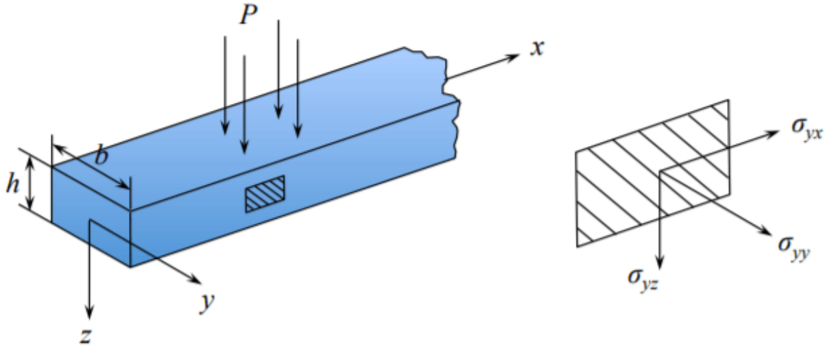
Figure 2.6.1: Vanishing components of the stress vector.
