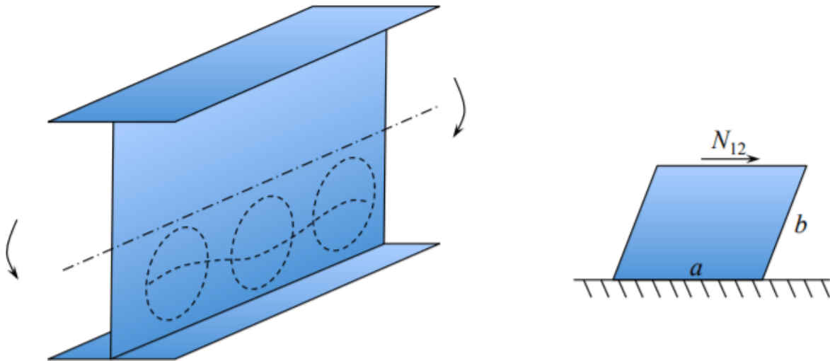
Figure 10.4.4: Buckling due to shear or bending.
