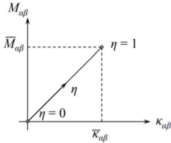
Figure 3.6.2: The straight loading path in the 3-dimensional space of bending moments..
