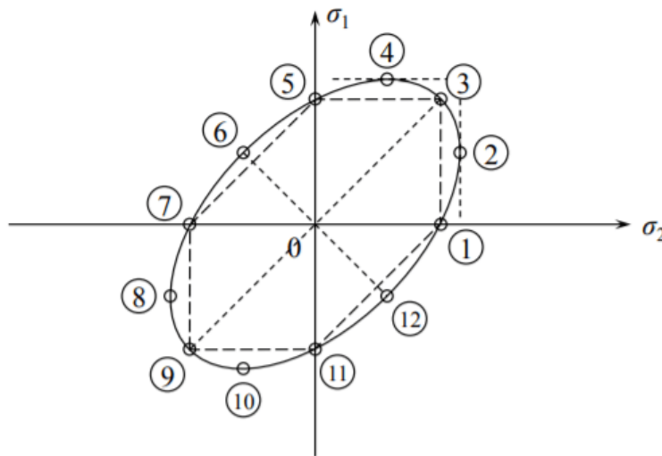
Figure 11.4.2: The von Mises ellipse in the principal coordinate system.
