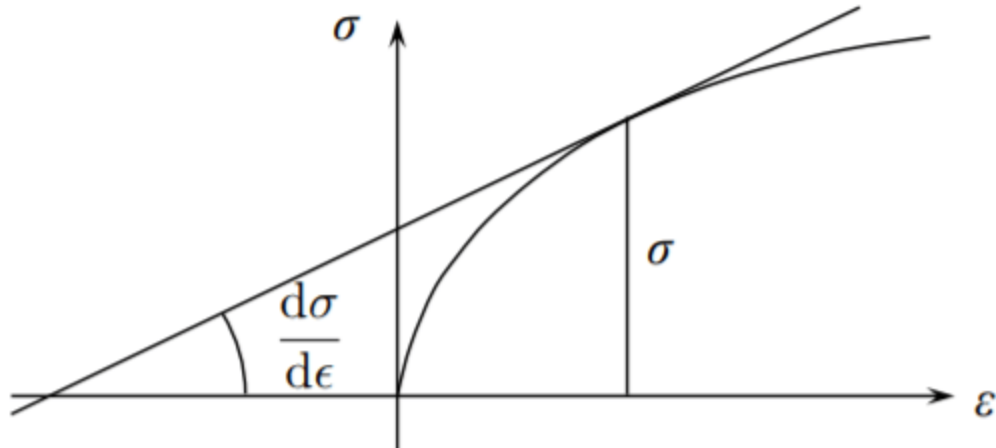
Figure 8.5.2: The construction of Considère' who was the first to derive Equation 8.5.4.
