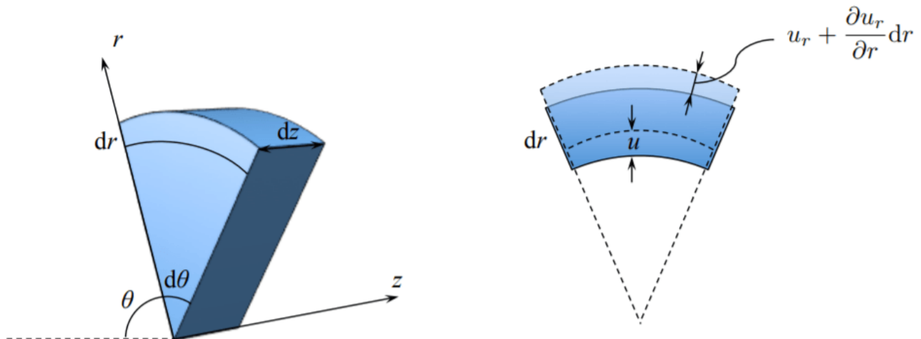
Figure 1.3.2: Change of length in the radial direction.
