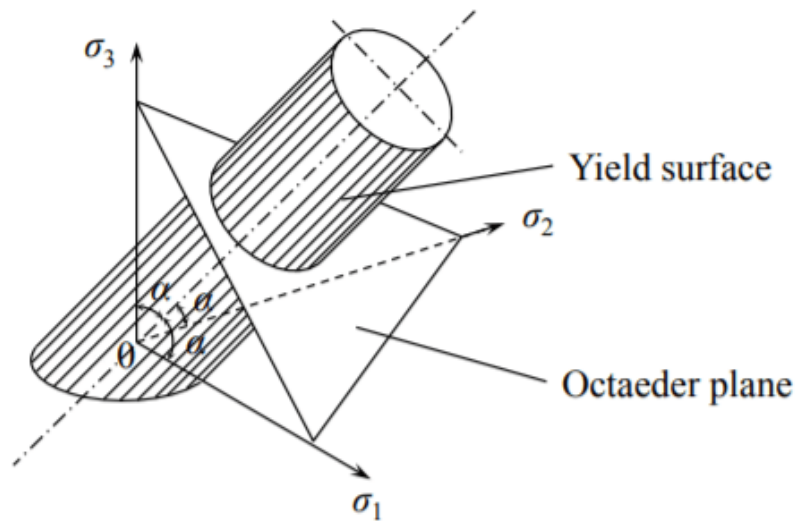
Figure 11.4.1: Representation of the von Mises yield condition in the space of principal stresses.
