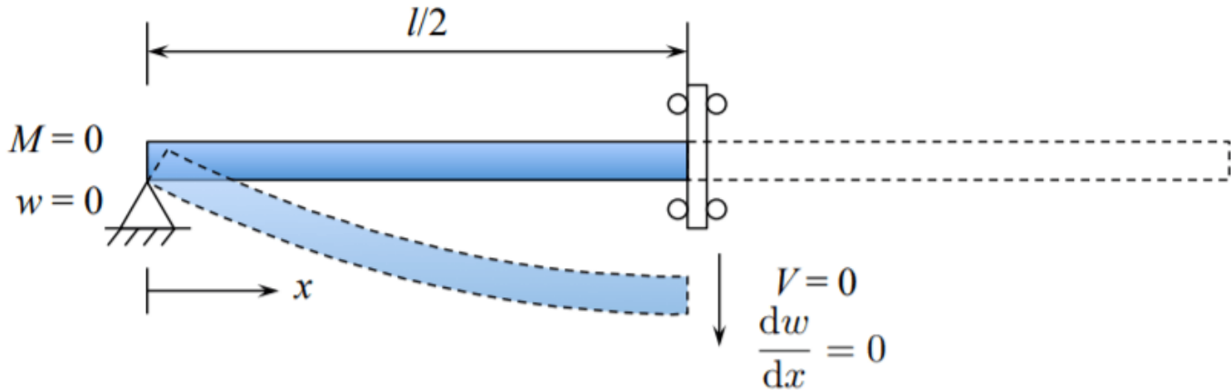
Figure 4.1.4: Simply-supported plate with symmetry boundary conditions.
