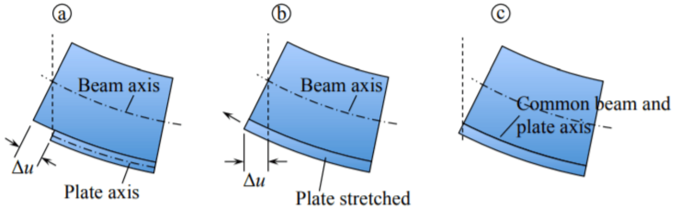
Figure 6.9.1: Incompatible and compatible interface between beam (stiffener) and plate.
