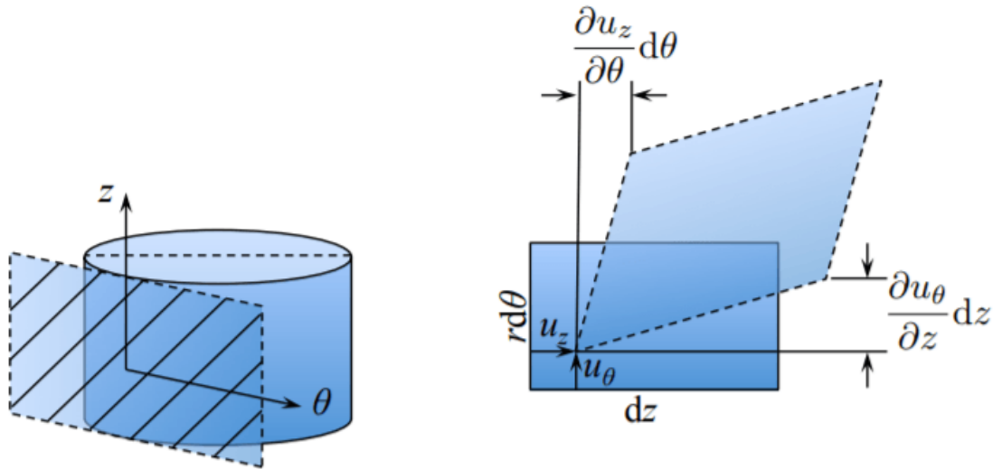
Figure 1.3.6: Visualization of the strain component \epsilon_{\theta z} .
