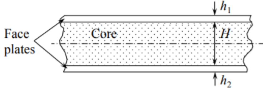
Figure 6.5.1: There are two materials and three different thicknesses in sandwich plates.
