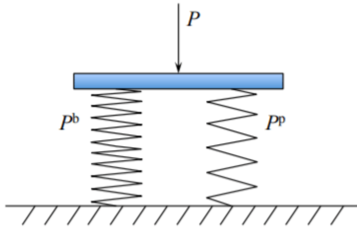
Figure 6.6.6: Two spring in series.
