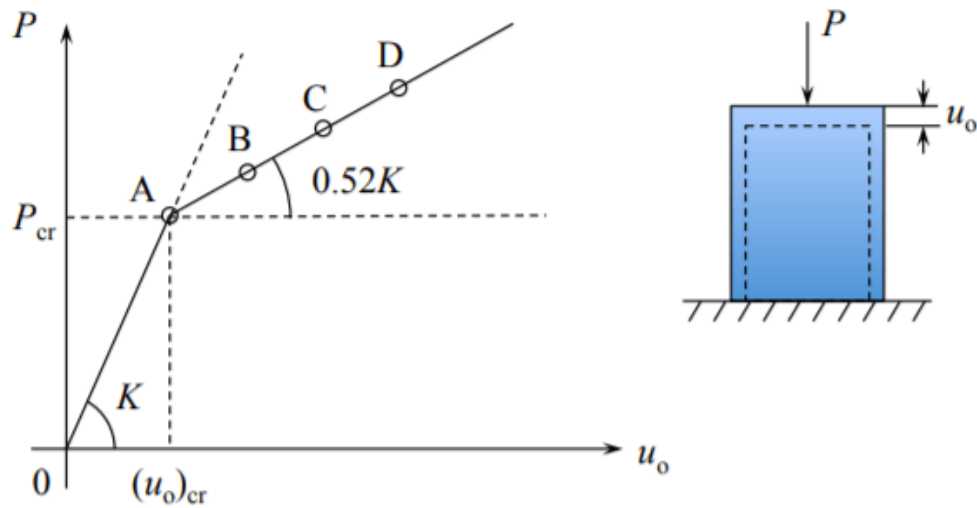
Figure 10.5.3: Pre and post-buckling response of a plate.
