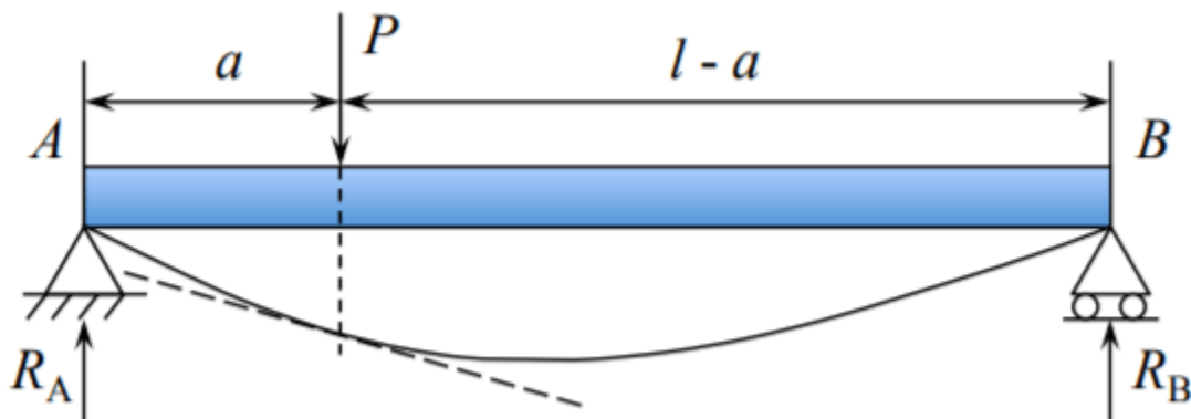
Figure 4.3.3: Beam under off-center point load.
