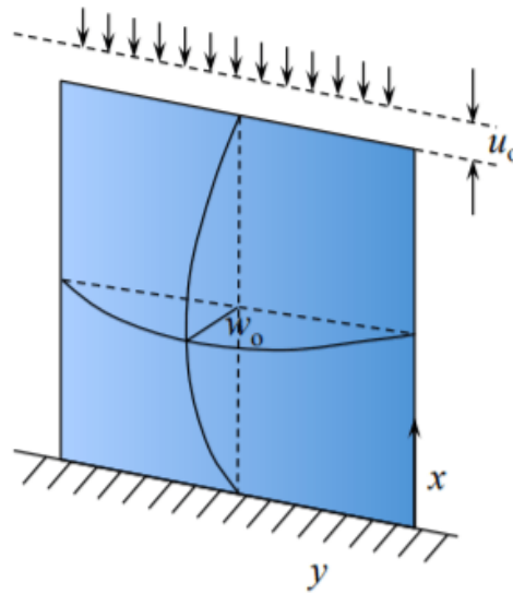
Figure 10.5.1: Two degree-of-freedom model of the buckled plate.
