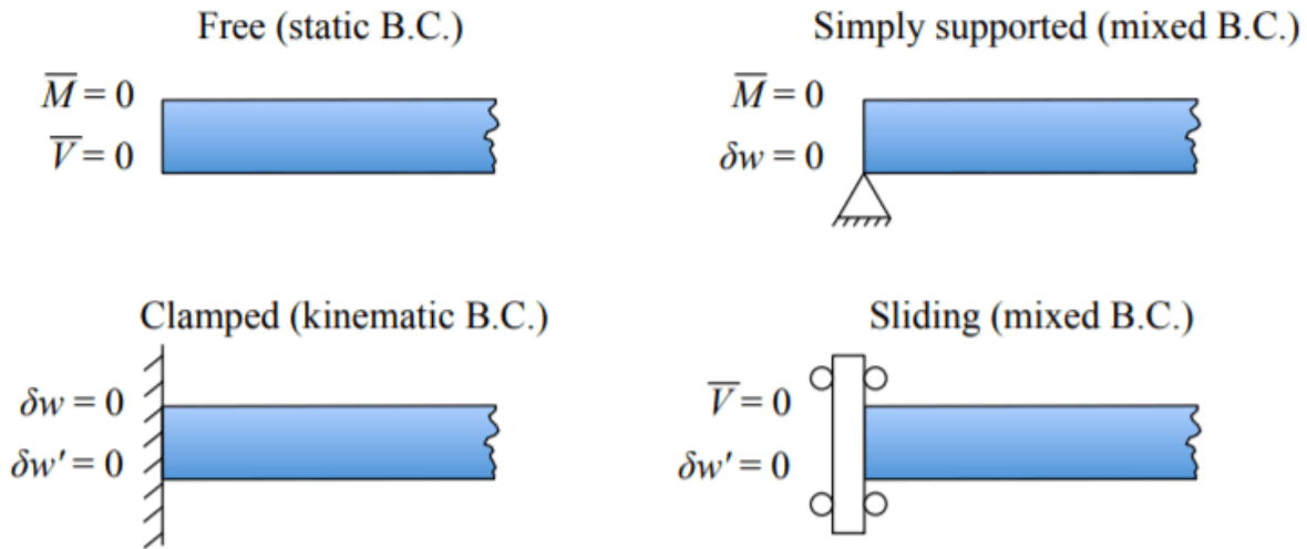
Figure 2.5.1: Boundary conditions in the axial direction.
