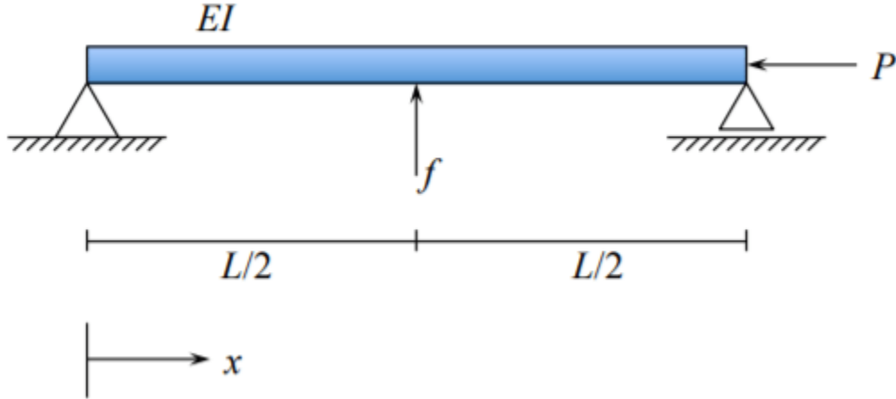
Figure 9.2.1: Simply supported beam with intermediate transverse load.
