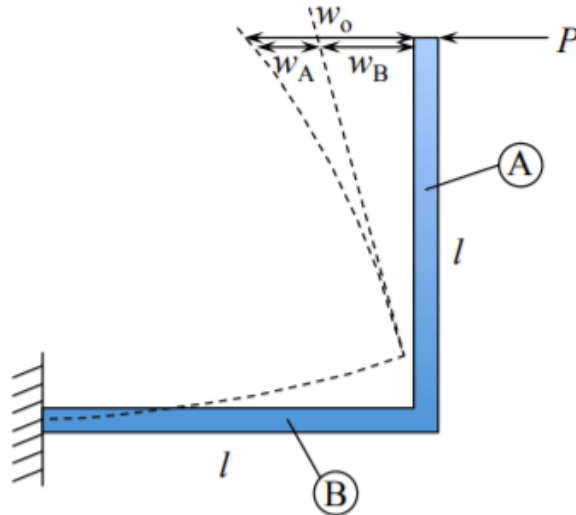
Figure 7.6.3: two welded beams forming an elbow.
