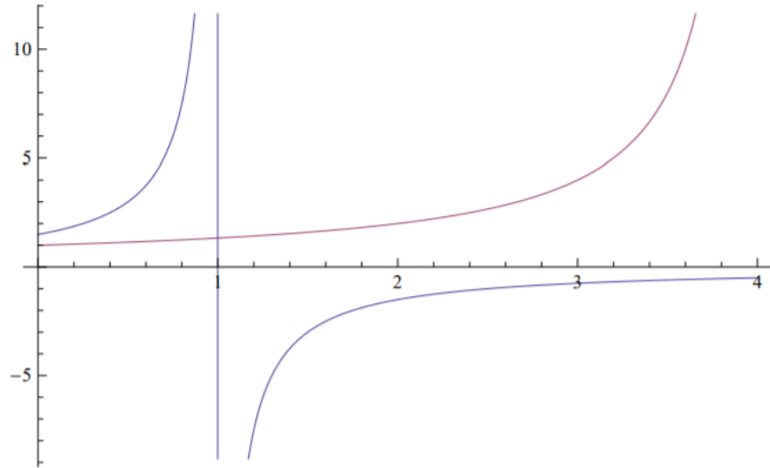
Figure 8.7.3: The deformation amplitudes B_1 , B_2 vs. load \bar{P} curves, for the case A_1 = 1.5 .
