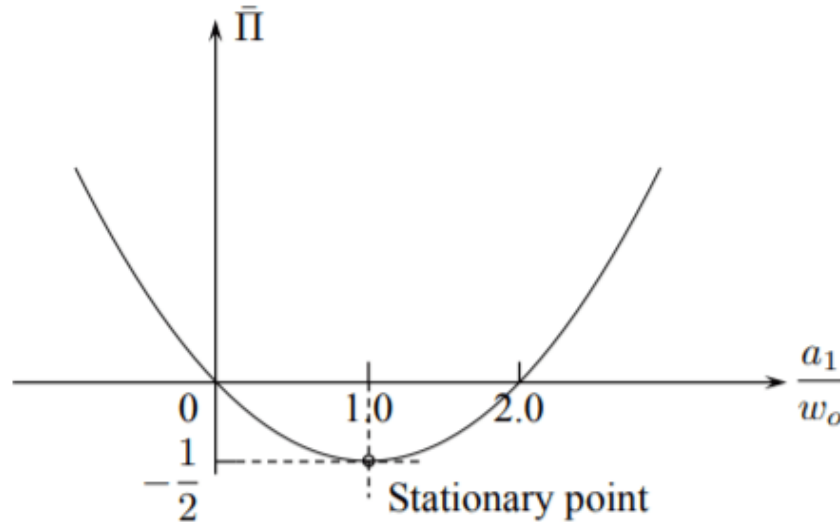
Figure 7.4.2: By varying the amplitude around \frac{a_1}{w_o} = 1 , \bar{\Pi} does not change.
