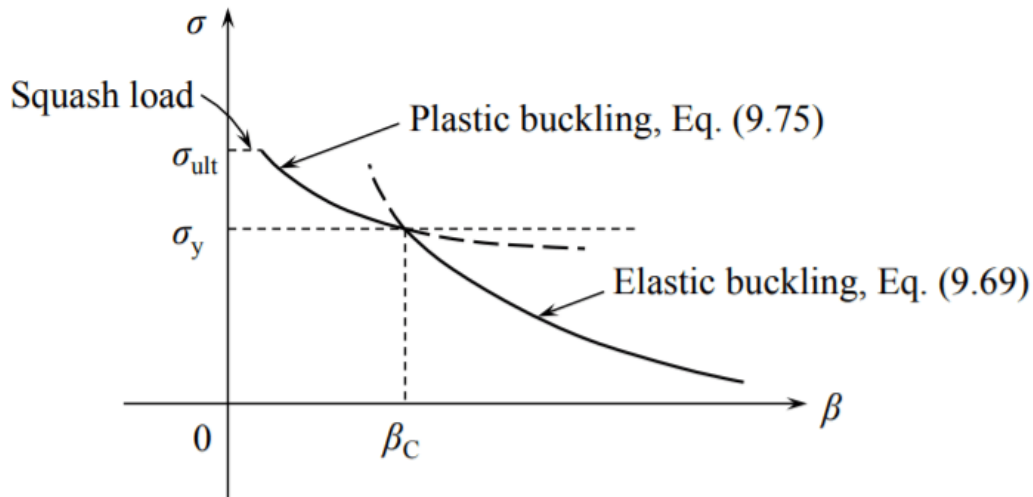
Figure 8.6.2: Range of elastic and plastic buckling.
