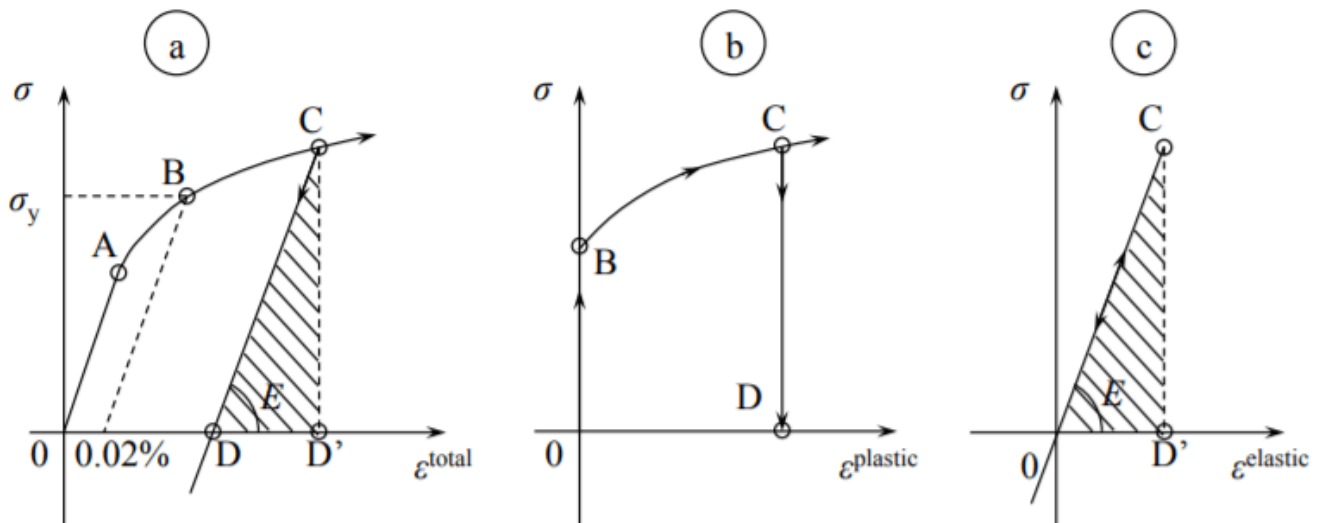
Figure 11.1.1: Elastic, plastic and total stress-strain curve.
