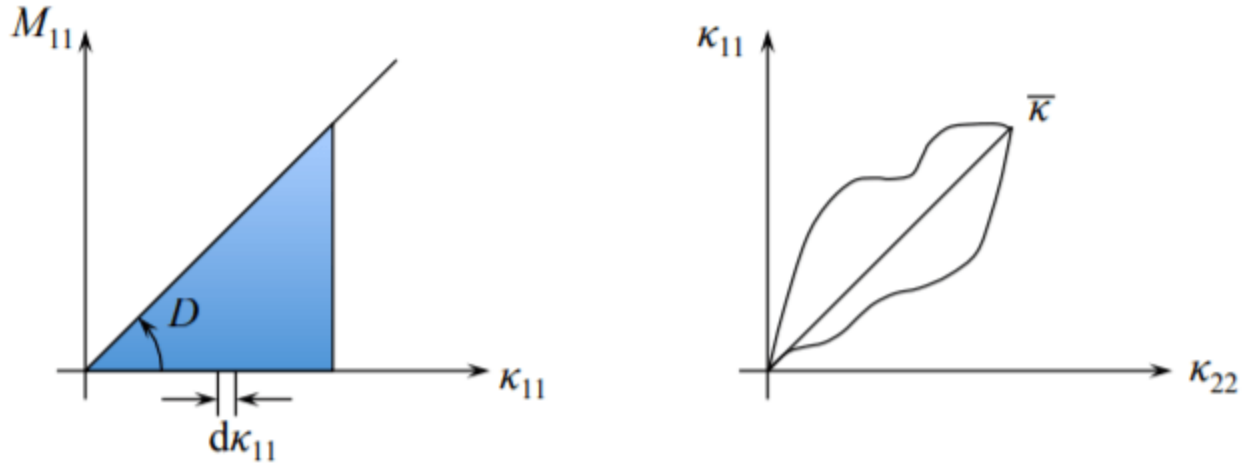
Figure 3.6.1: In one dimension the energy density is the area under the linear moment-curvature plot. In the multi-axial case the final value can be reached along the straight or nonlinear path.
