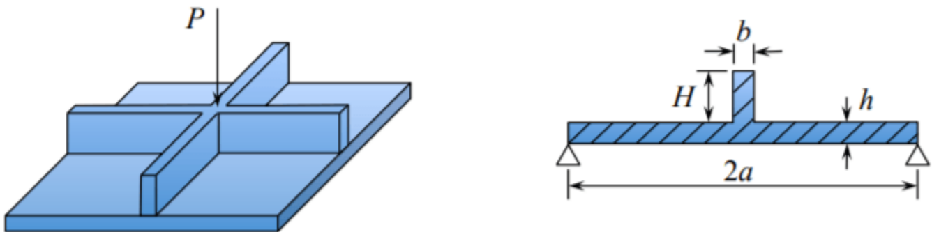
Figure 6.6.3: Geometry of the stiffened plate.
