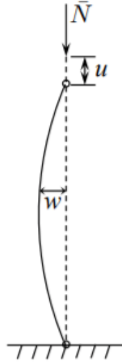
Figure 8.3.1: Initial and deformed elastic column.
