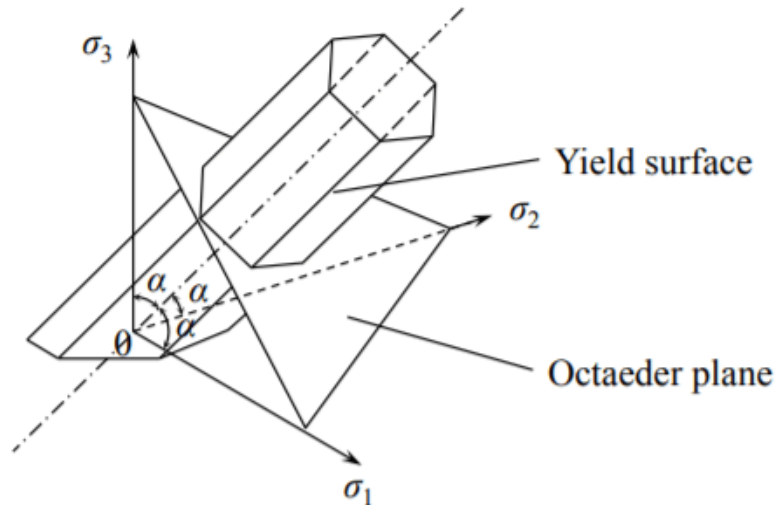
Figure 11.8.2: Representation of the Tresca yield condition in the space of principal stresses.
