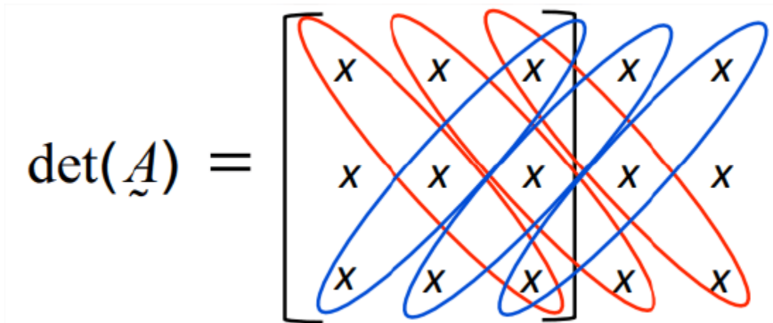
Figure 15.3.2: Elementary recipe for computing the determinant of a 3 \times 3 matrix for comparison with Equation 15.3.4. Combinations marked in red (blue) are added (subtracted).
