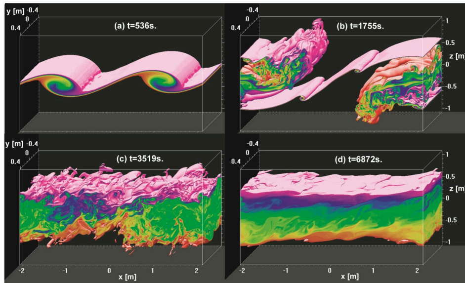
Figure 5.3.4: Evolution of turbulence between an upper layer of fresh water (blue-magenta) flowing to the right and a lower, salty layer (red) flowing to the left. Colors indicate intermediate salinity in the transition layer, with the outer layers rendered transparent for clarity. The flow was obtained as a numerical solution of the partial differential equations describing fluid motions in the Eulerian framework. These will be derived in chapter 6. (Image from Smyth and Thorpe 2012).
