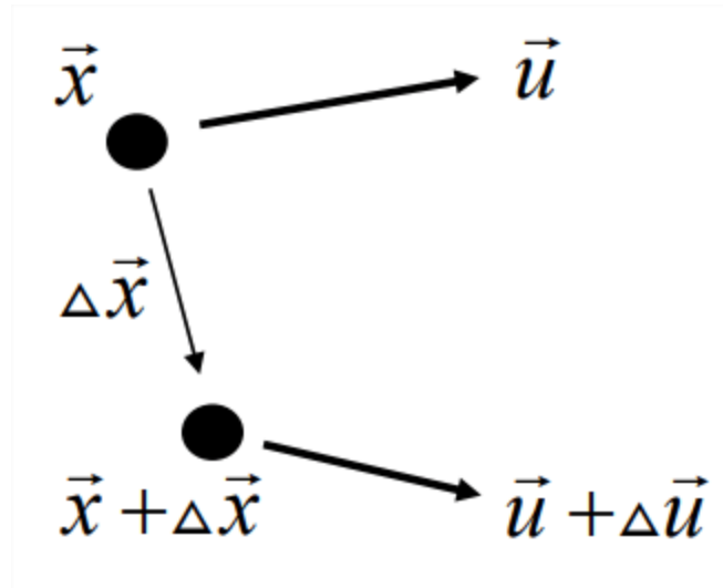
Figure 7.2.1: Relative motion of two nearby fluid particles, reproduced from Figure 5.3.2).
