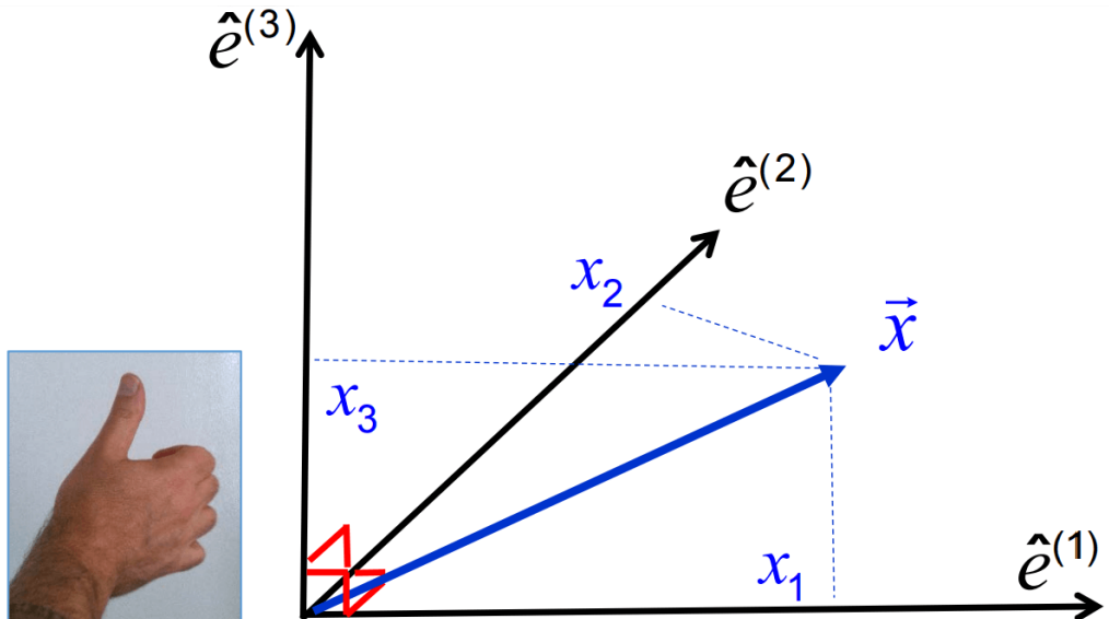
Figure 3.1.1: A position vector \vec{x} in a right-handed Cartesian coordinate system. The x_i are the components of \vec{x} or, equivalently, the coefficients for the linear combination Equation 3.1.2.
