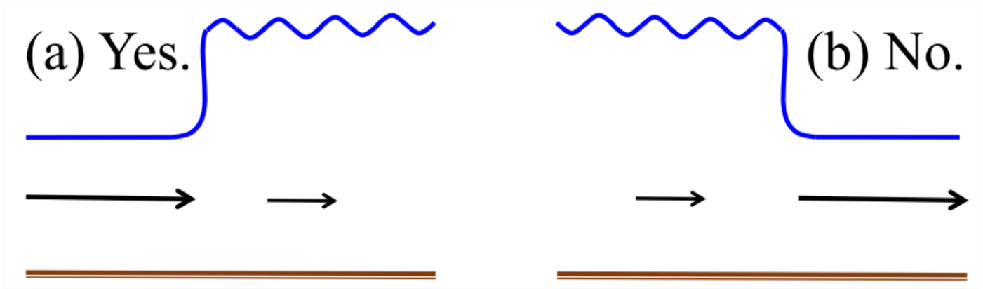
Figure 9.3.3: Why do hydraulic jumps always look like (a), and never (b)?
