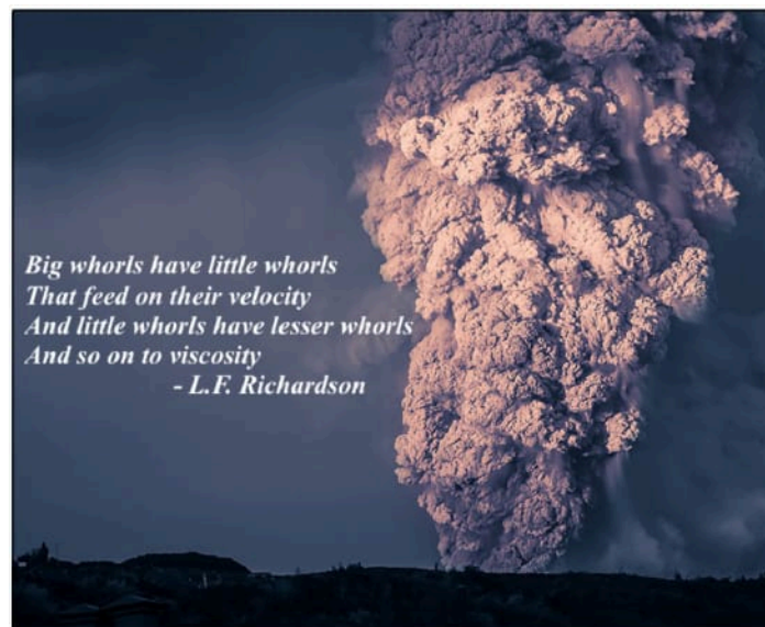
Figure 9.3.2: Based on the traditional nursery rhyme Fleas , Lewis Fry Richardson's tongue-in-cheek description of the turbulent energy cascade is both poetic and accurate. The “whorls” shown here, both big and little, were generated by the Colbuco volcano in Chile, photographed by Marcelo Reyes. Richardson, 1881-1953, was an English mathematician and psychologist. He invented the first algorithms for numerical weather forecasting decades before there were computers to execute them. He was also a dedicated pacifist and published important statistical studies on the causation and prevention of wars.
