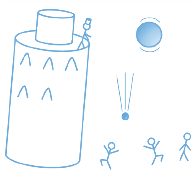
Figure 17.1.1: If the gravitational force was independent of mass.
