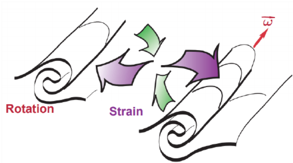
Figure 5.3.1: Schematic of co-rotating vortices, similar to (Figure 5.2.1), showing regions of rotation and strain.
