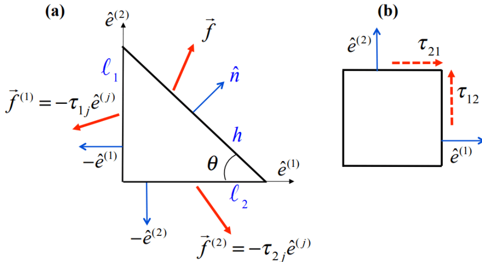
Figure 6.3.4: Two-dimensional representations of stresses acting on (a) a right triangle, (b) one corner of a rectangle. As the size of each figure goes to zero, net forces and torques must vanish.
