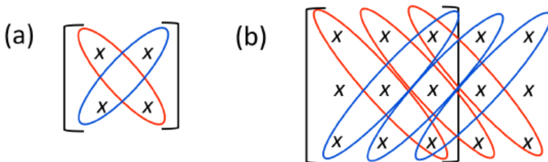
Figure 2.2.2: Groups of elements to be multiplied when computing the determinant. Products of terms outlined in red are added; products in blue are subtracted. In the 3 \times 3 case, the first two columns are repeated outside the matrix.
