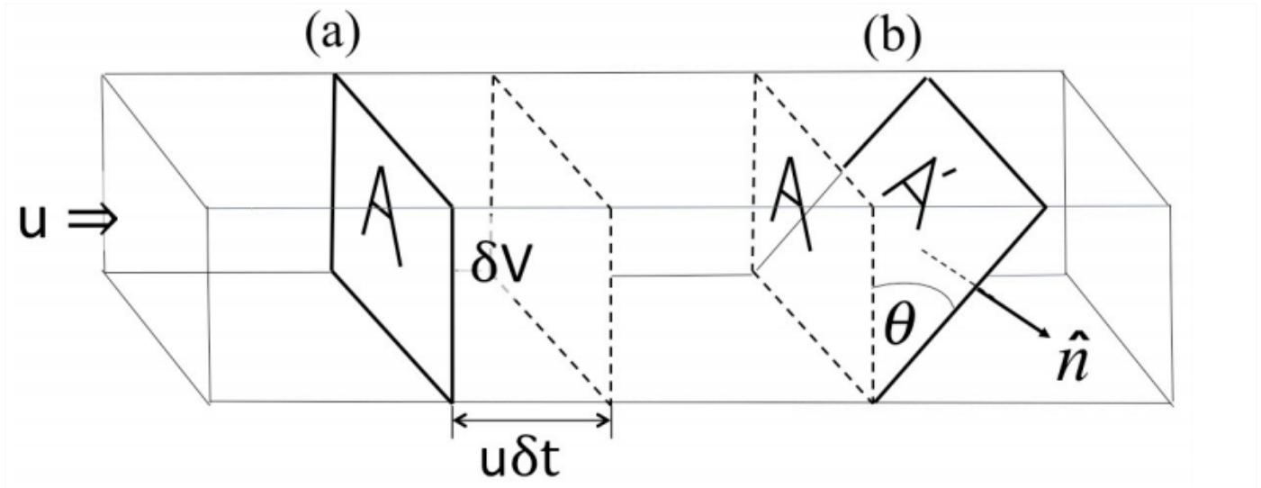
Figure 4.2.1: Volume flux through a rectangular channel. (a) A rectilinear cross-section showing the volume transport in a time \delta t . (b) A tilted cross-section with unit normal \hat{n} .
