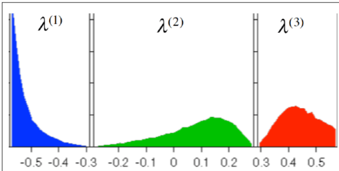
Figure 5.3.12: Probability distributions of the strain eigenvalues in a numerical simulation of sheared turbulence. The values are normalized by \sqrt{2e_{ij}e_{ij}} (Smyth 1999).
