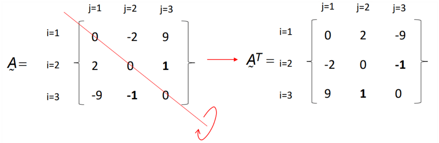
Figure 15.1.1: (a) Example of an antisymmetric two-dimensional matrix. Transposing the matrix changes the sign of every element.
