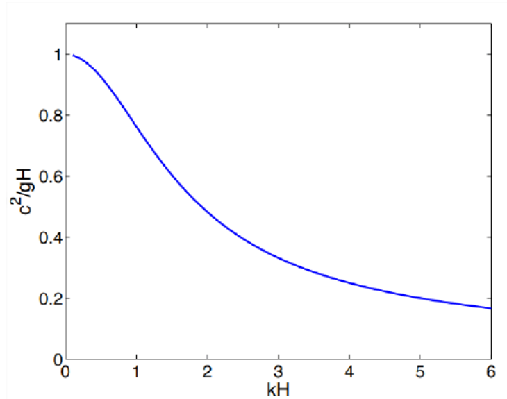
Figure 8.2.2: Dispersion relation Equation 8.2.23 for small-amplitude surface gravity waves.
