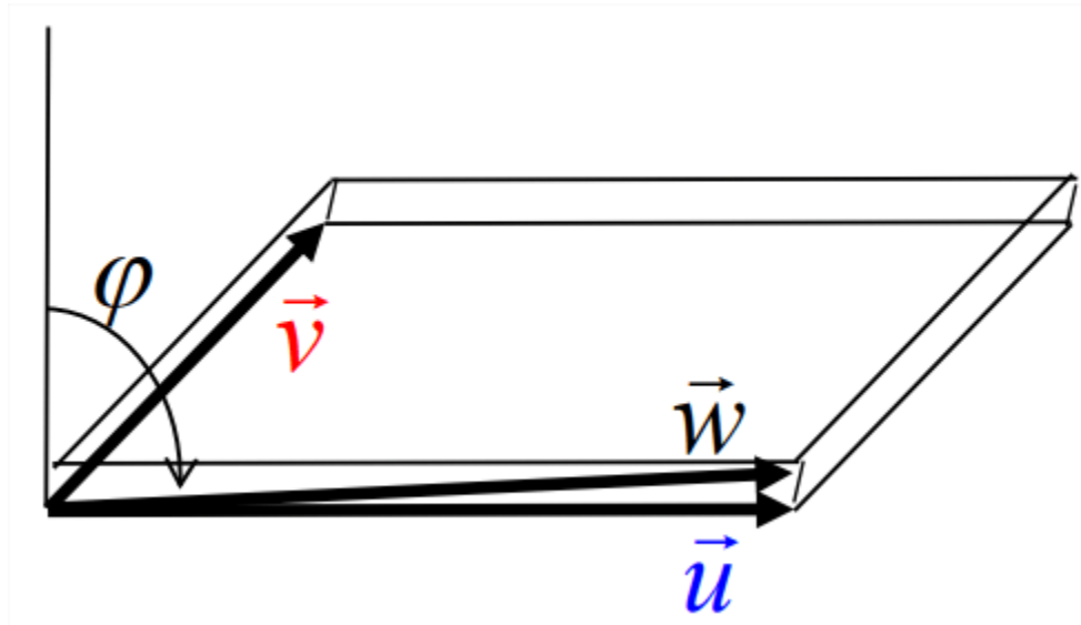
Figure 15.3.1: As \vec{w} turns into the plane of \vec{u}, \vec{v} , the volume of the parallelepiped shrinks to zero.
