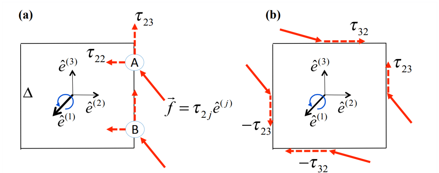
Figure 17.3.1: Forces acting to rotate a cube about \hat{e}^{(1)} . (a) Effects of the same force acting at points above and below the x_2 -axis. (b) Tangential forces acting on all four faces.
