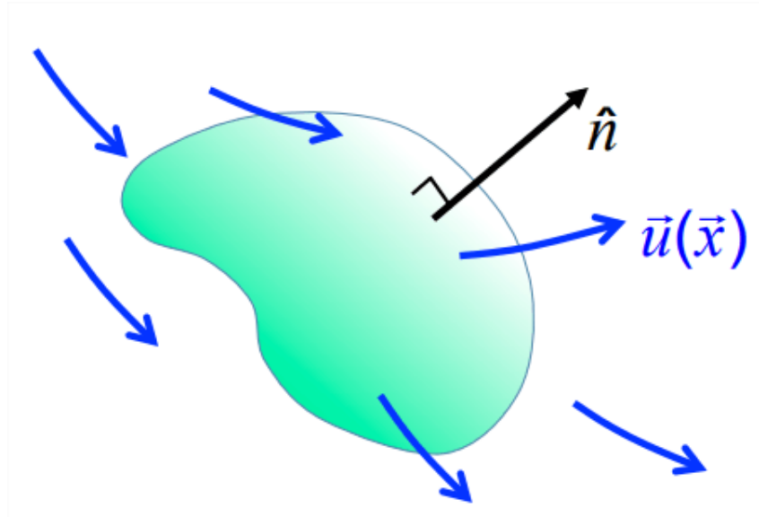
Figure 4.2.5: An arbitrary, simply connected volume, with outward normal \hat{n} , embedded in an arbitrary flow field \vec{u}(\vec{x}) .
