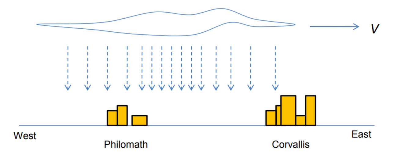
Figure 11.1: A rain storm moving eastward from Philomath to Corvallis.
