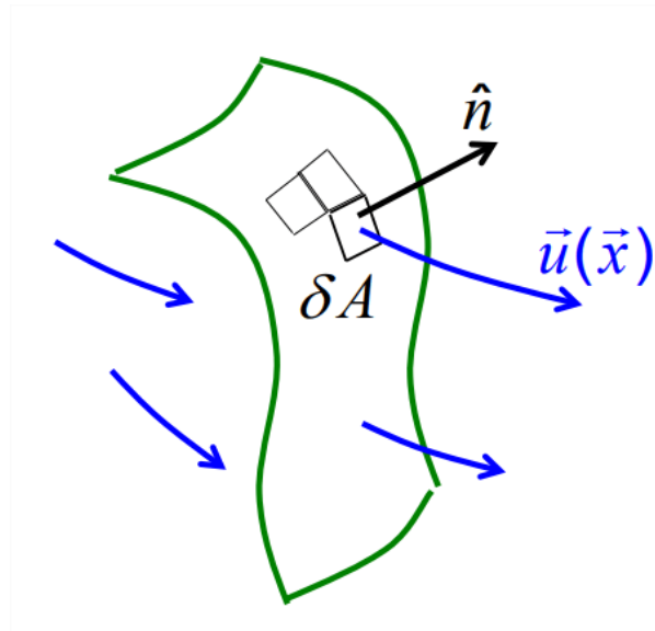
Figure 4.2.2: Volume flux through an arbitrary surface tiled by surface elements with area \delta A and unit normal \hat{n} .
