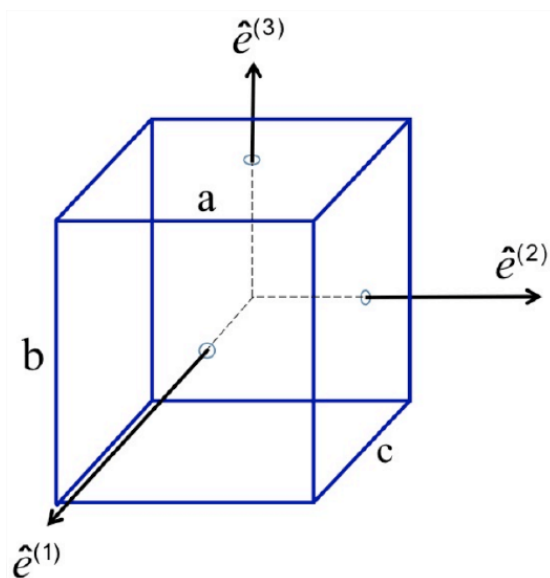
Figure 13.2.1: Definition sketch for the moment of inertia matrix. The example shown is a rectangular prism with sides a , b , and c .
