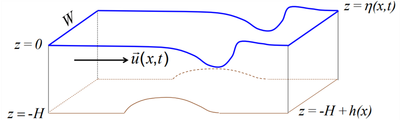
Figure 9.2.1: Two-dimensional flow in an inviscid, homogeneous fluid with a free surface. The vertical coordinate is directed opposite to gravity (upward). The mean surface is z = 0 and the mean depth is H .
