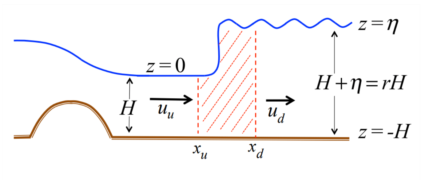
Figure 9.3.1: A hydraulic jump downstream of a constriction. The jump is enclosed by the region x_u < x < x_d . Upstream and downstream flows have velocity and depth equal to \{u_u, H\}, \{u_d, rH\} .
