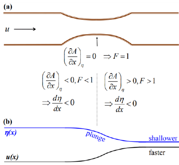
Figure 9.2.5: Flow through an arbitrary constriction. (a) Plan view. (b) Elevation and velocity profiles.
