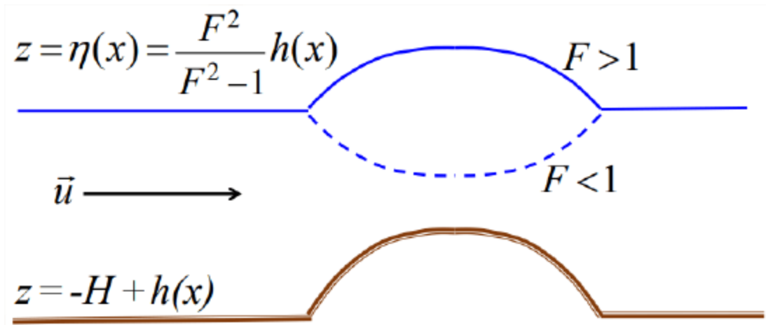
Figure 9.2.2: Steady, small-amplitude flow over an obstacle. The sign of the surface deflection depends on the Froude number in accordance with Equation ???.
