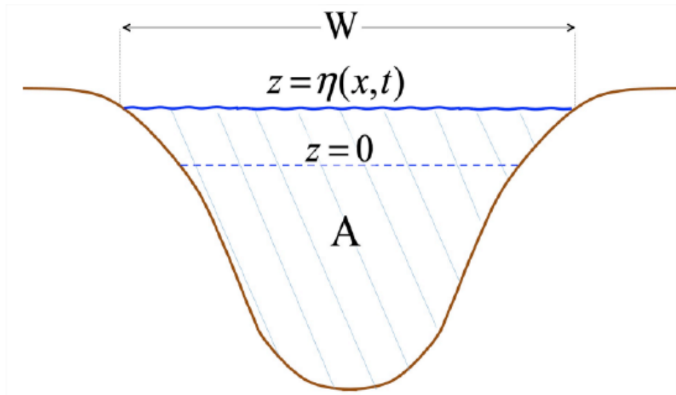
Figure 9.2.4: Cross section of a channel of arbitrary shape. W(x, \eta) is the surface width; A(x, \eta) is the wetted area.
