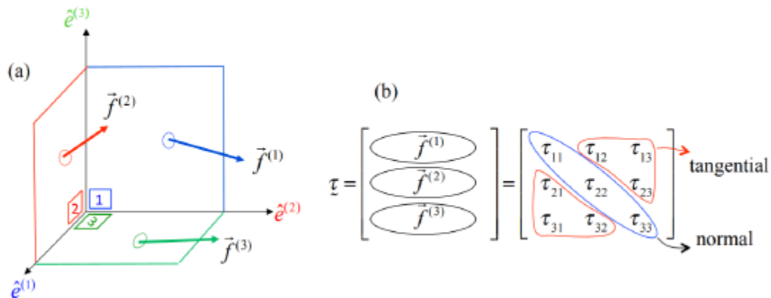
Figure 6.3.3: Stress on coordinate planes. (a) Vectors illustrate stress (force per unit area) acting on three coordinate planes. Colors indicate the force vector and the unit normal associated with each plane. (b) Array formed by the stress components, \tau_{ij} = f_j^{(i)} . Normal and tangential components are colored as in Figure 6.3.2.
