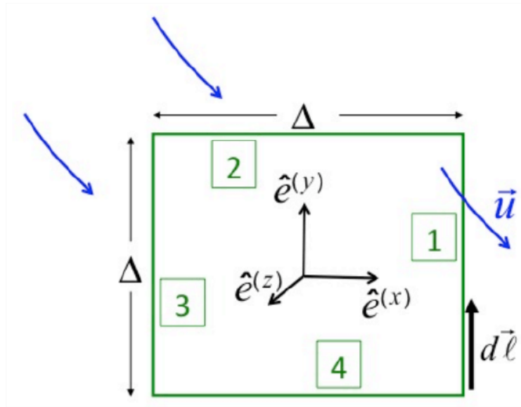
Figure 4.3.2: Circulation Equation 4.3.2 around a \Delta \times \Delta square on the \hat{e}^{(x)} - \hat{e}^{(y)} plane with line element d\vec{\ell} .
