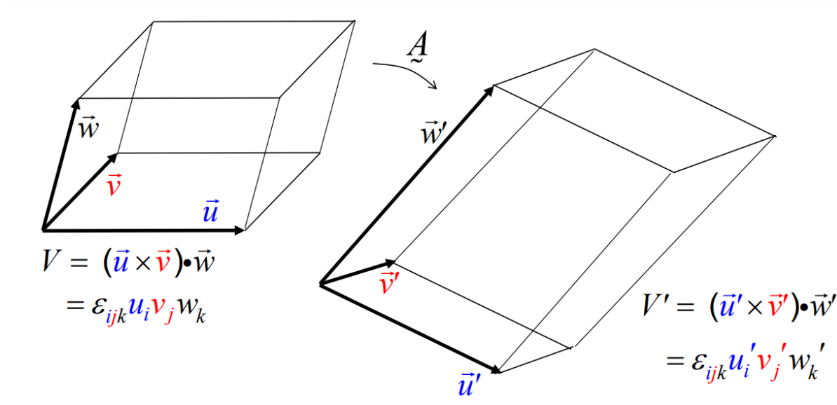
Figure 15.3.3: Transformation of the parallelepiped enclosed by three arbitrary vectors when the vectors are transformed by the arbitrary matrix A .
