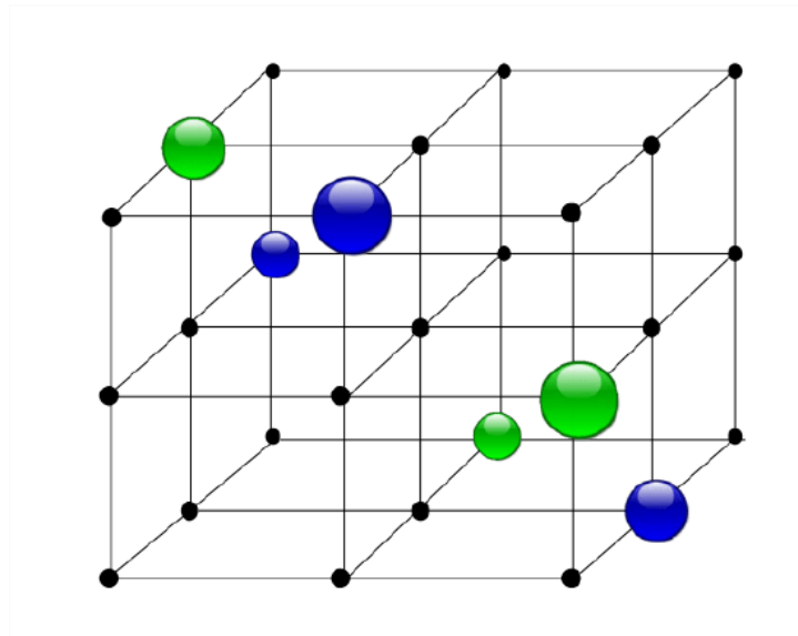
Figure 3.3.2: Schematic of the Levi-Civita alternating tensor. Blue = 1, green = -1, black = 0.
