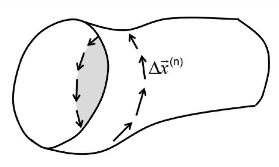
Figure 7.2.5: Line integral around a vortex tube represented as a sum of small increments.
