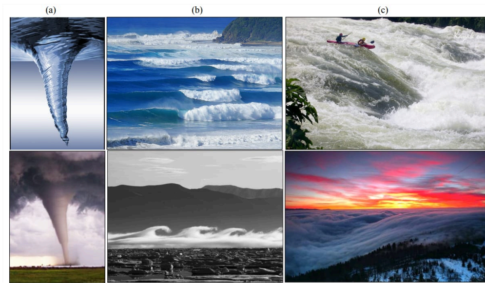
Figure 1.1.1: Fluid phenomena in water and air: (a) vortices, (b) gravity waves, and (c) hydraulic jumps. (For photo credits see page ii.)
