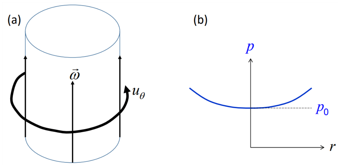
Figure 7.2.6: (a) A columnar vortex tube. (b) Radial pressure variation.
