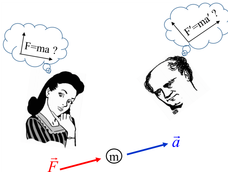
Figure 3.1.4: Two observers evaluating Newton's second law.
