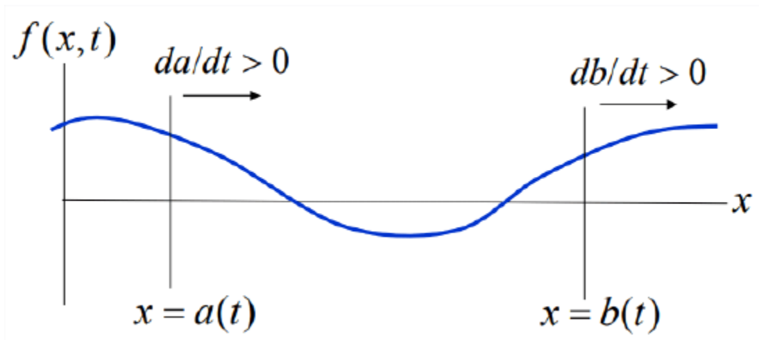
Figure 6.1.2: Definition sketch for the 1-dimensional form of Leibniz rule.
