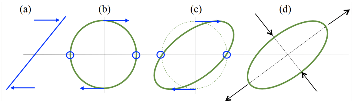
Figure 5.3.11: Evolution of an initially circular distribution of fluid particles in a uniform, transverse strain. (a) Velocity profile. (b) Initial circle. Arrows indicate the motion of the top and bottom of the circle; small circles indicate points that do not move. (c) After a short time the circle becomes a tilted ellipse. (d) When viewed in a tilted coordinate frame (dashed axes), the strains are purely extensional and compressive (black arrows).
