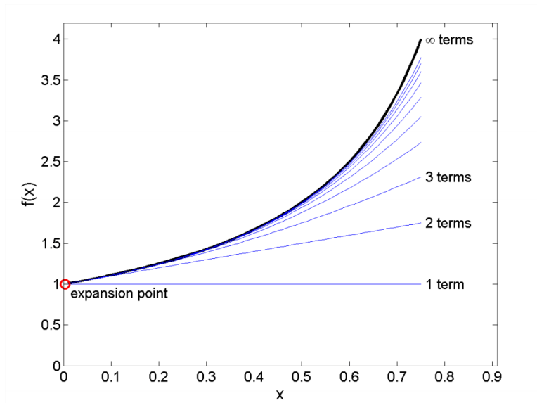
Figure 12.2: Taylor series expansions of the function f(x) = 1/(1-x) about x = 0 . Accuracy increases as more terms are retained. The thick curve is the exact function.
