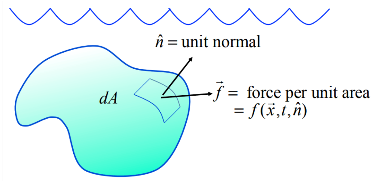
Figure 6.3.1: Definition sketch for the stress vector acting across an arbitrary surface A with unit normal \hat{n} .
