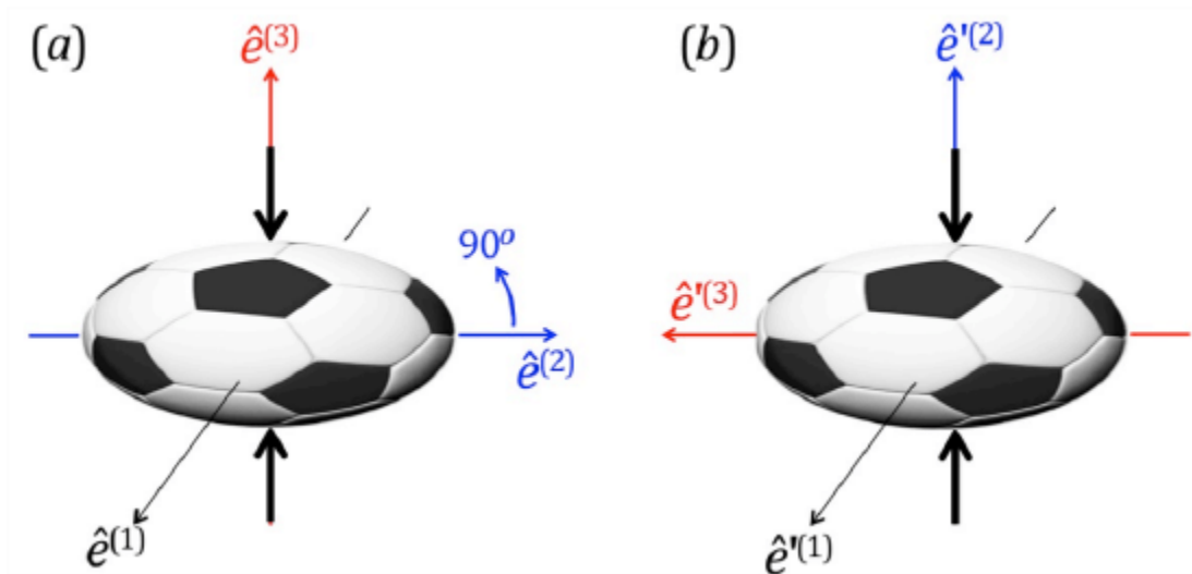
Figure 3.3.1: Somebody stepped on a soccer ball. (a) original coordinate system; (b) rotated coordinate system. The rotation is the one shown in figure 3.1.6, with \phi = 90^\circ .
