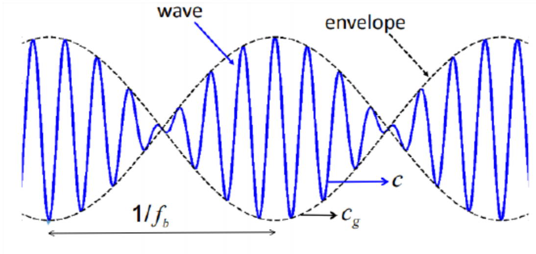
Figure 8.3.1: Two oscillations summed such that every seventh wave is especially large. The dashed curve shows the envelope function. Arrows indicate the phase velocity c , the group velocity c_g and the beat period 1/f_b .
