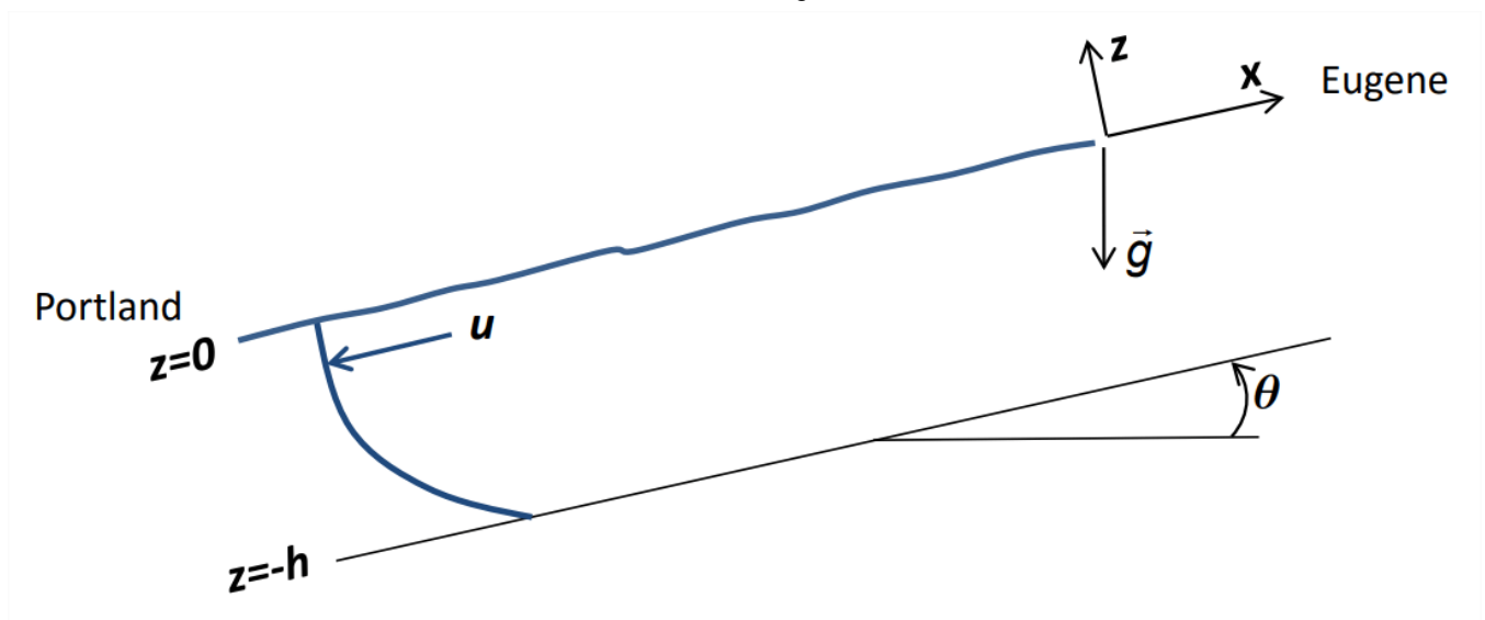
Figure 11.2: Definition sketch for the Willamette River, which flows northward between Eugene and Portland, Oregon.
