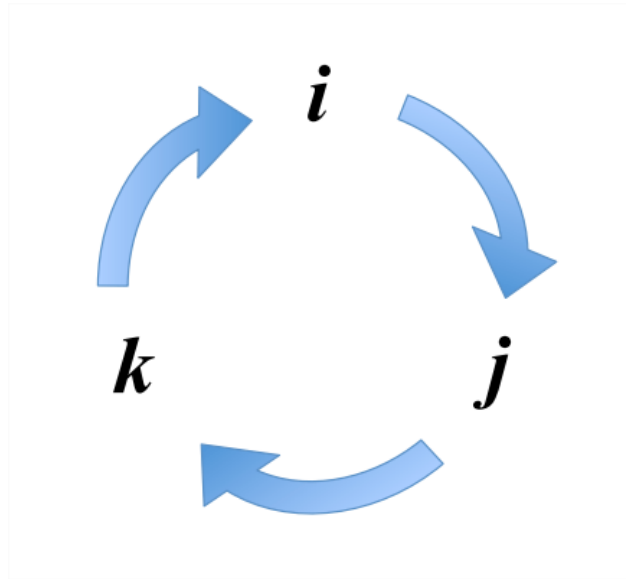
Figure 3.3.3: Cyclic permutations of the indices i, j and k .
