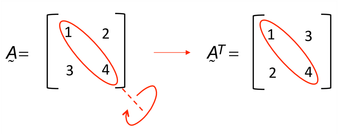
Figure 2.2.1: Taking the transpose of a 2 \times 2 matrix.
