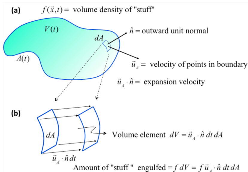
Figure 6.1.1: Definition sketch for Leibniz rule. (a) An arbitrary volume V(t) enclosed by the closed surface A(t) . (b) A small volume engulfed as the surface element dA evolves over a brief time interval dt .
