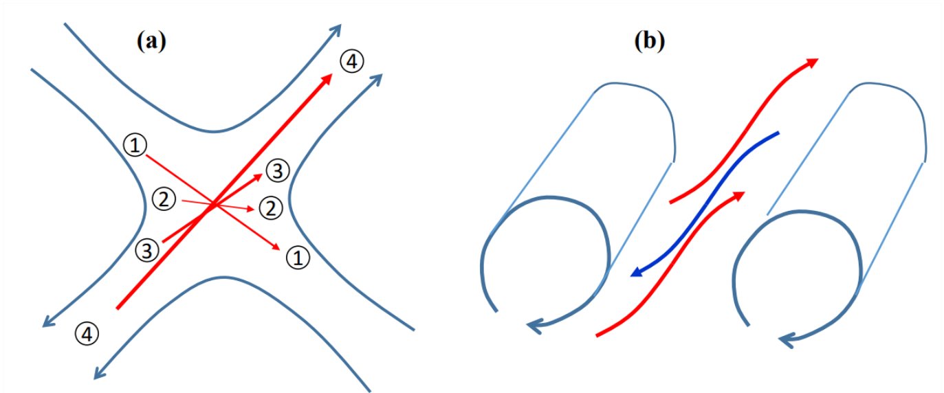
Figure 7.2.3: (a) A vorticity element (red) being tilted and stretched in a steady strain field (blue). Numerals indicate the direction of time. (b) Counterrotating secondary vortices amplified by stretching in the extensional strain between corotating primary vortices.
