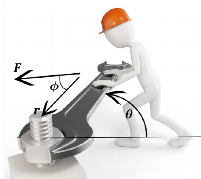
Figure 13.1.1: Definition sketch for Newton's second law in rotational form. A force F is exerted at a distance r from the axis of rotation, changing the angle \theta .
