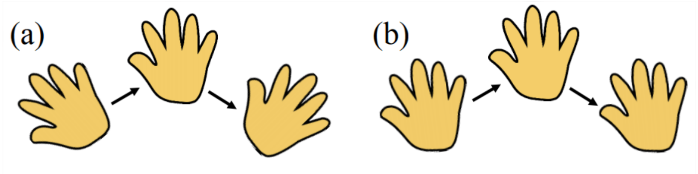
Figure 5.3.7: Waving (a) and wiping (b) motions.
