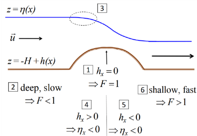
Figure 9.2.3: Steady, large-amplitude flow over an obstacle. Numerals indicate the points described in the text.
