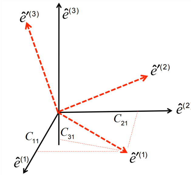
Figure 3.1.5: Original (black, solid) and rotated (red, dashed) Cartesian coordinate systems. Thin dashed lines show the components of \hat{e}'^{(1)} in the original coordinates, which also make up the first column of the rotation matrix \tilde{C} .
