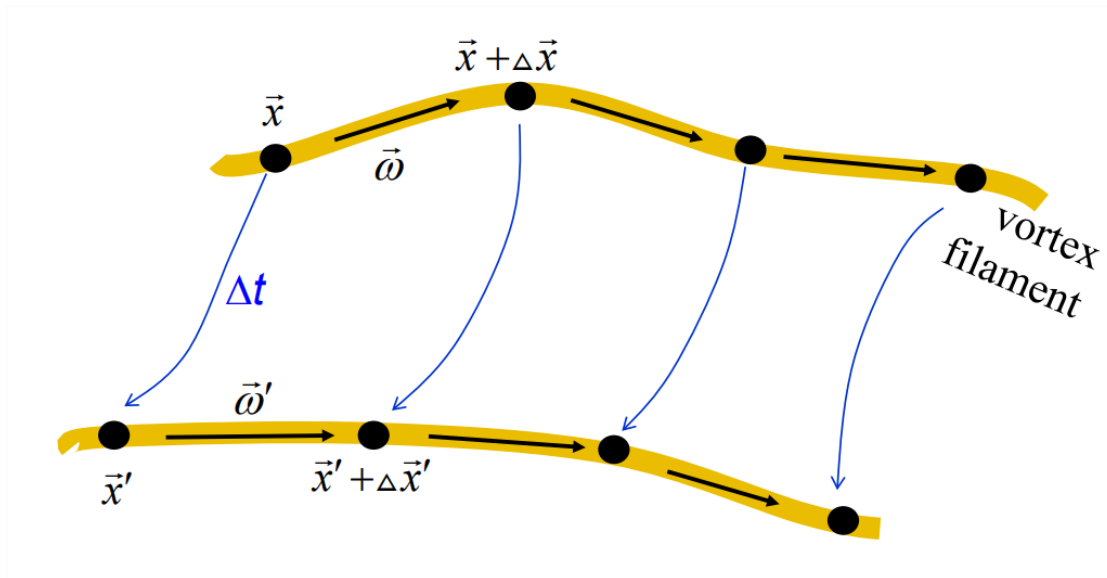
Figure 7.2.2: Motion over a time increment \Delta t of points lying on a vortex filament.
