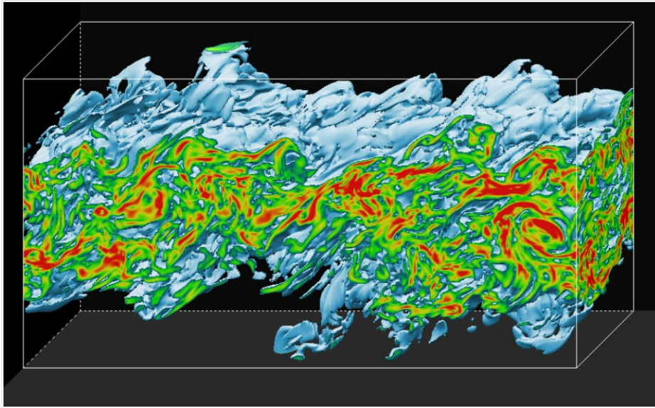
Figure 5.3.5: A snapshot of the strain magnitude e_{ij}^2 at t = 3451 s in the turbulent shear layer shown in Figure 5.3.4. Red indicates regions of intense strain. The lowest values are rendered transparent.
