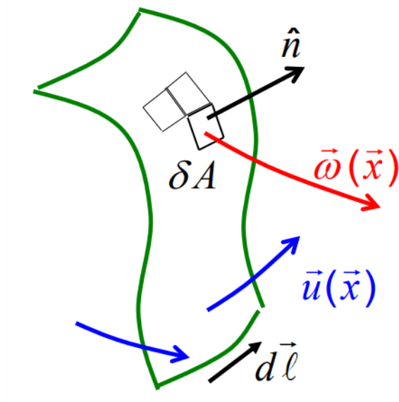
Figure 4.3.3: An arbitrary closed curve, with line element d\vec{\ell} , is embedded in an arbitrary flow field \vec{u}(\vec{x}) with vorticity \vec{\omega}(\vec{x}) . A surface bounded by the curve (but otherwise arbitrary) is approximated by a collection of infinitesimal tiles with area \delta A and unit normal \hat{n} .
