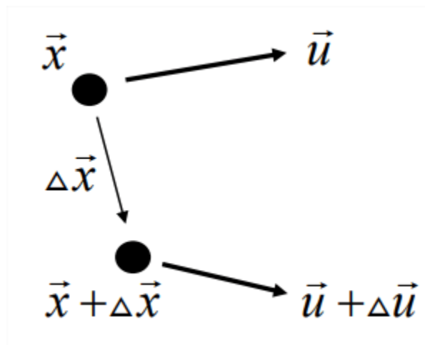
Figure 5.3.2: Relative motion of two nearby fluid particles.
