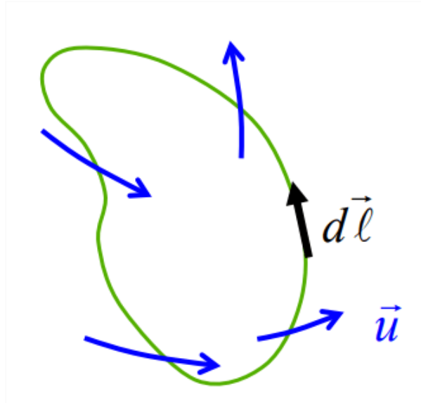
Figure 4.3.1: Definition sketch for the circulation. An arbitrary closed curve, with line element d\vec{\ell} , is embedded in an arbitrary flow field \vec{u}(\vec{x}) .
