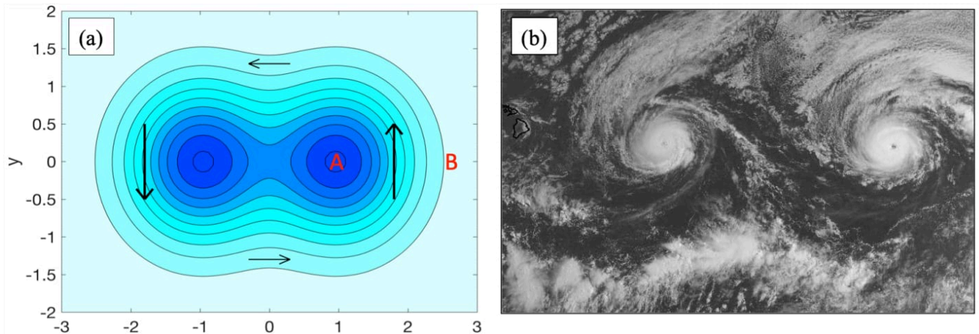
Figure 5.2.1: (a) Streamfunction for a pair of Gaussian vortices located at x = \pm 1 : \psi = -e^{-(x-1)^2-y^2} - e^{-(x+1)^2-y^2} . Blue indicates negative values. The sign of the streamfunction corresponds to positive vorticity (counterclockwise rotation as indicated by arrows). (b) An example in nature: satellite photo of hurricanes Madeline and Lester approaching Hawaii, August 29, 2016 (NASA Earth Observatory).
