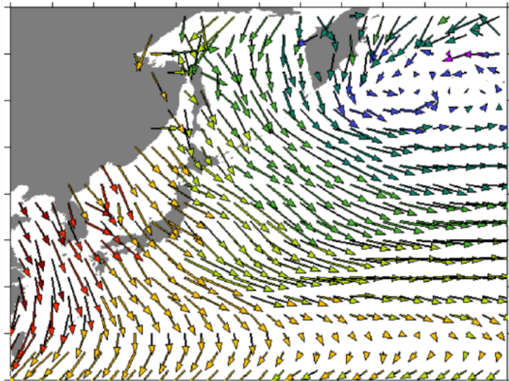
Figure 4.1: Vector field representation of the wind over the northwest Pacific ocean. The curl of this vector field is a dominant influence on ocean currents. Its divergence can tell us about vertical motion and precipitation (Ansley Manke, NOAA).
