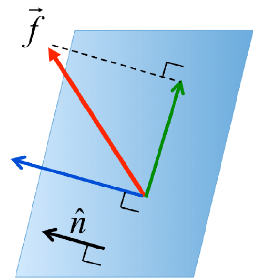
Figure 6.3.2: Stress vector at a surface, with unit normal \hat{n} , resolved into normal (blue) and tangential (green) components.
