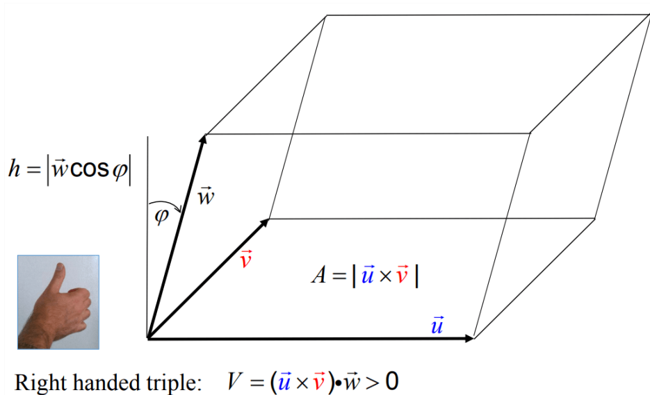
Figure 15.2.1: Relation of the triple product to the volume of the parallelepiped bounded by three vectors \vec{u} , \vec{v} and \vec{w} .
