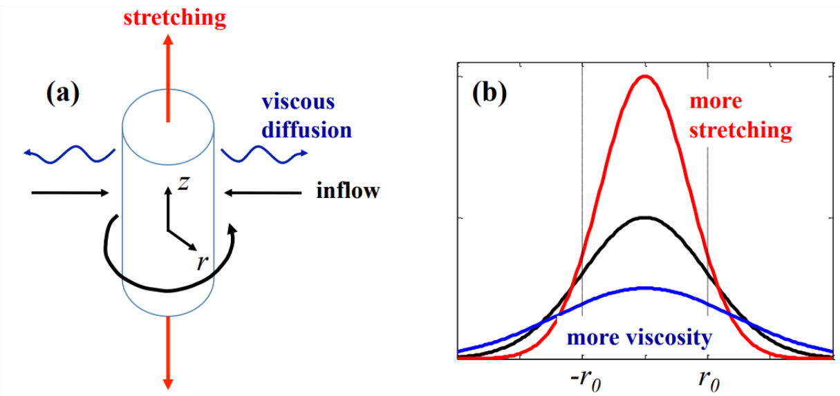
Figure 7.3.1: (a) An axisymmetric vortex tube maintained by a balance of stretching and diffusion. (b) The black curve is a vorticity profile for Burgers vortex 7.3.10. For the red (blue) curve, the circulation is the same but \lambda(v) is doubled.
