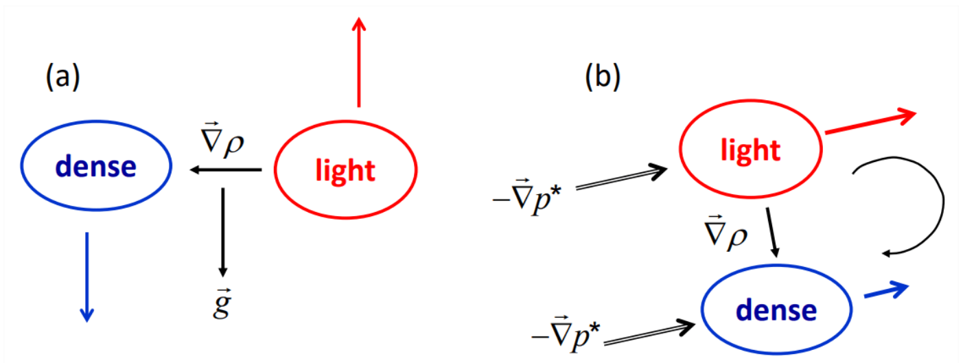
Figure 7.4.1: Schematics illustrating the two parts of the baroclinic torque via their action on two fluid parcels of different density: (a) buoyancy, (b) inertia.
