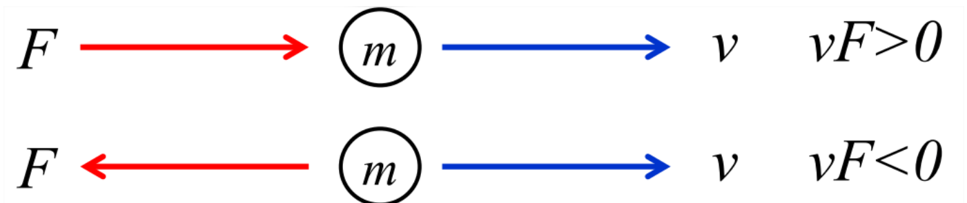
Figure 6.4.1: Schematic of the rate of working by a force on a solid object.
