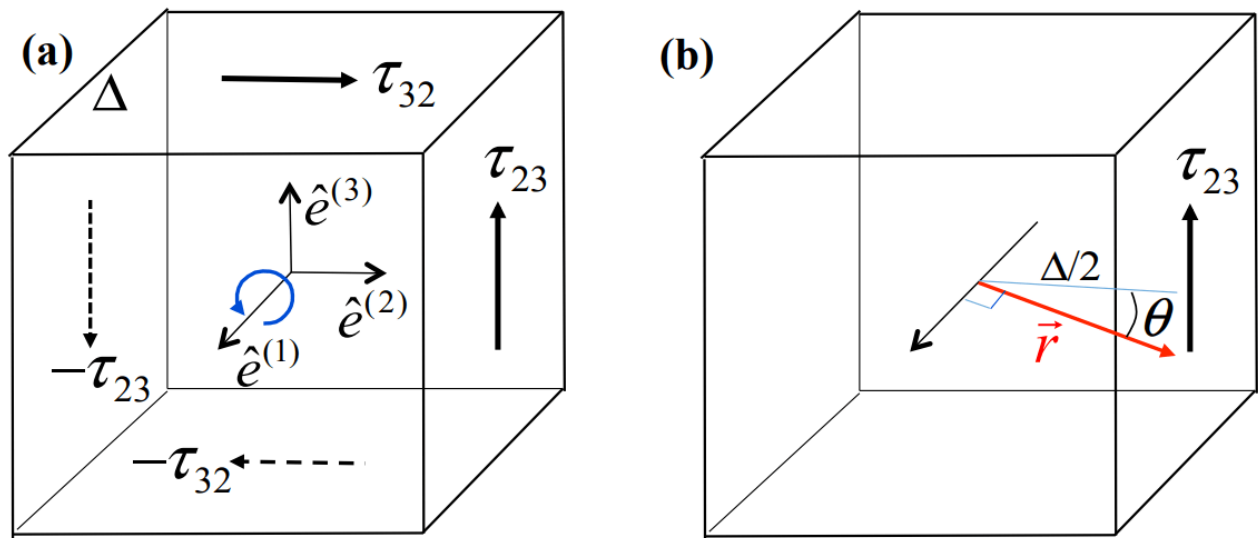
Figure 17.3.2: Torques about the \hat{e}^{(1)} axis on a cube with side \Delta . (a) Tangential stresses. (b) The moment arm.
