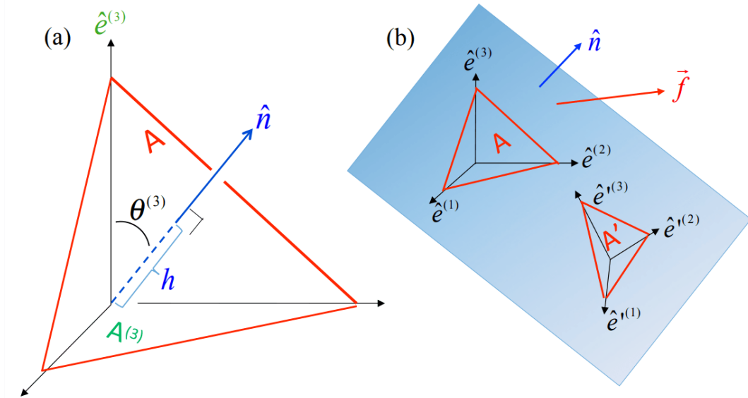
Figure 17.2.2: (a) Geometry of a tetrahedron, showing the outward unit normal to the hypotenuse \hat{n} , the perpendicular distance h , and the angle \theta from \hat{e}^{(3)} . The area A^{(3)} = A \cos \theta^{(3)} , and the volume is Ah/3 . (b) Tetrahedra formed by the same plane (with unit normal \hat{n} and stress vector \vec{f} ) intersecting two different sets of Cartesian axes. The derivation of Equation 17.2.5 works in either case, demonstrating that \tau_{ij} is a tensor.
