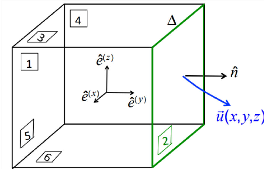
Figure 4.2.3: Definition sketch for the volume flux through a cube.
