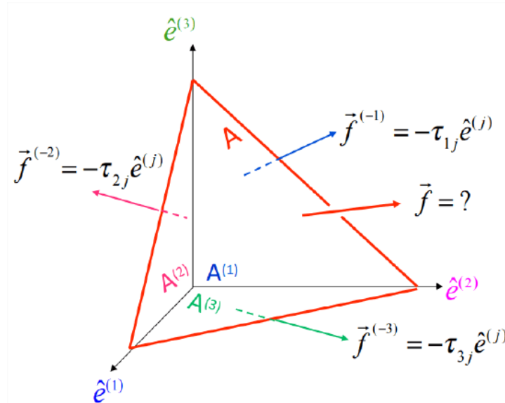
Figure 17.2.1: Stresses on the faces of a tetrahedron. Colors indicate the area of each face and the stress vector acting upon it.
