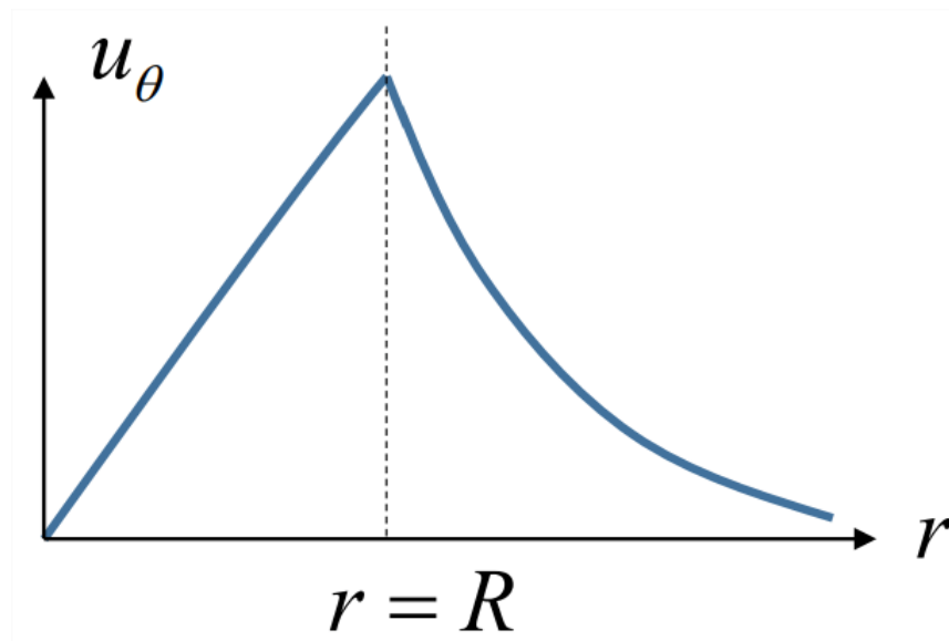
Figure 5.3.8: Azimuthal velocity in the Rankine vortex.
