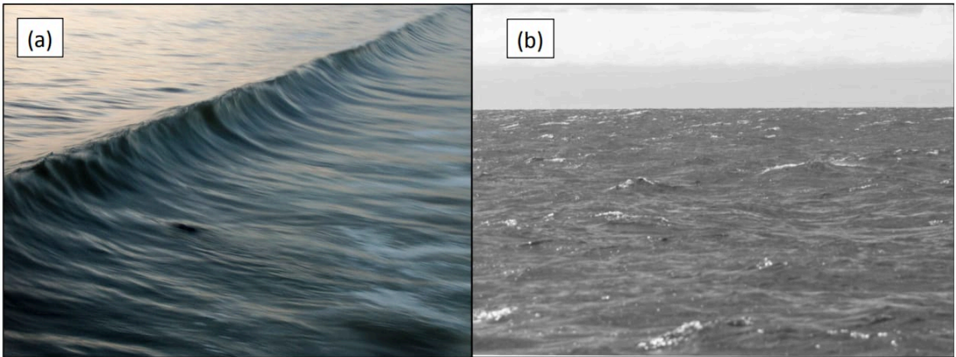
Figure 8.4.1: (a) The sport of surfing is possible because shallow-water waves can maintain a consistent shape, at least briefly. Photo by Barry Tuck. (b) Deep-water waves tend to be choppy and inconsistent, with random orientation and wavelength. Photo by Aurelie Moulin. Details on page iii.
