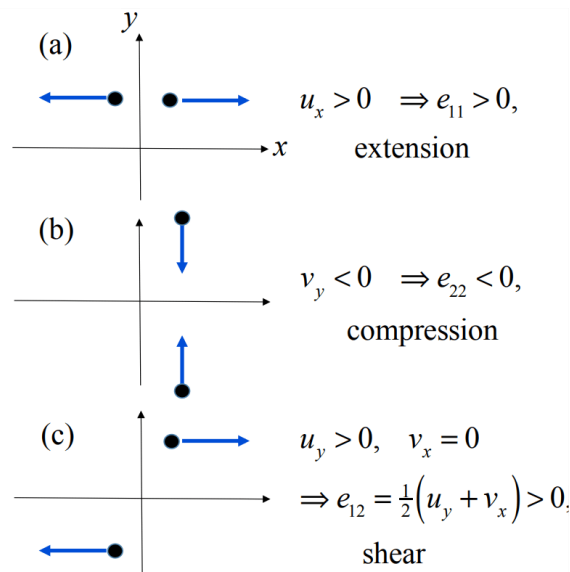
Figure 5.3.10: Pairs of particles in relative motion on the x - y plane, illustrating the types of strain.
