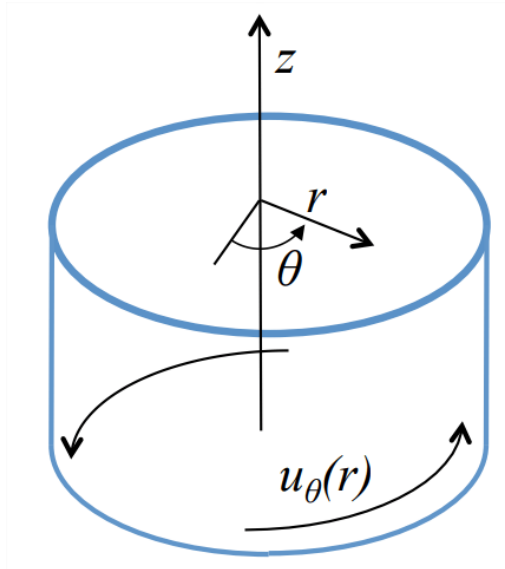
Figure 5.3.6: Axisymmetric (circular) vortex with cylindrical coordinates.
