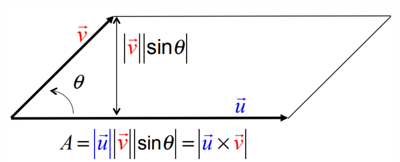
Figure 3.3.4: The area of the parallelogram bounded by two vectors \vec{u} and \vec{v} is the magnitude of their cross product.
