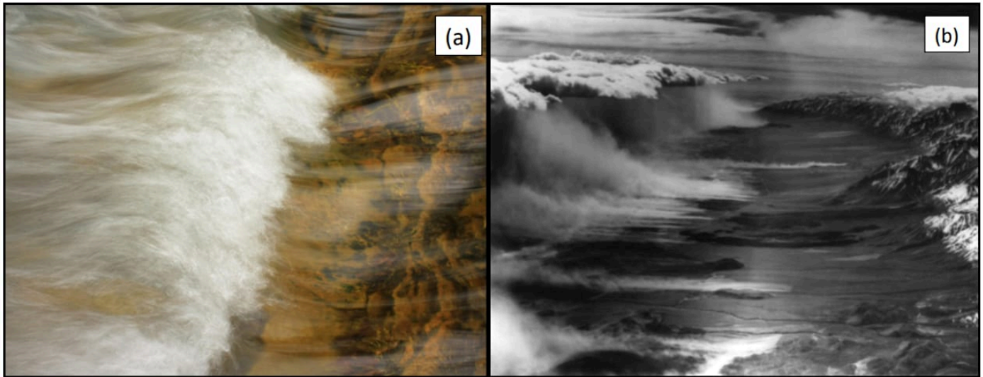
Figure 9.1.1: (a) River flow over an obstruction. Photo by Jonathan Ball. (b) “The Bishop Wave”, a storm on the downwind slope of the Sierra Nevada mountain range. Wind is from right to left; clouds and dust at left indicate rapidly rising, turbulent air. Note the similarity to (a). (Photo by Robert Symons, 5 March 1950.) Further details are on page iii.
