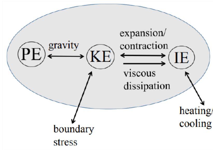
Figure 6.4.2: The energy associated with a fluid parcel is partitioned into three reservoirs: kinetic (KE), potential (PE) and internal (IE). Arrows show the various processes that mediate exchanges of energy between the reservoirs and between the parcel and its environment. These are described mathematically by Equations 6.4.13, 6.4.14, and 6.4.15.
