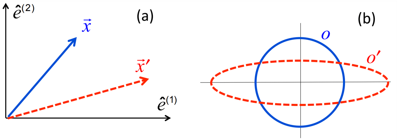
Figure 3.1.2: Transformation by the matrix Equation 3.1.5. (a) Transformation of an arbitrary vector. (b) Transformation of a unit circle.
