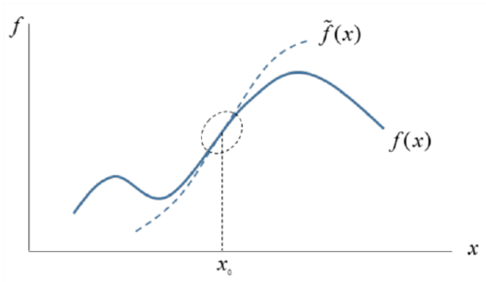
Figure 12.1: Definition sketch for Taylor series expansions. The original function f(x) is approximated by \tilde{f}(x) . The approximation is accurate near the expansion point x_0 .
