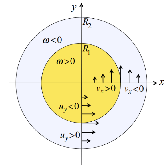
Figure 5.3.9: Vortex with a velocity maximum at r = R_1 and velocity dropping to zero by r = R_2 . Vorticity \omega = v_x - u_y (where subscripts denote partial derivatives) is positive in the inner region and negative in the outer ring.
