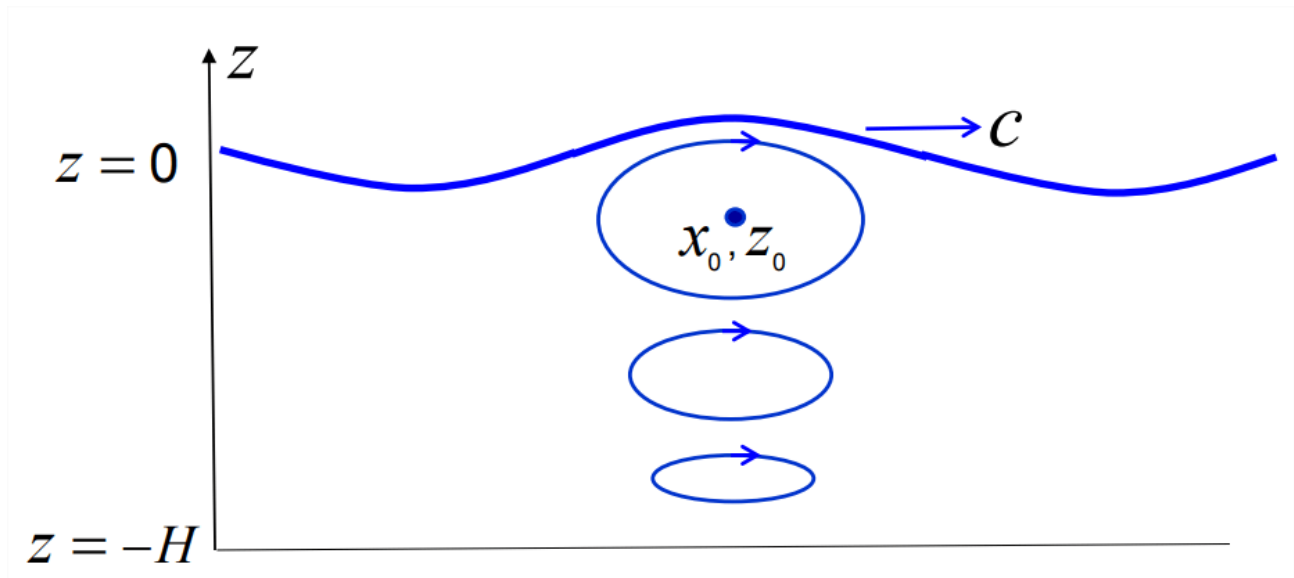
Figure 8.2.3: Elliptical particle trajectories under a small-amplitude surface wave propagating to the right with phase velocity c .
