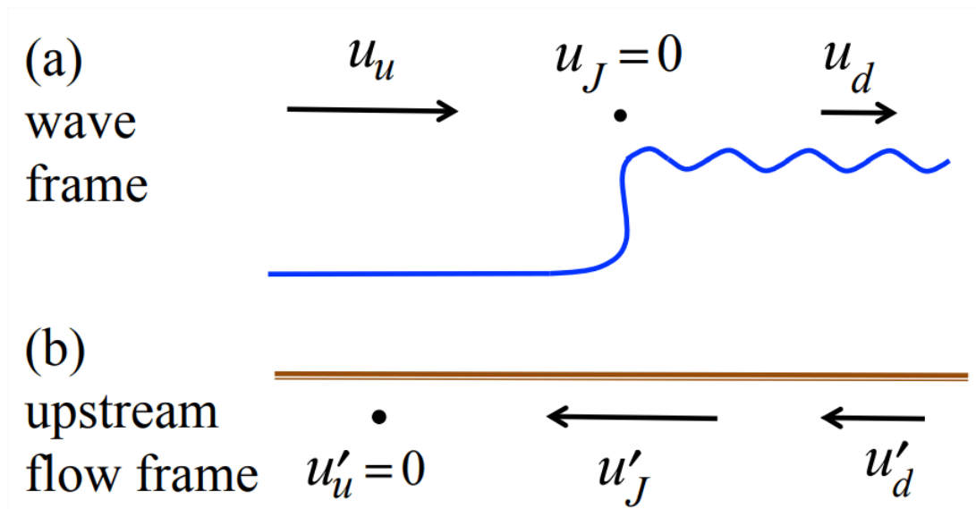
Figure 9.3.4: Definition sketch for velocities in (a) a stationary hydraulic jump (upper) and (b) a bore moving into still water (lower). The wave is the same; the only difference is the reference frame. The velocities u_u and u_d are given by Equation 9.3.9 and Equation 9.3.8.
