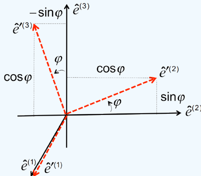
Figure 3.1.6: Original (black, solid) and rotated (red, dashed) basis vectors after a rotation by an angle \phi about \hat{e}^{(x)} . Dashed lines show the components of the rotated basis vectors in the original coordinates.
