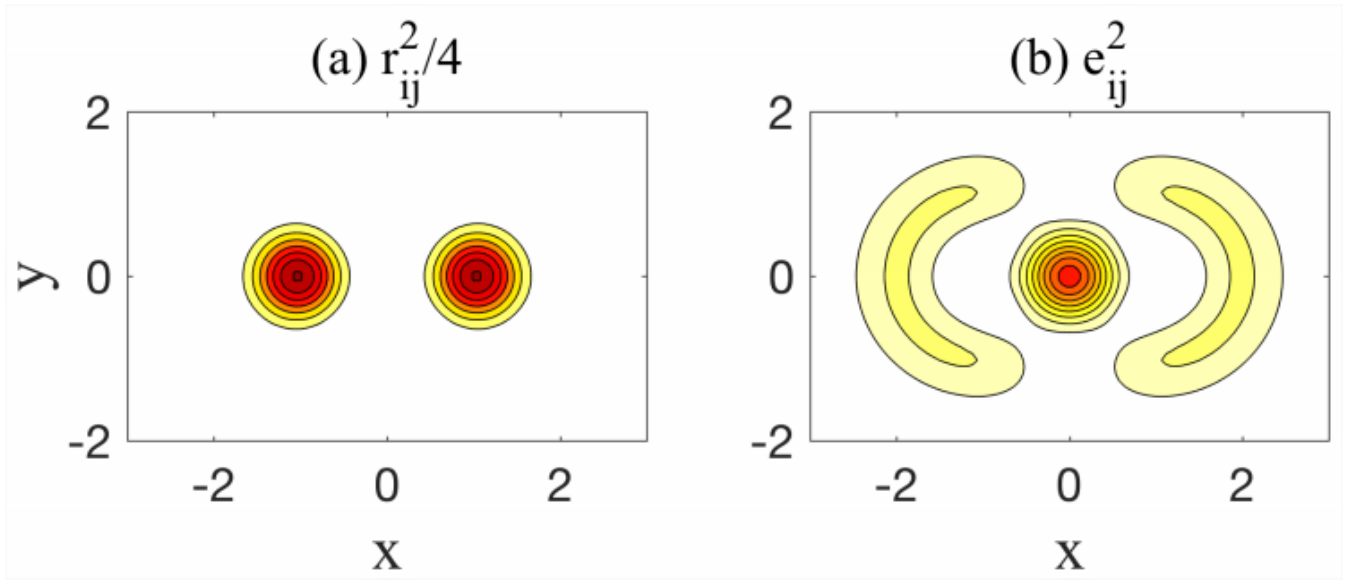
Figure 5.3.3: Strain and rotation magnitudes for the pair of two-dimensional, co-rotating Gaussian vortices shown in (Figure 5.2.1). Note that this flow geometry is also qualitatively similar to that sketched in (Figure 5.3.1). (a) the rotation magnitude \frac{1}{4}r_{ij}^2 , (b) the strain magnitude e_{ij}^2 .
