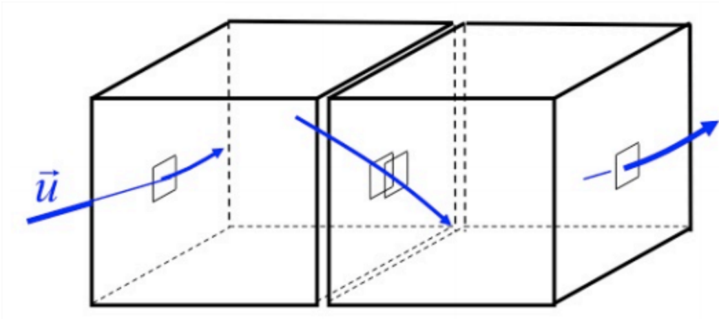
Figure 4.2.4: Volume flux through two cubes, showing that fluxes through adjacent interior surfaces cancel.
