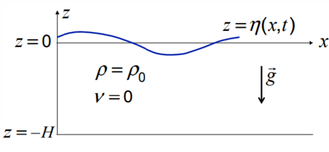
Figure 8.2.1: Two-dimensional flow in an inviscid, homogeneous fluid with a free surface. The vertical coordinate is directed opposite to gravity (upward). The mean surface is z = 0 and the mean depth is H .
