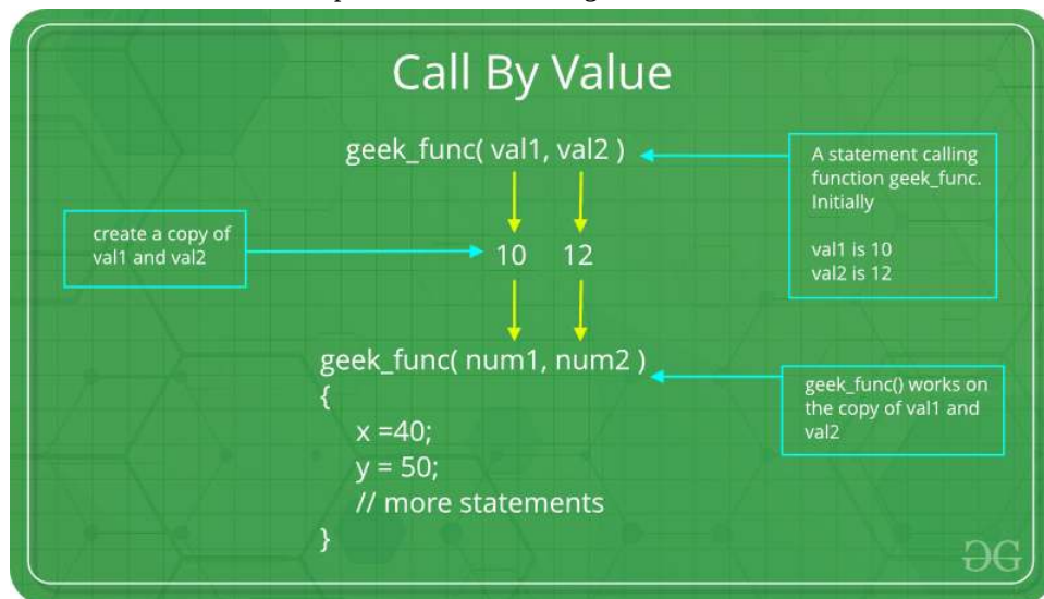
Figure 8.3.1: Call by Value. ("Call by Value" by Geeks for Geeks, Geek for Geeks is licensed under CC BY-SA 4.0 )
