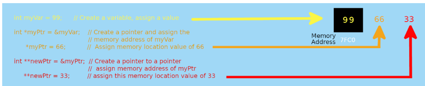
Figure 10.2.1: Copy and Paste Caption here. ("Pointers-in-C++.png" by Patrick McClanahan is in the Public Domain, CC0 )
