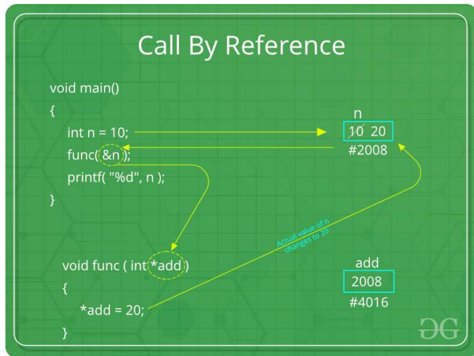
Figure 8.3.1: Pass by Reference. ("Call by Reference" by Geeks for Geeks, Geek for Geeks is licensed under CC BY-SA 4.0 )
