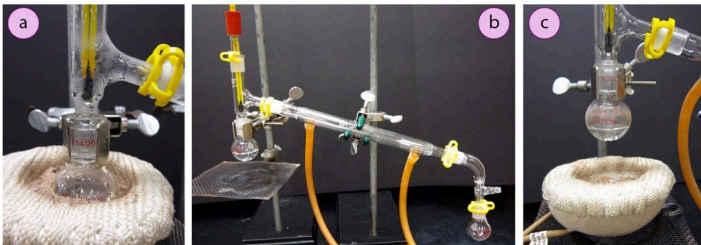
Figure 1.52: a+b) Distillation using a heating mantle, c) Cooling of a flask after heating.
