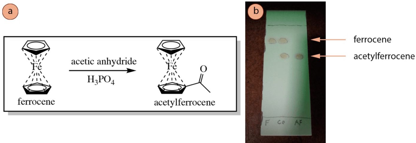
Figure 2.8: a) Reaction scheme of the acetylation of ferrocene, b) TLC plate (visualized with UV light) with 3 lanes: F for pure ferrocene, Co for the co-spot, and AF for the acetylferrocene product.
