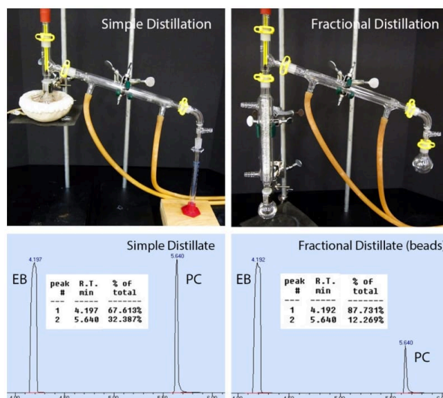
Figure 5.40: Simple and fractional distillation of a 75 mol% ethylbenzene/25 mol% p-cymene mixture, with GC analysis. In each GC spectrum, ethylbenzene is the peak at 4.192 min and p-cymene is the peak at 5.640 min.
