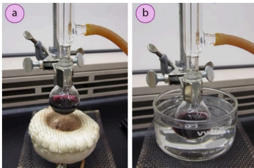
Figure 1.65: a) Raising the flask to cool, b) Cooling quickly in tap water bath.
