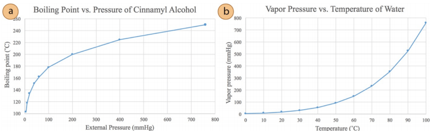
Figure 5.47: a) Graph of boiling point vs. pressure of cinnamyl alcohol, 12 b) Graph of vapor pressure vs. temperature of water. 13
