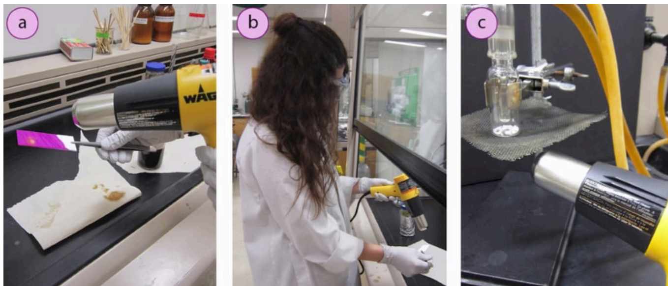
Figure 1.56: a+b) Using a heat gun to develop a TLC plate, c) Using a heat gun for a sublimation.
