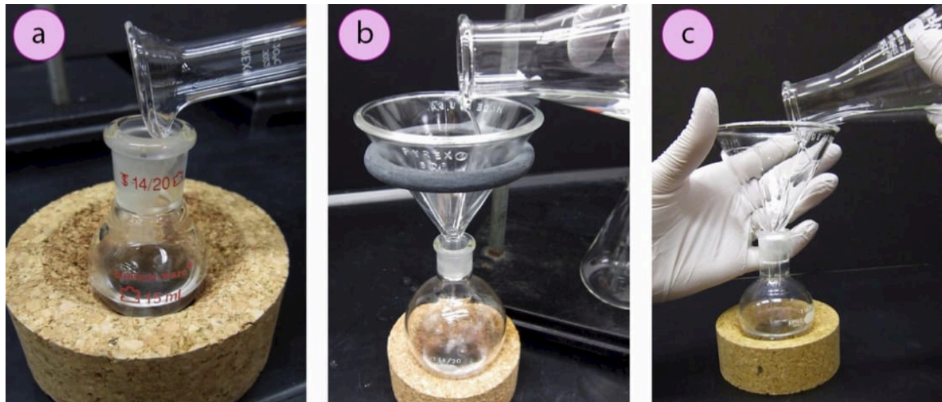
Figure 1.17: a) Pouring liquid, b) Pouring into a funnel held with ring clamp, c) Pouring into a funnel held by hand.
