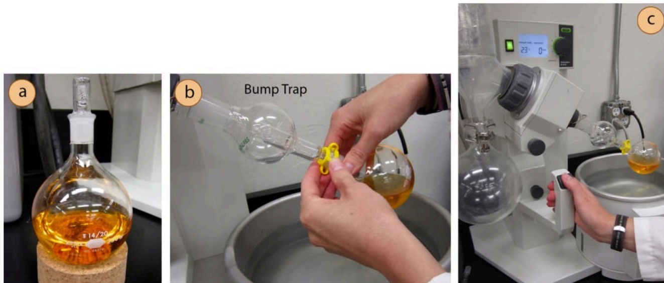
Figure 5.67: a) Sample to be evaporated, b) Attachment of sample to bump trap on rotary evaporator, c) Lowering of sample into water bath.
