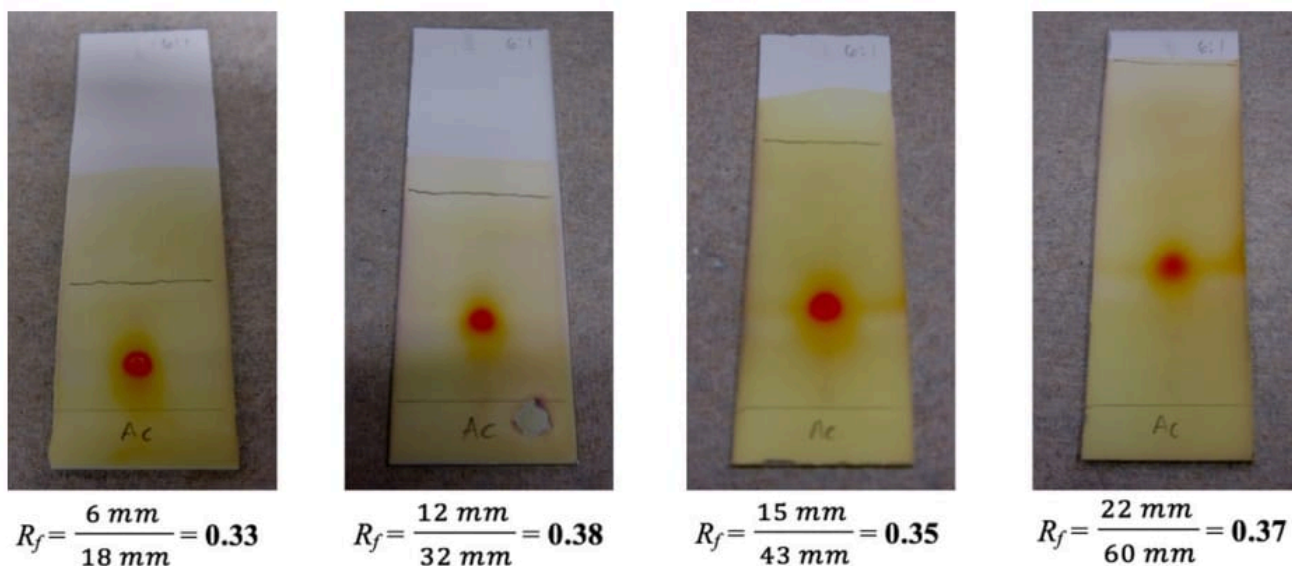
Figure 2.15: Acetophenone run to different heights on the TLC plate, using 6:1 hexanes:ethyl acetate and visualized with anisaldehyde stain.
