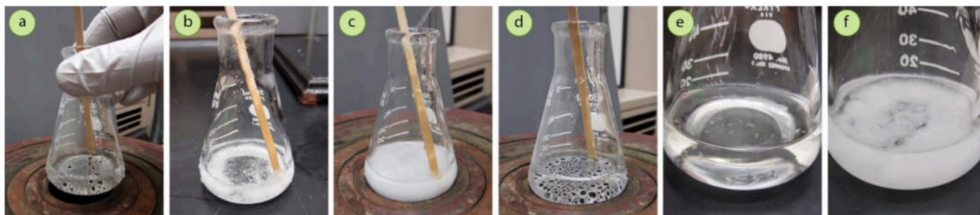
Figure 3.60: a) The minimal amount of methanol/water was used to dissolve a sample of trans -cinnamic acid, b) Upon cooling, the solid immediately crashed out, c) The cloudy solution was placed back on the heat source and extra methanol was added, d) The solid dissolved, e+f) The solid crystallized more slowly when using more solvent.
