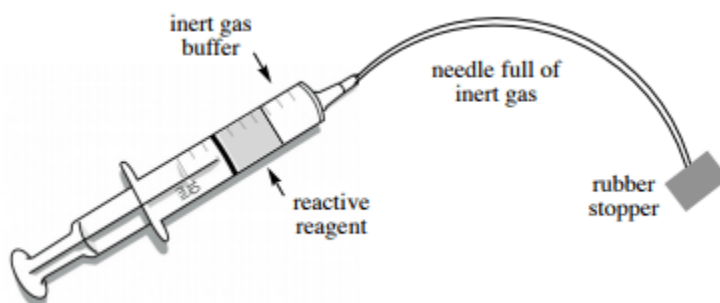
Figure 1.36: Syringe full of air-sensitive reagent ready for transport.
