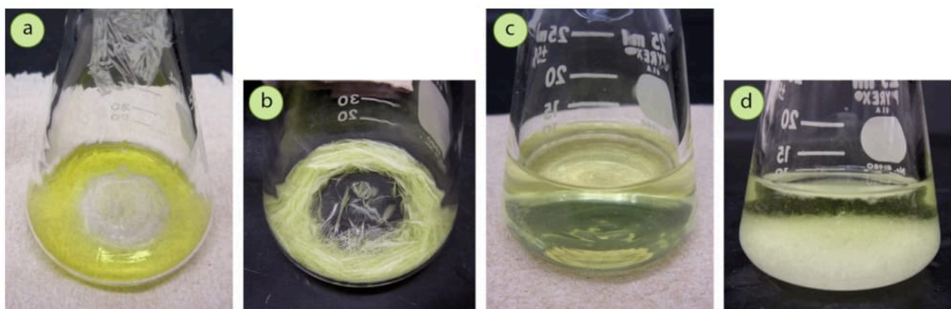
Figure 3.44: a) The flask is too large for the sample, and the solvent is too shallow, b) After crystallization the solvent is completely adsorbed (or evaporated), c) The flask is the correct size for the amount of sample, d) The solvent is an appropriate height in the flask.
