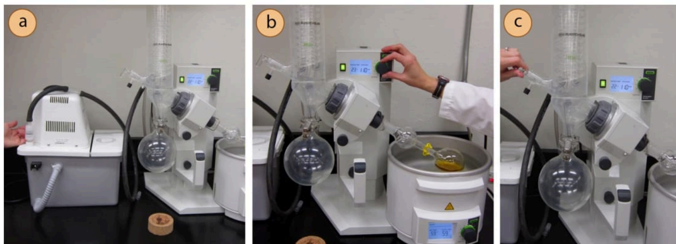
Figure 5.69: a) Turning on the water aspirator, b) Adjustment of the flask's rotation, c) Closing the stopcock to further reduce the pressure.
