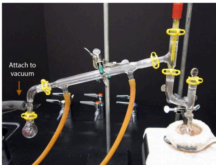
Figure 5.48: Vacuum distillation variation with a simple distillation.
