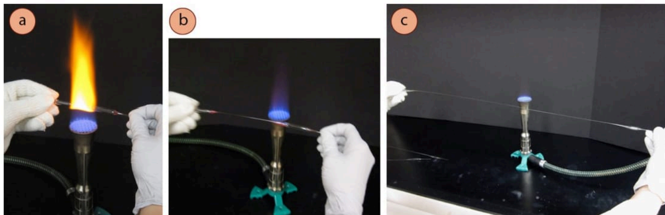
Figure 2.28: a) Warming a pipette in a Meker burner, b+c) Stretching the pipette.
