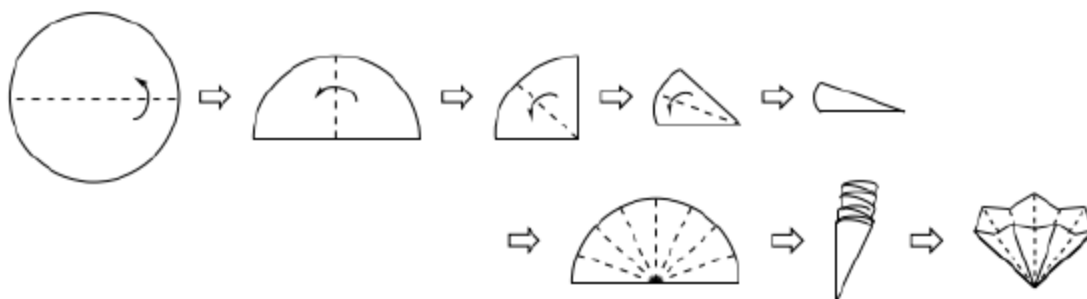
Figure 1.86: Creating a fluted filter paper. The dotted lines represent locations to crease and fold the filter paper. The arrows show the direction of folding.
