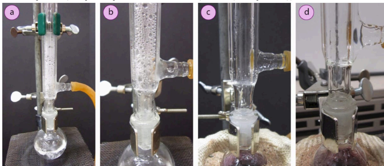
Figure 1.64: a+b) Condensation seen in the condenser when refluxing water, c) Reflux ring of ethanol seen subtly in the bottom third of the condenser, d) Distortion of the ring stand in the condenser due to the refluxing ethanol solution.
