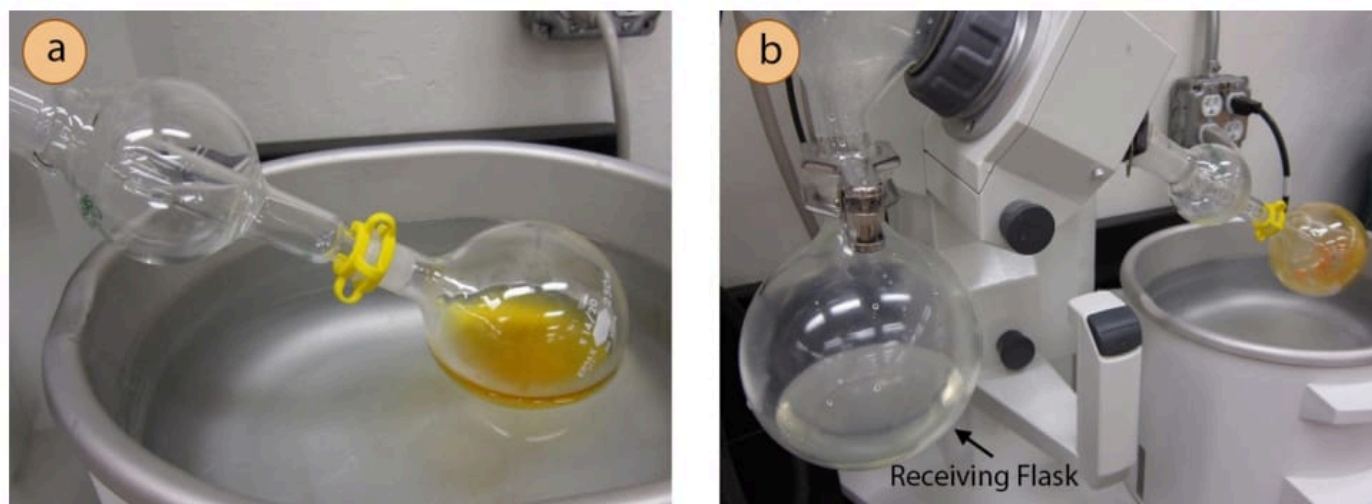
Figure 5.66: a) Solution is placed on a rotary evaporator, b) After evaporation (solvent is in the receiving flask).
