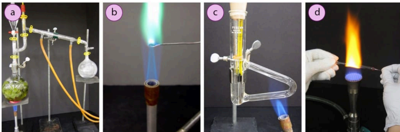
Figure 1.44: Uses of Bunsen burners in: a) Steam distillation, b) Beilstein test, c) Thiele tube, d) Softening pipettes.
