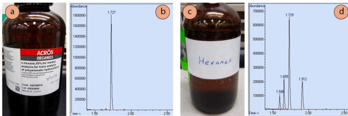
Figure 2.77: a) Bottle of n -hexane, b) GC spectrum of n -hexane, c) Bottle of "hexanes", d) GC spectrum of "hexanes". The compounds present in hexanes are: 2-methylpentane, 3-methylpentane, n -hexane, and methylcyclopentane (in order of elution). 13
