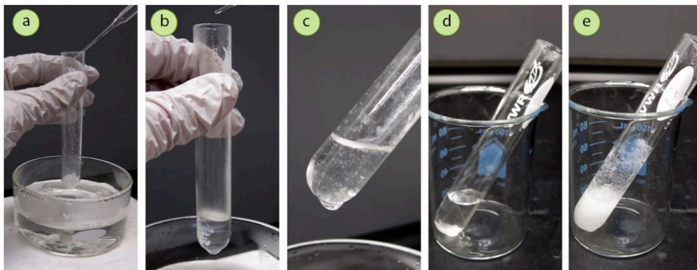
Figure 3.15: a) Addition of methanol (soluble solvent) to trans-cinnamic acid, b) Addition of water (insoluble solvent) to the solution, c) Sustained cloudiness/fine crystals after enough water was added, d) Tube set aside to cool after a few drops of methanol were added to clarify the solution, e) The return of crystals after cooling.
