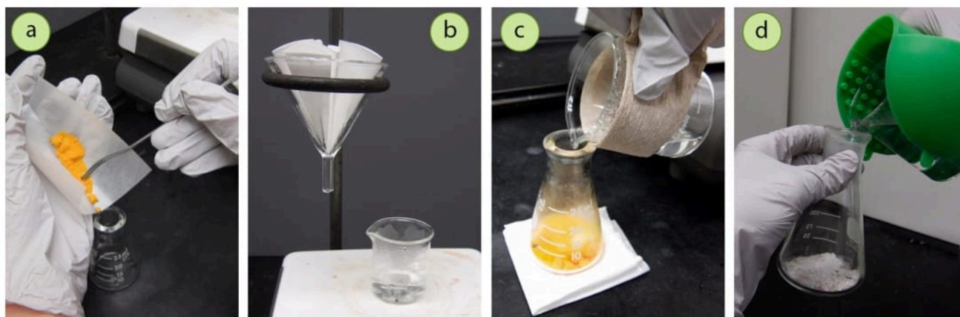
Figure 3.50: a) Impure NBS added to the flask, b) Heating water on a hotplate, c) Addition of hot water to the solid, using a paper towel holder to hold the beaker, d) Addition of hot water to the solid (not NBS, a different system) using a silicone hot hand protector.
