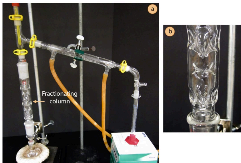
Figure 5.37: a) Fractional distillation setup, b) Zoom in of fractionating column during distillation, with condensation dripping from the glass indentations.
