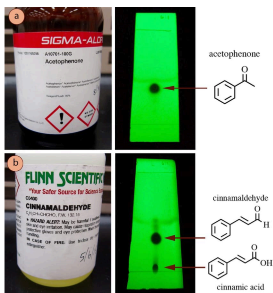
Figure 2.7: Eluted TLC plates visualized with UV light of: a) Acetophenone, b) Cinnamaldehyde.
