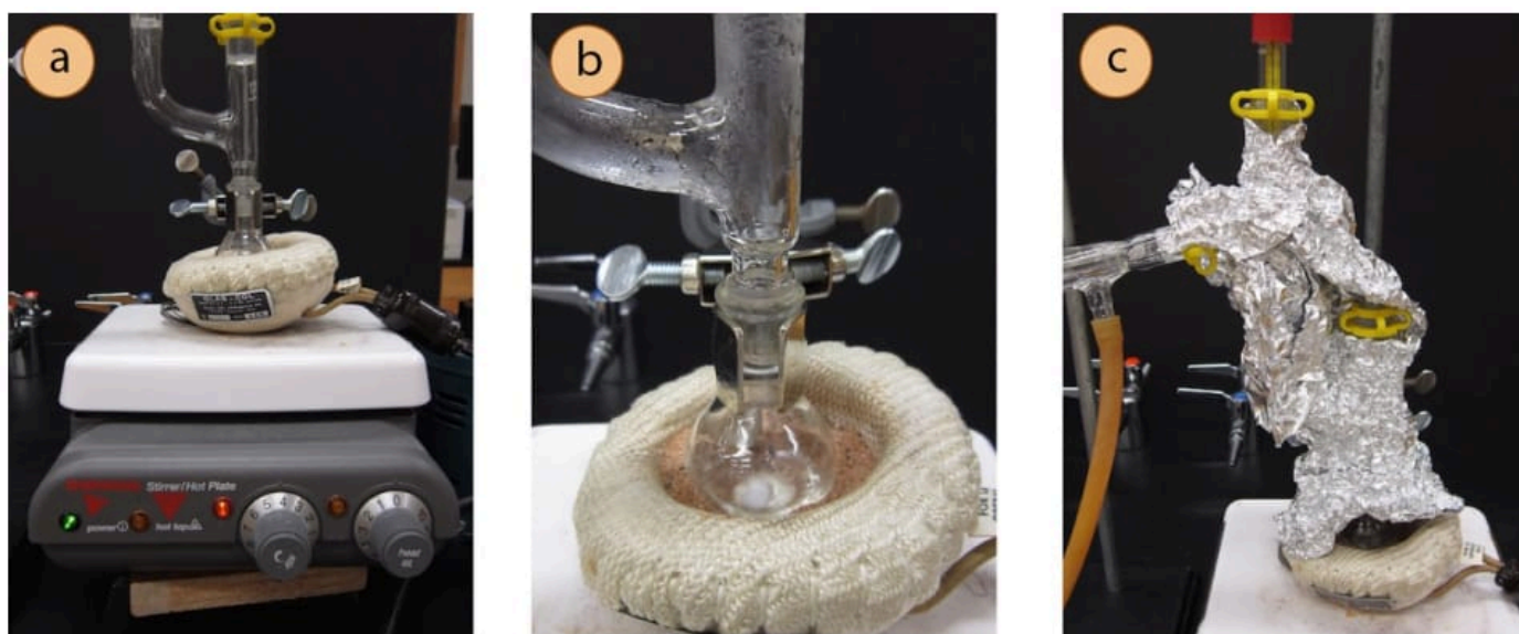
Figure 5.52: a) Stir plate with wood block to allow for lowering of the apparatus, b) Active distillation, c) Insulating the Claisen and three-way adapters with foil.
