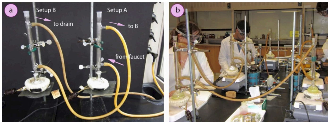
Figure 1.62: Connecting reflux condensers in series.
