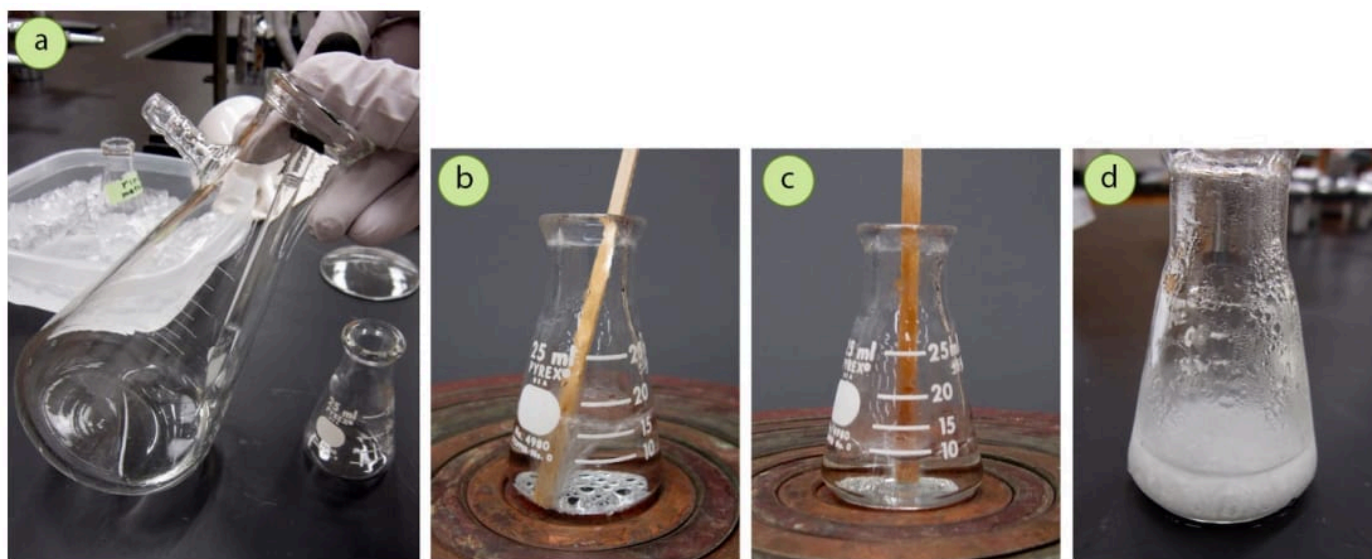
Figure 3.32: Crystallization of a "second crop" of trans -cinnamic acid from water and methanol.
