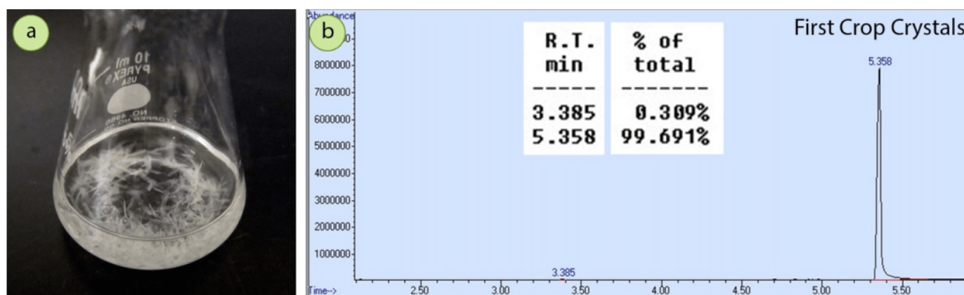
Figure 3.35: a) First crop of 4-bromoacetophenone crystals coming out of solution, b) GC spectrum of the crystallized mixture.
