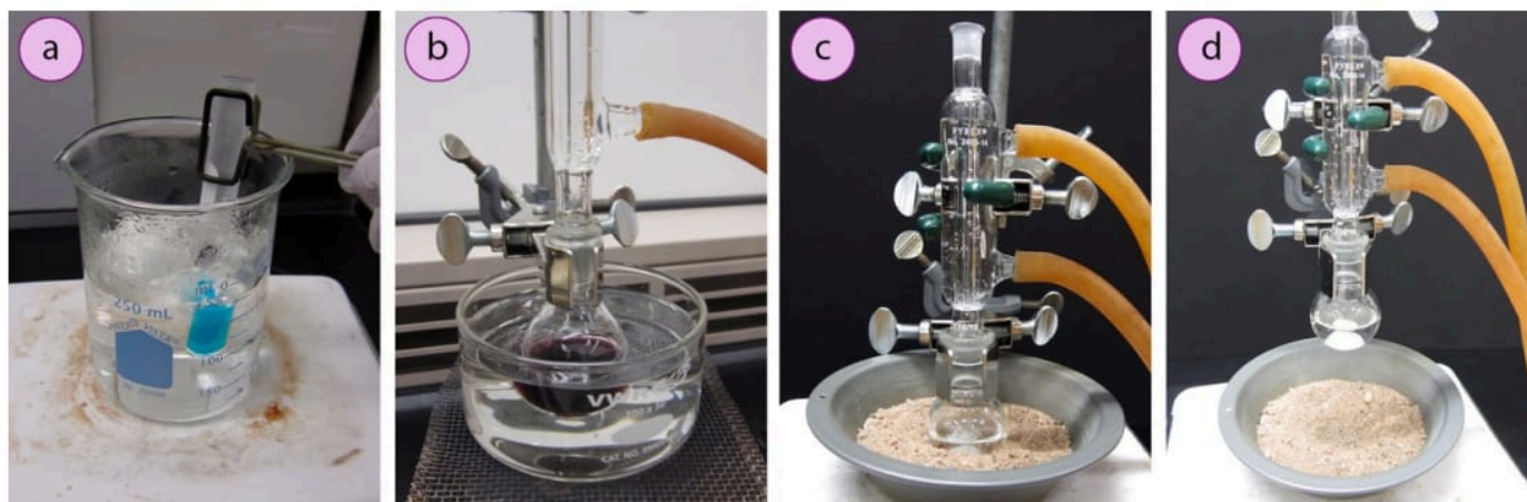
Figure 1.54: a) Boiling water bath, b) Water bath to cool an apparatus, c) Heating a flask with a sand bath, d) Allowing a flask to cool.
