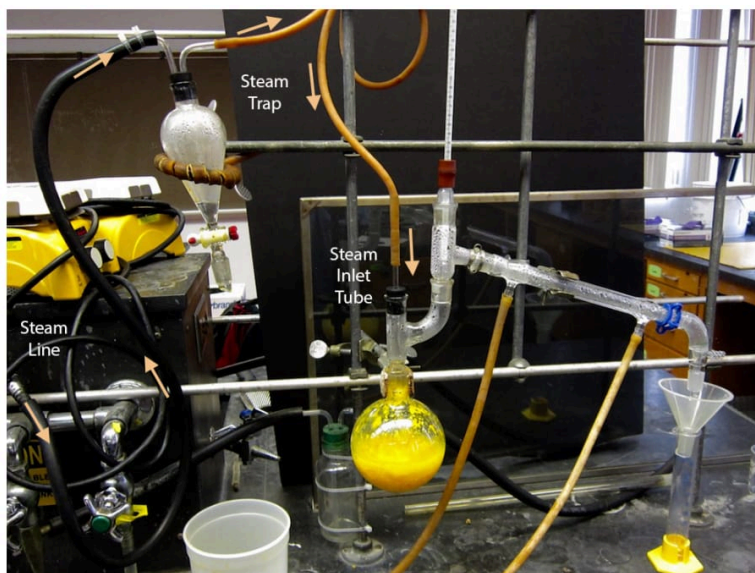
Figure 7.12: Steam distillation apparatus.
