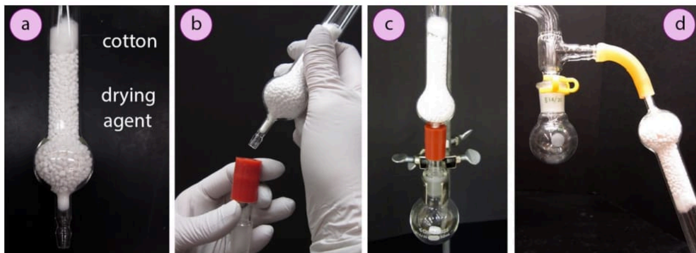
Figure 1.13: a) Drying tube with anhydrous \text{CaCl}_2 , b) Inserting drying tube into a thermometer adapter, Drying tube attached to a: c) round bottomed flask, d) distillation apparatus.
