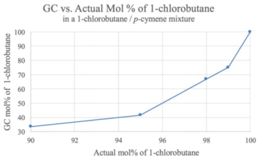
Figure 5.9: Calibration curve for GC analysis of a 1-chlorobutane/ p -cymene mixture.
