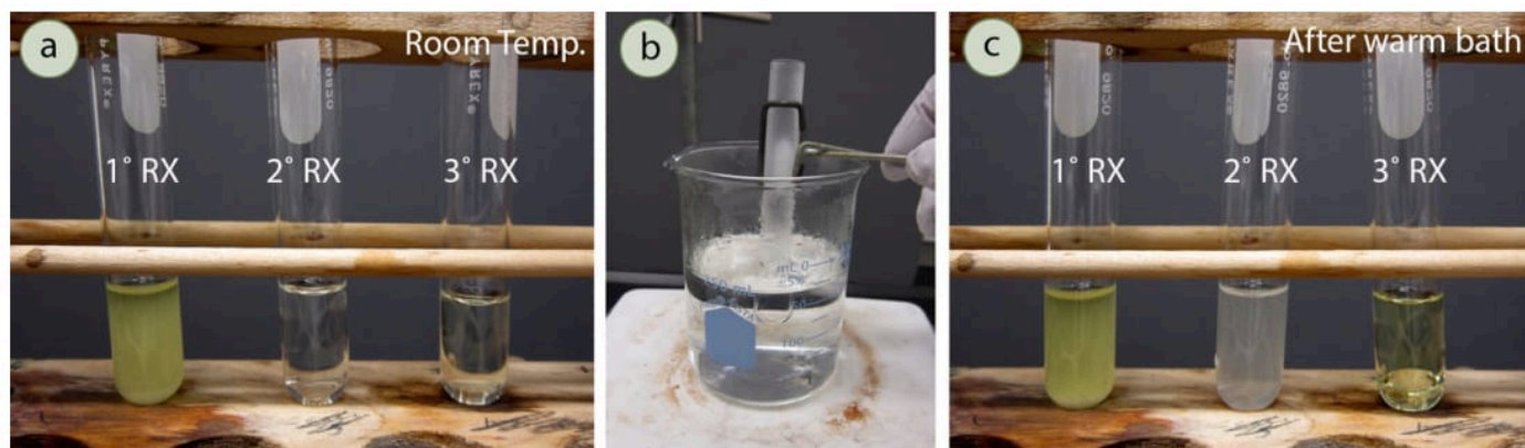
Figure 6.74: Sodium iodide results at room temperature for (left to right), 1-chlorobutane (primary, positive), 2-chlorobutane (secondary, negative), 2-chloro-2-methylpropane (tertiary, negative), b) Heating in a warm water bath, using a thermometer to monitor the temperature, c) Results after the warm water bath, resulting in the clouding of the middle tube (secondary, positive).
