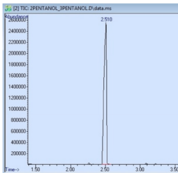
Figure 2.78: GC spectrum of a sample containing 2-pentanol and 3-pentanol. Both compounds are represented by the peak at 2.510 min.
