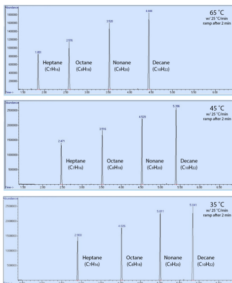
Figure 2.90: GC runs of a mixture containing heptane, octane, nonane, and decane at different oven temperatures. Each run was held at 65°C, 45°C, or 35°C for 2 min, then ramped 25°C/min.
