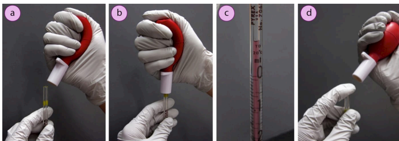
Figure 1.24: a+b) Applying suction to the pipette, c) Liquid withdrawn above the desired volume, d) The bulb is released and tip of the pipette sealed with a finger to maintain the liquid's position.
