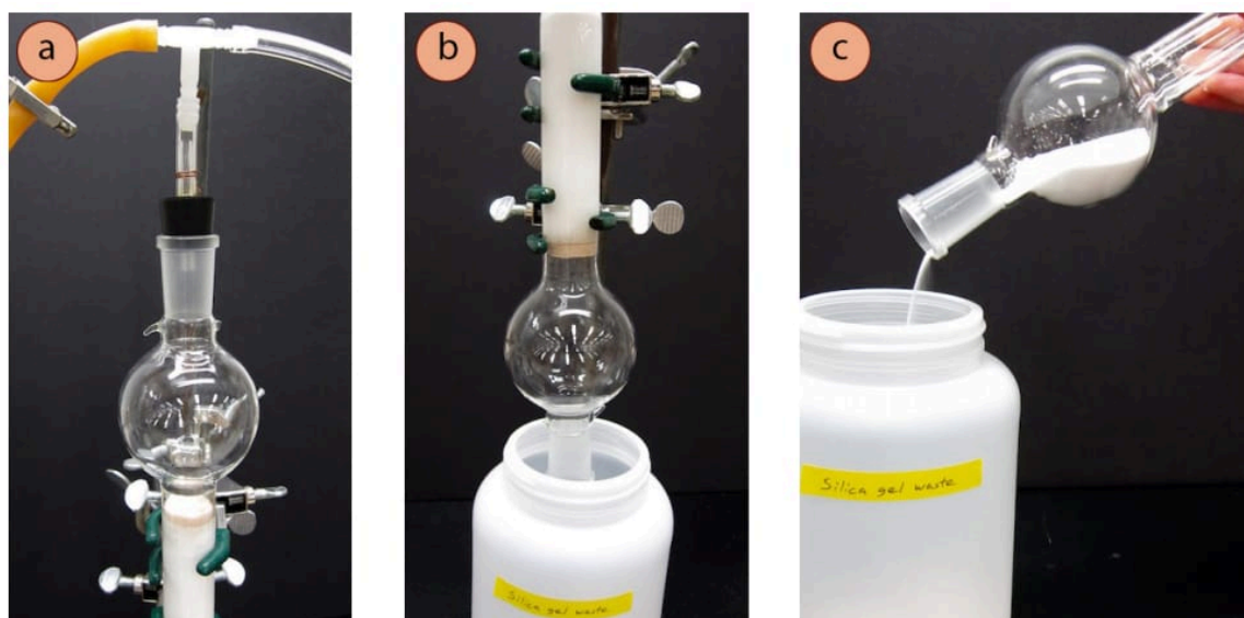
Figure 2.64: a) Using air pressure to dry the column, b) Allowing the column to dry upside-down, c) Collecting the waste silica.
