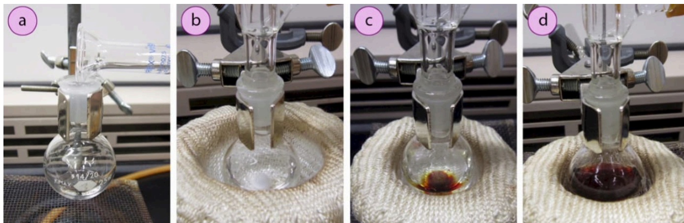
Figure 1.59: a) Pouring in solution, b) Reaction using a stir bar (solution is colorless), c+d) Same reaction using boiling stones.
