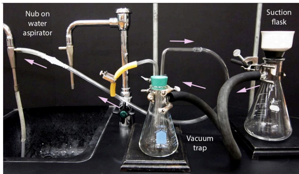
Figure 7.1: Suction filtration vacuum trap apparatus.
