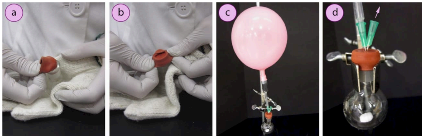
Figure 1.32: a+b) Alternative way to hold a hot flask and attach the rubber septum, c) Flushing a reaction flask with a gas balloon, d) Close-up of the "exit needle."
