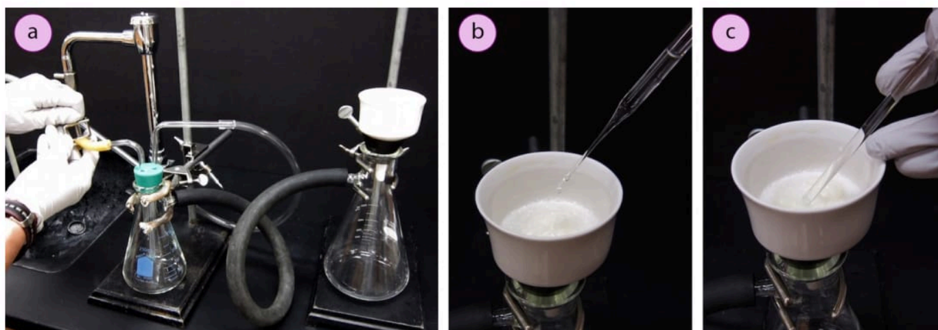
Figure 1.78: a) Breaking the vacuum by opening the pinch clamp on the vacuum trap, b) Adding rinse solvent, c) Breaking up the solid.
