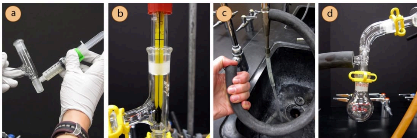
Figure 5.51: a) Applying grease to a joint, b) Adequately greased joint, c) Testing an aspirator's suction, d) Vacuum tubing attached to the vacuum adapter.
