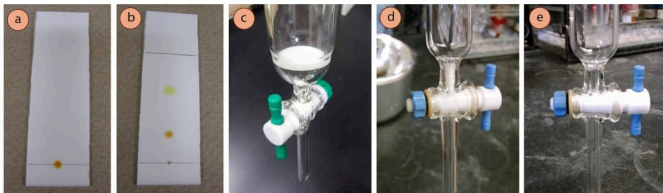
Figure 2.52: a) TLC plate of crude ferrocene/acetylferrocene mixture before elution, b) After elution, c) Column with frit, d) Column with cotton wedged in the bottom, e) Column lacking the cotton wedge (would need to be inserted before use).
