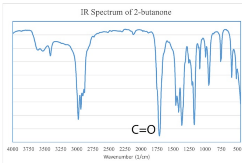
Figure 6.42: IR spectrum of 2-butanone.
