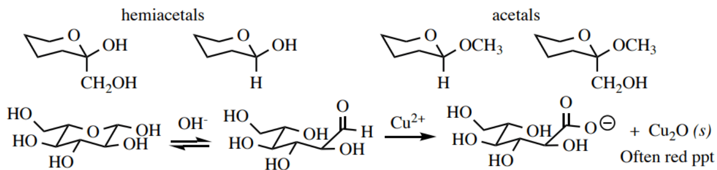
Figure 6.47: Structure of hemiacetals and acetals, along with the reaction of a hemiacetal with the Benedict's reagent.
