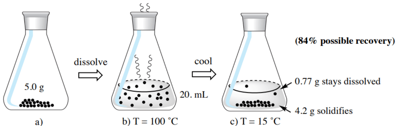
Figure 3.21: Calculations using the minimum amount of hot water to dissolve 5.0 g of 2-furoic acid.
