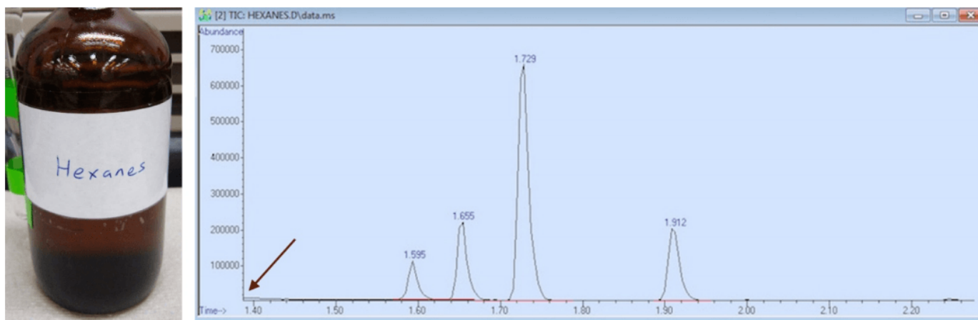
Figure 2.89: GC spectrum of hexanes, with arrow indicating the time the solvent delay is turned off.
