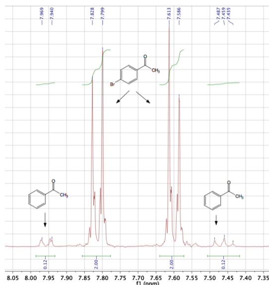
Figure 3.34: Partial 300 MHz ^1\text{H} NMR spectrum of the original mixture of 4-bromoacetophenone and acetophenone (two signals for the methyl groups are at 2.58 and 2.61 ppm). The integrations show a similar composition as the GC data.
