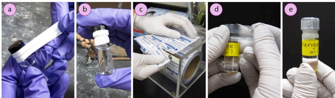
Figure 1.14: a+b) Stretching Teflon tape to seal a joint, c) Removing Parafilm from the roll, d+e) Stretching Parafilm over a joint.
