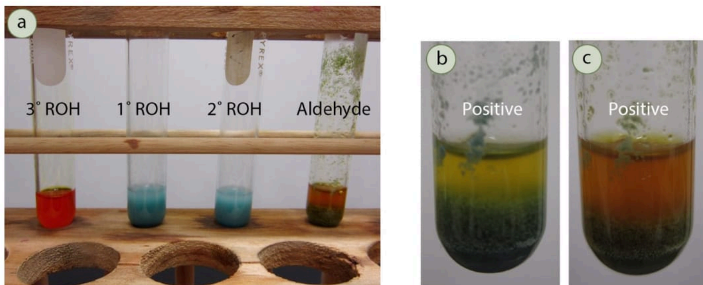
Figure 6.58: a) Chromic acid results (left to right): t-butanol (tertiary, negative), 1-propanol (primary, positive), 2-propanol (secondary, positive), benzaldehyde (positive), b) Immediate reaction of benzaldehyde, c) Benzaldehyde reaction after 1 minute.
