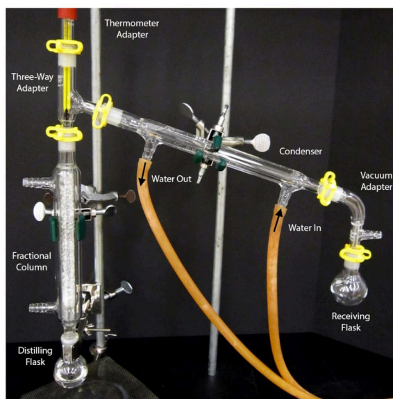
Figure 5.43: Fractional distillation apparatus.
