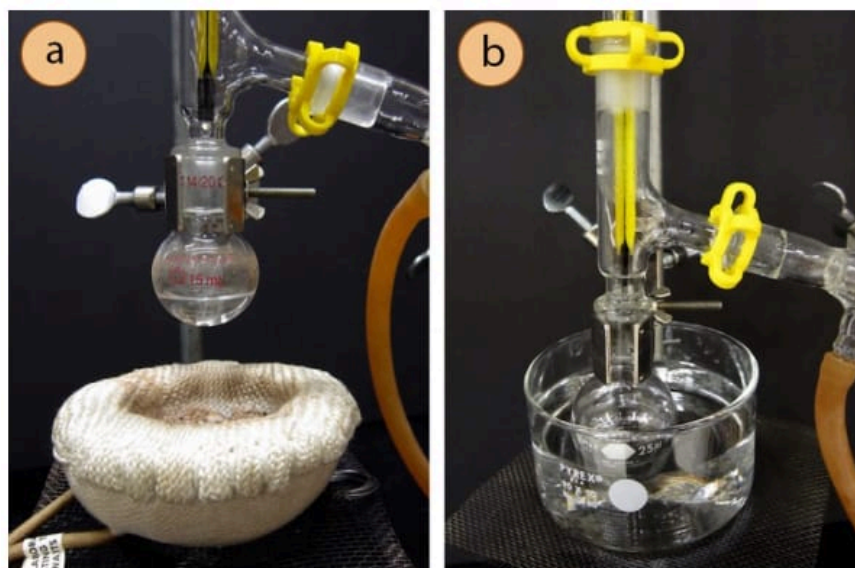
Figure 5.28: a) Raising the flask to cool, b) Cooling in a tap water bath.
