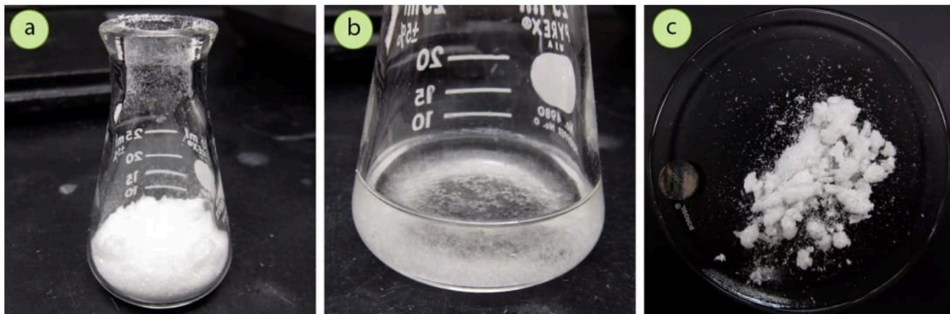
Figure 3.56: a) Initial sample of trans -cinnamic acid, b) Crystallization using methanol/water, c) Crystallized trans -cinnamic acid.
