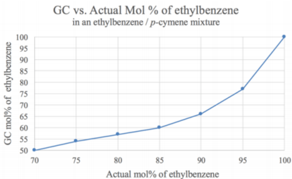
Figure 5.11: Calibration curve for GC analysis of an ethylbenzene/p-cymene mixture.
