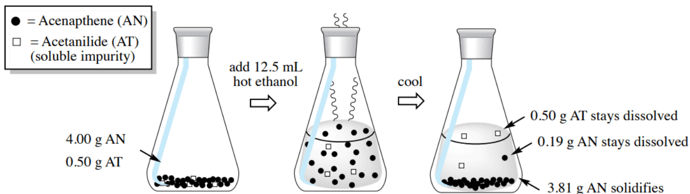
Figure 3.29: Crystallization of an impure sample containing 4.00 g acenaphthene and 0.50 g acetanilide from nearly boiling ethanol. This represents a crystallization with a "soluble" impurity.
