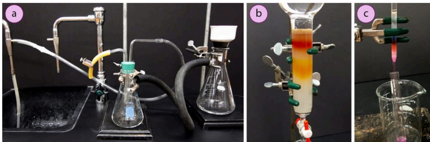
Figure 1.5: Examples where three-fingered clamps are used to hold: a) Flasks, b) Chromatography columns, c) Pipette columns.
