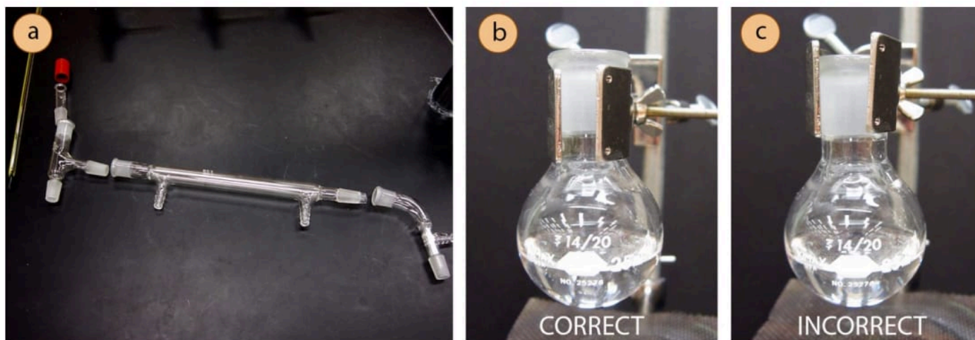
Figure 5.21: a) Distillation apparatus arranged on the benchtop, b) Correct clamping of the round bottomed flask, c) Incorrect clamping.
