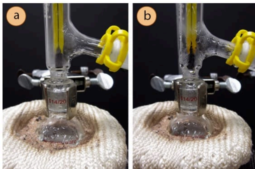
Figure 5.31: a) Before the solution is actively distilling, b) Actively distilling solution where the thermometer is registering the vapors.
