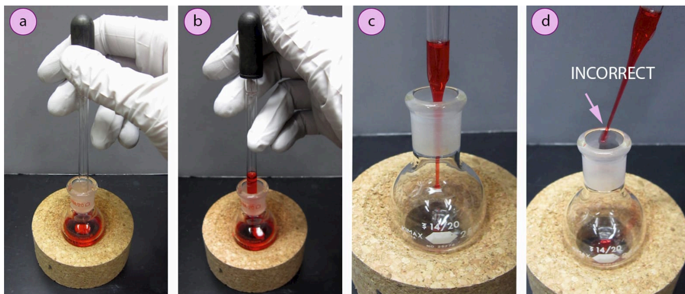
Figure 1.20: a+b) Creating suction with a Pasteur pipette, c) Delivering liquid from a Pasteur pipette, d) Incorrect delivering of reagent (liquid should not touch the sides of the glass).
