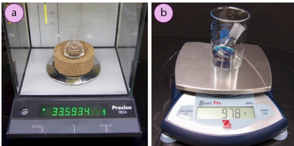
Figure 1.18: Round bottomed flasks supported by: a) Cork ring on an analytical balance, b) Beaker on a pan balance.
