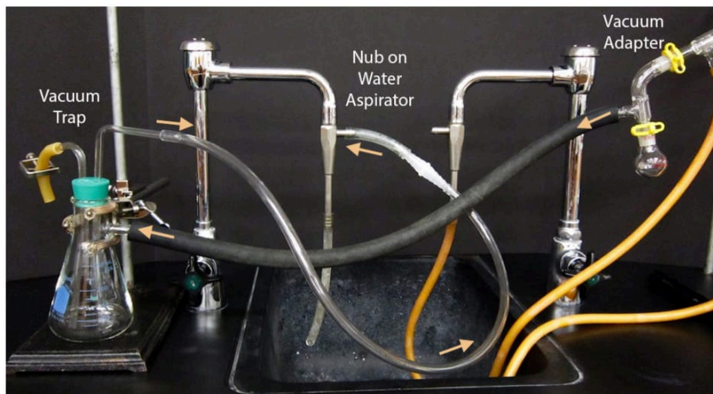
Figure 7.11: Vacuum distillation connection to a vacuum trap and the aspirator.
