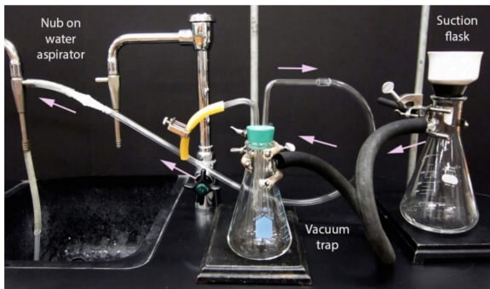
Figure 1.74: Suction filtration flask attached to a vacuum trap and water aspirator. The arrows show the direction of suction.
