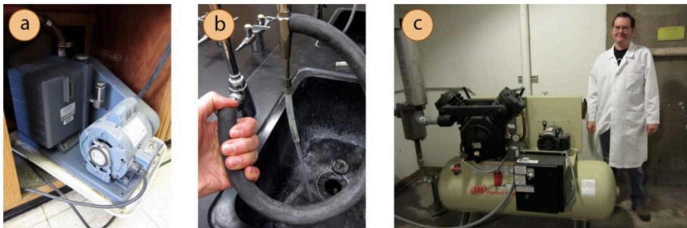
Figure 5.49: Vacuum sources: a) Portable vacuum pump, b) Water aspirator, c) House vacuum.
