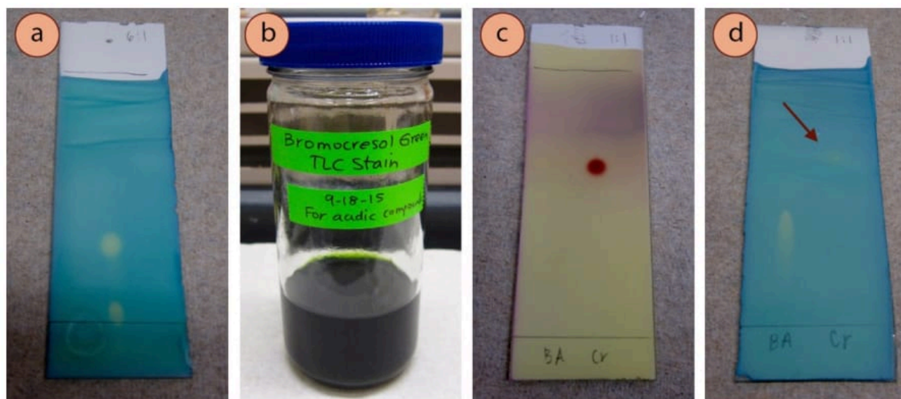
Figure 2.43: a) A plate stained with bromocresol green, b) Bromocresol green stain jar, c) Benzoic acid (lane 1) and p-cresol (lane 2) stained with p-anisaldehyde to show position of p-cresol, d) Same plate stained with bromocresol green (p-cresol is very faint and is indicated with an arrow).
