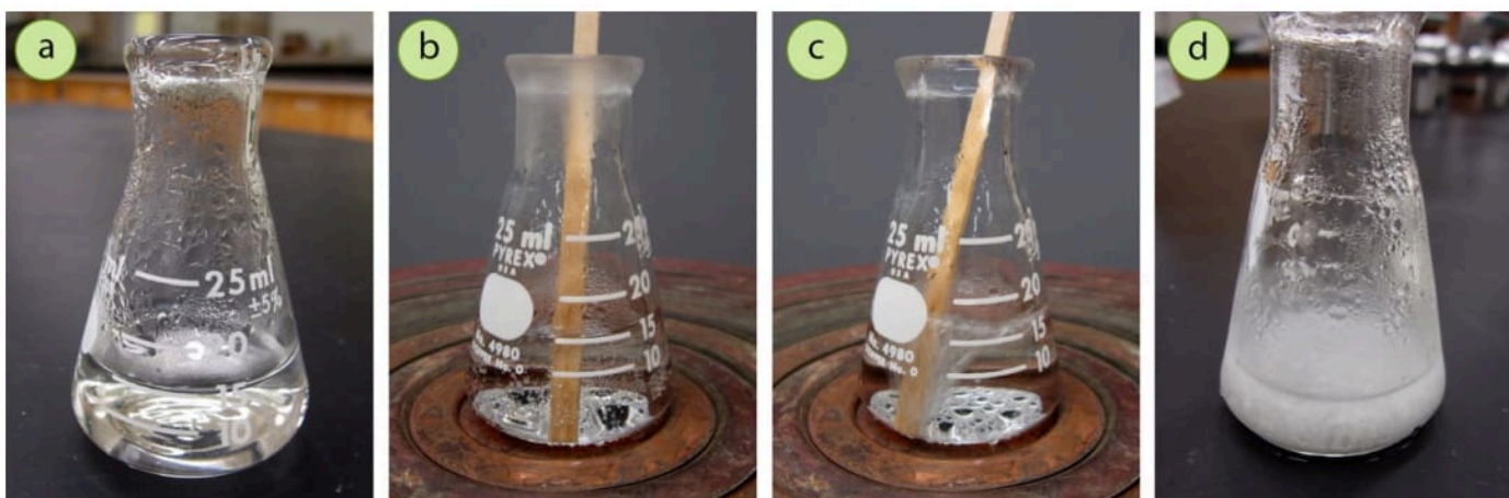
Figure 3.48: a) No crystals formed when cooled, b+c) Reducing the solvent volume on a steam bath, d) Crystals then formed when cooled.
