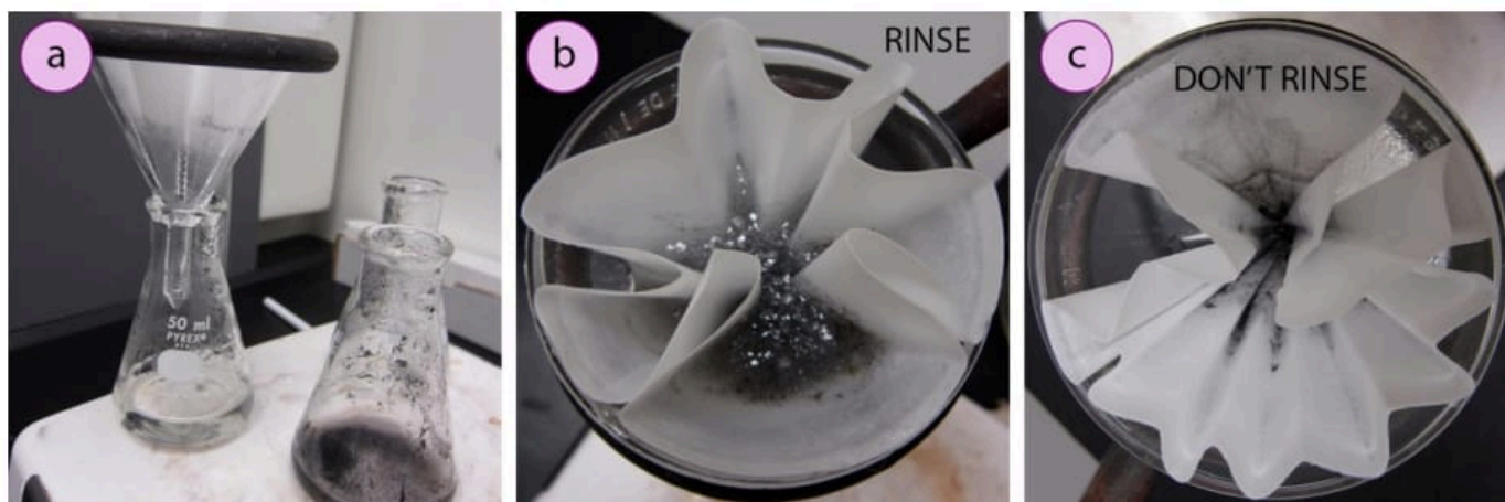
Figure 1.88: a) Flask is returned to the heat source in between pouring, Filter papers that b) should be rinsed, c) should not be rinsed.
