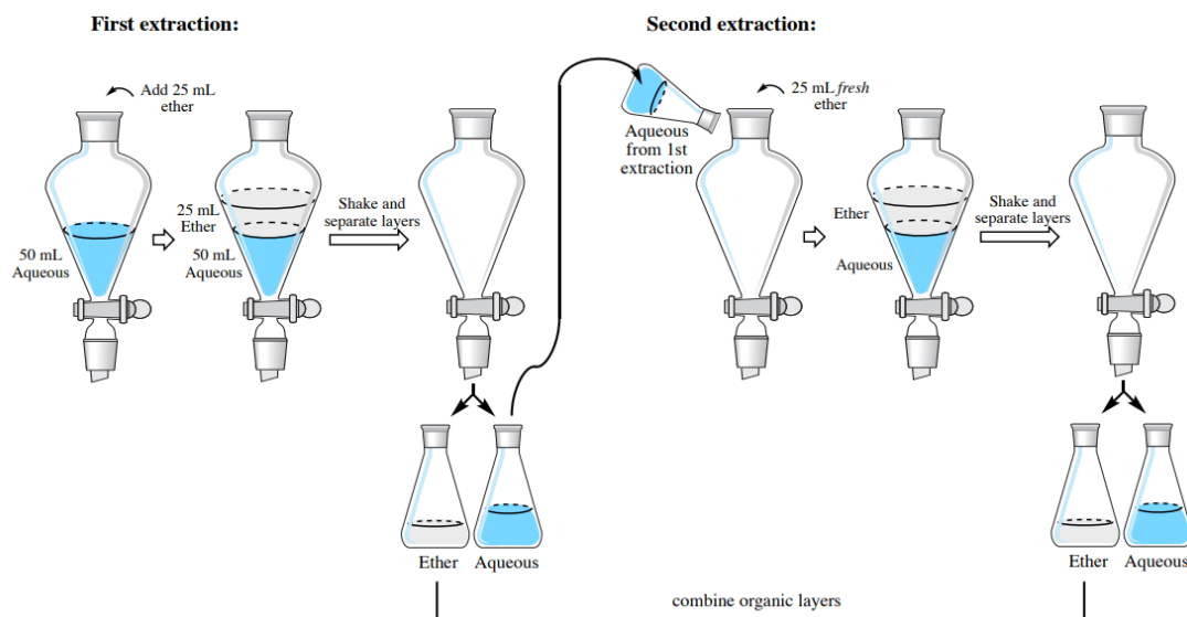
Figure 7.6: Multiple extraction flow-chart when the organic layer is on the top.
