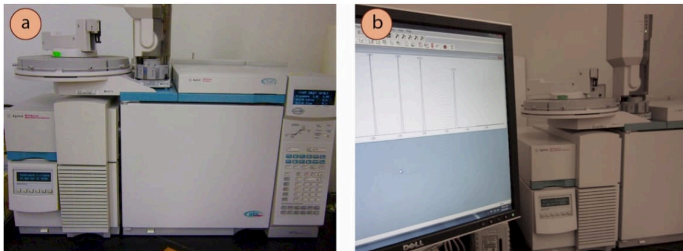
Figure 2.75: a) Gas chromatograph with mass spectrometer detector, b) GC-MS alongside a computer, which runs the instrument and can be used to manipulate the spectrum.
