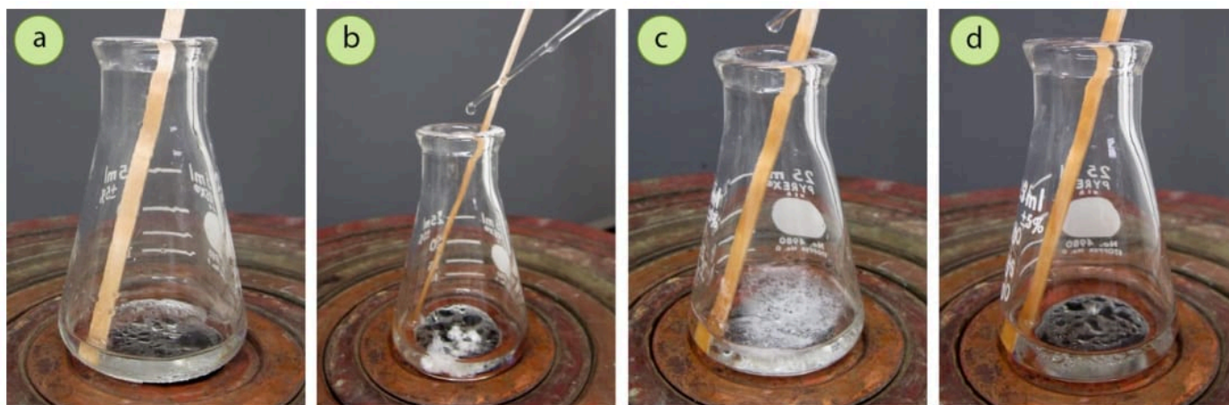
Figure 3.58: a) Addition of just enough soluble solvent (methanol) to dissolve the solid, b) Addition of the insoluble solvent (water) dropwise, c) Sustained cloudiness after addition of enough insoluble solvent, d) Addition of soluble solvent to clarify.
