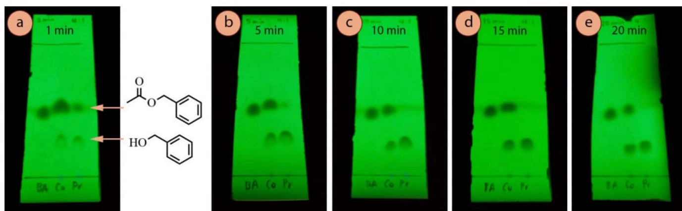
Figure 2.12: Monitoring of the transesterification reaction of benzyl acetate with TLC at 5-minute increments (using 4:1 hexanes:ethyl acetate and visualized with UV light): a) After 1 minute, b) 5 minutes, c) 10 minutes, d) 15 minutes, e) 20 minutes.
