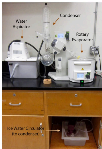
Figure 7.13: Rotary evaporator setup.
