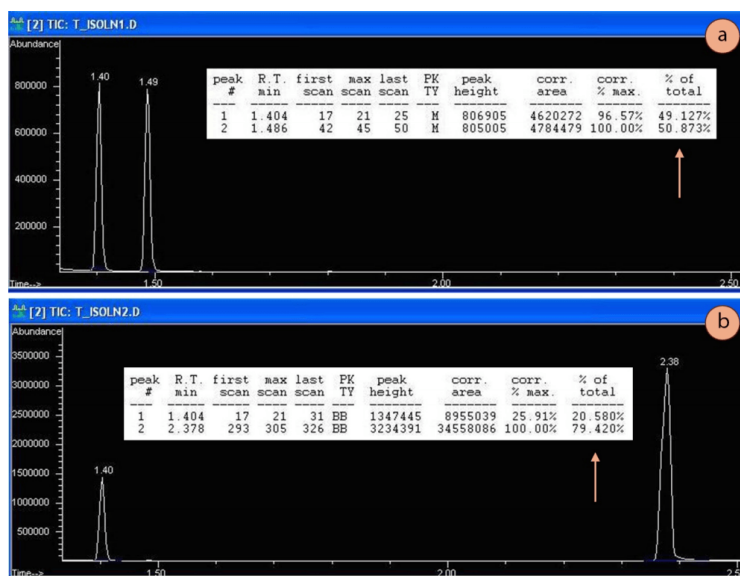
Figure 2.84: a) GC spectrum of a sample containing equimolar quantities of 1-butanol and 2-butanol, b) GC spectrum of a sample containing equimolar quantities of 2-butanol and 1-heptanol. Method for both runs: 60°C, ramp 20°C/min, MS detector. Arrows indicate the percentages reported by the GC for each spectrum.
