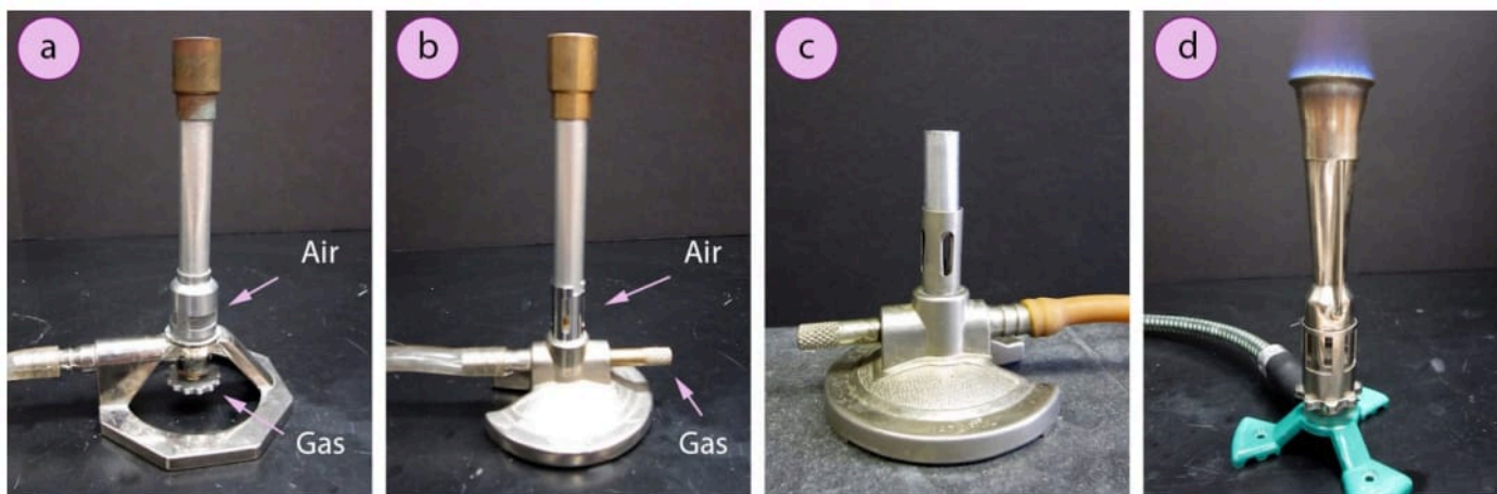
Figure 1.45: a) Bunsen burner, b) Tirrill burner, c) Microburner, d) Meker burner.
