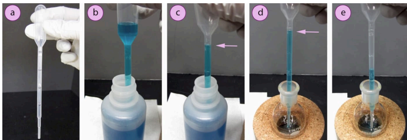
Figure 1.21: a) 1 mL calibrated plastic pipette, b) Suction of liquid, c) Depressing bulb to required volume (the arrow points to the 1 mL mark), d+e) Transfer of liquid.
