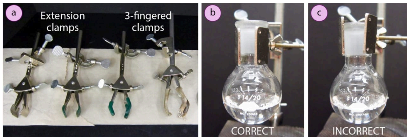
Figure 1.4: a) Extension and three-fingered clamps, b) Correct use of an extension clamp on a round bottomed flask, c) Incorrect clamping (flask may slip).
