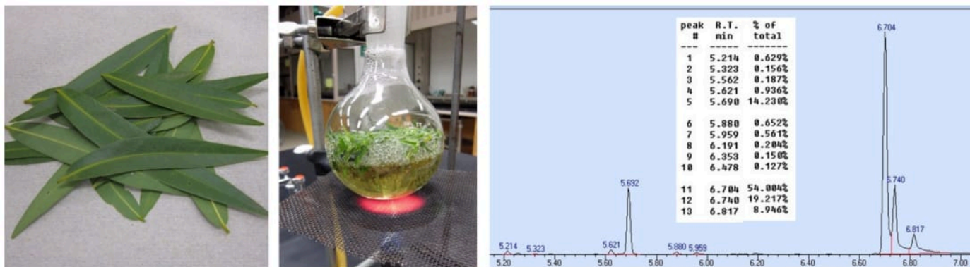
Figure 5.57: Steam distillation of bay leaves. The main peaks in the GC spectrum of the essential oil are eucalyptol (5.69 min, 14%), umbellulone (6.70 min, 54%), and 4-terpineol (6.74 min, 19%).
