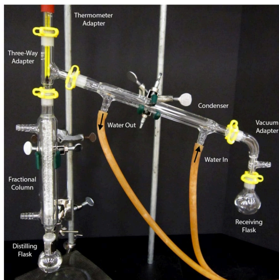
Figure 7.10: Fractional distillation apparatus.
