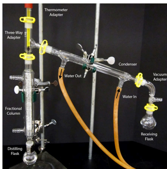
Figure 5.46: Fractional distillation setup.
