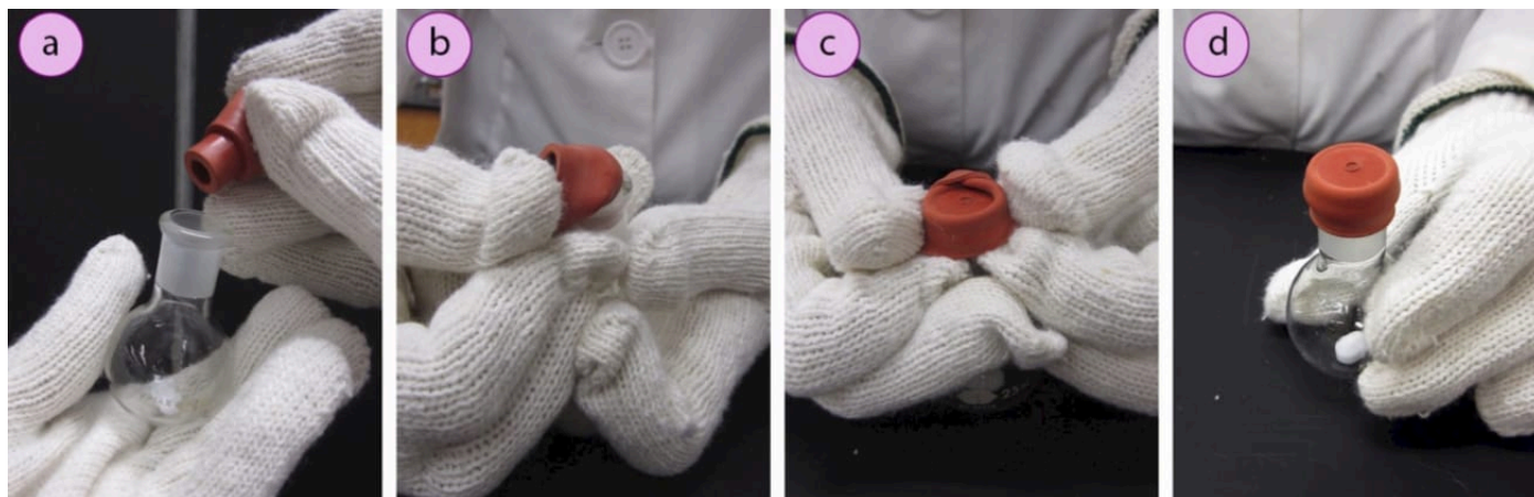
Figure 1.31: a) Inserting rubber septum into the joint of a hot flask, b-d) Folding septum flaps over the joint.
