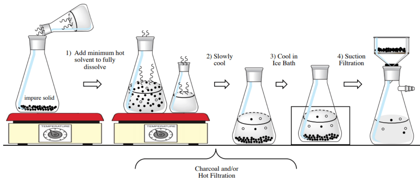
Figure 7.5: Single solvent crystallization flow-chart.
