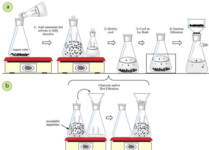
Figure 3.38: a) General procedure for crystallization, b) Modification when insoluble impurities are present.
