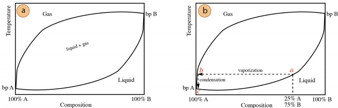
Figure 5.14: a) Generic distillation curve for a two-component system of A+B with widely different boiling points, b) Same curve with additional markings.
