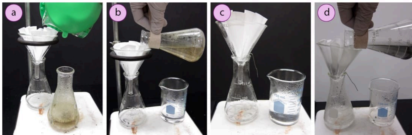
Figure 1.81: a) Pouring solvent through the funnel hot (note: hotplate is used in this situation as the solvent is water), b) Filtering a solution containing insoluble impurities, c+d) Variations using a paper clip instead of a ring clamp to hold the funnel.
