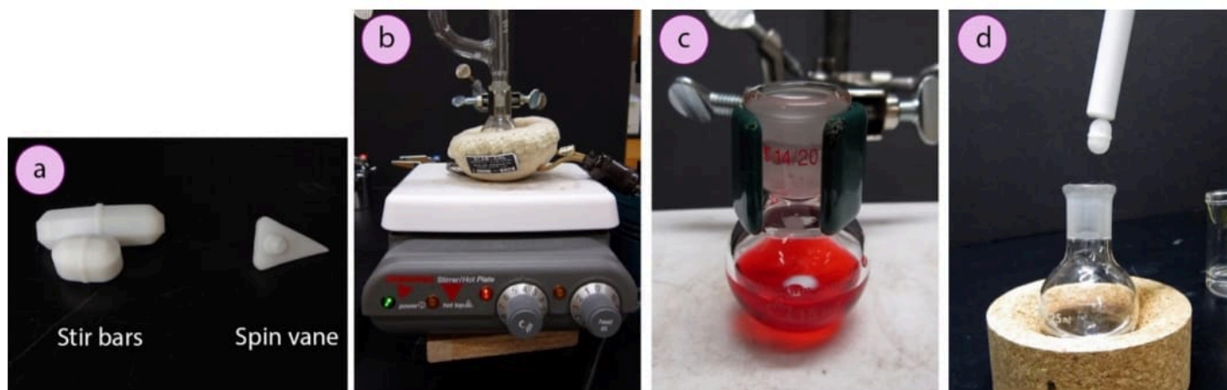
Figure 1.42: a) Stir bars and spin vanes, b) Stir plate, c) Stirring solution, d) Removal of a stir bar using a magnet (stir bar retriever).
