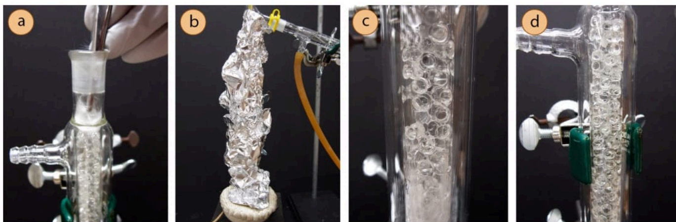
Figure 5.44: a) Removal of glass wool plug on a beaded fractionating column, b) Insulating the column with foil, c+d) Condensation on the beads of a fractionating column.
