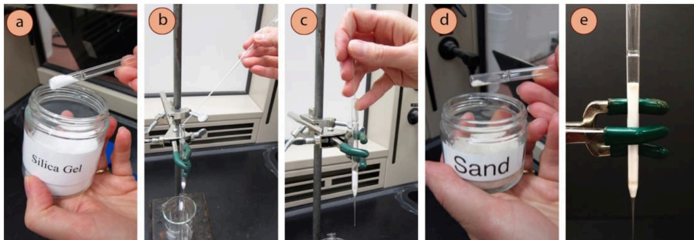
Figure 2.70: a) Scooping silica gel into the pipette column, b+c) Using a pipette as a funnel, d) Scooping sand, e) Complete dry column.
