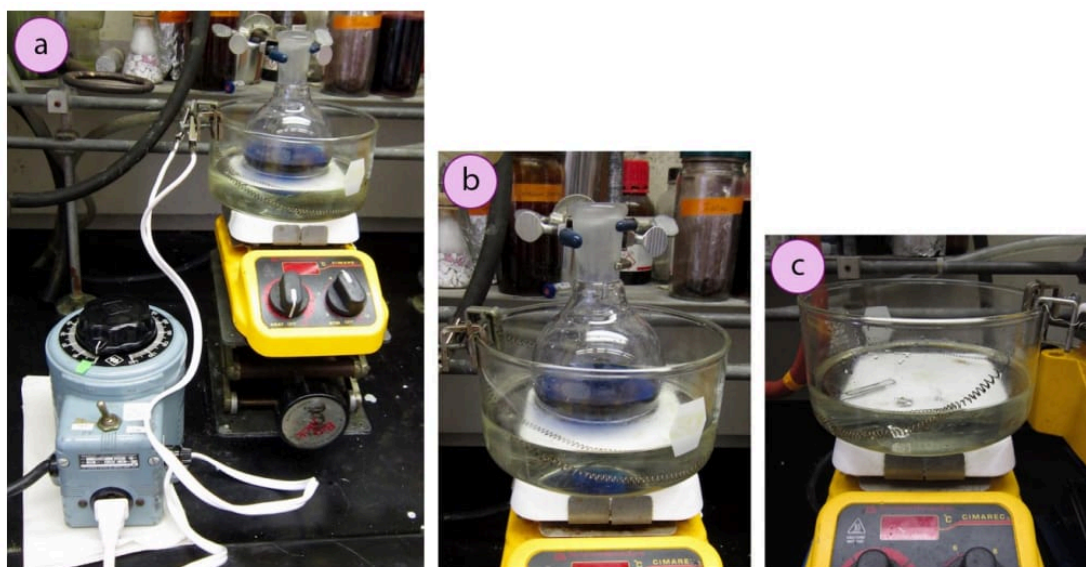
Figure 1.55: a) Oil bath connected to a Variac, b) Oil bath, c) Paper clip in the bath for stirring.
