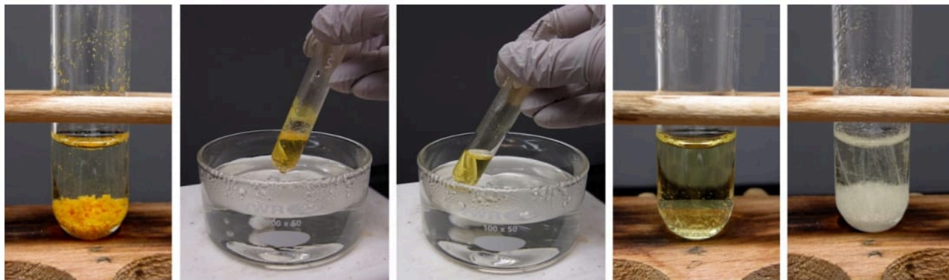
Figure 7.2: Crystallization testing process.
