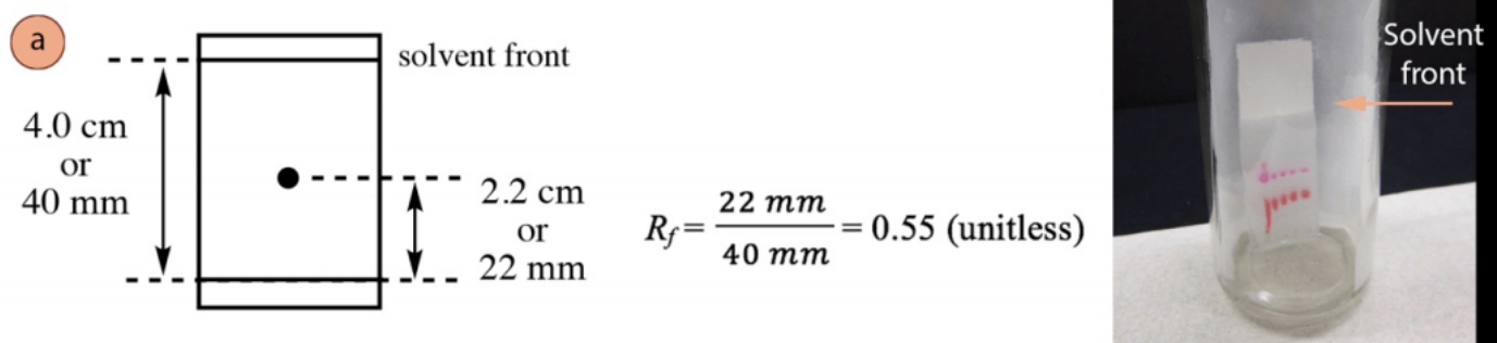
Figure 2.14: a) Sample R_f calculation, b) Appearance of the solvent front on an eluting TLC plate.
