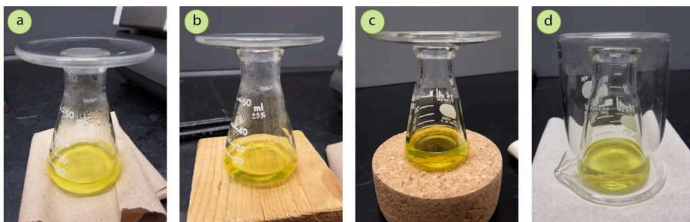
Figure 3.43: Methods to prevent a flask from cooling too quickly: a) Paper towel, b) Wood block, c) Cork ring, d) Inverted beaker.
