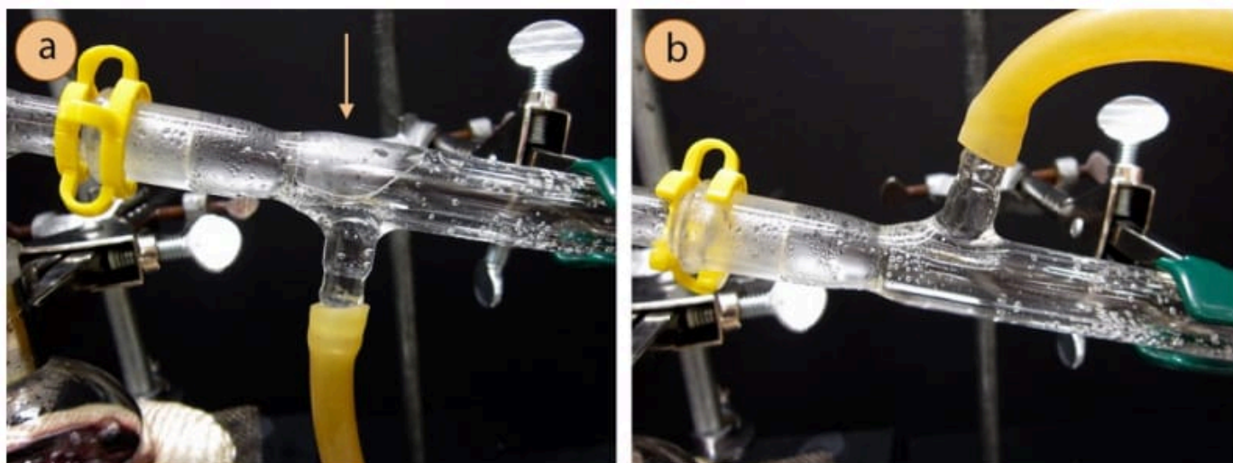
Figure 5.18: a) Condenser hoses pointed downward:notice the small pocket where water does not circulate, b) Hoses upwards.
