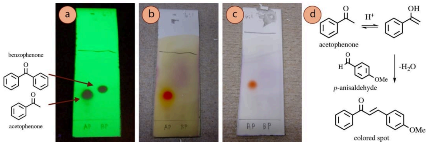
Figure 2.38: TLC's of acetophenone (lane 1) and benzophenone (lane 2), using 6:1 hexanes:ethyl acetate and visualized with: a) UV light, b) p -Anisaldehyde stain, c) Vanillin stain, d) A proposed reaction of acetophenone with p -anisaldehyde stain.
