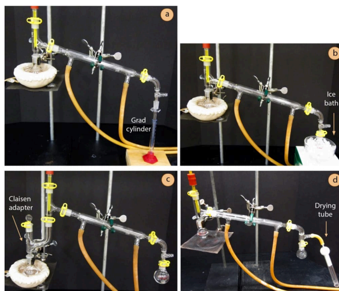
Figure 5.30: a) Distillation with graduated cylinder receiving flask, b) Distillation with receiving flask submerged in an ice bath, c) Distillation using a Claisen adapter, d) Attachment of a drying tube.
