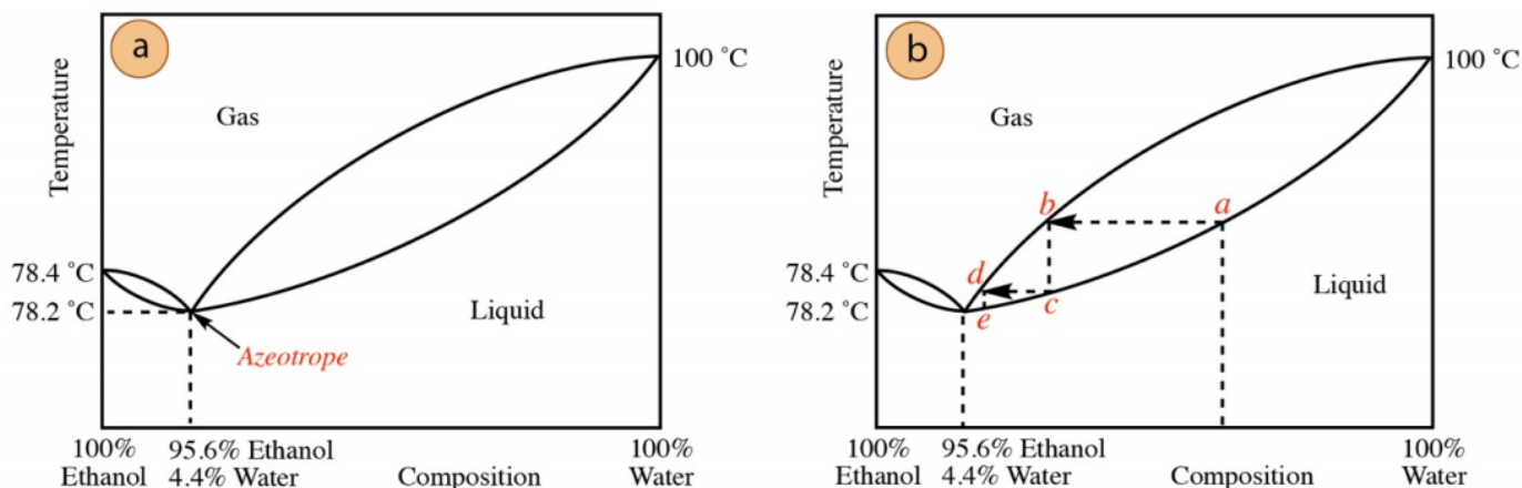
Figure 5.16: a) Distillation curve for the ethanol-water azeotrope (not drawn to scale), b) Same diagram with additional markings.
