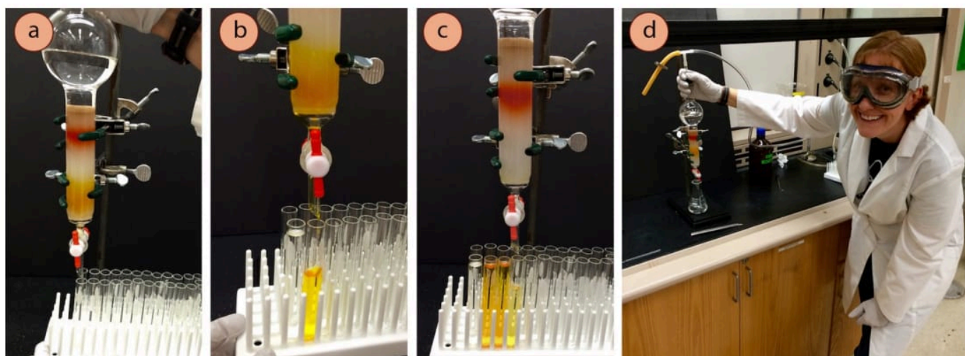
Figure 2.58: a-c) Collecting fractions, d) Author running a column.
