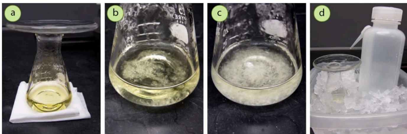
Figure 3.53: a-c) Cooling and crystallization of NBS, d) Further cooling in an ice bath along with some solvent (in the bottle) for rinsing.
