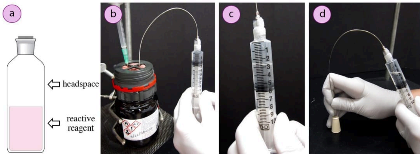
Figure 1.35: a) Headspace of a bottle, b) Inserting needle into the headspace of the reagent bottle, c) Inert gas buffer in the syringe, d) Placing the needle tip in a rubber stopper for transport.
