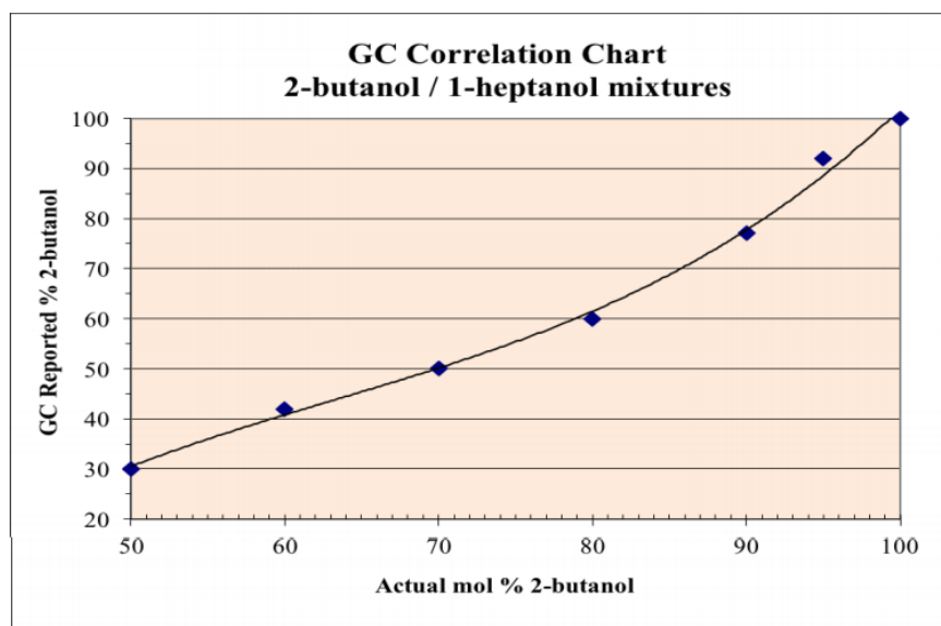
Figure 2.85: Known molar percentages of 2-butanol in a 2-butanol/1-heptanol mixture are correlated to the reported GC % of 2-butanol.
