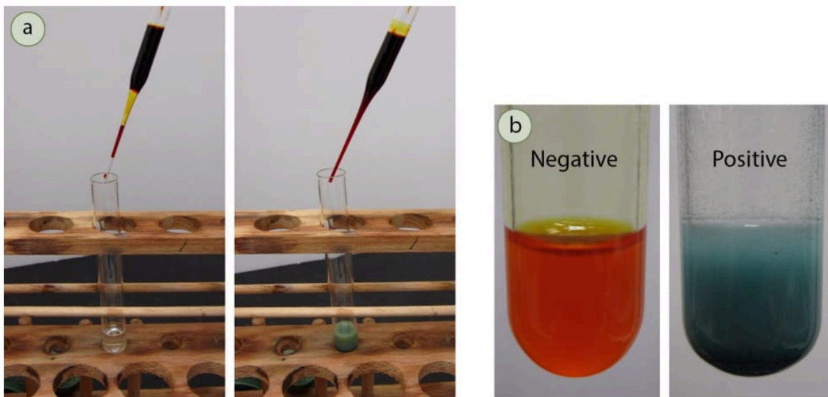
Figure 6.37: a) Addition of orange chromic acid reagent to a solution of 2-butanol in acetone (before and after), b) Negative result and positive results for the chromic acid test.
