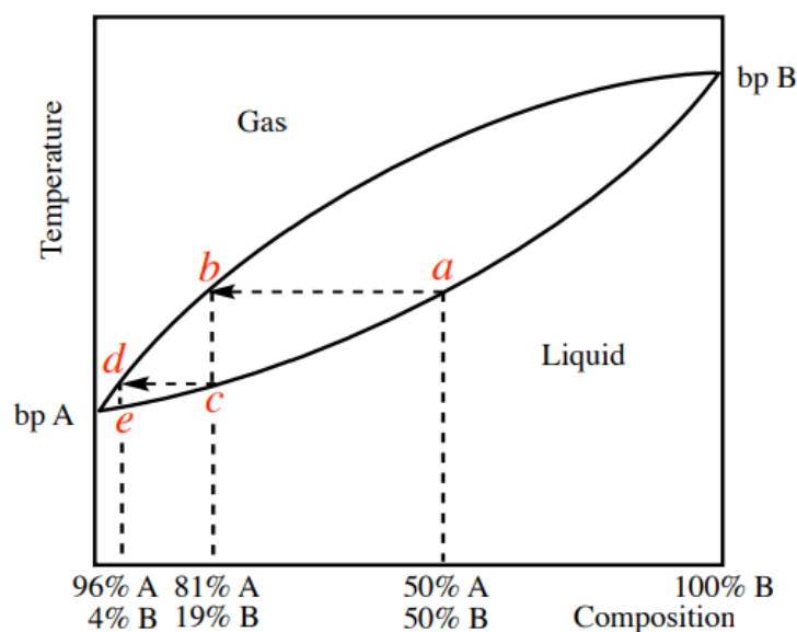
Figure 5.38: Distillation curve of a two-component system of A+B, showing two theoretical plates.
