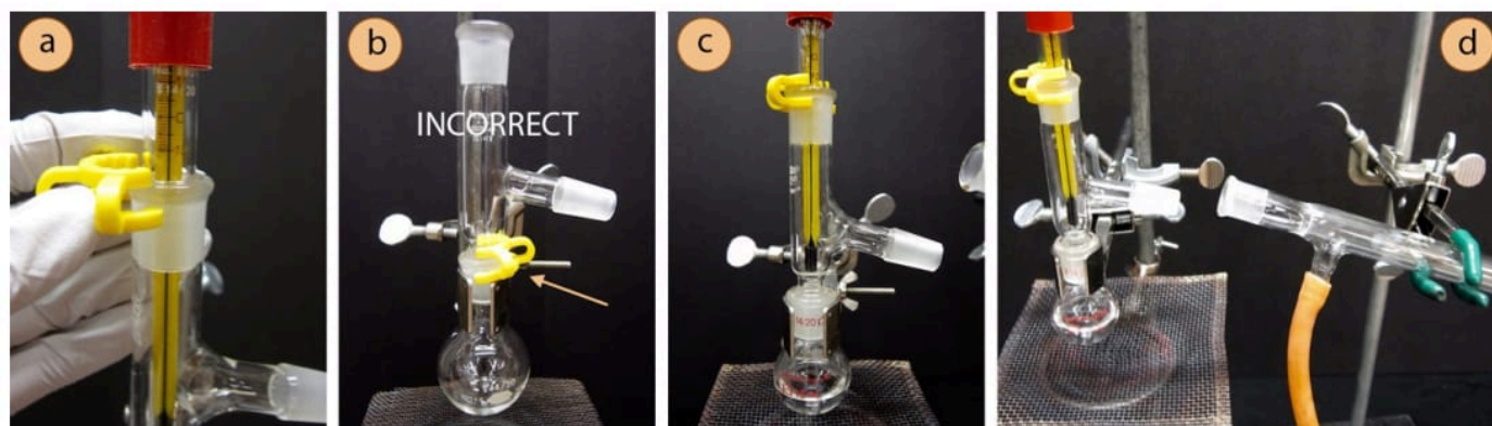
Figure 5.23: a) Connecting a plastic clip to secure a joint, b) Incorrect clamping: a plastic clip should not be used to connect the distilling flask to the three-way adapter (as indicated with the arrow), c) Correct positioning of the thermometer in the three-way adapter, d) Preparing the condenser.
