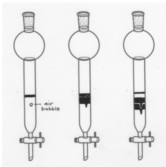
Figure 2.66: Effect of an air bubble on the separation in a column.
