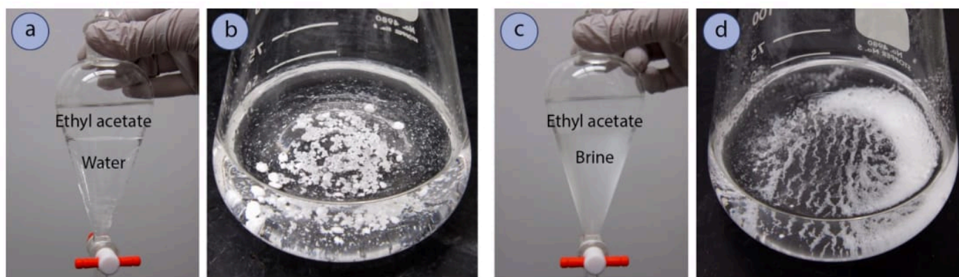
Figure 4.44: a) Ethyl acetate and water layers shaken together, b) Appearance of the ethyl acetate layer upon addition of anhydrous \text{MgSO}_4 , c) Ethyl acetate and brine layers shaken together, d) Appearance of the ethyl acetate layer with anhydrous \text{MgSO}_4 .
