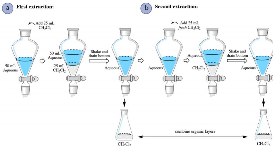
Figure 4.17: Multiple Extractions of an aqueous layer when the organic layer is on the bottom: a) First extraction, b) Second extraction.
