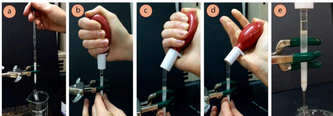
Figure 2.71: a) Adding eluent, b-d) Applying bulb pressure and correctly breaking the seal, e) Eluting the column.
