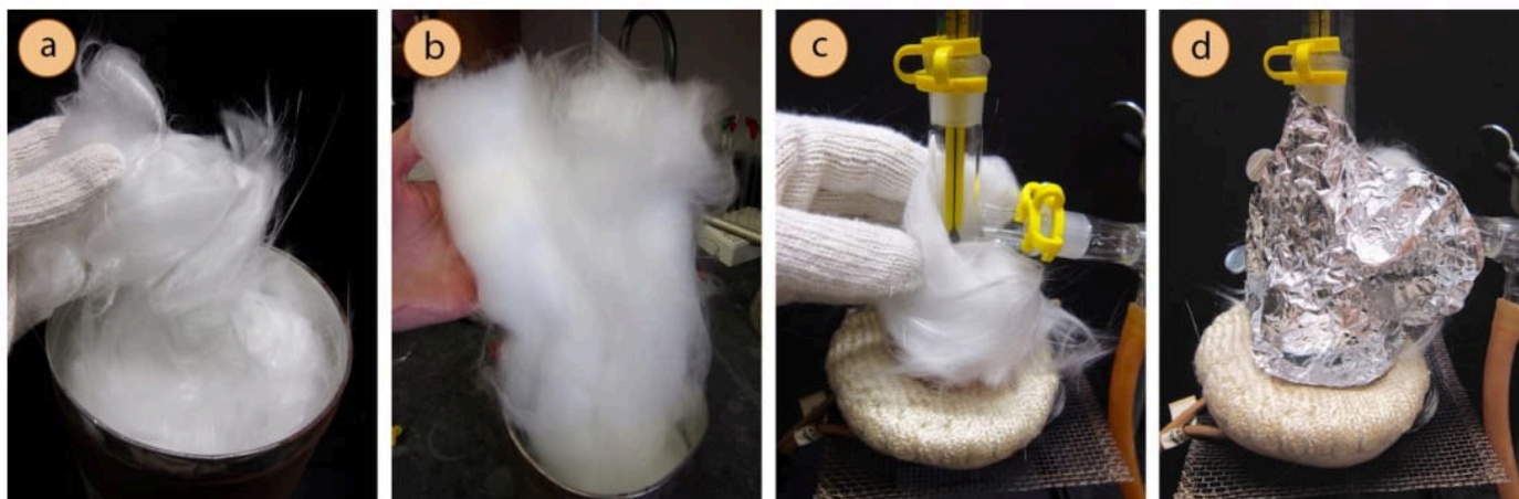
Figure 5.32: a) Fibrous glass wool, b) Cotton-like glass wool, c) Wrapping flask and three-way adapter with glass wool, d) Foil over top of glass wool.
