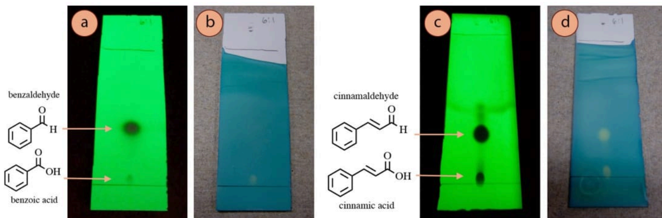
Figure 2.48: TLC plates of: a) Benzaldehyde with UV light, b) Benzaldehyde with bromocresol green stain, c) Cinnamaldehyde with UV light, d) Cinnamaldehyde with bromocresol green stain.
