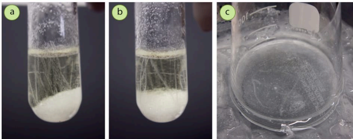
Figure 3.46: Lines of crystals seen in the initial stages of crystal growth, originating from where the glass was scratched: a+b) N -bromosuccinimide crystallizing from water, c) Acetanilide crystallizing from water.
