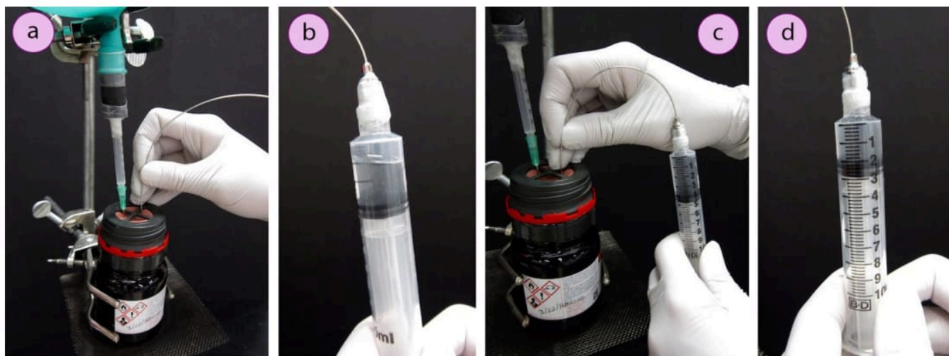
Figure 1.34: a) Inserting the flushed syringe into the air-sensitive reagent, b) Inevitable gas bubble after withdrawal, c) Removal of slightly more liquid than is needed, d) Adjustment to the correct volume.
