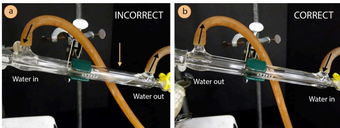
Figure 5.17: a) Condenser hoses connected incorrectly: notice that water does not fill the condenser's jacket (as indicated with the small arrow), b) Condenser hoses connected correctly.
