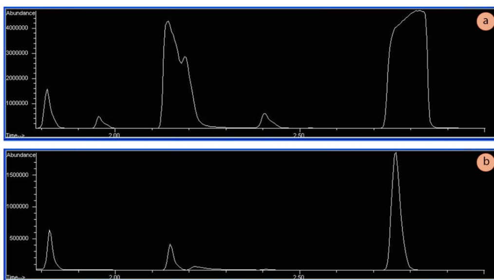
Figure 2.87: a) An overloaded sample with bad peak shape (note the y-axis has abundances around 4.5 million), b) The same sample diluted appropriately (abundances around 2 million). A too dilute sample will have abundances less than 100,000 (MS detector).
