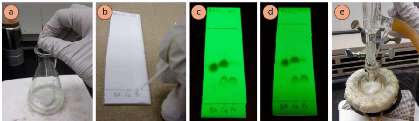
Figure 2.13: a) Obtaining an "aliquot" from a reaction mixture, b) Spotting the reaction mixture multiple times in the same lane, c) The appearance of the reaction mixture when it was not fully dried before elution, d) When the sample was fully dried before elution, e) Obtaining an aliquot for a refluxing solution.
