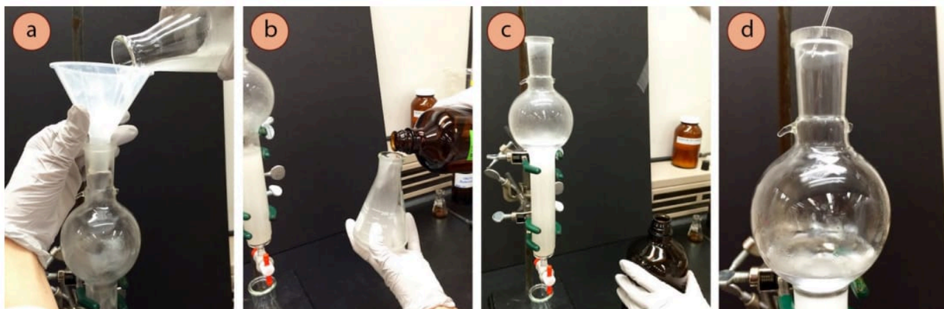
Figure 2.54: a) Pouring the slurry into the column, b) Rinsing the flask, c) Adsorbent adhered to the sides of the column, d) Rinsing off the clinging adsorbent.
