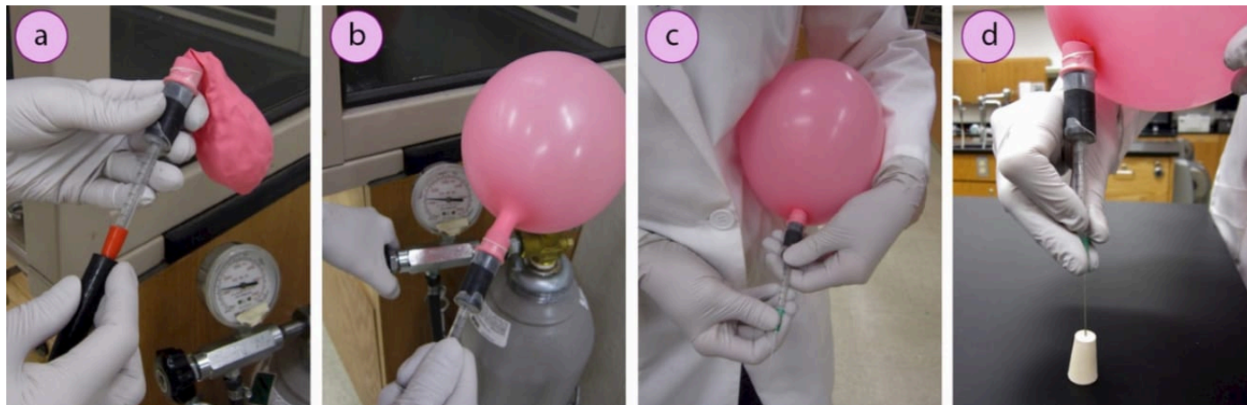
Figure 1.30: a) Attaching the balloon to a tank of nitrogen gas, b) Filling the balloon, c) Attaching the needle, d) Temporarily plugging the needle with a rubber stopper.
