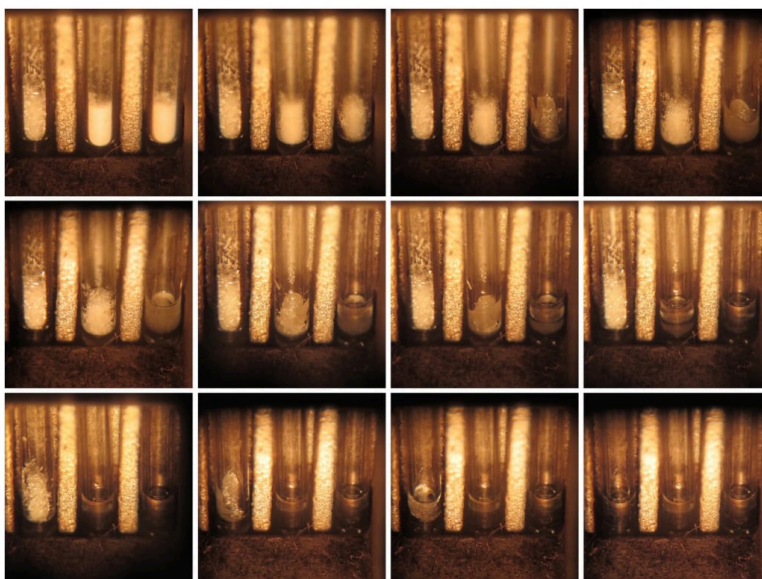
Figure 6.5: Time-lapse melting of three samples side by side in a melting point apparatus. Pure benzoic acid (left), benzoic acid with 10 mol% acetanilide (middle), benzoic acid with 20 mol% acetanilide (right).
