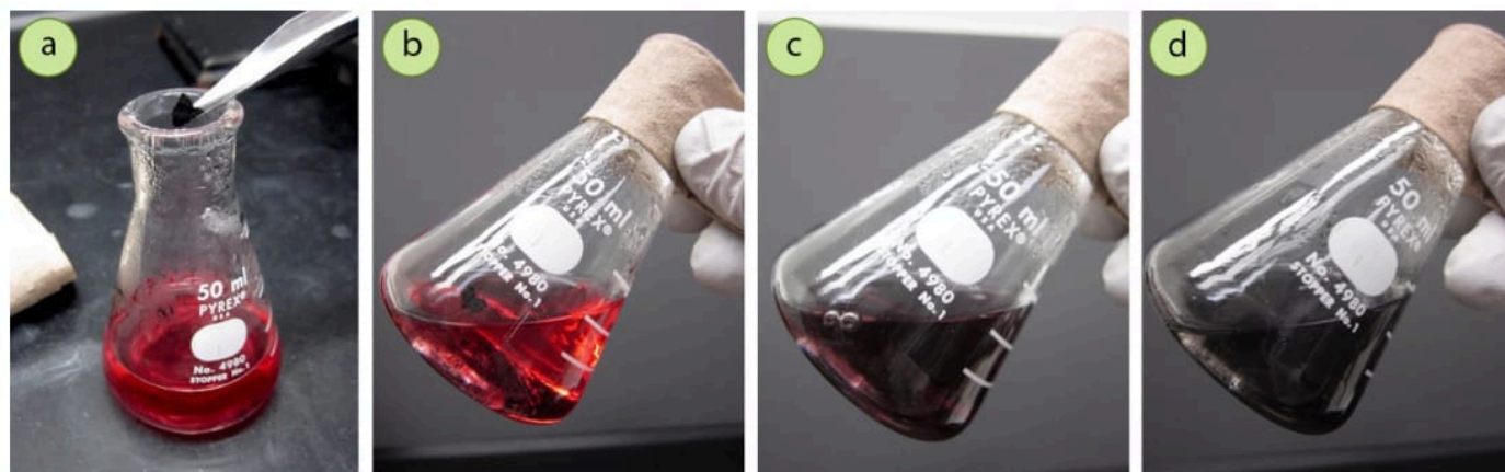
Figure 3.40: Use of charcoal with a highly-colored impurity (acetanilide contaminated with methyl red): a) Addition of charcoal to the aqueous solution, b) Pre-swirling, c) After swirling (color remains), d) Addition of another small scoop of charcoal to fully decolorize.
