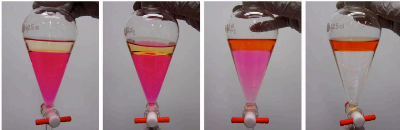
Figure 4.20: Progress of the extraction of methyl red (the colored compound) from the acidic aqueous layer (bottom) into the organic layer (top). The inversions were done slowly in order to see the extraction stepwise. With even gentle mixing, the methyl red extracts rapidly.
