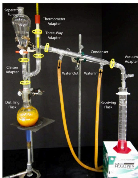
Figure 5.58: Steam distillation of orange peel using water in the distilling flask and a Bunsen burner.
