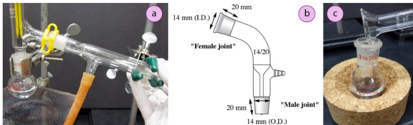
Figure 1.2B.1: a) Connections of ground glass joints, b) Ground glass joint measurements (for a 14/20 piece of glassware), c) Pouring liquid into a flask.
