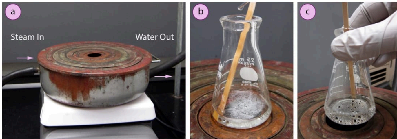
Figure 1.50: a) Steam bath, b) Heating a flask on the bath, c) Hovering the flask over the opening if the heating rate is too great.
