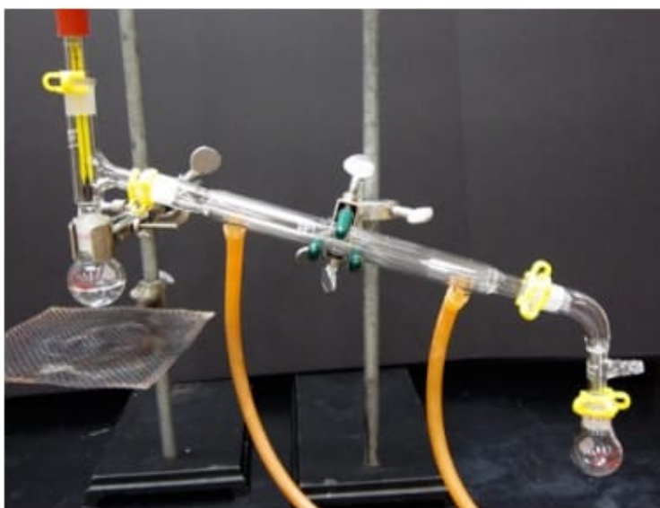
Figure 6.19: Simple distillation.
