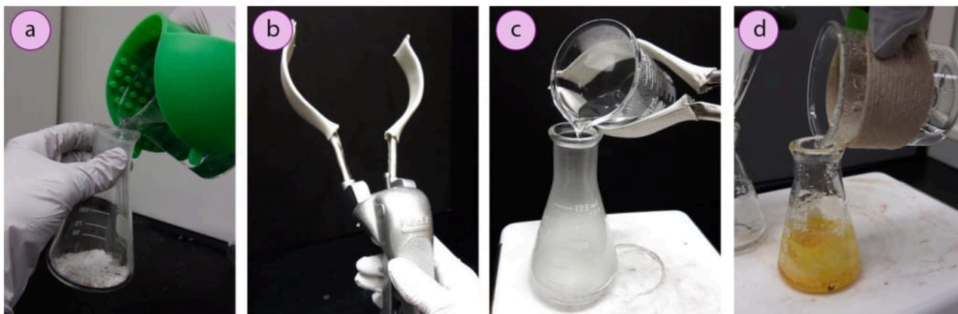
Figure 1.26: Pouring liquids with a: a) hot hand protector, b+c) Beaker tongs, d) paper towel holder.
