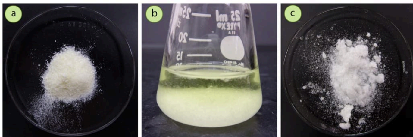
Figure 3.5: a) A mixed solid containing 85 mol% p -bromobenzoic acid and 15 mol% benzoic acid, b) Crystallization of the mixture using ethanol, c) Crystallized solid.
