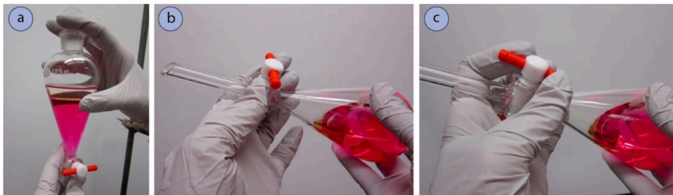
Figure 4.26: a) Holding the separatory funnel before shaking, b) Inverting the funnel to mix the components, c) Venting to release pressure.
