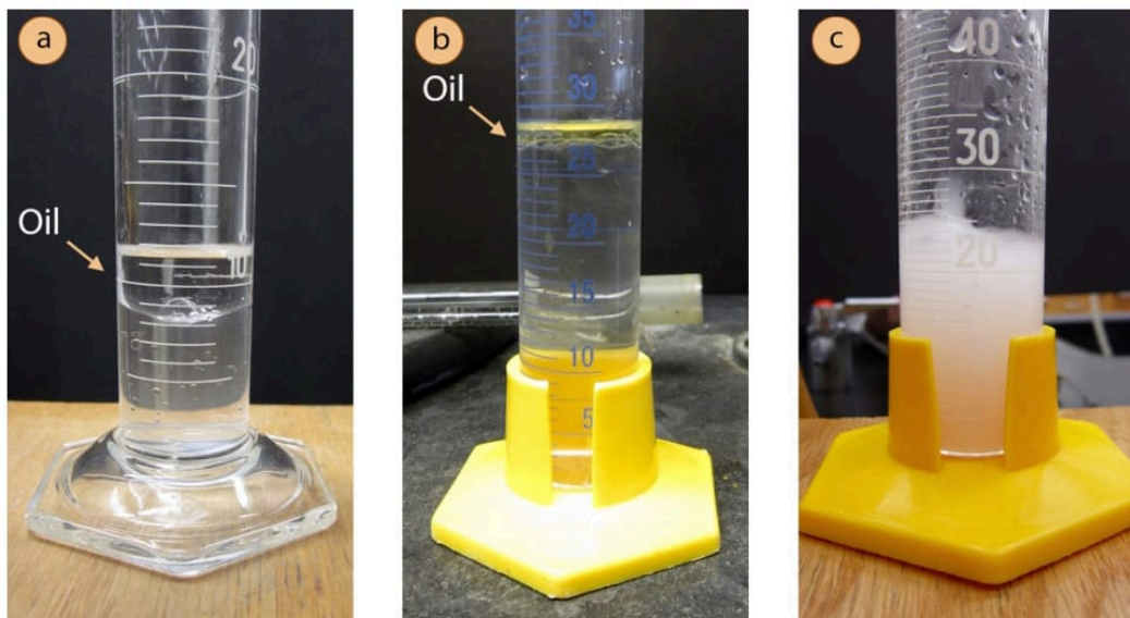
Figure 5.62: a+b) Distillate with organic oil atop water (orange oil in both), c) Milky distillate (clove oil).
