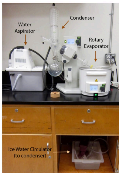
Figure 5.72: Rotary evaporation setup.
