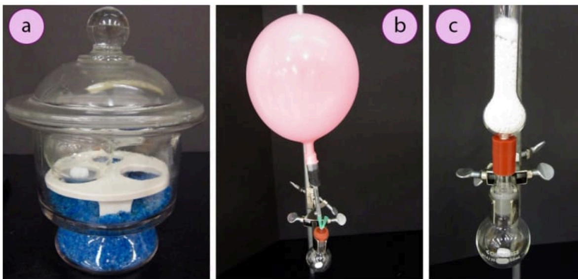
Figure 1.12: Drying hot glassware: a) In a desiccator, b) Under a balloon of inert gas, c) With a drying tube.
