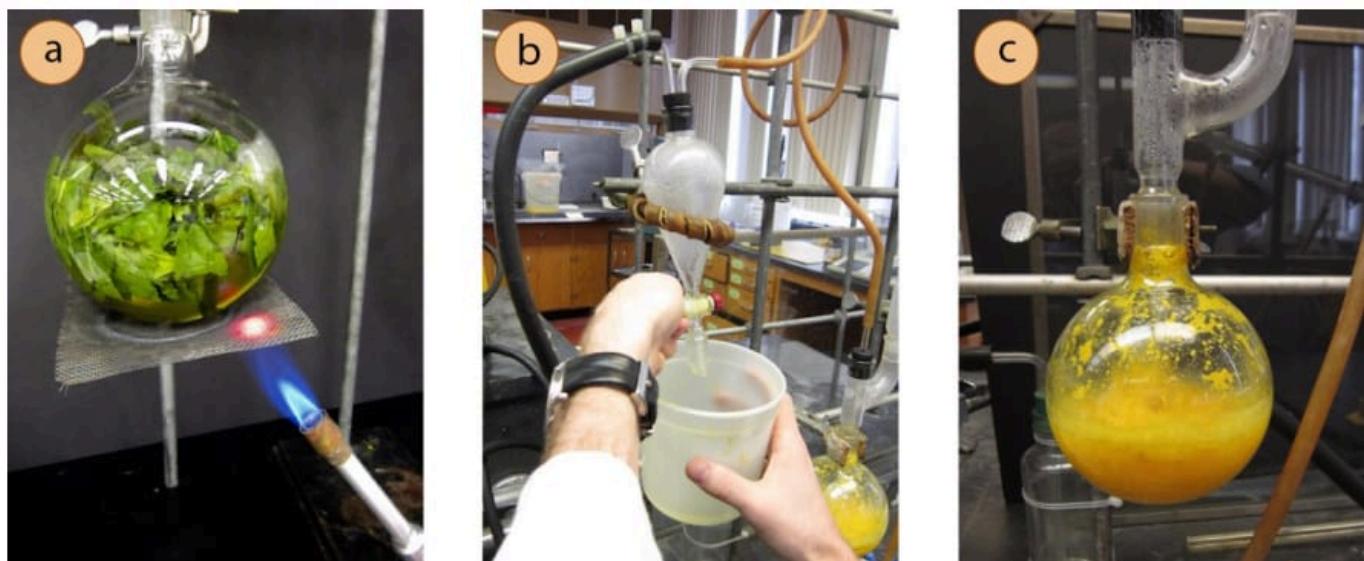
Figure 5.61: a) Waving the burner to heat the distilling flask (with mint), b) Draining the water from the steam trap after opening the steam line, c) Steam bubbling through the distilling flask (with orange peels).
