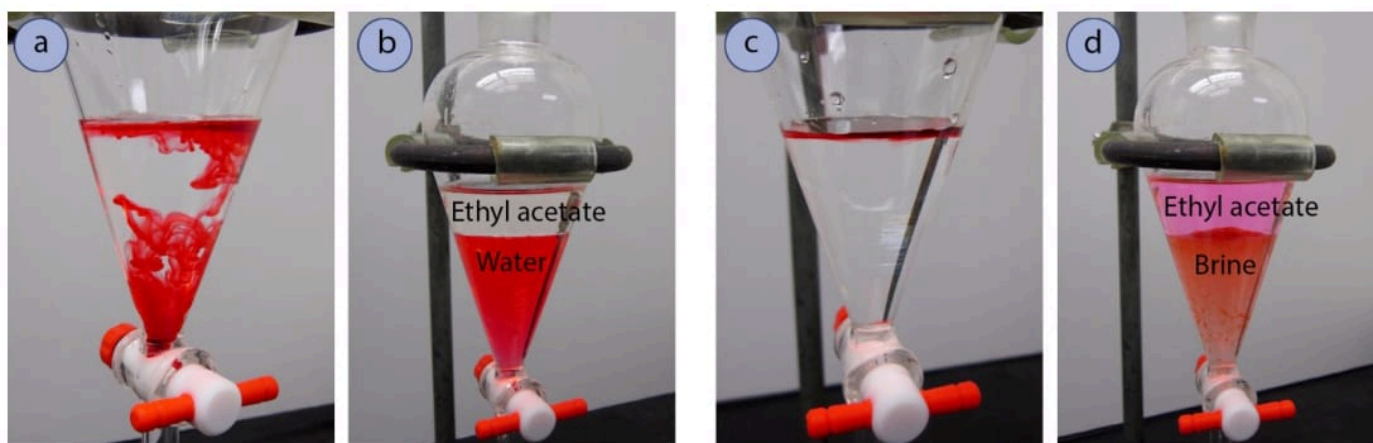
Figure 4.47: a) Water with the addition of one drop of red food dye, before swirling, b) Ethyl acetate, water, and dye at equilibrium, c) Brine with the addition of one drop of red food dye, before swirling, d) Ethyl acetate, brine, and dye at equilibrium.
