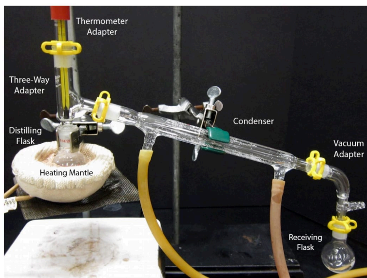
Figure 5.19: Simple distillation apparatus.
