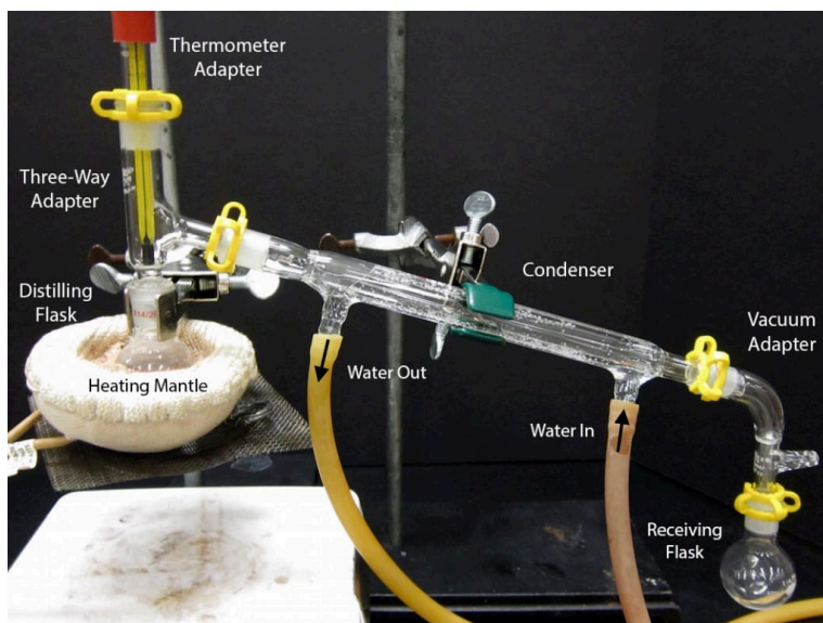
Figure 7.9: Simple distillation apparatus.
