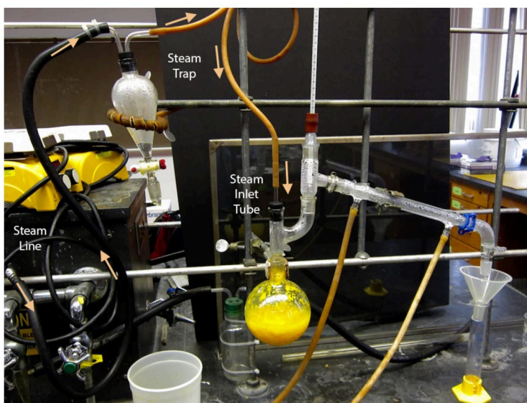
Figure 5.59: Steam distillation variation using a steam line from the building. Arrows show the direction of the steam.
