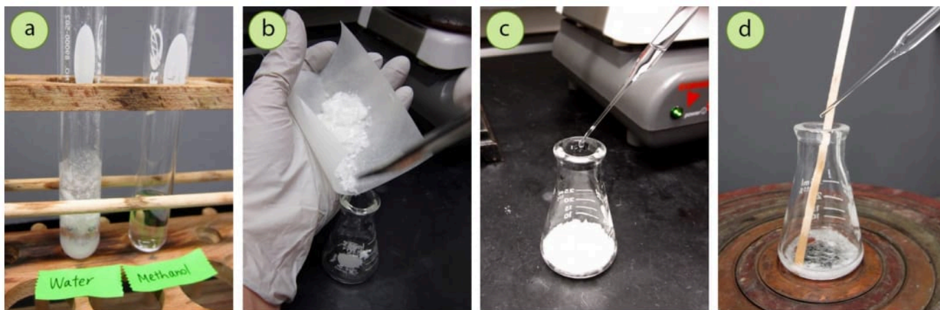
Figure 3.57: a) Trans -cinnamic acid is insoluble in water and soluble in methanol, b) Adding solid to the flask, c) Adding methanol off the heat source, d) Adding enough methanol to dissolve the solid.
