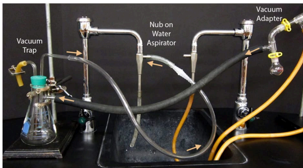
Figure 5.55: Vacuum distillation connection to a vacuum trap and the aspirator.
