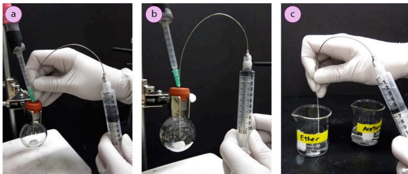
Figure 1.37: a) Inserting the syringe into the reaction flask, b) Delivering the liquid, c) Rinsing the needle and syringe.
