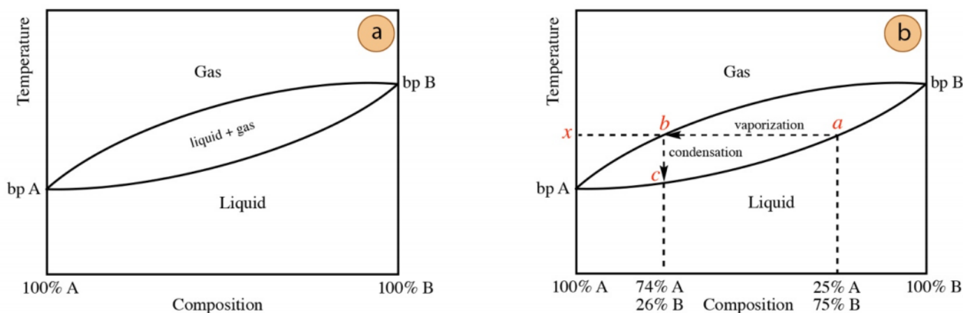
Figure 5.13: a) Generic distillation curve for a two-component system of A+B, b) Same curve with additional markings.
