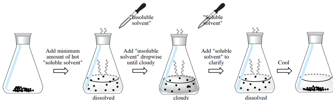
Figure 7.4: Mixed solvent crystallization flow-chart.
