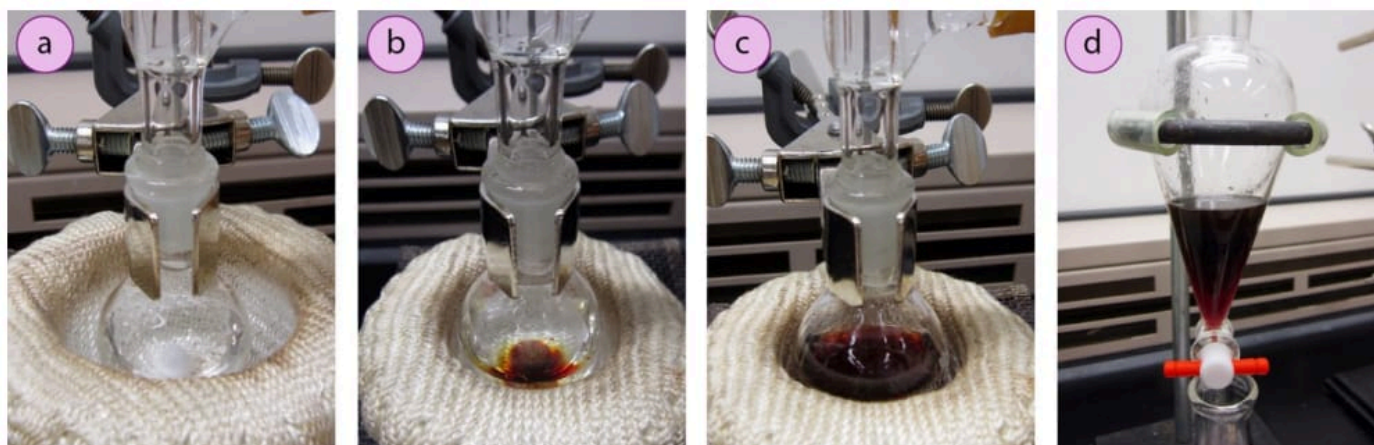
Figure 1.40: a) Fischer esterification reaction using a stir bar (solution is colorless), b) Same reaction using boiling stones, c) Same reaction after a few minutes of heating, d) Two dark layers in the separatory funnel as a result of the darkened solution.
