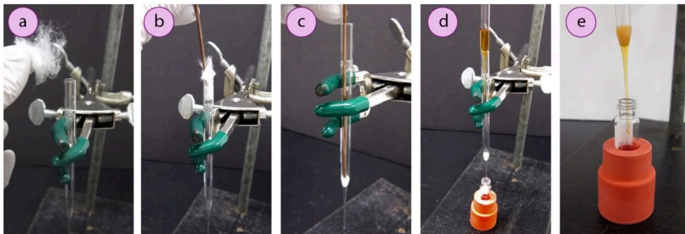
Figure 1.89: Creating and using a filter pipette: a) Piece of cotton, b+c) Shoving cotton to the bottom of the pipette, d) Filtering a mixture into a GC vial, e) GC vial held with an upside down large septum.
