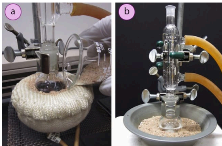
Figure 1.63: a) Filling a heating mantle with sand to ensure a perfect fit, b) Heating a reflux apparatus with a sand bath.
