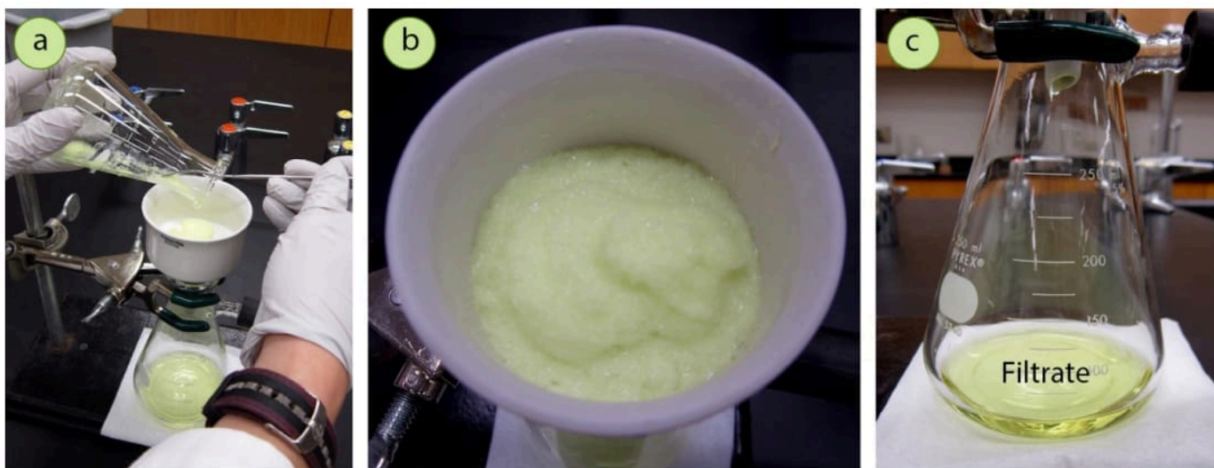
Figure 3.24: Loss of yield due to the solubility of compound in the cold solvent: a) Suction filtration, b) Recovered yellow solid, c) Yellow filtrate, indicating some yellow compound remained dissolved in the mother liquor.
