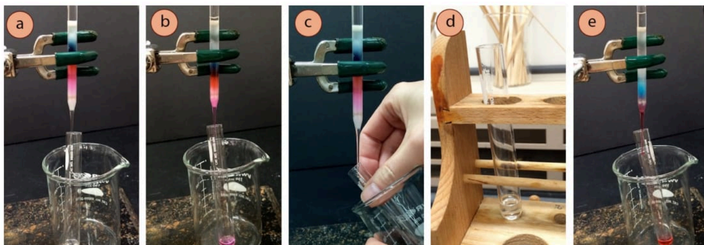
Figure 2.73: a) Eluting, b) Collecting the pink fraction, c) Changing the collection tube, d) Storing fractions in a rack, e) Collecting the red fraction.
