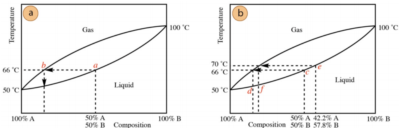
Figure 5.15: a) Distillation curve for a two-component mixture of A (b.p. 50 °C) and B (b.p. 100 °C), b) Additional markings.
