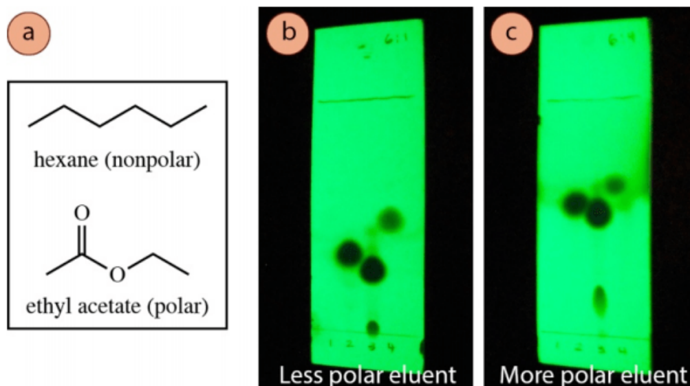
Figure 2.21: a) Structures of hexane and ethyl acetate, b) Three compounds visualized by UV light and run with 6:1 hexanes:ethyl acetate mixtures, c) Same three compounds with a 3:2 ratio (more polar).
