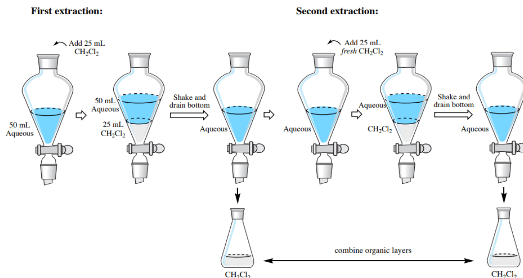
Figure 4.30: Two extractions when the organic layer is on the bottom.
