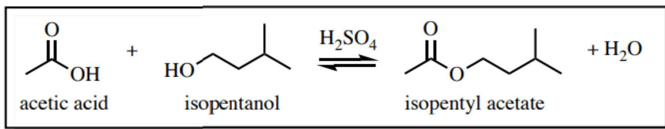
Figure 4.6: Reaction scheme to produce isopentyl acetate.
