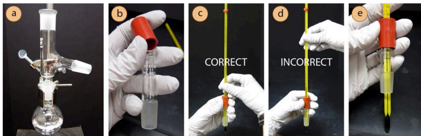
Figure 5.22: a) Flask and three-way adapter, b) Attachment of rubber fitting to thermometer adapter, c) Correct way to insert the thermometer, d) Incorrect way (thermometer will break), e) Assembled thermometer piece.
