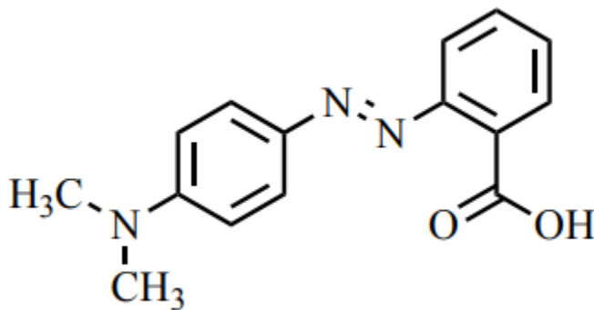
Figure 4.21: Structure of methyl red in highly acidic solution.
