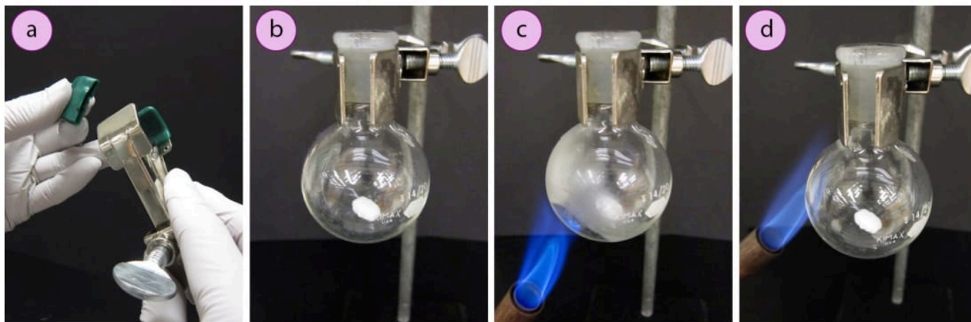
Figure 1.11: Flame drying glassware: a) Removal of vinyl sleeves, b) Clamped, c) First moments with a flame, d) After the flame.
