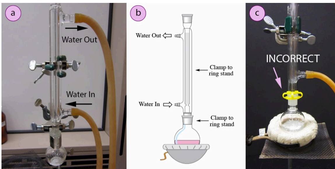
Figure 1.60: a) Reflux apparatus, with arrows indicating the direction of water flow, b) Reflux diagram, c) Incorrect clamping of a reflux apparatus.
