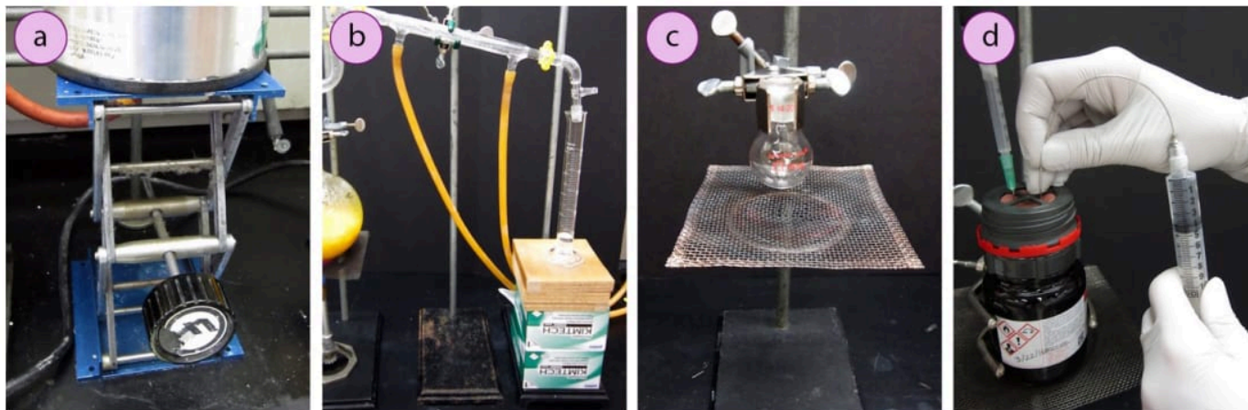
Figure 1.43: Adjustable platforms: a) Lab jack, b) Wood blocks and KimWipe boxes, c) Ring clamp with wire mesh, d) Air-sensitive reagent held in place with a ring clamp/wire mesh platform.
