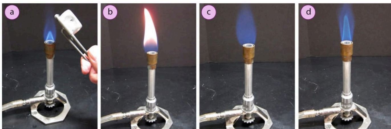
Figure 1.47: a) Lighting a burner with a striker, b) Too orange of a flame, c) No blue cone, d) Properly lit burner.
