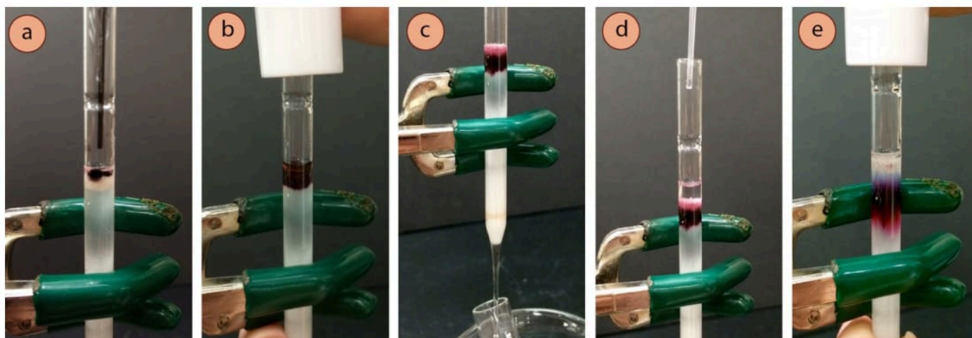
Figure 2.72: a) Adding sample, b) Applying pressure, c) Dye pushed onto the adsorbent, d) Filling with eluent, e) Eluting.
