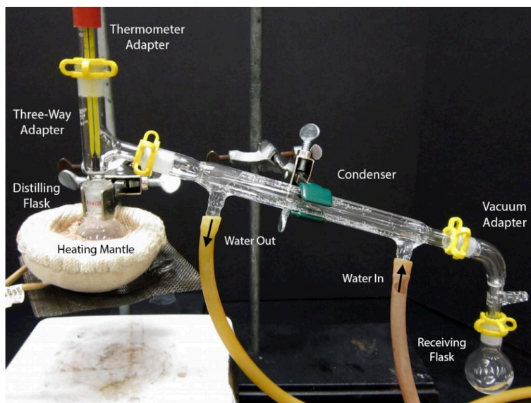
Figure 5.29: Simple distillation apparatus.
