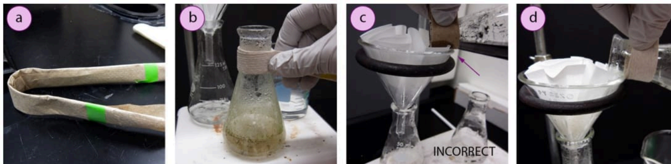
Figure 1.27: a) Paper towel holder, b) Holding an Erlenmeyer flask with a paper towel holder, c) A too-wide holder, causing liquid to wick onto the paper as it is poured, d) A narrower holder, which pours without wicking.
