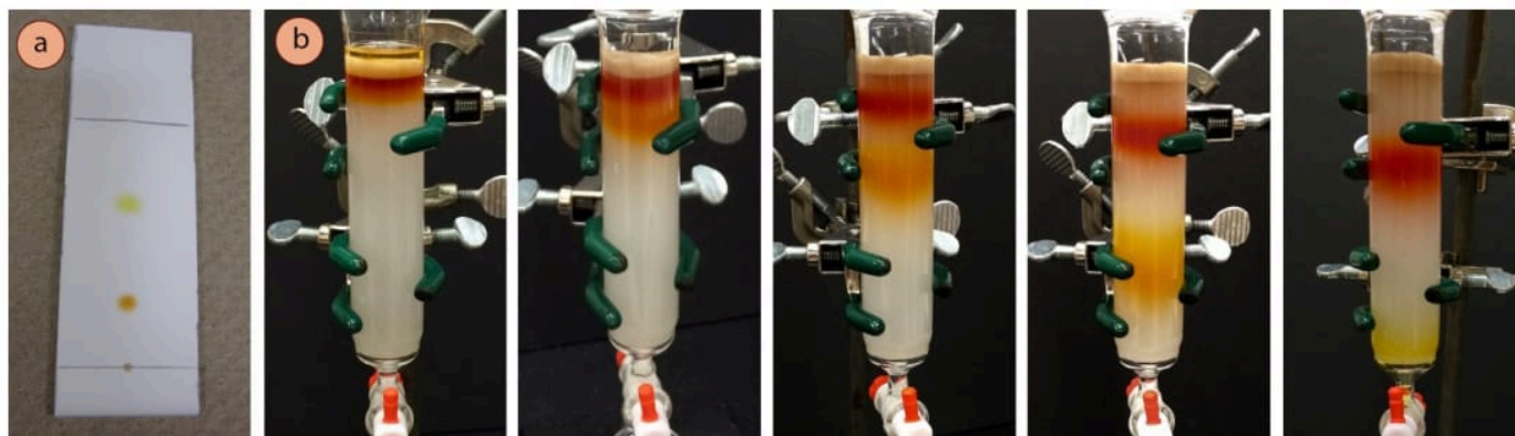
Figure 2.51: a) TLC of ferrocene/acetylferrocene mixture, b) Column chromatography.
