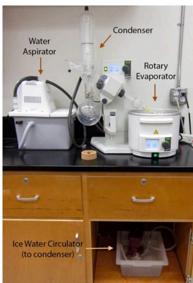
Figure 5.65: Rotary evaporator, water aspirator, condenser, and ice water circulator.
