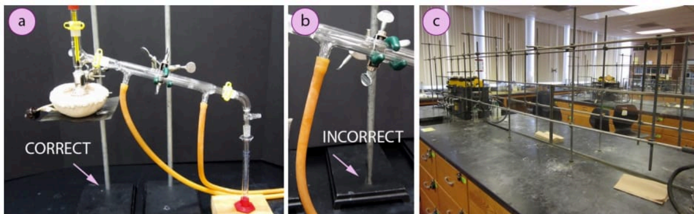
Figure 1.3: a) Correct clamping of an apparatus to a ring stands, with the apparatus directly over the metal base, b) Incorrect use of a ring stand, where the apparatus is not directly over the metal base, c) Metal lattice-work for clamping apparatuses.
