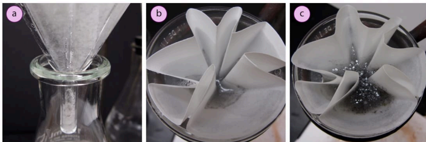
Figure 1.82: A filtration that was conducted at too low a temperature: a) Crystallization occurred in the stem of the funnel, b) A sheen can be seen on the filter paper, representing solid that has crystallized somewhat on the filter paper, c) Obvious crystals formed on the filter paper.
