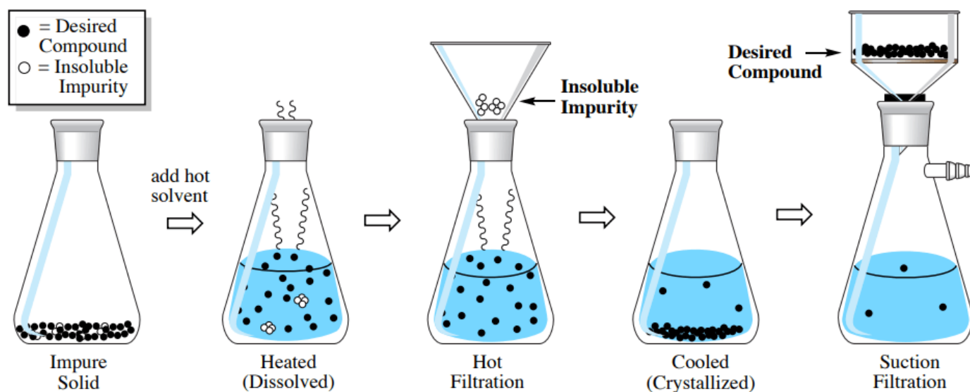
Figure 3.10: Crystallization sequence to remove an insoluble impurity. In the second flask, the white circles aggregate as an insoluble material, while the black circles are dispersed and therefore dissolved and invisible.
