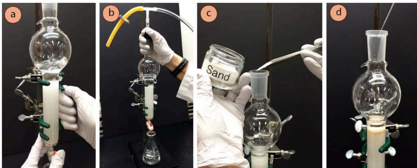
Figure 2.55: a) Jostling the column to remove air bubbles, b) Applying air pressure, c) Adding sand, d) Rinsing sand from the sides.
