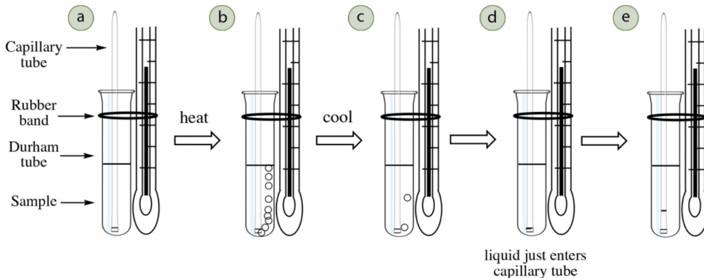
Figure 6.23: Boiling point determination: a) Initial setup, b) After heating past the boiling point, c) Cooling, d) Liquid just enters the capillary tube (temperature is the boiling point), e) Liquid is inside the capillary tube (temperature is lower than the boiling point).
