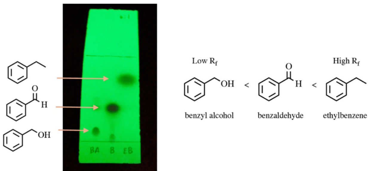
Figure 2.18: TLC of benzyl alcohol (lane 1), benzaldehyde (lane 2), and ethylbenzene (lane 3). The plate was eluted using 6:1 hexanes:ethyl acetate and visualized with UV light.
