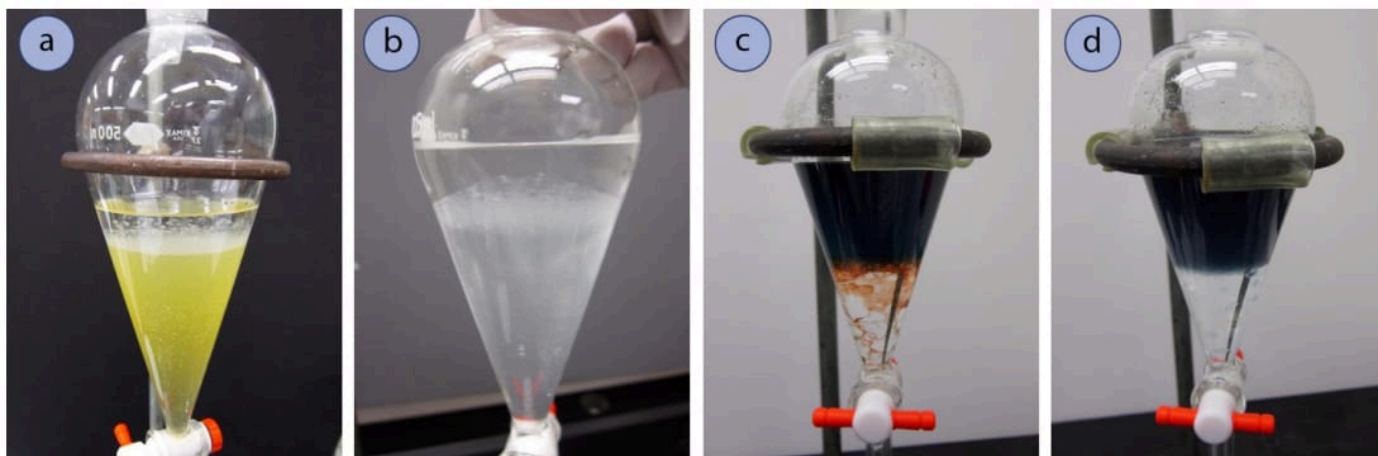
Figure 4.34: a) An emulsion with biodiesel and methanol, b) An emulsion with brine and ethyl acetate, c) An emulsion with dichloromethane and brine (as well as food coloring), d) The emulsion is resolved after addition of water that decreases the density of the top brine layer.
