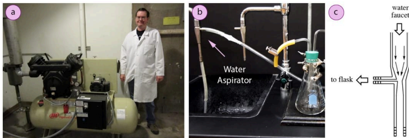
Figure 1.73: a) House vacuum system at Butte College, b) Water aspirator (indicated with an arrow), c) Diagram of an aspirator.
