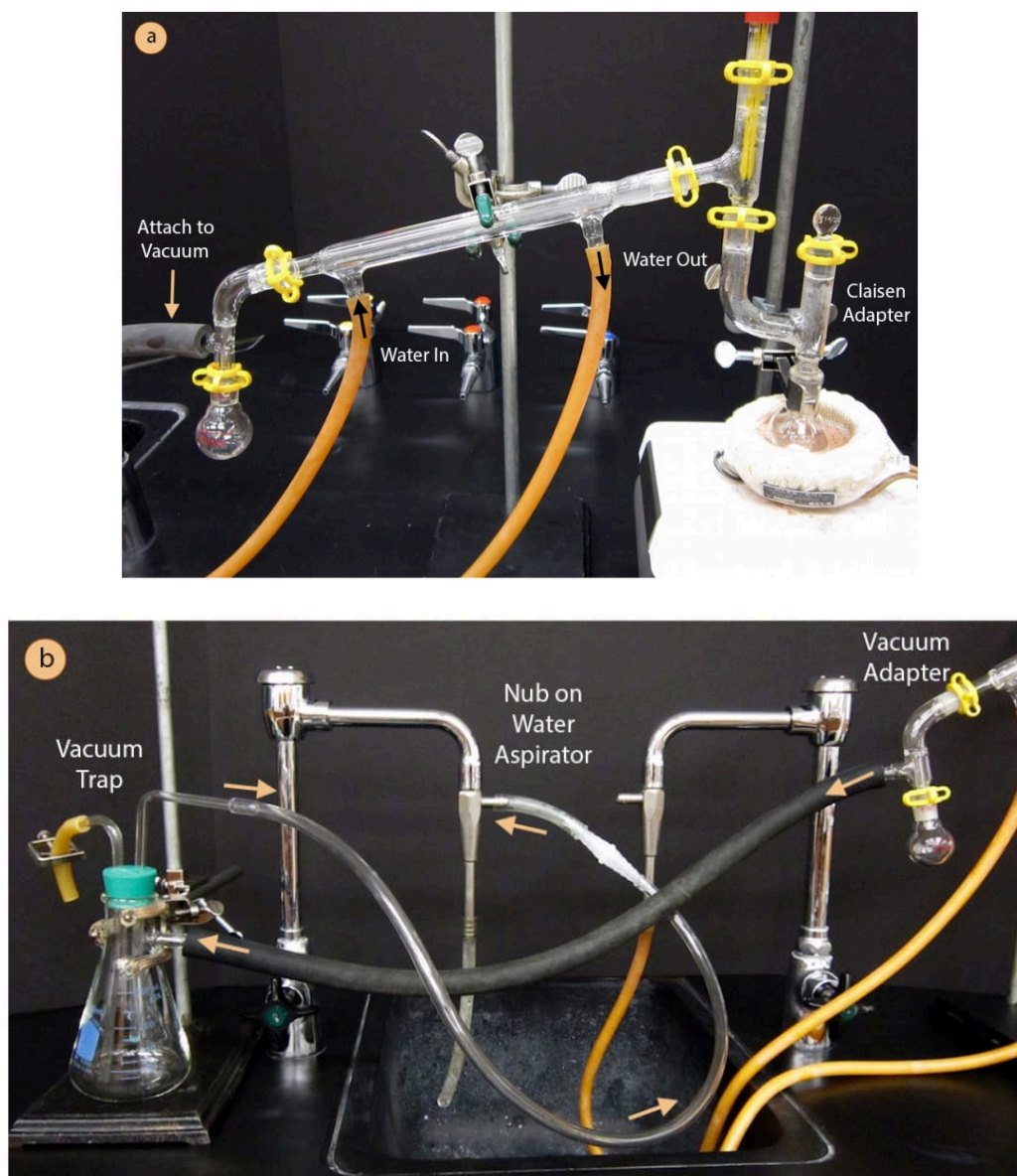
Figure 5.50: a) Vacuum distillation setup, b) Apparatus connected to a vacuum trap and water aspirator. Arrows show direction of suction.
