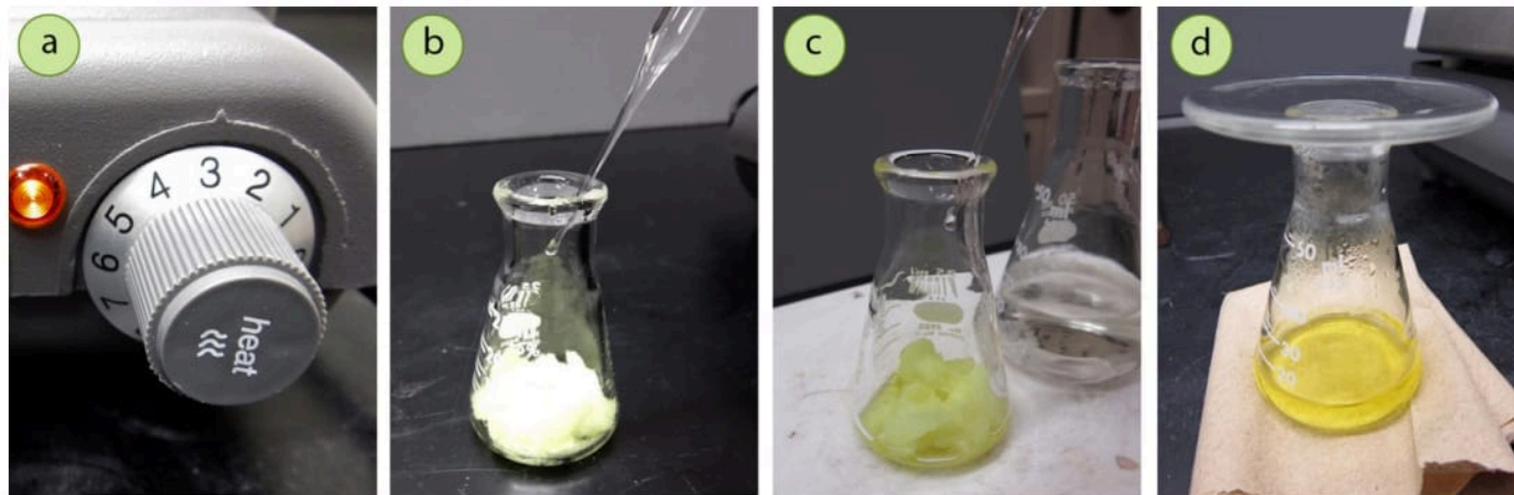
Figure 3.54: a) Hotplate set to low (for ethanol), b+c) Adding solvent via pipette, d) Crystallizing atop some paper towels to encourage slow cooling.
