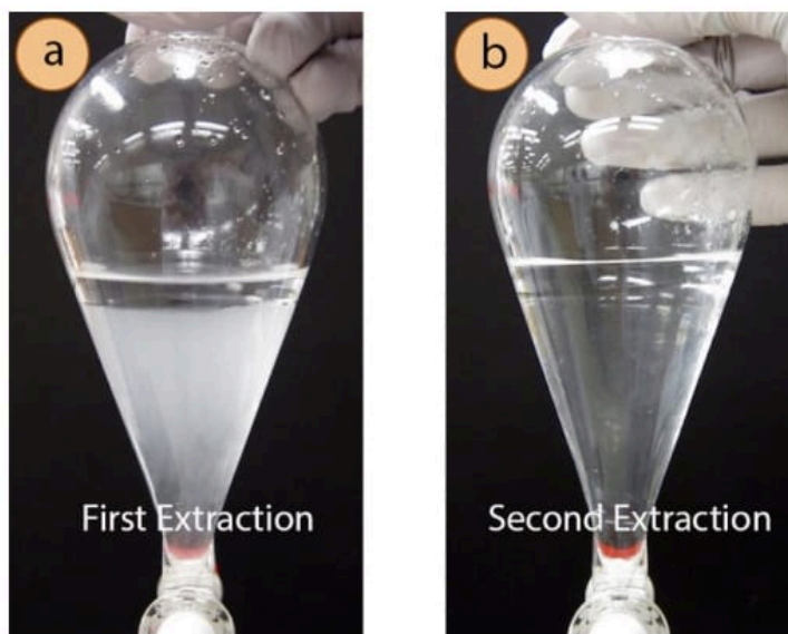
Figure 5.63: a) First extraction of clove oil distillate into ethyl acetate, b) Second extraction.
