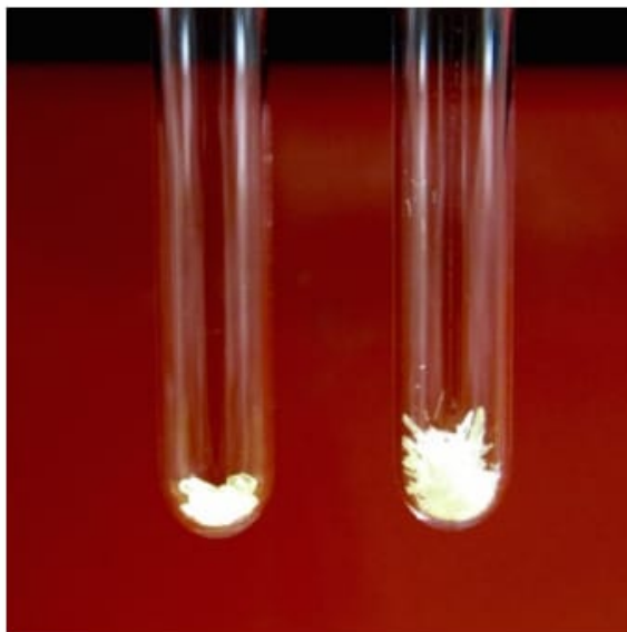
Figure 3.62: Two 6.5 mg samples of benzil: (left) from reagent jar, (right) crystallized sample.
