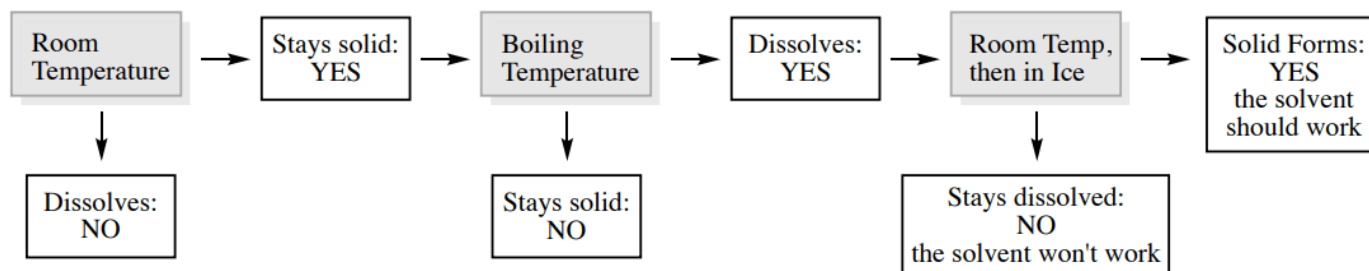
Figure 3.11: Flow chart for testing a crystallization solvent by mixing solid and solvent, as described on this page.
