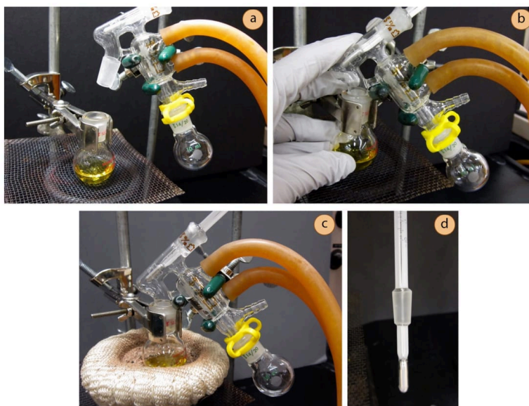
Figure 5.36: a) Clamping prior to assembly, b) Adjusting tightness of the joint, c) Distillation setup, d) Thermometer with ground glass fitting.
