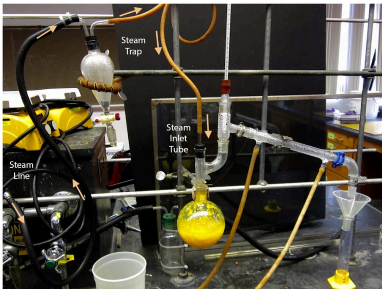
Figure 5.64: Steam distillation apparatus.
