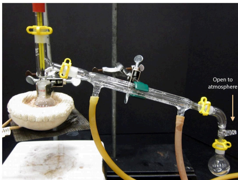
Figure 5.25: Completed simple distillation setup.
