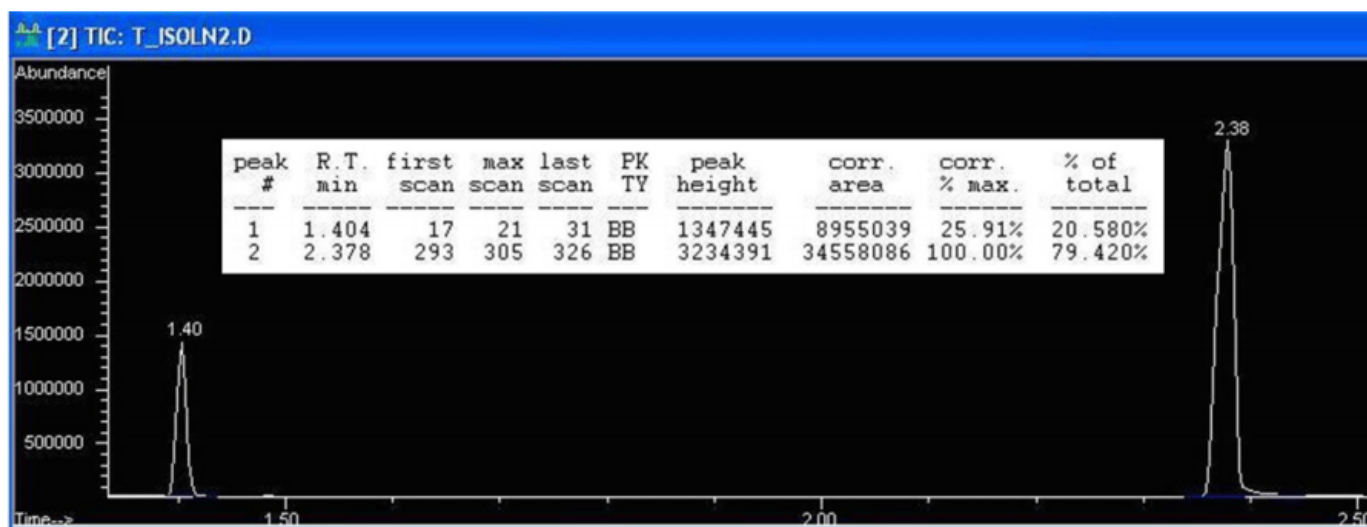
Figure 2.86: GC spectrum generated from a sample that contained equimolar quantities of 2-butanol and 1-heptanol.
