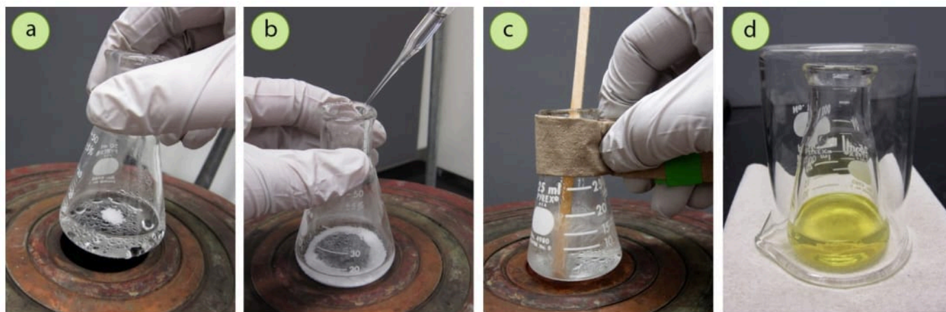
Figure 3.55: a) Hovering a flask above the steam bath , b) Adding solvent by pipette , c) Inevitable vigorous boiling , d) Using an inverted beaker during crystallization .
