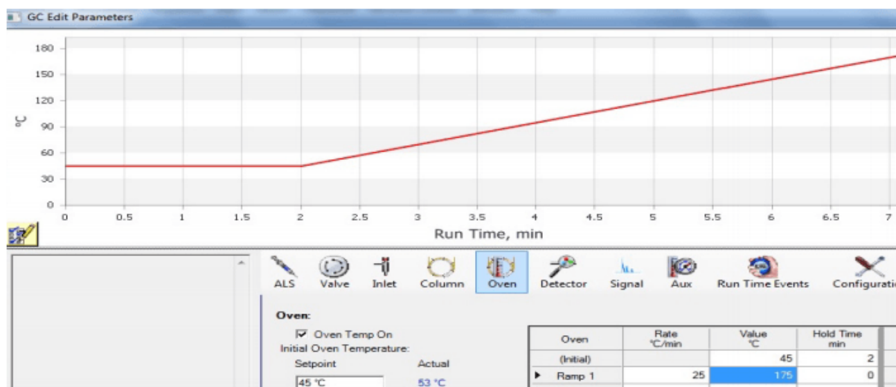
Figure 2.91: Graphical display of the GC method, which includes a "ramp".
