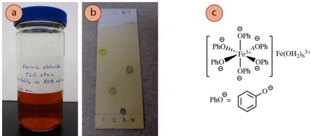
Figure 2.42: a) \text{FeCl}_3 reagent jar, b) TLC plate with various phenols stained with \text{FeCl}_3 , c) Generic phenol- \text{Fe}^{3+} colored complex.
