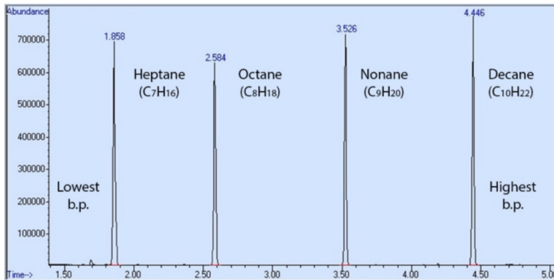
Figure 2.82: GC spectrum of a mixture containing heptane, octane, nonane, and decane (Method: held at 65°C for 2 min, then ramped 25°C/min).
