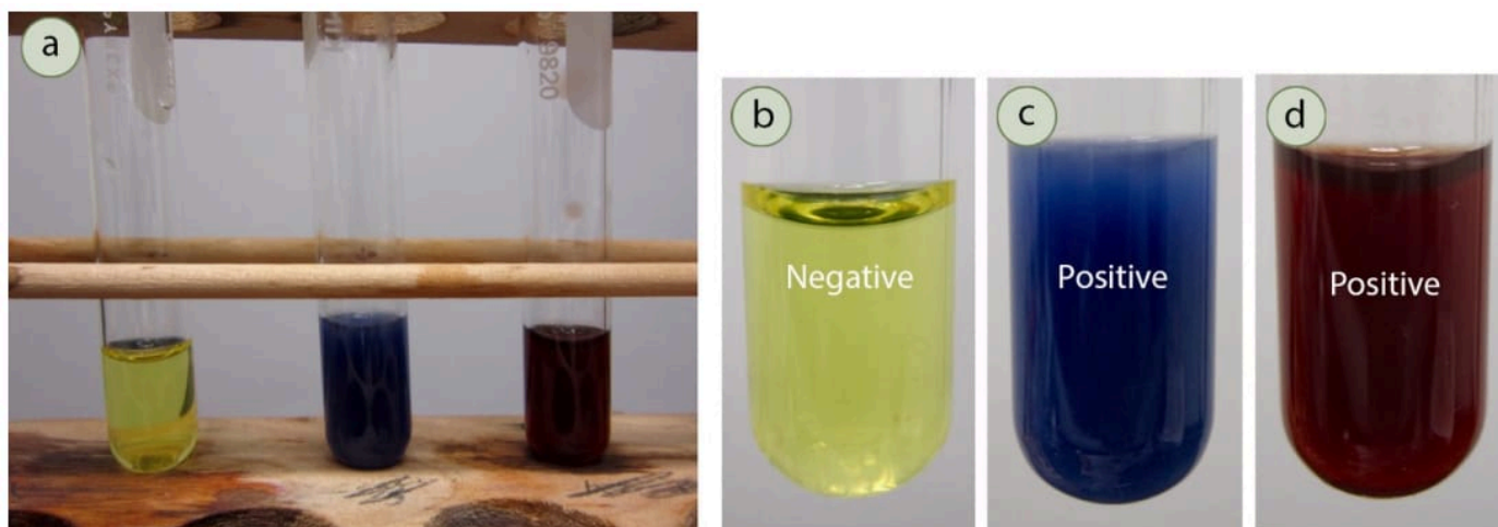
Figure 6.70: a) Phenol test results for (left to right) lactic acid (negative), p-cresol (positive), pyrogallol (positive), b) Negative result, c) Positive result (typical color), d) Positive result (less common color, by pyrogallol, a bidentate ligand).
