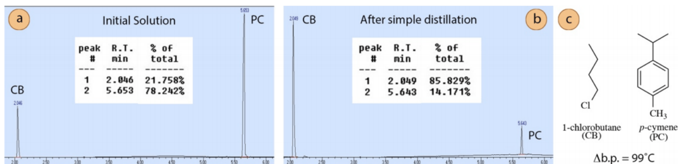
Figure 5.10: a) GC spectrum of a 75 mol% 1-chlorobutane and 25 mol% p-cymene mixture - note GC% need to be interpreted by a calibration curve. 1-chlorobutane is the peak at 2.1 min and p-cymene is the peak at 5.6 min, b) GC spectrum of the distillate from a simple distillation, c) Structures of 1-chlorobutane (CB) and p-cymene (PC).
