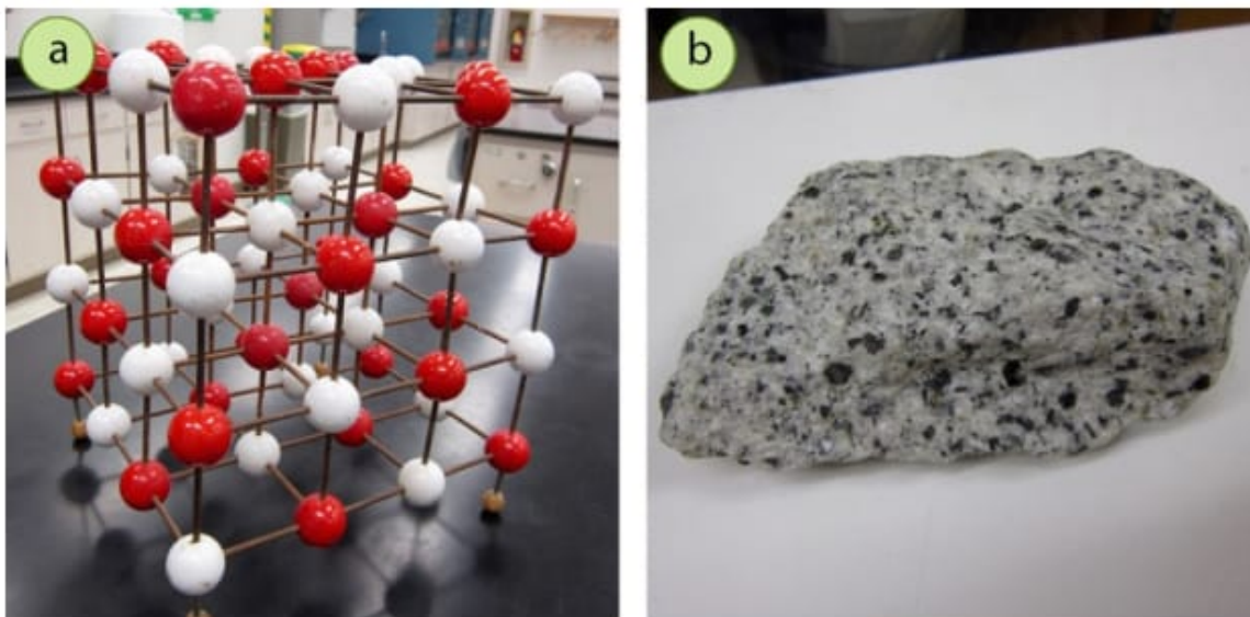
Figure 3.16: a) An example of a crystal lattice (this model is of NaCl), b) Granite, a heterogeneous rock.
