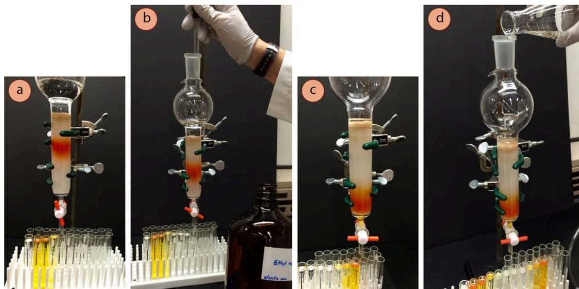
Figure 2.60: a) Elution, b) Addition of ethyl acetate to increase the solvent polarity, c) Solvent level nears the sand layer, d) Refilling.
