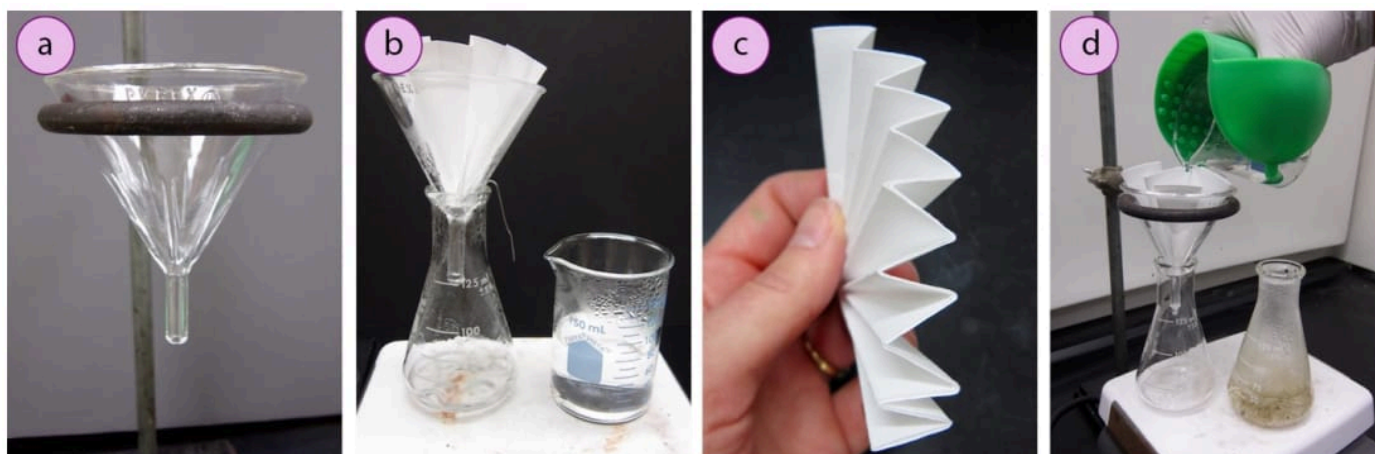
Figure 1.85: a) Short-stemmed funnel, b) If not using a ring clamp, place a bent paper clip between the funnel and Erlenmeyer flask, c) Fluted filter paper (unfolded), d) Pouring solvent through the funnel to get the funnel hot.
