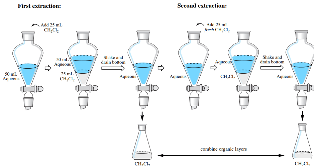
Figure 7.7: Multiple extraction flow-char when the organic layer is on the bottom.
