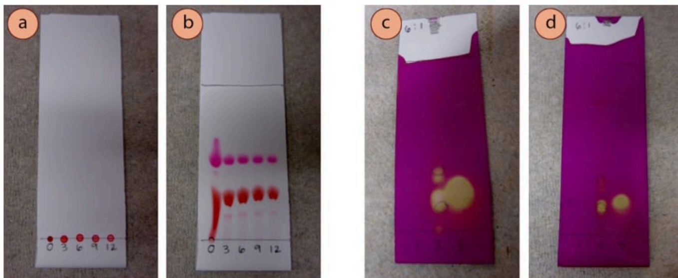
Figure 2.27: a) Before elution of red food dye samples at different aqueous dilutions, b) After elution, c) Alkene and alkyne samples too concentrated (visualized with \text{KMnO}_4 stain), d) Alkene and alkyne samples at proper dilution.
