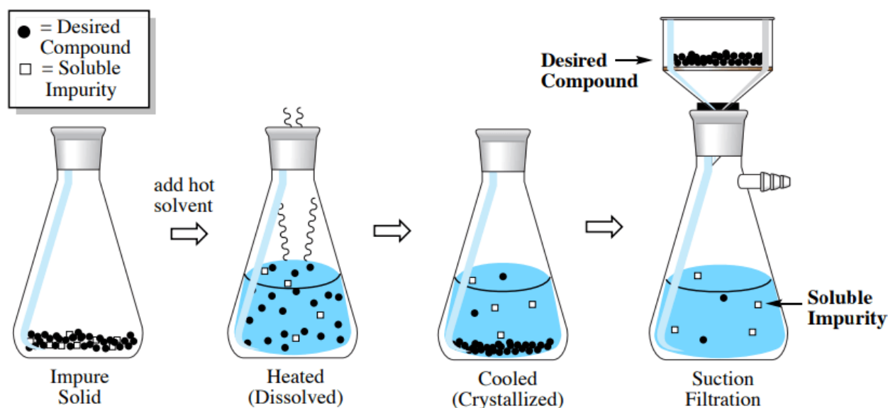
Figure 3.9: Crystallization sequence in order to remove a soluble impurity, using black circles and white squares to represent individual particles. As in reality individual particles are too small to see, the liquids in each of these scenarios would appear completely transparent.
