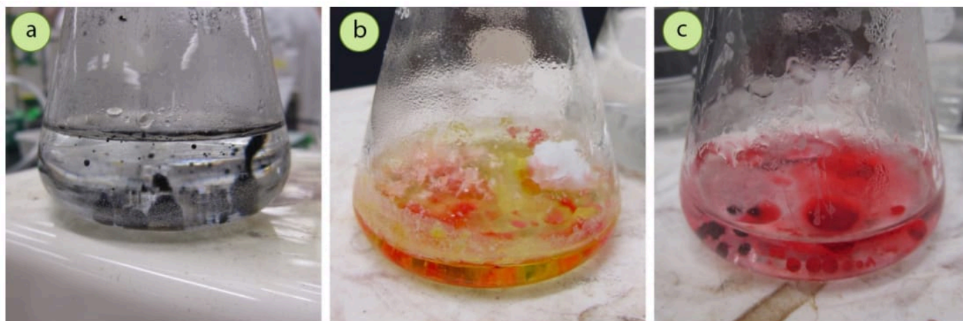
Figure 3.52: Examples of samples "oiling out" during dissolving: a) Oily droplets of acetanilide in a solution decolorized with charcoal, b+c) Oily droplets containing methyl red and acetanilide in water.
