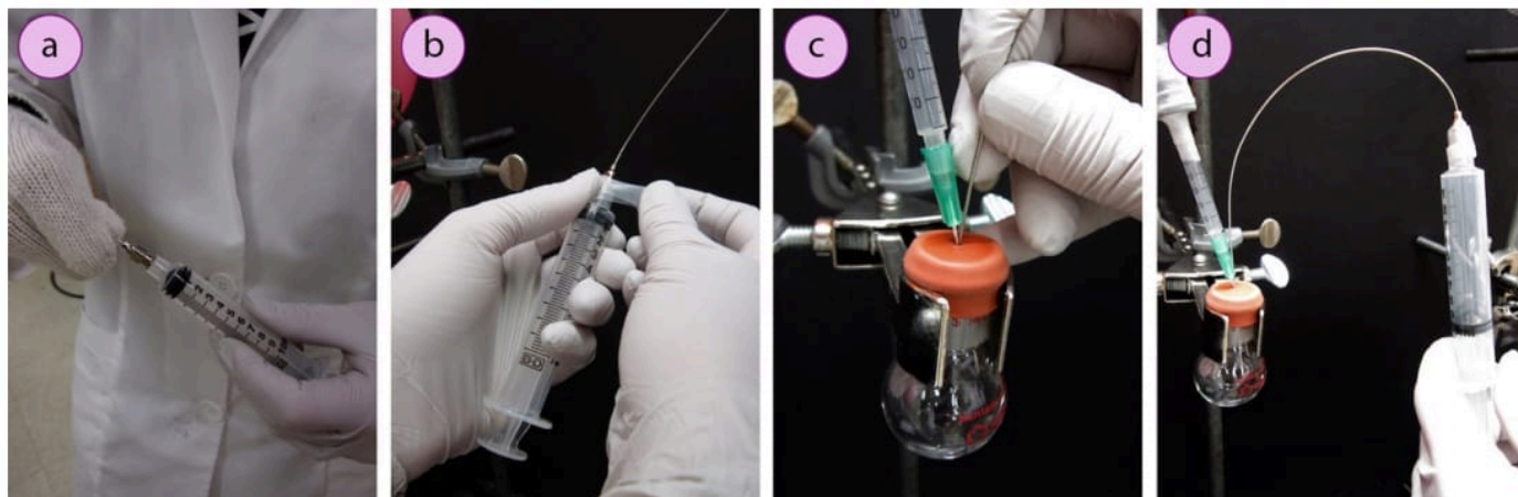
Figure 1.33: a) Screwing the needle onto the syringe head, b) Wrapping the joint with Parafilm, c) Inserting the needle into a flask filled with inert gas, d) Withdrawing inert gas in order to flush the syringe.
