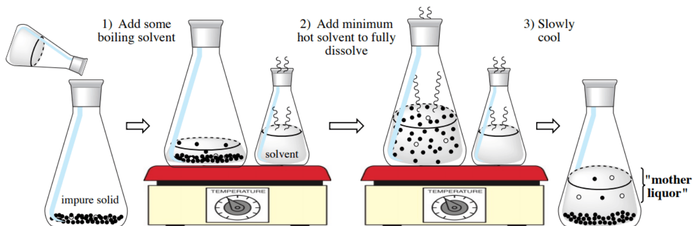
Figure 3.2: Procedural sequence for crystallization.
