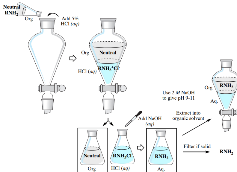
Figure 7.8: Flow-charts for acid-base extraction.
