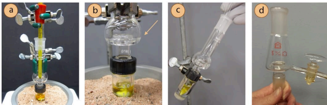
Figure 5.35: a) Microscale distillation using a Hickman head, b) Collection of distillate in the lip of the head (indicated with an arrow), c) Retrieval of the distillate by pipette, d) Hickman head with a side arm port.
