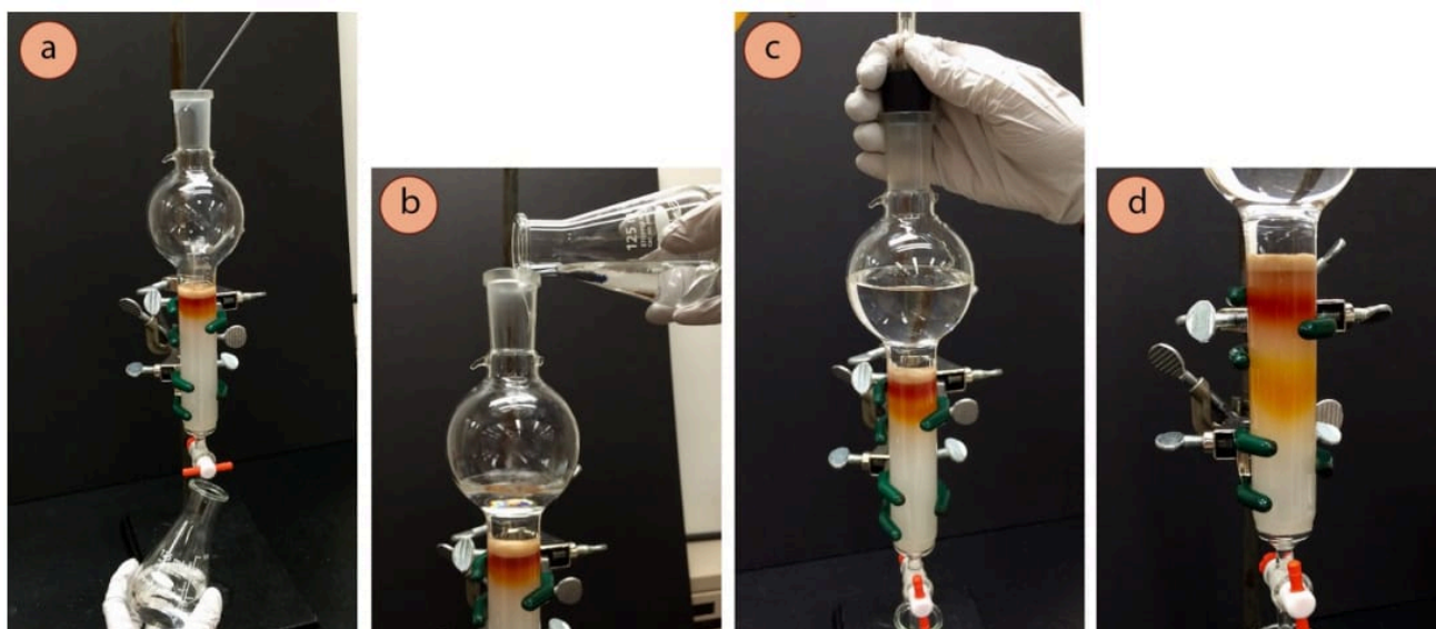
Figure 2.57: a+b) Filling the solvent reservoir, c+d) Eluting the column.
