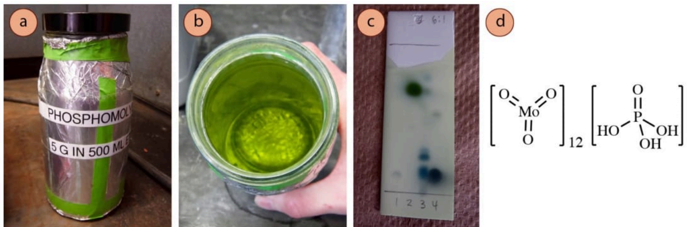
Figure 2.41: a+b) Phosphomolybdic acid reagent jar, c) TLC plate stained with the reagent (#1: benzoic acid, #2: 2,6-di-t-butylphenol, #3: 1-methylcyclohexene - not seen, but impurities stain, #4: benzyl alcohol), d) Formula of phosphomolybdic acid.
