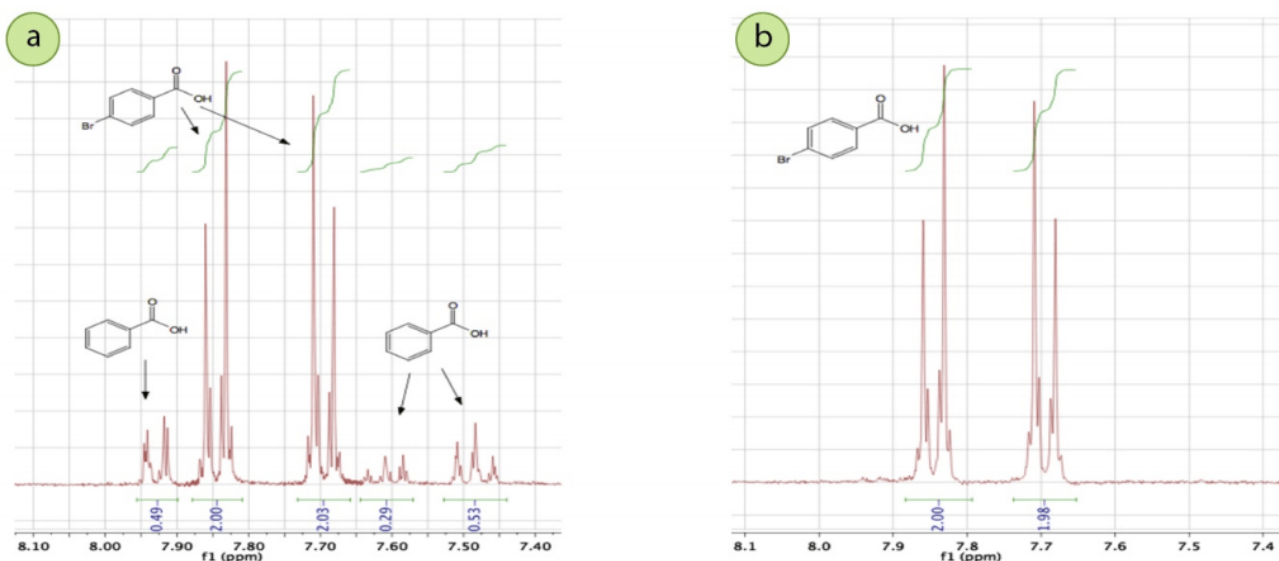
Figure 3.6: a) 300 MHz 1 H NMR spectrum of the crude mixture of benzoic acid and p-bromobenzoic acid (taken in DMSO- d 6 ; carboxylic acid hydrogen is at 13.0 ppm and is not shown), b) 1 H NMR spectrum of solid after crystallization from ethanol, showing the sample is mostly p-bromobenzoic acid.
