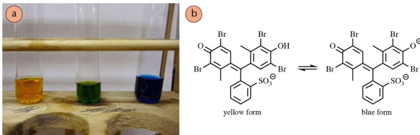
Figure 2.44: a) The colors of the bromocresol green stain (left = very acidic, middle = color of reagent jar, right = higher pH), b) The chemical structures of the yellow and blue forms of bromocresol green.
