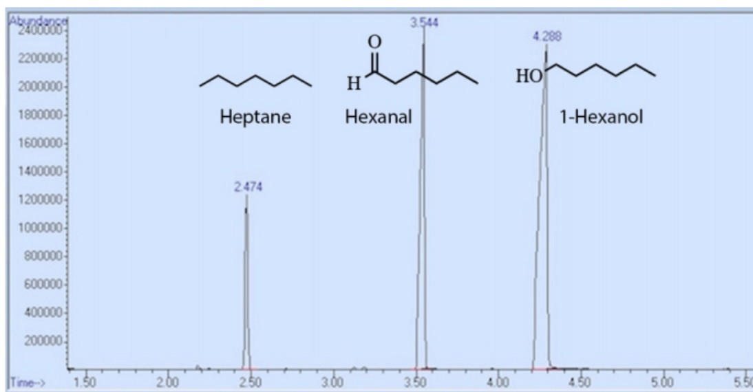
Figure 2.83: GC spectrum of a mixture containing heptane, hexanal, and 1-hexanol.
