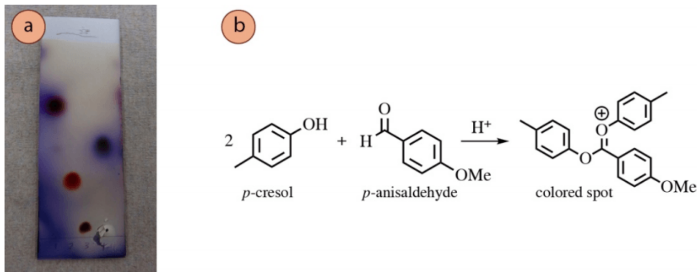
Figure 2.39: a) TLC of various phenols visualized with p -anisaldehyde stain, b) Proposed reaction of p -cresol (lane 2) with the stain.
