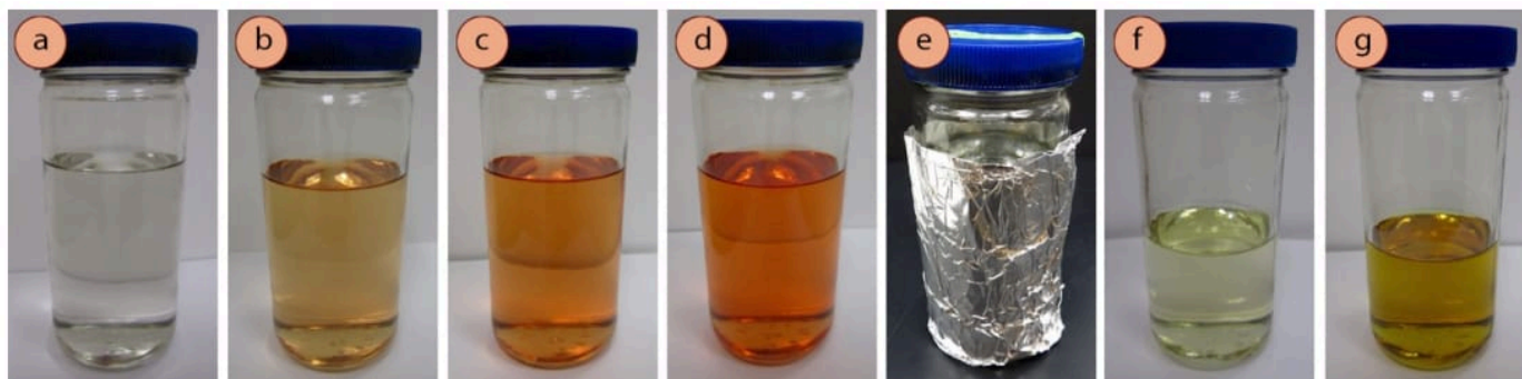
Figure 2.37: a) p -Anisaldehyde stain, within 1 week of preparation, b) After 10 weeks (covered with foil and in the refrigerator), c) After 20 weeks, d) After 30 weeks, e) Stain covered in foil for storage, f) Vanillin stain, as it appeared immediately after preparation, g) After 9 weeks.
