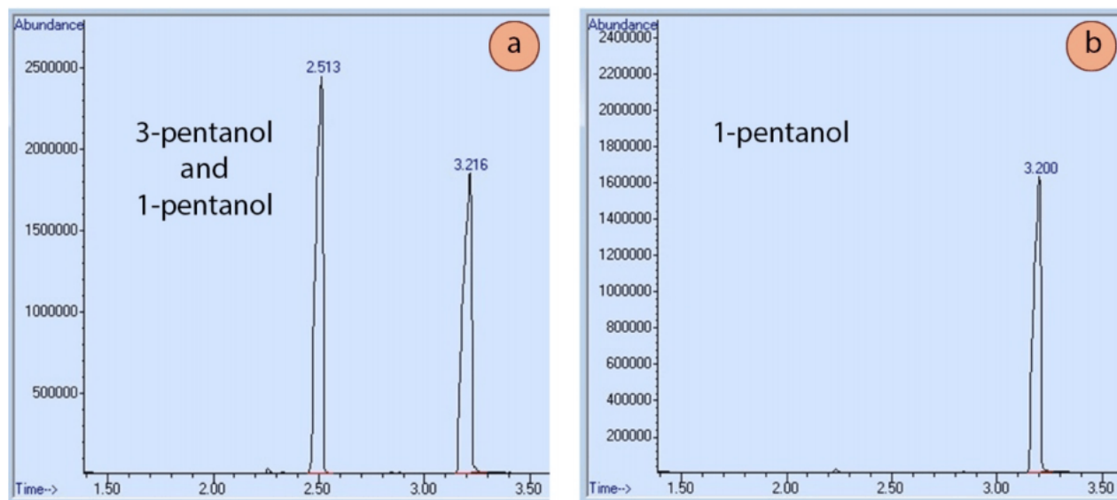
Figure 2.79: a) GC spectrum of a sample containing 3-pentanol and 1-pentanol, b) GC spectrum of pure 1-pentanol.
