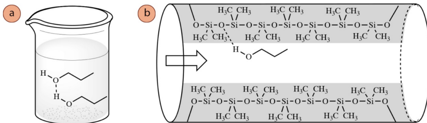
Figure 2.81: a) Hydrogen bonding shown for 1-propanol in the liquid phase, b) Hydrogen bonding shown between 1-propanol and the polymeric coating of the GC column.
