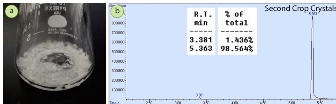
Figure 3.36: a) Second crop of 4-bromoacetophenone crystals coming out of solution, b) GC spectrum of the second crop solid.
