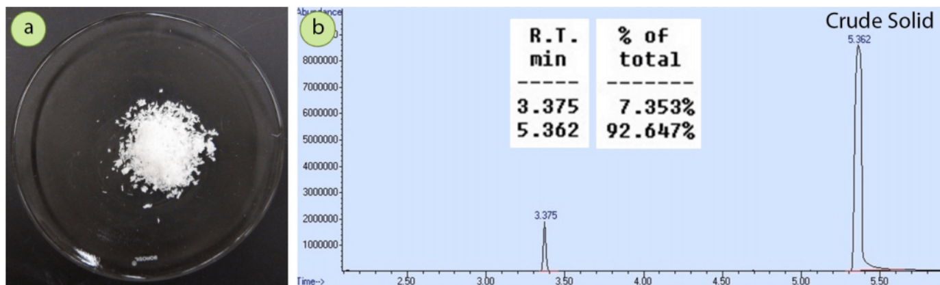
Figure 3.33: a) Initial solid mixture, b) GC spectrum of solid mixture. 13
