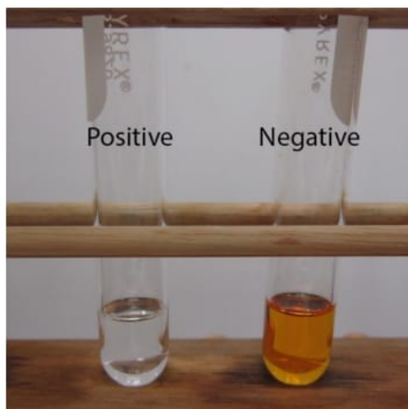
Figure 6.38: Results of two aldehydes in the bromine test (left tube is isobutylaldehyde and right tube is benzaldehyde).
