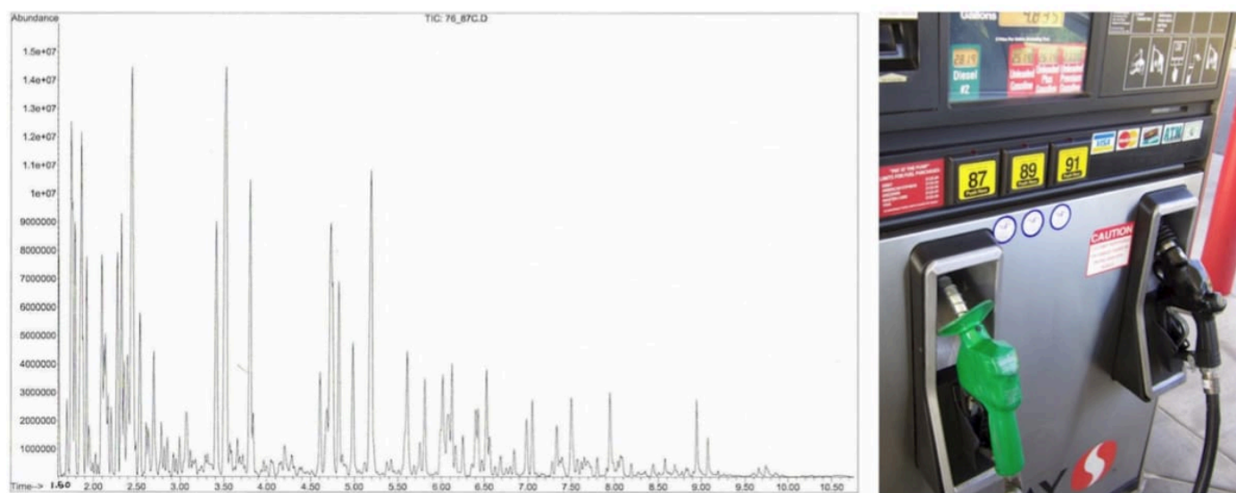
Figure 2.76: GC spectrum of 87 octane gasoline.
