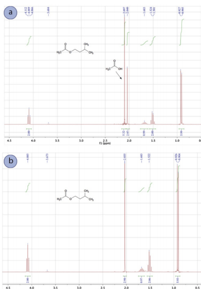
Figure 4.39: 300 MHz 1 H NMR spectra of the Fischer esterification mixture, a) Before the work-up, b) After the complete work-up (water, sodium bicarbonate, and brine washes).
