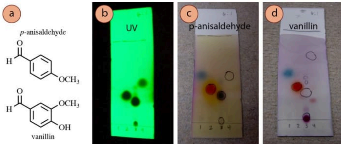
Figure 2.36: a) Structures of p -anisaldehyde and vanillin. 4-Heptanone (lane 1), acetophenone (lane 2), cinnamaldehyde (lane 3), and ethyl benzoate (lane 4) visualized with: b) UV light, c) p -Anisaldehyde stain, d) Vanillin stain.
