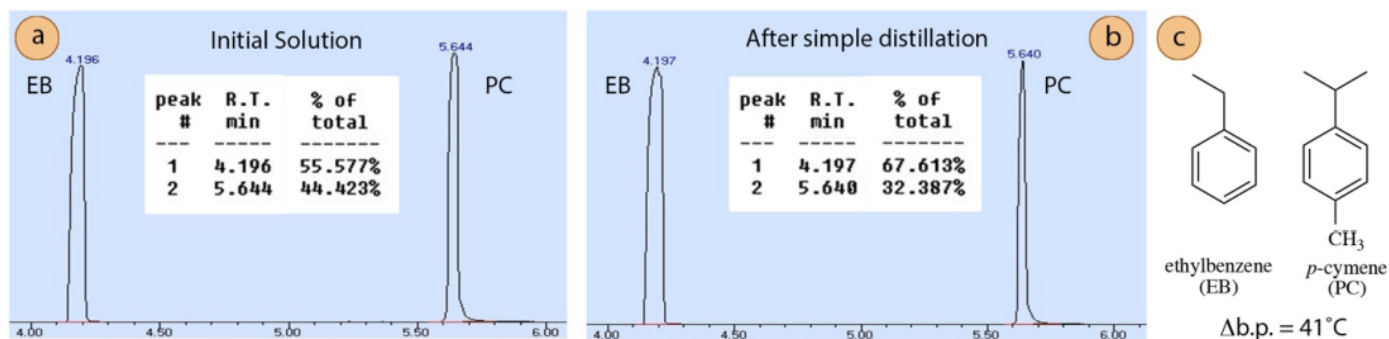
Figure 5.12: a) GC spectrum of a 75 mol% ethylbenzene and 25 mol% p -cymene mixture, note GC% need to be interpreted by a calibration curve. Ethylbenzene is the peak at 4.2 min and p -cymene is the peak at 5.6 min, b) GC spectrum of the distillate, c) Structures of ethylbenzene (EB) and p -cymene (PC).
