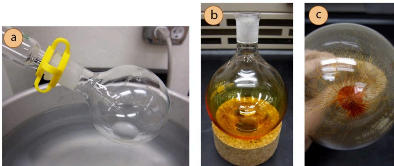
Figure 5.71: a) Residual liquid after evaporation, b) A sample after evaporation that left a film on the flask, c) The sample sample that crystallized after allowing the flask to dry overnight.
