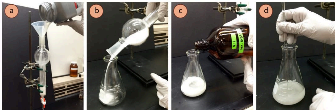
Figure 2.53: a) Pouring in silica to 5-6" high in the fume hood, b) Pouring the silica into an Erlenmeyer flask, c+d) Making a slurry.
