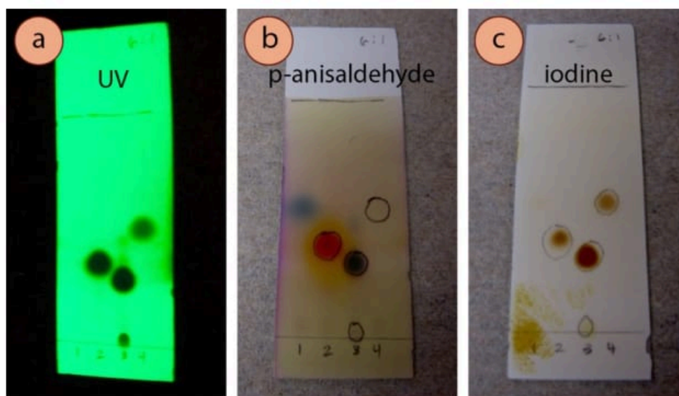
Figure 2.46: Four compounds eluted with 6:1 hexanes:ethyl acetate and visualized with 3 methods: a) UV, b) p -anisaldehyde, c) iodine 7 . The compounds were: #1: 4-heptanone, #2: acetophenone, #3: cinnamaldehyde, and #4: ethyl benzoate.
