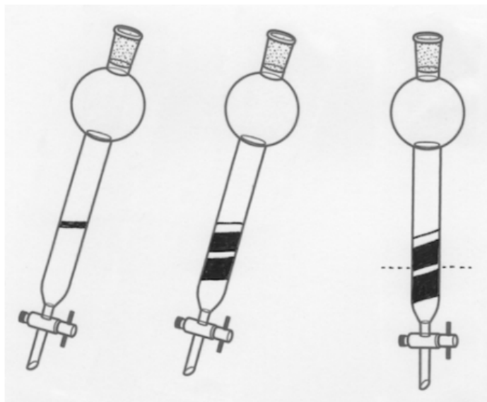
Figure 2.67: Effect of a crooked column on separation.
