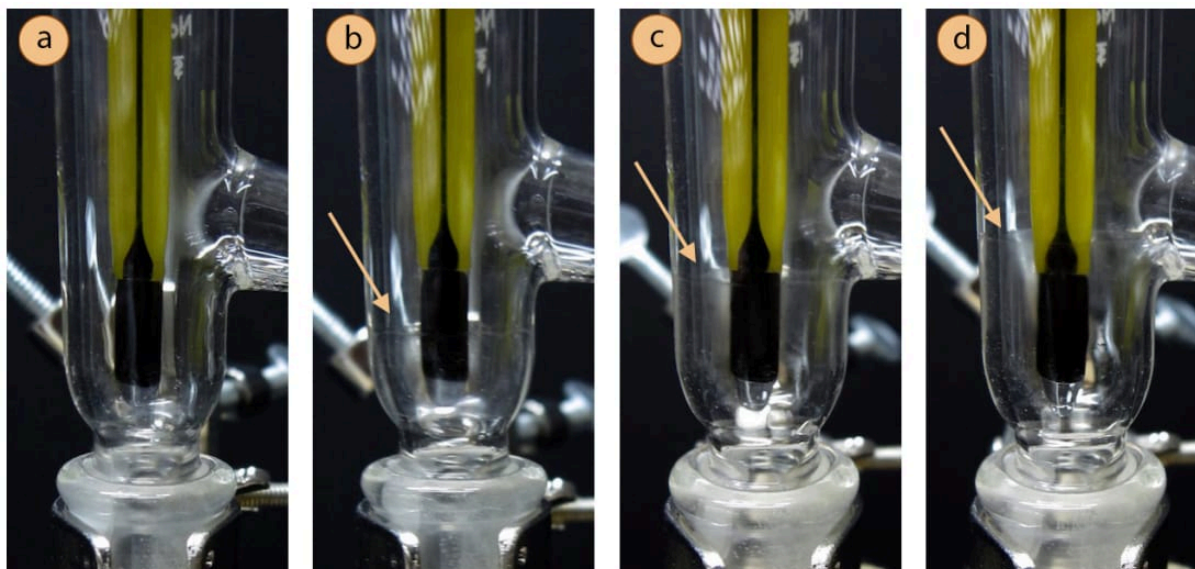
Figure 5.27: Gradual ascension of the vapor ring (pointed to with an arrow in each progression), to immerse the thermometer. Note: not all compounds behave in this manner.
