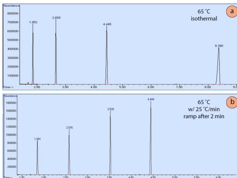
Figure 2.92: A sample composed of heptane, octane, nonane, and decane, run with two different GC methods. a) The run was kept under isothermal conditions, at a steady 65 °C, b) The method utilized a "ramp" after 2 minutes.
