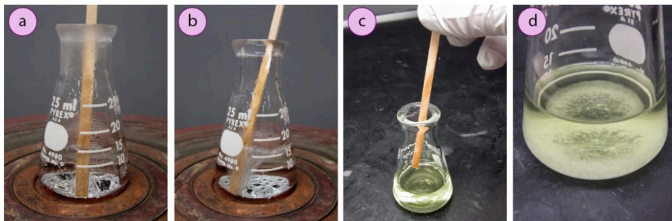
Figure 1.41: Use of a wood splint to promote smooth boiling, a+b) Bubbles originating from the wood splint, c) Removal of the splint before crystallization, d) Crystallization.
