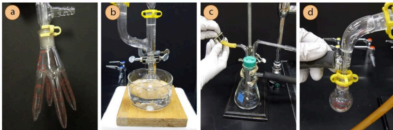
Figure 5.53: a) "Cow" receiving flask for collecting multiple fractions: when a new fraction is distilling, the flask is rotated to allow for the distillate to collect into an empty section of the "udder", b) Cooling the flask with a tap water bath, c) Opening the vacuum on the trap before turning off the vacuum, d) Alternative way to open the apparatus before turning off the vacuum.
