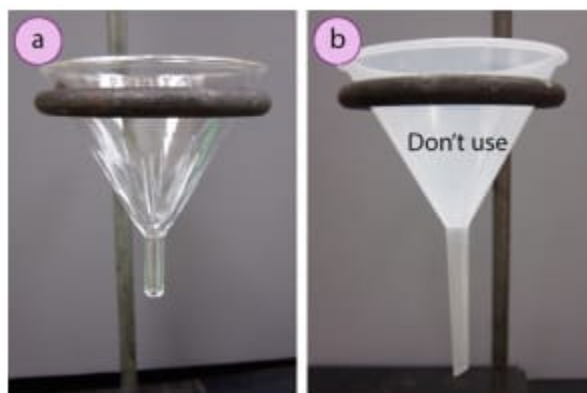
Figure 1.83: a) Short-stemmed funnel, b) Long-stemmed funnel (don't use for hot filtration).
