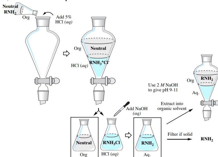
Figure 4.59: Flowchart for separating a mixture containing acidic, basic, and neutral components.
