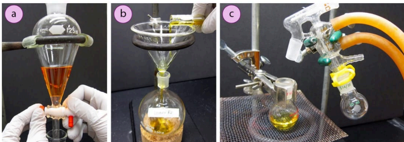
Figure 1.6: Using ring clamps for: a) Holding separatory funnels, b) Holding funnels, c) Assembly of an adjustable platform.
