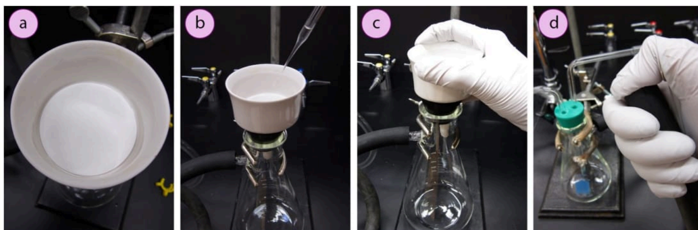
Figure 1.76: a) Filter paper in the funnel, b) Wetting the filter paper with solvent, c) Pressing the Buchner funnel to create a good seal, d) Testing the suction of the aspirator.
