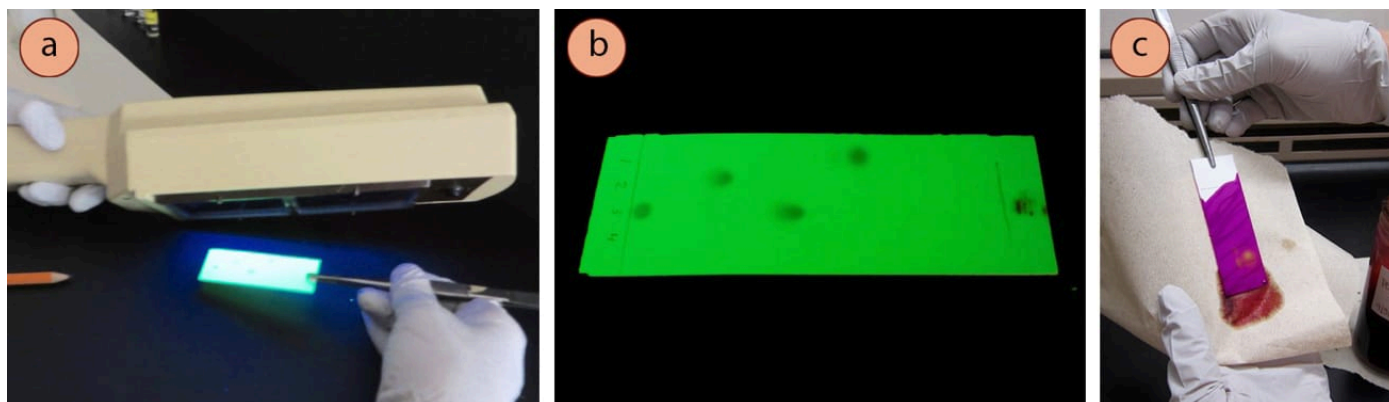
Figure 2.6: a) Visualization of a TLC plate using UV light, b) Compounds appear dark against a fluorescent green background, c) Use of a chemical stain to visualize a plate.
