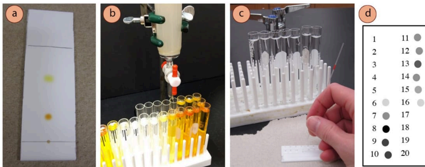
Figure 2.61: a) Original TLC plate, b) Fractions collected by the column, c) Spotting fractions onto a TLC plate, d) A visualized TLC plate of samples of each fraction.
