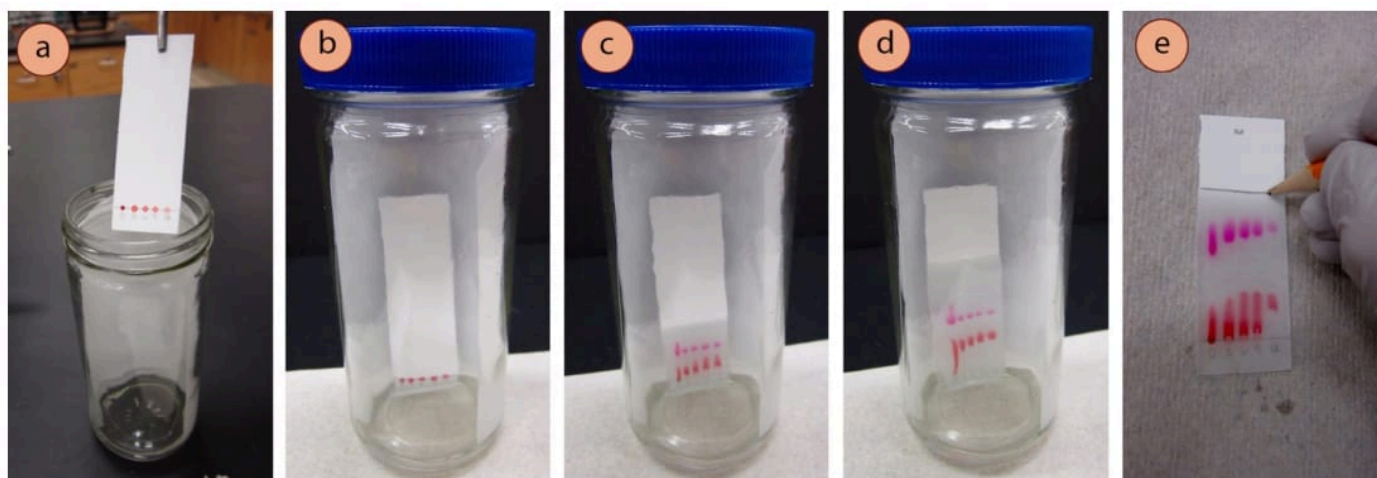
Figure 2.26: a) Using forceps to place the TLC plate into the chamber, b-d) Elution, e) Marking the solvent line with a pencil.
