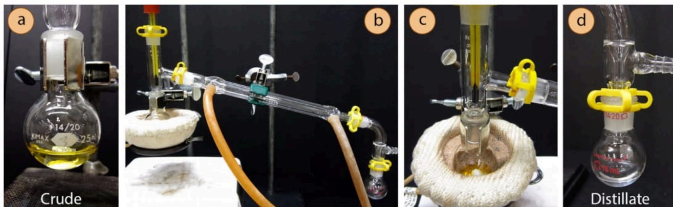
Figure 5.6: a) Crude yellow isoamyl acetate formed from a Fischer esterification, b+c) Simple distillation, d) Colorless distillate.
