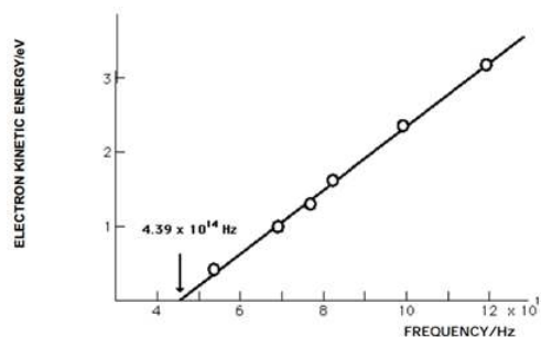
Figure 1.6. Photoelectric data for sodium (Millikan, 1916). The threshold frequency \nu_0 , found by extrapolation, equals 4.39 \times 10^{14} Hz.
