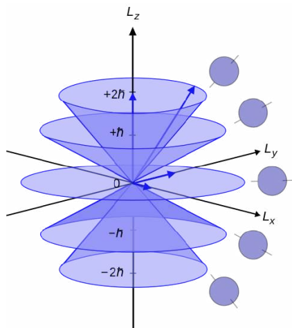
Figure 6.5: Vector model for angular momentum, showing the case \ell = 2 . (Public Domain; Maschen).
