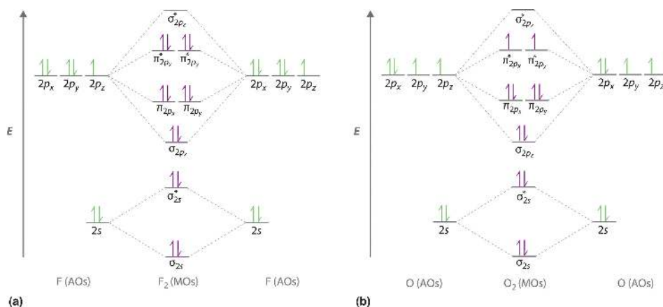
Figure 11.4: Molecular Orbital Energy-Level Diagrams for Homonuclear Diatomic Molecules. (a) For F 2 , with 14 valence electrons (7 from each F atom), all of the energy levels except the highest, \sigma_{2p}^* , are filled. This diagram shows 8 electrons in bonding orbitals and 6 in antibonding orbitals, resulting in a bond order of 1. (b) For O 2 , with 12 valence electrons (6 from each O atom), there are only 2 electrons to place in the (\pi_{2p}^*, \pi_{2p}^*) pair of orbitals. Hund's rule dictates that one electron occupies each orbital, and their spins are parallel, giving the O 2 molecule two unpaired electrons. This diagram shows 8 electrons in bonding orbitals and 4 in antibonding orbitals, resulting in a predicted bond order of 2.
