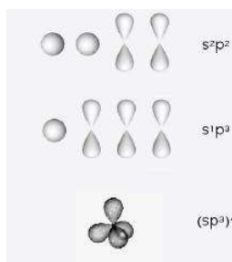
Figure 10.4. Promotion and hybridization of atomic orbitals in carbon atom.
