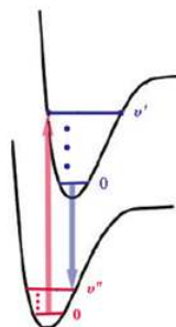
Figure 7. Franck-Condon principle
