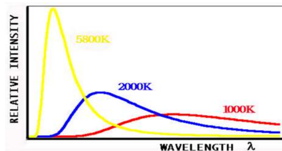
Figure 1.5. Intensity distributions of blackbody radiation at three different temperatures. The total radiation intensity varies as T^4 (Stefan-Boltzmann law) so the total radiation at 2000K is actually 2^4 = 16 times that at 1000K.
