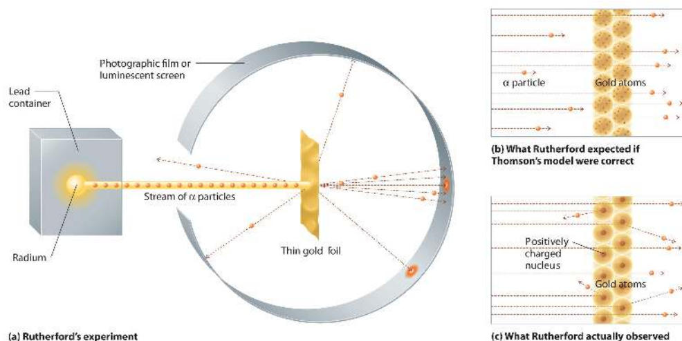
Figure 1.2: A Summary of Rutherford's Experiments (a) A representation of the apparatus Rutherford used to detect deflections in a stream of \alpha particles aimed at a thin gold foil target. The particles were produced by a sample of radium. (b) If Thomson's model of the atom were correct, the \alpha particles should have passed straight through the gold foil. (c) But a small number of \alpha particles were deflected in various directions, including right back at the source. This could be true only if the positive charge were much more massive than the \alpha particle. It suggested that the mass of the gold atom is concentrated in a very small region of space, which he called the nucleus.
