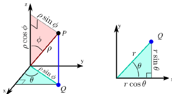
Figure 6.2: Spherical coordinates.
