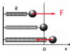
Figure 5.1: Spring obeying Hooke's law.
