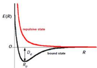
Figure 10.2. Energy curves for a diatomic molecule.
