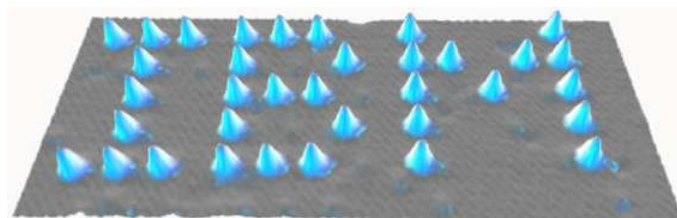
Figure 1.1: Image showing electron clouds of individual xenon atoms on a nickel(110) surface produced by a scanning tunneling microscope at IBM Laboratories.
