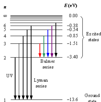
Figure 7.7: Energy levels of atomic hydrogen. Taken from http://eilat.sci.brooklyn.cuny.edu/c...hws/hw2d_c.htm
