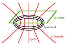
Figure 11.1: Prolate spheroidal coordinates.
