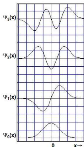
Figure 5.3: Harmonic oscillator eigenfunctions for n=0, 1, 2, 3 .
