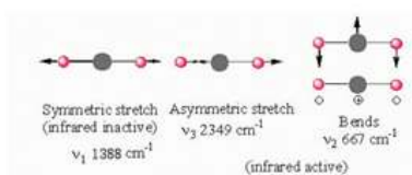
Figure 4. Normal modes of CO 2 .
