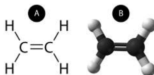
Figure 10.4.3: (A) The structural model for C_2H_4 consists of a double covalent bond between the two carbon atoms and single bonds to the hydrogen atoms. (B) Molecular model of C_2H_4 .
