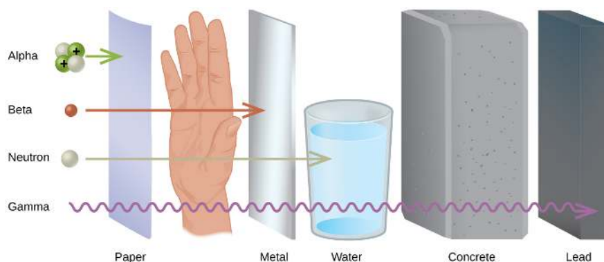
Figure 11.9.4: The ability of different types of radiation to pass through material is shown. From least to most penetrating, they are \alpha < \beta < \text{neutron} < \gamma .
