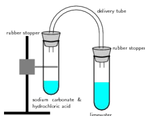
Figure 7.7.1: Reaction of acids with carbonates. In this reaction setup, lime water (water + calcium hydroxide) is poured into one of the test tubes and sealed with a stopper. A small amount of hydrochloric acid is carefully poured into the remaining test tube. A small amount of sodium carbonate is added to the acid, and the tube is sealed with a rubber stopper. The two tubes are connected. As a result of the acid-carbonate reaction, carbon dioxide is produced and the lime water turns milky.
