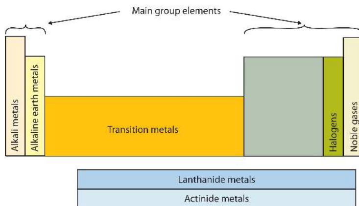
Figure 4.7.3: Special Names for Sections of the Periodic Table. (CC BY-NC-SA; Anonymous by request)
