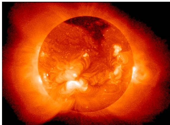
Figure 11.6.3: The energy that comes from the sun and other stars is produced by fusion. (Public Domain; NASA.)
