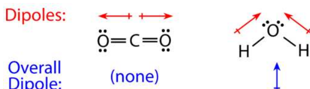
Figure 10.8.7: The molecular geometry of a molecule affects its polarity. Each CO bond has a dipole moment, but they point in opposite directions so that the net CO 2 molecule is nonpolar. In contrast, water is polar because the OH bond moments do not cancel out.
