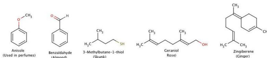
Figure 16.1.3: Different order receptor molecules. (CC0; C5perez via Wikipedia )
