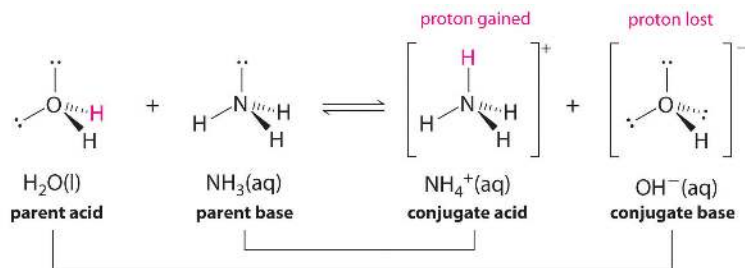
Figure 15.4.1. The pairing of parent acids and bases with conjugate acids and bases.
