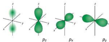
Figure 9.5.2: p orbitals have an orientational preference and resemble dumbbells.
