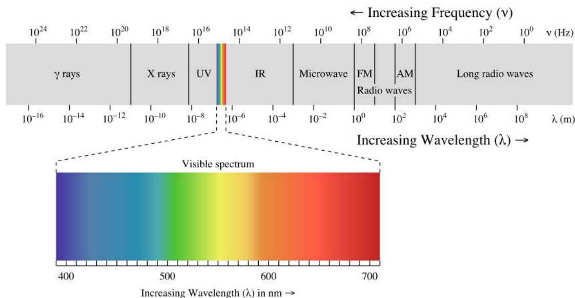
Figure 9.2.1: The electromagnetic spectrum, with its various regions labeled. The borders of each region are approximate. (CC BY-NC-SA; anonymous by request).
