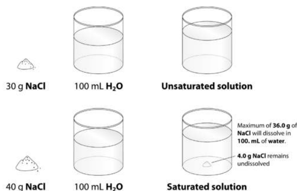
Figure 14.3.1: When 30.0 g of NaCl is added to 100 mL, it all dissolves, forming an unsaturated solution. When 40.0 g is added, 36.0 g dissolves and 4.0 g remains undissolved, forming a saturated solution.
