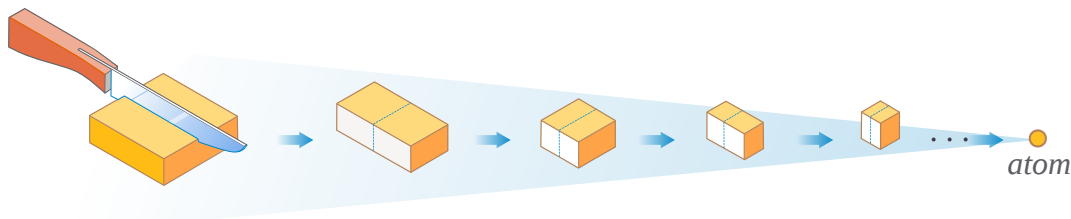
Figure 4.1.1: Democritus argued that matter, like an aluminum block, cannot be repeatedly cut in half perpetually. At some point, a limit is reached before the substance can no longer be called "aluminum"; this is the atomic limit. (CC BY-NC; Ümit Kaya via LibreTexts)
