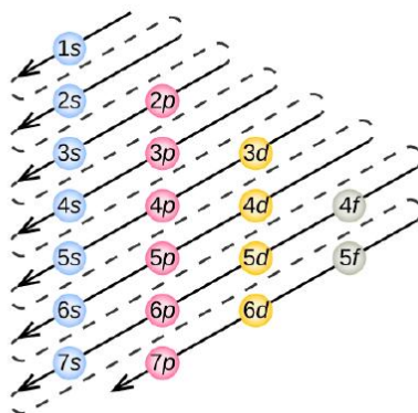
Figure 9.5.6: The arrow leads through each subshell in the appropriate filling order for electron configurations. This chart is straightforward to construct. Simply make a column for all the s orbitals with each n shell on a separate row. Repeat for p, d, and f. Be sure to only include orbitals allowed by the quantum numbers (no 1p or 2d, and so forth). Finally, draw diagonal lines from top to bottom as shown.
