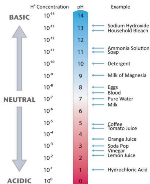
Figure 15.9.1: The pH values for several common materials.
