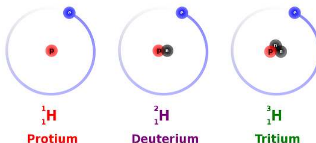
Figure 4.9.1: The three most stable isotopes of hydrogen: protium ( A = 1 ), deuterium ( A = 2 ), and tritium ( A = 3 ). (CC SA-BY 3.0; Balajijagadesh via Wikipedia).
