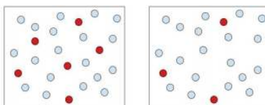
Figure 14.5.1: The solution on the left is more concentrated than the solution on the right because there is a greater ratio of solute (red balls) to solvent (blue balls) particles. The solution particles are closer together. The solution on the right is more dilute (less concentrated). (CC-SA-BY-3.0 Tracy Poulsen).
