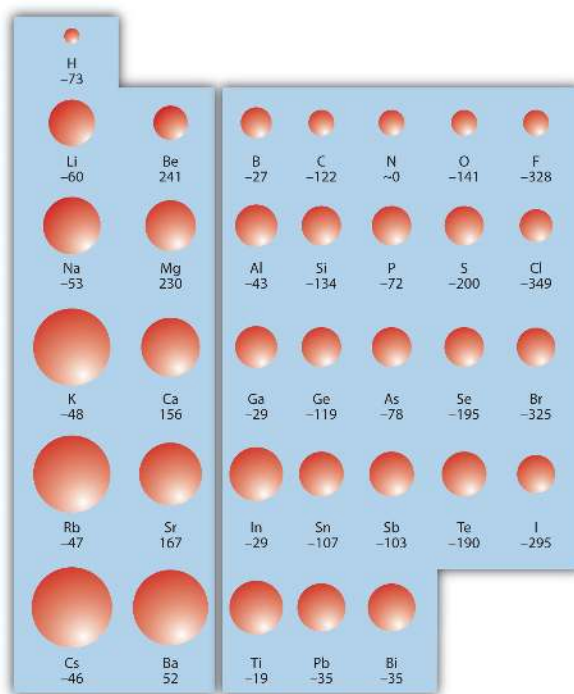
Figure 9.8.3: Electron Affinity on the Periodic Table. Values are in kJ/mol.
