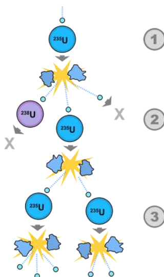
Figure 11.6.2: A possible nuclear fission chain reaction. 1. A uranium-235 atom absorbs a neutron, and fissions into two new atoms (fission fragments), releasing three new neutrons and a large amount of binding energy. 2. One of those neutrons is absorbed by an atom of uranium-238, and does not continue the reaction. Another neutron leaves the system without being absorbed. However, one neutron does collide with an atom of uranium-235, which then fissions and releases two neutrons and more binding energy. 3. Both of those neutrons collide with uranium-235 atoms, each of which fissions and releases a few neutrons, which can then continue the reaction. (Public Domain.)
