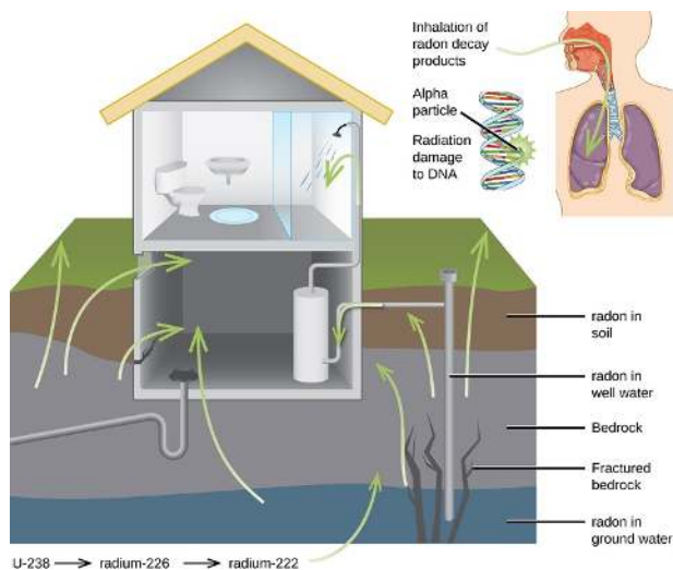
Figure 11.9.5: Radon-222 seeps into houses and other buildings from rocks that contain uranium-238, a radon emitter. The radon enters through cracks in concrete foundations and basement floors, stone or porous cinderblock foundations, and openings for water and gas pipes.
