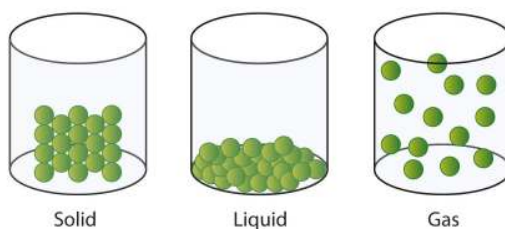
Figure 13.2.3: A Representation of the Solid, Liquid, and Gas States. A solid has definite volume and shape, a liquid has a definite volume but no definite shape, and a gas has neither a definite volume nor shape.
