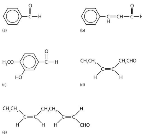
Figure 16.14.2 Some Interesting Aldehydes. (a) Benzaldehyde is an oil found in almonds; (b) cinnamaldehyde is oil of cinnamon; (c) vanillin gives vanilla its flavor; (d) cis-3-hexenal provides an herbal odor; and (e) trans-2-cis-6-nonadienal gives a cucumber odor.
