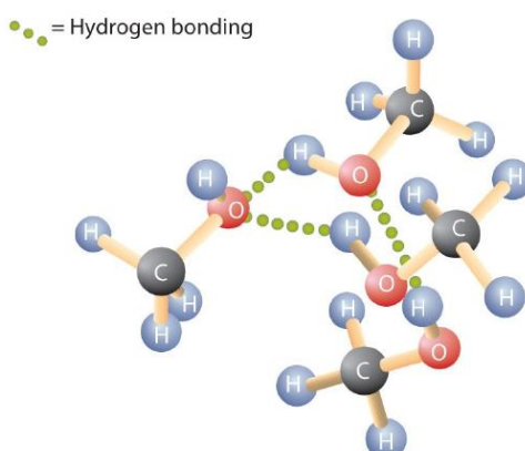
Figure 16.12.1: Intermolecular Hydrogen Bonding in Methanol. The OH groups of alcohol molecules make hydrogen bonding possible.
