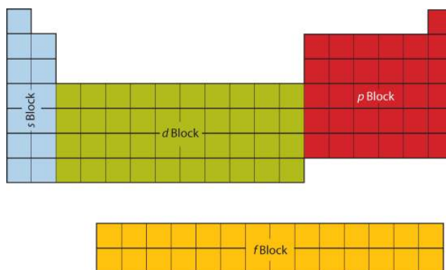
Figure 9.6.9: Blocks on the Periodic Table. The periodic table is separated into blocks depending on which subshell is being filled for the atoms that belong in that section.
