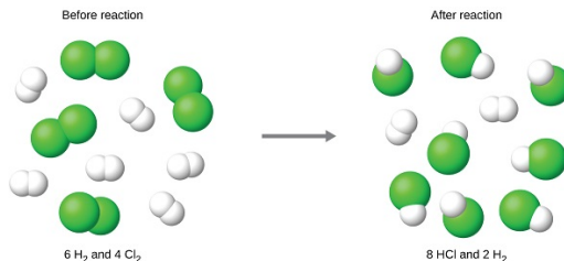
Figure 8.6.2: When H_2 and Cl_2 are combined in nonstoichiometric amounts, one of these reactants will limit the amount of HCl that can be produced. This illustration shows a reaction in which hydrogen is present in excess and chlorine is the limiting reactant. The figure shows a space-filling molecular models reacting. There is a reaction arrow pointing to the right in the middle. To the left of the reaction arrow there are three molecules each consisting of two green spheres bonded together. There are also five molecules each consisting of two smaller, white spheres bonded together. Above these molecules is the label, "Before reaction," and below these molecules is the label, "6 H subscript 2 and 4 Cl subscript 2." To the right of the reaction arrow, there are eight molecules each consisting of one green sphere bonded to a smaller white sphere. There are also two molecules each consisting of two white spheres bonded together. Above these molecules is the label, "After reaction," and below these molecules is the label, "8 H C l and 2 H subscript 2."
