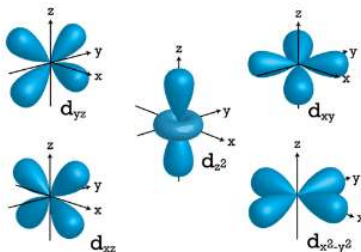
Figure 9.5.3: d orbitals have an orientational preference and exhibit complex structures.
