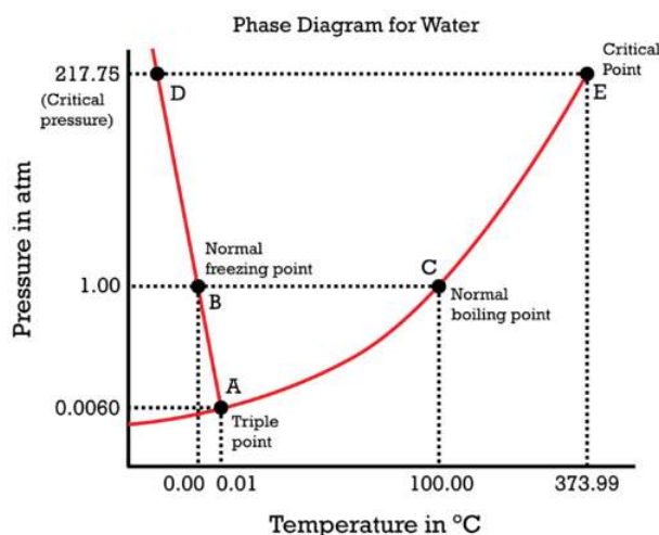
Figure 13.8.1: Phase diagram for water.
