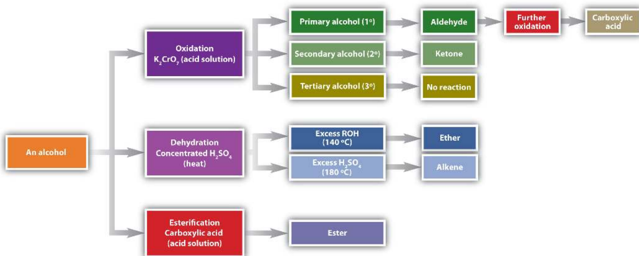
Figure 16.12.1: Reactions of Alcohols. Oxidation and dehydration of alcohols are considered here.
