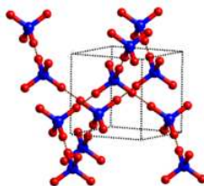
Figure 13.7.4: Ice crystal structure.
