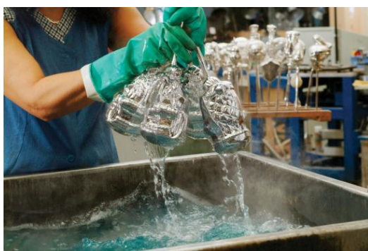
Figure 16.14.1: Aldehyde Reactions. A reaction related to the Tollens' reaction is often used to silver mirrors. These ornaments were silvered by such a reaction. Glucose, a simple sugar with an aldehyde functional group, is used as the reducing agent. Source: Photo courtesy of Krebs Glas Lauscha, commons.wikimedia.org/wiki/File:Silvering.jpg.
