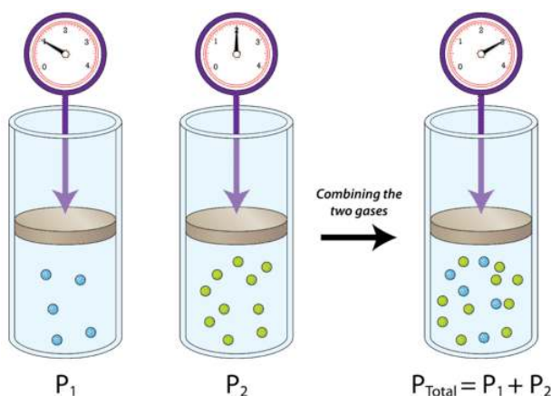
Figure 12.10.1: Dalton's Law states that the pressure of a gas mixture is equal to the partial pressures of the combining gases.
