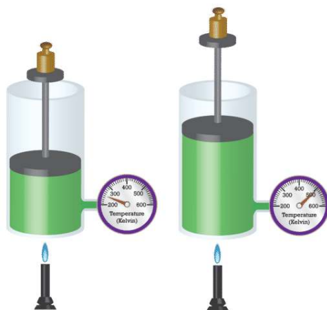
Figure 12.6.1: As a container of confined gas is heated, its molecules increase in kinetic energy and push the movable piston outward, resulting in an increase in volume.
