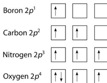
Figure 9.5.8: The 2p sublevel, for the elements boron ( Z = 5 ), carbon ( Z = 6 ), nitrogen ( Z = 7 ), and oxygen ( Z = 8 ). According to Hund's rule, as electrons are added to a set of orbitals of equal energy, one electron enters each orbital before any orbital receives a second electron.
