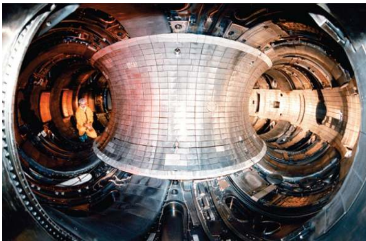
Figure 11.7.2: A Possible Design for a Nuclear Fusion Reactor. The extraordinarily high temperatures needed to initiate a nuclear fusion reaction would immediately destroy a container made of any known material. One way to avoid contact with the container walls is to use a high-energy plasma as the fuel. Because plasma is essentially a gas composed of ionized particles, it can be confined using a strong magnetic field shaped like a torus (a hollow donut).
