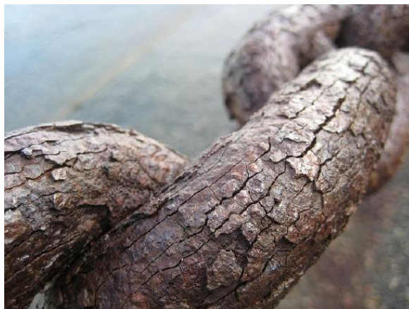
Figure 3.5.2: Heavy rust on the links of a chain near the Golden Gate Bridge in San Francisco; it was continuously exposed to moisture and salt spray, causing surface breakdown, cracking, and flaking of the metal. (CC BY-SA 3.0; Marlith).
