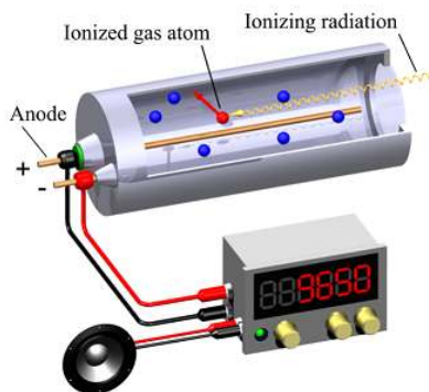
Figure 11.3.1: Schematic of a Geiger-Müller counter using an "end window" tube for low penetration radiation. A loudspeaker is also used for indication. (CC-BY-SA-3.0 Svjo-2 vai Wikipedia (opens in new window)).
