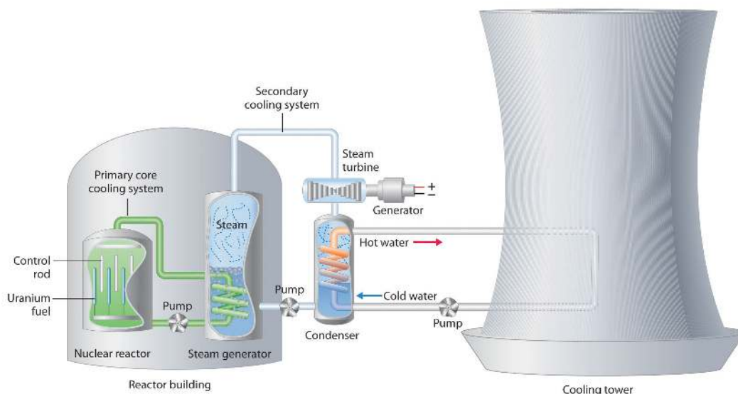
Figure 11.7.1: A Light-Water Nuclear Fission Reactor for the Production of Electric Power. The fuel rods are made of a corrosion-resistant alloy that encases the partially enriched uranium fuel; controlled fission of ^{235}\text{U} in the fuel produces heat. Water surrounds the fuel rods and moderates the kinetic energy of the neutrons, slowing them to increase the probability that they will induce fission. Control rods that contain elements such as boron, cadmium, or hafnium—which are very effective at absorbing neutrons—are used to control the rate of the fission reaction. A heat exchanger is used to boil water in a secondary cooling system, creating steam to drive the turbine and produce electricity. The large hyperbolic cooling tower, which is the most visible portion of the facility, condenses the steam in the secondary cooling circuit; it is often located at some distance from the actual reactor.
