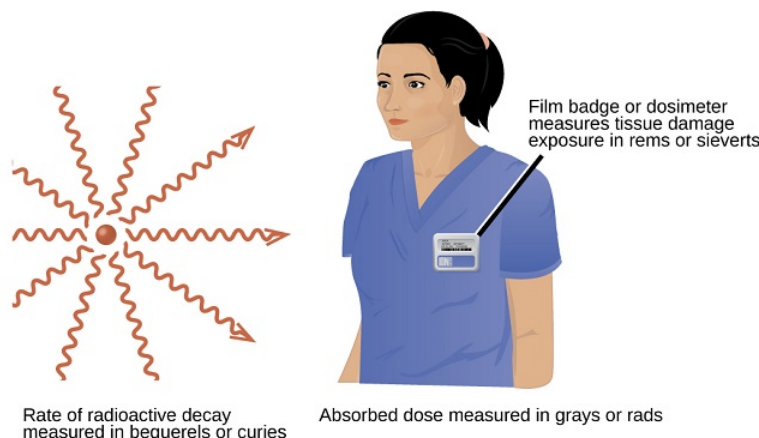
Figure 11.9.7: Different units are used to measure the rate of emission from a radioactive source, the energy that is absorbed from the source, and the amount of damage the absorbed radiation does. (CC by 4.0; OpenStax)
