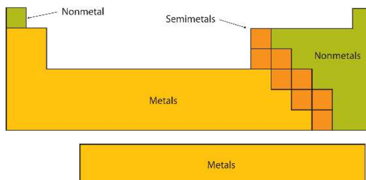
Figure 4.7.2: Types of Elements. Elements are either metals, nonmetals, or metalloids (or semi metals). Each group is located in a different part of the periodic table. (CC BY-NC-SA; Anonymous by request)
