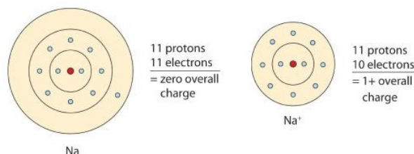
Figure 4.8.1: The Formation of a Sodium Ion. On the left, a sodium atom has 11 electrons. On the right, the sodium ion only has 10 electrons and a 1+ charge. Neutral sodium atom on left has 11 protons and 11 electrons. Sodium ion on right has 11 protons and 10 electrons, with a +1 overall charge.
