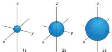
Figure 9.5.1: s orbitals have no orientational preference and resemble spheres.
