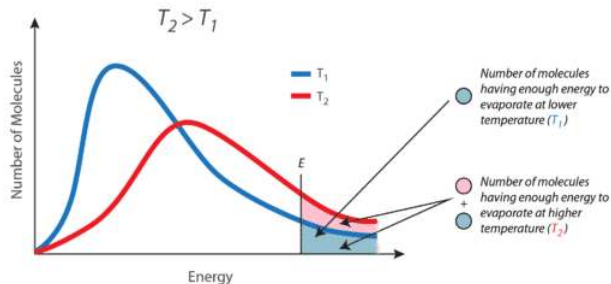
Figure 13.4.3: Kinetic energy distribution curves for a liquid at two temperatures T_1 and T_2 . The shaded area represents the molecules with enough kinetic energy to escape the liquid and become vapor.
