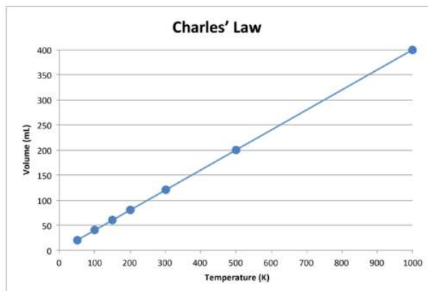
Figure 12.6.2: The volume of a gas increases as the Kelvin temperature increases.
