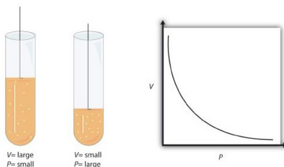
Figure 12.5.1: Boyle's Law. A piston having a certain pressure and volume (left piston) will have half the volume when its pressure is twice as much (right piston). One can also plot P versus V for a given amount of gas at a certain temperature; such a plot will look like the graph on the right.
