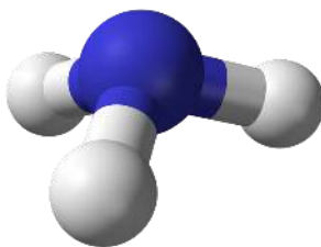
Figure 15.3.1: Ball-and-stick model of the ammonia molecule. (Public Domain; Ben Mills).
