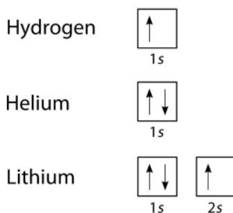
Figure 9.5.9: Orbital filling diagrams for hydrogen, helium, and lithium.
