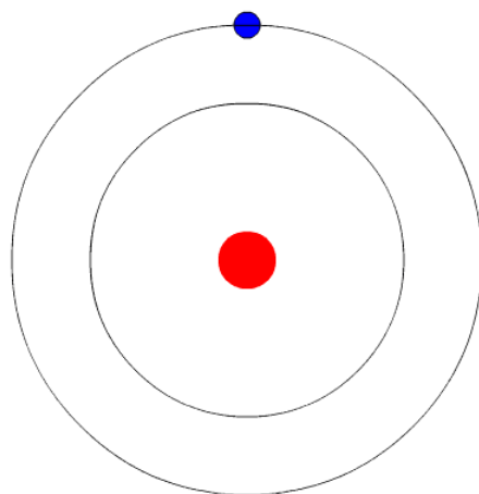
Figure 9.3.5: In Bohr's Model of the atom, electrons absorb energy to move to a higher level and release energy to move to lower levels. (CC BY-SA 3.0; Kurzon).
