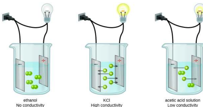
Figure 7.4.1: Solutions of nonelectrolytes, such as ethanol, do not contain dissolved ions and cannot conduct electricity. Solutions of electrolytes contain ions that permit the passage of electricity. The conductivity of an electrolyte solution is related to the strength of the electrolyte. This diagram shows three separate beakers. Each has a wire plugged into a wall outlet. In each case, the wire leads from the wall to the beaker and is split resulting in two ends. One end leads to a light bulb and continues on to a rectangle labeled with a plus sign. The other end leads to a rectangle labeled with a minus sign. The rectangles are in a solution. In the first beaker, labeled “Ethanol No Conductivity,” four pairs of linked small green spheres suspended in the solution between the rectangles. In the second beaker, labeled “K C l Strong Conductivity,” six individual green spheres, three labeled plus and three labeled minus are suspended in the solution. Each of the six spheres has an arrow extending from it pointing to the rectangle labeled with the opposite sign. In the third beaker, labeled “Acetic acid solution Weak conductivity,” two pairs of joined green spheres and two individual spheres, one labeled plus and one labeled minus are shown suspended between the two rectangles. The plus labeled sphere has an arrow pointing to the rectangle labeled minus and the minus labeled sphere has an arrow pointing to the rectangle labeled plus.
