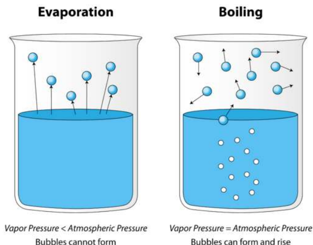
Figure 13.4.4: Comparison between evaporation and boiling.
