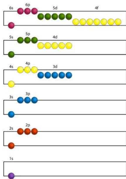
Figure 9.5.5: Electrons are added to atomic orbitals in order from low energy (bottom of the graph) to high (top of the graph) according to the Aufbau principle. Principle energy levels are color coded, while sublevels are grouped together and each circle represents an orbital capable of holding two electrons.
