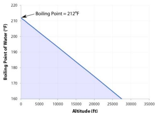
Figure 13.4.5: Influence of altitude on the boiling point of water.
