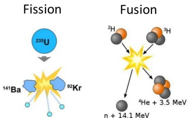
Figure 11.6.1: (left) Nuclear fission occurs when one large nucleus is split into two or more smaller nuclei. (right) Nuclear fusion happens when two small nuclei combine to make a larger nucleus.
