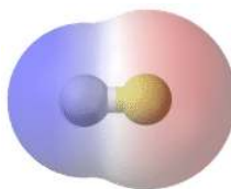
Figure 10.8.3: In the polar covalent bond of \text{HF} , the electron density is unevenly distributed. There is a higher density (red) near the fluorine atom, and a lower density (blue) near the hydrogen atom.
