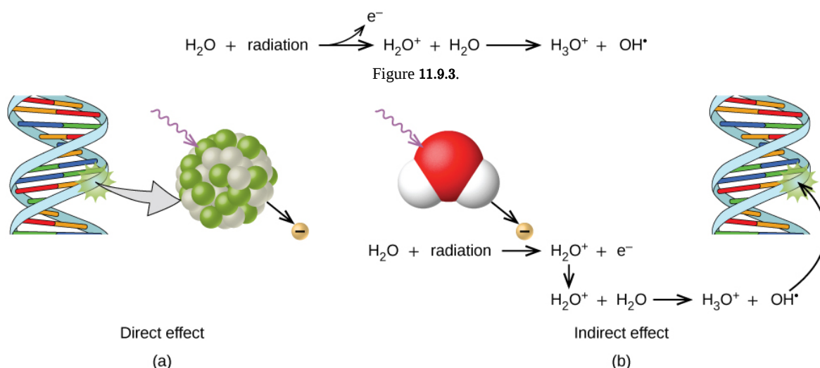
Figure 11.9.3: Ionizing radiation can (a) directly damage a biomolecule by ionizing it or breaking its bonds, or (b) create an \text{H}_2\text{O}^+ ion, which reacts with \text{H}_2\text{O} to form a hydroxyl radical, which in turn reacts with the biomolecule, causing damage indirectly.
