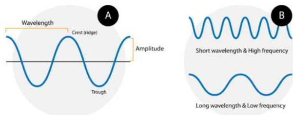
Figure 9.1.1: (A) A wave consists of alternation crests and troughs. The wavelength ( \lambda ) is defined as the distance between any two consecutive identical points on the waveform. The amplitude is the height of the wave. (B) A wave with a short wavelength (top) has a high frequency because more waves pass a given point in a certain amount of time. A wave with a longer wavelength (bottom) has a lower frequency.
