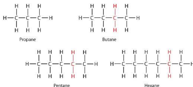
Figure 16.5.3: Members of a Homologous Series. Each succeeding formula incorporates one carbon atom and two hydrogen atoms more than the previous formula.
