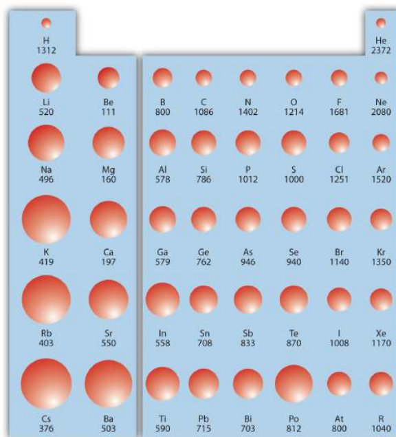
Figure 9.8.2: Ionization Energy on the Periodic Table. Values are in kJ/mol.
