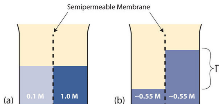
Figure 14.10.1: Osmosis. (a) Two solutions of differing concentrations are placed on either side of a semipermeable membrane. (b) When osmosis occurs, solvent molecules selectively pass through the membrane from the dilute solution to the concentrated solution, diluting it until the two concentrations are the same. The pressure exerted by the different height of the solution on the right is called the osmotic pressure. (CC BY-SA-NC 3.0; anonymous)
