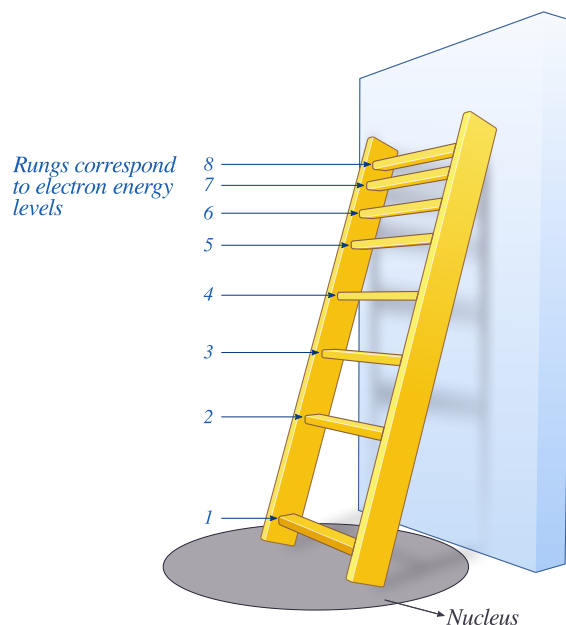
Figure 9.3.4: The energy levels of the electrons can be viewed as rungs on a ladder. Note that the spacing between rungs gets smaller at higher energies (CC BY-NC; Ümit Kaya)
