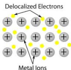
Figure 13.7.2: Metallic crystal lattice with free electrons able to move among positive metal atoms.
