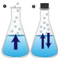
Figure 13.4.2: Evaporation (A) and condensation (B).
