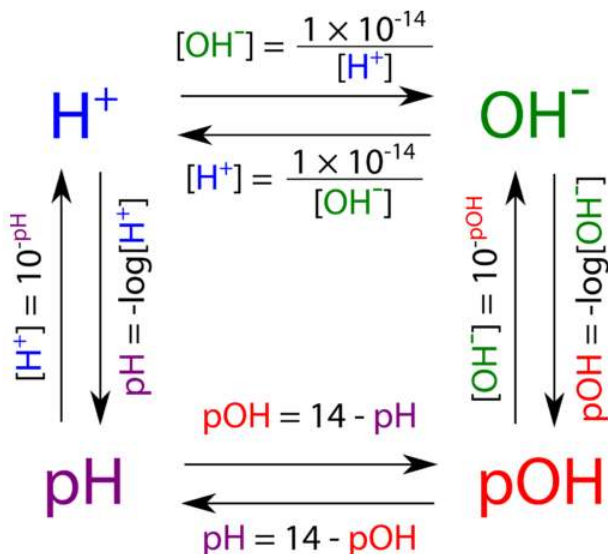
Figure 15.9.1: Relationships between hydrogen ion concentration, hydroxide ion concentration, pH and pOH.
