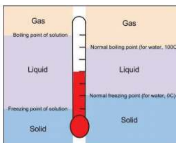
Figure 14.9.1: Comparison of boiling and freezing points of a pure liquid (right side) with a solution (left side).
