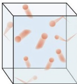
Figure 12.2.1: The Kinetic Theory of Gases. The kinetic theory of gases describes this state of matter as composed of tiny particles in constant motion with a lot of distance between the particles.
