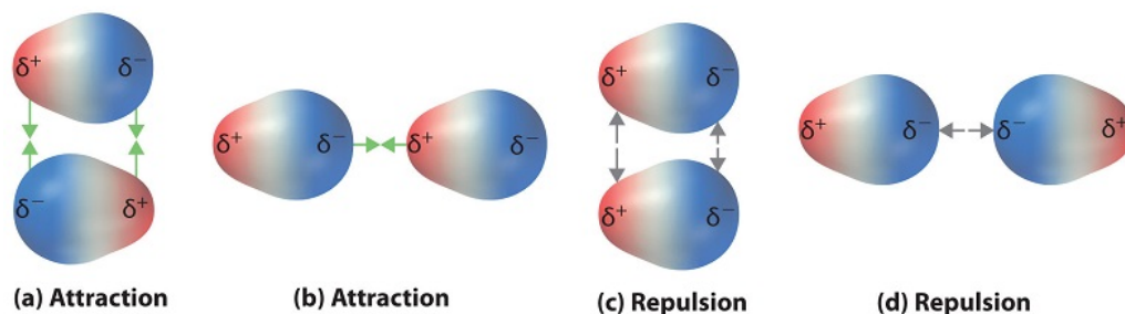
Figure 13.6.1: Attractive and Repulsive Dipole–Dipole Interactions. (a and b) Molecular orientations in which the positive end of one dipole ( \delta^+ ) is near the negative end of another ( \delta^- ) (and vice versa) produce attractive interactions. (c and d) Molecular orientations that juxtapose the positive or negative ends of the dipoles on adjacent molecules produce repulsive interactions. (CC BY-SA-NC; anonymous)
