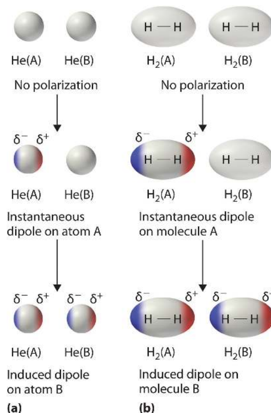
Figure 13.6.3: Instantaneous Dipole Moments. The formation of an instantaneous dipole moment on one He atom (a) or an H 2 molecule (b) results in the formation of an induced dipole on an adjacent atom or molecule.
