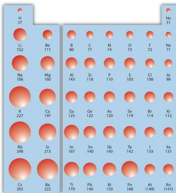
Figure 9.8.1: Atomic Radii Trends on the Periodic Table. Although there are some reversals in the trend (e.g., see Po in the bottom row), atoms generally get smaller as you go across the periodic table and larger as you go down any one column. Numbers are the radii in pm.
