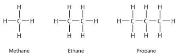
Figure 16.5.1: The Three Simplest Alkanes
