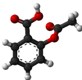
Figure 15.2.5: Ball-and-stick model of the aspirin molecule. (Public Domain; Ben Mills).
