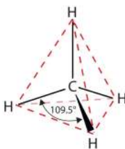
Figure 16.5.2: The Tetrahedral Methane Molecule
