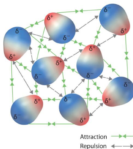
Figure 13.6.2: Both attractive and repulsive dipole–dipole interactions occur in a liquid sample with many molecules. (CC BY-SA-NC; anonymous)
