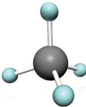
Figure 16.4.1 Three-Dimensional Representation of Methane © Thinkstock. The methane molecule is three dimensional, with the H atoms in the positions of the four corners of a tetrahedron.
