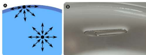
Figure 13.3.1: (A) Molecules at the surface of a liquid are pulled downwards into the liquid, creating a tightened surface. (B) Surface tension allows a paper clip to float on water's surface.
