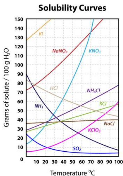
Figure 14.3.4: Solubility curves for several compounds.
