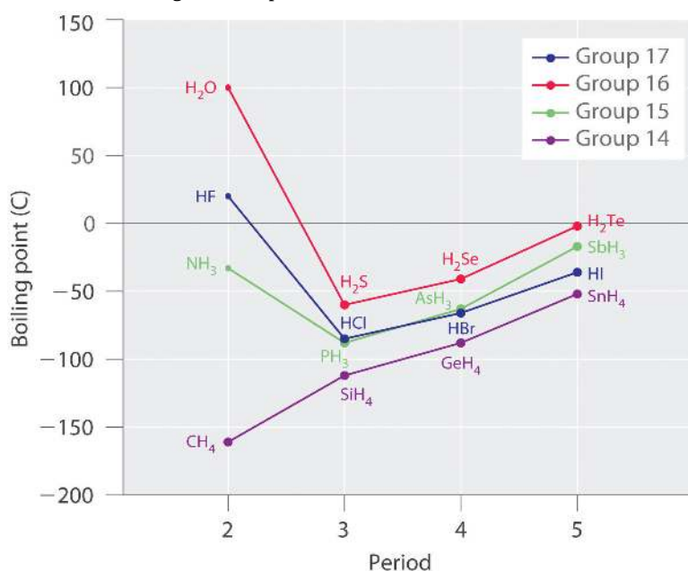
Figure 13.6.5: The Effects of Hydrogen Bonding on Boiling Points. These plots of the boiling points of the covalent hydrides of the elements of groups 14–17 show that the boiling points of the lightest members of each series for which hydrogen bonding is possible ( \text{HF} , \text{NH}_3 , and \text{H}_2\text{O} ) are anomalously high for compounds with such low molecular masses.
