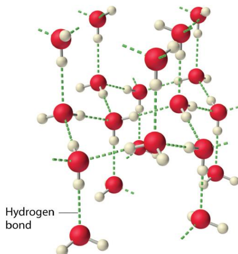
Figure 13.6.6: The Hydrogen-Bonded Structure of Ice
