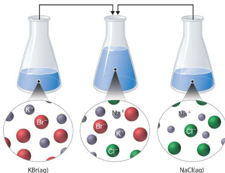
Figure 7.5.1: The Effect of Mixing Aqueous KBr and NaCl Solutions. Because no net reaction occurs, the only effect is to dilute each solution with the other. (Water molecules are omitted from molecular views of the solutions for clarity.)
