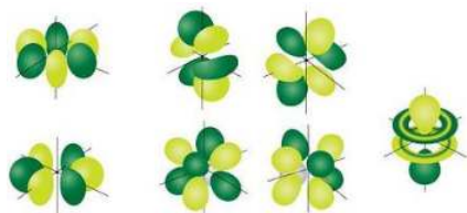
Figure 9.5.4: f orbitals have an orientational preference and exhibit quite complex structures.
