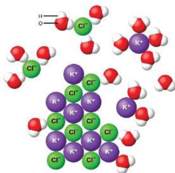
Figure 7.4.2: As potassium chloride (KCl) dissolves in water, the ions are hydrated. The polar water molecules are attracted by the charges on the K^+ and Cl^- ions. Water molecules in front of and behind the ions are not shown. The diagram shows eight purple spheres labeled K superscript plus and eight green spheres labeled Cl superscript minus mixed and touching near the center of the diagram. Outside of this cluster of spheres are seventeen clusters of three spheres, which include one red and two white spheres. A red sphere in one of these clusters is labeled O. A white sphere is labeled H. Two of the green Cl superscript minus spheres are surrounded by three of the red and white clusters, with the red spheres closer to the green spheres than the white spheres. One of the K superscript plus purple spheres is surrounded by four of the red and white clusters. The white spheres of these clusters are closest to the purple spheres.
