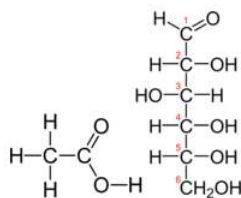
Figure 6.9.2: Acetic acid (left) has a molecular formula of \text{C}_2\text{H}_4\text{O}_2 , while glucose (right) has a molecular formula of \text{C}_6\text{H}_{12}\text{O}_6 . Both have the empirical formula \text{CH}_2\text{O} .
