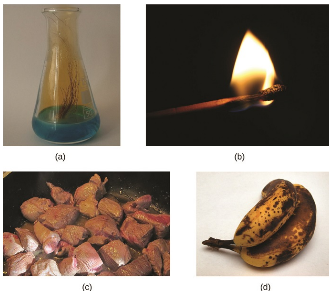
Figure 7.1.1: (a) Copper and nitric acid undergo a chemical change to form copper nitrate and brown, gaseous nitrogen dioxide. (b) During the combustion of a match, cellulose in the match and oxygen from the air undergo a chemical change to form carbon dioxide and water vapor. (c) Cooking red meat causes a number of chemical changes, including the oxidation of iron in myoglobin that results in the familiar red-to-brown color change. (d) A banana turning brown is a chemical change as new, darker (and less tasty) substances form. (Credit b: modification of work by Jeff Turner; credit c: modification of work by Gloria Cabada-Leman; credit d: modification of work by Roberto Verzo.)
