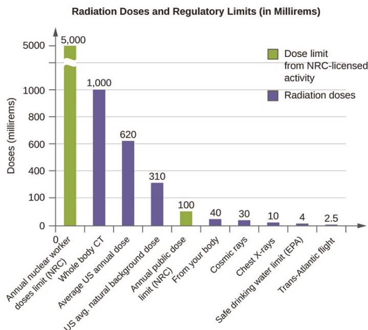
Figure 11.9.8: The total annual radiation exposure for a person in the US is about 620 mrem. The various sources and their relative amounts are shown in this bar graph. (source: U.S. Nuclear Regulatory Commission).
