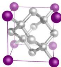
Figure 13.7.3: Diamond is a network solid and consists of carbon atoms covalently bonded to one another in a repeating three-dimensional pattern. Each carbon atom makes for single covalent bonds in a tetrahedral geometry.
