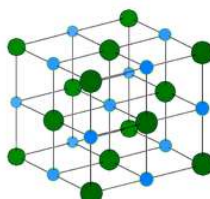
Figure 13.7.1: NaCl crystal.
