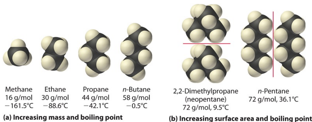
Figure 13.6.4: Mass and Surface Area Affect the Strength of London Dispersion Forces. (a) In this series of four simple alkanes, larger molecules have stronger London forces between them than smaller molecules do, and consequently have higher boiling points. (b) Linear n -pentane molecules have a larger surface area and stronger intermolecular forces than spherical neopentane molecules. As a result, neopentane is a gas at room temperature, whereas n -pentane is a volatile liquid.
