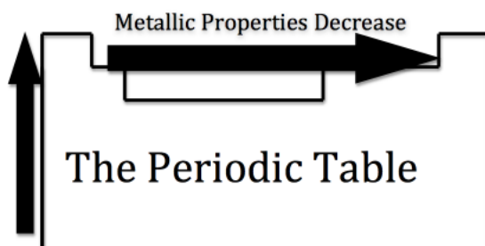
Figure 9.8.4: Courtesy of Jessica Thornton (UCD)
