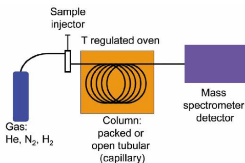
Gas chromatography-mass spectrometry (GC-MS) schematic
