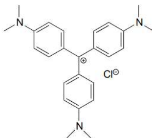
crystal violet
