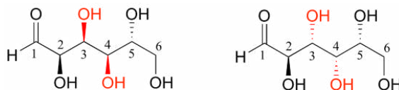
D-glucose
