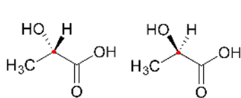
lactic acid
