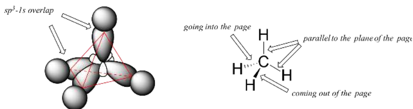
tetrahedral sp^3 bonding in methane
