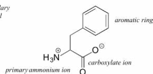
phenylalanine
