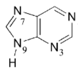
purine
