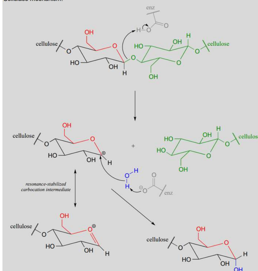
Cellulase mechanism:
