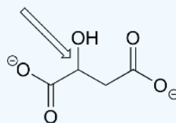
( R )-malate
