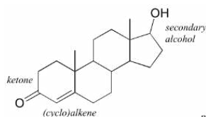
testosterone
