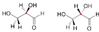
glyceraldehyde
