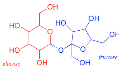
sucrose
