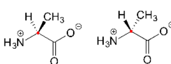
alanine
