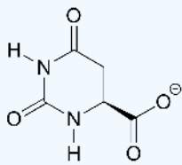
dihydroorotate
