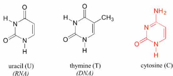
pyrimidine bases
