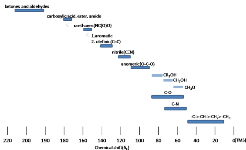
^{13}\text{C} Chemical shift range for organic compounds
