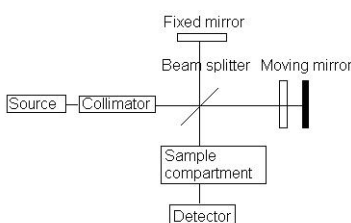
Figure 4.3.2. Block diagram of an FTIR spectrometer
