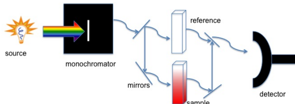
Figure 3.5.2 Illustration of a double beam UV-vis instrument.
