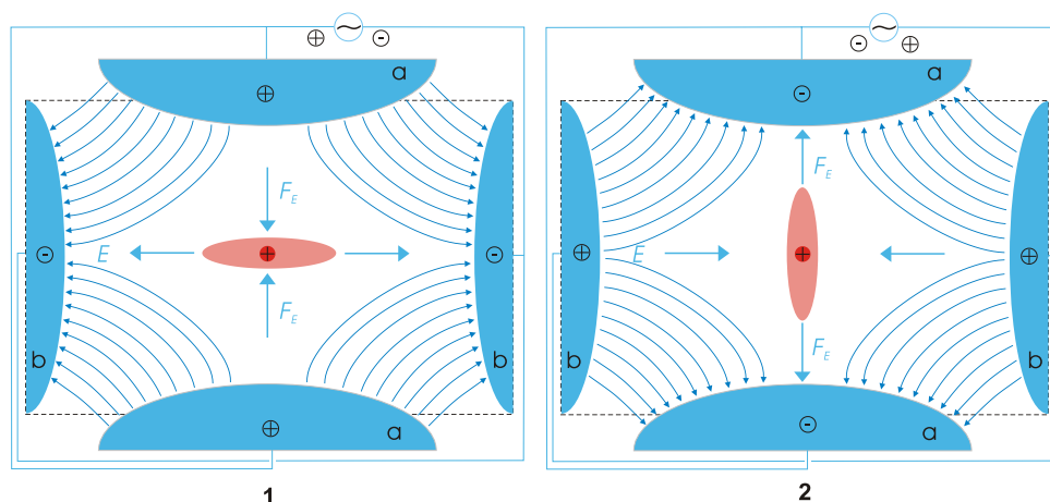
Scheme of a Quadrupole ion trap of classical setup with a particle of positive charge (dark red), surrounded by a cloud of similarly charged particles (light red). The electric field E (blue) is generated by a quadrupole of endcaps (a, positive) and a ring electrode (b). Picture 1 and 2 show two states during an AC cycle. (CC BY 2.5; Arian Kriesch Akriesch via Wikipedia ).
