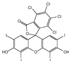
Figure 3.5.4 The molecular structure of Rose Bengal (4,5,6,7-tetrachloro-2',4',5',7'-tetraiodofluorescein).
