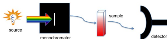
Figure 3.5.1 Illustration of a single beam UV-vis instrument.
