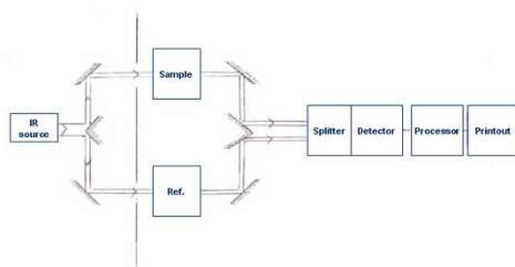
Figure 4.3.1. Simplified representation of a dispersive IR spectrometer.
