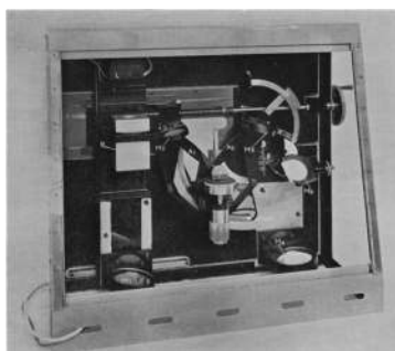
Figure 4.3.5 The first ATR Infrared Spectrometer designed by Jacques Fahrenfort featuring a hemicylindrical ATR crystal. Reproduced from J. Fahrenfort, Spectrochim. Acta , 1961, 17 , 698. Copyright: Elsevier (1961).
