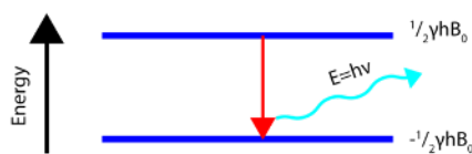
Figure 5.2.5: The process of relaxation
