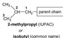
Figure 2.2j 2-methylpropyl or isobutyl
