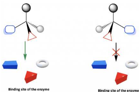
Figure 5.4g Binding site of the enzyme
