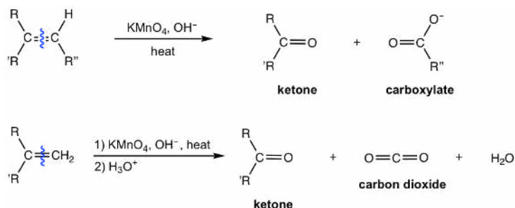
Figure 10.7g Cleavage with Potassium Permanganate \text{KMnO}_4
