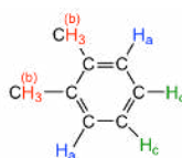
1,2-dimethylbenzene
