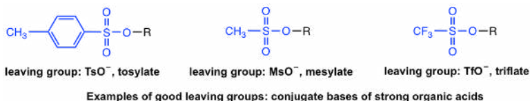
Figure 7.3a Examples of good leaving groups: Conjugate bases of strong organic acids
