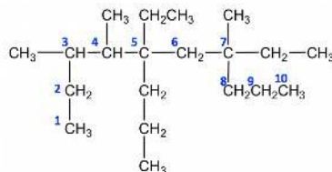
5,7-diethyl-3,4,7-trimethyl-5-propyldecane
