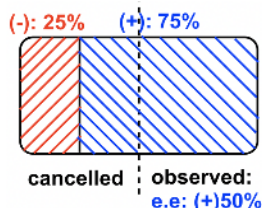
Figure 5.4e Cancelled & observed
