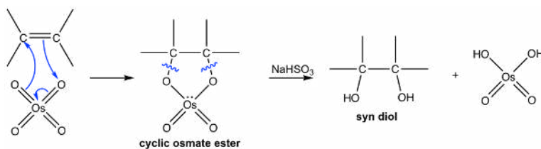
Figure 10.7c 1,2-dihydroxylation mechanism
