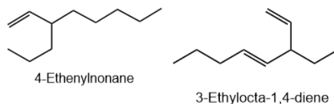
Figure 2.2n 4-Ethenynonane & 3-ethylocta-1,4-diene
