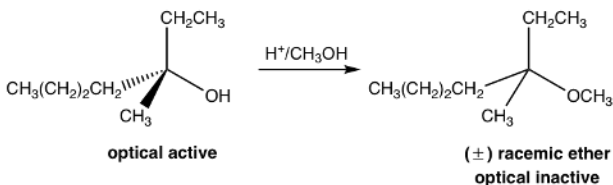
Figure 7.6e Reaction
