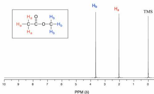
Fig. 6.6d The ^1H NMR spectrum of methyl acetate with signals assignment
