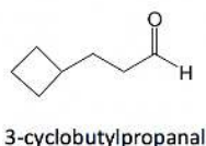
Figure 2.2o 3-cyclobutylpropanal
