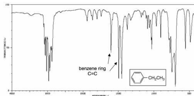
Figure 6.4e IR Spectrum of ethyl benzene
