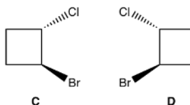
trans -1-bromo-2-chlorocyclobutane:
