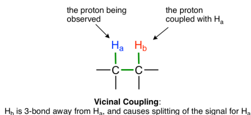
Figure 6.7c Vicinal Coupling
