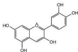
Cyanidin: an anthocyanin in reddish color
