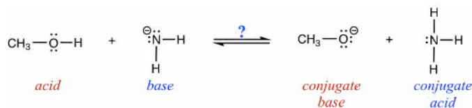
Figure 3.3b Acid-Base Reaction
