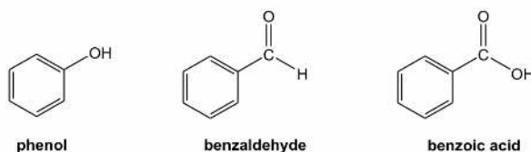
Figure 2.4b Phenol, benzaldehyde, benzoic acid
