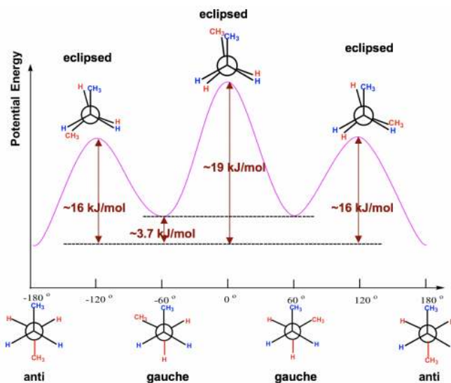
Figure 4.1l Potential Energy of Butane vs the Angle of Rotation about the C2-C3 bond
