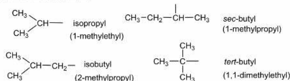
Figure 2.2b Branched alkyl groups
