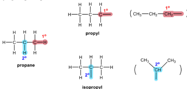
Figure 2.2g The primary and secondary hydrogen of propane
