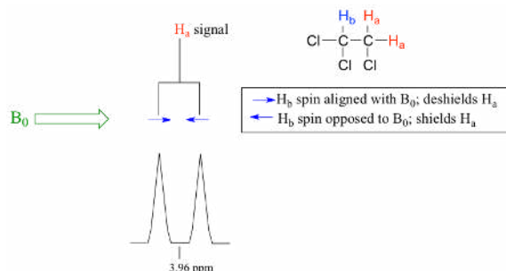
Figure 6.7d 1,1,2-trichloromethane
