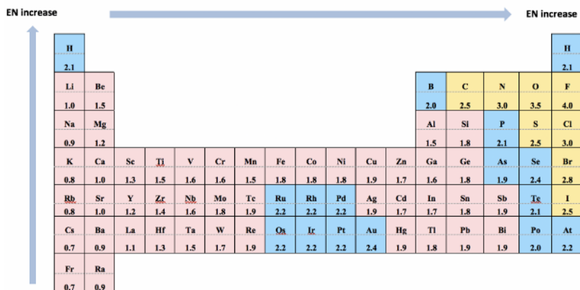
Figure 1.1b Electronegativity Values in Pauling Scale
