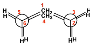
Figure 4.3b Newman projection of boat conformation
