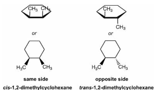
Figure 4.4c cis-1,2-dimethylcyclohexane (same side) & trans-1,2-dimethylcyclohexane (opposite side)
