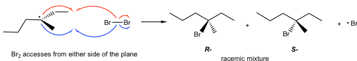
Figure 9.5b Propagation steps
