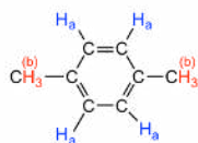
1,4-dimethylbenzene
