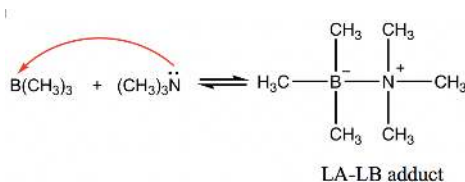
Figure 3.5b LA-LB adduct
