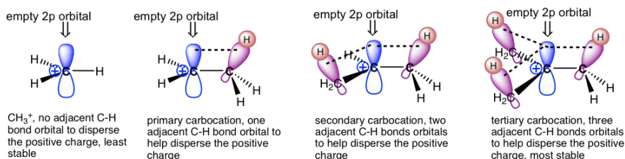
Figure 7.4d Hyperconjugation effect
