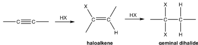
Figure 10.8l Haloalkene and geminal dihalide
