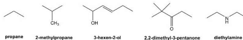
Examples of Short-line Structures
