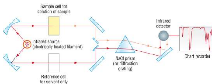
Fig. 6.2b Diagram of the IR Spectrometer
