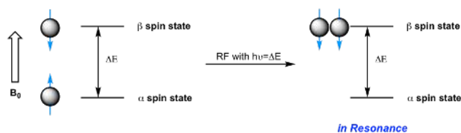
Figure 6.5c Resonance
