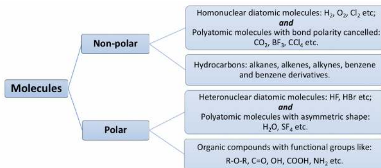
Figure 2.6g Summary of Molecular Polarities
