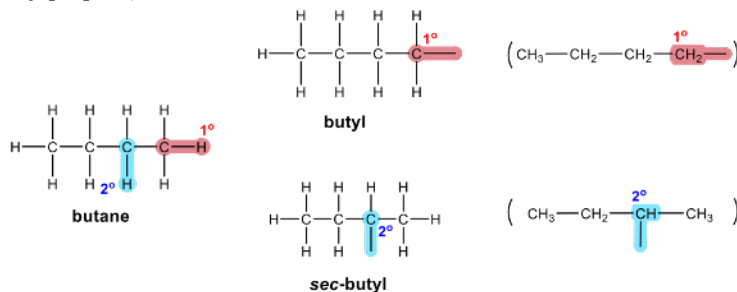
Figure 2.2h The primary and secondary hydrogen of butane
