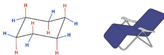
Chair conformation of cyclohexane
