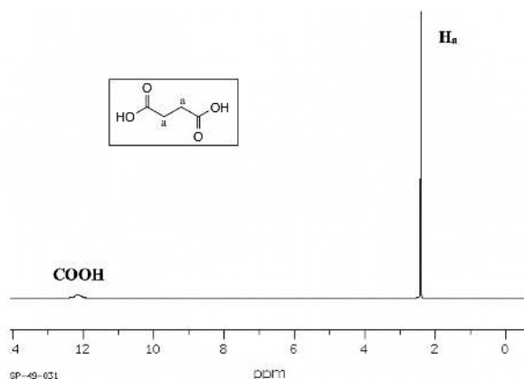
Figure 6.7f ^1\text{H} NMR spectrum of succinic acid
