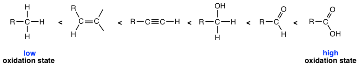
Figure 10.7a The relative oxidation state of some common organic functional groups
