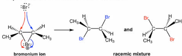
Figure 10.4d Mechanism: addition of Br 2 to (Z)-2-butene
