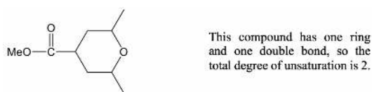
Figure 2.5b Total degree of unsaturation is 2
