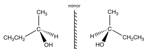
the two enantiomers of 2-butanol
