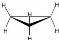
Figure 4.2d Cyclopropane
