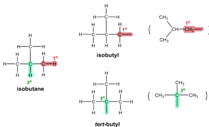
Figure 2.2i The primary and tertiary hydrogen of isobutane
