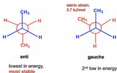
Figure 4.1j Anti and gauche conformations
