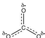
Figure 1.3c Dashed lines drawn on the CO 3 molecule Lewis structure to show the actual structure and partial charges
