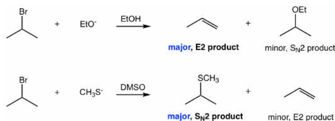
Figure 8.4b Reactions for secondary substrates
