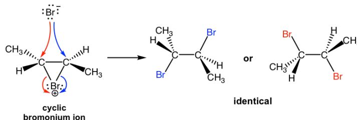
Figure 10.4c Mechanism: addition of Br 2 to E -2-butene
