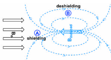
Anisotropy effect of the induced magnetic field B_{induced}
