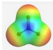
Figure 1.2d The electrostatic potential map of carbonate anion
