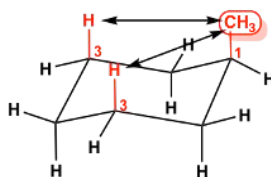
Figure 4.4b 1,3-diaxial interaction
