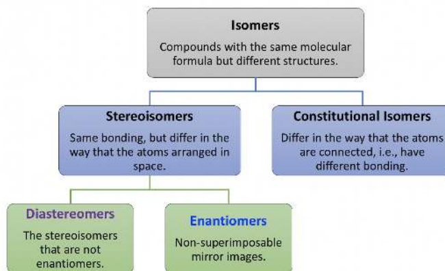
Figure 5.6a Updated Summarization of isomers
