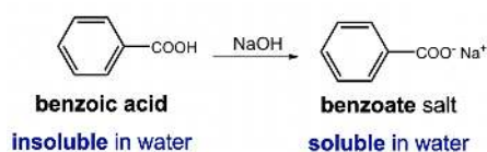
Figure 2.6i Convert insoluble organic compound to the soluble salt derivative
