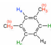
1,3-dimethylbenzene
