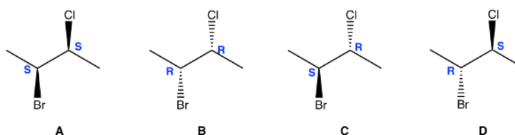
Four stereoisomers of 2-bromo-3-chlorobutane in perspective formula
