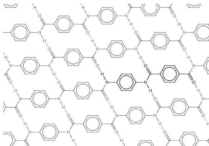
Figure 1.5.7: The diagram shows the polymer structure of Kevlar, with hydrogen bonds between polymer chains represented by dotted lines.
