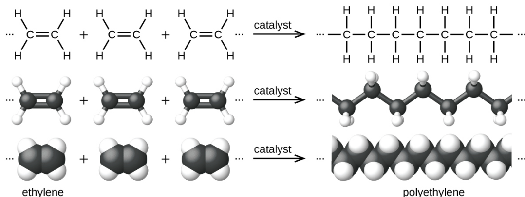
Figure 1.2.7: The reaction for the polymerization of ethylene to polyethylene is shown.
