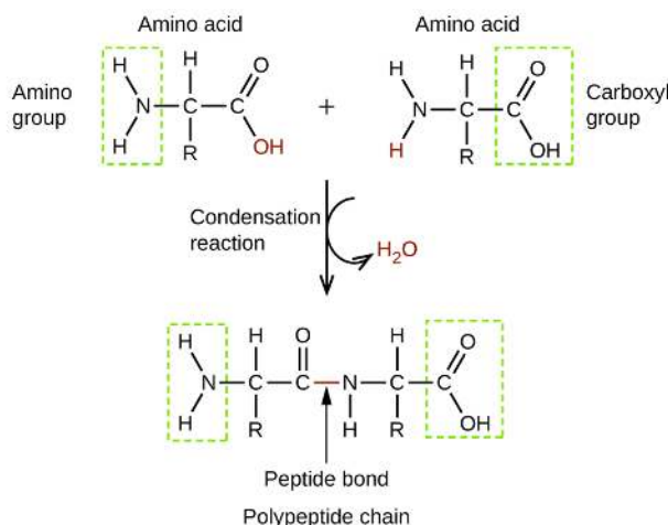
Figure 1.5.4: This condensation reaction forms a dipeptide from two amino acids and leads to the formation of water.
