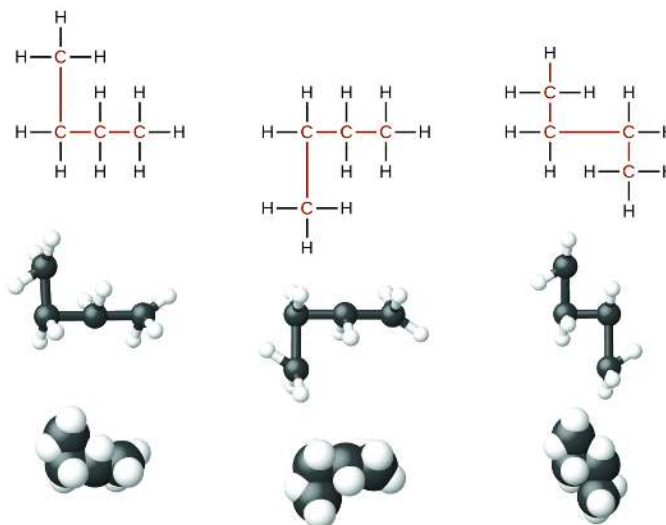
Figure 1.2.3: These three representations of the structure of n -butane are not isomers because they all contain the same arrangement of atoms and bonds.
