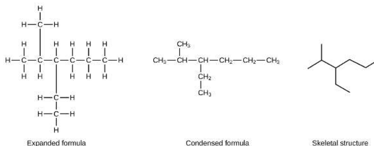
Figure 1.2.2: The same structure can be represented three different ways: an expanded formula, a condensed formula, and a skeletal structure.
