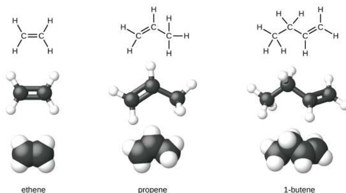
Figure 1.2.6: Expanded structures, ball-and-stick structures, and space-filling models for the alkenes ethene, propene, and 1-butene are shown.
