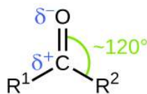
Figure 1.4.1: The carbonyl group is polar, and the geometry of the bonds around the central carbon is trigonal planar.
