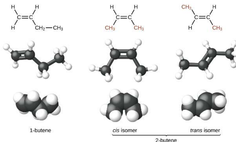
Figure 1.2.9: These molecular models show the structural and geometric isomers of butene.
