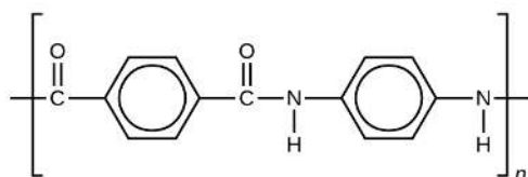
Figure 1.5.6: This illustration shows the formula for polymeric Kevlar.
