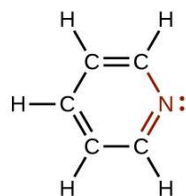
Figure 1.5.1: The illustration shows one of the resonance structures of pyridine.
