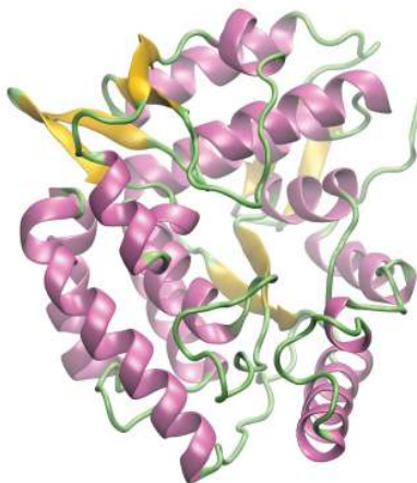
Figure 1.5.5: A computer rendering shows the three-dimensional structure of the enzyme phenylalanine hydroxylase. In the disease phenylketonuria, a defect in the shape of phenylalanine hydroxylase causes it to lose its function in breaking down phenylalanine.
