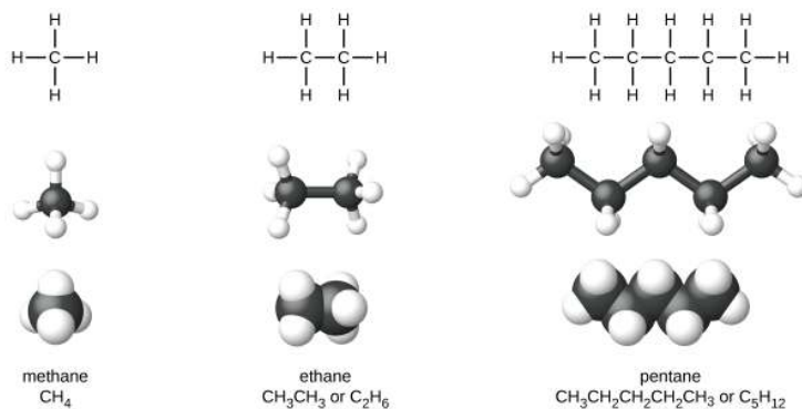
Figure 1.2.1: Pictured are the Lewis structures, ball-and-stick models, and space-filling models for molecules of methane, ethane, and pentane.
