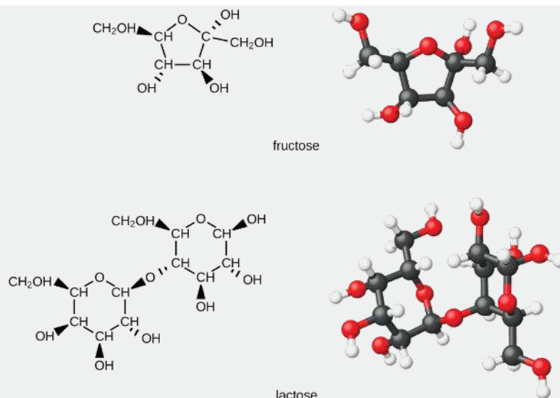
Figure 1.3.1: The illustrations show the molecular structures of fructose, a five-carbon monosaccharide, and of lactose, a disaccharide composed of two isomeric, six-carbon sugars.
