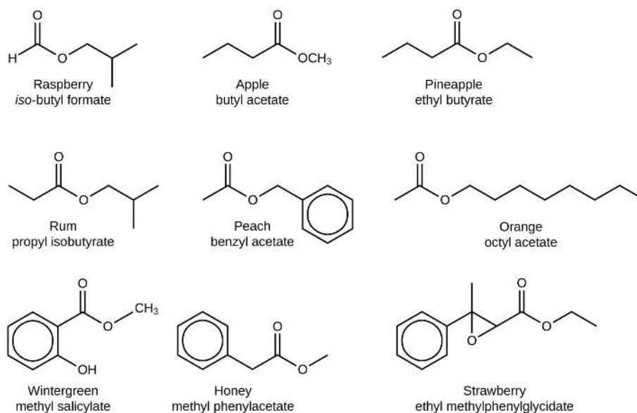
Figure 1.4.2: Esters are responsible for the odors associated with various plants and their fruits.
