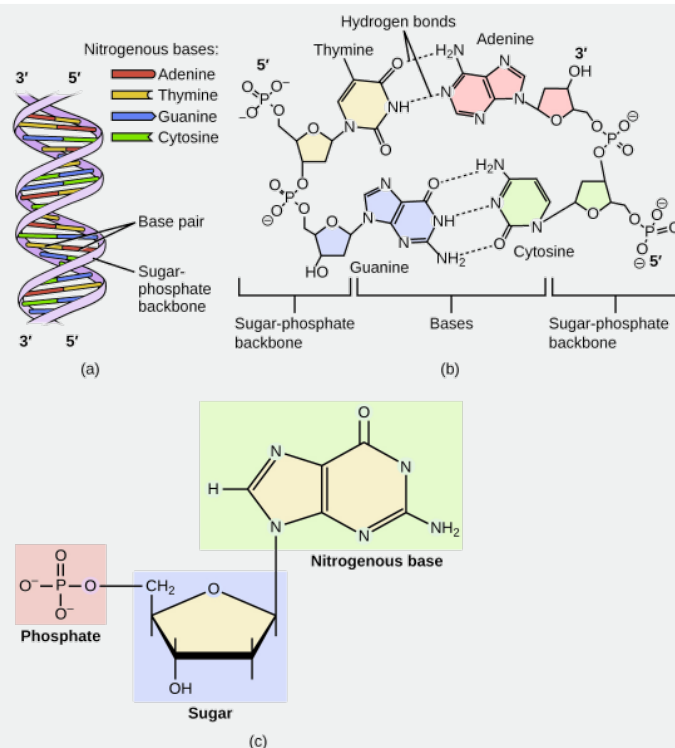
Figure 1.5.2: DNA is an organic molecule and the genetic material for all living organisms. (a) DNA is a double helix consisting of two single DNA strands hydrogen bonded together at each nitrogenous base. (b) This detail shows the hydrogen bonding (dotted lines) between nitrogenous bases on each DNA strand and the way in which each nucleotide is joined to the next, forming a backbone of sugars and phosphate groups along each strand. (c) This detail shows the structure of one of the four nucleotides that makes up the DNA polymer. Each nucleotide consists of a nitrogenous base (a double-ring molecule, in this case), a five-carbon sugar (deoxyribose), and a phosphate group.
