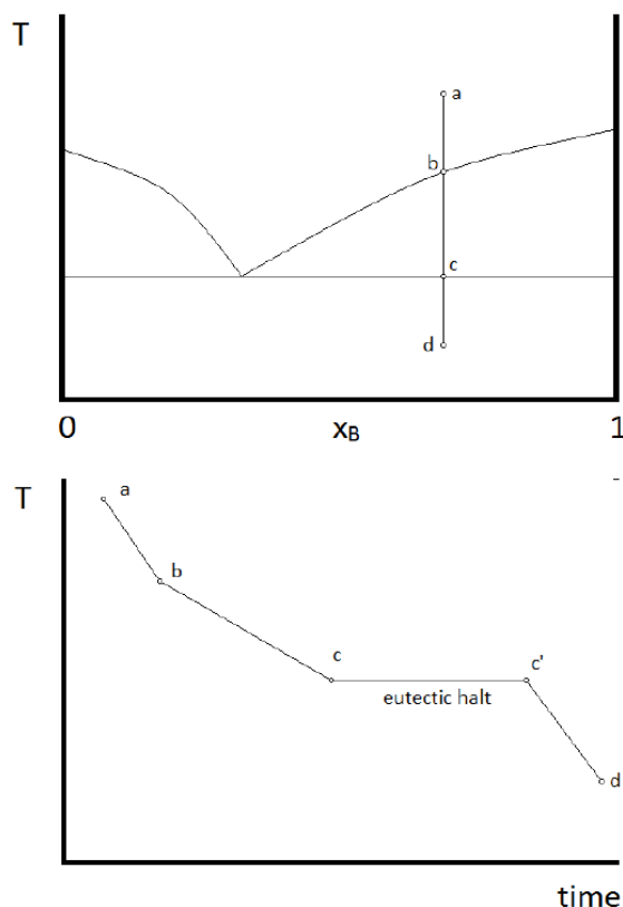
Figure 27.2.1: (A) cooling of a two-component system from liquid to solid. (B) Corresponding cooling curve for this process.
