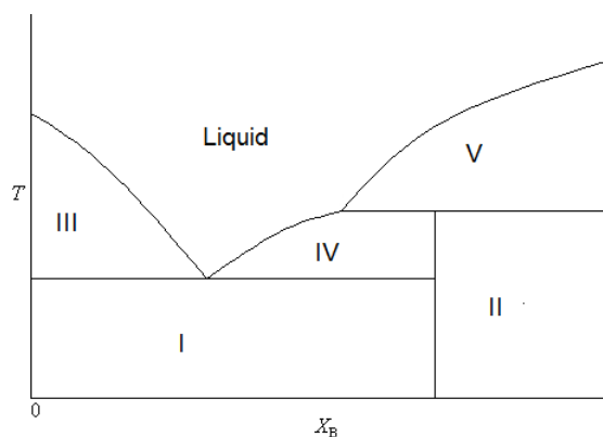
Figure 27.1.4: A phase diagram of a two-component system that exhibits incongruent melting.
