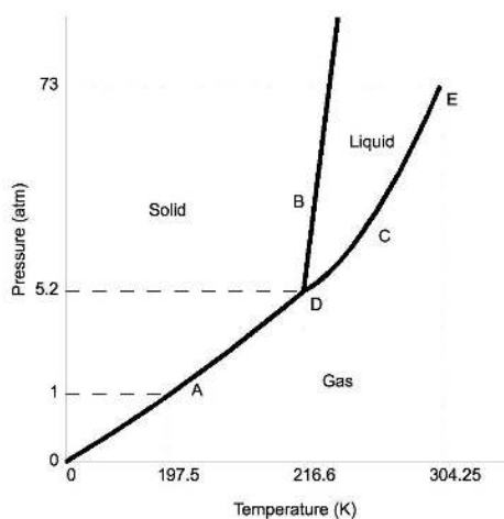
Figure 22.2.2a: Phase diagrams for CO 2
