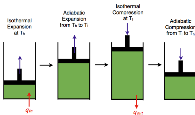
Figure 13.1.1: An ideal gas-piston model of the Carnot cycle. (CC BY 4.0; XiSen Hou via Hope College)
