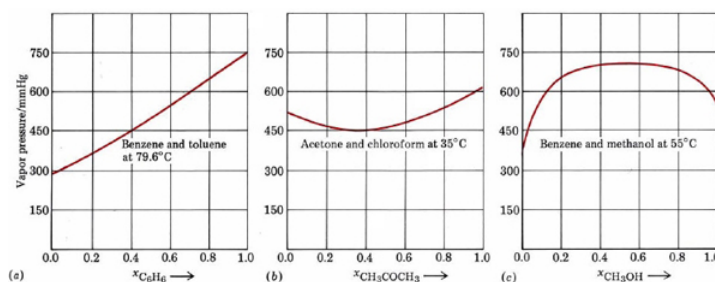
Figure 24.1.2: Deviations from Raoult's law. (a) When Raoult's law is obeyed, a plot of vapor pressure against mole fraction yields a straight line. This is nearly true for the benzene and toluene mixture at 79.6°C. (b) A mixture of acetone and chloroform shows negative deviations from Raoult's law at 35°C, indicating that the two different molecules prefer each other's company to their own. (c) The opposite behavior is shown at 55°C by a benzene-methanol mixture where the polar and nonpolar molecules prefer the company of their own kind.
