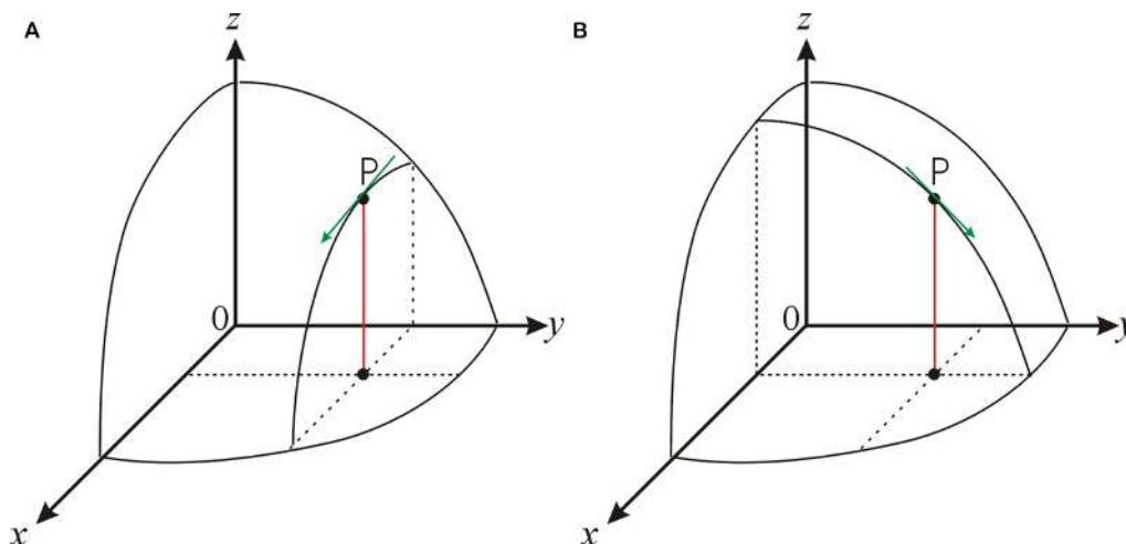
Figure 9.2.2: Geometric interpretation of a partial derivative. (CC BY-NC-SA; Marcia Levitus)
