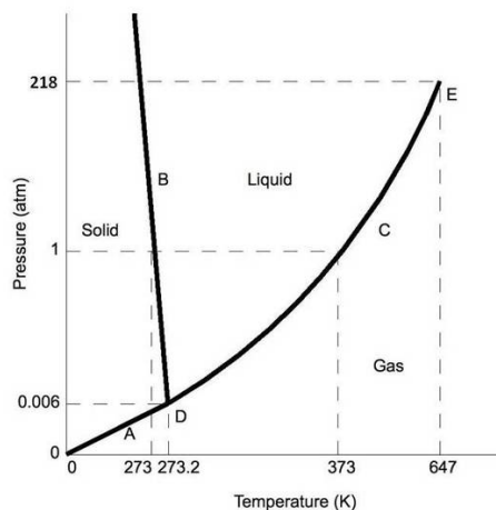
Figure 22.2.2b: Phase diagrams for H 2 O
