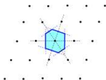
Figure 1 Wigner-Seitz cell. Shaded: domain of influence.
