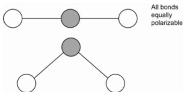
Figure 5.3: Representation of the Raman inactive bending vibration of carbon dioxide.
