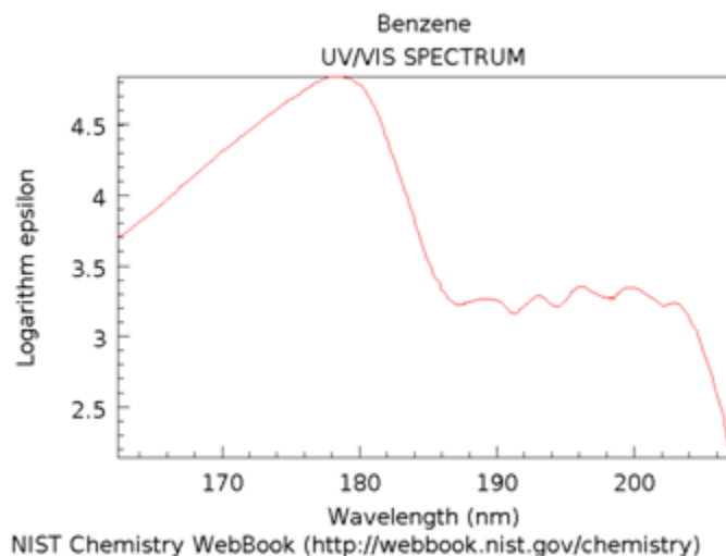
Figure 2.3.18. Ultraviolet absorption spectrum of benzene.
