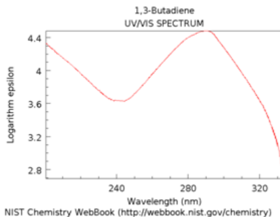
Figure 2.2.15. Ultraviolet absorption spectrum of 1,3-butadiene.
