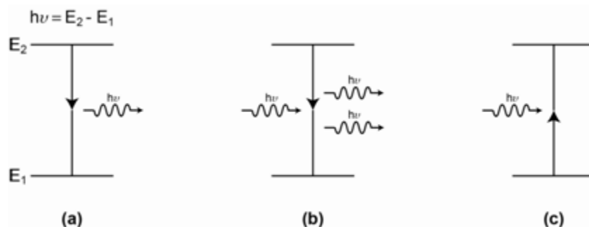
Figure 1.3A.8. Representation of (a) emission of a photon, (b) stimulated emission and (c) absorption. The waves represent photons.
