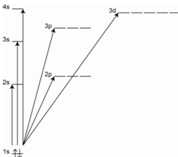
Figure 2.1.2. Absorption transitions of helium.
