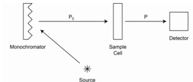
Figure 1.1.1. Block diagram of a spectrophotometer
