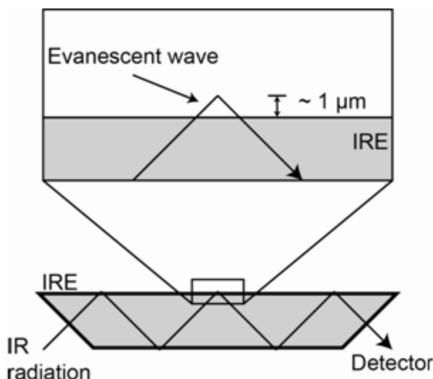
Figure 4.2.7. Representation of a device for measuring attenuated total reflectance spectra.
