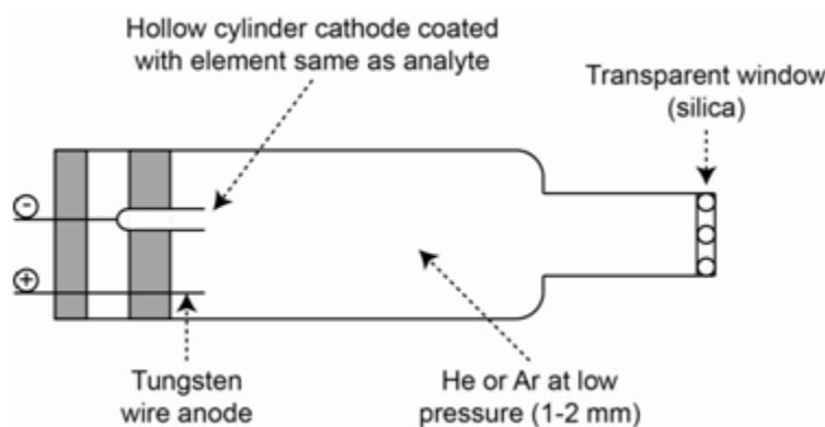
Figure 6.3A.9. Illustration of a hollow cathode lamp.
