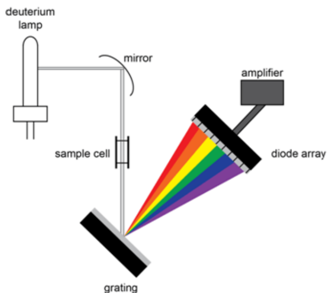
Figure 1.3C.16: Representation of a diode array detector.
