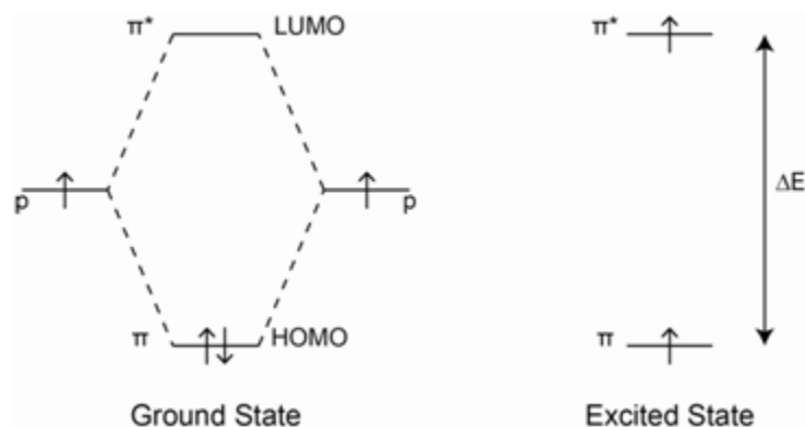
Figure 3.2.1. Energy level diagram for \pi - and \pi^* -orbitals of a typical organic compound.
