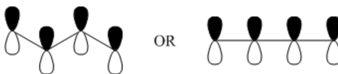
Figure 2.2.12. Representation of the four p-orbitals in 1,3-butadiene.
