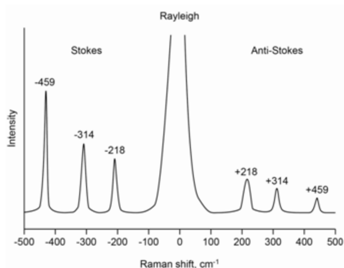
Figure 5.5: Complete Raman spectrum of carbon tetrachloride ( \text{CCl}_4 ).
