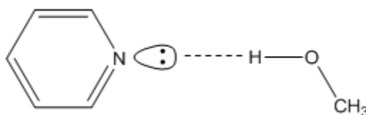
Figure 2.4.22. Hydrogen bond between methanol and pyridine.
