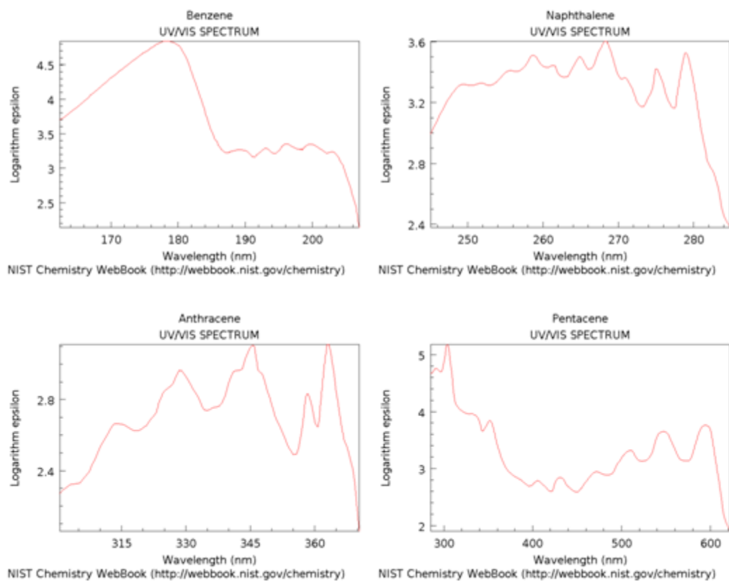
Figure 2.2.16. UV/VIS absorption spectra of benzene, naphthalene, anthracene and pentacene.
