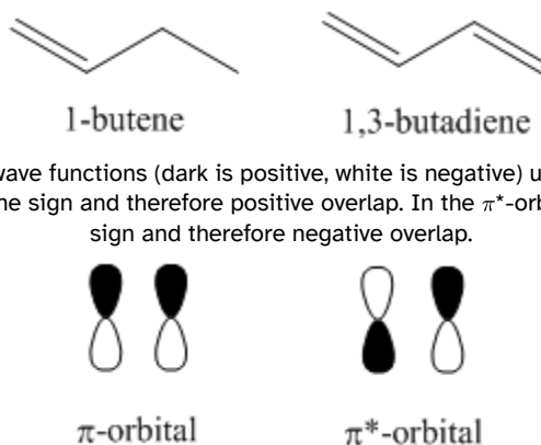
Figure 2.2.8. Representation of overlap of p-orbitals of a double bond.
