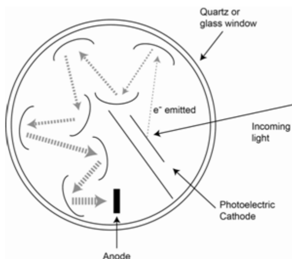
Figure 1.3C.15: Representation of a photomultiplier tube.
