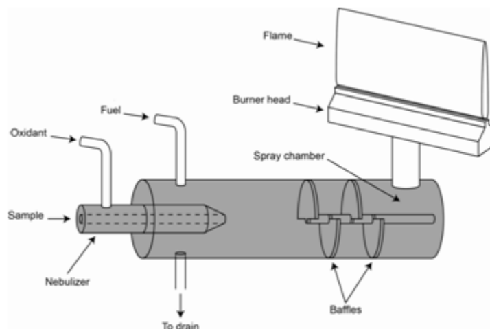
Figure 6.2A.1. Illustration of a laminar flow or pre-mix burner.
