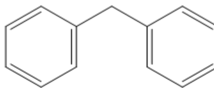
diphenylmethane
