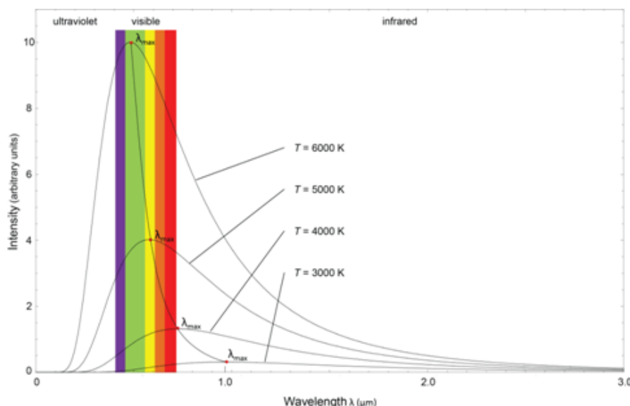
Figure 1.3A.7. Output from blackbody radiators at different temperatures.
