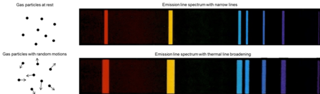
Figure 2.1.7. Effect of Doppler broadening on the emission from a gas phase atomic substance.
