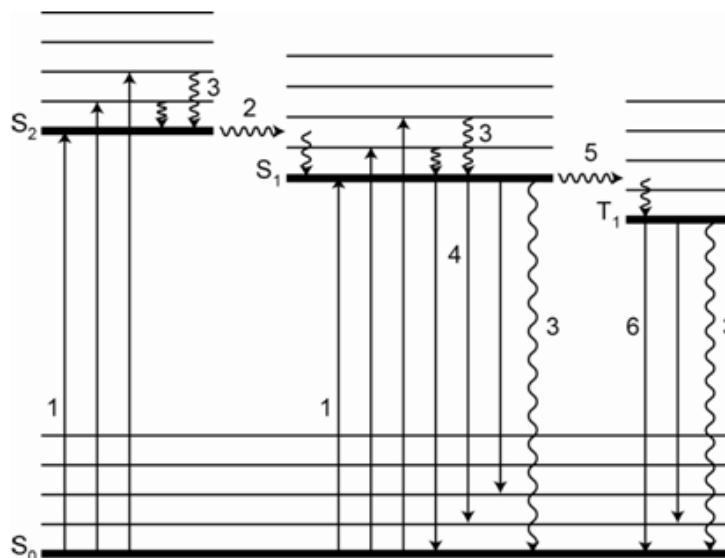
Figure 3.2.4. Energy level diagram for a molecular species.
