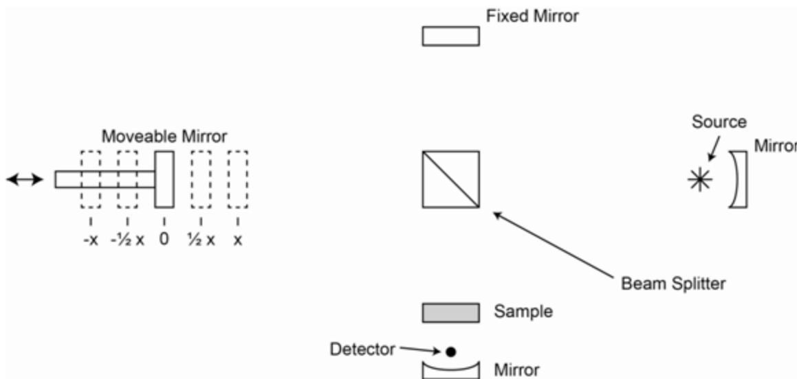
Figure 4.3.10. Diagram of a Michelson interferometer.
