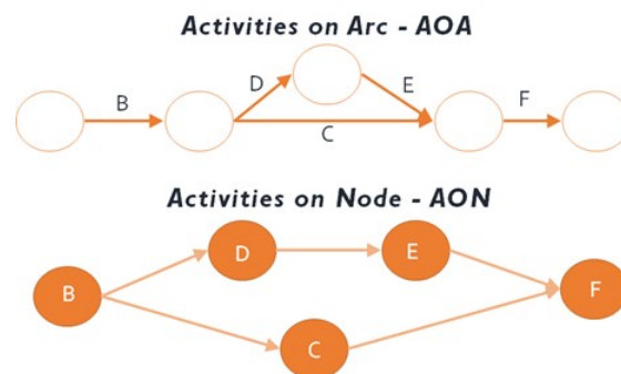
Figure 7.1: Activity Networks (either on Arc or Node)
