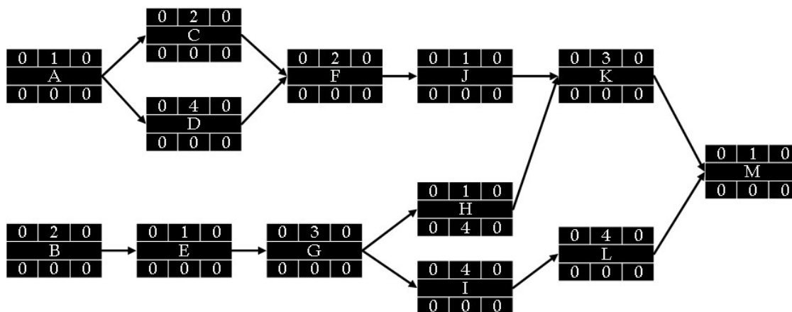
Figure 7.10: Activity Network Diagram with Durations
