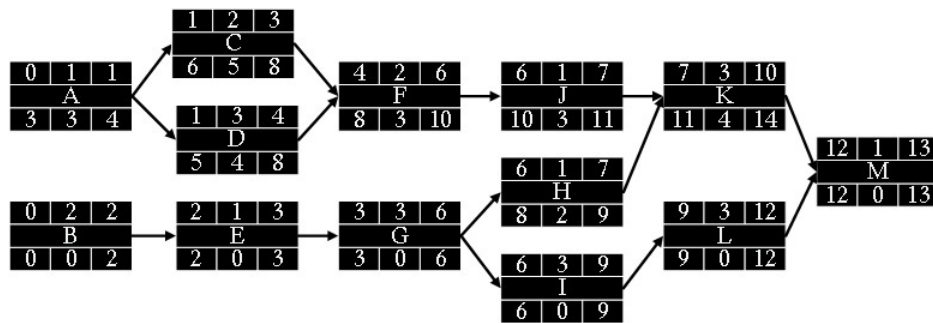
Figure 8.7: Activity Network Diagram after Crashing I and L
