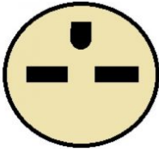
15 AMPERE, 250 VOLT, NEMA 6-15R RECEPTACLE, CAN BE USED ON 15 AMPERE MAXIMUM BRANCH CIRCUITS. STANDARD 125 VOLT PLUGS WILL NOT FIT. OFTEN USED FOR 240 VOLT WINDOW AC UNITS.
