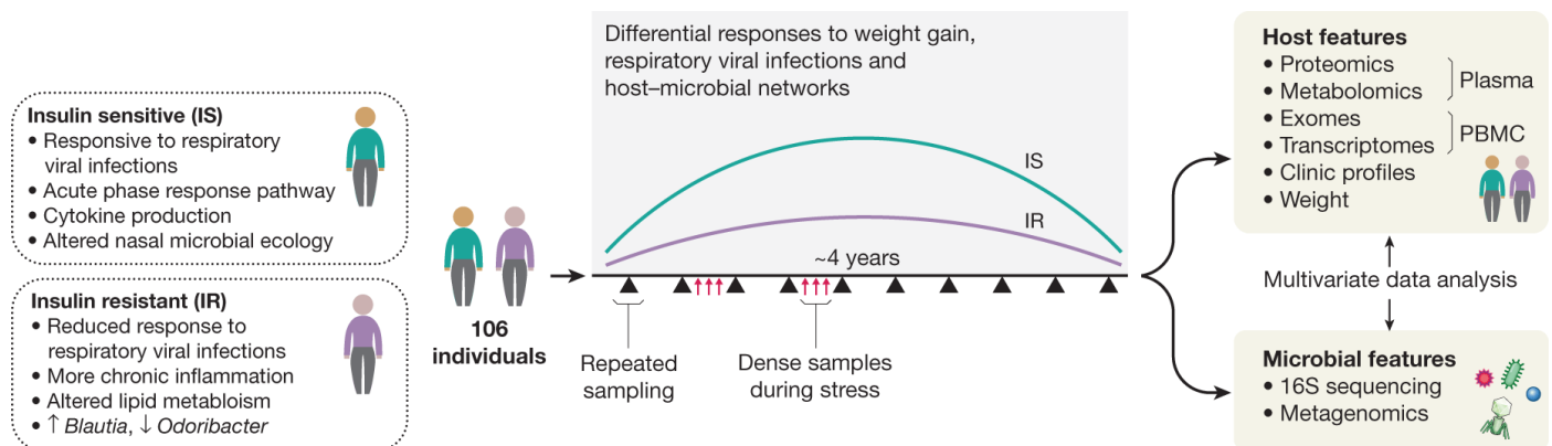
Fig. 4. Differential host and microbial responses to dietary perturbations and infectious disease in individuals with prediabetes. For integrated personal 'omics profiling of the microbiome during prediabetes, 106 participants were followed for up to four years, with samples (primarily blood and stool) collected quarterly and additional samples collected during periods of RVI and other stresses. The genomes of the participants were sequenced and measurements of transcriptomes, proteomes, metabolomes, and microbiomes taken at each visit, in addition to clinical details. Insulin-resistant individuals showed differences from insulin-sensitive participants in various measurements, both at baseline and in response to the stresses such as weight loss and RVI.
