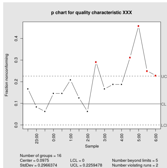
Figure 2.2.1: Example of a Statistical Process Control Chart. P Chart for Quality , by Daniel Penfield, CC BY 3.0.
