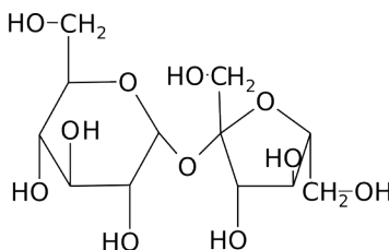
Sucrose, a disaccharide
