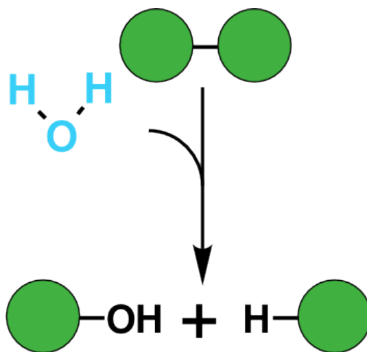
Hydrolysis reaction
