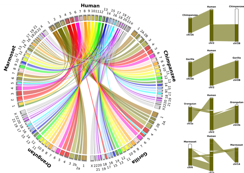
Syntenic map of Human, Chimpanzee, Gorilla, Orangutan, and Marmoset (non-ape primate). Mapping of chromosome 2a and 2b in the apes compared to 6 and 14 in the marmoset illustrates the relatedness of the chromosomal structure of the apes. Minor inversions are apparent in the orangutan chromosome.
