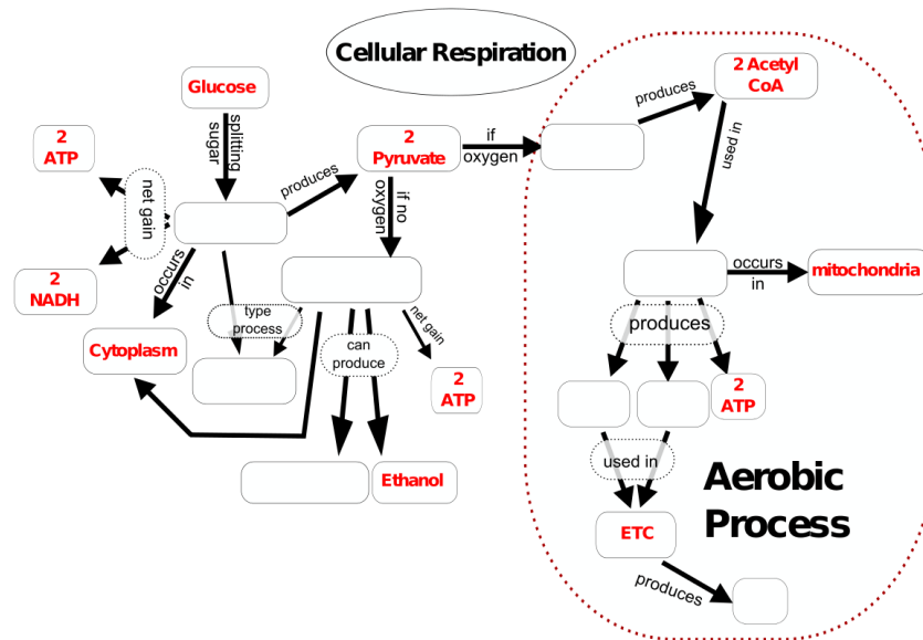
Cellular Respiration concept map.
