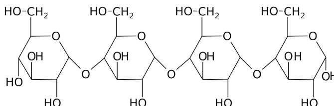
Amylose (Starch), a polysaccharide
