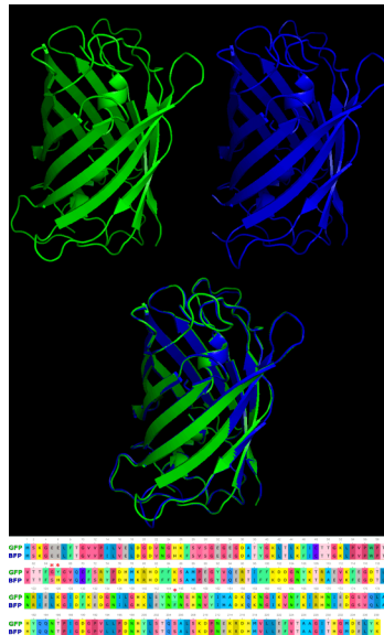
3D model of GFP (Top Left), BFP (Top Right), structural alignment of GFP and BFP (Center) and the sequence alignment (Bottom) illustrating the 3 amino acid changes to produce the alternative protein. Red asterisks indicate the location of mutations.
