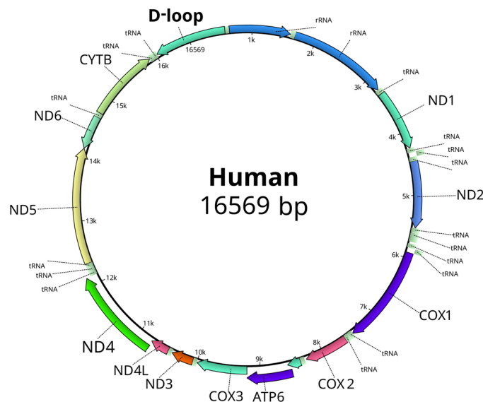
Human mitochondrial genome
