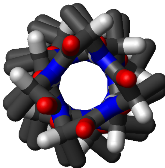
Top-down view of an \alpha -helix
