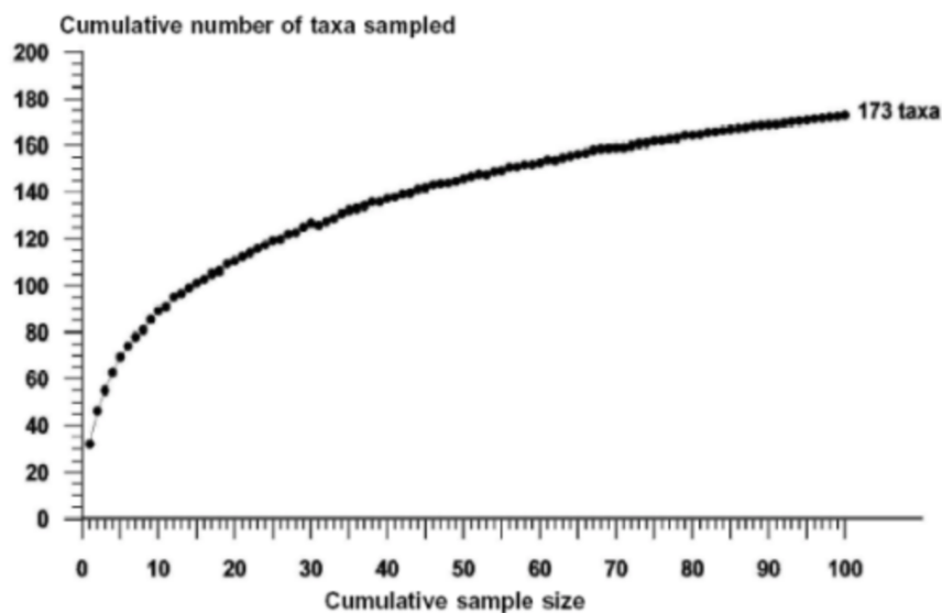
Figure 5.3.3 An example of a collectors curve. Cumulative sample size represents the number of individuals classified. The cumulative number of taxa sampled refers to the number of new species detected.
