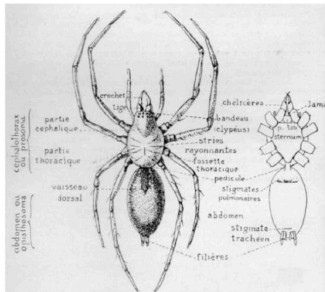
Figure 5.3.1 Basic external characteristics of spiders useful for identifying individuals to species.
