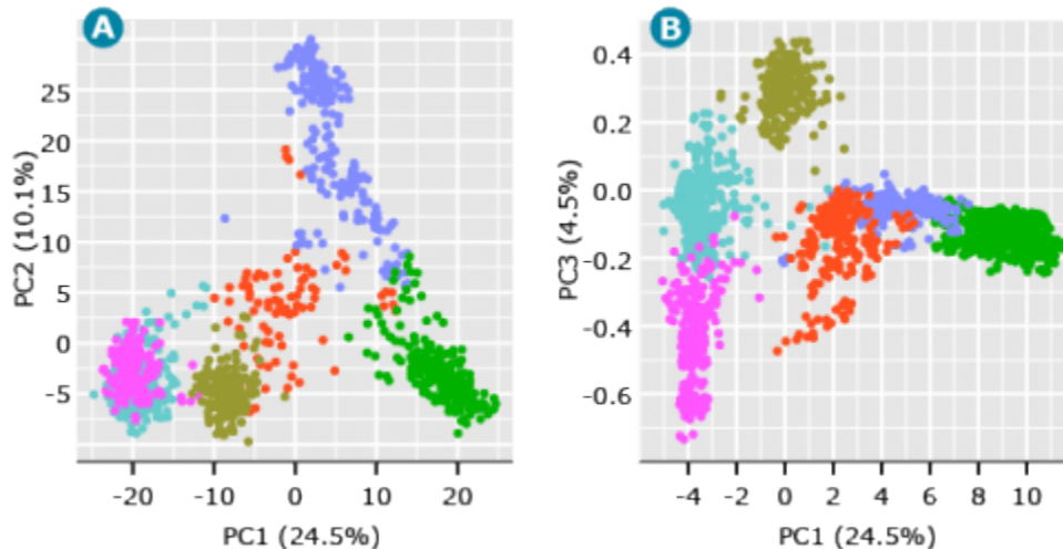
Fig. 5 PCA-produced k-means.
