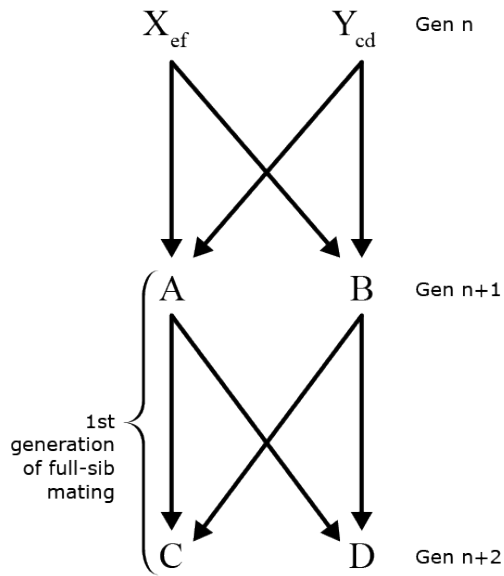
Fig. 3 Full-sib mating design.
