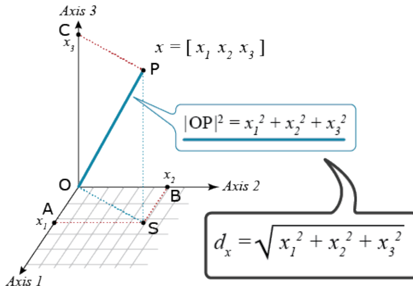
Fig. 8 Pythagoras' theorem extended into three-dimensional space.
