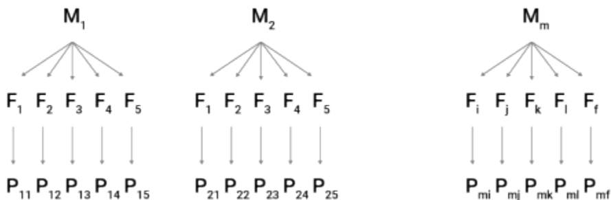
Fig. 2 North Carolina Design II (NC II), Mating Design (AB).
