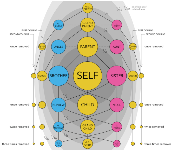
Fig. 2 Fractional relationships in the calculation of coefficients of relationships and inbreeding.
