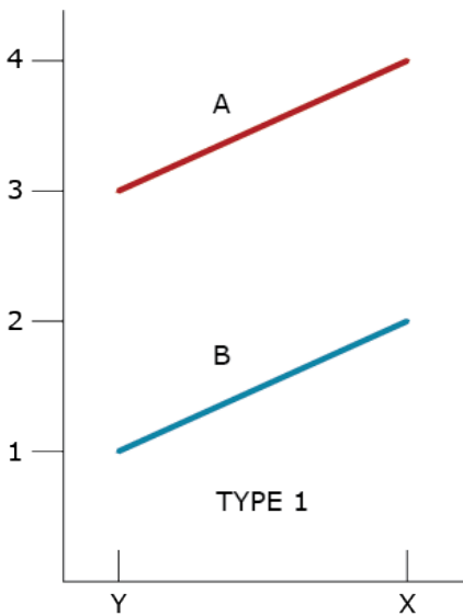
Fig. 2 No interaction type phenotype response in two environments.
