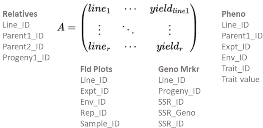
Fig. 8 A relational database for data management plant breeding research.
