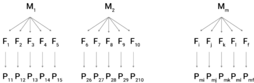
Fig. 1 North Carolina Design I (NC I), Nested Mating Design (A/B).
