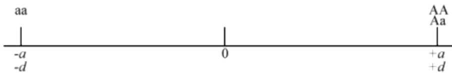
Fig. 4 Line diagrammatic representation of complete dominance of A over a allele or a over A allele.
